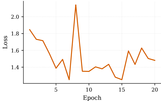
mAP@0.5:0.95
