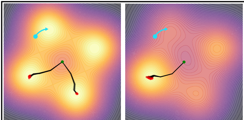
Fine-tuning Landscape #1
