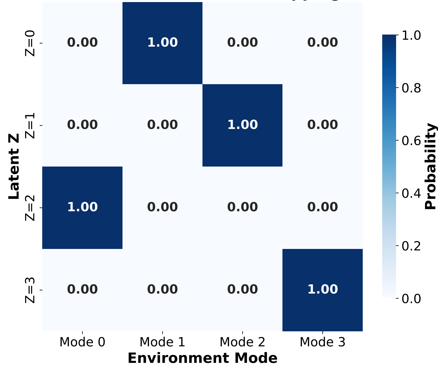
Seed 2222: Z -> Mode Mapping
