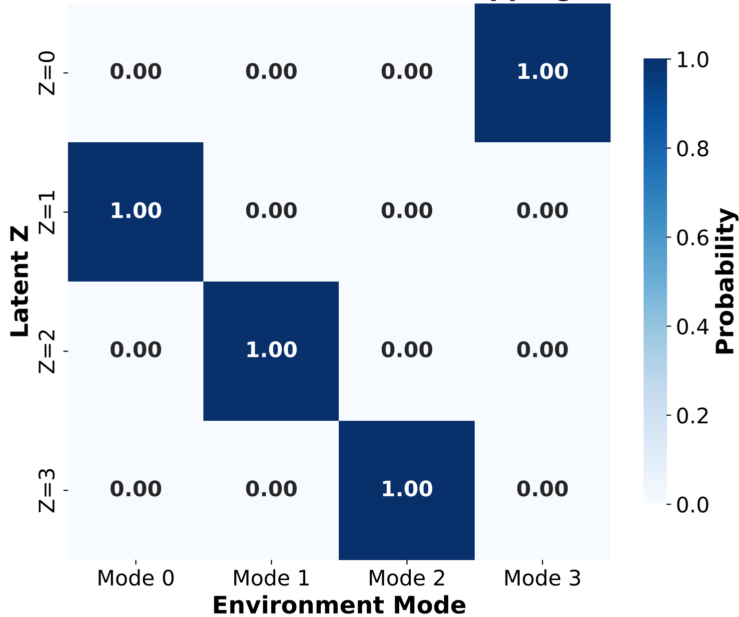
Seed 1234: Z -> Mode Mapping
