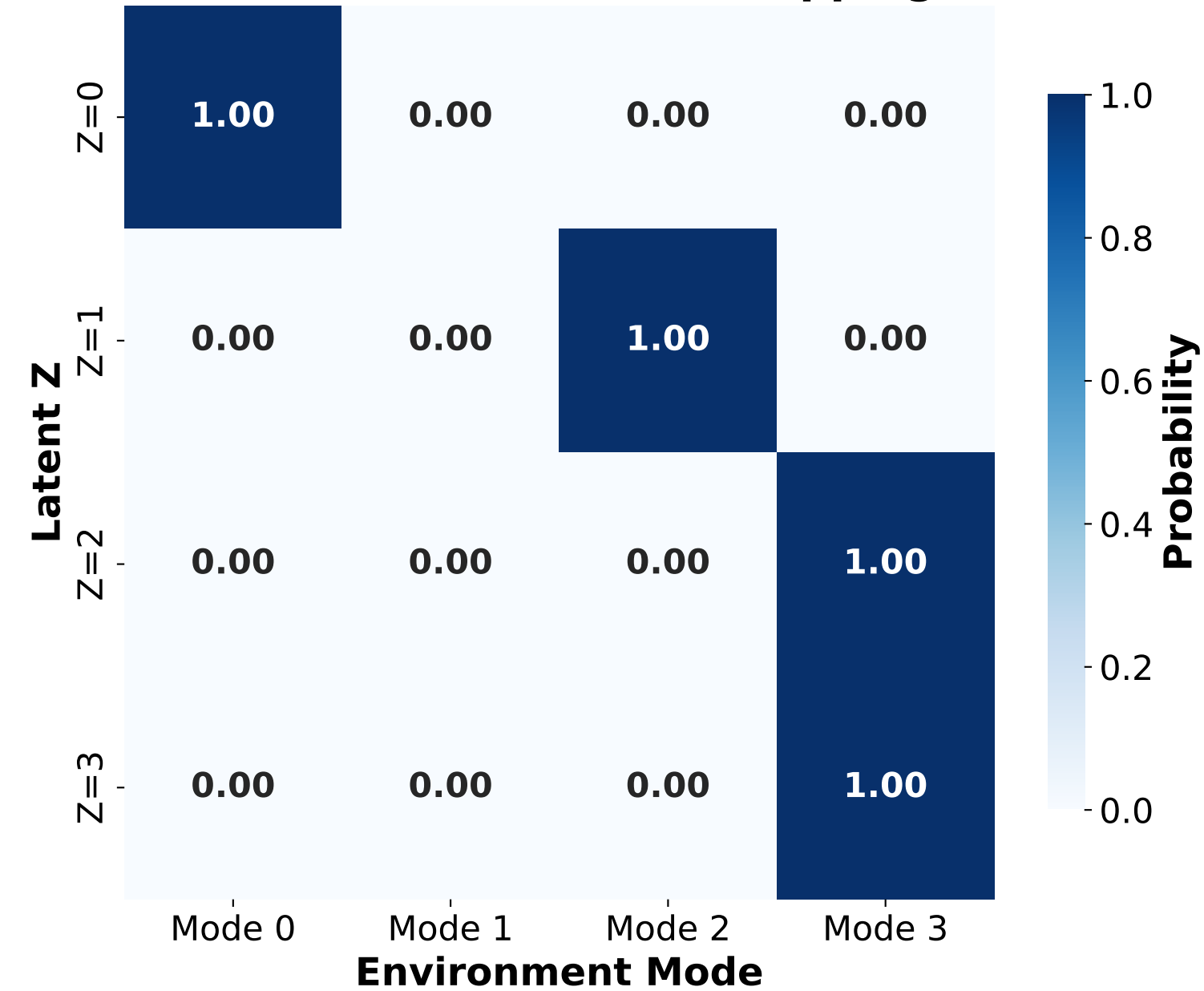
Seed 4444: Z -> Mode Mapping
