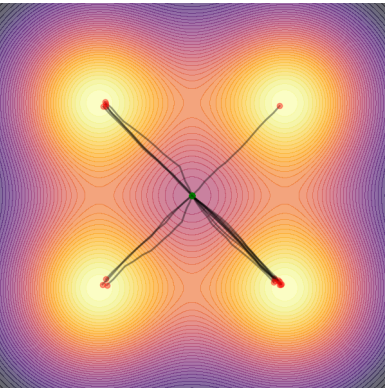
Pre-trained
