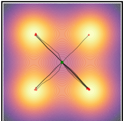
Pre-trained
