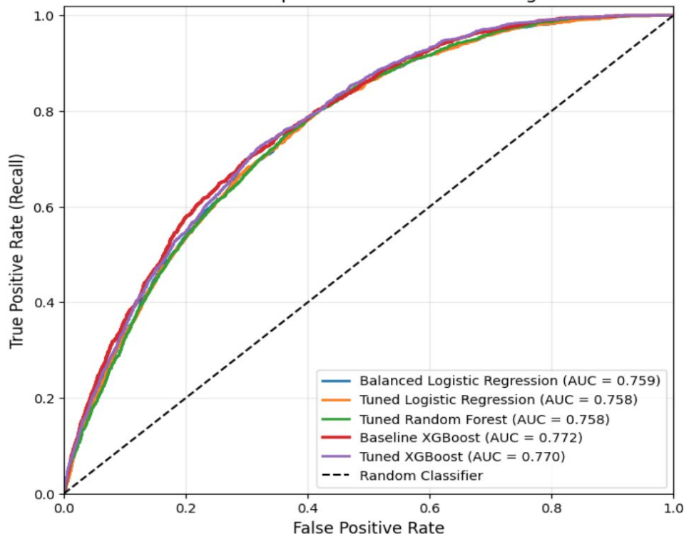
ROC Curve Comparison of Best-Performing Models
