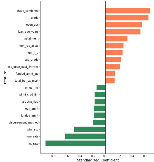
Balanced Logistic Regression Top 20 Important Features
