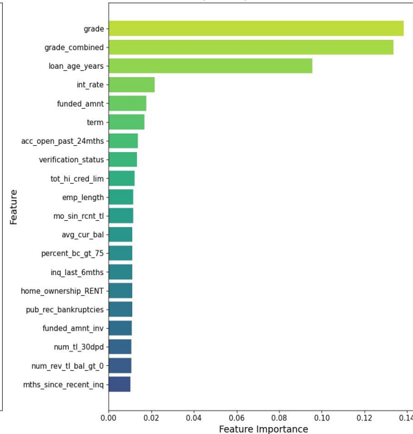
Baseline XGBoost Top 20 Important Features
