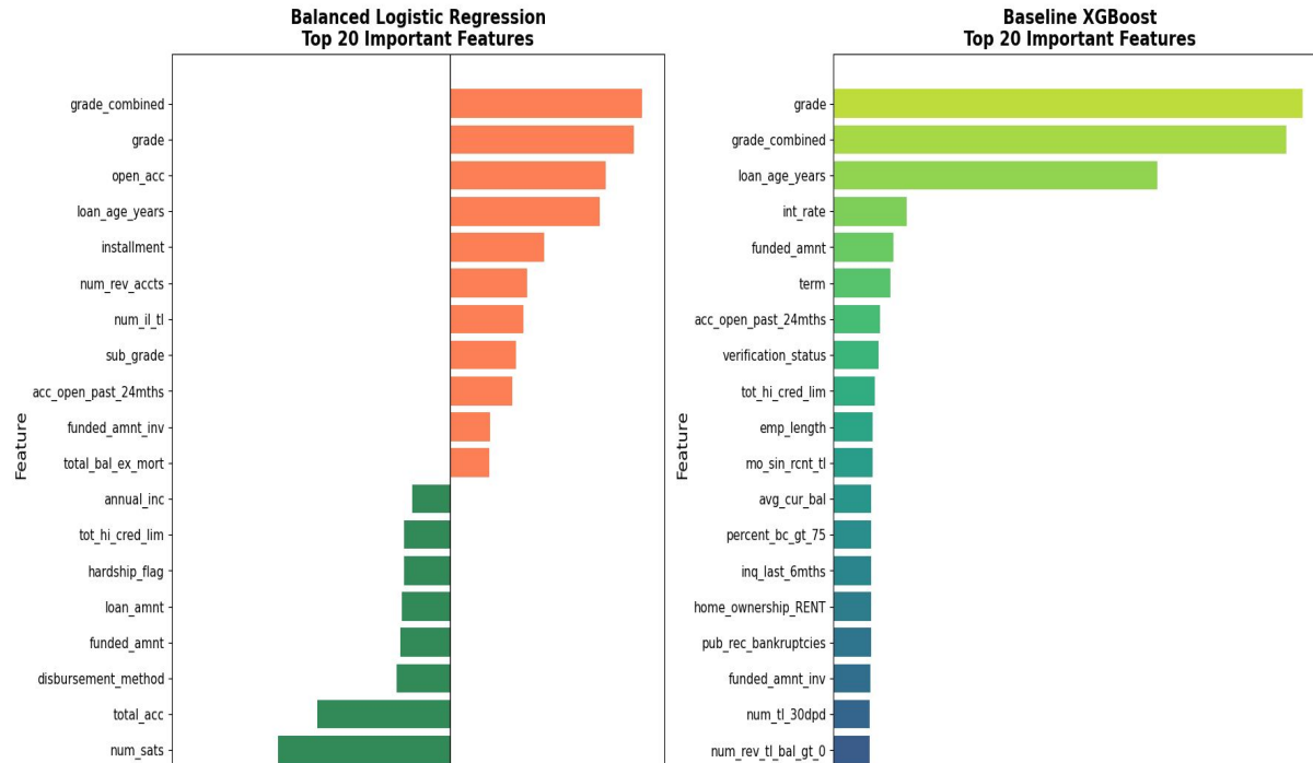
Comparison of Feature Importance Across the Final Models
