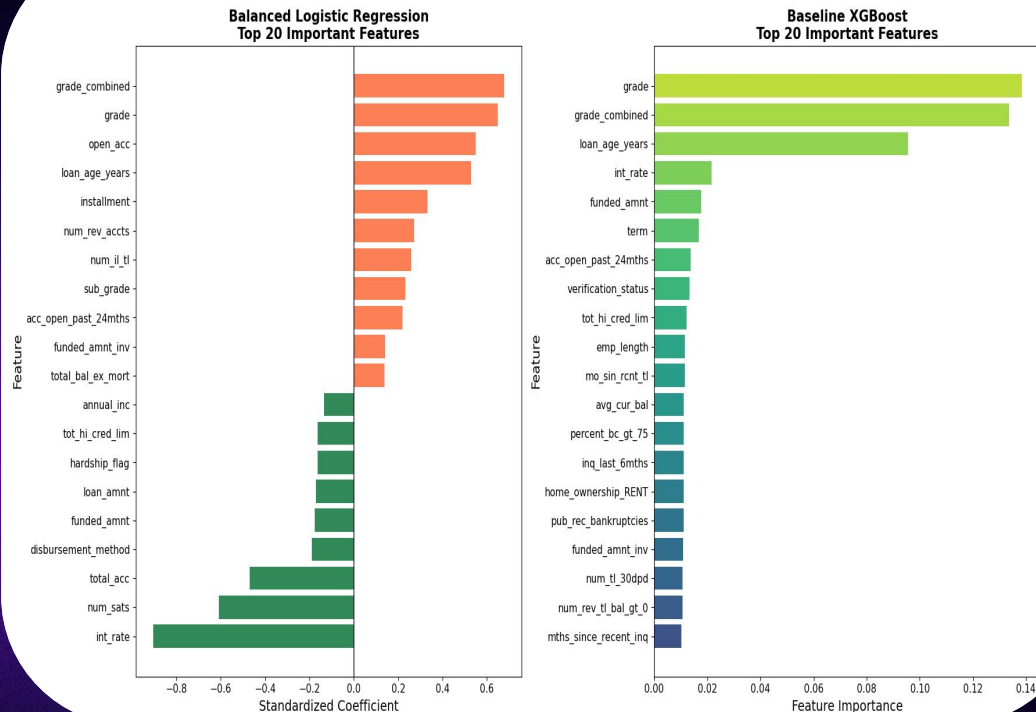
Comparison of Feature Importance Across the Final Models
