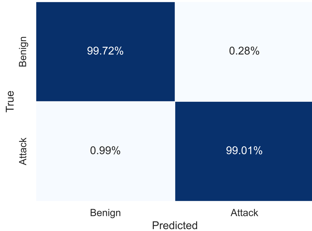
Confusion Matrix — Random Forest
