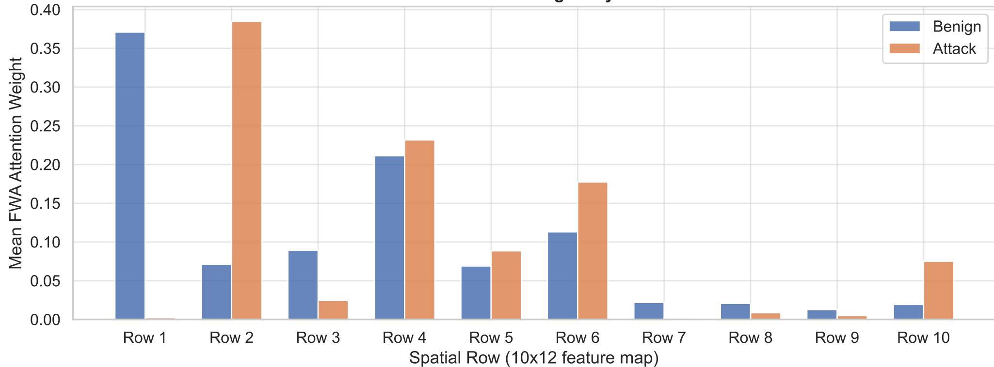
FWA Attention Weights by Class
