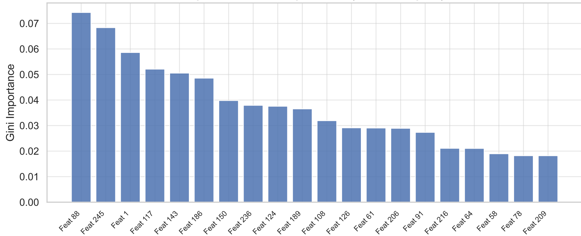
Top-20 RF Feature Importances (DL Latent Space)
