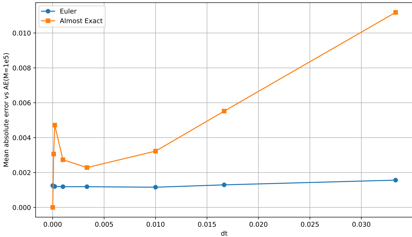
Error vs dt (reference: Almost Exact, M=1e5)
