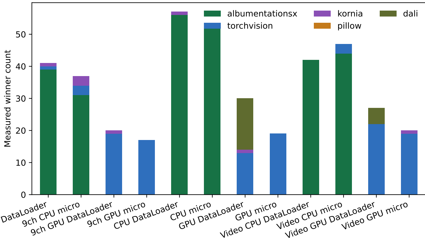
Winner counts among comparable measured transforms
