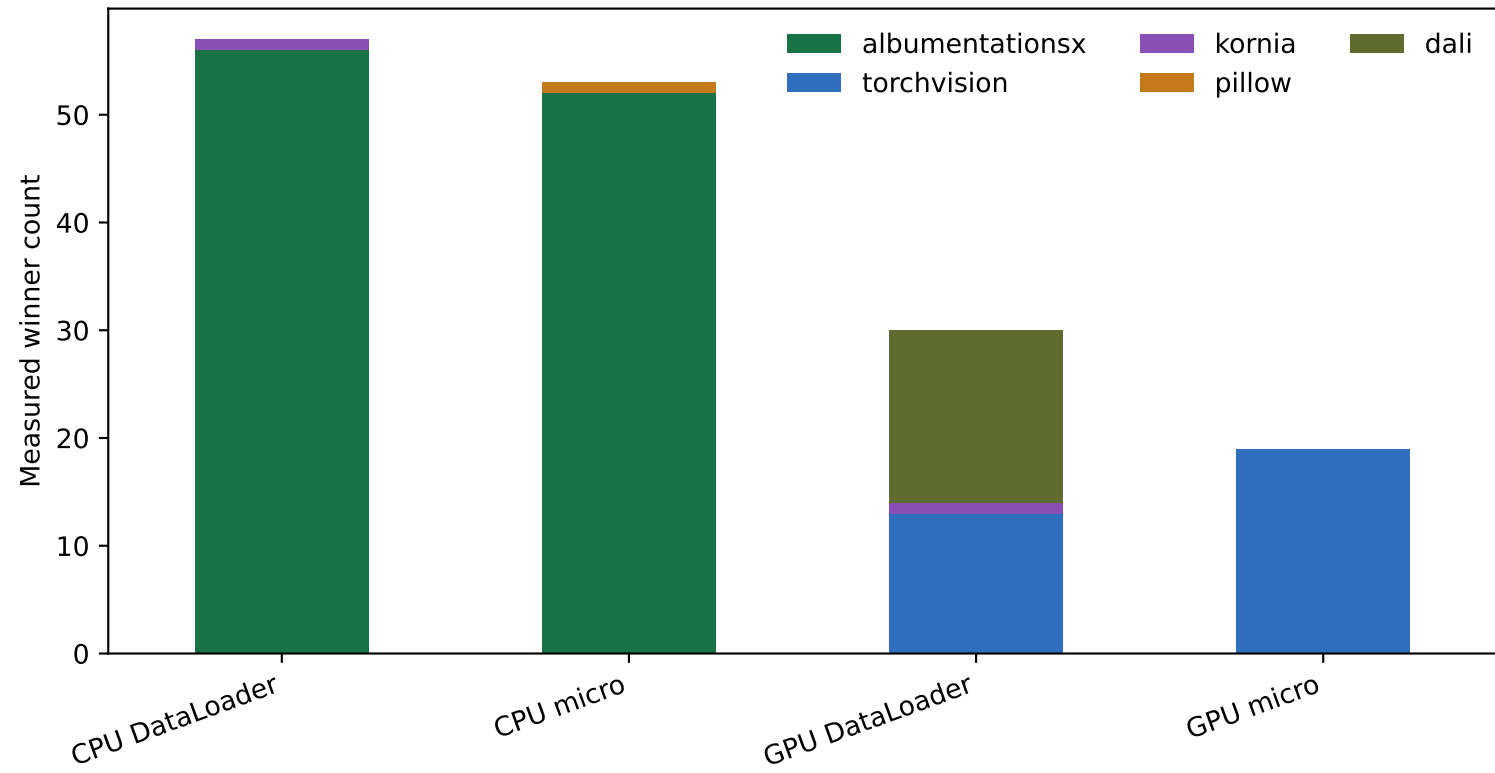
Winner counts among comparable measured transforms
