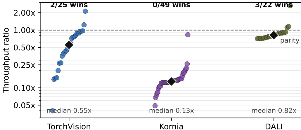
GPU DataLoader / AlbumentationsX CPU
