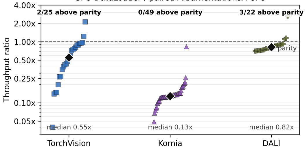
GPU DataLoader / paired AlbumentationsX CPU
