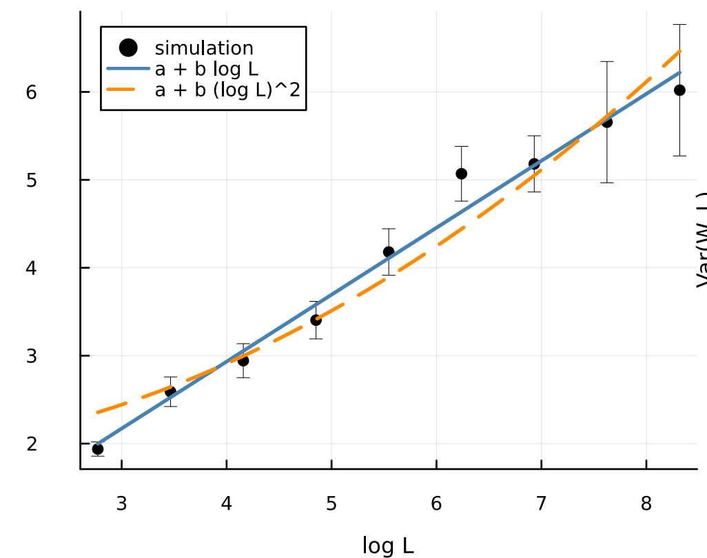
gamma (shape=2.0)
