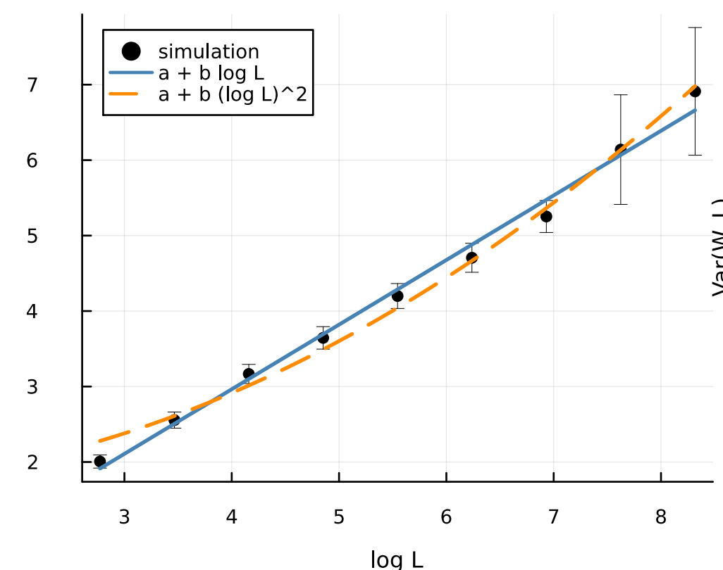
weibull (shape=0.7)
