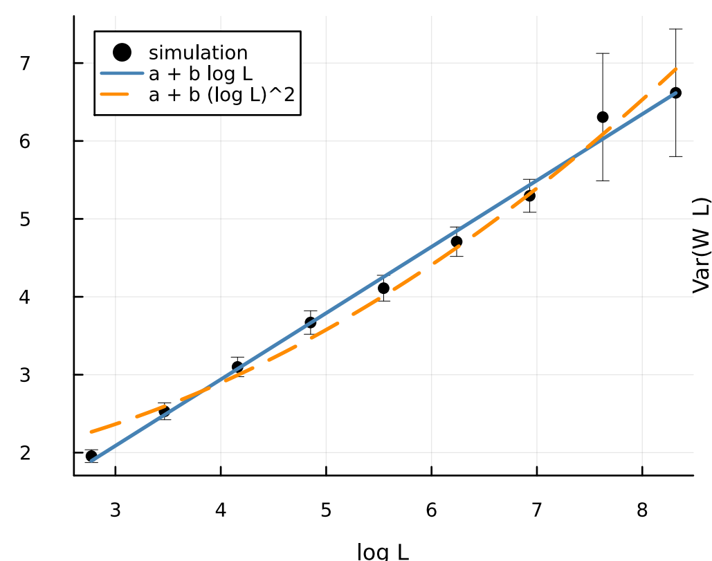
uniform ( a=0.7 )
