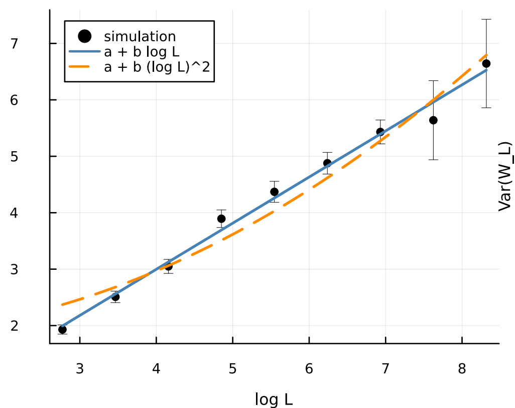
lognormal (sigma=0.5)
