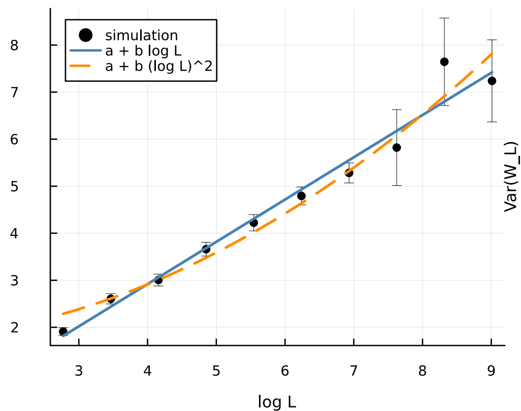
gamma (shape=0.5)
