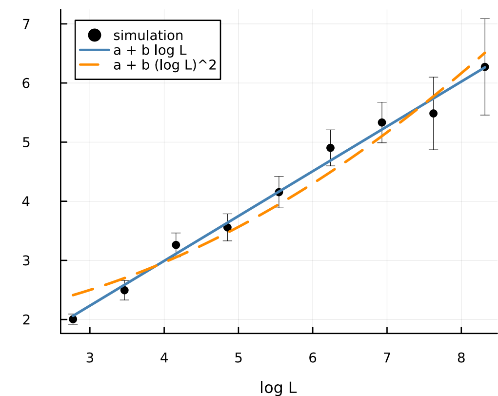
pareto (alpha=3.0)
