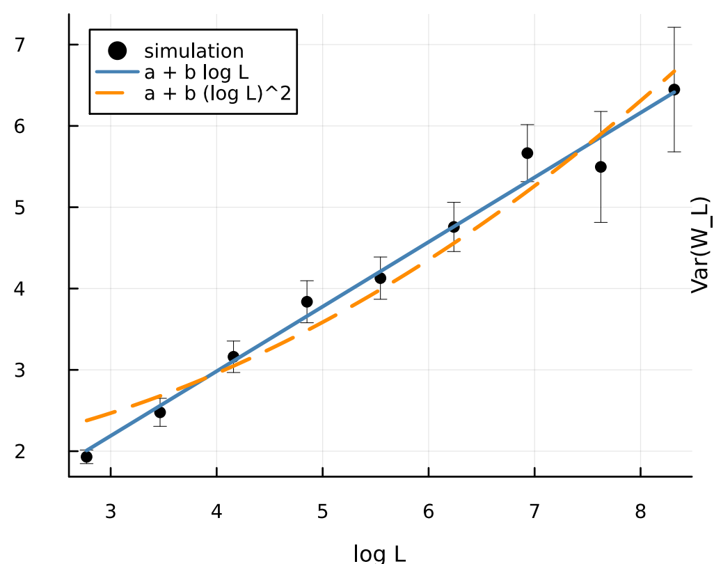
triangular ( a=0.8 )
