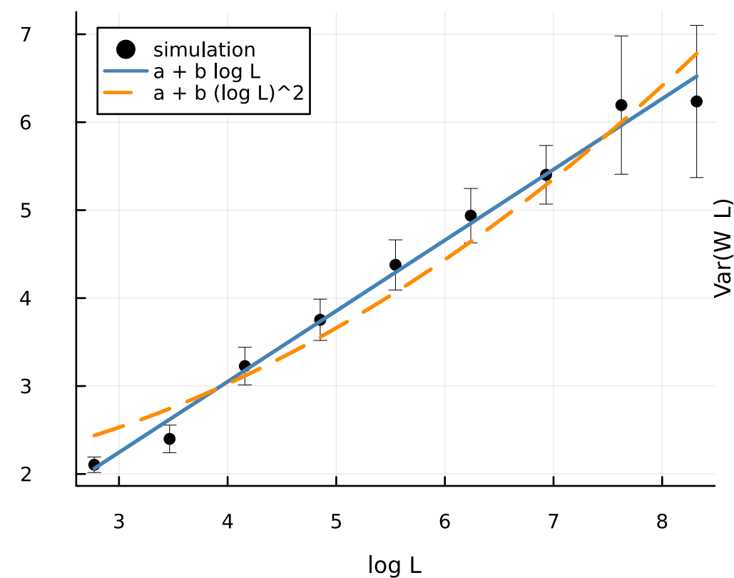
gamma (shape=1.0)
