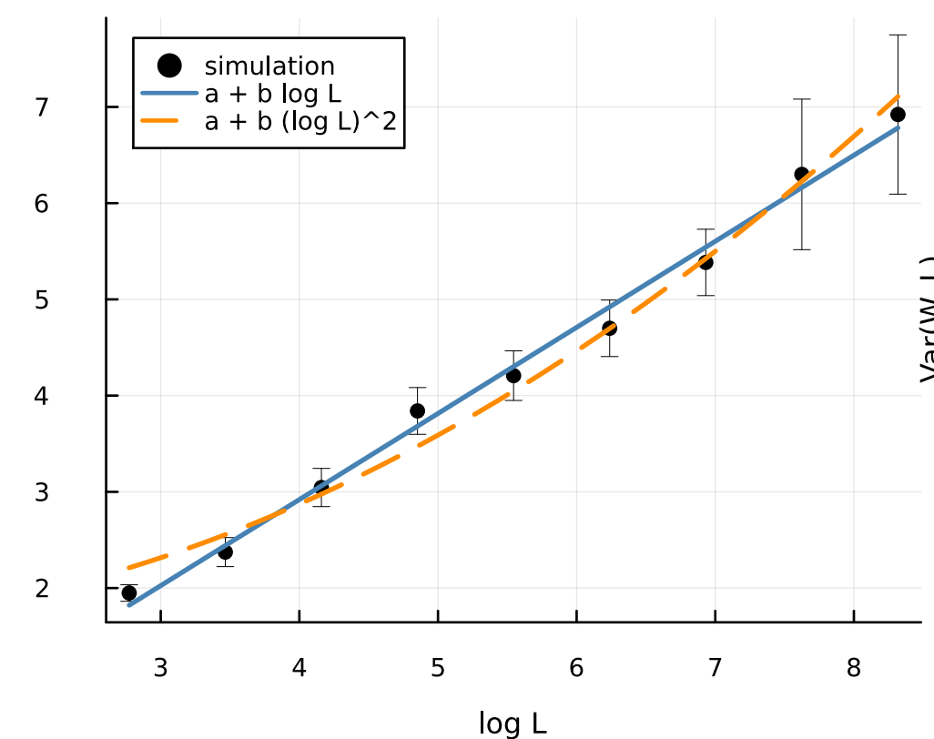
pareto (alpha=2.0)
