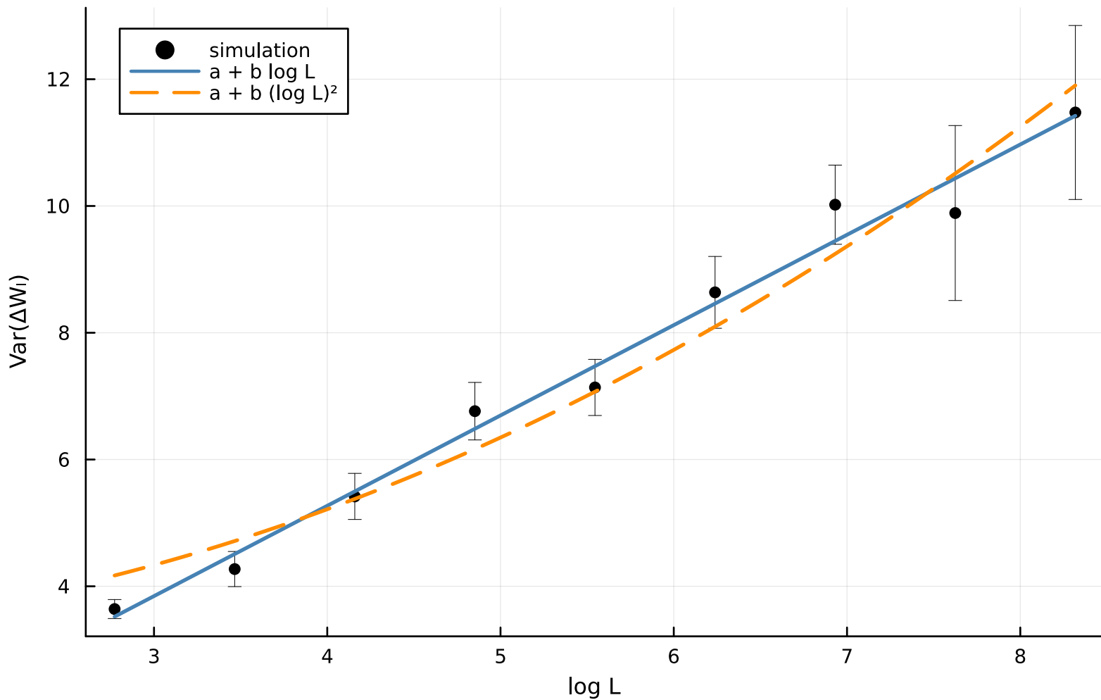
Bernoulli (a=0.8)
