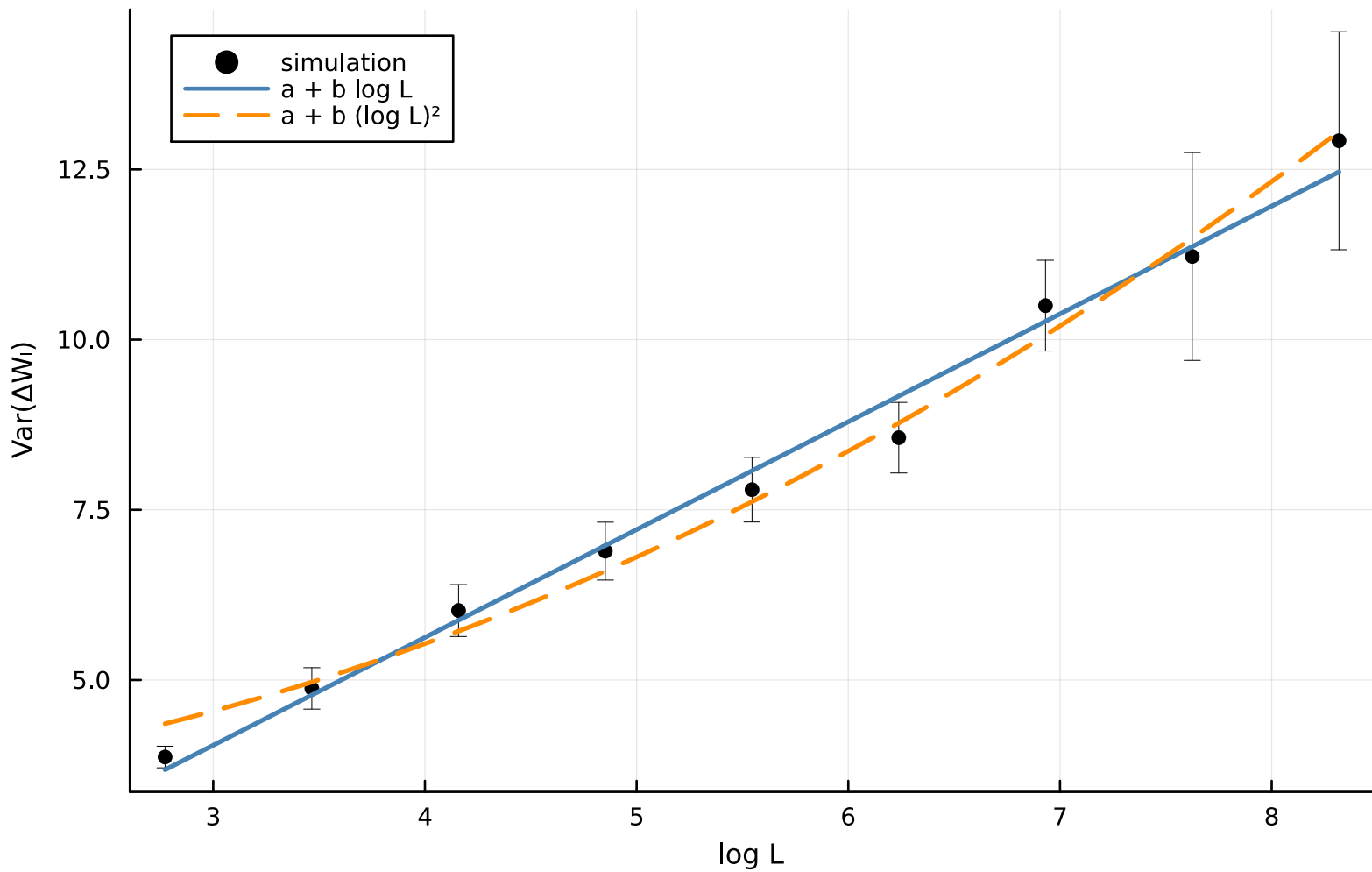
Lognormal ( \sigma=0.5 )
