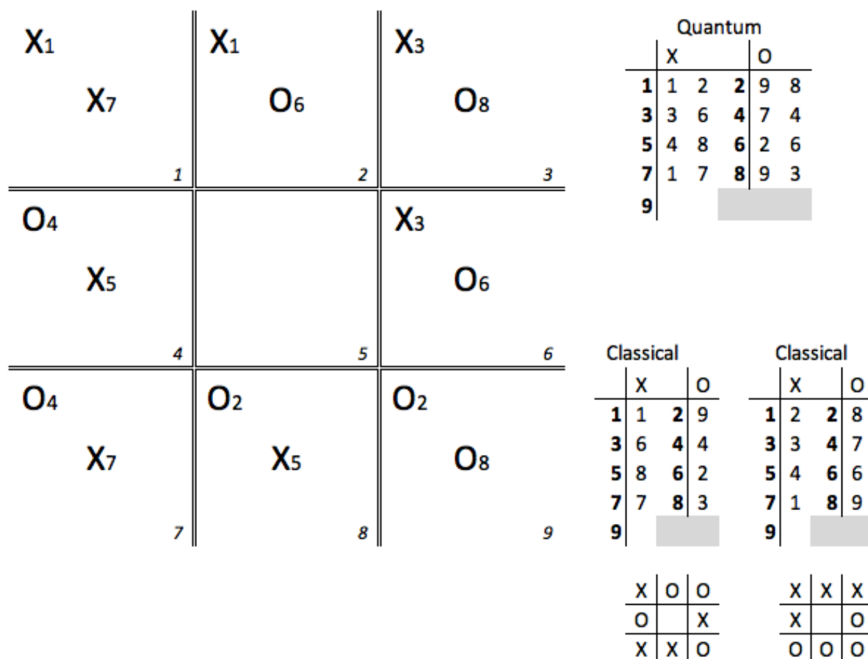
Figure 4 – Last Move Exception: If there is only one square where moves can be made, both spooky marks of the last move may be placed there.
