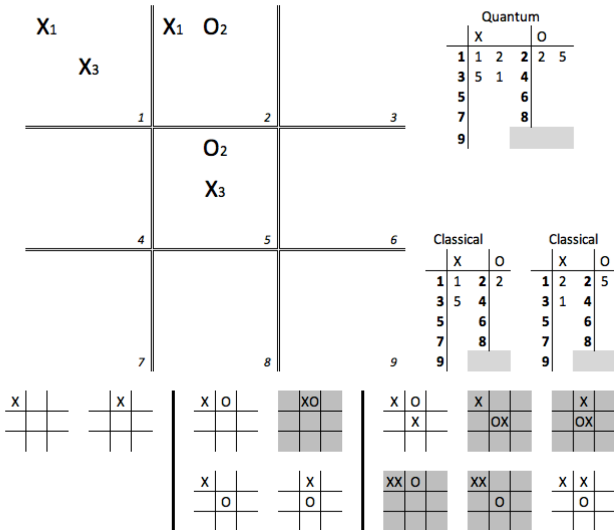
Figure 1 – Nomenclature for Quantum Tic-Tac-Toe: The quantum board is indicated by doubled lines, numbered squares, and subscripted spooky-marks . A list of quantum moves specifies two squares, one for each spooky mark. A quantum game implies a set of classical games, the classical ensemble ; three are shown in this figure, the state after each successive move. Contradictory games are pruned from the ensemble (gray background). Upon a cyclic entanglement, a final pruning, a choice, must be made between two possible classical games.
