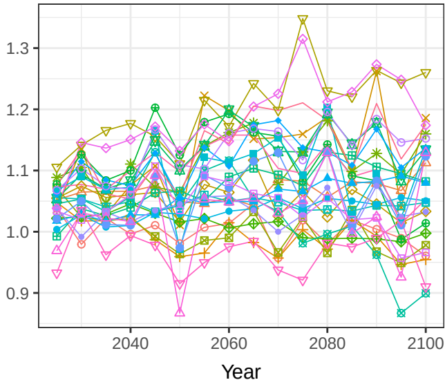
Global crop vegetation scalars
