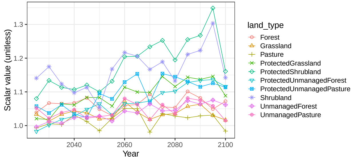
Global non-crop vegetation scalars
