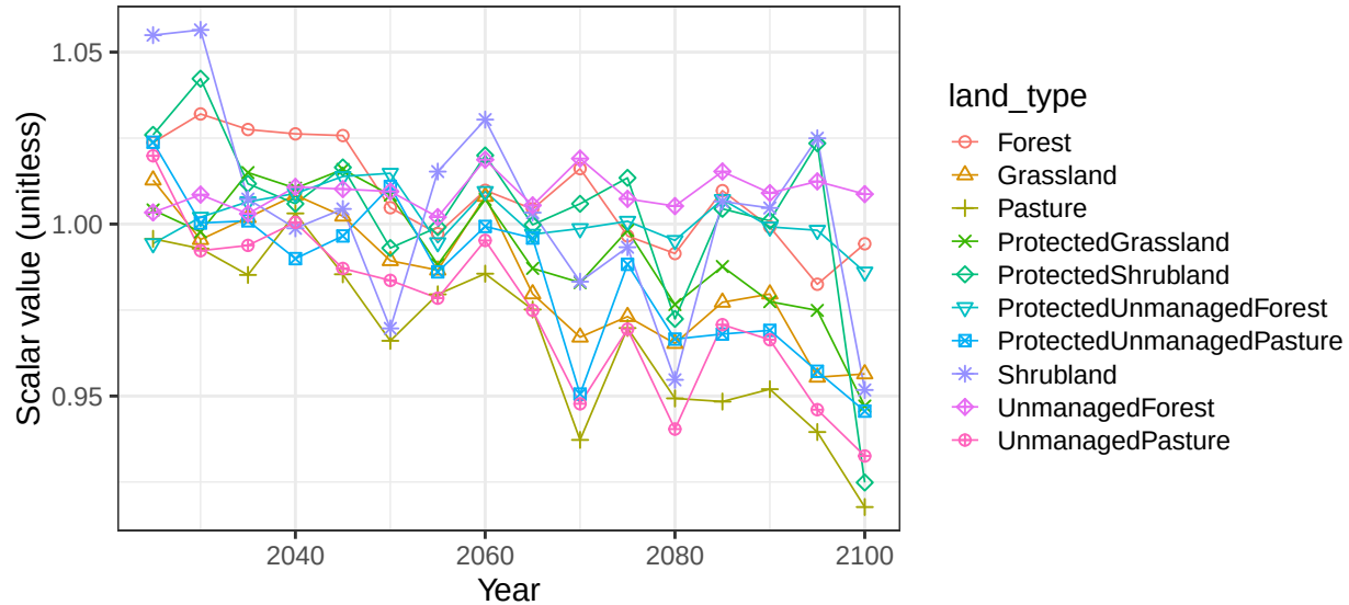
Global non-crop soil scalars
