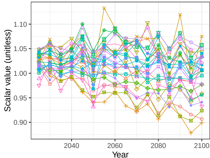
Global crop soil scalars
