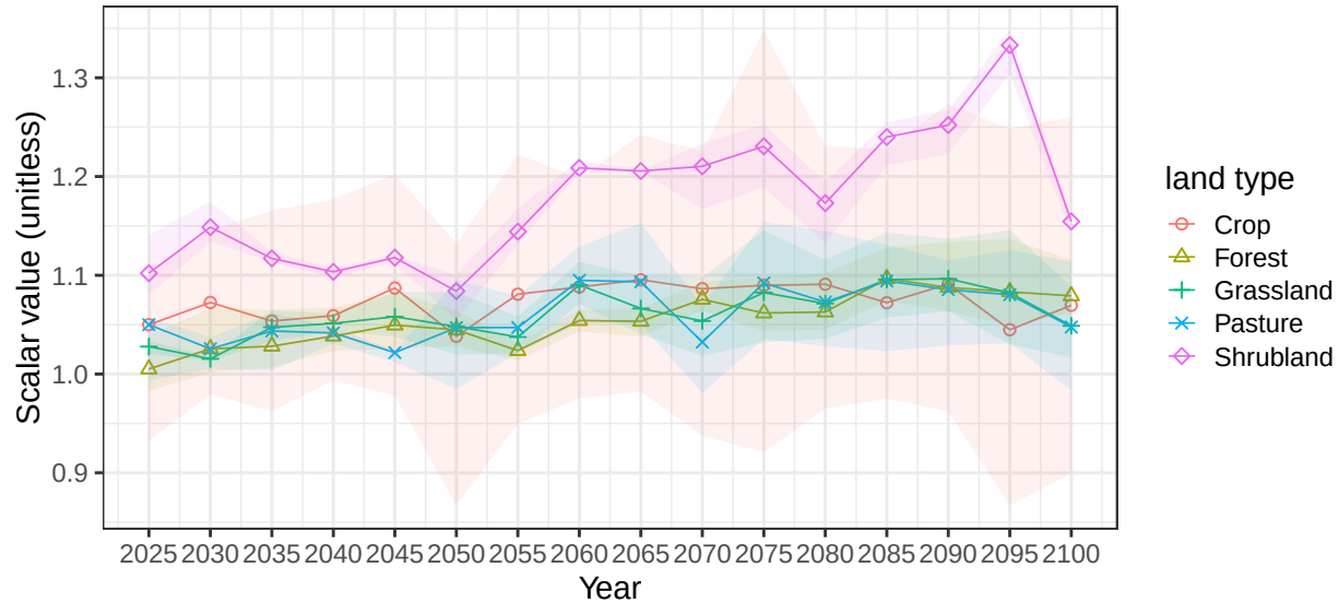
Global average vegetation scalars
