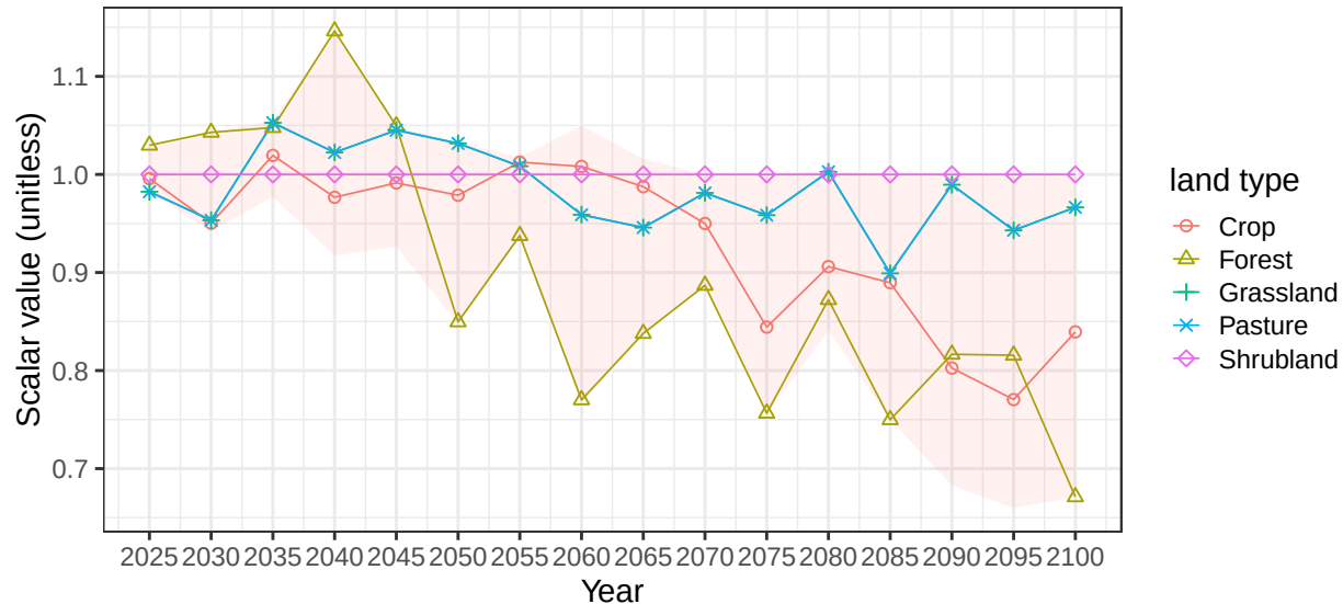
Region Africa_Western basin LChad average soil scalars
