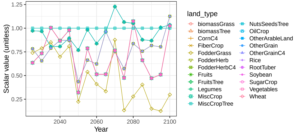
Region Europe_Eastern basin DonR crop vegetation scalars
