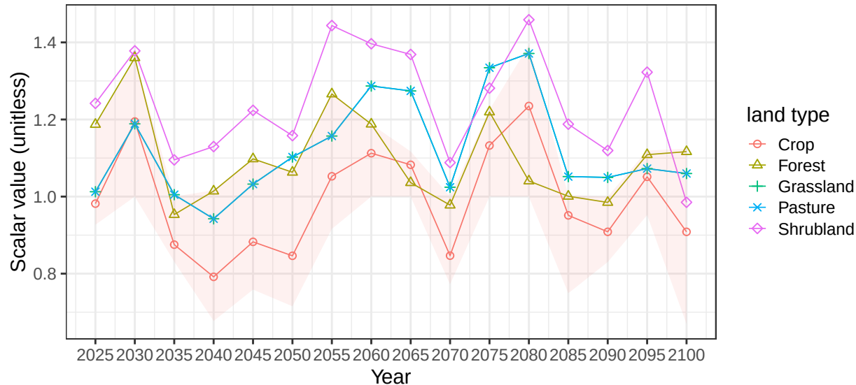
Region Europe_Non_EU basin BlackSeaS average vegetation scalars
