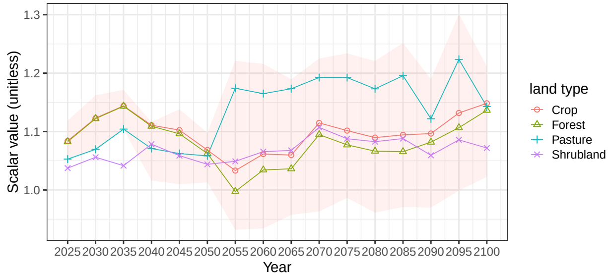
Region Southeast Asia basin GangesR average soil scalars
