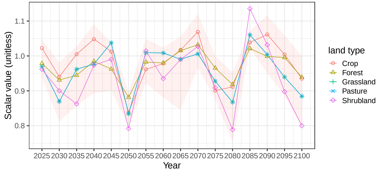
Region Australia_NZ basin AusCstE average soil scalars
