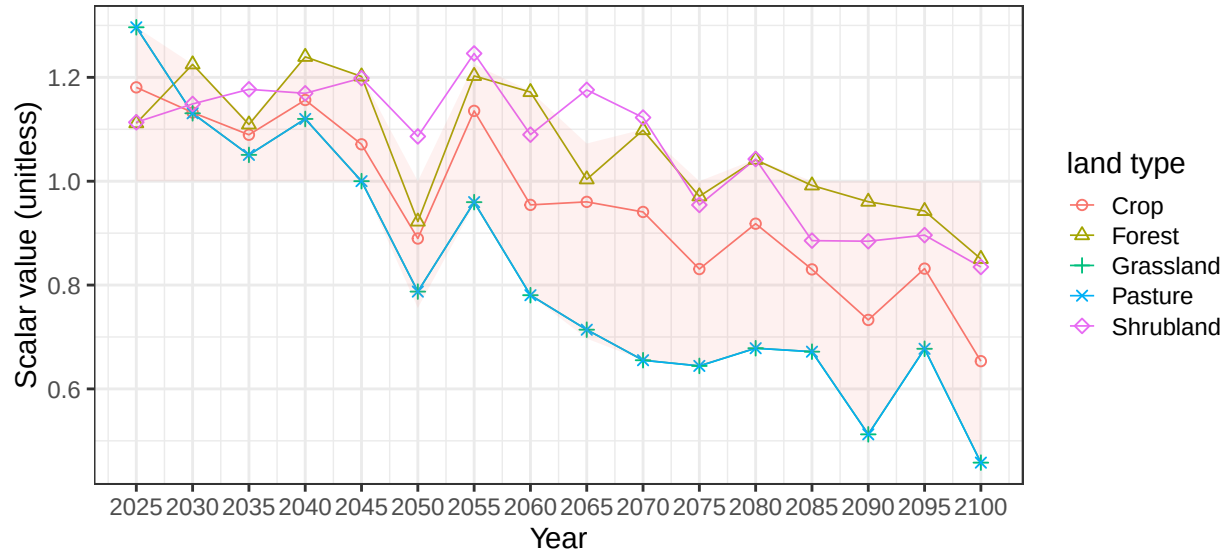
Region EU-15 basin Meditlsl average vegetation scalars
