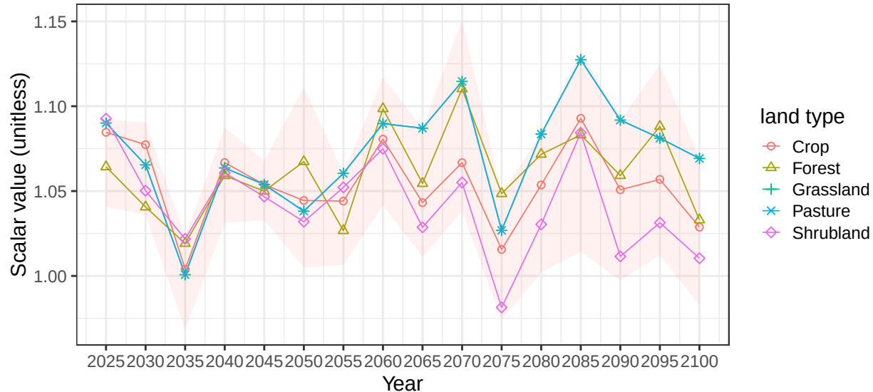
Region China basin Hong average soil scalars
