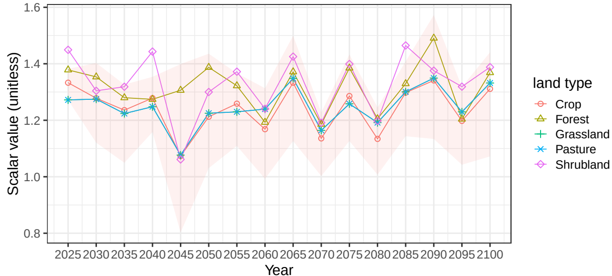
Region Mexico basin MexInt average vegetation scalars
