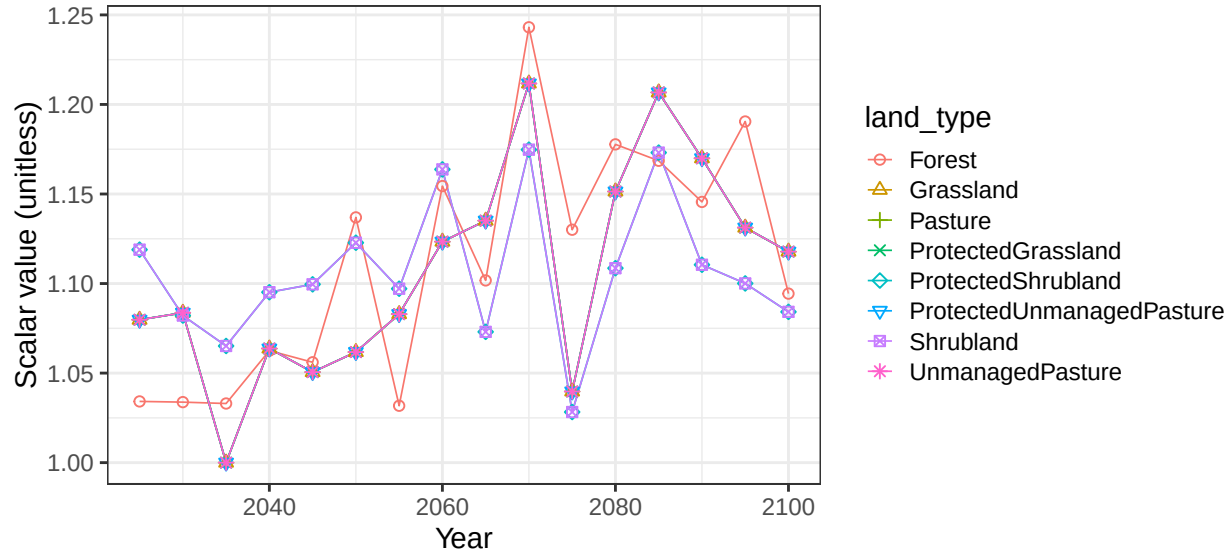
Region China basin Hong non-crop vegetation scalars
