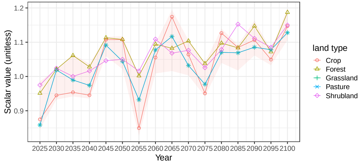
Region Southeast Asia basin IrrawaddyR average vegetation scalars
