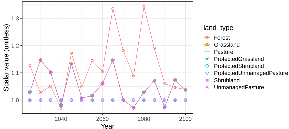
Region India basin MahanadiR non-crop soil scalars
