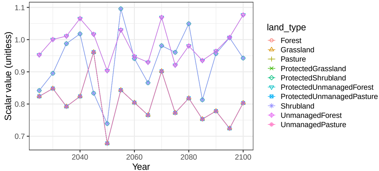
Region Europe_Eastern basin DnieperR non-crop soil scalars
