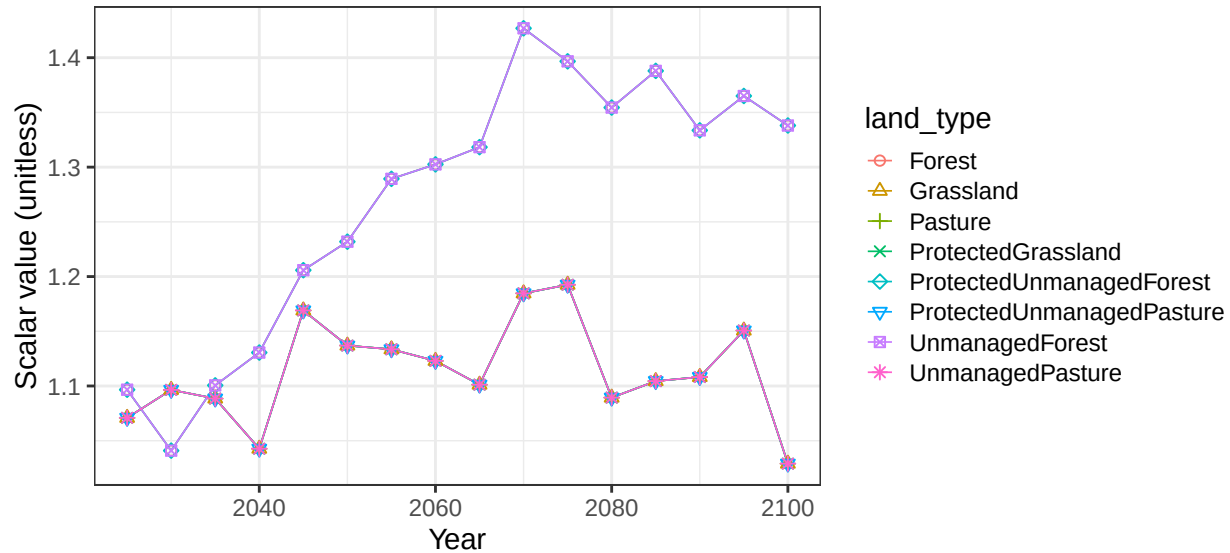
Region South America_Southern basin NegroR non-crop vegetation scalar
