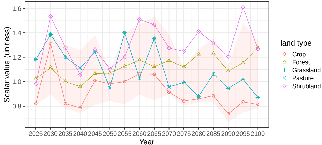
Region Australia_NZ basin AusCstW average vegetation scalars
