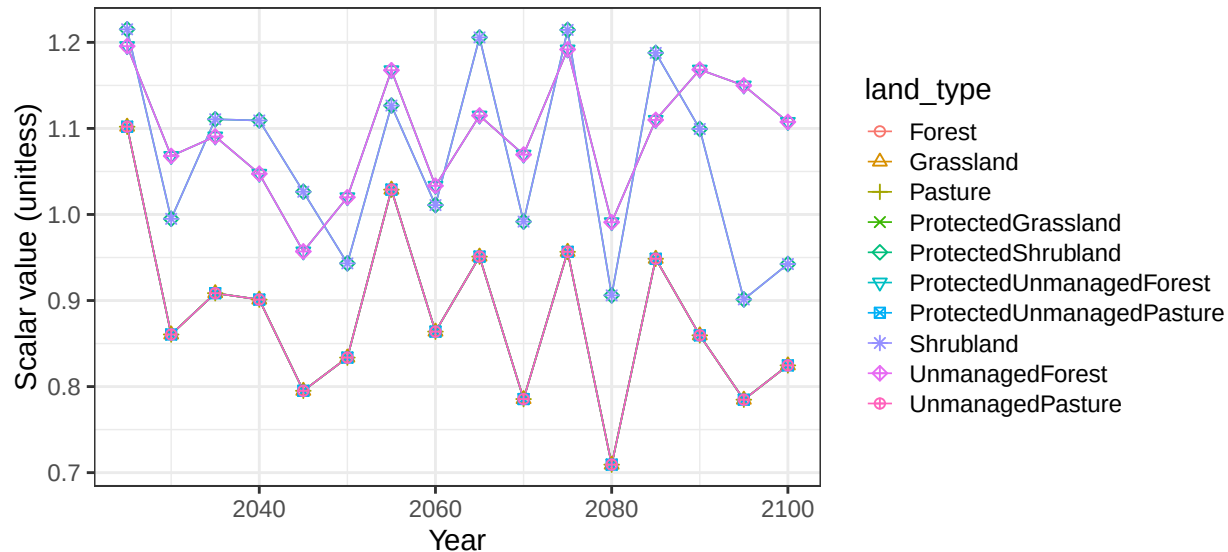
Region USA basin TexasCst non-crop soil scalars
