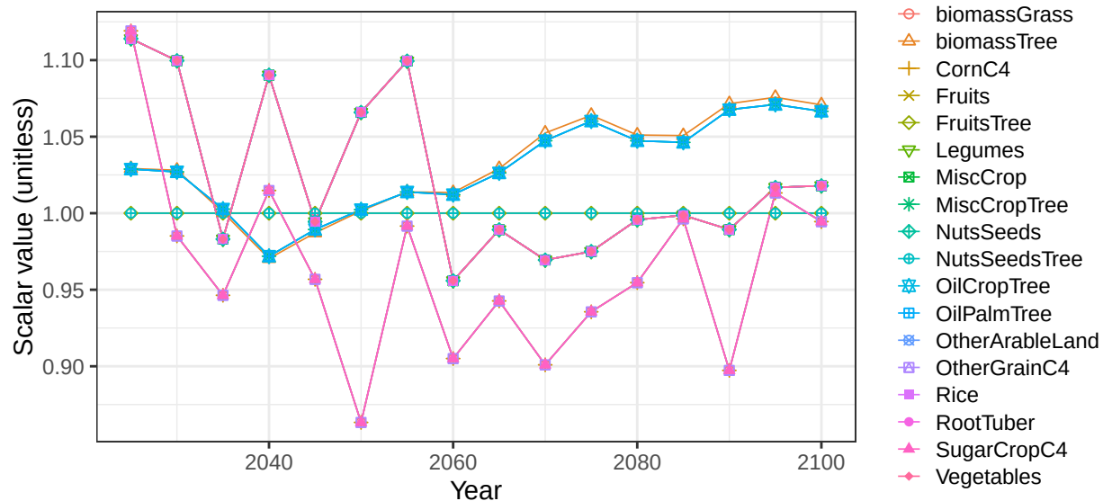
Region Southeast Asia basin PapuaCst crop vegetation scalar and type
