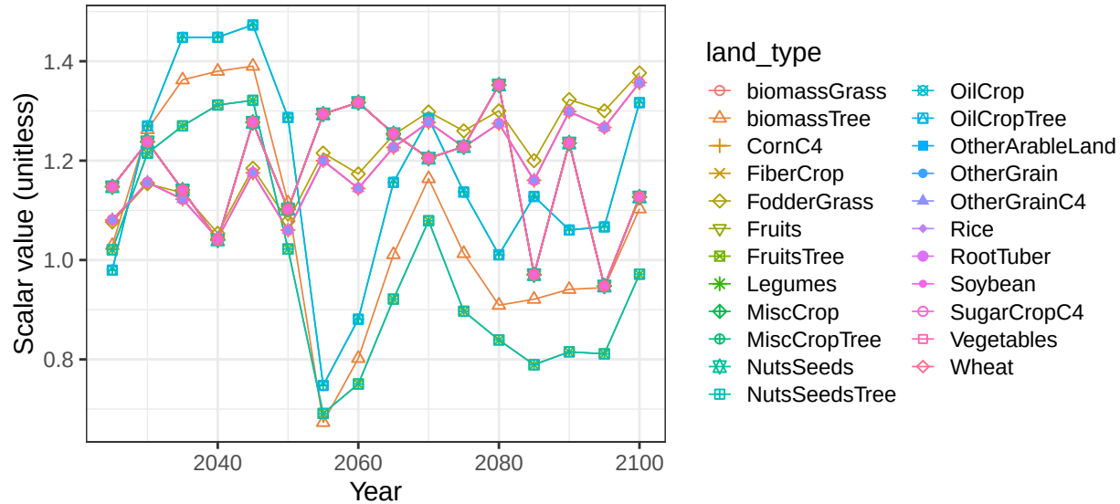
Region India basin GangesR crop vegetation scalars
