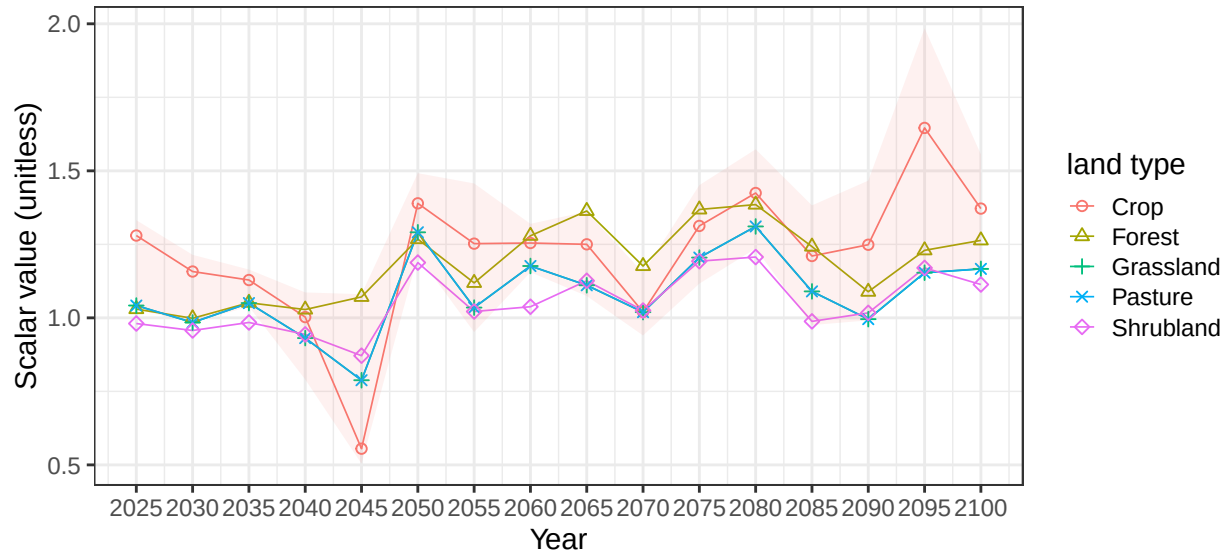
Region Central Asia basin LBalkash average vegetation scalars
