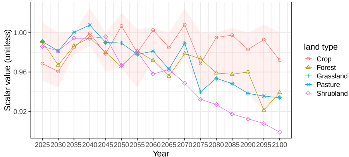
Region South America_Southern basin LaPuna average soil scalars
