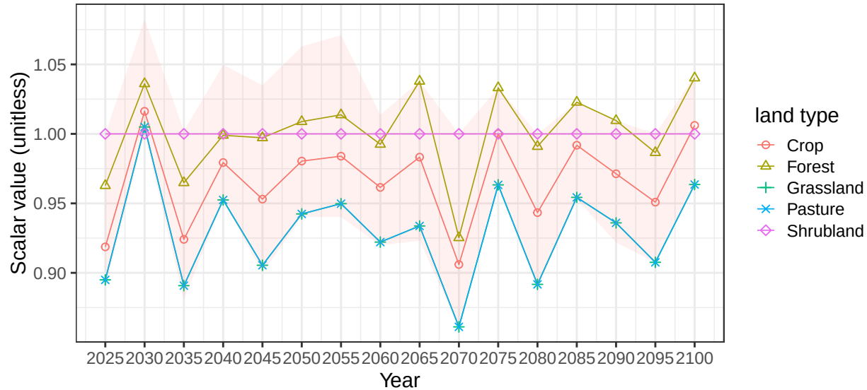
Region Mexico basin MexCstW average soil scalars
