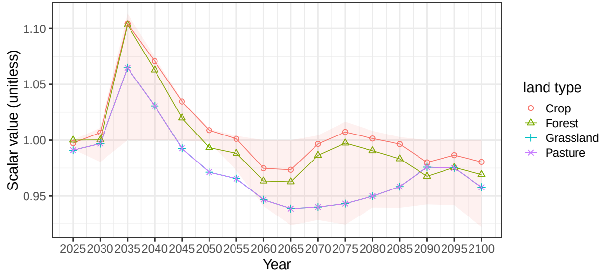
Region EU-15 basin Ireland average soil scalars
