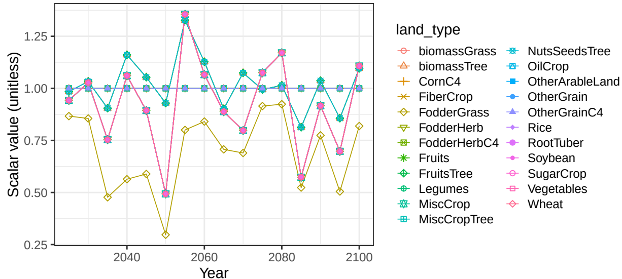
Region Europe_Eastern basin DanubeR crop vegetation scalars
