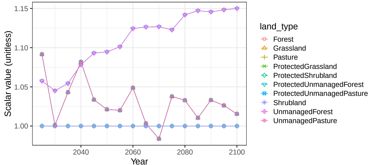
Region Africa_Western basin CongoR non-crop vegetation scalars
