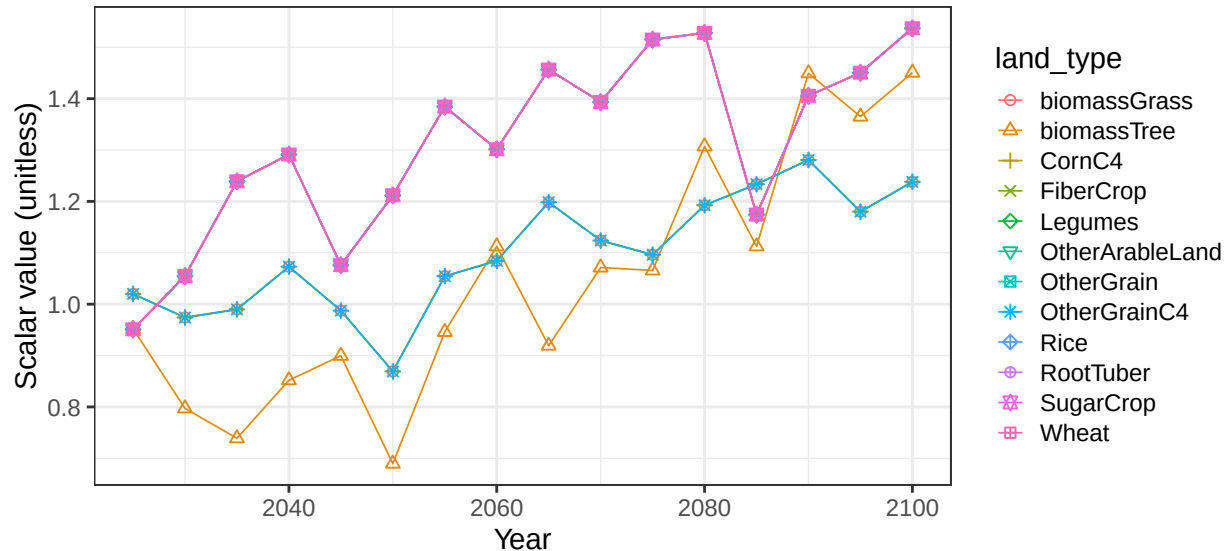
Region South Asia basin AmuDaryaR crop vegetation scalars
