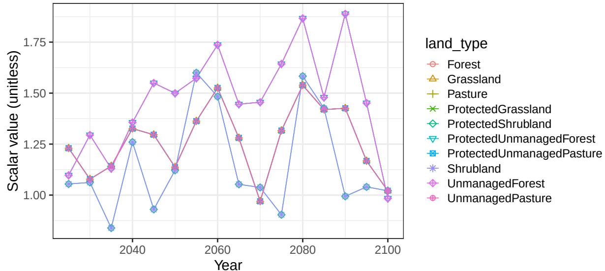
Region Africa_Southern basin LimpopoR non-crop vegetation scalars
