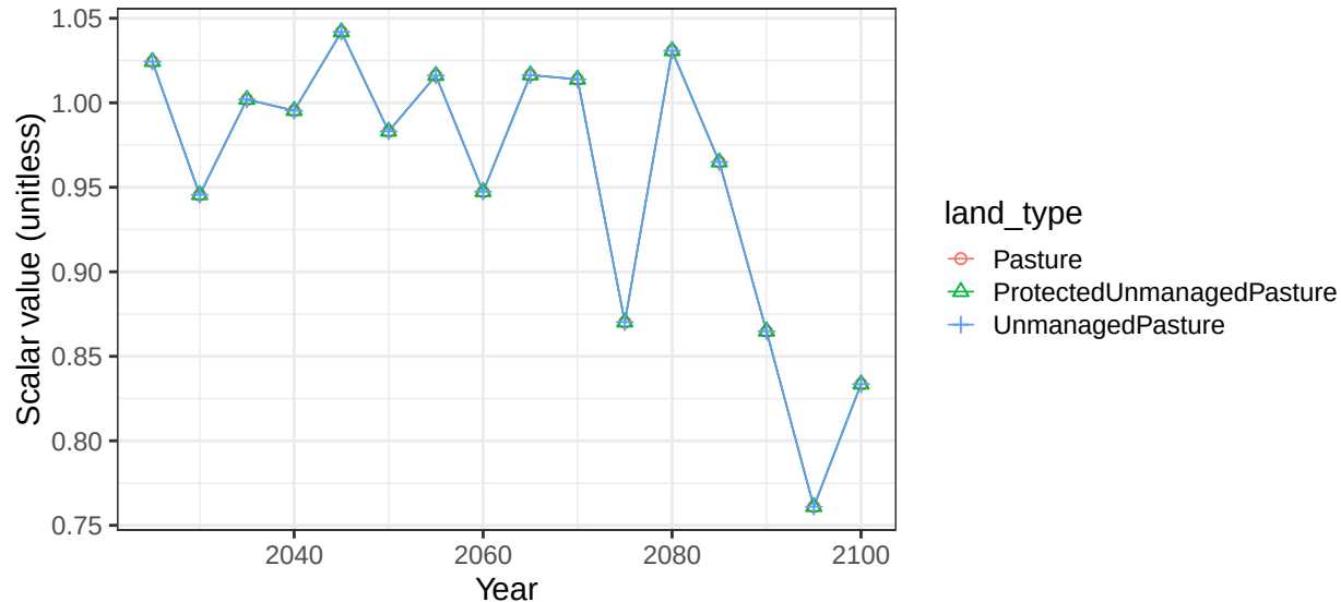
Region Pakistan basin Tarim non-crop soil scalars
