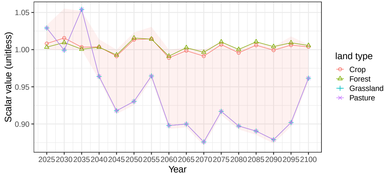
Region Southeast Asia basin BorneoCstN average soil scalars
