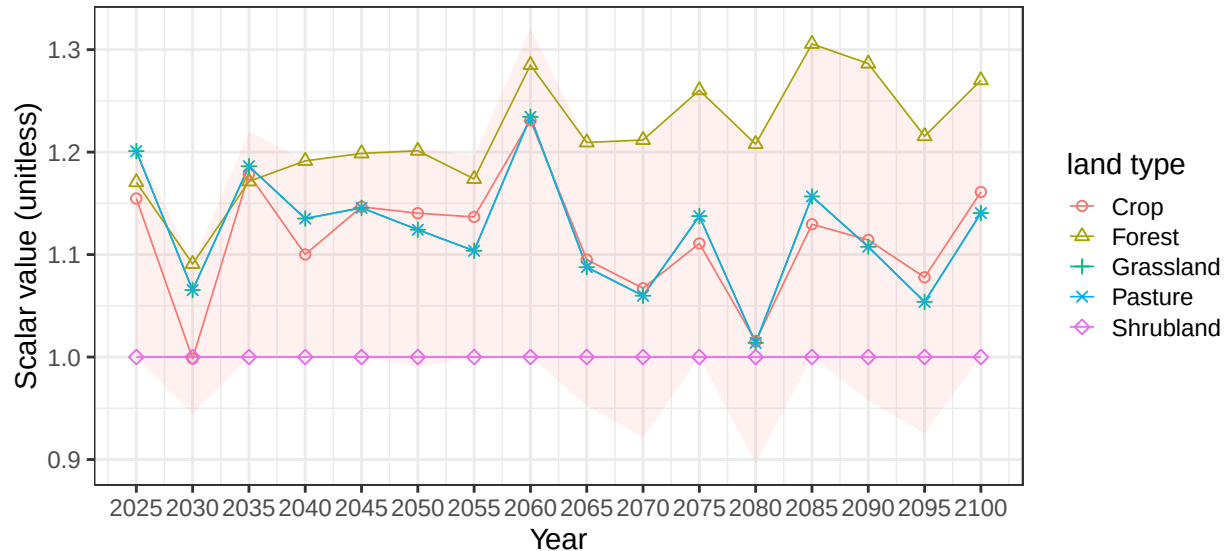
Region Africa_Southern basin CongoR average vegetation scalars
