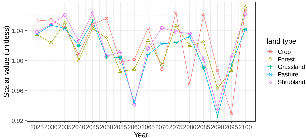
Region USA basin PacArctic average soil scalars
