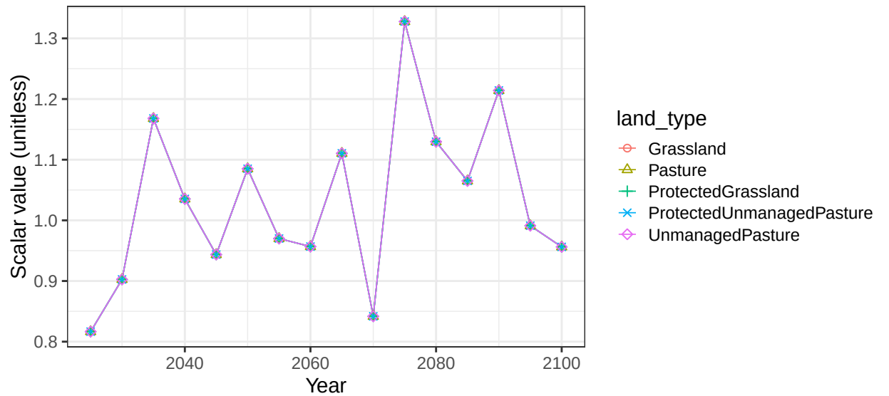
Region South America_Southern basin BrzCstS non-crop vegetation scala
