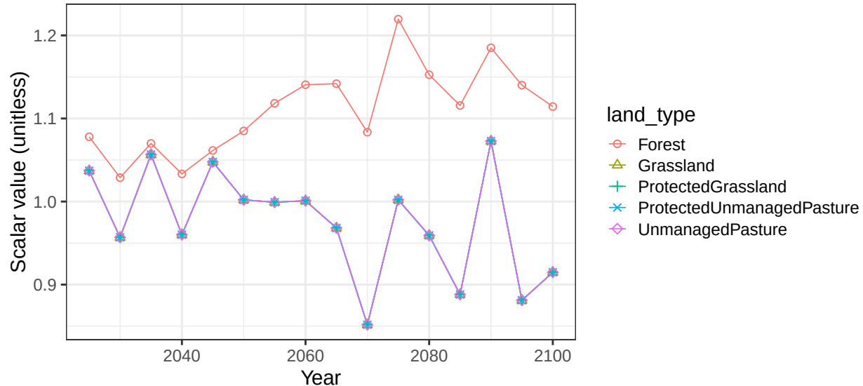
Region EU-15 basin EngWales non-crop vegetation scalars
