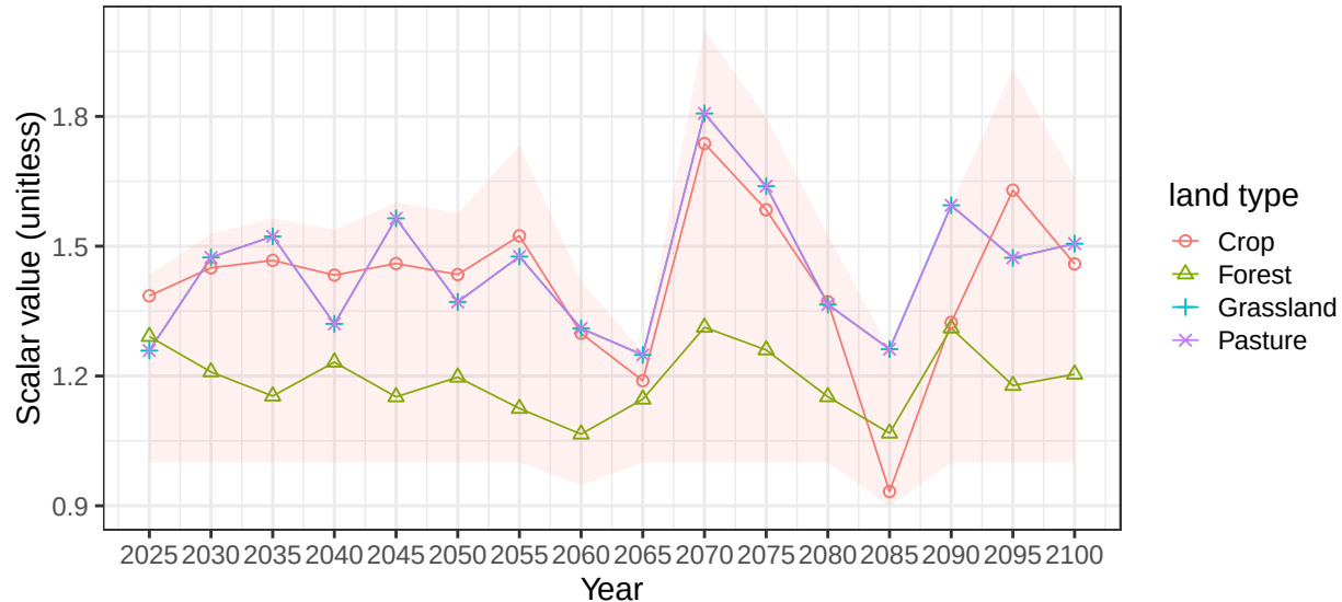
Region USA basin NelsonR average vegetation scalars
