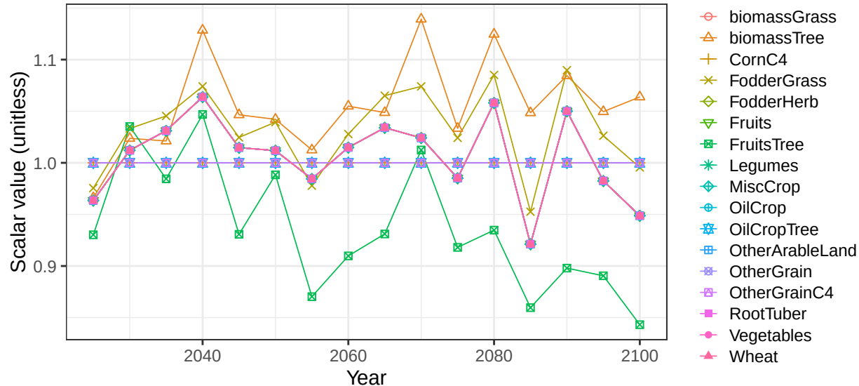
Region Australia_NZ basin Tasmania crop vegetation scalars
