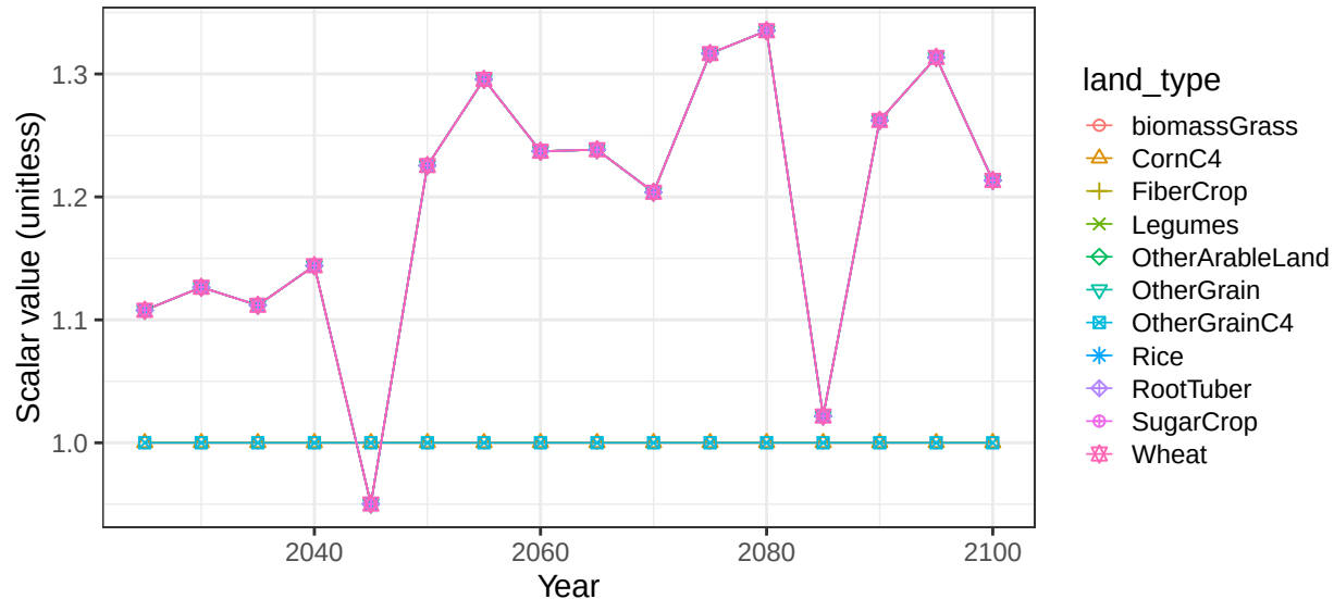
Region South Asia basin CaspianE crop soil scalars
