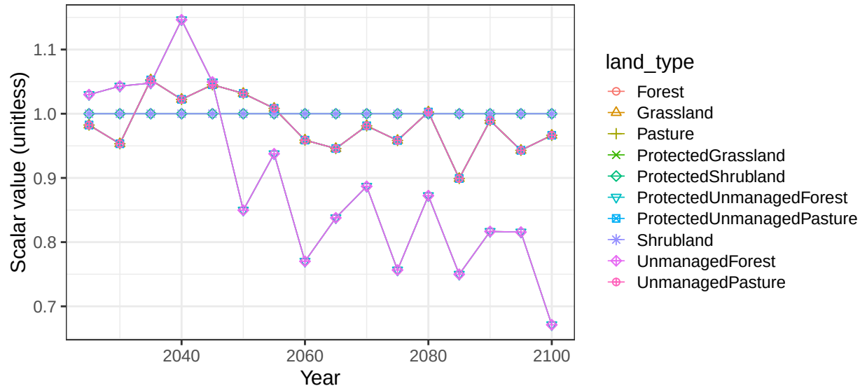
Region Africa_Western basin LChad non-crop soil scalars
