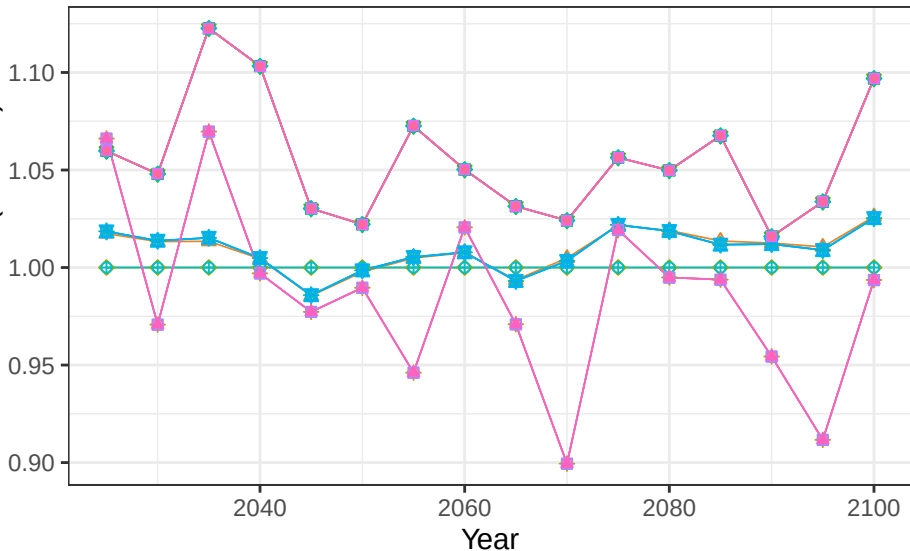
Region Southeast Asia basin FlyR crop soil scalars
