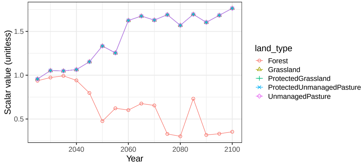
Region EU-15 basin NevaR non-crop vegetation scalars
