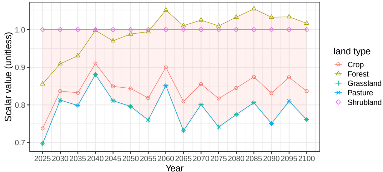
Region Brazil basin BrzCstN average vegetation scalars
