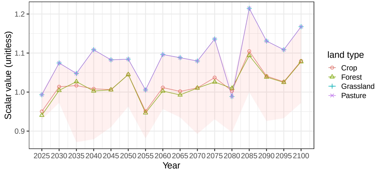
Region USA basin UsaCstNE average vegetation scalars
