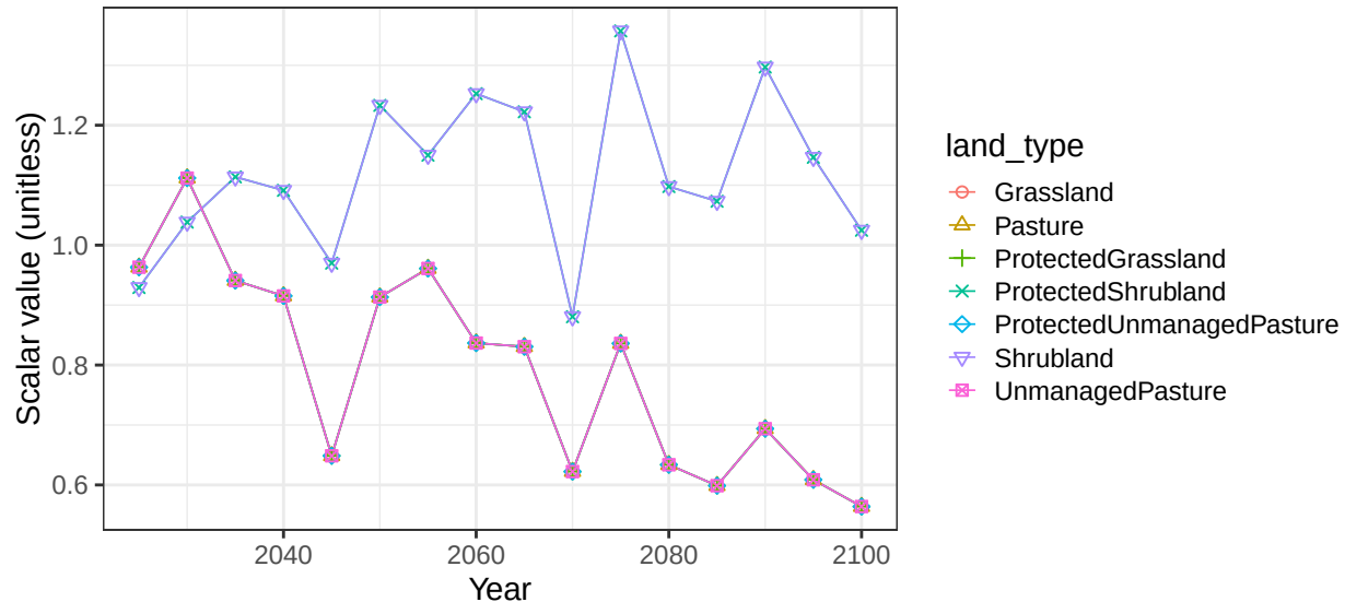
Region Middle East basin DeadSea non-crop vegetation scalars
