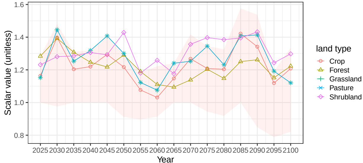
Region USA basin California average vegetation scalars
