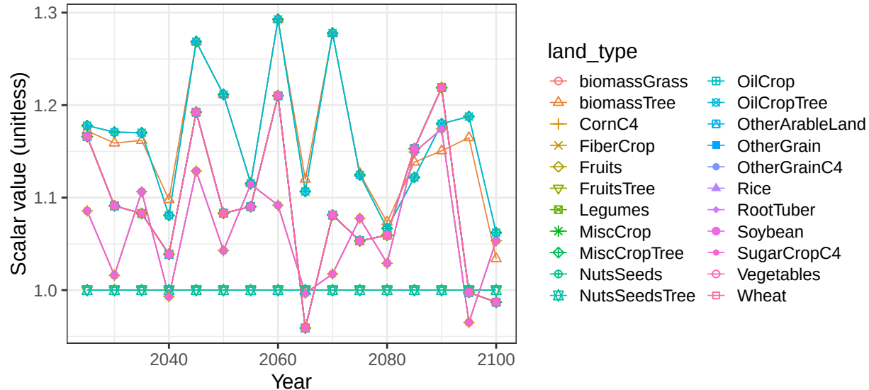
Region Africa_Southern basin AfrCstSE crop soil scalars
