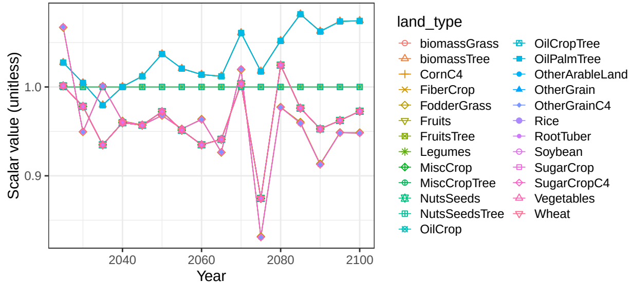
Region Southeast Asia basin MalaysiaP crop vegetation scalars
