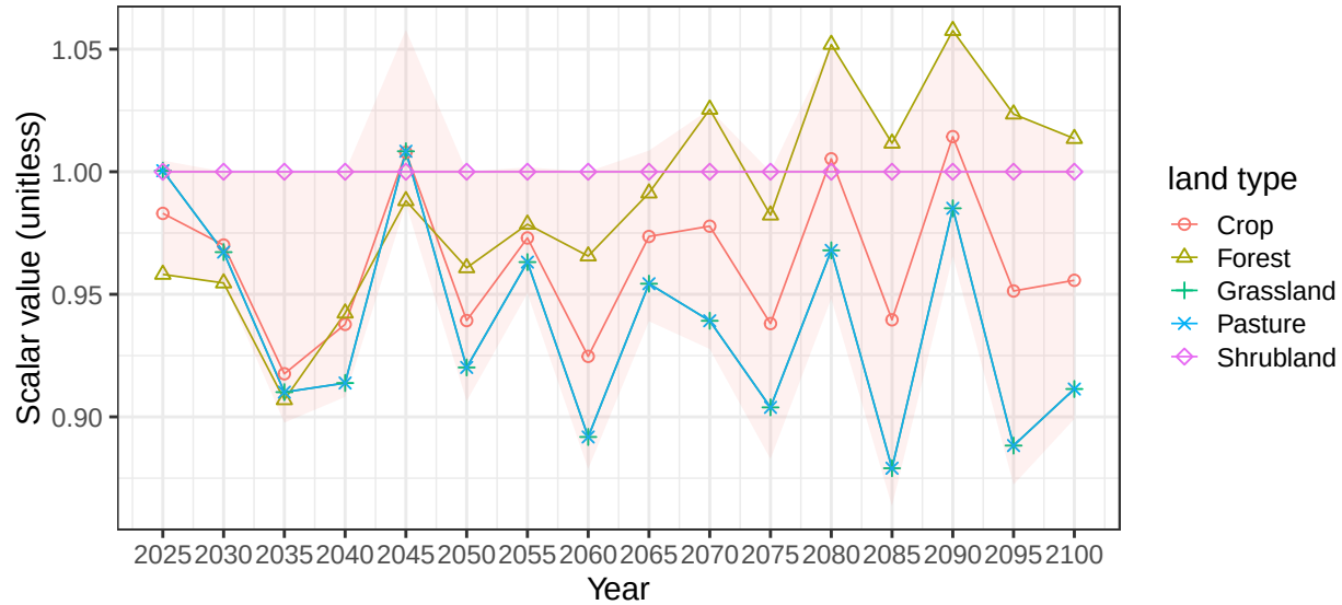
Region Central America and Caribbean basin CntAmer average vegetation
