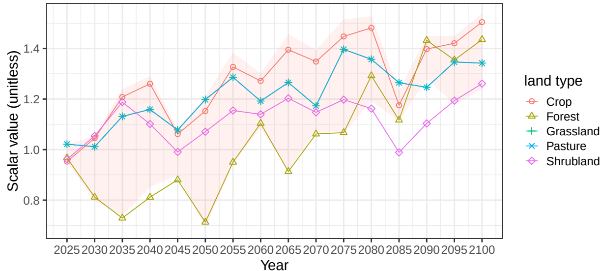
Region South Asia basin AmuDaryaR average vegetation scalars
