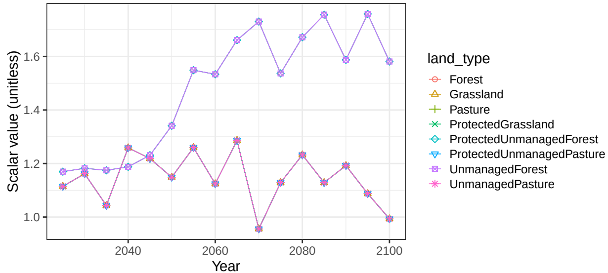
Region Africa_Southern basin AfrCstS non-crop vegetation scalars
