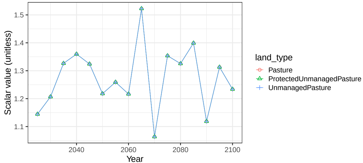
Region South America_Southern basin ArgColoR non-crop vegetation scal
