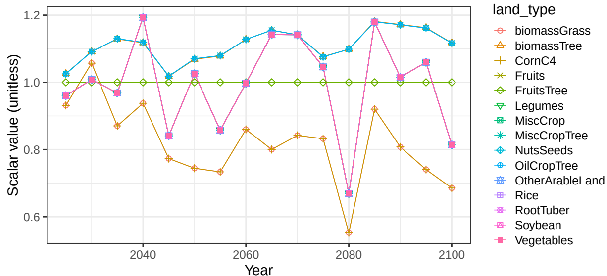
Region Southeast Asia basin JavaTimor crop vegetation scalars
