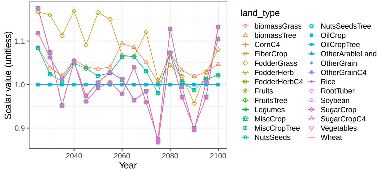
Region EU-15 basin TagusR crop soil scalars
