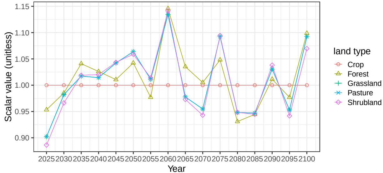
Region Russia basin ScndnvN average soil scalars
