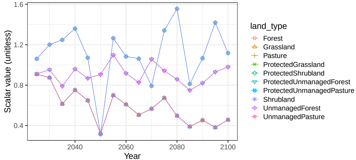
Region Europe_Eastern basin BlackSeaN non-crop vegetation scalars
