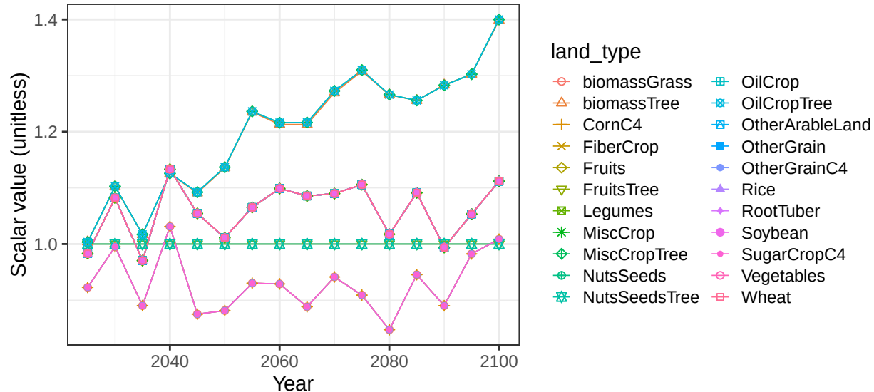
Region Brazil basin SaoFrancR crop soil scalars
