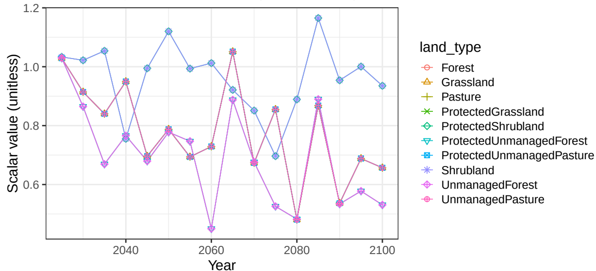
Region Argentina basin Pampas non-crop soil scalars
