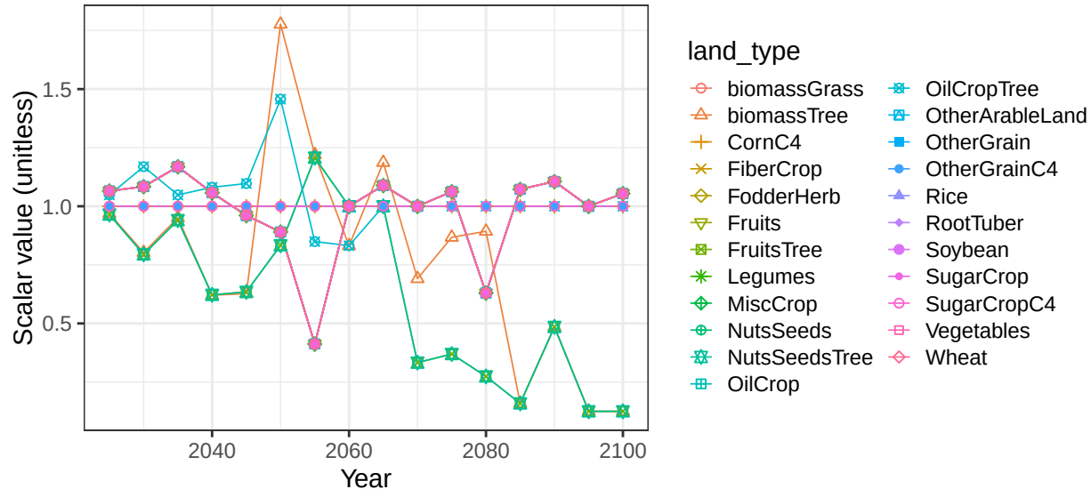
Region Africa_Northern basin NileR crop soil scalars
