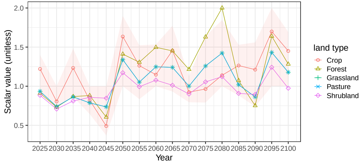
Region China basin LBalkash average vegetation scalars
