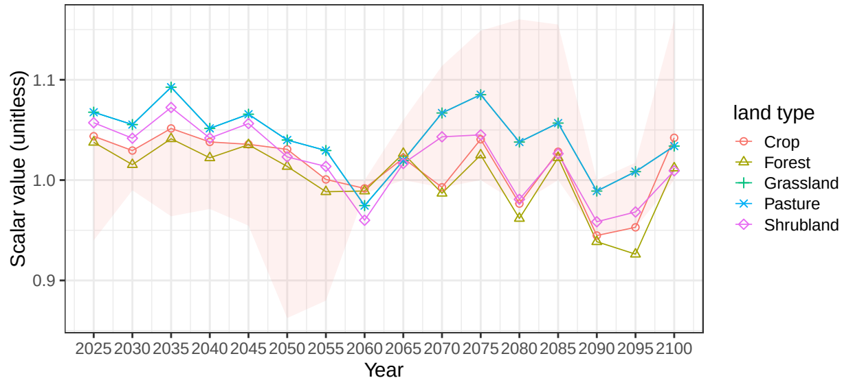
Region Canada basin PacArctic average soil scalars
