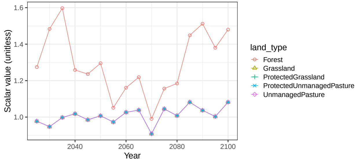
Region EU-15 basin RhineR non-crop vegetation scalars
