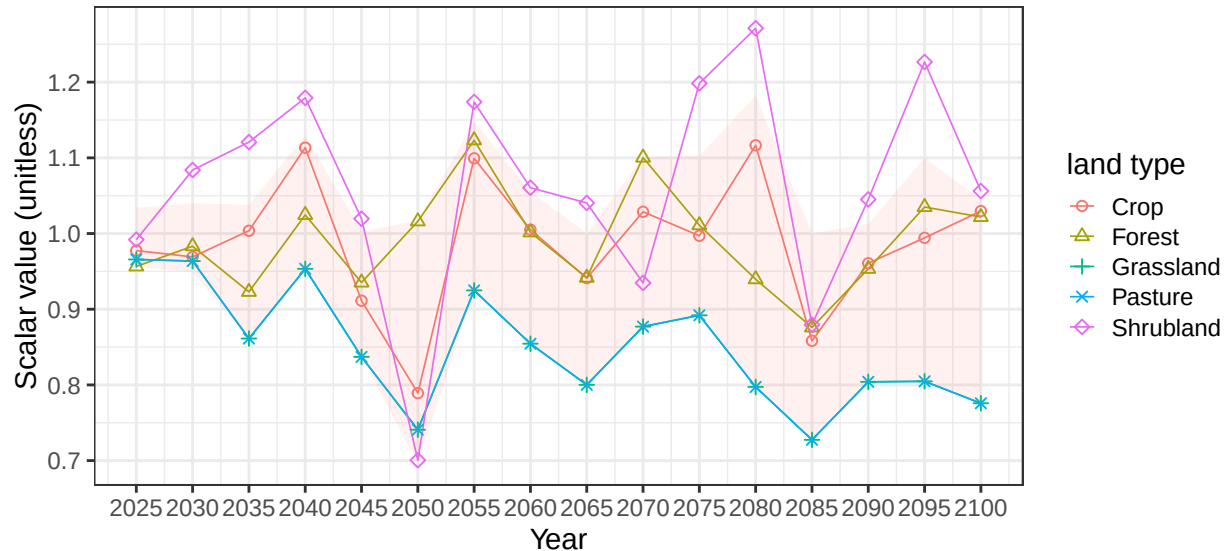
Region Europe_Eastern basin BlackSeaN average soil scalars
