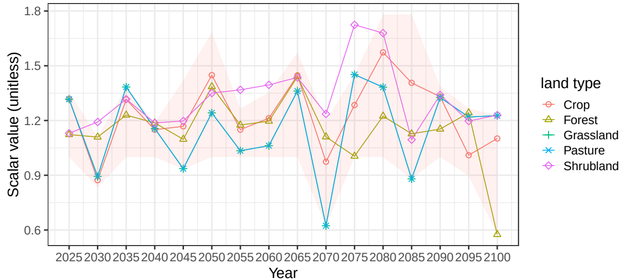
Region Africa_Eastern basin AfrCstE average vegetation scalars
