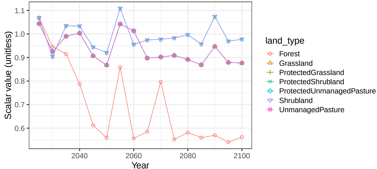
Region EU-15 basin TiberR non-crop soil scalars
