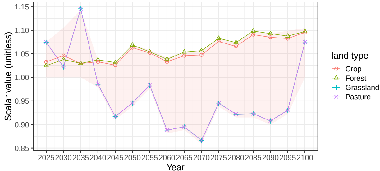
Region Southeast Asia basin BorneoCstN average vegetation scalars
