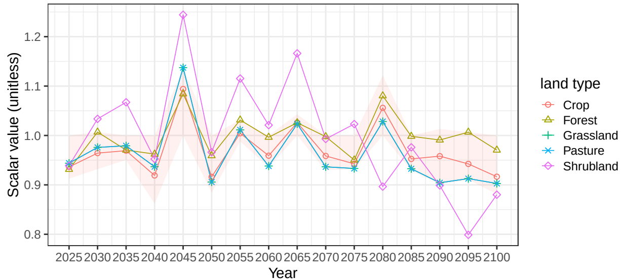
Region Central America and Caribbean basin Caribbean average soil scala
