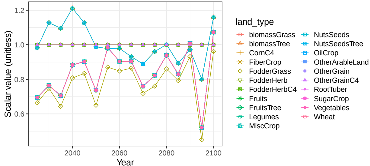
Region EU-12 basin WislaR crop vegetation scalars
