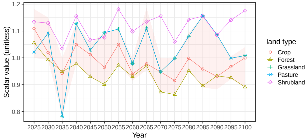
Region EU-15 basin SpainCstSE average soil scalars
