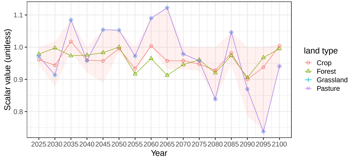
Region Russia basin BalticSea average soil scalars
