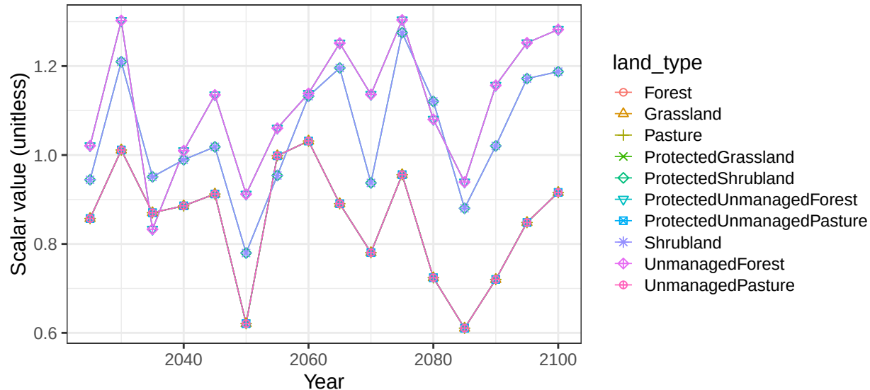
Region Russia basin BlackSeaN non-crop vegetation scalars
