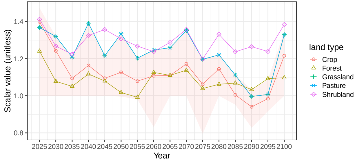
Region EU-15 basin DouroR average vegetation scalars
