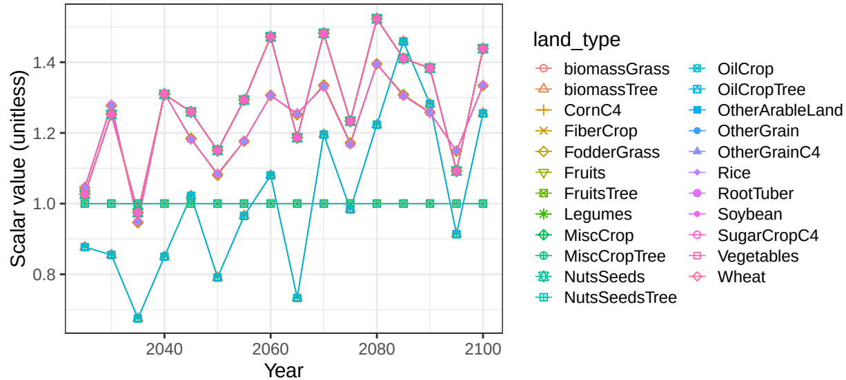
Region India basin TaptiR crop vegetation scalars
