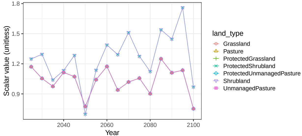
Region Australia_NZ basin AusInt non-crop vegetation scalars
