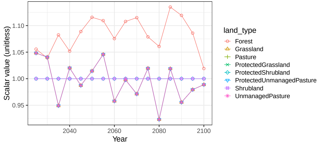
Region China basin SChinaSea non-crop soil scalars
