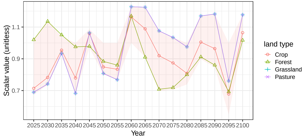
Region Russia basin PolandCst average vegetation scalars
