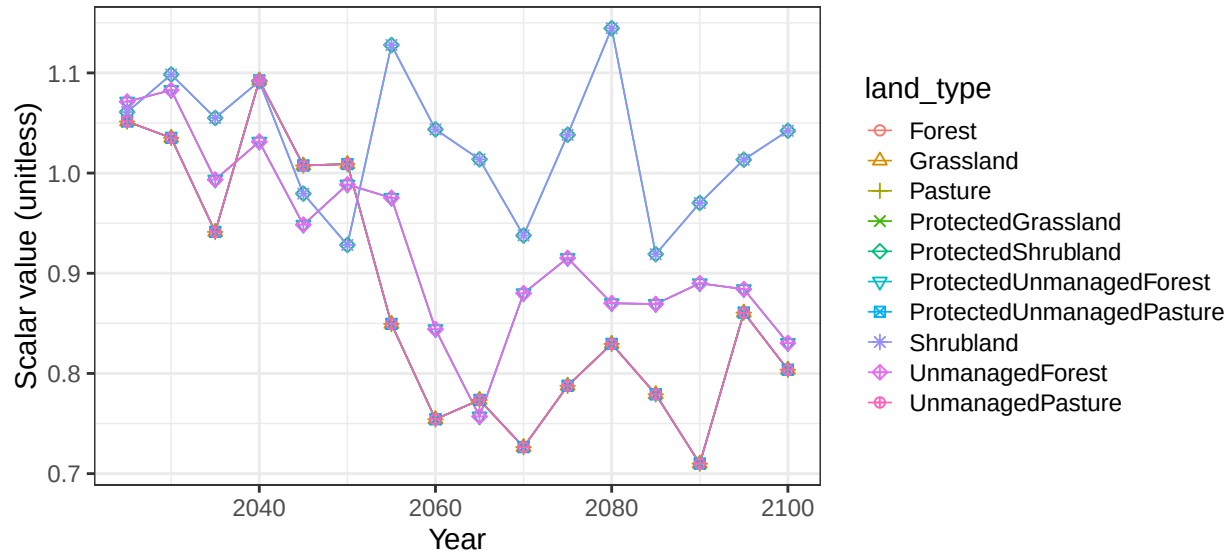
Region EU-12 basin AdrBlkSea non-crop soil scalars
