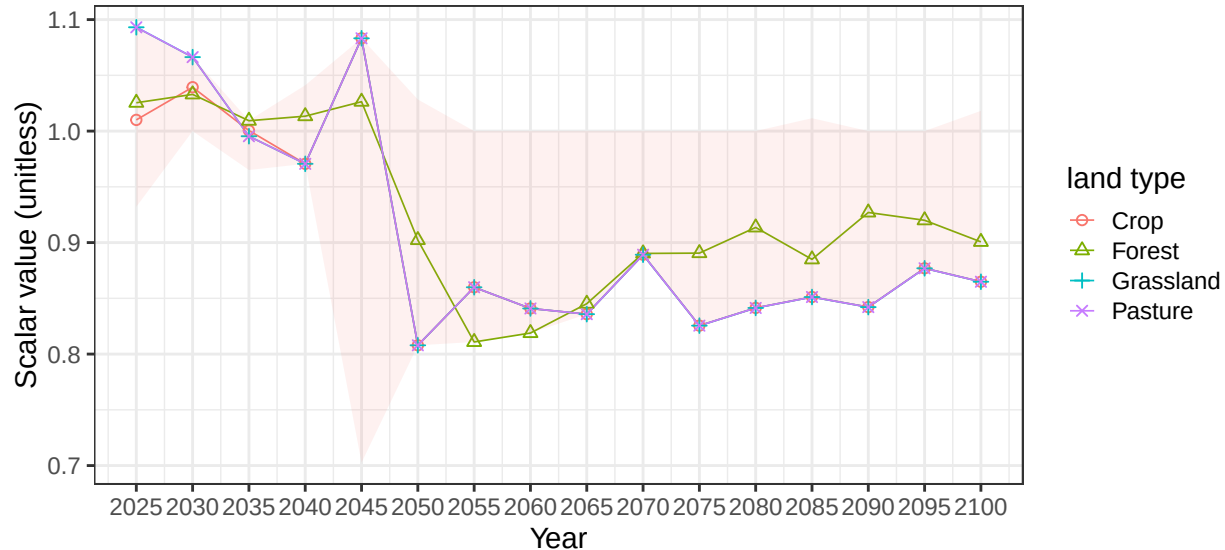
Region Southeast Asia basin SolomonIsl average vegetation scalars
