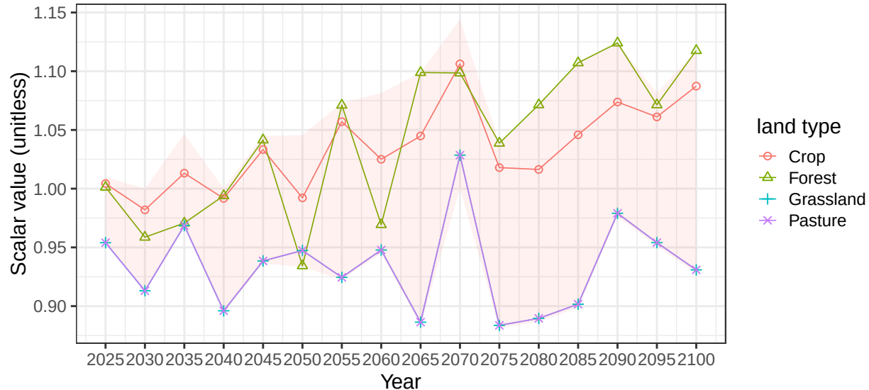
Region South Asia basin SriLanka average vegetation scalars
