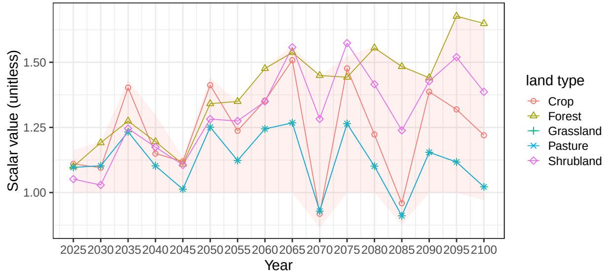
Region Middle East basin CaspianSW average vegetation scalars
