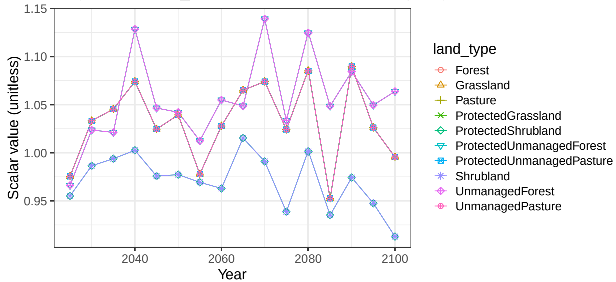
Region Australia_NZ basin Tasmania non-crop vegetation scalars
