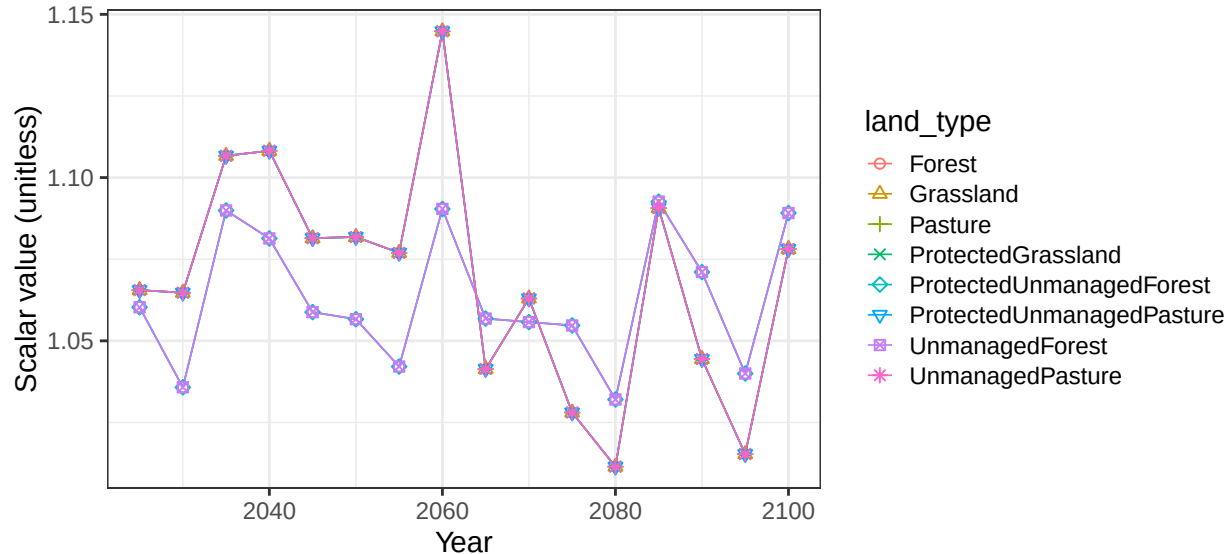
Region Africa_Western basin ZambeziR non-crop soil scalars
