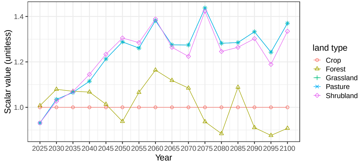
Region EU-15 basin ScndnvN average soil scalars
