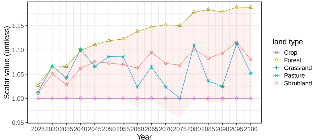
Region Africa_Western basin GuineaGulf average vegetation scalars
