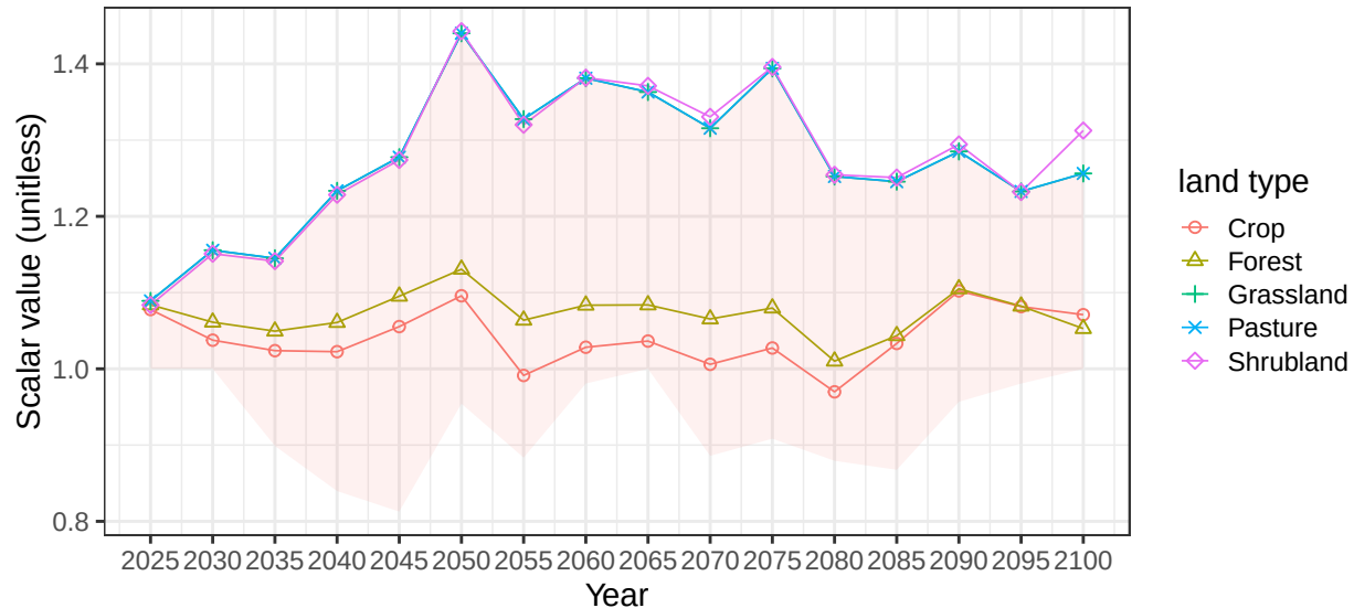
Region European Free Trade Association basin Sweden average soil scalar
