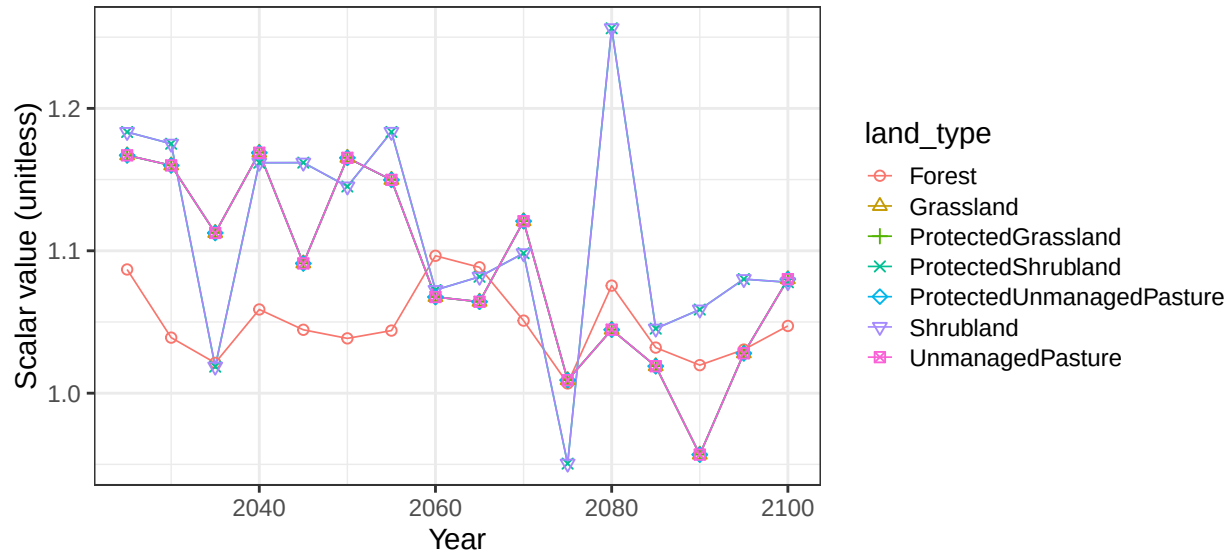
Region EU-15 basin TagusR non-crop soil scalars
