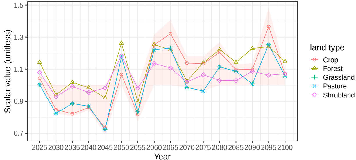
Region Central Asia basin AmurR average vegetation scalars
