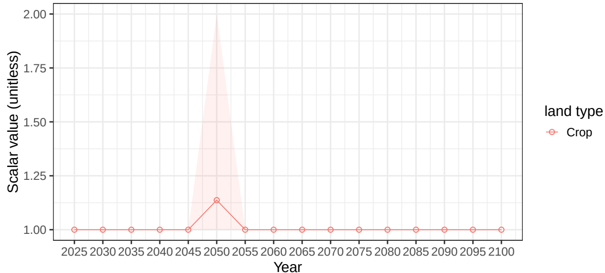
Region Africa_Northern basin SinaiP average vegetation scalars
