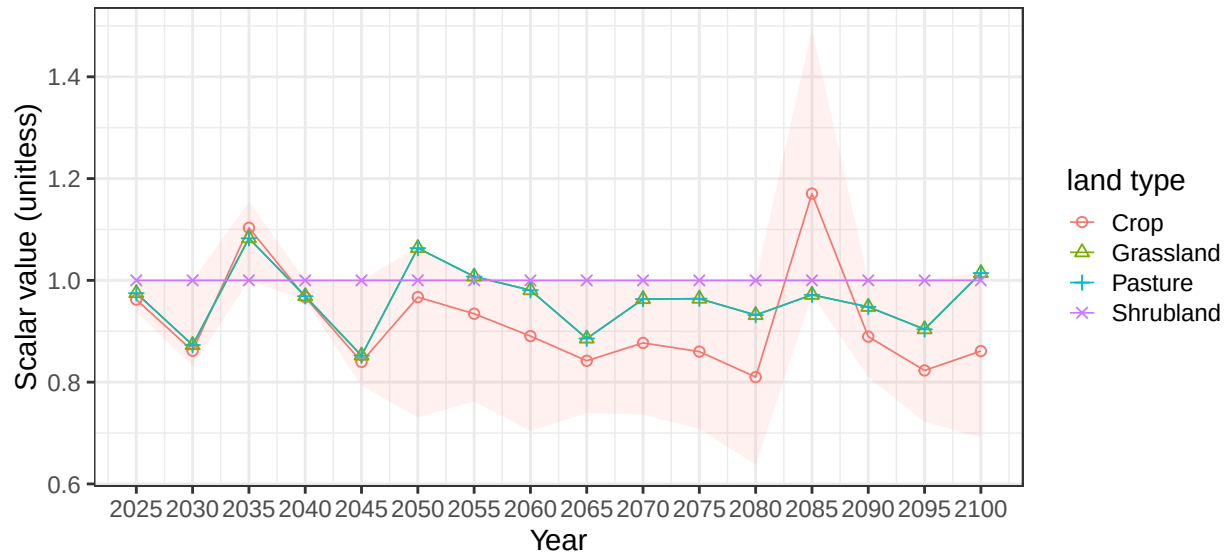
Region Africa_Eastern basin LChad average soil scalars
