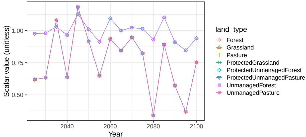
Region EU-12 basin BalticSea non-crop vegetation scalars
