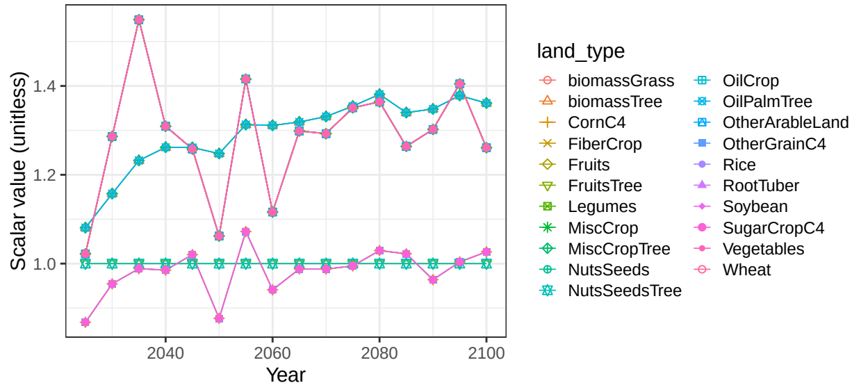
Region Africa_Southern basin GuineaGulf crop vegetation scalars
