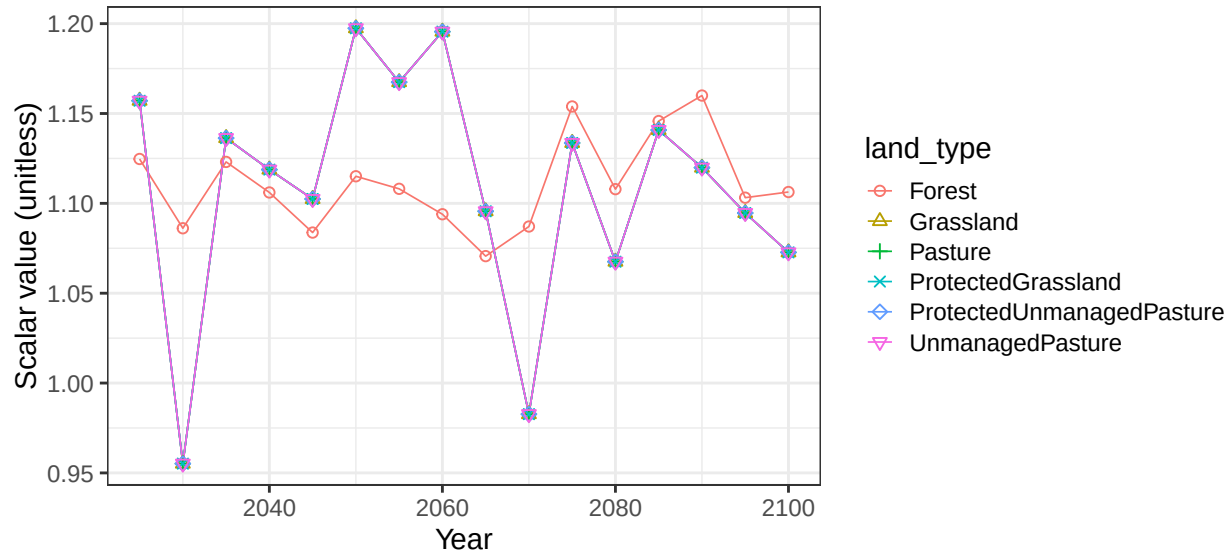
Region Africa_Eastern basin CongoR non-crop vegetation scalars
