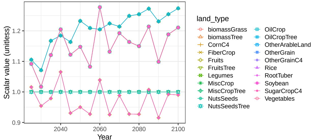
Region Brazil basin ParnaibaR crop soil scalars
