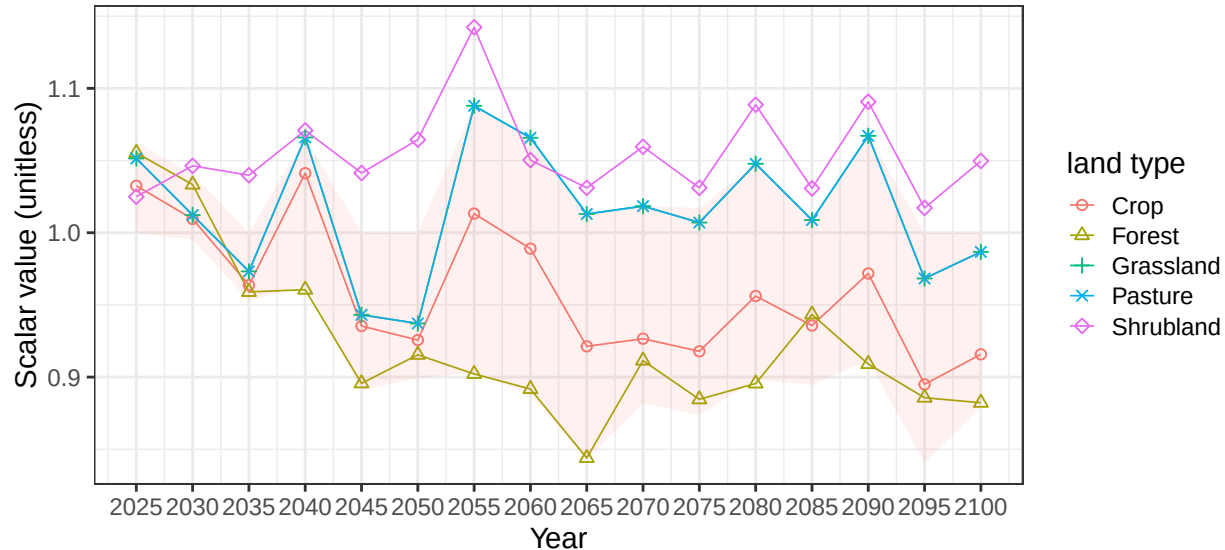
Region EU-15 basin ItalyCstE average soil scalars
