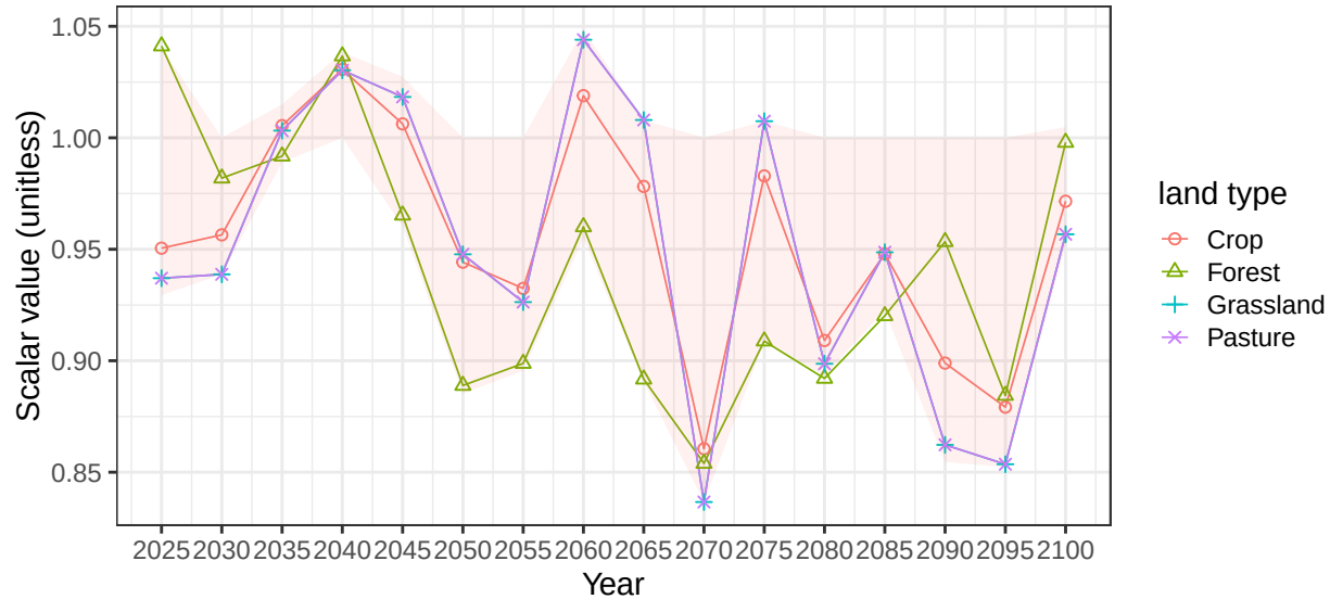
Region EU-15 basin ElbeR average soil scalars
