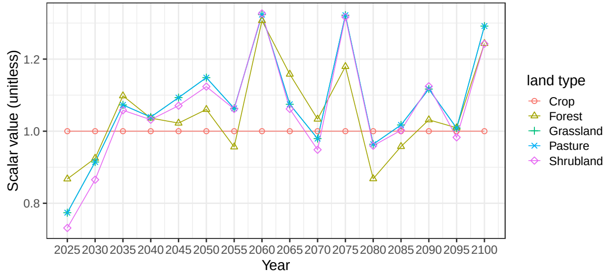
Region Russia basin ScndnvN average vegetation scalars
