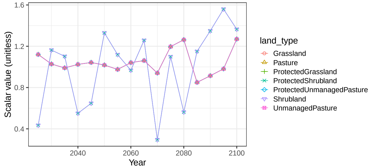
Region Middle East basin RedSeaE non-crop vegetation scalars
