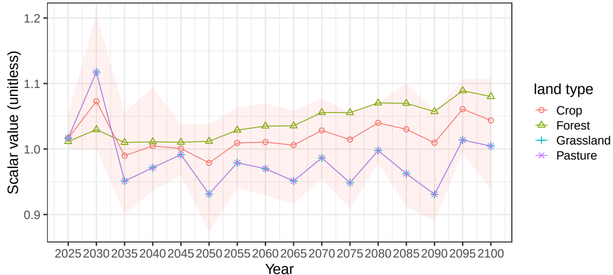
Region Southeast Asia basin SepikR average vegetation scalars
