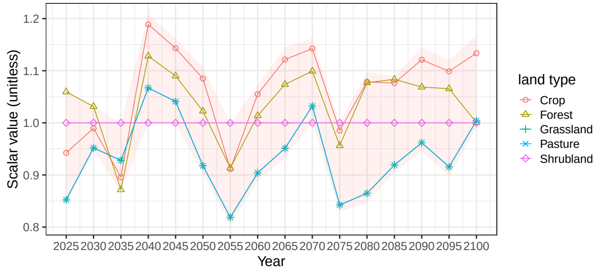
Region Southeast Asia basin SittaungR average vegetation scalars
