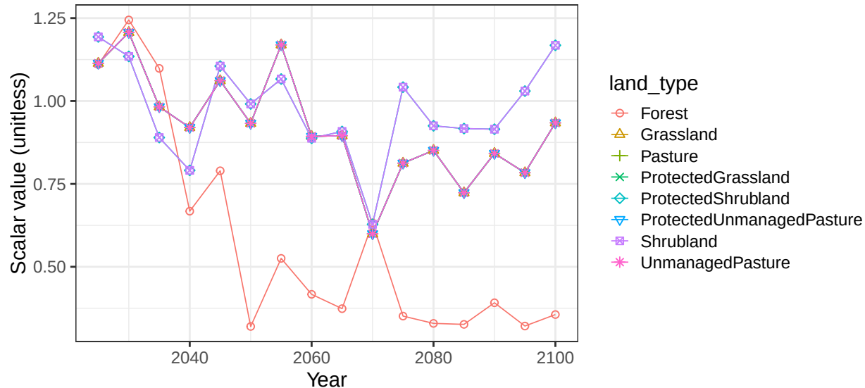
Region Pakistan basin IndusR non-crop vegetation scalars
