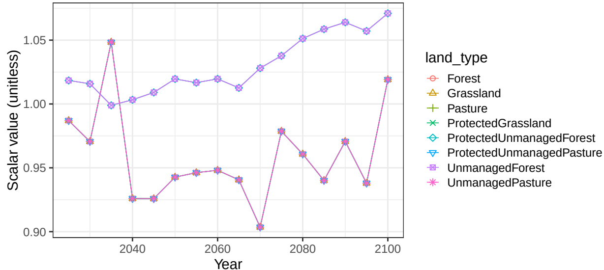
Region Colombia basin AmazonR non-crop vegetation scalars
