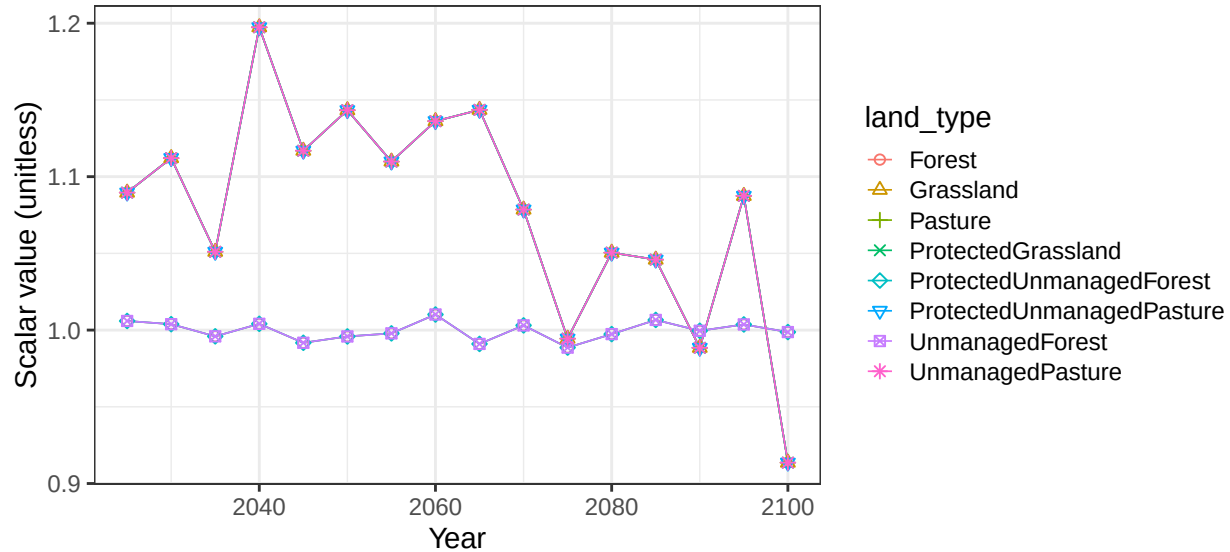
Region South America_Northern basin AmazonR non-crop soil scalars
