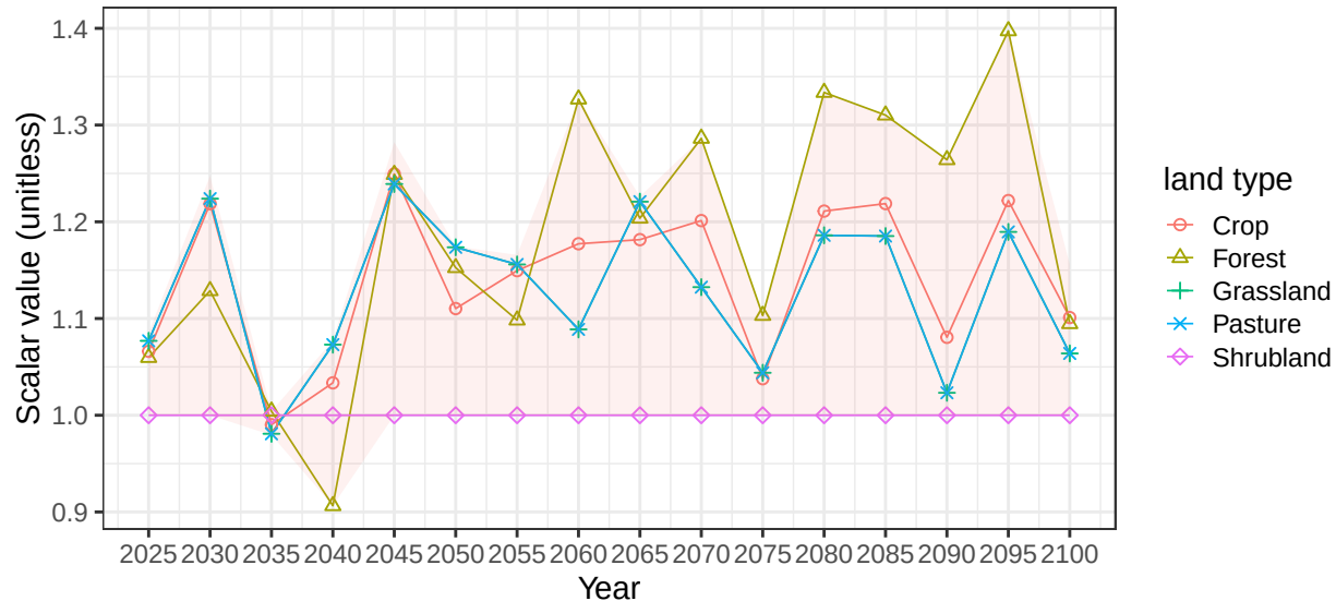
Region India basin KrishnaR average vegetation scalars
