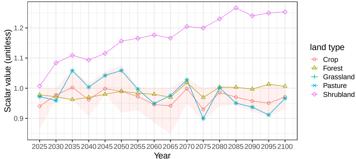
Region Colombia basin OrinocoR average vegetation scalars
