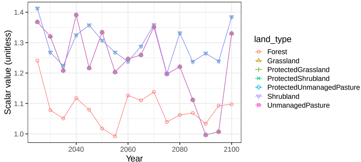
Region EU-15 basin DouroR non-crop vegetation scalars
