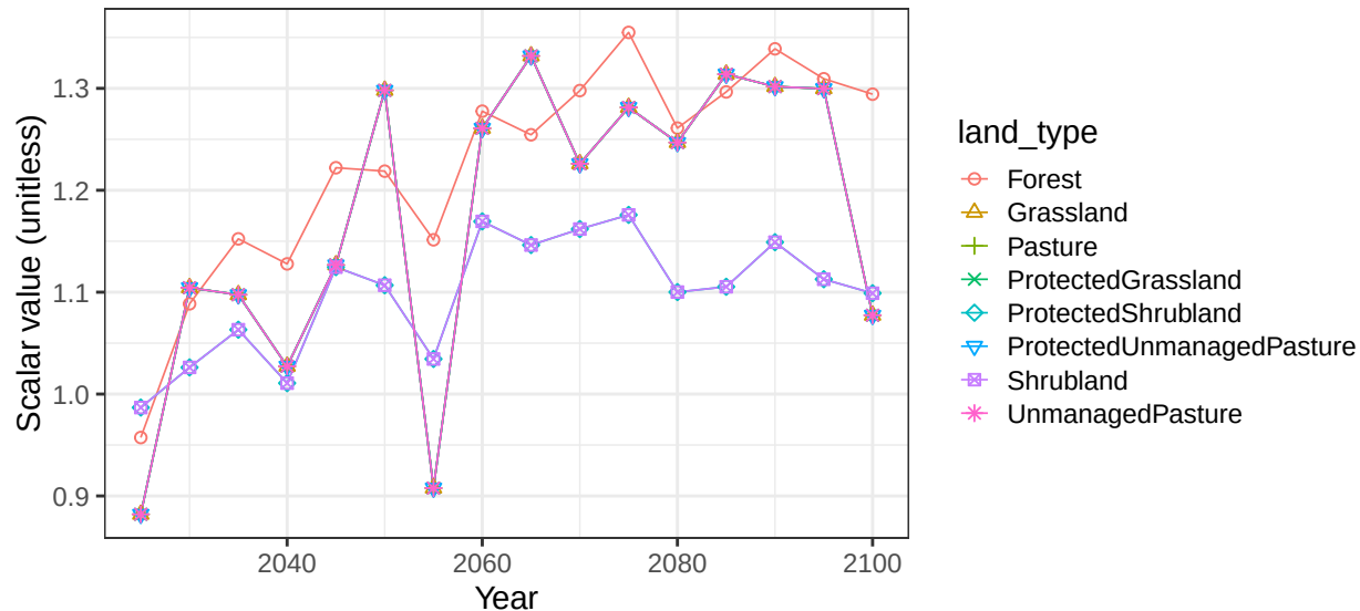
Region China basin AmurR non-crop vegetation scalars
