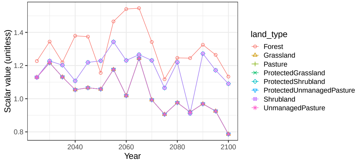
Region Africa_Northern basin MeditS non-crop vegetation scalars
