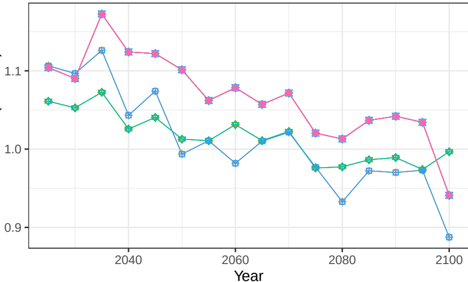
Region Southeast Asia basin Korea crop soil scalars
