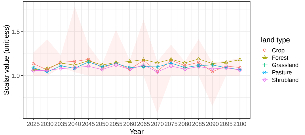
Region South America_Southern basin ChileCstS average vegetation scalar
