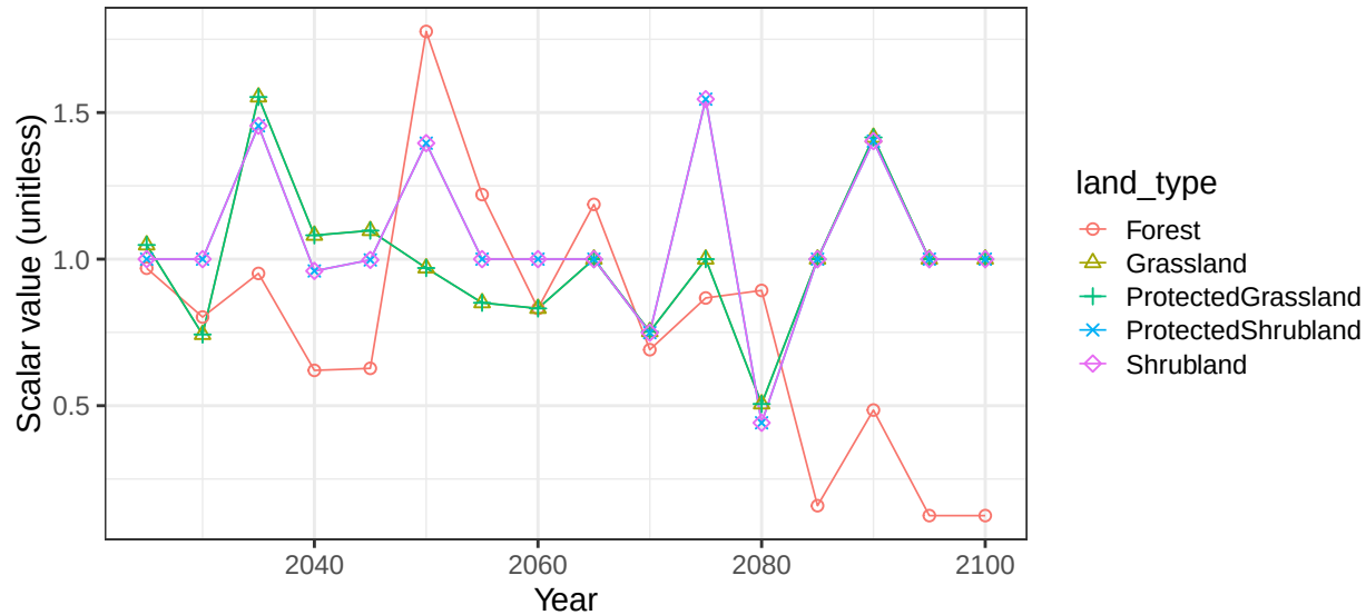
Region Africa_Northern basin NileR non-crop soil scalars
