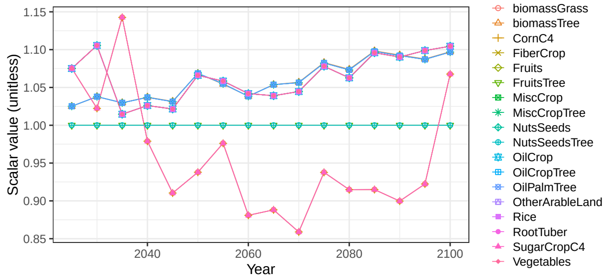
Region Southeast Asia basin BorneoCstN crop vegetation and type
