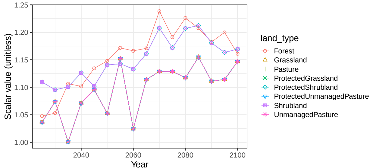
Region China basin XunJiang non-crop vegetation scalars
