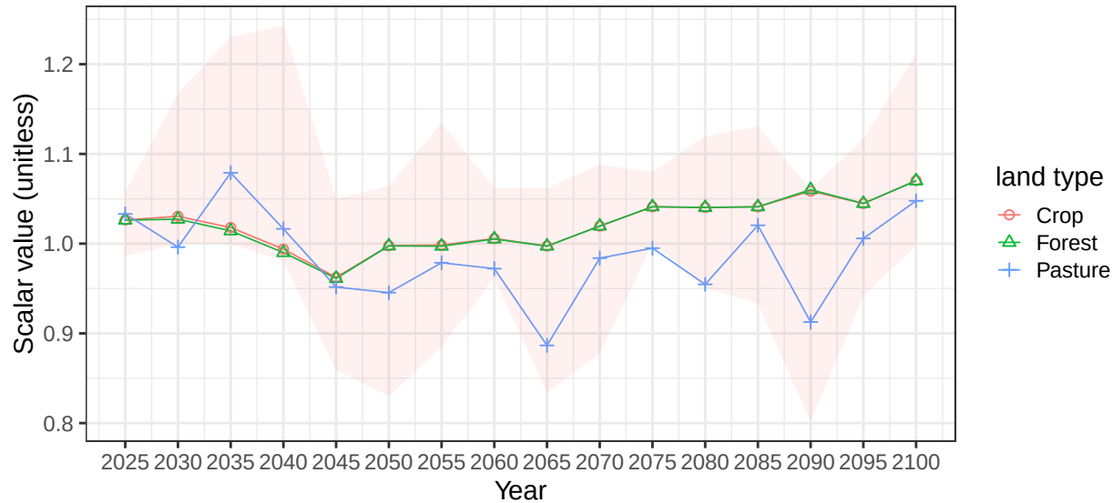
Region Indonesia basin FlyR average vegetation scalars
