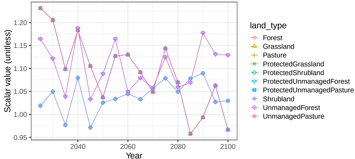
Region Canada basin NelsonR non-crop vegetation scalars
