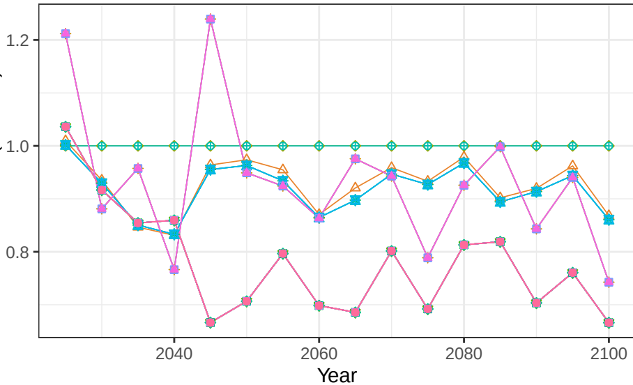
Region Southeast Asia basin NewCaledn crop vegetation scalars
