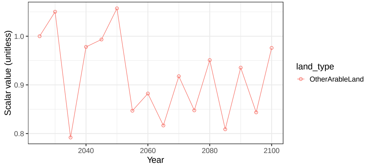
Region USA basin Hawaii crop soil scalars
