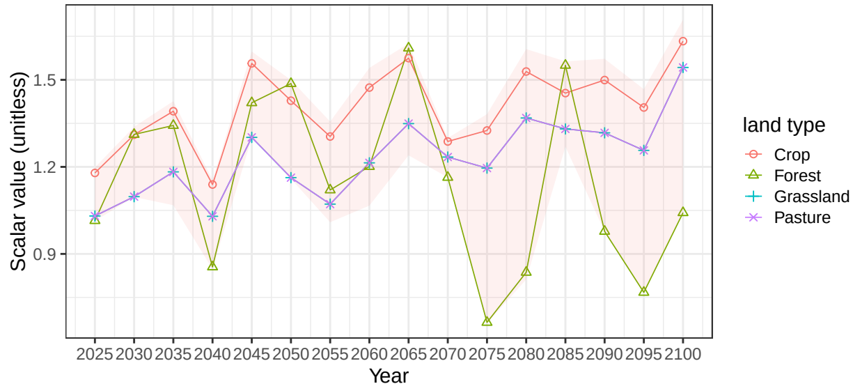
Region India basin BengalW average vegetation scalars
