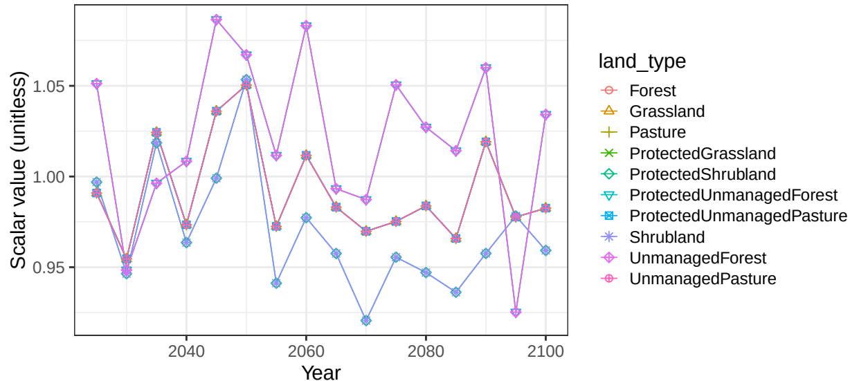
Region Russia basin Gobi non-crop soil scalars
