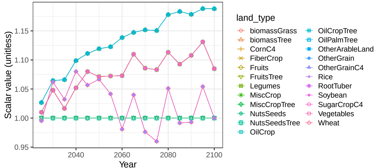
Region Africa_Western basin GuineaGulf crop vegetation scalars
