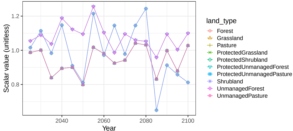
Region Europe_Eastern basin DanubeR non-crop soil scalars
