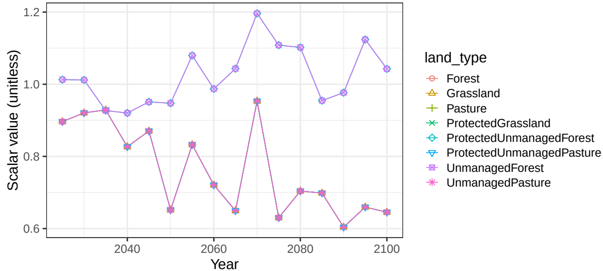
Region Europe_Eastern basin DonR non-crop soil scalars
