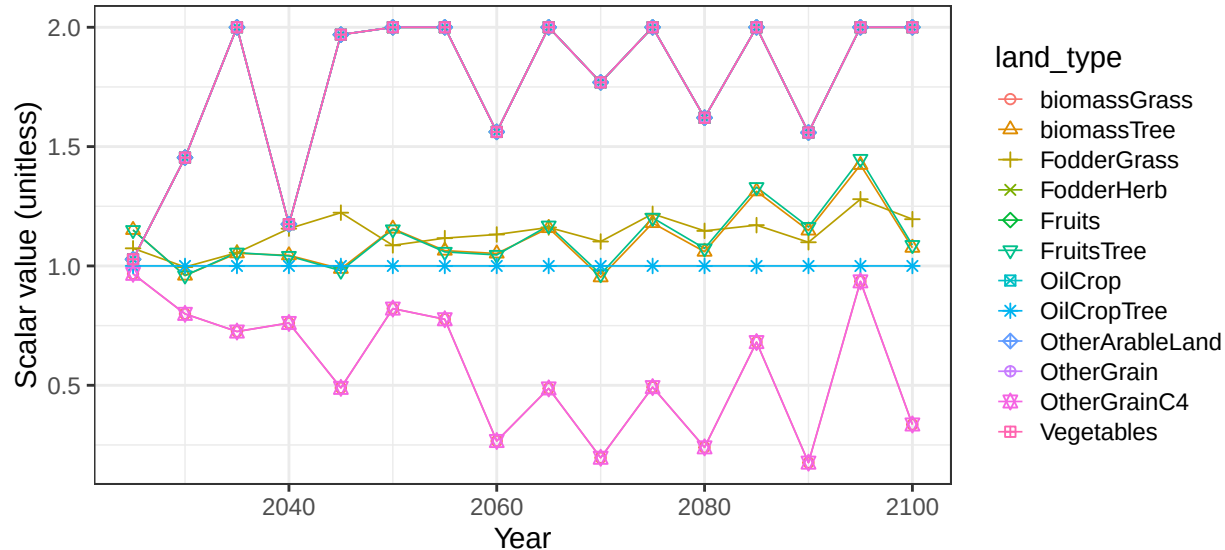
Region Argentina basin Patagonia crop vegetation scalars
