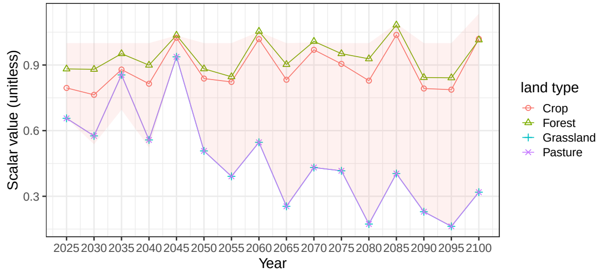
Region EU-12 basin DaugavaR average vegetation scalars
