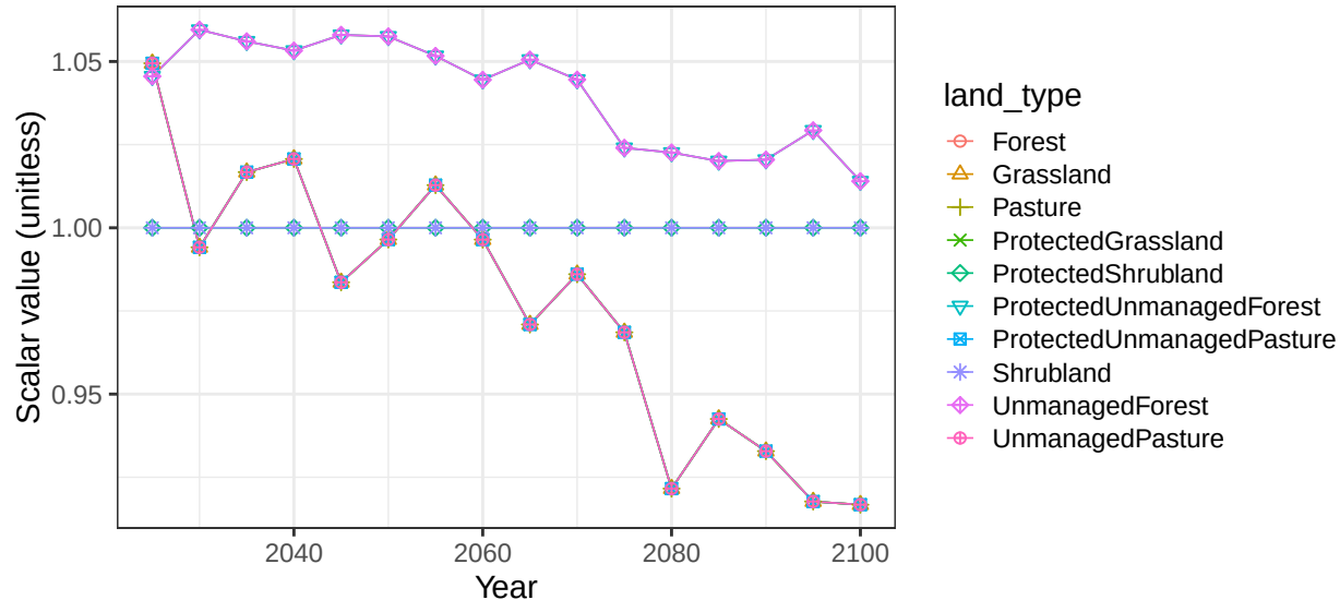
Region Africa_Western basin NileR non-crop soil scalars
