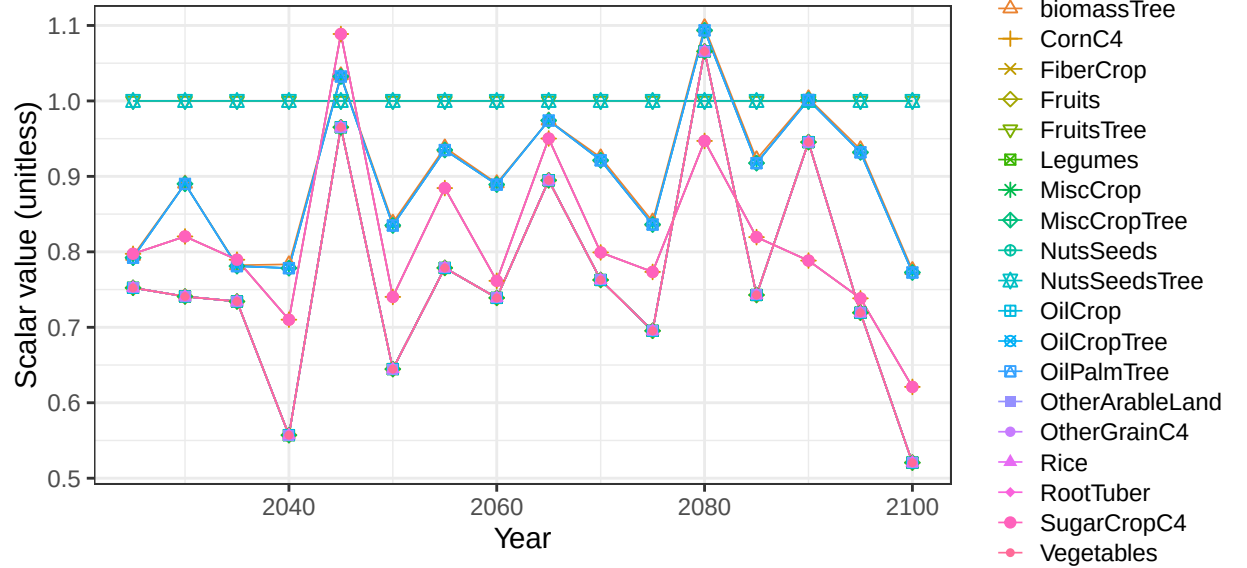
Region Central America and Caribbean basin Caribbean crop vegetation scalar values
