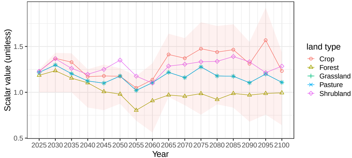
Region USA basin GreatBasin average vegetation scalars
