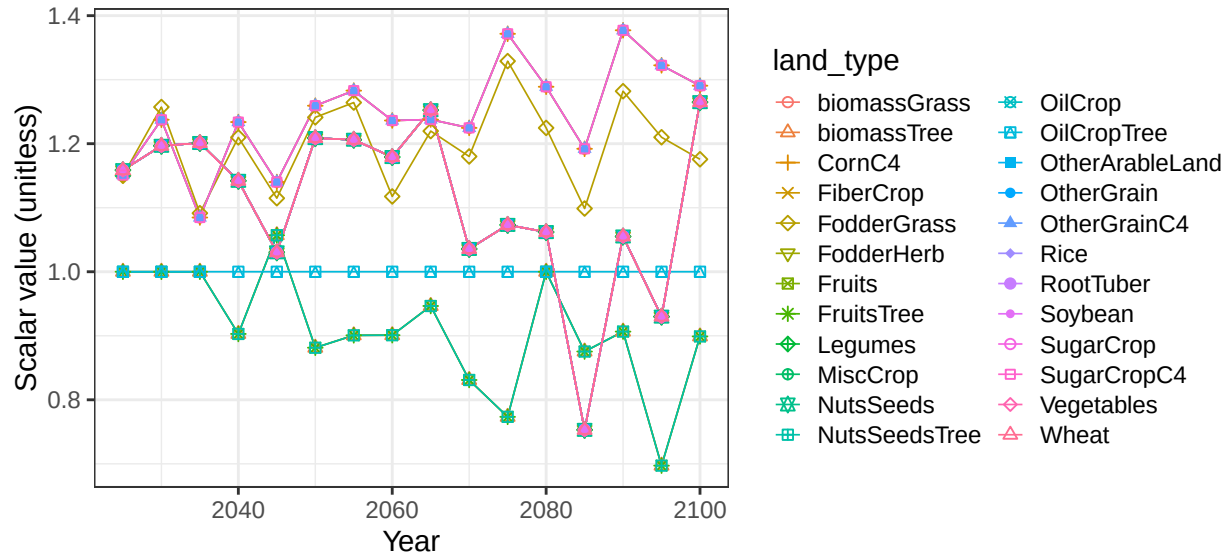
Region Middle East basin CaspianE crop soil scalars
