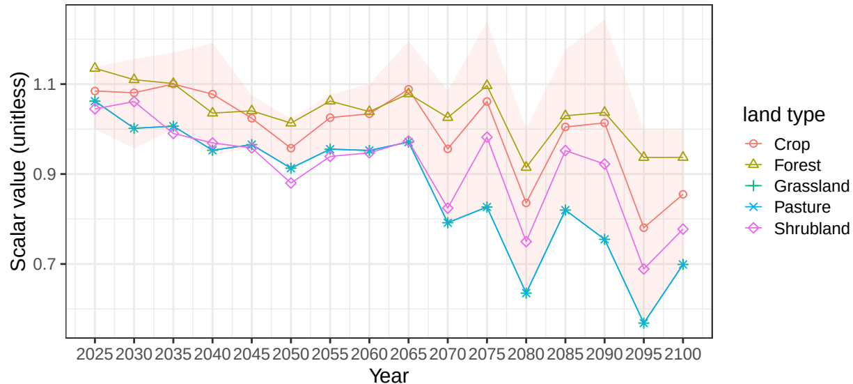
Region USA basin ArkWhtRedR average soil scalars
