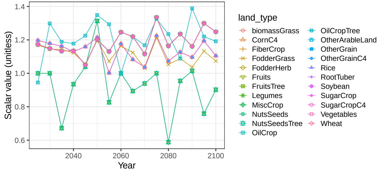
Region Middle East basin PersianGulf crop soil scalars
