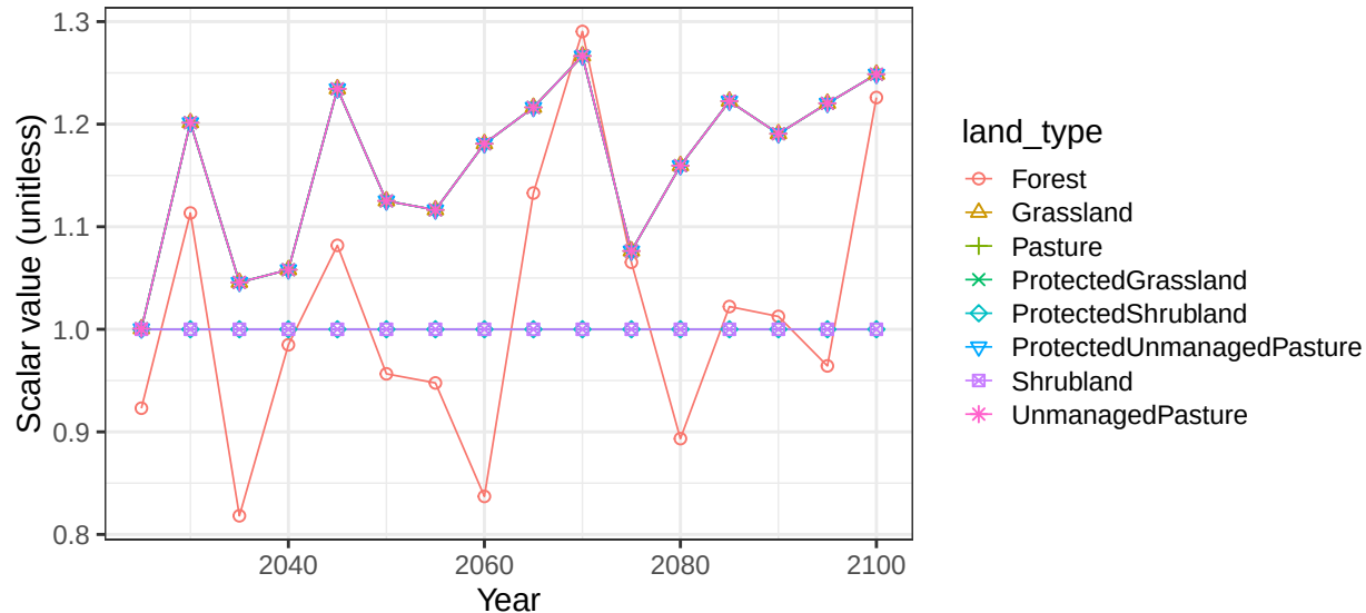
Region India basin CauveryR non-crop vegetation scalars
