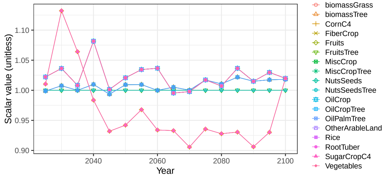
Region Southeast Asia basin Kalimantan crop soil scalarsland_type
