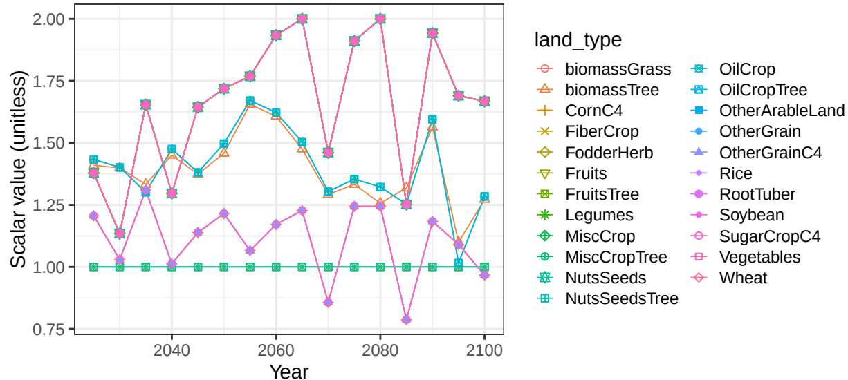
Region Africa_Eastern basin ShebJubR crop vegetation scalars
