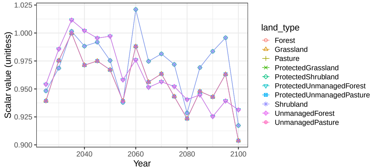
Region Canada basin CanAtl non-crop soil scalars
