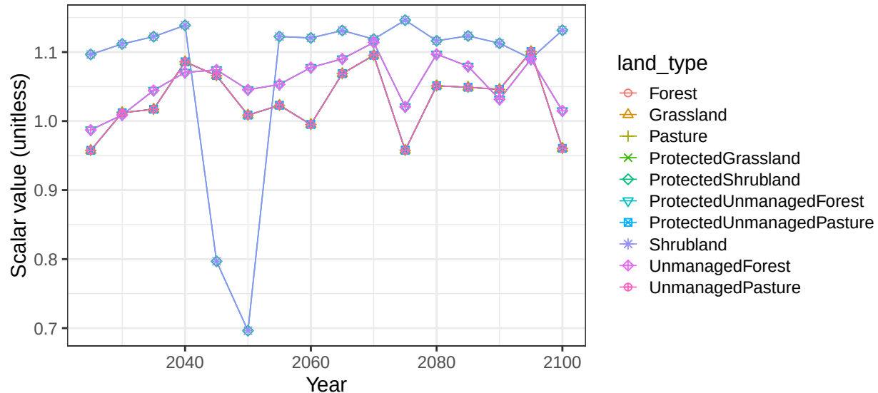
Region South America_Northern basin SAmerCstN non-crop soil scalars
