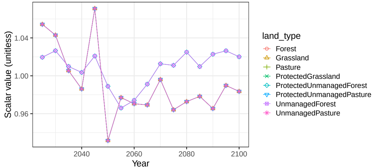
Region Southeast Asia basin SolomonIs non-crop soil scalars
