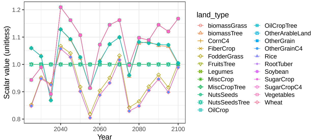
Region Southeast Asia basin SittaungR crop vegetation scalars
