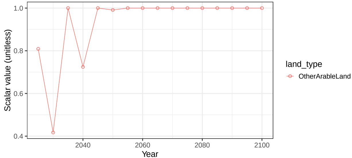
Region Africa_Northern basin DeadSea crop vegetation scalars
