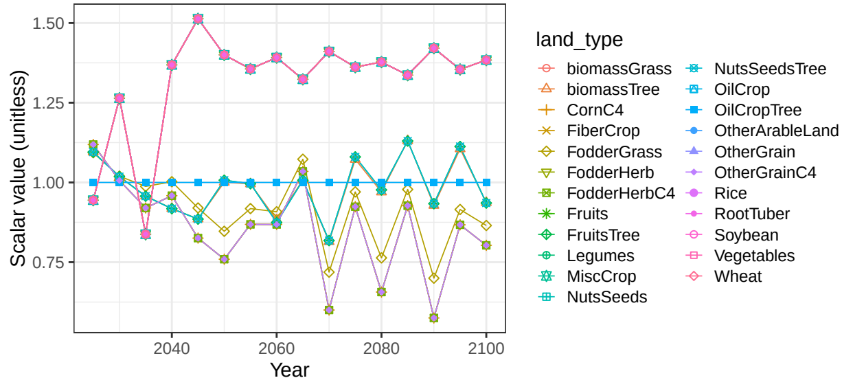
Region Argentina basin ArgColoR crop soil scalars
