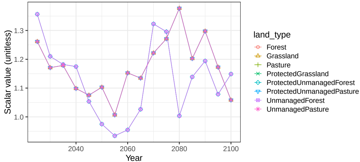
Region USA basin MissppRN non-crop vegetation scalars
