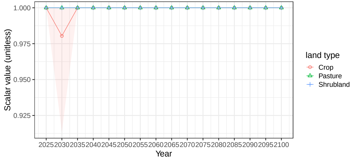
Region Middle East basin AfrCstNE average soil scalars
