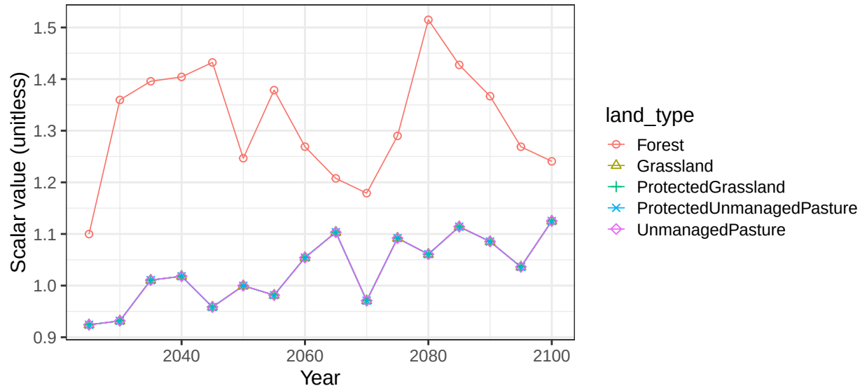
Region EU-15 basin EmsWeserR non-crop soil scalars
