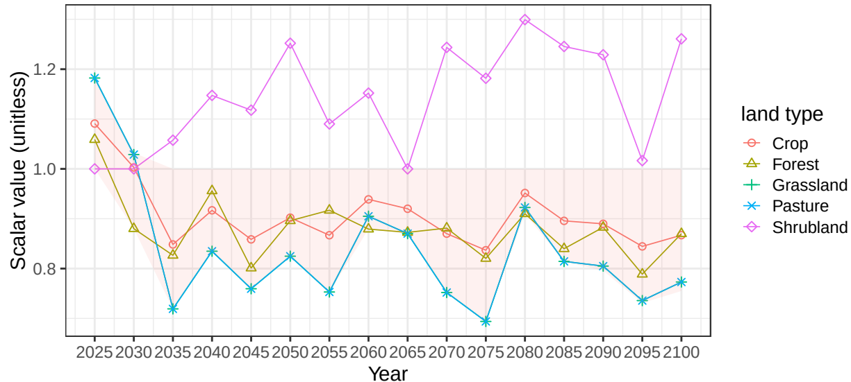
Region USA basin MexCstNW average soil scalars
