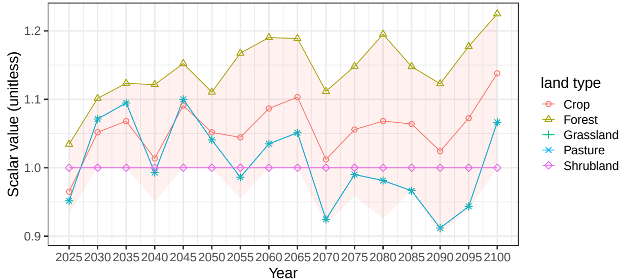
Region Mexico basin Tehuantpc average vegetation scalars
