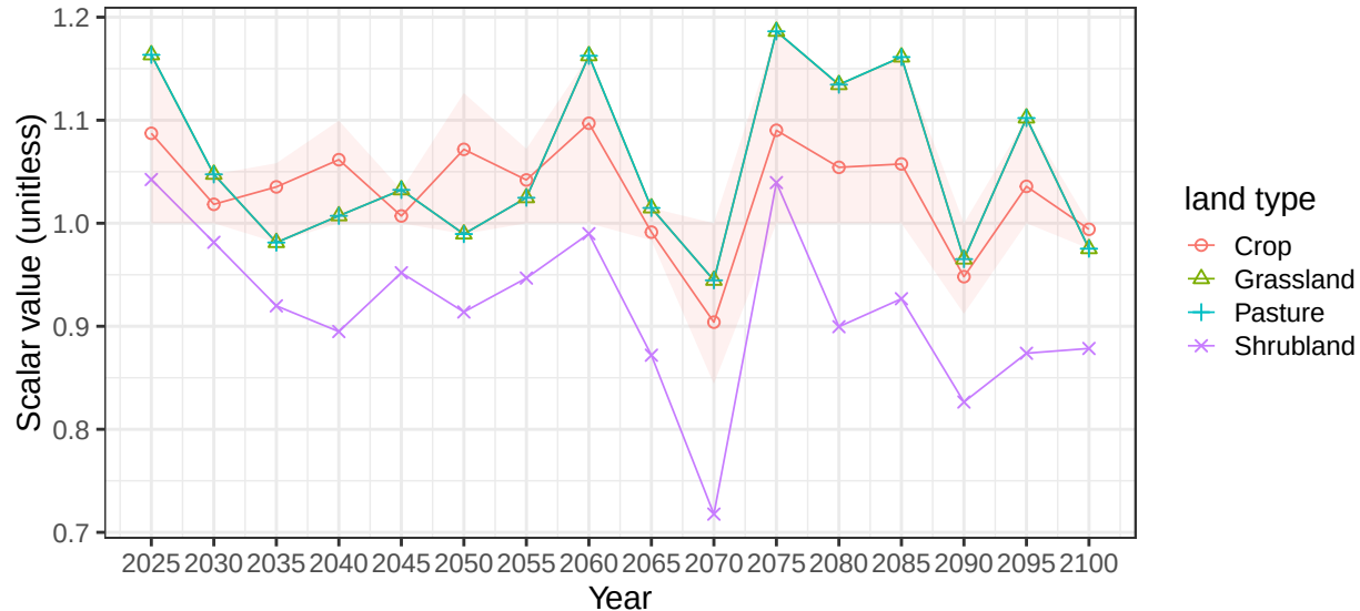
Region Middle East basin FarahrudR average soil scalars
