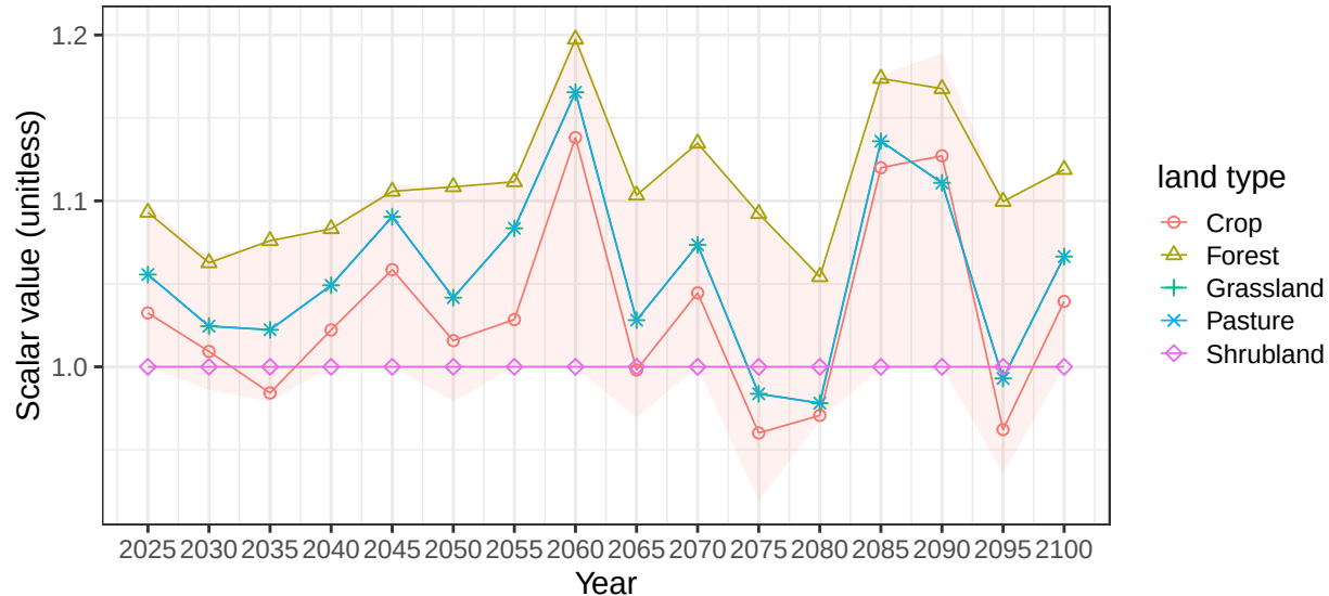
Region Africa_Southern basin ZambeziR average soil scalars
