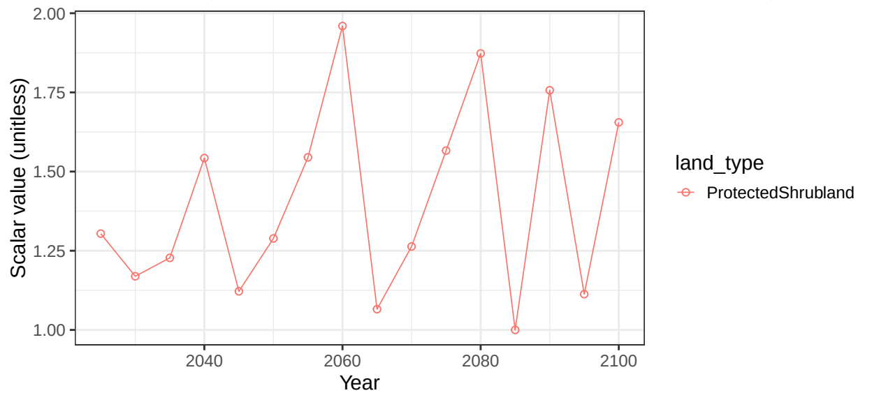
Region European Free Trade Association basin ArcticIsI non-crop vegetati
