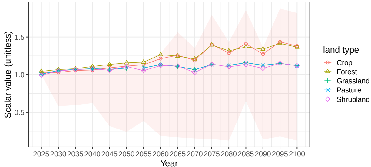
Region Argentina basin ArgCstS average vegetation scalars
