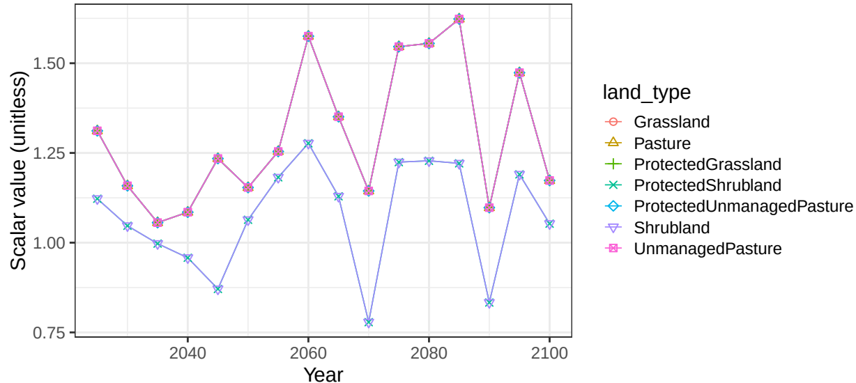
Region Middle East basin FarahrudR non-crop vegetation scalars
