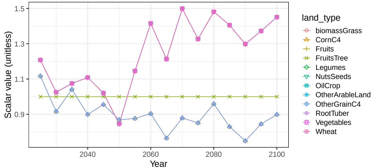
Region Africa_Southern basin AfrCstSW crop soil scalars
