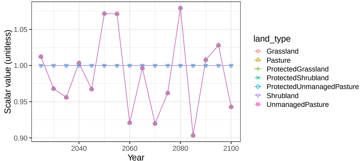
Region Africa_Eastern basin AfrIntN non-crop soil scalars
