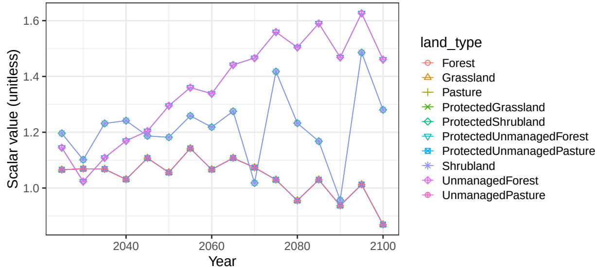
Region Argentina basin NegroR non-crop vegetation scalars
