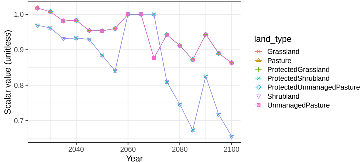
Region Middle East basin HamuMashR non-crop soil scalars
