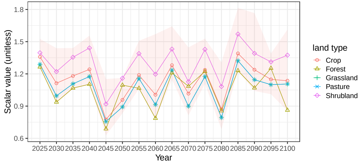
Region Mexico basin RioGrande average vegetation scalars
