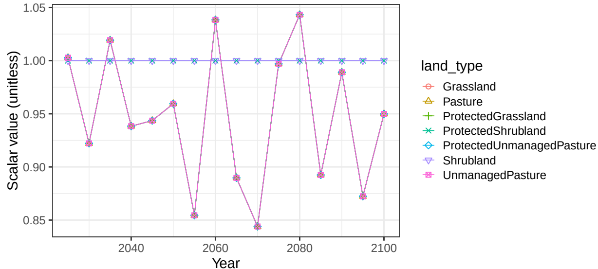
Region Africa_Western basin AfrCstNW non-crop soil scalars
