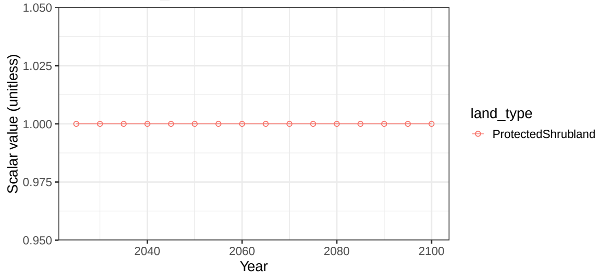
Region Africa_Northern basin LChad non-crop soil scalars
