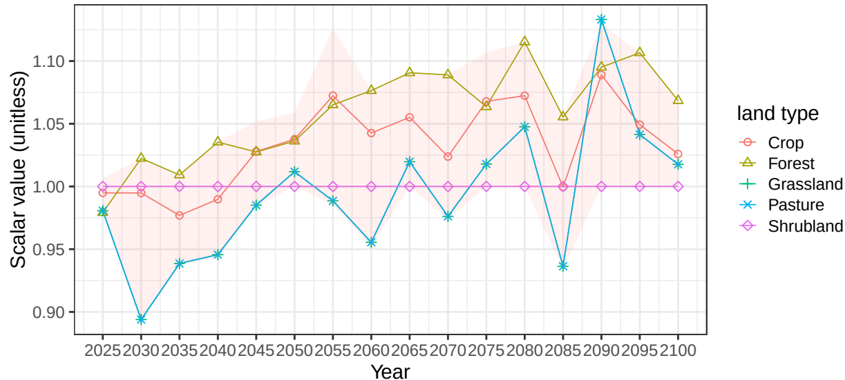
Region Africa_Western basin AfrCstW average vegetation scalars
