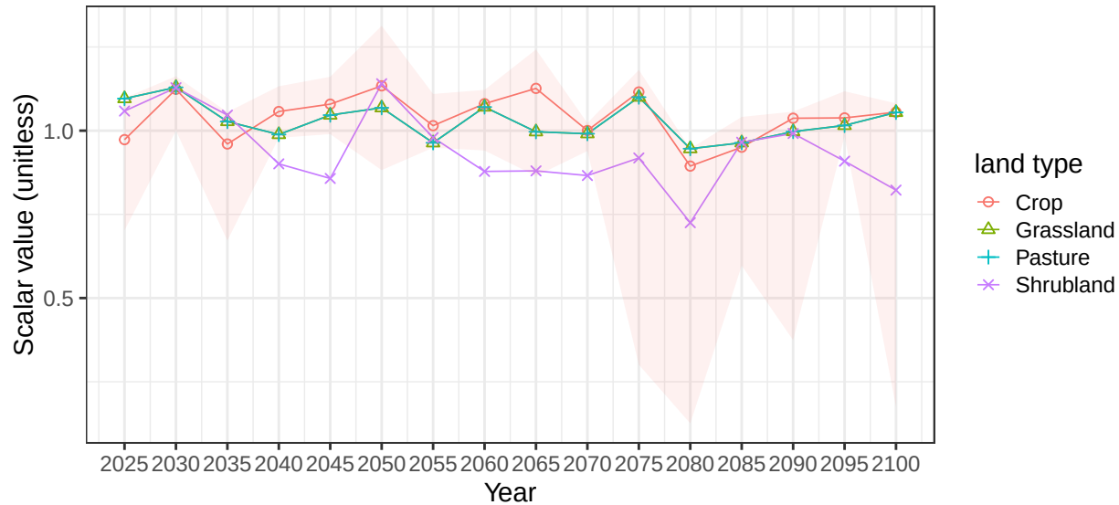
Region Middle East basin ArabianP average soil scalars
