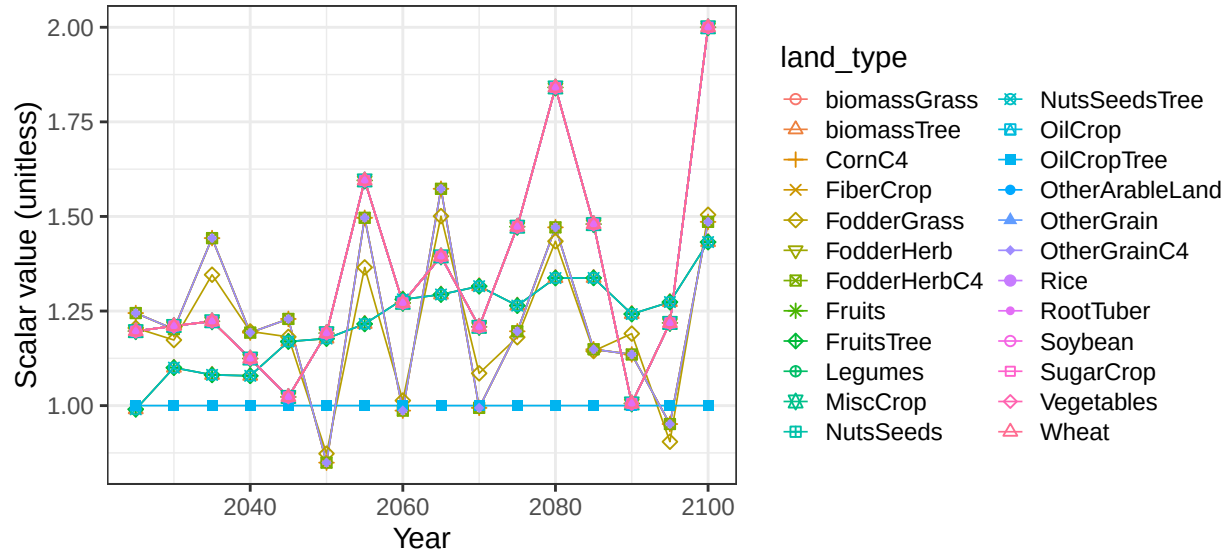
Region Central Asia basin CaspianNE crop vegetation scalars
