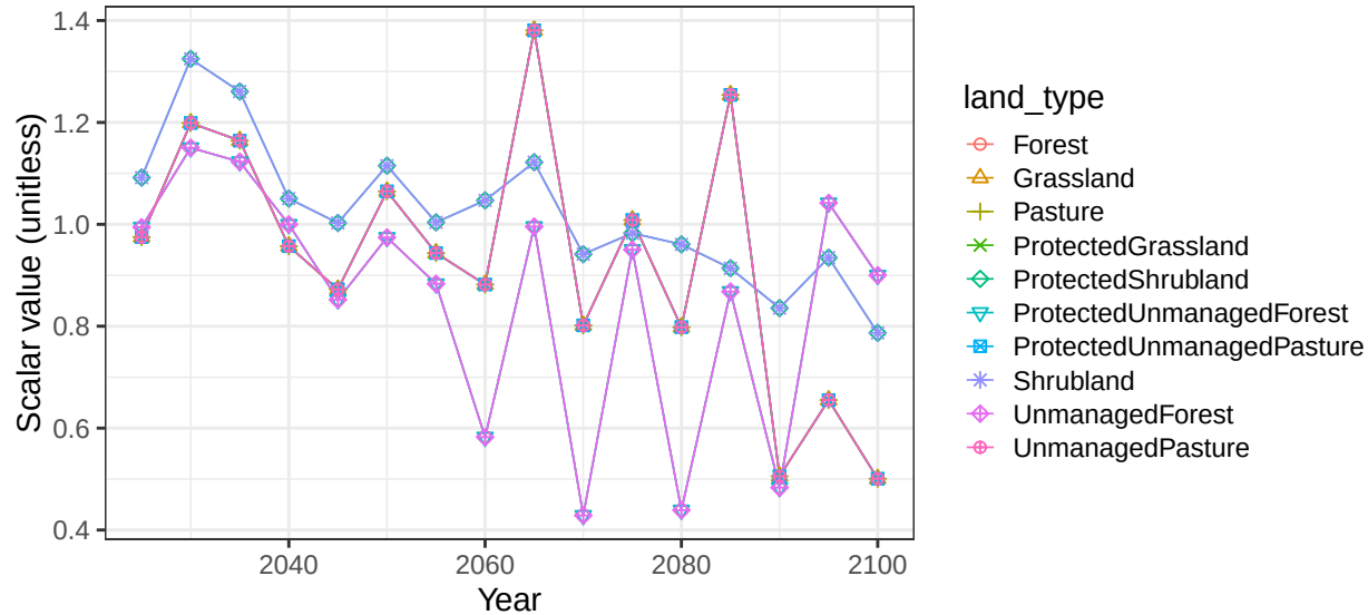
Region Argentina basin MarChiq non-crop vegetation scalars
