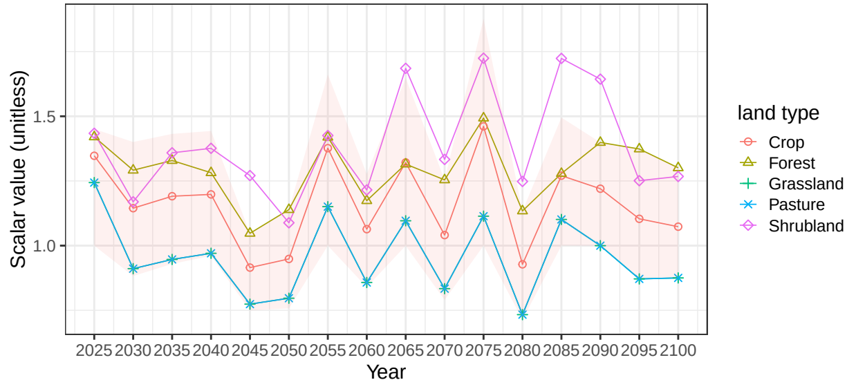
Region USA basin TexasCst average vegetation scalars
