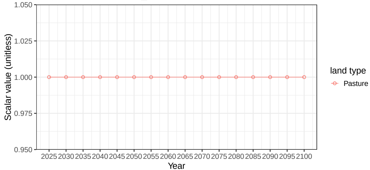
Region South America_Southern basin Salinas average vegetation scalar
