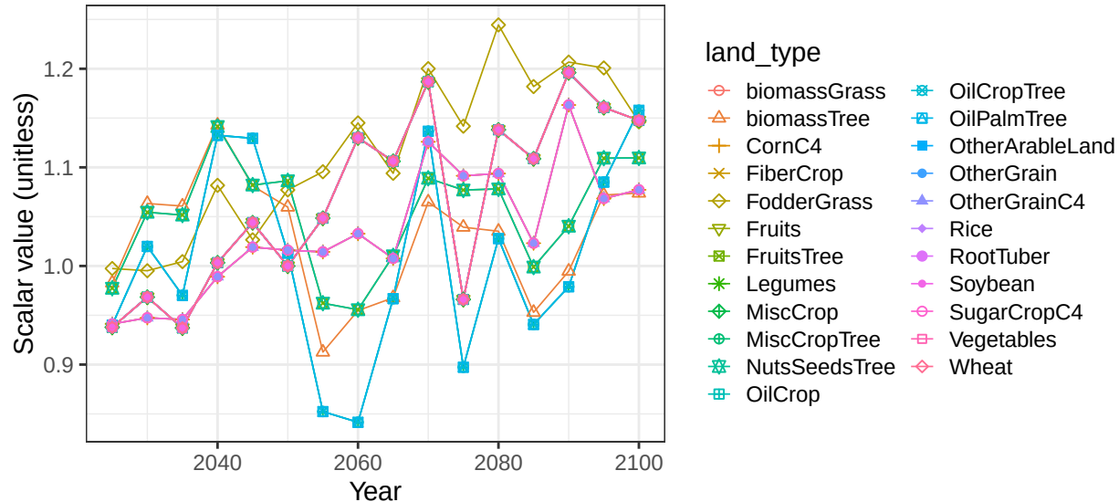
Region China basin GangesR crop vegetation scalars
