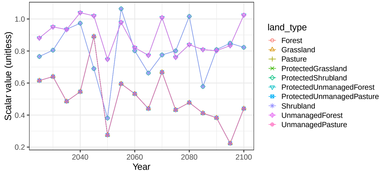
Region Europe_Eastern basin DnieperR non-crop vegetation scalars
