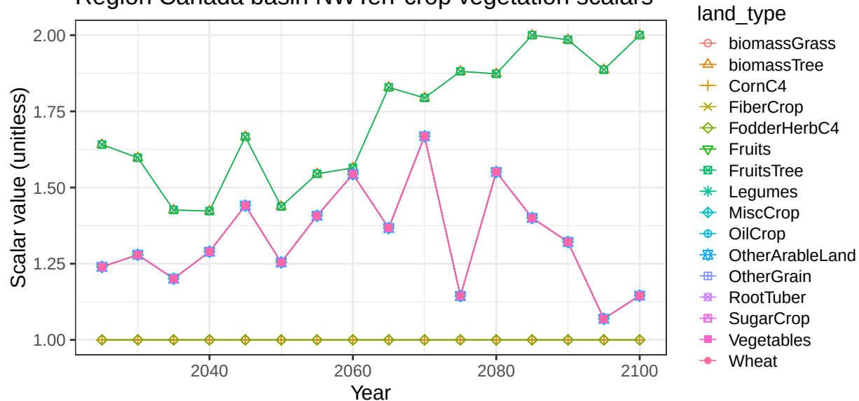
Region Canada basin NWTerr crop vegetation scalars
