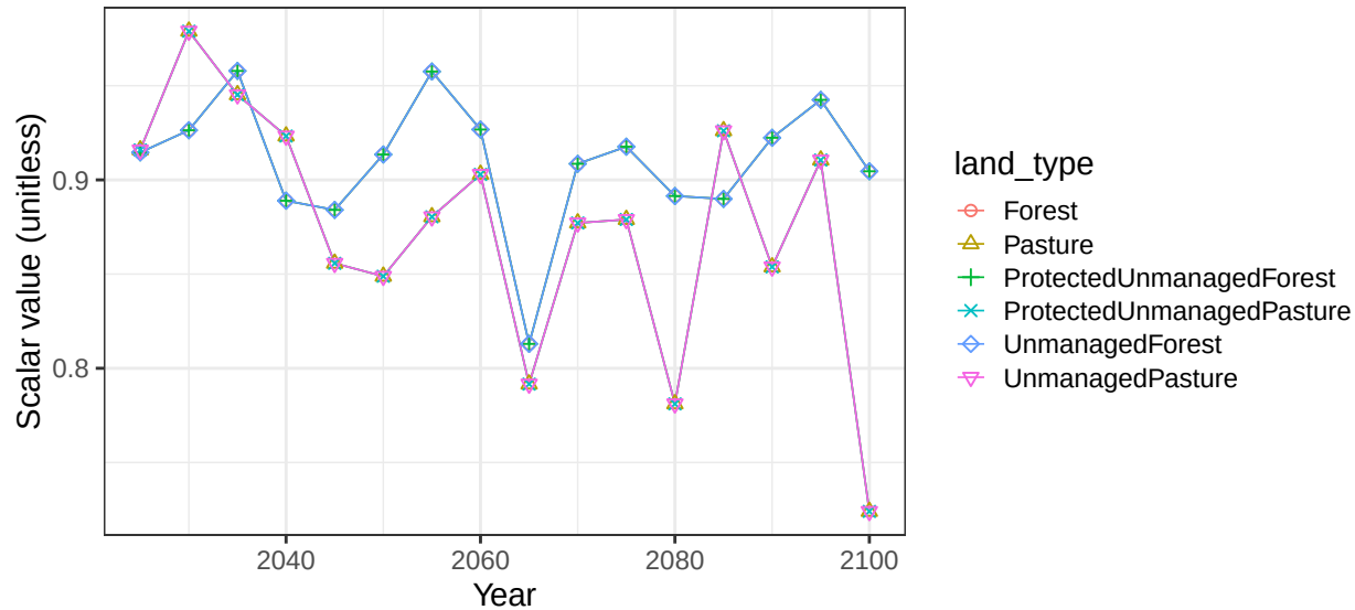
Region Southeast Asia basin IdnE non-crop soil scalars
