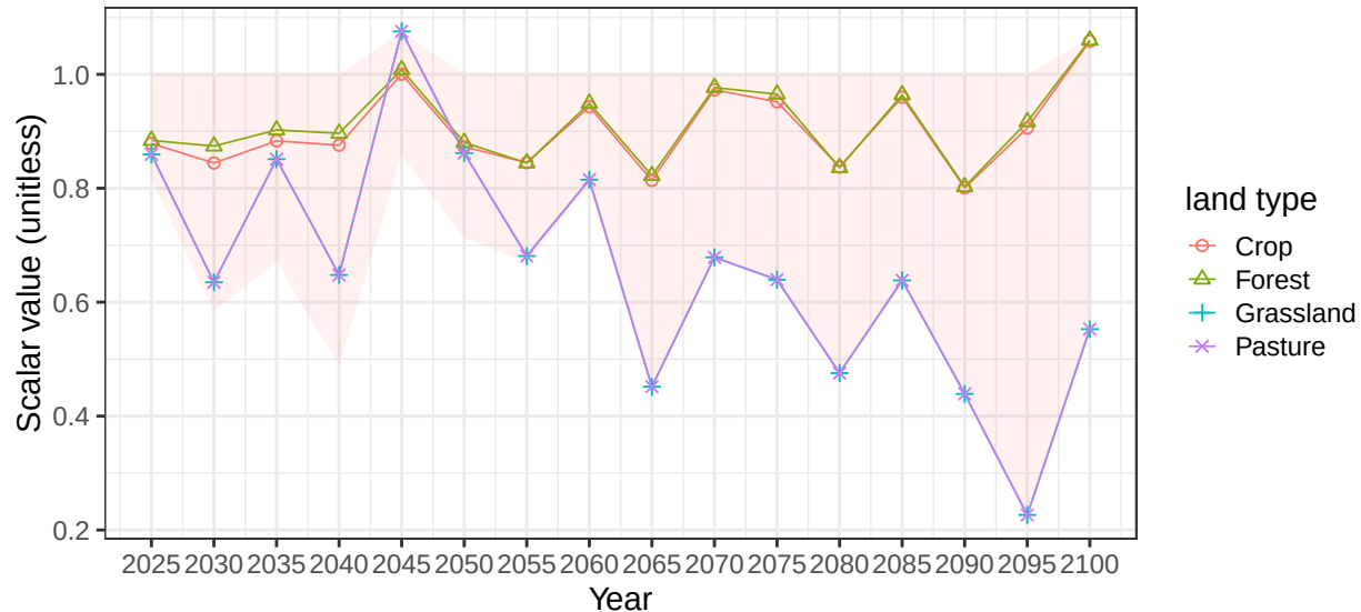
Region Russia basin NarvaR average vegetation scalars
