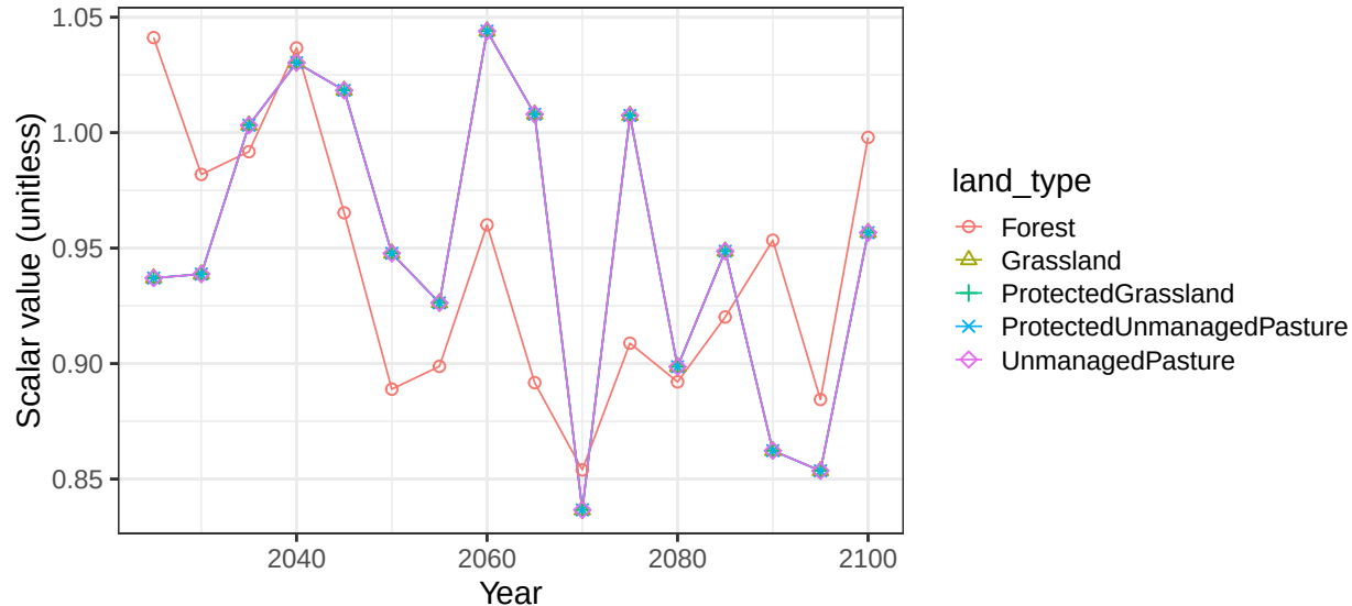
Region EU-15 basin ElbeR non-crop soil scalars
