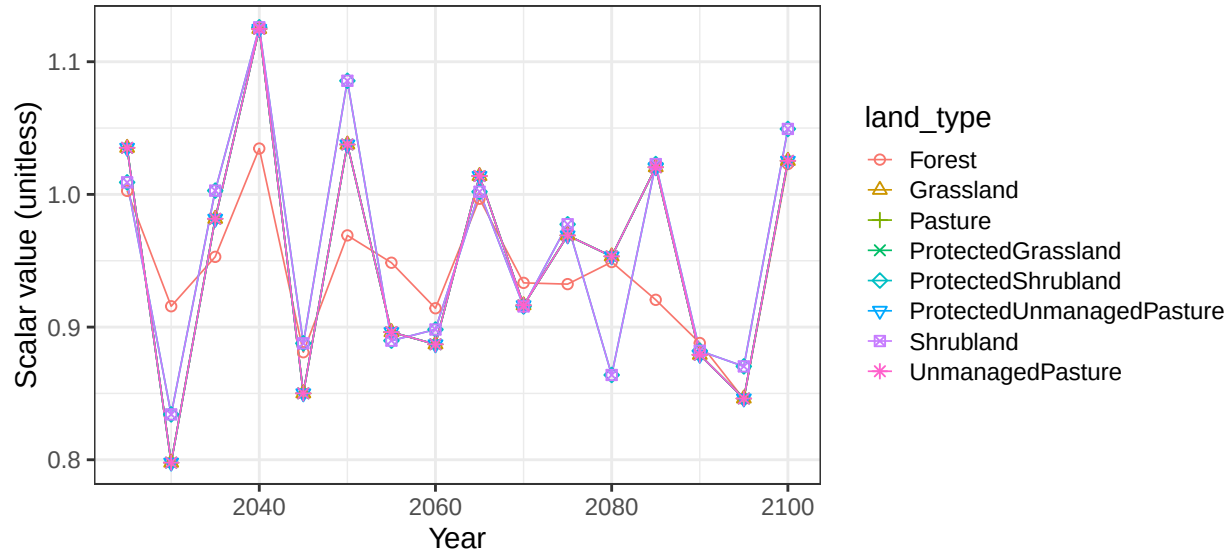
Region China basin ZiyaHe non-crop soil scalars
