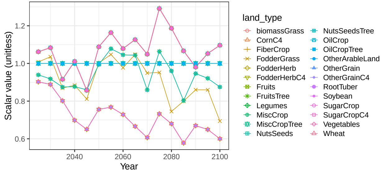
Region Middle East basin MeditE crop vegetation scalars
