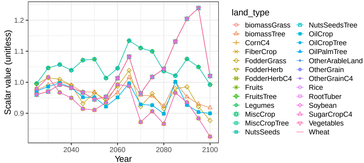
Region South America_ Southern basin RioLaPlata crop soil scalars
