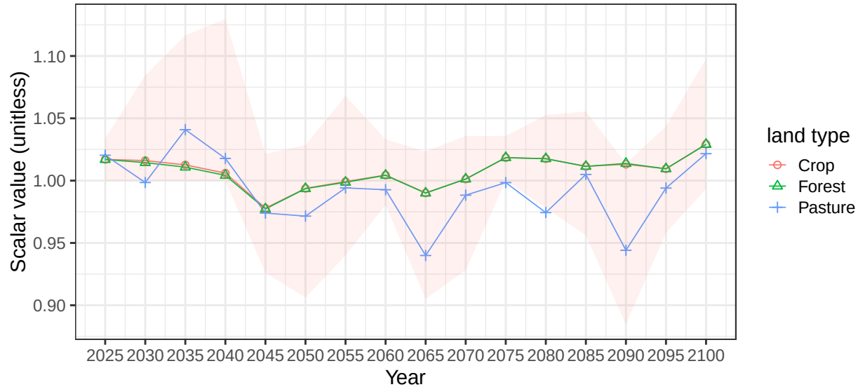
Region Indonesia basin FlyR average soil scalars
