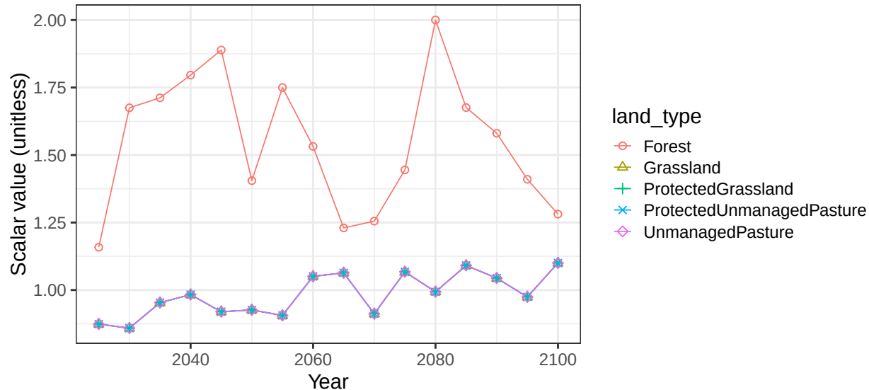
Region EU-15 basin EmsWeserR non-crop vegetation scalars
