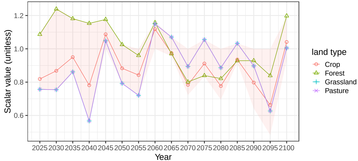
Region EU-12 basin PolandCst average vegetation scalars
