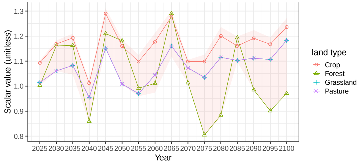
Region India basin BengalW average soil scalars
