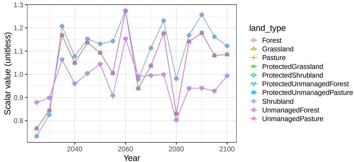
Region Russia basin BarentsSea non-crop vegetation scalars
