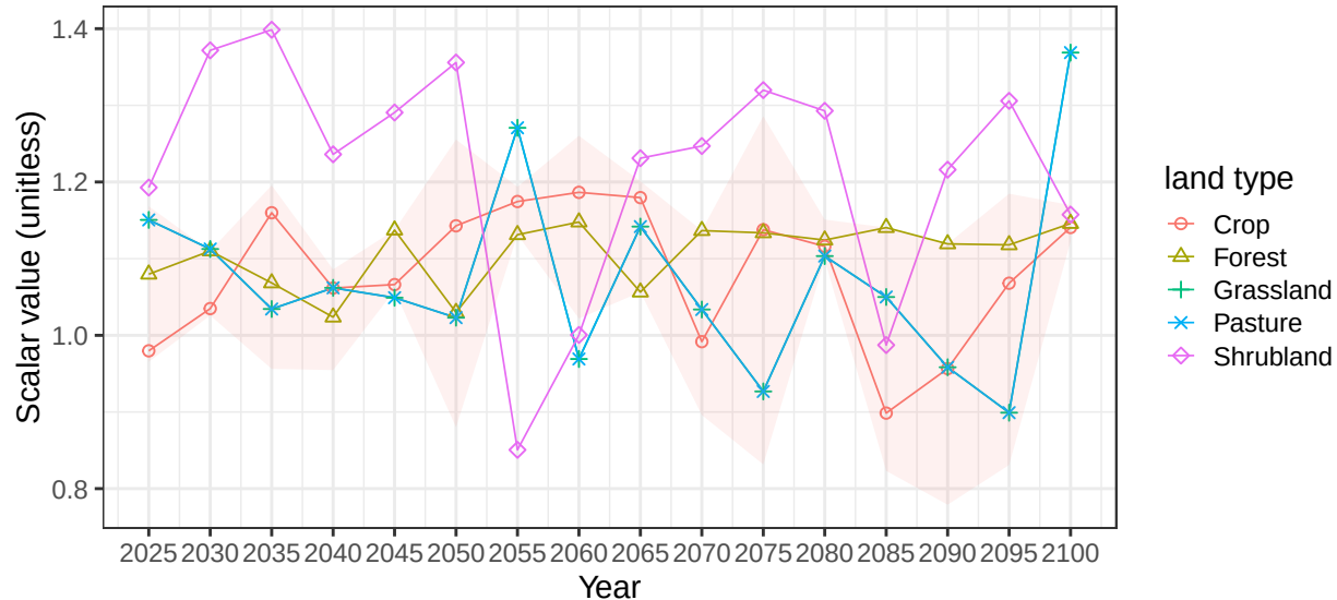
Region Central Asia basin VolgaR average soil scalars
