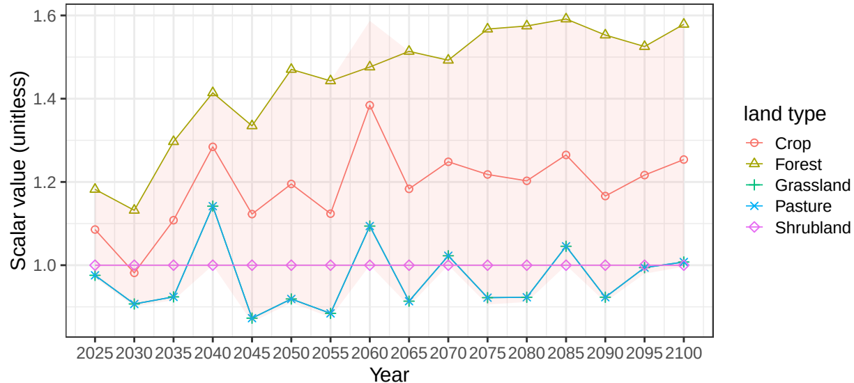
Region Brazil basin ParnaibaR average vegetation scalars
