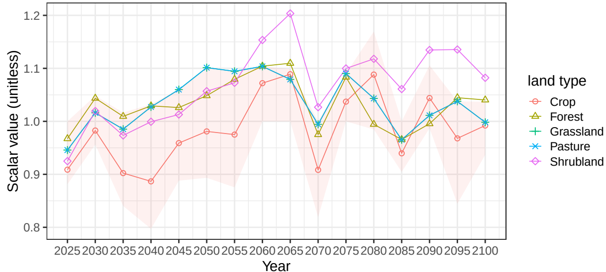
Region Central Asia basin CaspianSW average soil scalars
