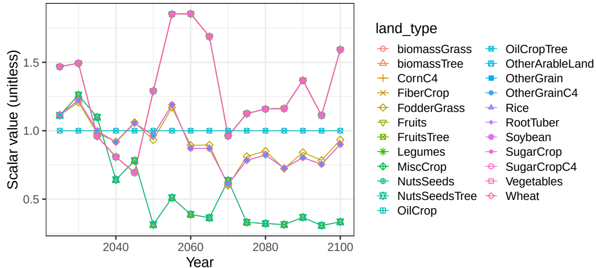
Region Pakistan basin IndusR crop vegetation scalars
