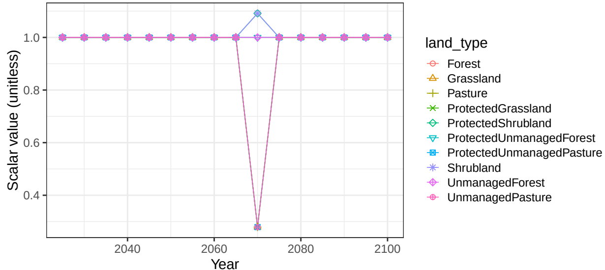
Region Mexico basin California non-crop soil scalars
