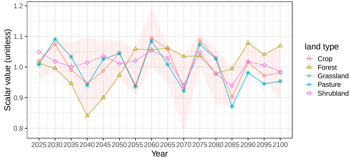
Region Europe_Non_EU basin TigrEuphR average soil scalars
