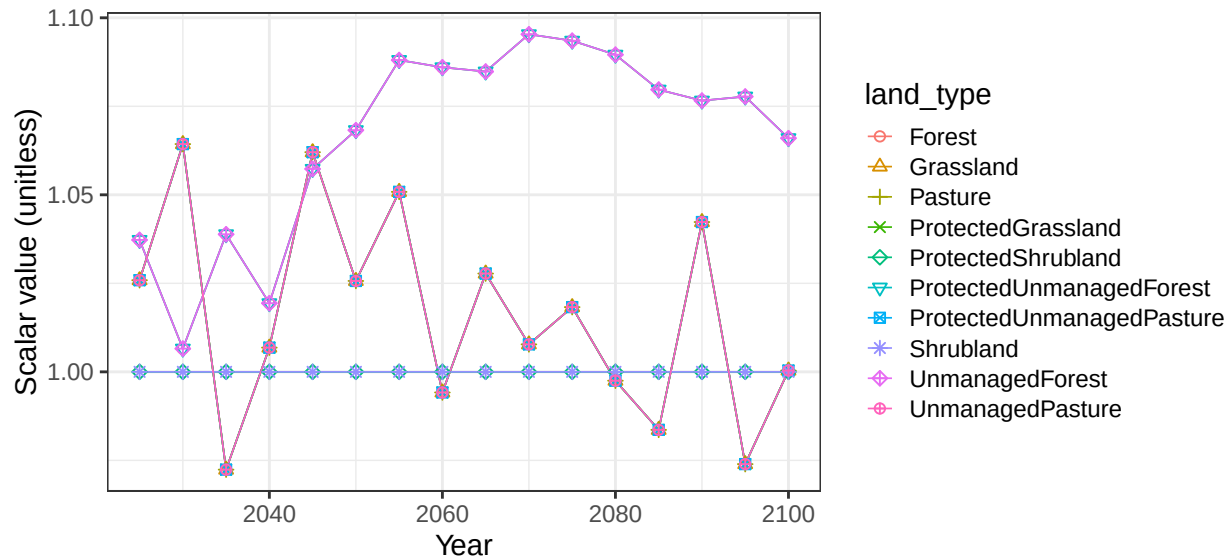
Region Southeast Asia basin XunJiang non-crop soil scalars
