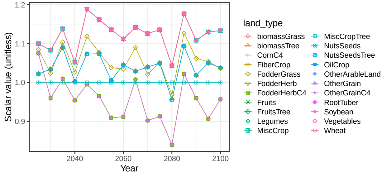
Region USA basin TennR crop vegetation scalars
