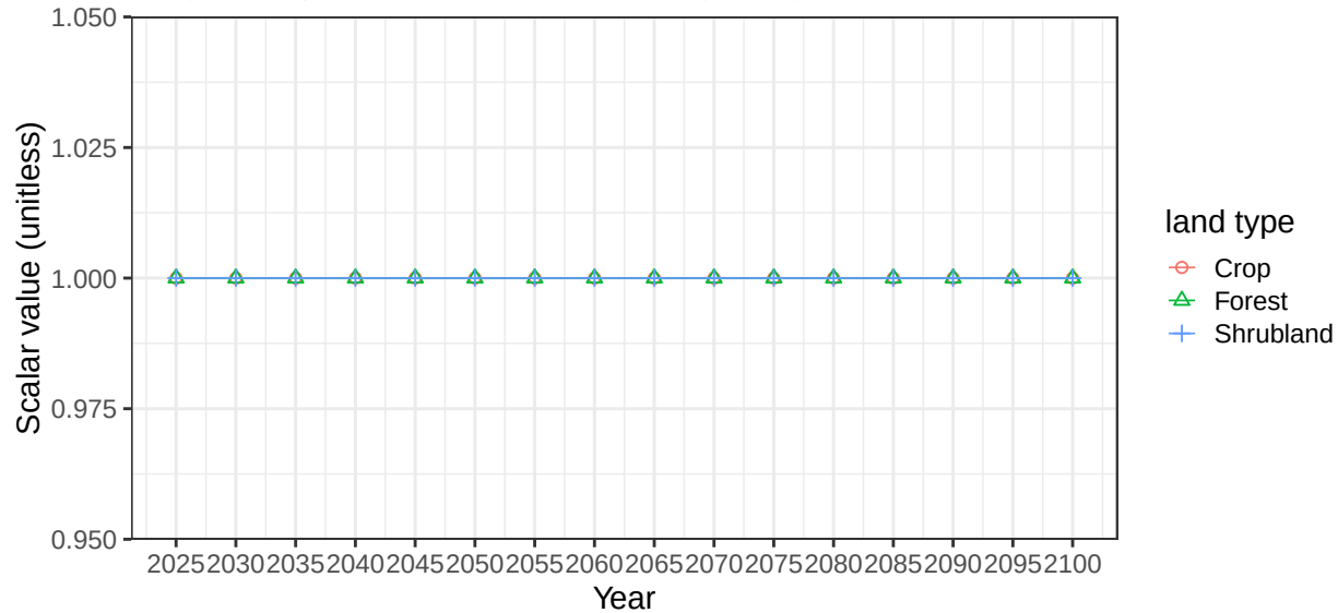
Region Japan basin Taiwan average vegetation scalars
