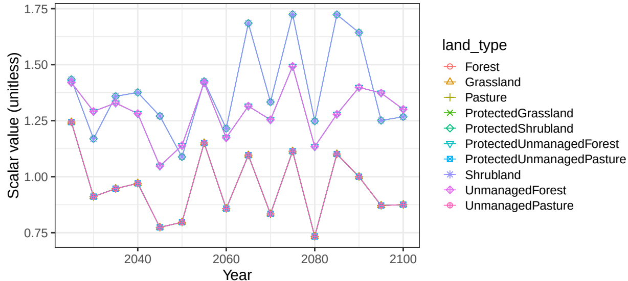
Region USA basin TexasCst non-crop vegetation scalars
