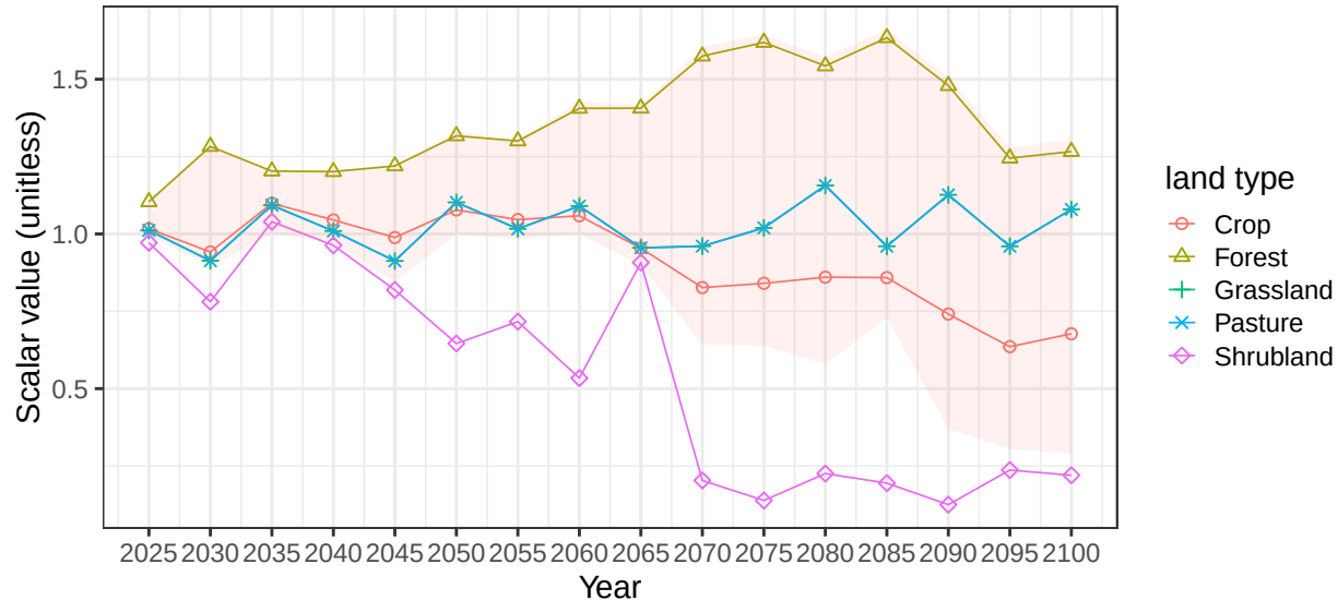
Region Africa_Eastern basin NileR average vegetation scalars
