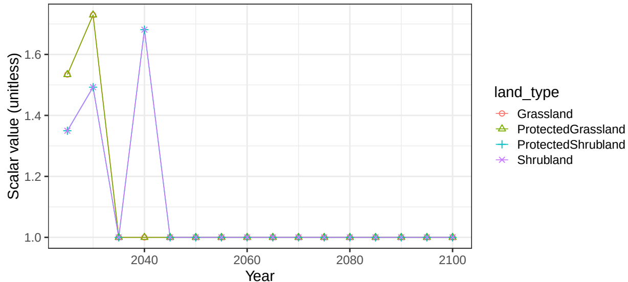
Region Africa_Northern basin MeditE non-crop vegetation scalars
