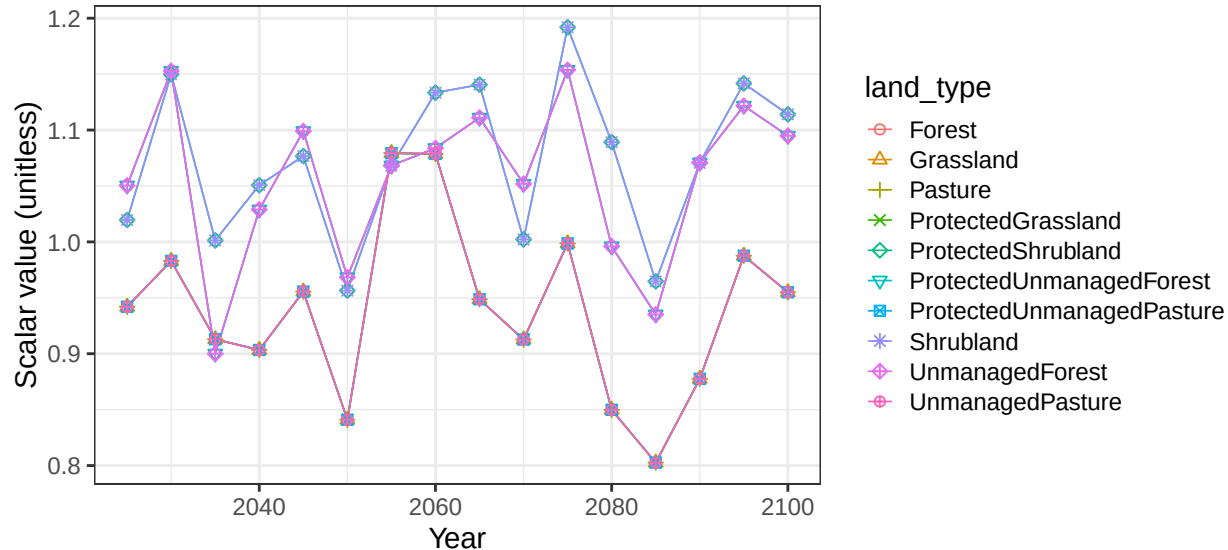
Region Russia basin BlackSeaN non-crop soil scalars
