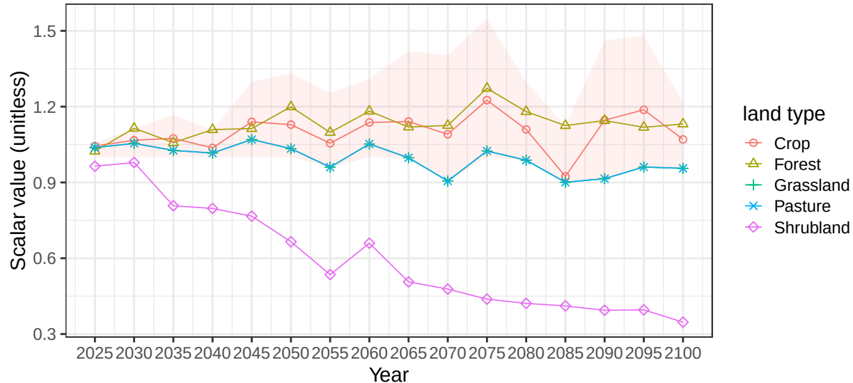
Region Africa_Eastern basin AfrCstNE average soil scalars
