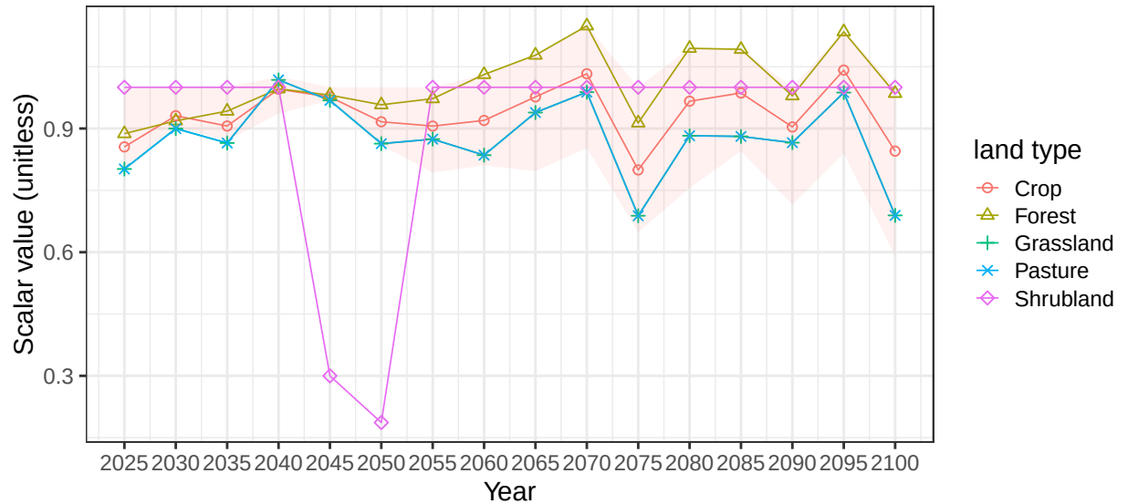
Region South America_Northern basin SAMerCstN average vegetation sca
