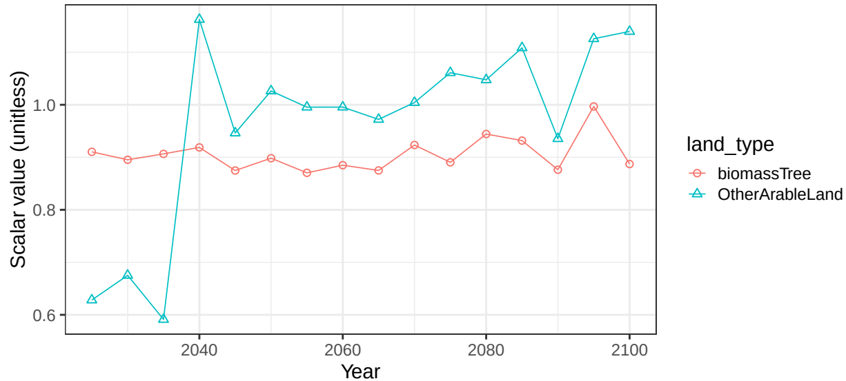
Region Brazil basin OrinocoR crop vegetation scalars
