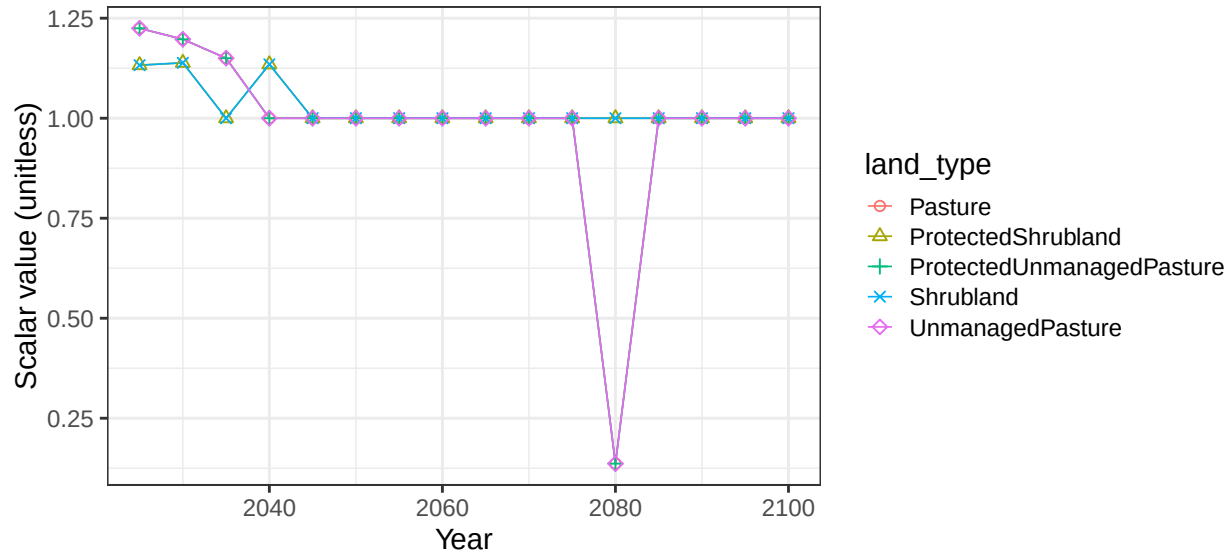
Region Middle East basin SinaiP non-crop soil scalars
