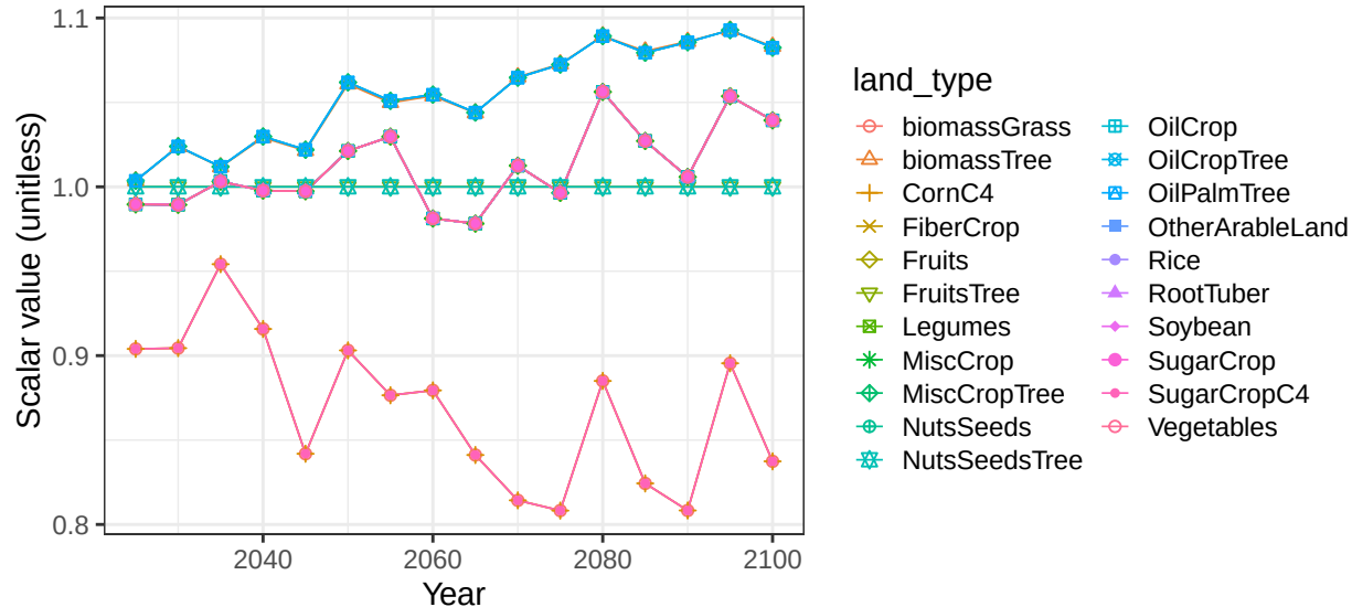
Region Indonesia basin Sumatra crop vegetation scalars
