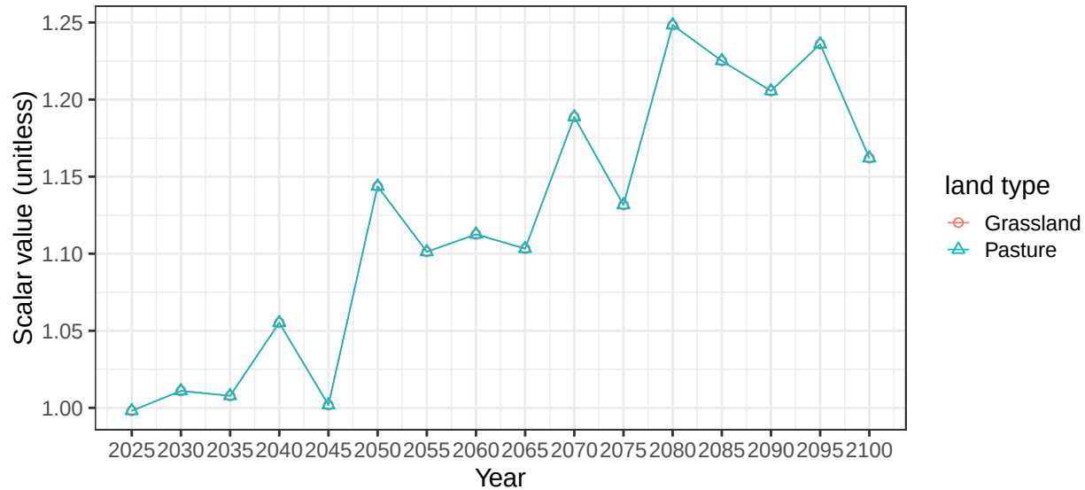
Region China basin Tibet average vegetation scalars
