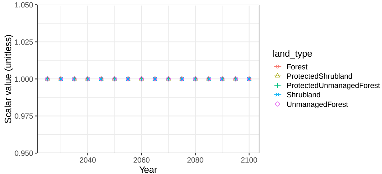
Region Japan basin Taiwan non-crop vegetation scalars
