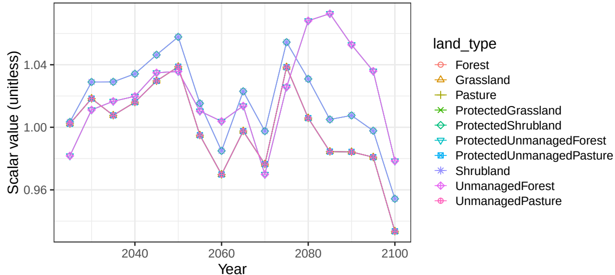
Region Russia basin LenaR non-crop soil scalars
