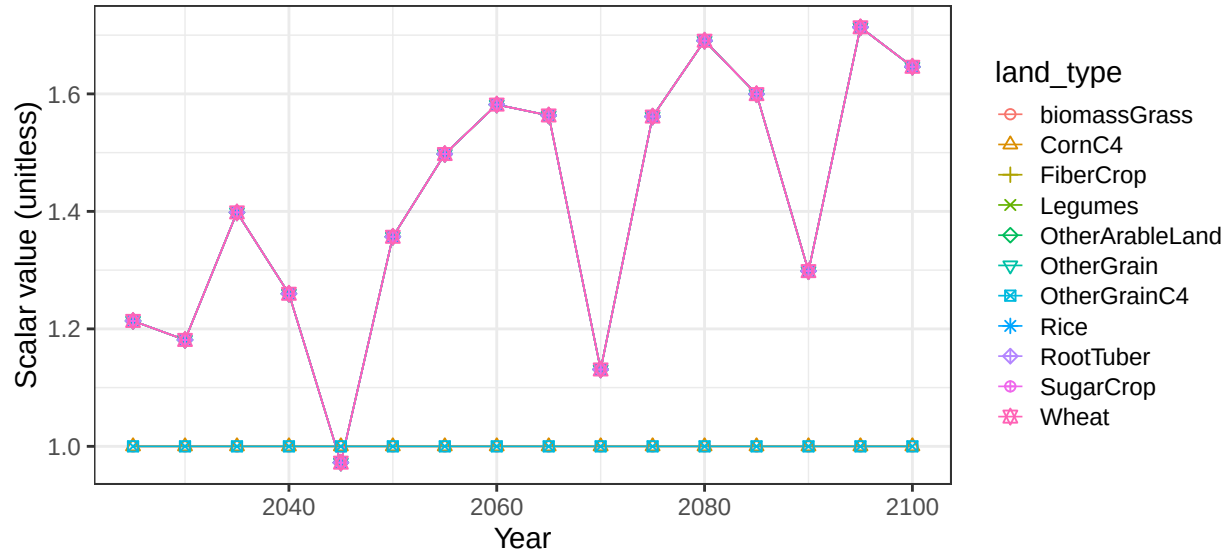
Region South Asia basin FarahrudR crop vegetation scalars
