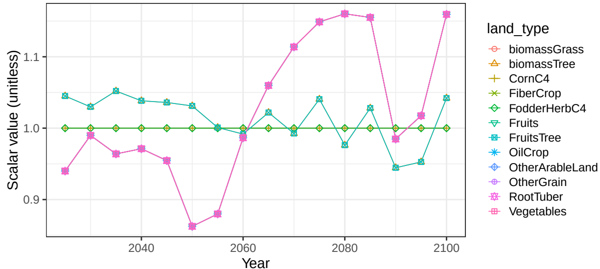
Region Canada basin PacArctic crop soil scalars
