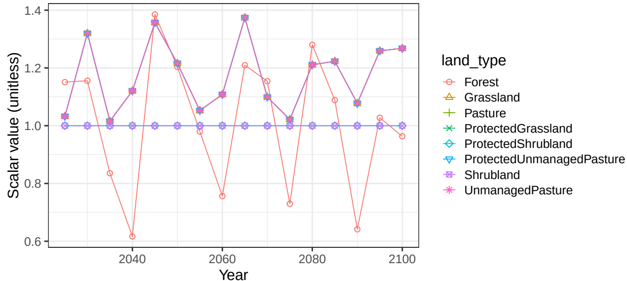
Region India basin IndCstNE non-crop vegetation scalars
