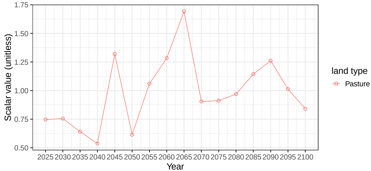
Region EU-15 basin AfrCstNW average vegetation scalars
