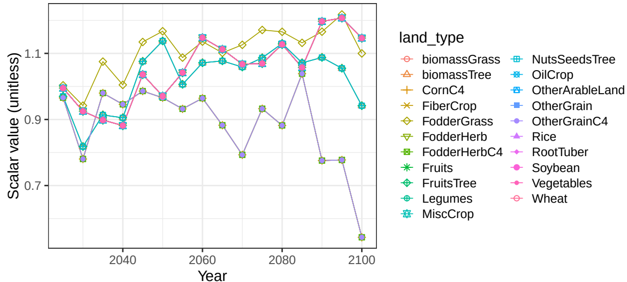
Region Russia basin YeniseiR crop vegetation scalars
