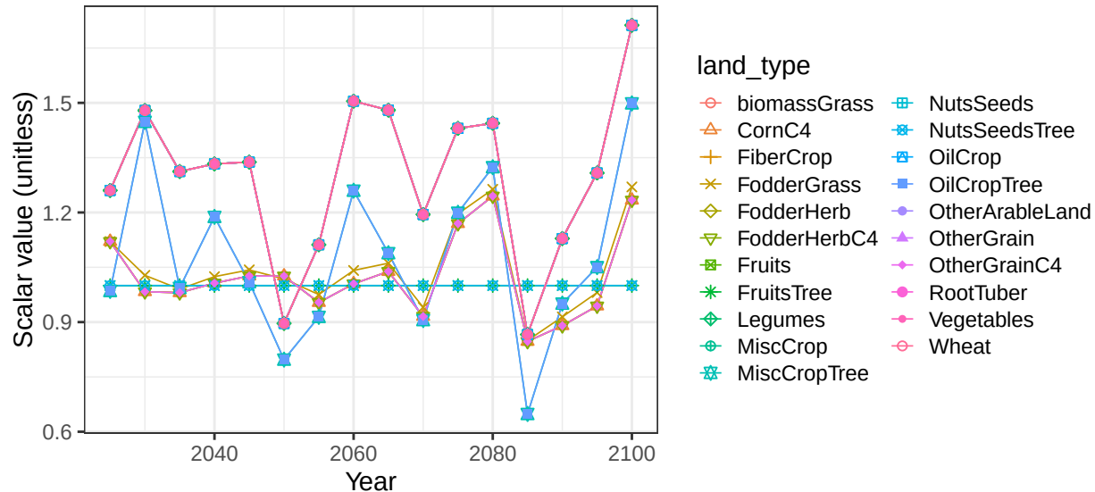
Region Middle East basin RedSeaE crop vegetation scalars
