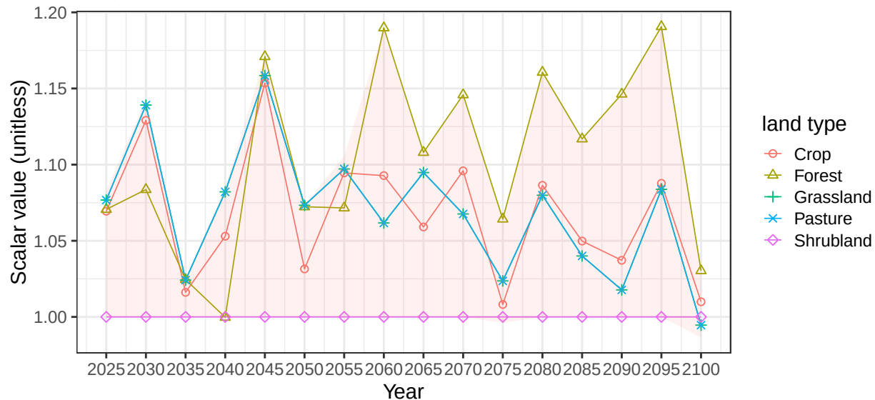
Region India basin KrishnaR average soil scalars
