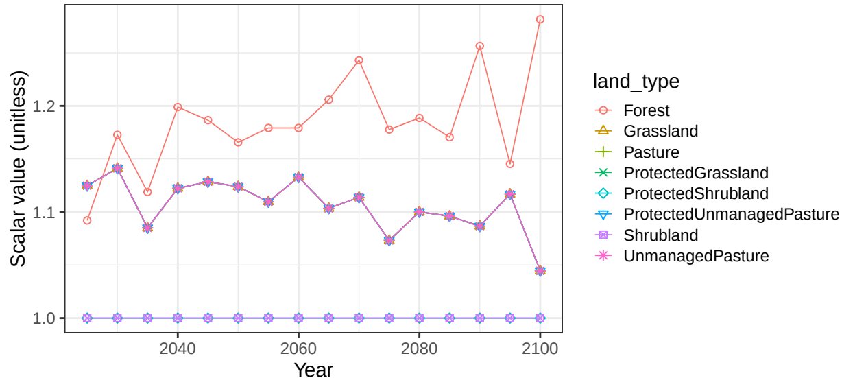
Region India basin IndCstW non-crop soil scalars
