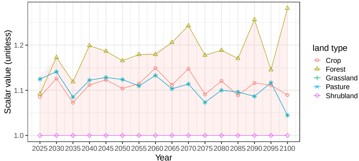
Region India basin IndCstW average soil scalars
