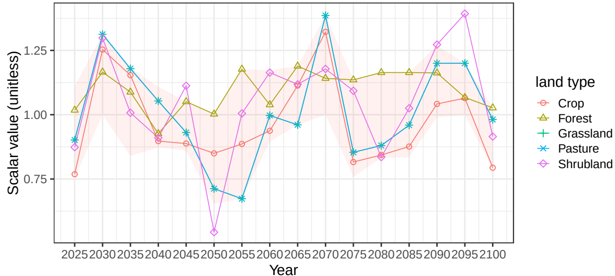
Region Australia_NZ basin AusCstS average vegetation scalars
