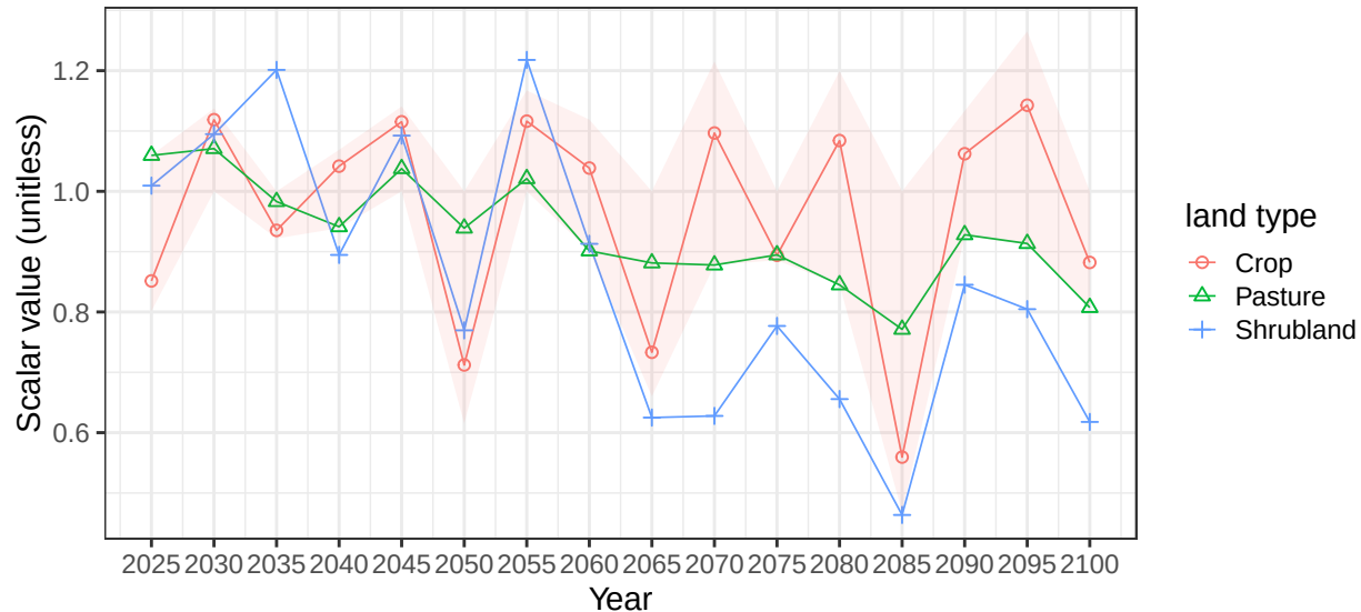
Region Pakistan basin SabarmatiR average soil scalars
