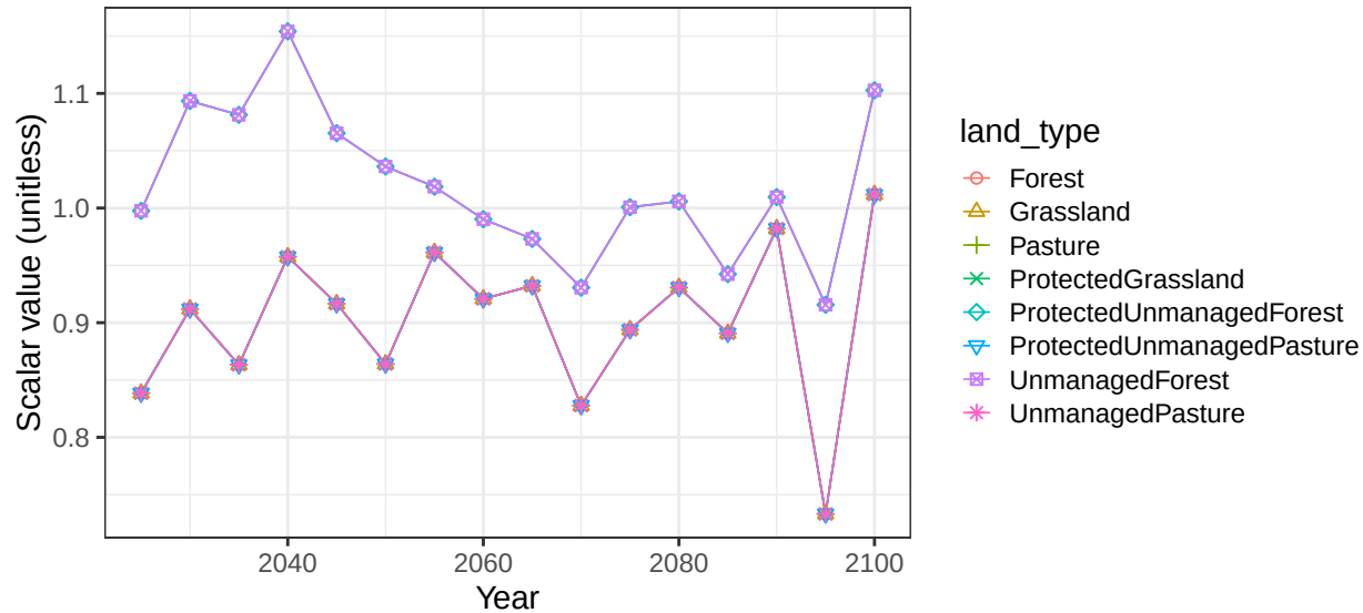
Region EU-12 basin WislaR non-crop soil scalars
