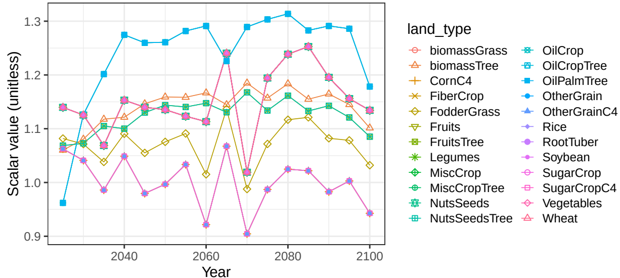
Region China basin ChinaCst crop vegetation scalars
