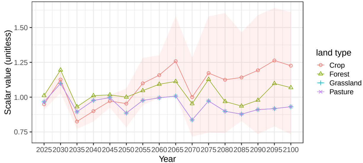
Region Central Asia basin BlackSeaS average soil scalars
