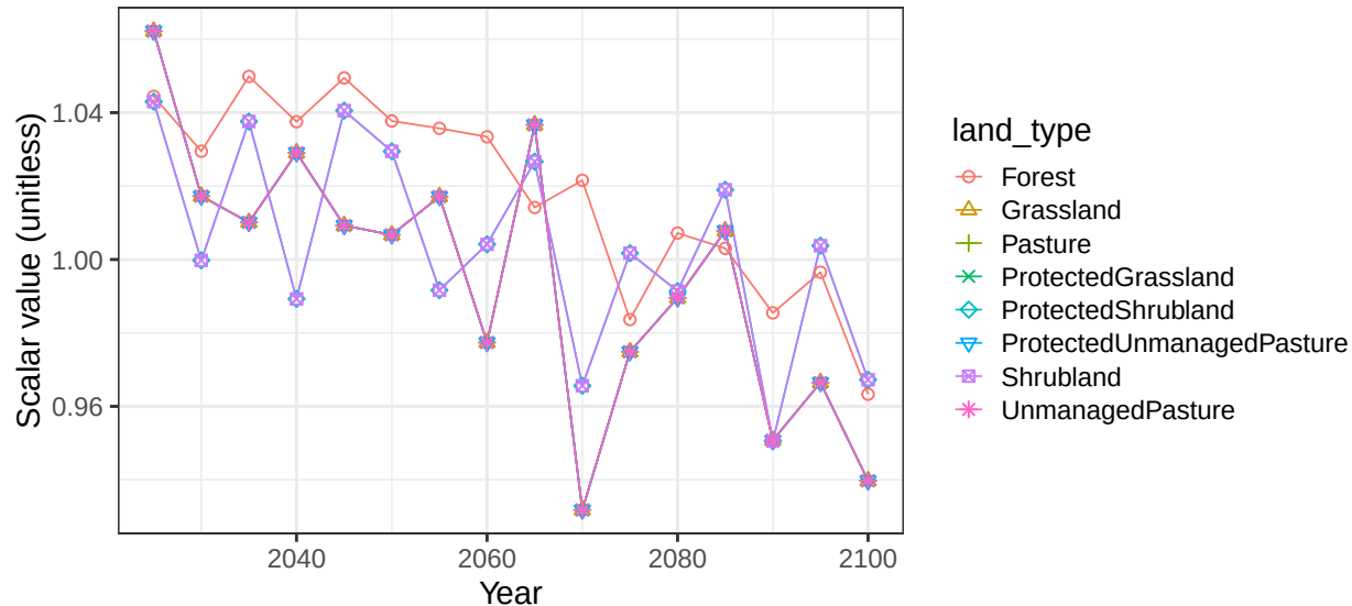
Region China basin ChinaCst non-crop soil scalars
