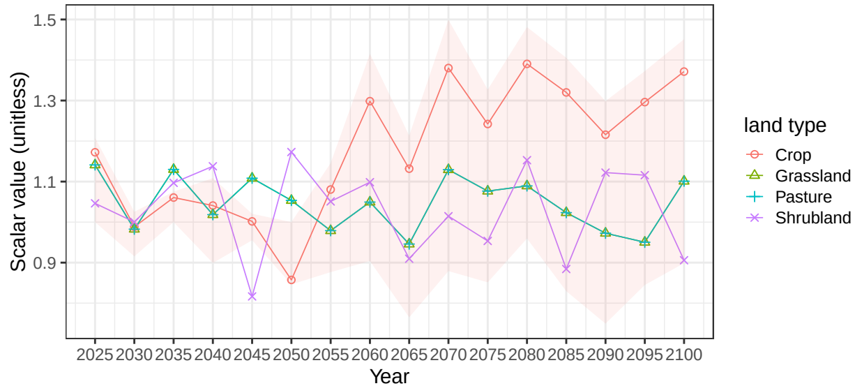
Region Africa_Southern basin AfrCstSW average soil scalars
