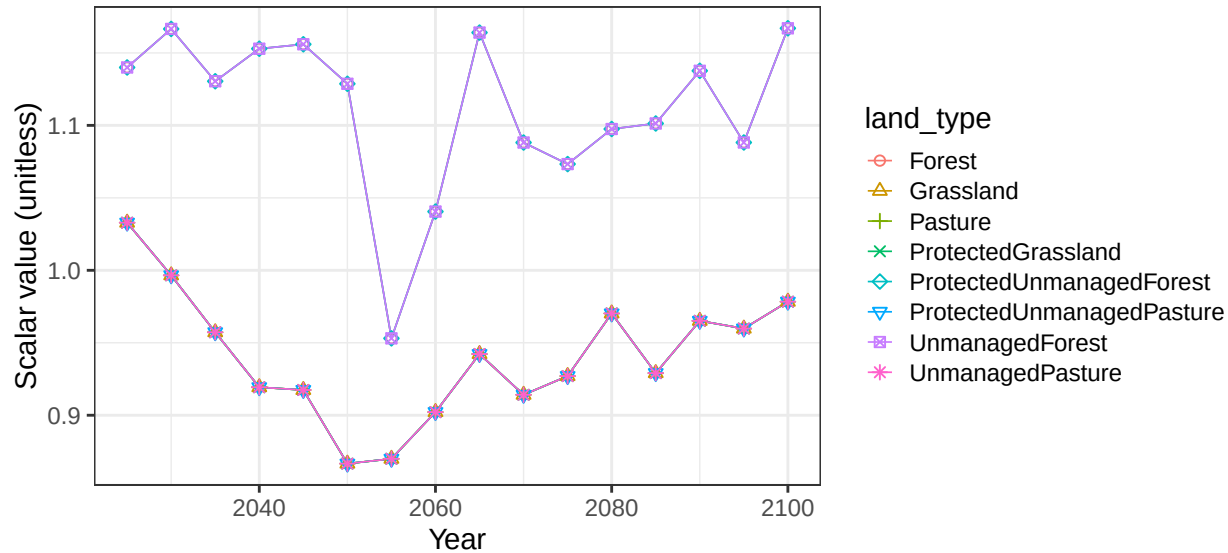
Region South Asia basin BengalBay non-crop soil scalars
