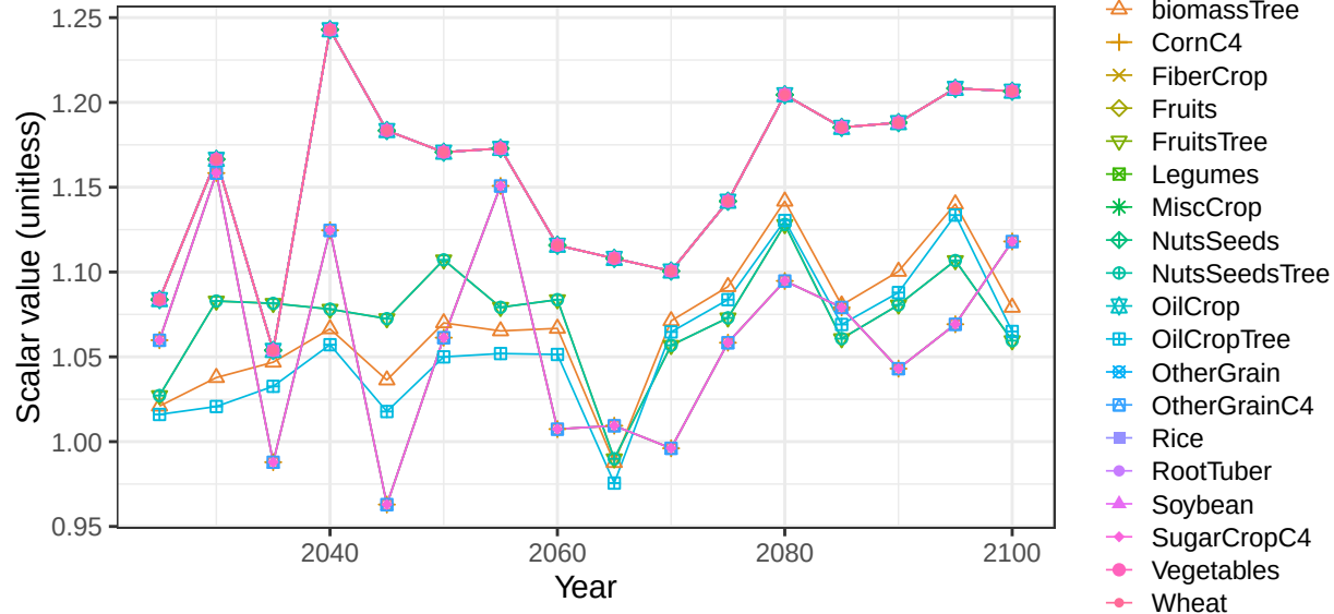
Region Taiwan basin Taiwan crop vegetation scalars
