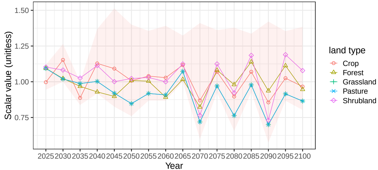
Region Argentina basin ArgColoR average soil scalars
