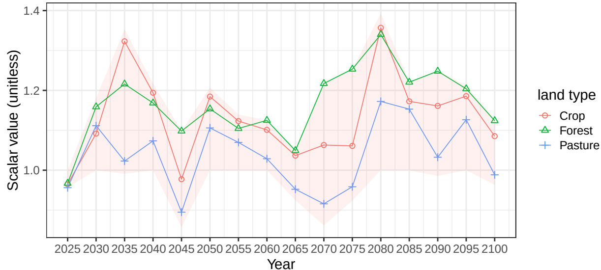
Region Taiwan basin ChinaCst average vegetation scalars
