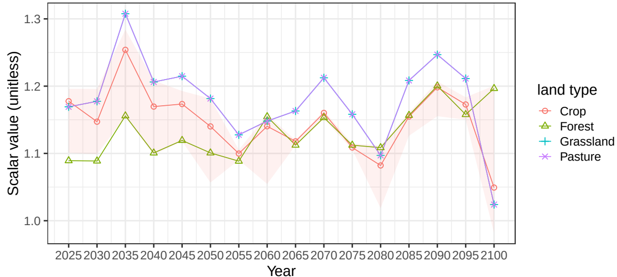
Region Southeast Asia basin Korea average vegetation scalars
