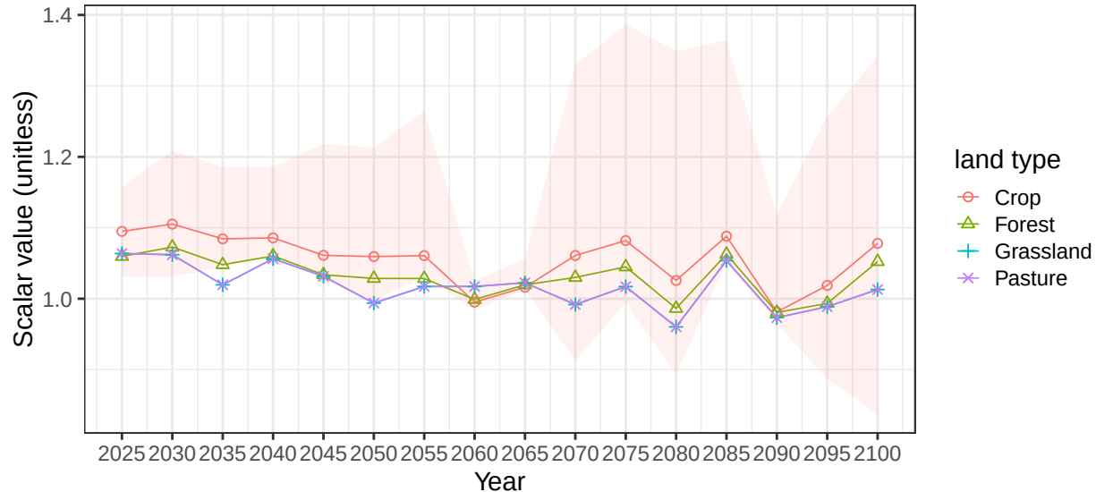
Region Canada basin UsaPacNW average soil scalars
