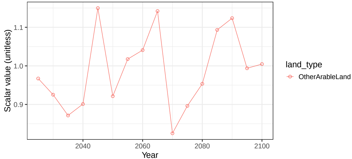
Region EU-15 basin AfrCstNW crop soil scalars
