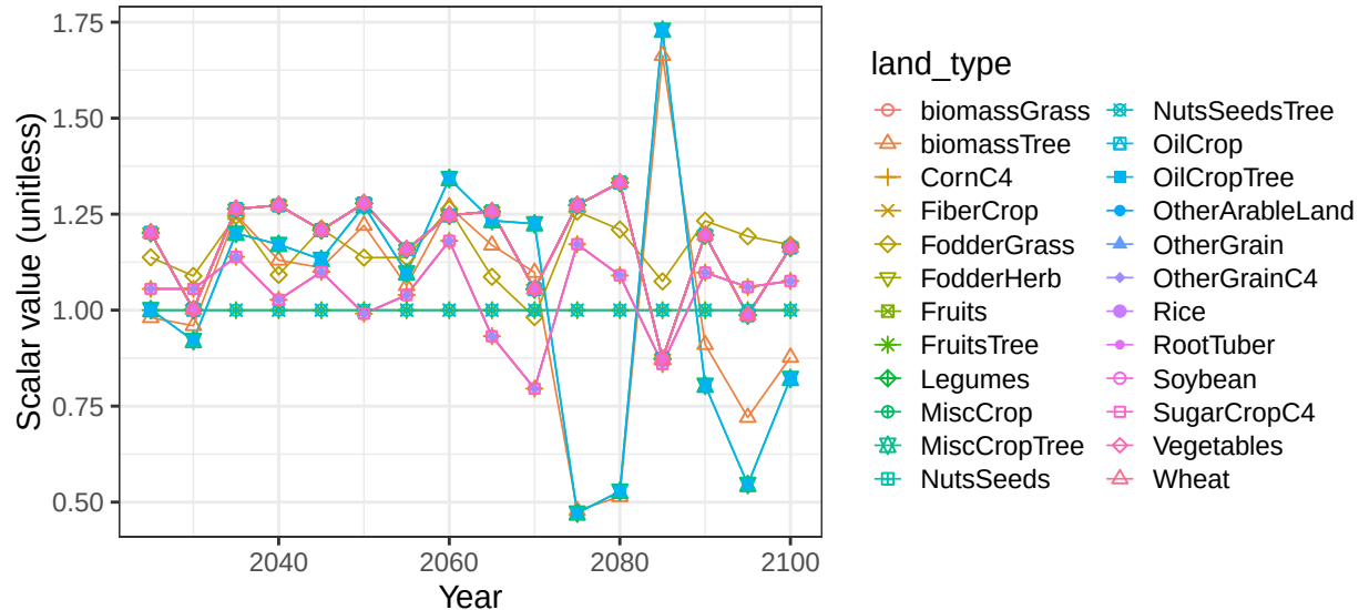
Region Africa_Eastern basin RiftValley crop vegetation scalars
