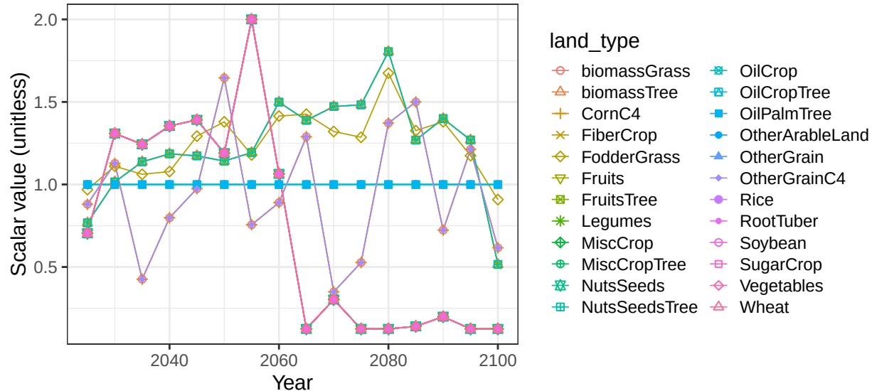
Region China basin ObR crop vegetation scalars
