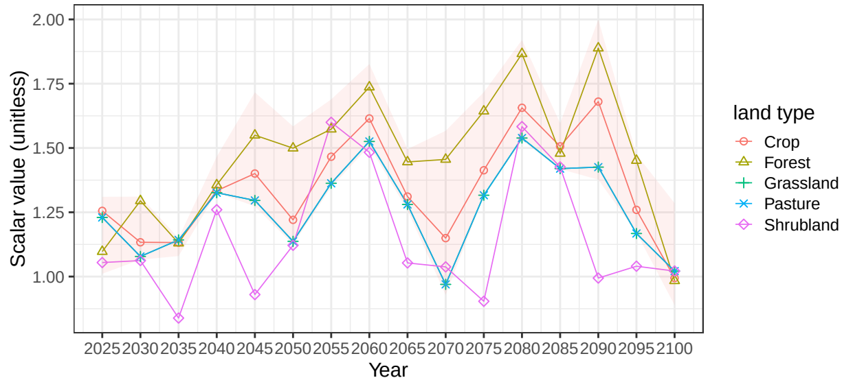
Region Africa_Southern basin LimpopoR average vegetation scalars
