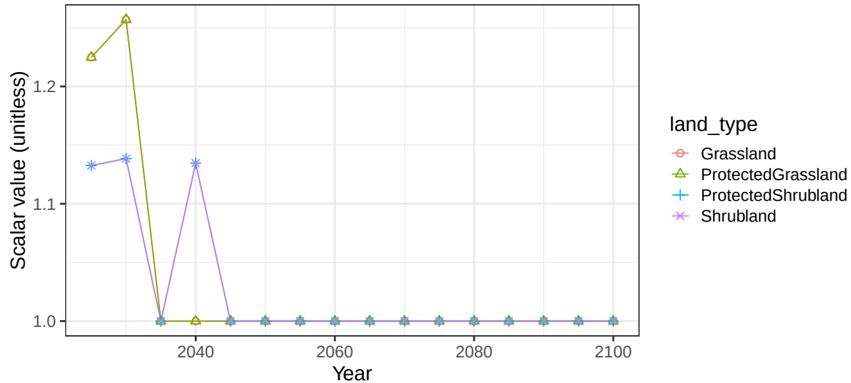
Region Africa_Northern basin MeditE non-crop soil scalars
