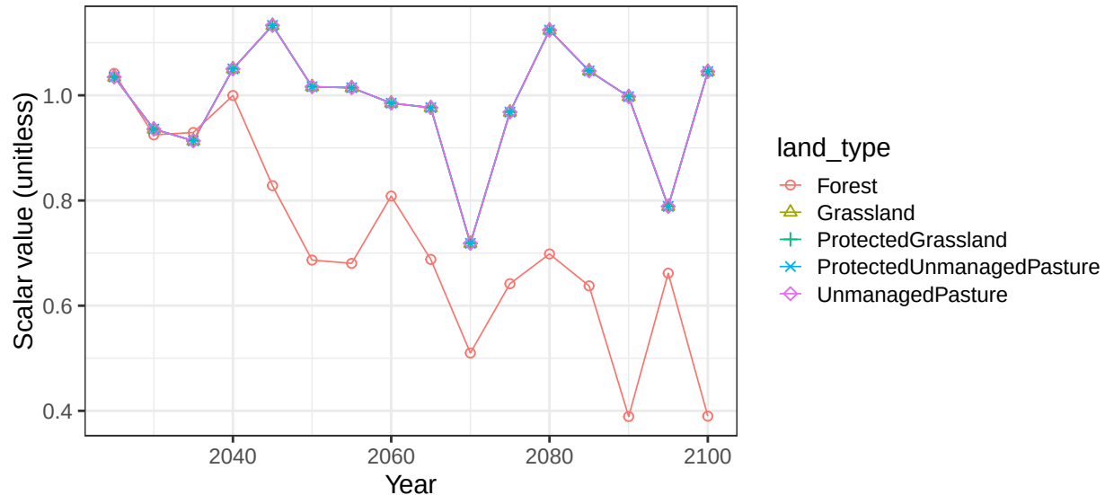
Region EU-15 basin SeineR non-crop vegetation scalars
