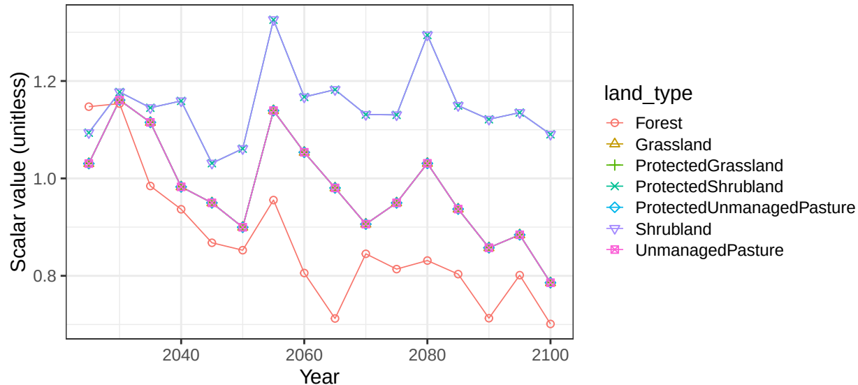
Region EU-15 basin AdrBlkSea non-crop vegetation scalars
