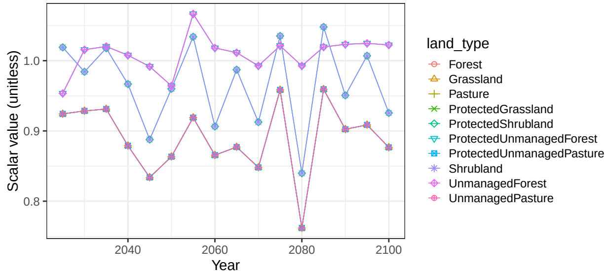
Region Mexico basin MexGulf non-crop soil scalars
