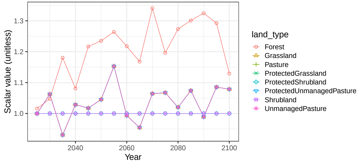
Region China basin SChinaSea non-crop vegetation scalars
