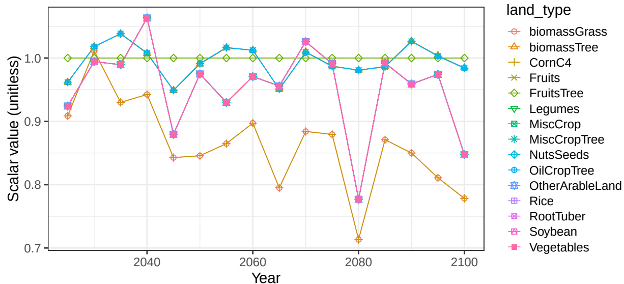
Region Southeast Asia basin JavaTimor crop soil scalars
