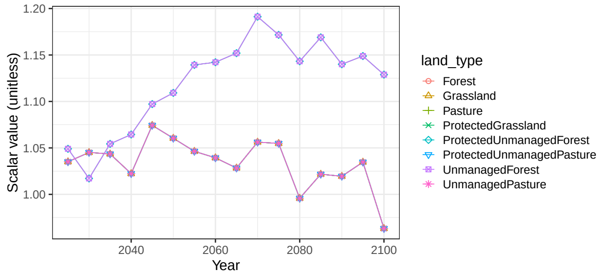
Region South America_Southern basin NegroR non-crop soil scalars
