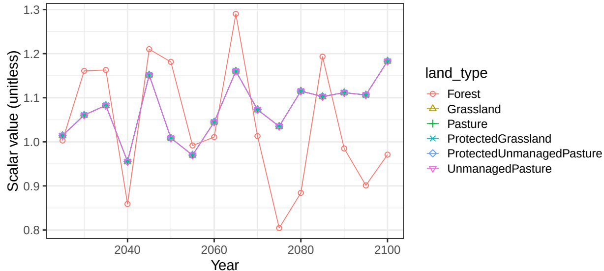
Region India basin BengalW non-crop soil scalars
