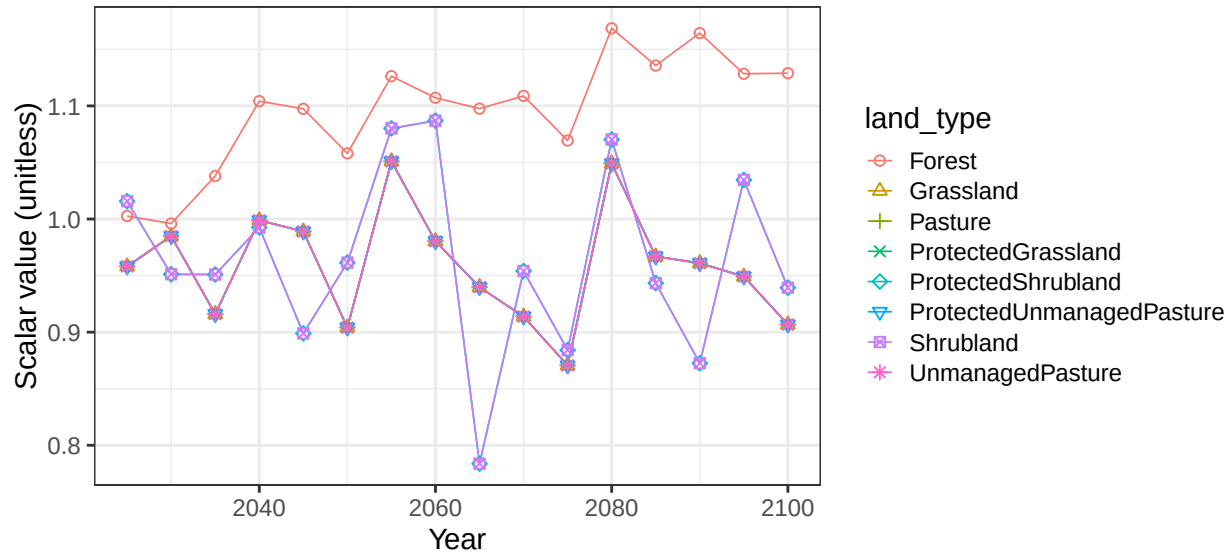
Region South Africa basin OrangeR non-crop soil scalars
