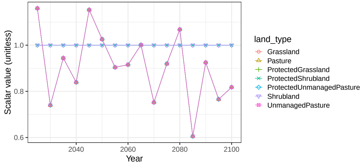
Region Africa_Western basin AfrIntN non-crop vegetation scalars
