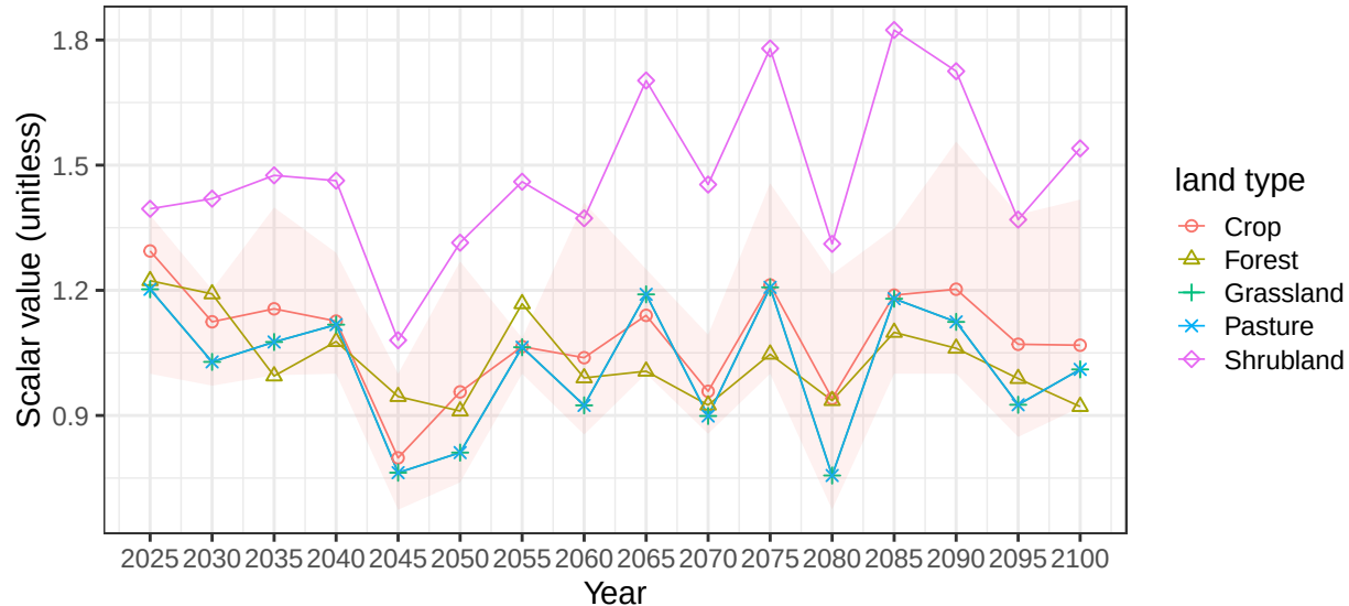
Region USA basin RioGrande average vegetation scalars
