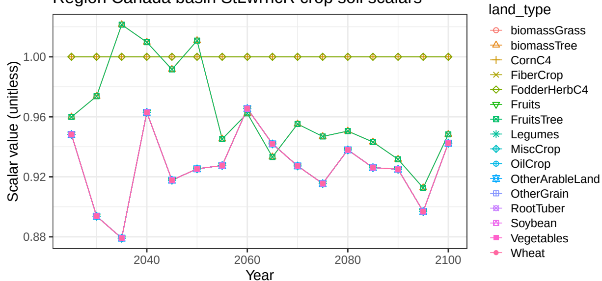
Region Canada basin StLwrncR crop soil scalars
