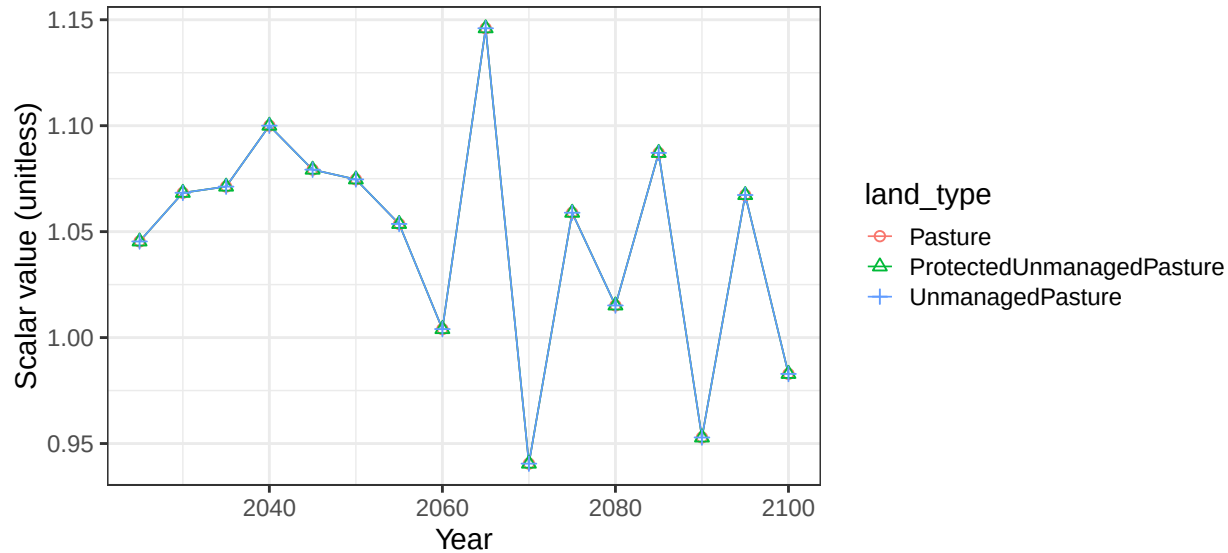
Region South America_Southern basin ArgColoR non-crop soil scalars
