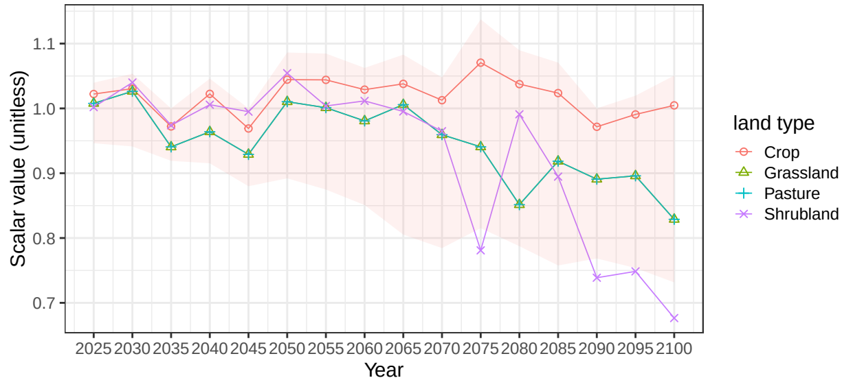
Region Middle East basin MeditE average soil scalars
