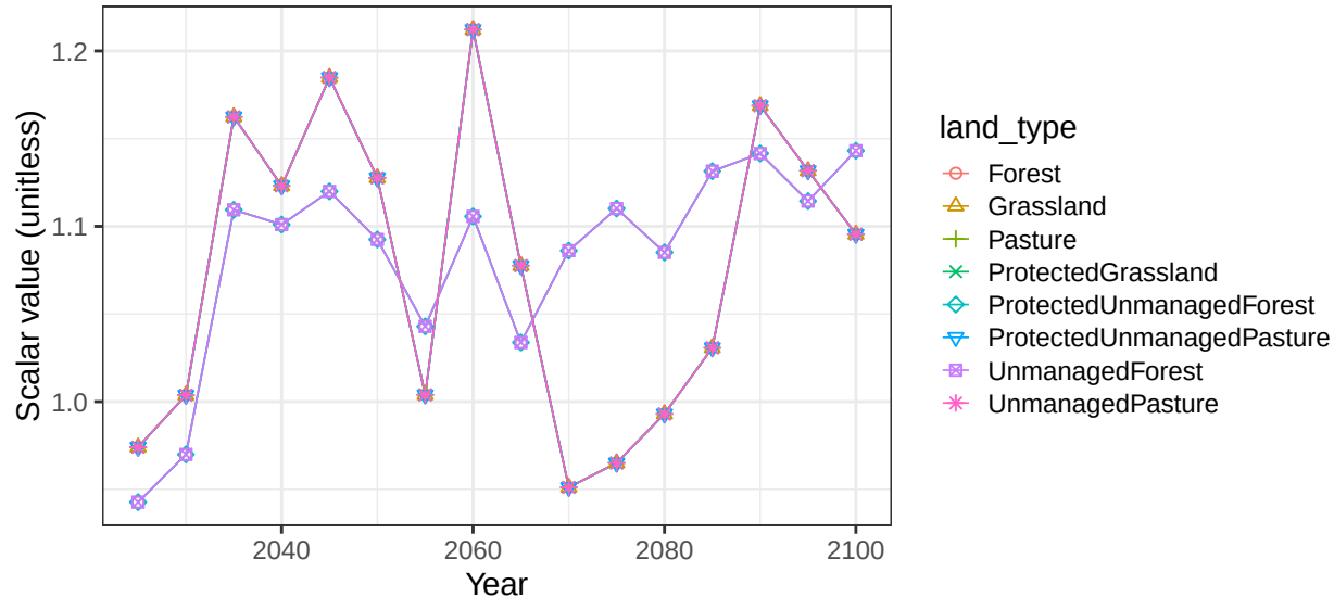
Region Southeast Asia basin RusCstSE non-crop vegetation scalars
