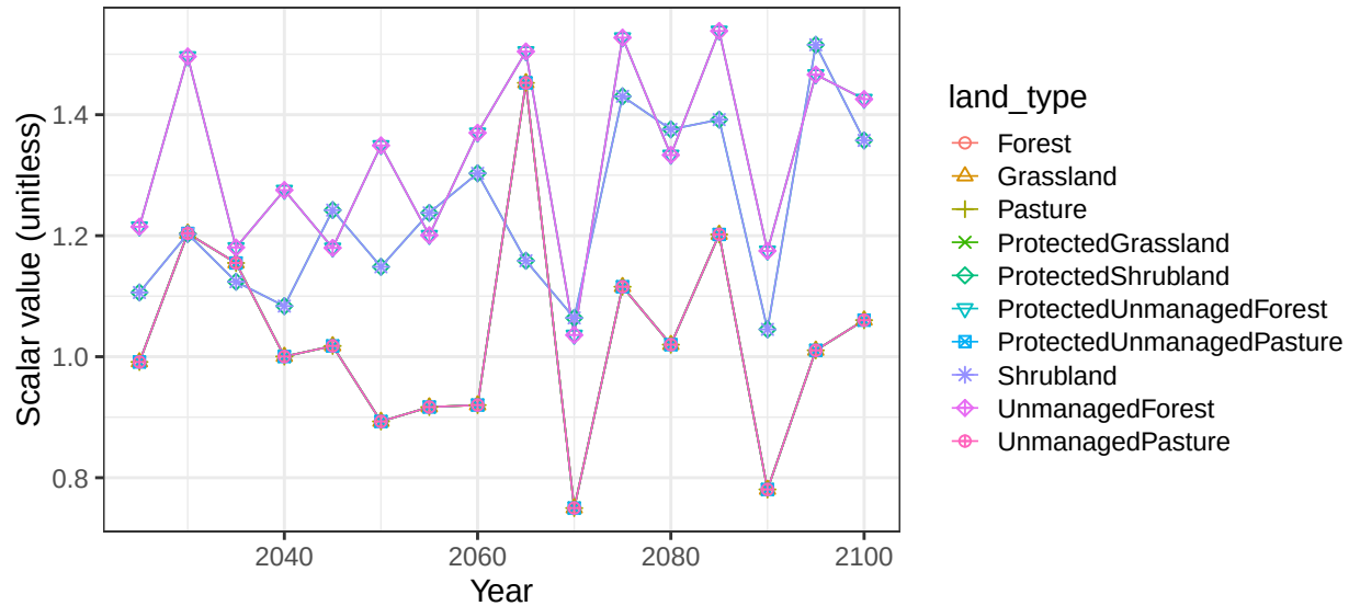
Region Argentina basin Salinas non-crop vegetation scalars
