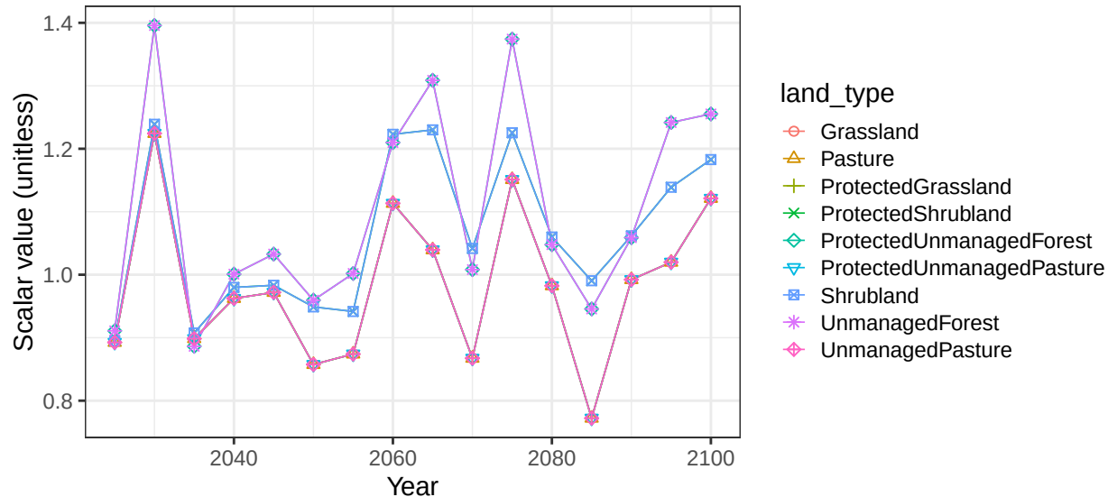
Region Russia basin BlackSeaS non-crop vegetation scalars
