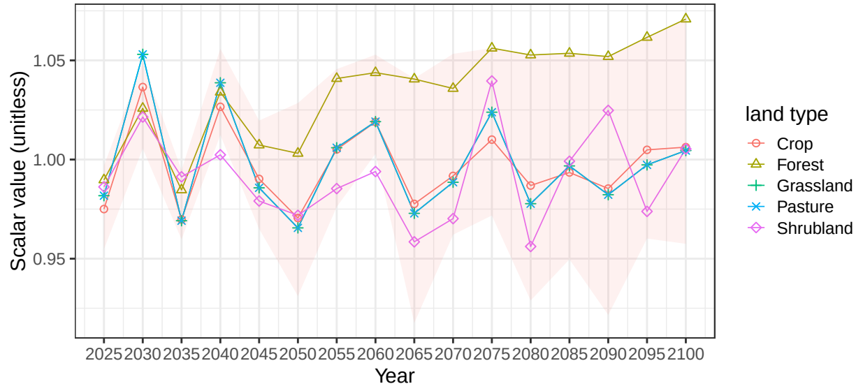
Region Brazil basin BrzCstS average soil scalars
