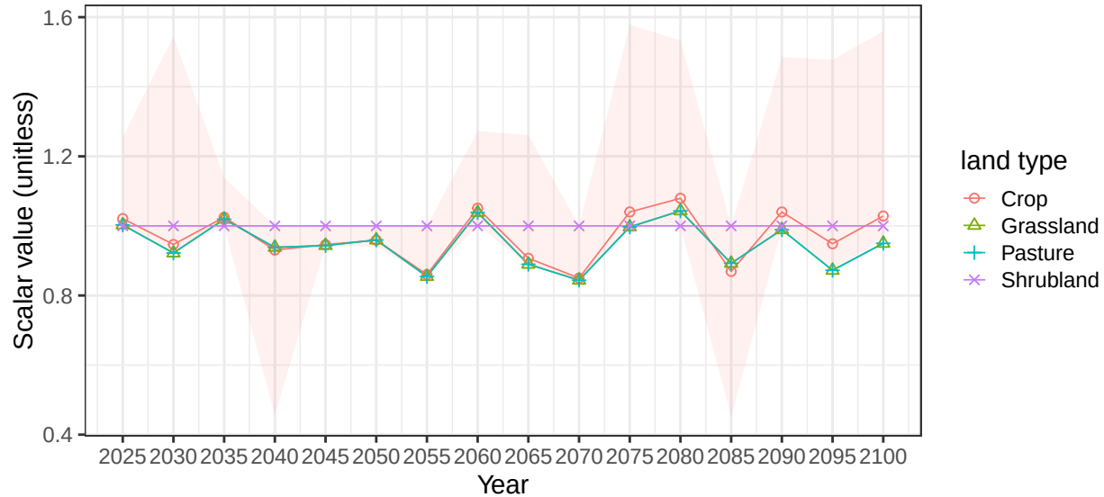
Region Africa_Western basin AfrCstNW average soil scalars
