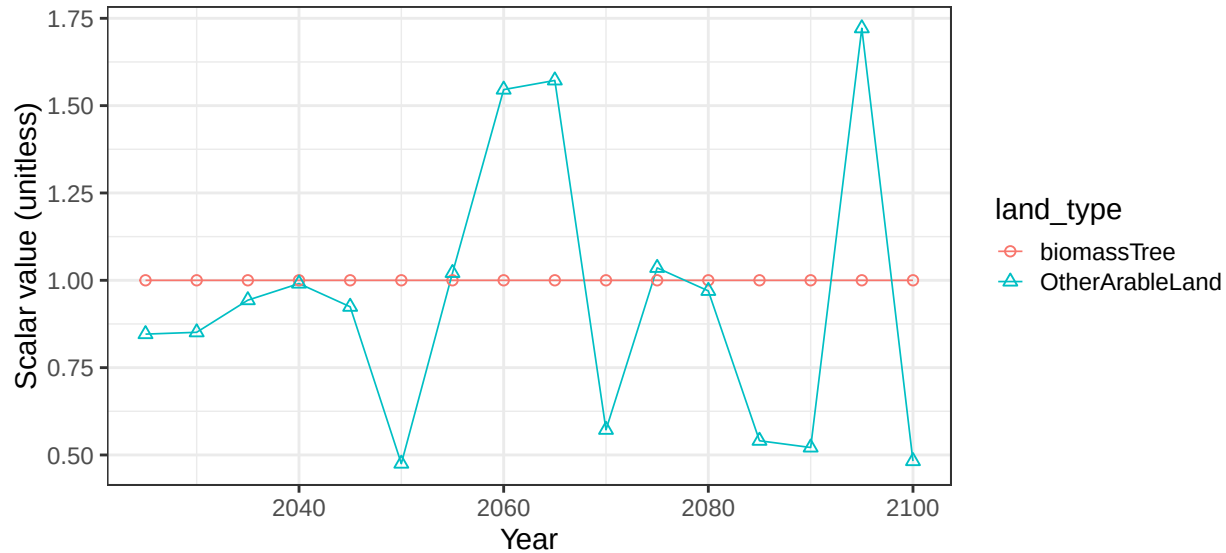
Region Russia basin ScndnvN crop soil scalars
