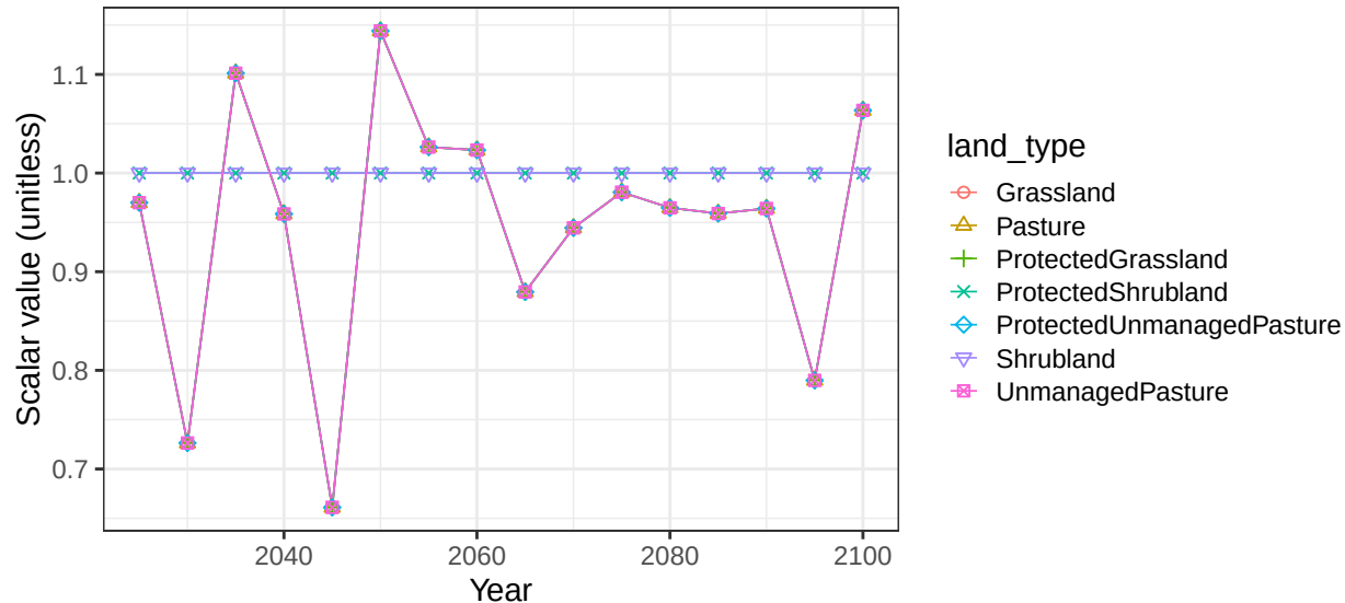
Region Africa_Eastern basin LChad non-crop vegetation scalars
