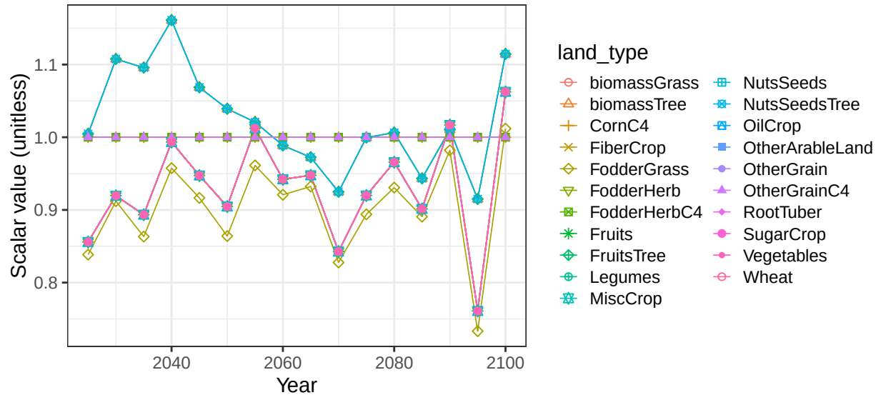
Region EU-12 basin WislaR crop soil scalars
