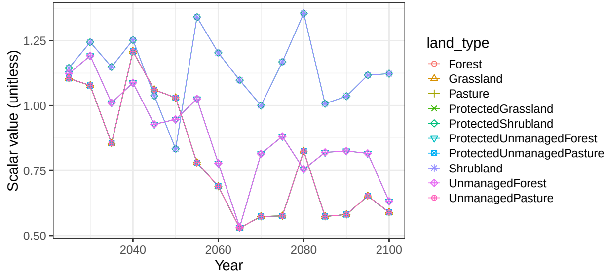
Region EU-12 basin AdrBlkSea non-crop vegetation scalars
