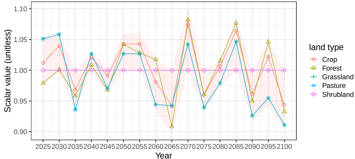
Region China basin Hainan average soil scalars
