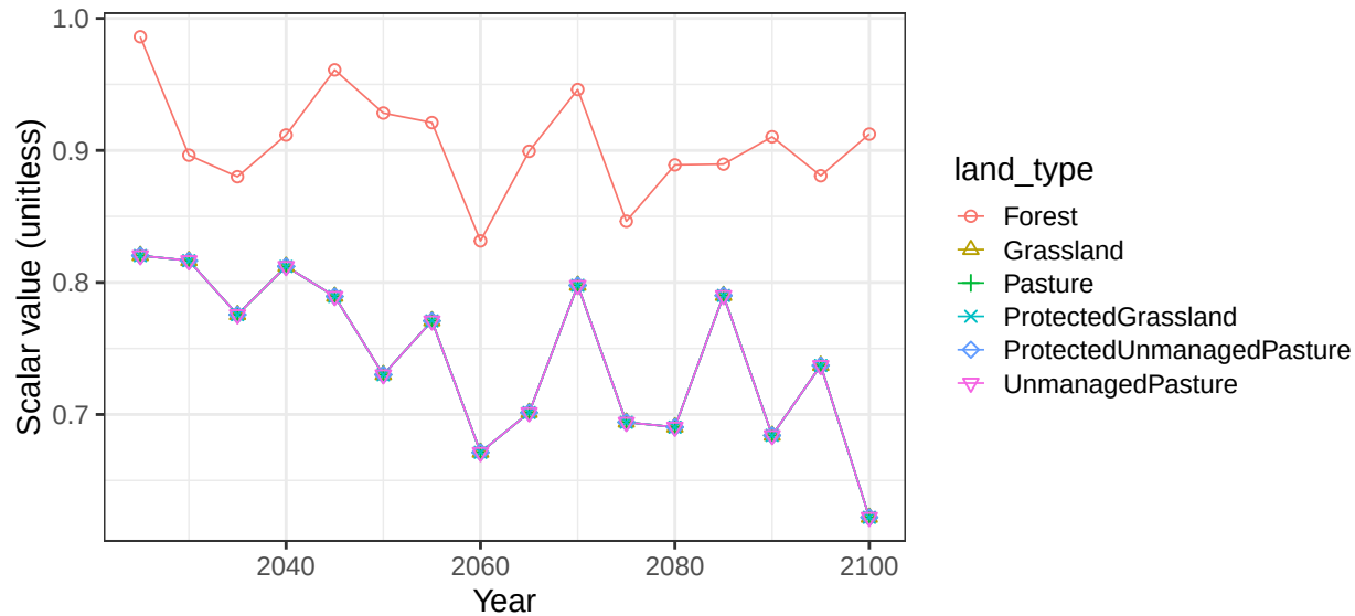
Region India basin AdnNicIsl non-crop vegetation scalars
