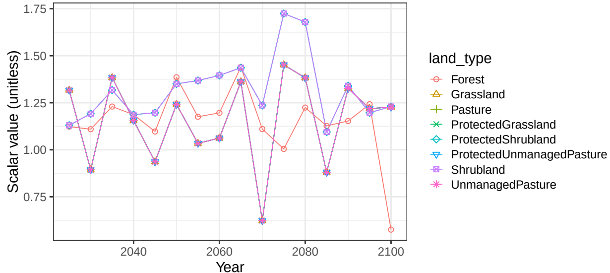
Region Africa_Eastern basin AfrCstE non-crop vegetation scalars
