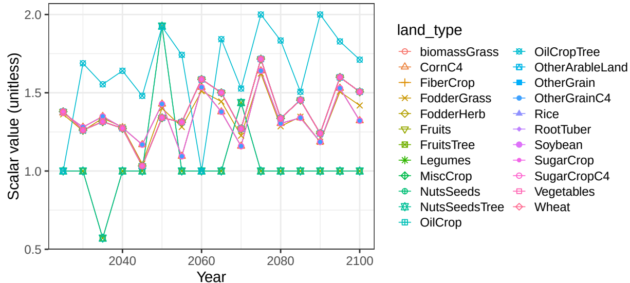
Region Middle East basin PersianGulf crop vegetation scalars
