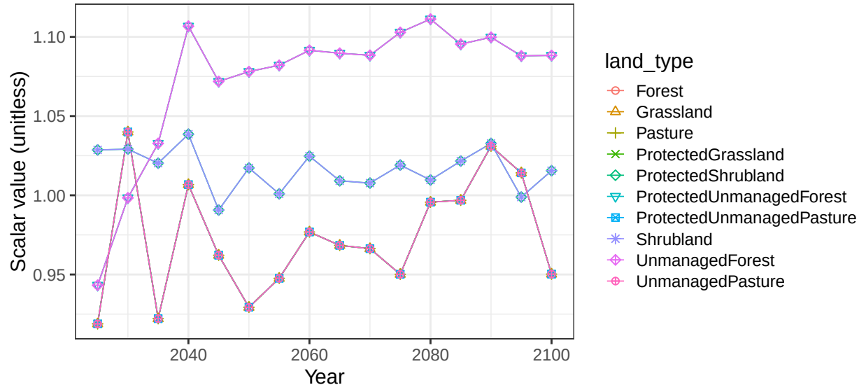
Region Brazil basin RioLaPlata non-crop soil scalars
