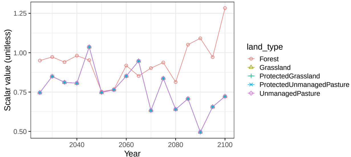
Region EU-15 basin OderR non-crop vegetation scalars
