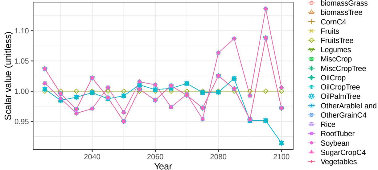
Region Central America and Caribbean basin SAMerCstNcropSoil scalars
