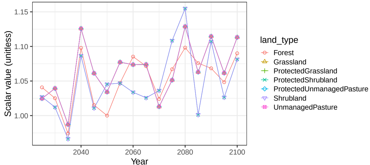
Region EU-15 basin Gironde non-crop soil scalars
