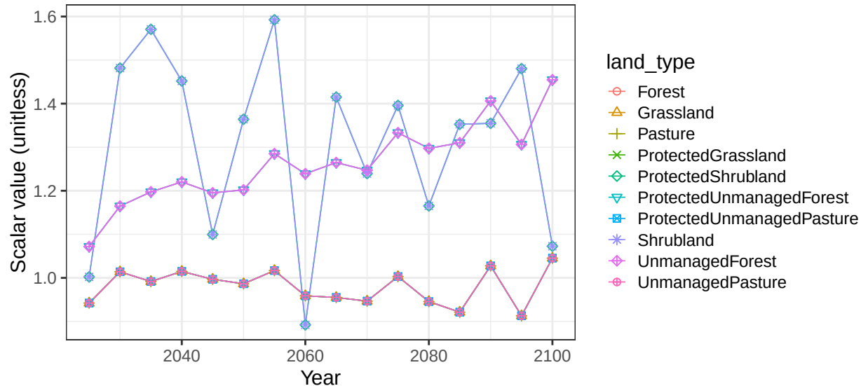
Region Mexico basin RioVerde non-crop vegetation scalars
