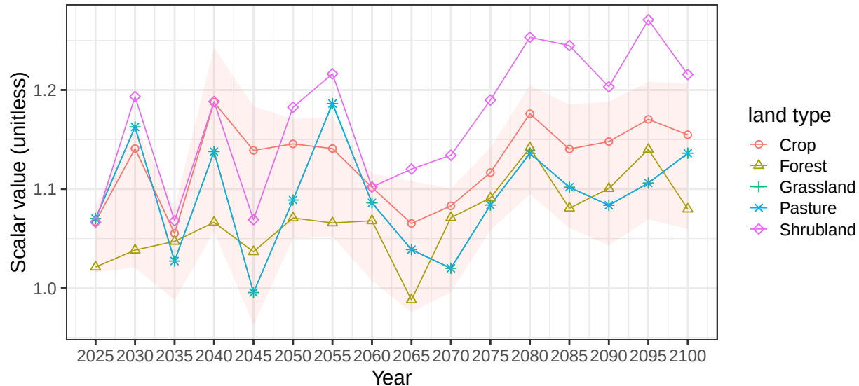
Region Taiwan basin Taiwan average vegetation scalars
