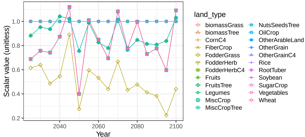
Region Europe_Eastern basin DnieperR crop vegetation scalars
