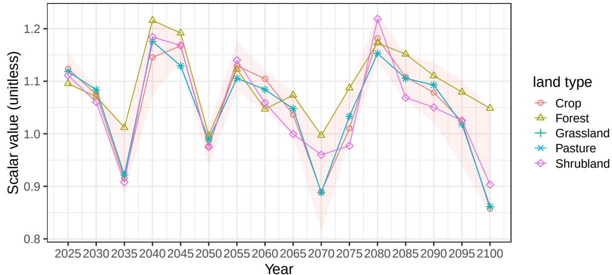
Region South Africa basin LimpopoR average soil scalars
