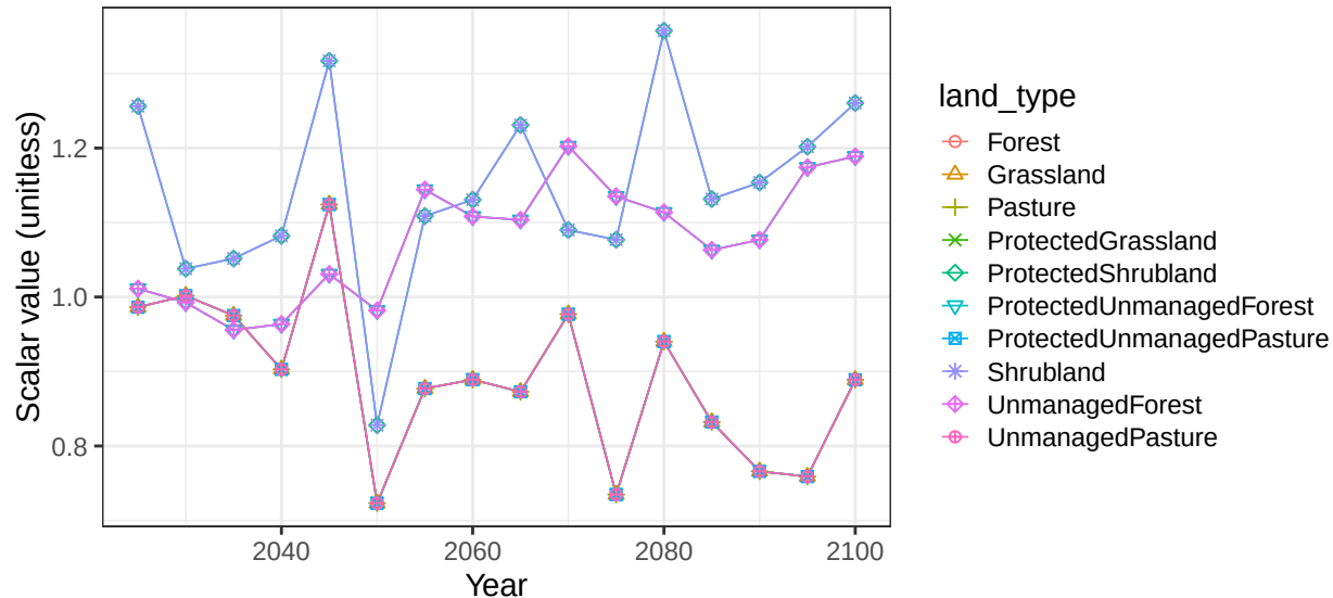
Region Russia basin DonR non-crop soil scalars
