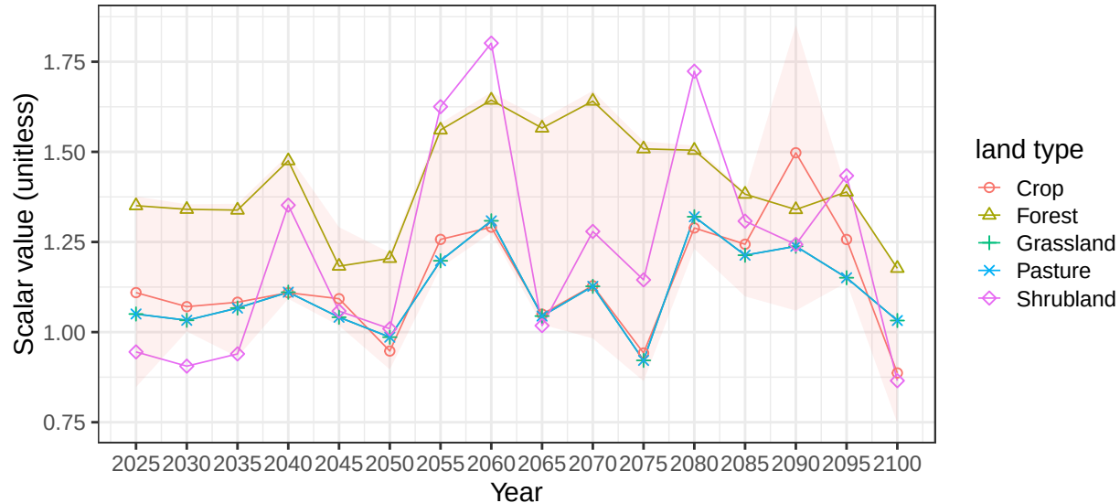
Region Africa_Southern basin AfrIntS average vegetation scalars
