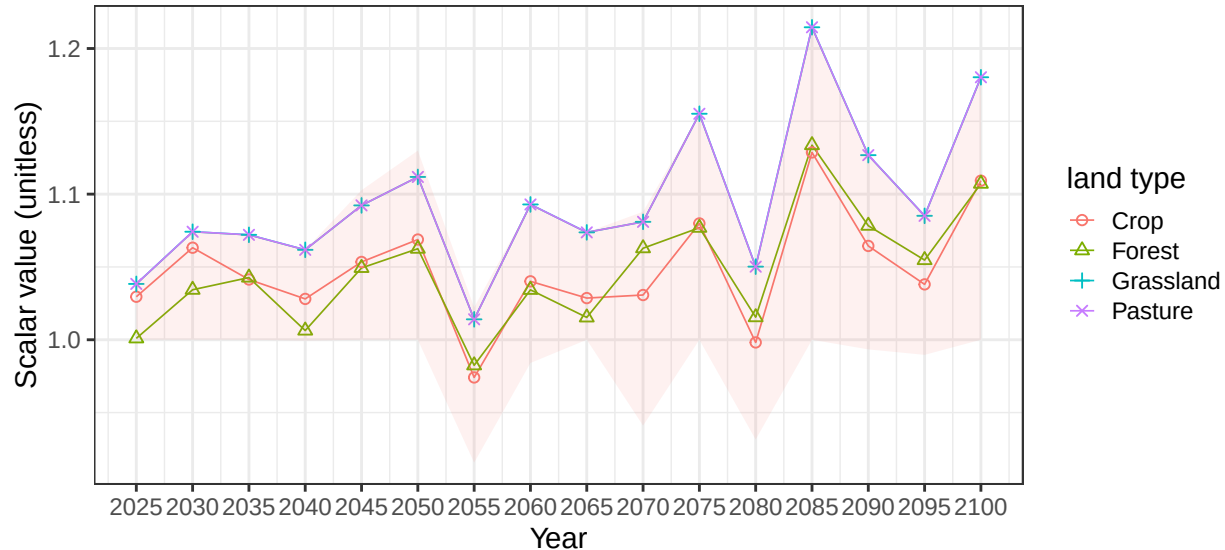
Region USA basin UsaCstE average vegetation scalars
