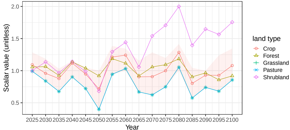
Region EU-12 basin DanubeR average vegetation scalars
