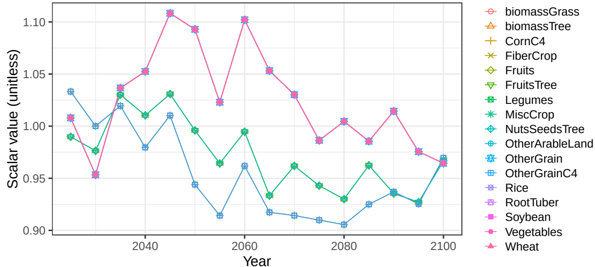
Region Southeast Asia basin RusCstSE crop soil scalars land_type
