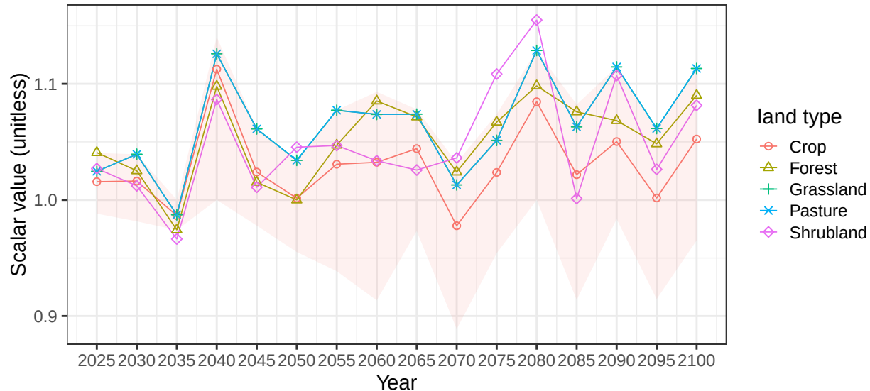
Region EU-15 basin Gironde average soil scalars
