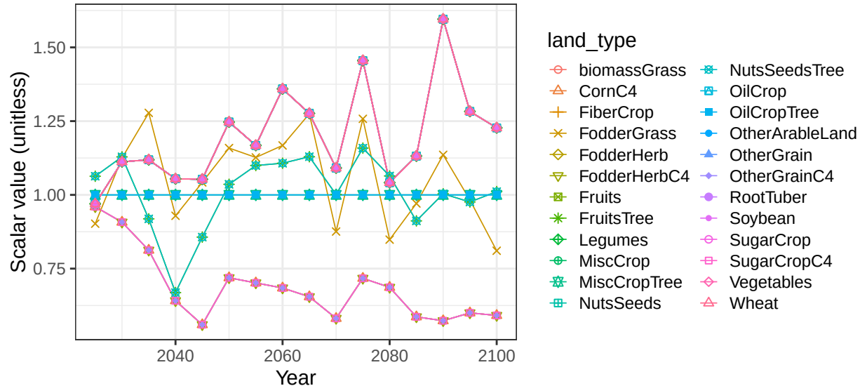
Region Middle East basin EJrdnSyr crop vegetation scalars
