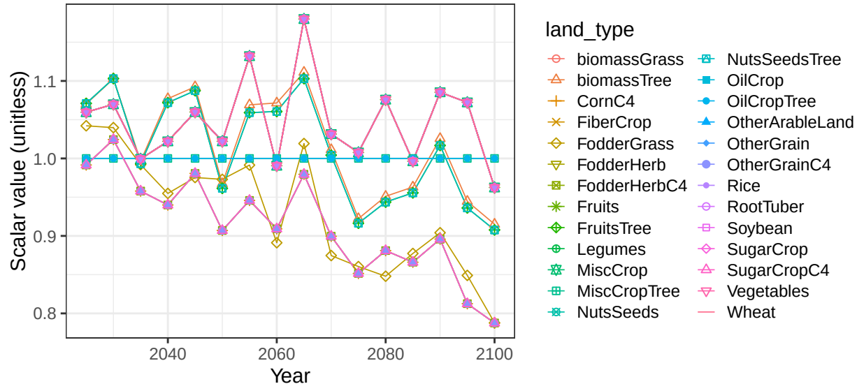
Region Africa_Northern basin MeditS crop soil scalars
