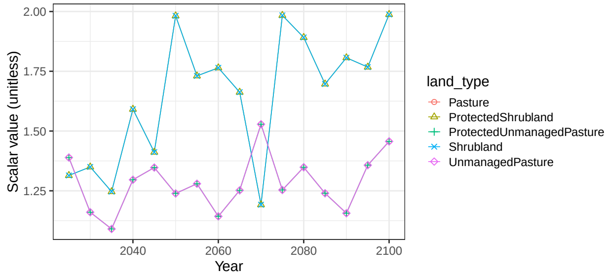
Region Pakistan basin Helmand non-crop vegetation scalars
