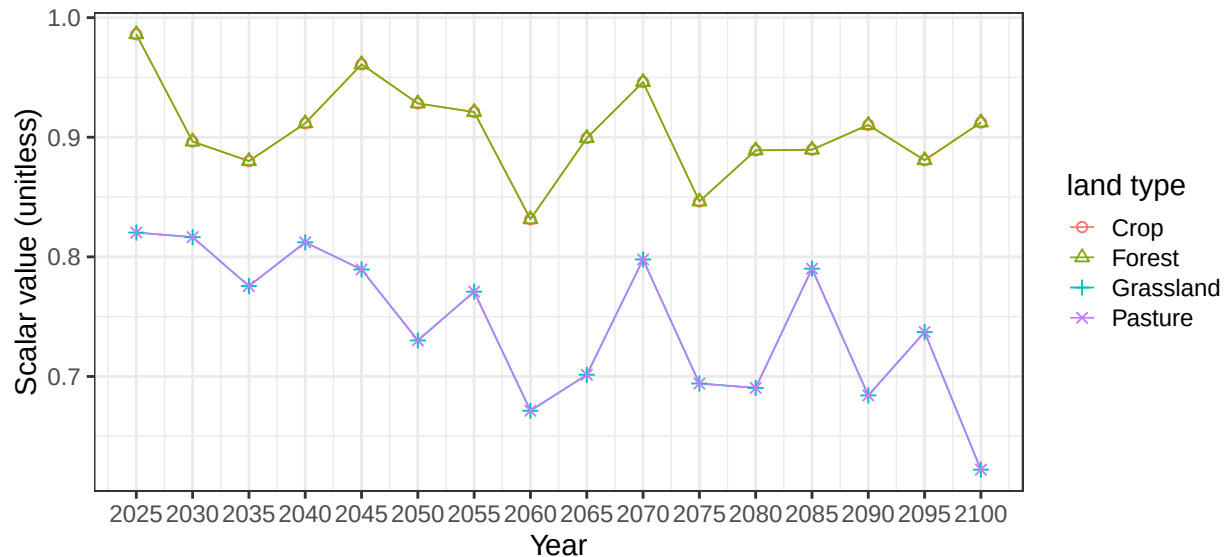
Region India basin AdnNicIsl average vegetation scalars
