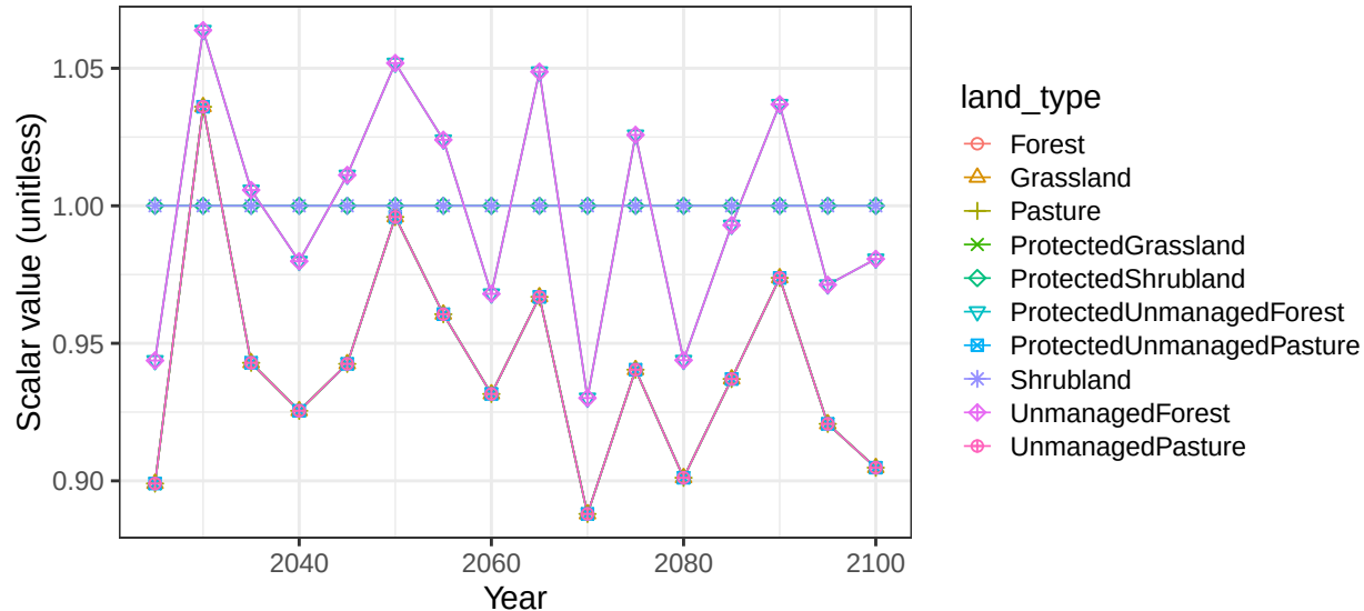
Region Mexico basin RioLerma non-crop soil scalars
