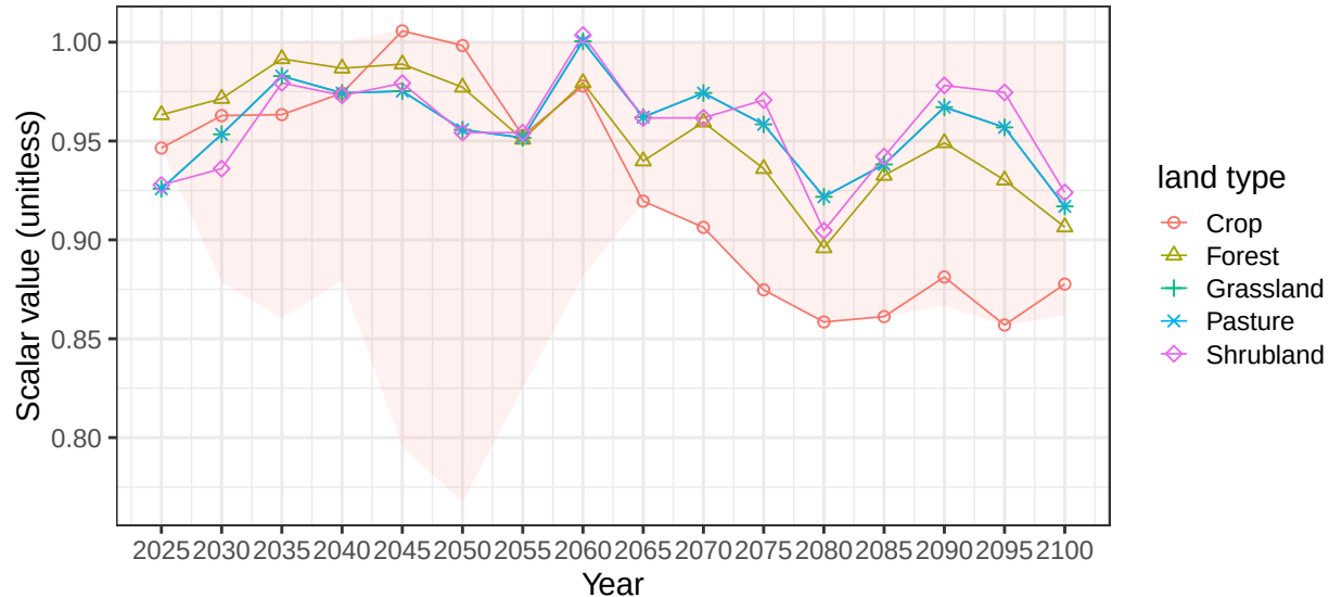
Region Canada basin HudsonBay average soil scalars
