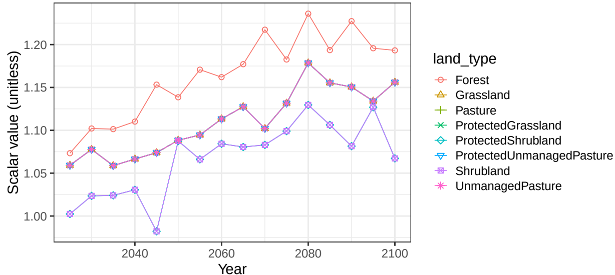
Region China basin Yangtze non-crop vegetation scalars
