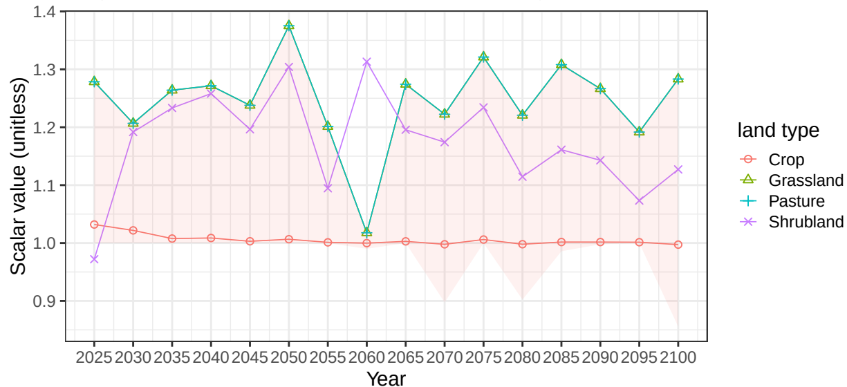
Region Middle East basin ArabianSea average soil scalars
