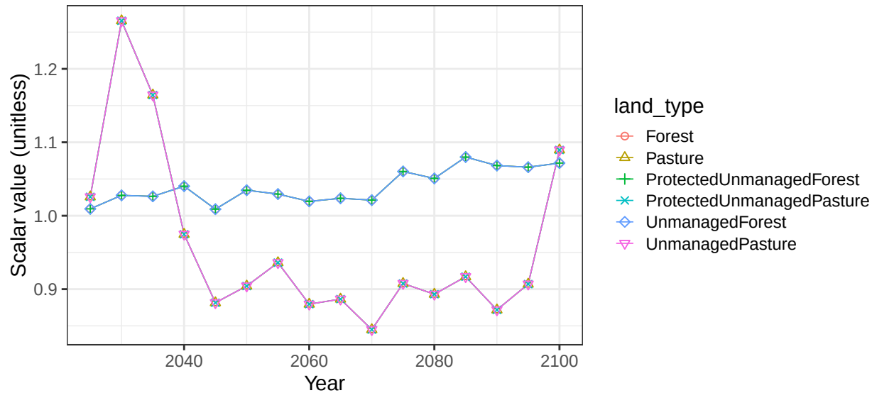
Region Southeast Asia basin Kalimantan non-crop vegetation scalars
