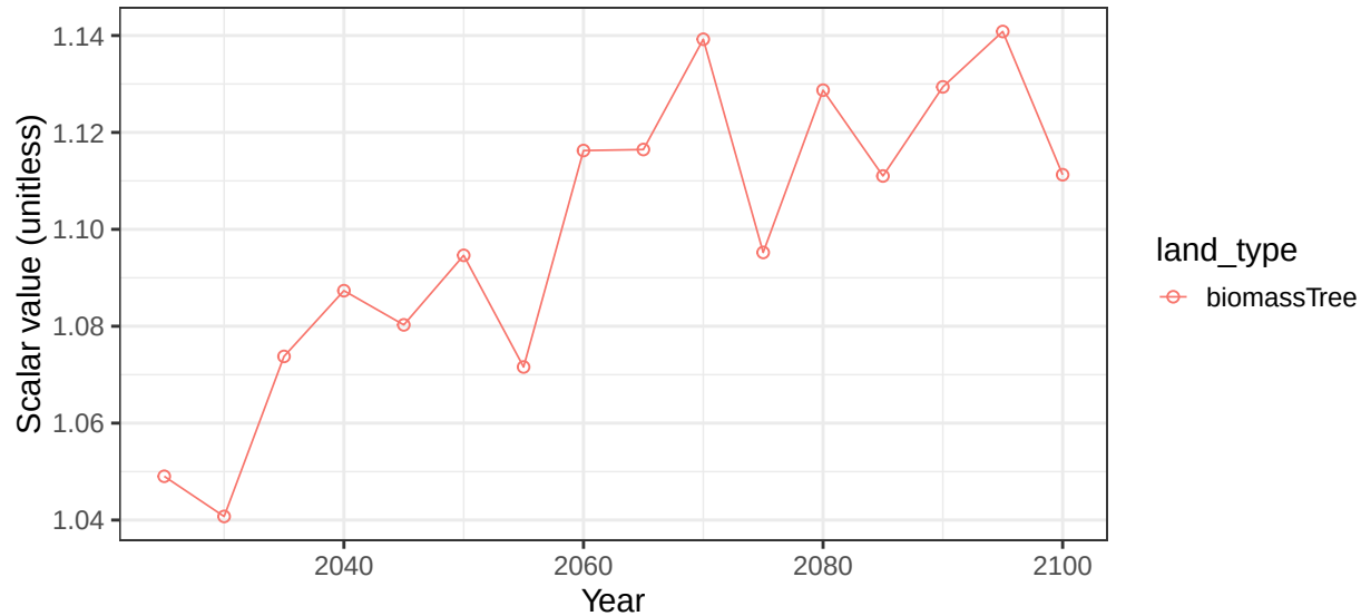
Region South America_Northern basin MagdalenaR crop soil scalars
