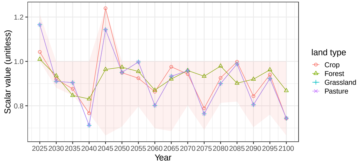
Region Southeast Asia basin NewCaledn average vegetation scalars
