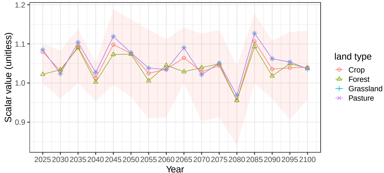
Region USA basin TennR average vegetation scalars
