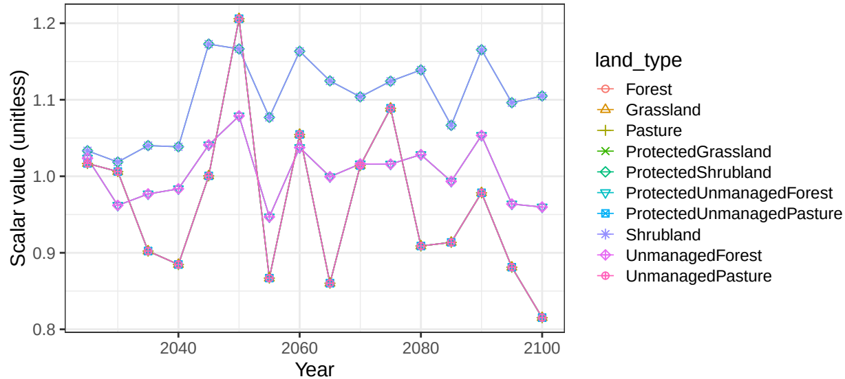
Region Central Asia basin ObR non-crop soil scalars
