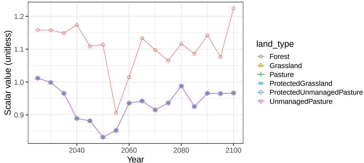
Region India basin BengalBay non-crop soil scalars
