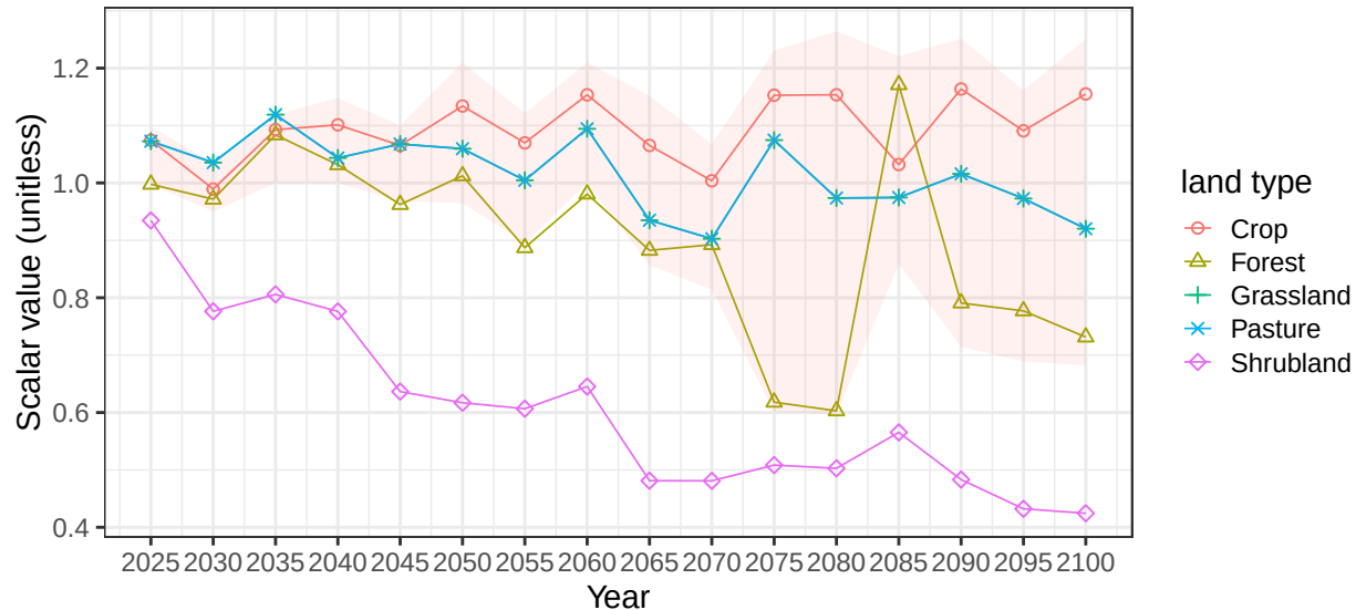
Region Africa_Eastern basin RiftValley average soil scalars
