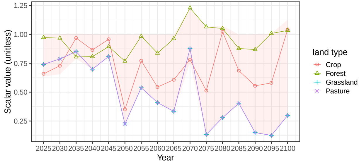
Region Europe_Eastern basin DonR average vegetation scalars
