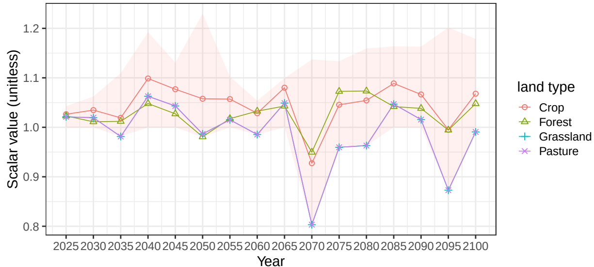
Region EU-15 basin LoireR average soil scalars
