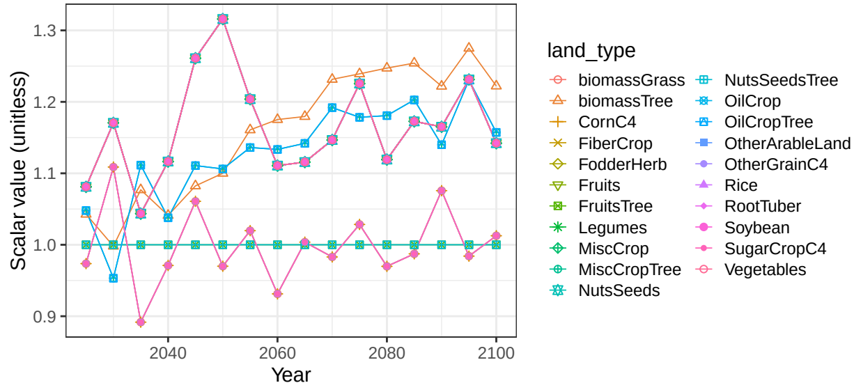
Region Southeast Asia basin XunJiang crop vegetation scalars
