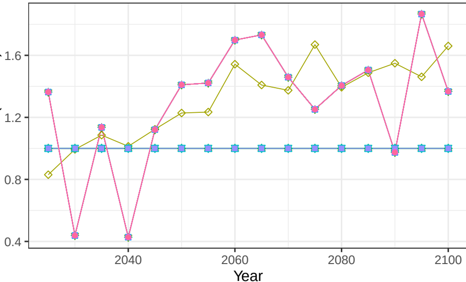
Region Russia basin Finland crop vegetation scalars
