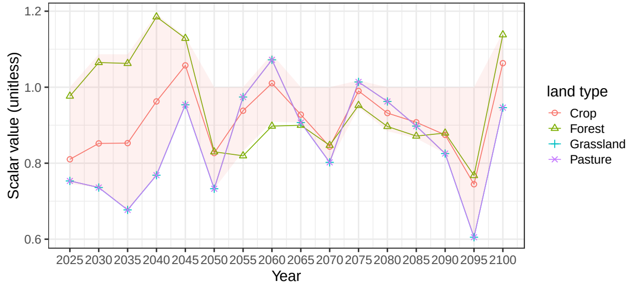
Region EU-12 basin OderR average vegetation scalars
