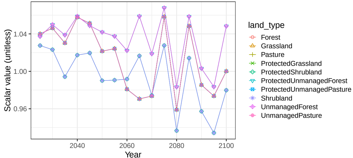
Region Canada basin FraserR non-crop soil scalars
