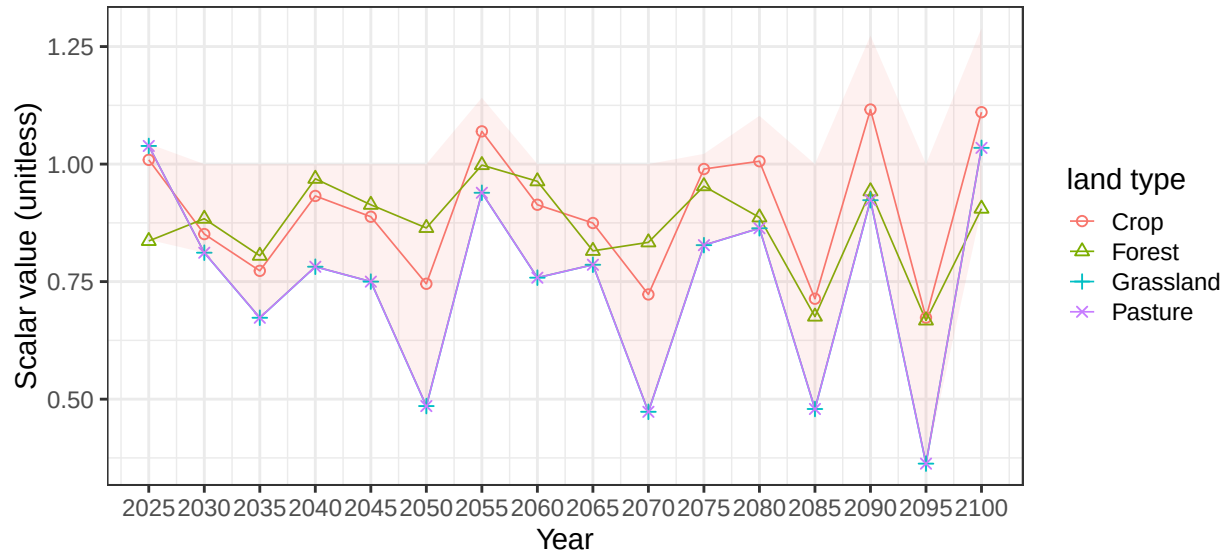
Region EU-12 basin DniesterR average vegetation scalars
