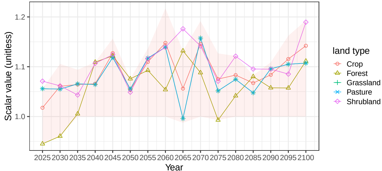
Region India basin IndCstS average soil scalars
