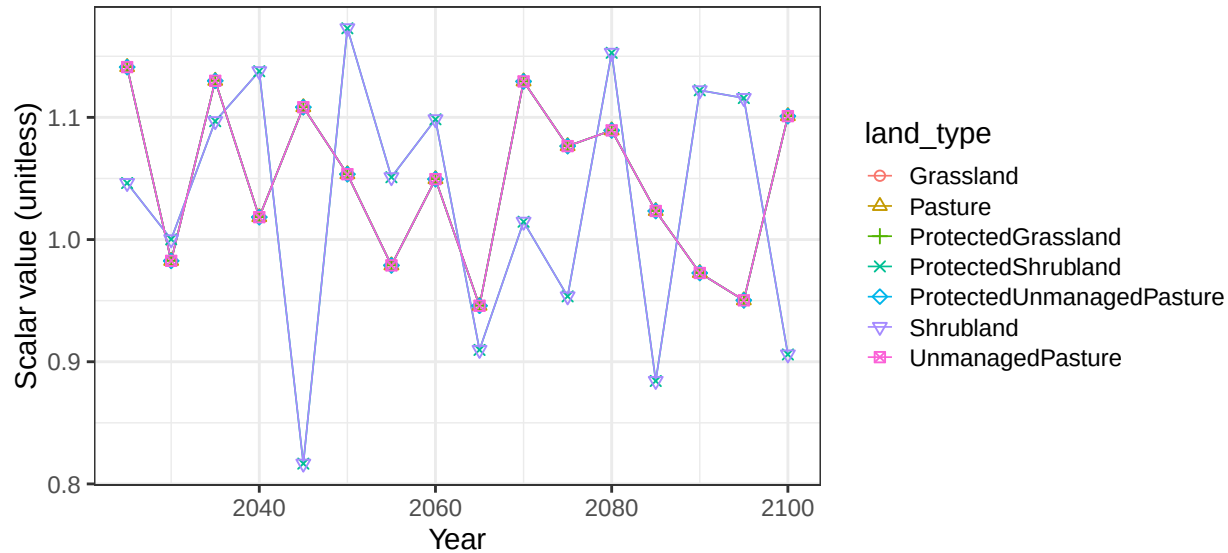
Region Africa_Southern basin AfrCstSW non-crop soil scalars
