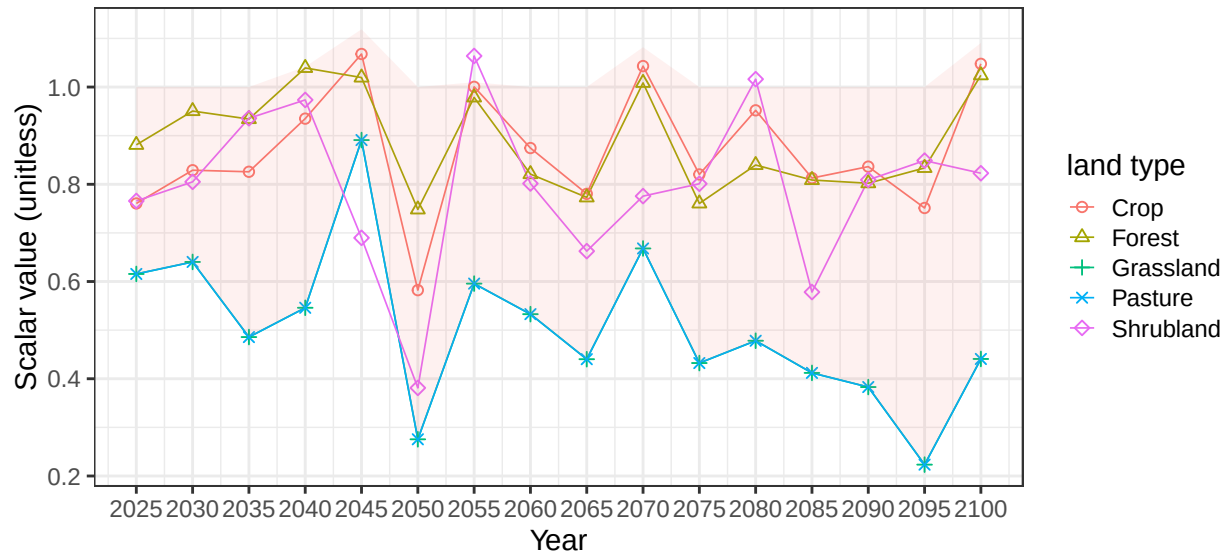
Region Europe_Eastern basin DnieperR average vegetation scalars
