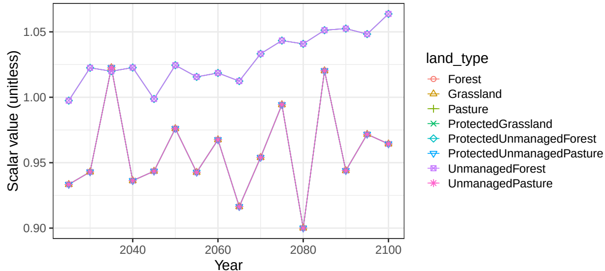
Region Indonesia basin IrianJaya non-crop vegetation scalars
