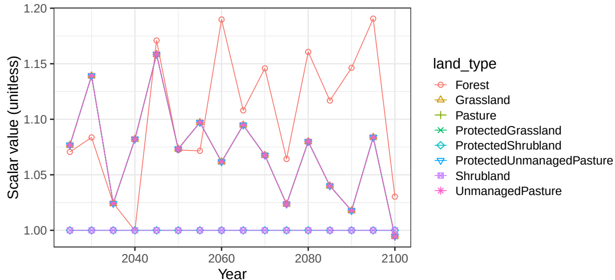
Region India basin KrishnaR non-crop soil scalars
