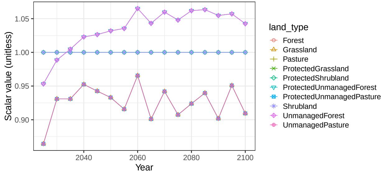
Region Brazil basin BrzCstN non-crop soil scalars
