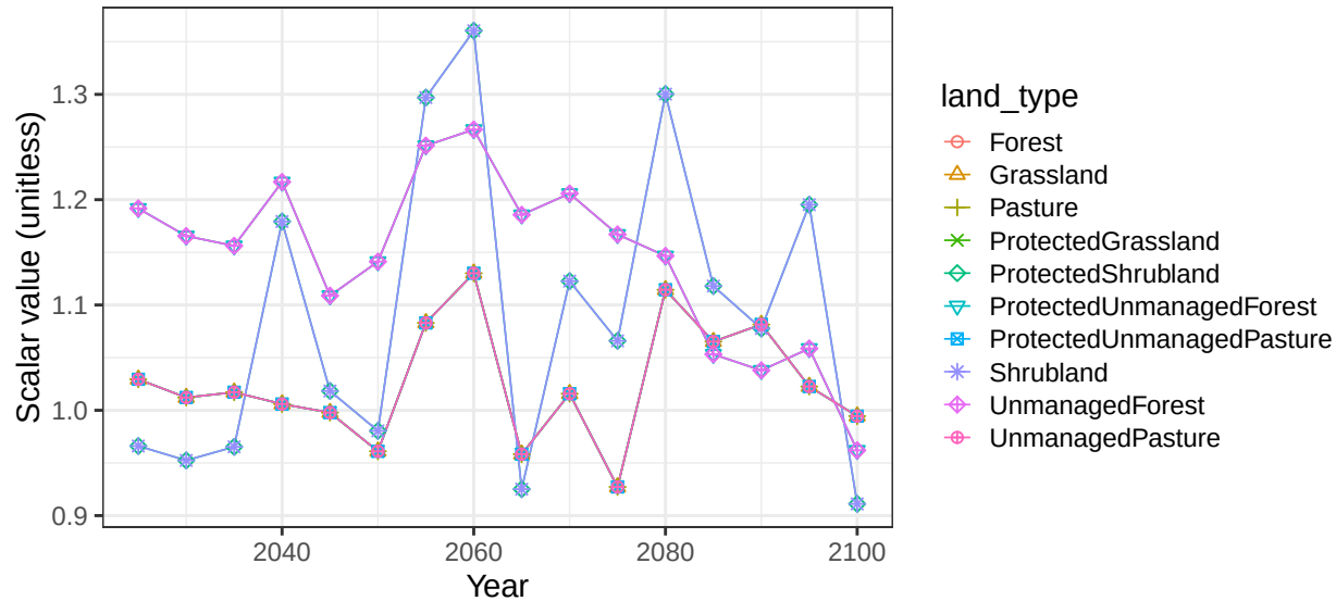
Region Africa_Southern basin AfrIntS non-crop soil scalars
