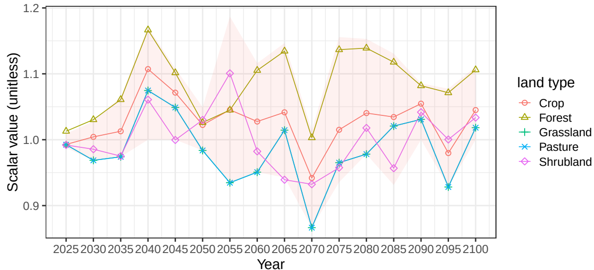
Region EU-15 basin FranceCstW average soil scalars
