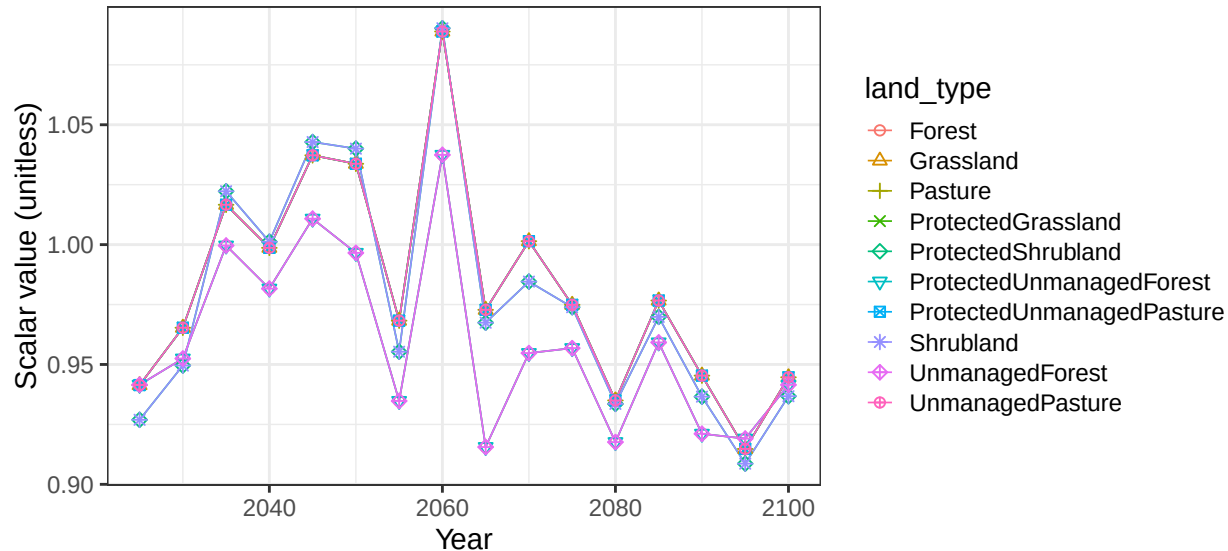
Region Russia basin DvinaRN non-crop soil scalars
