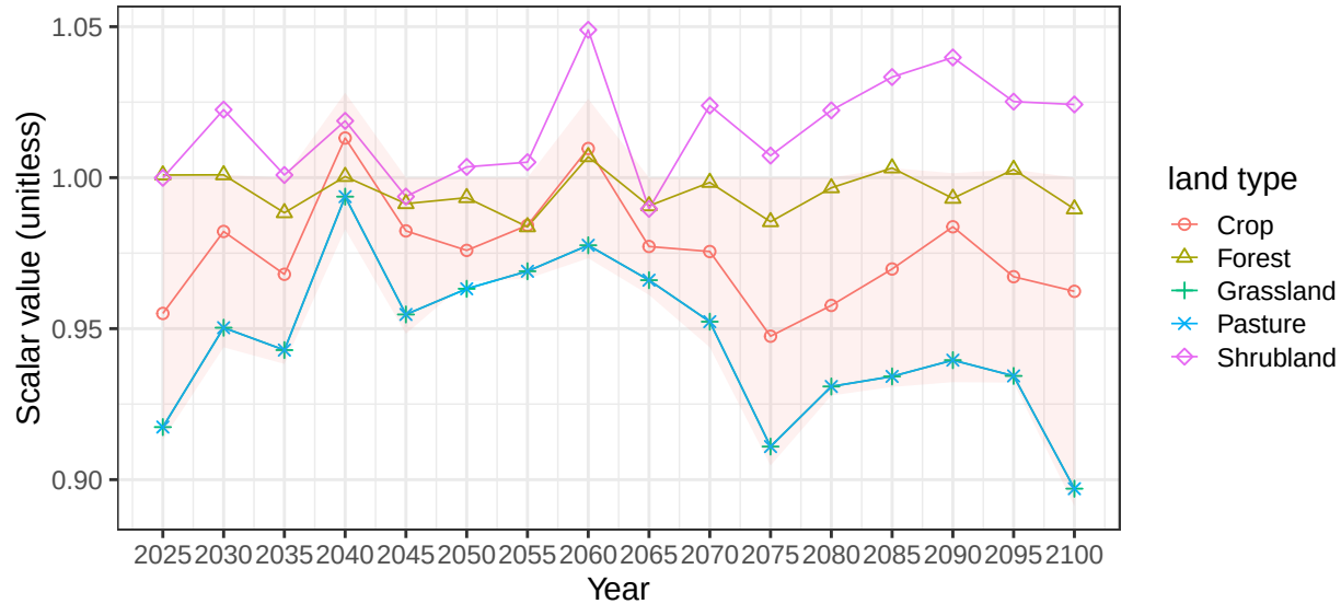
Region Brazil basin AmazonR average soil scalars
