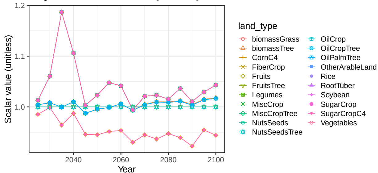
Region Indonesia basin SepikR crop soil scalars
