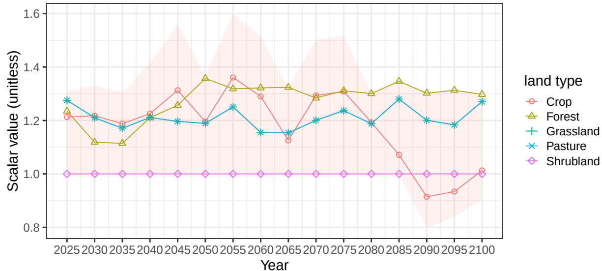
Region Africa_Southern basin AngolaCst average vegetation scalars
