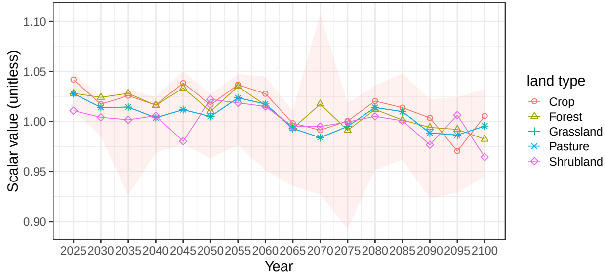
Region China basin Yangtze average soil scalars
