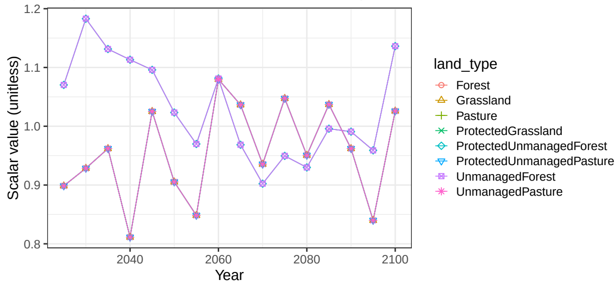
Region EU-12 basin PolandCst non-crop soil scalars
