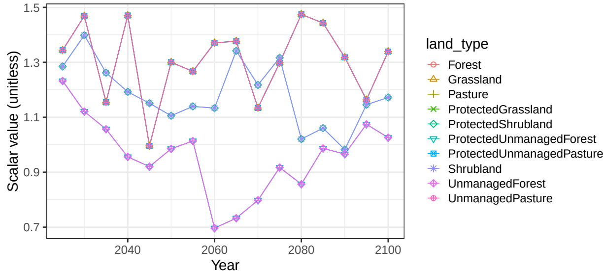
Region Canada basin MissouriR non-crop vegetation scalars
