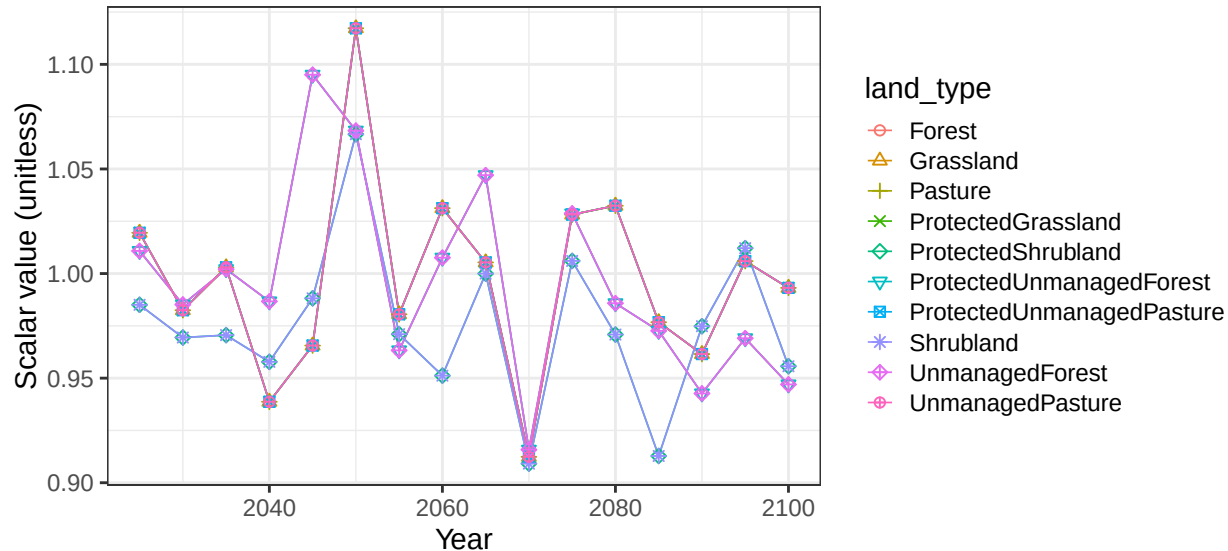
Region Central Asia basin LBalkash non-crop soil scalars
