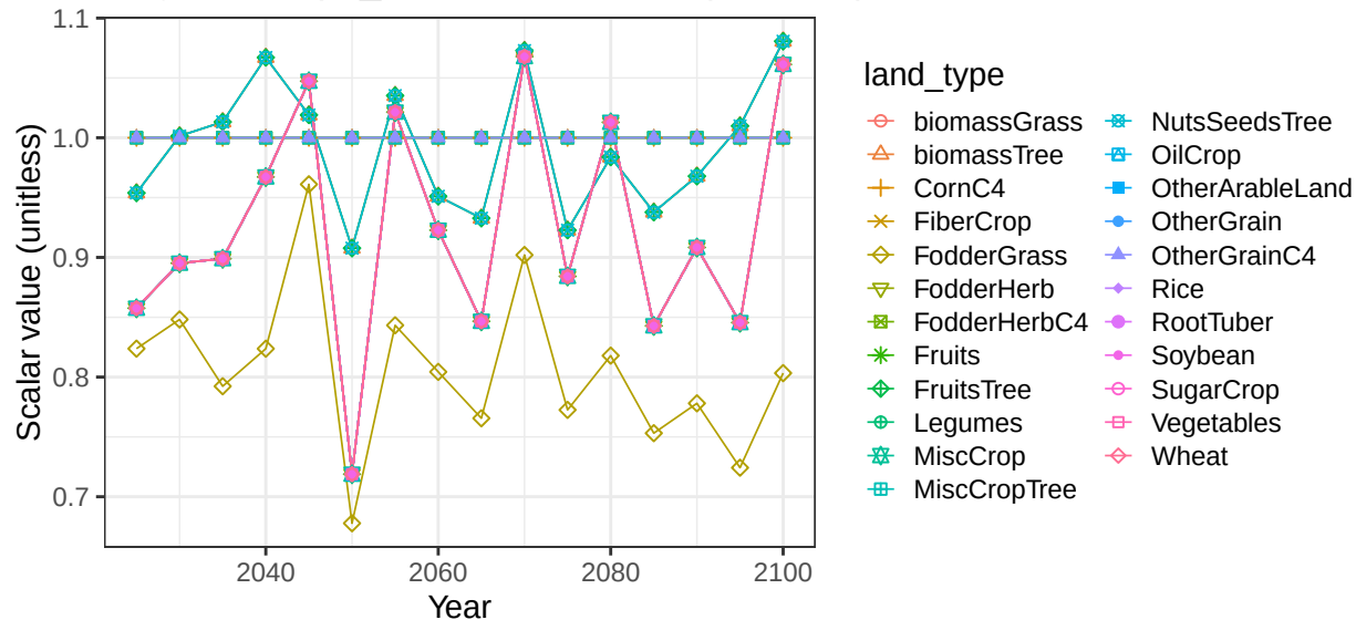
Region Europe_Eastern basin DnieperR crop soil scalars
