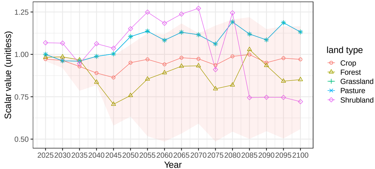
Region Africa_Eastern basin Madagascar average soil scalars
