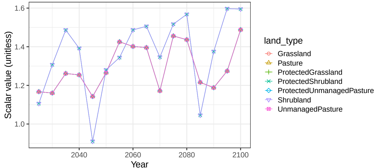
Region South Asia basin CaspianE non-crop vegetation scalars
