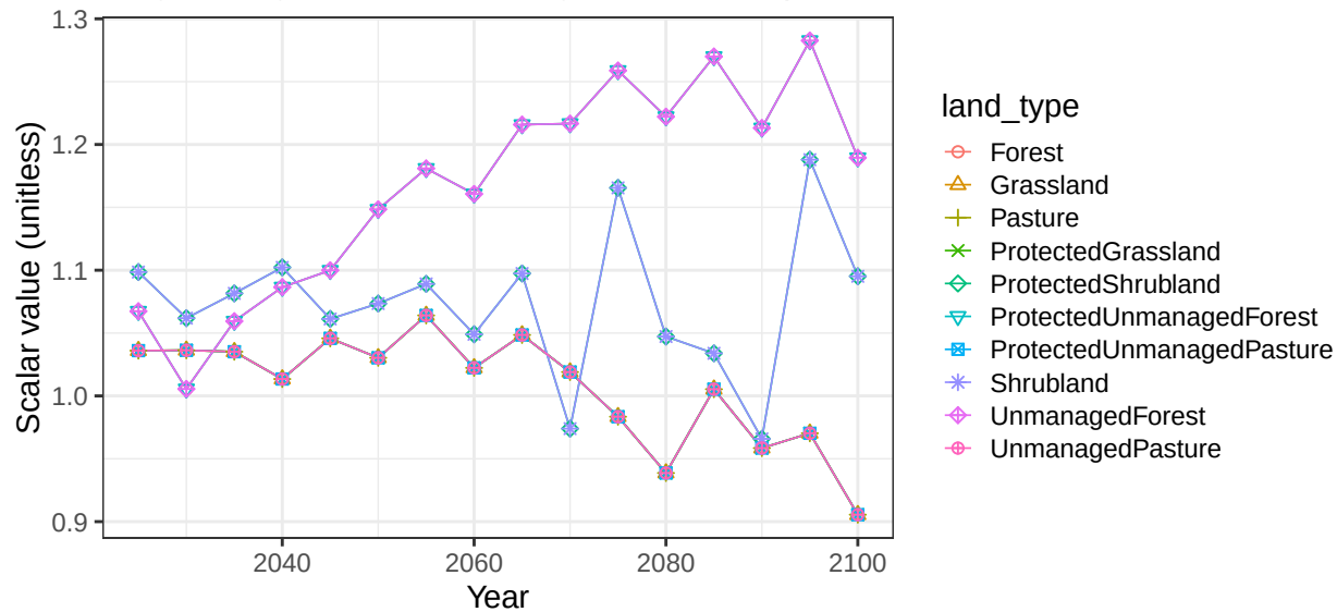
Region Argentina basin NegroR non-crop soil scalars
