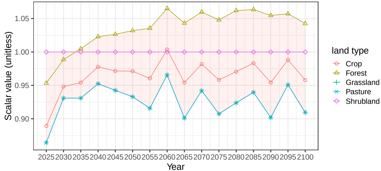
Region Brazil basin BrzCstN average soil scalars
