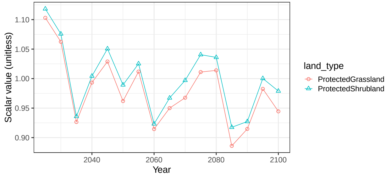
Region EU-15 basin ArcticIsI non-crop soil scalars
