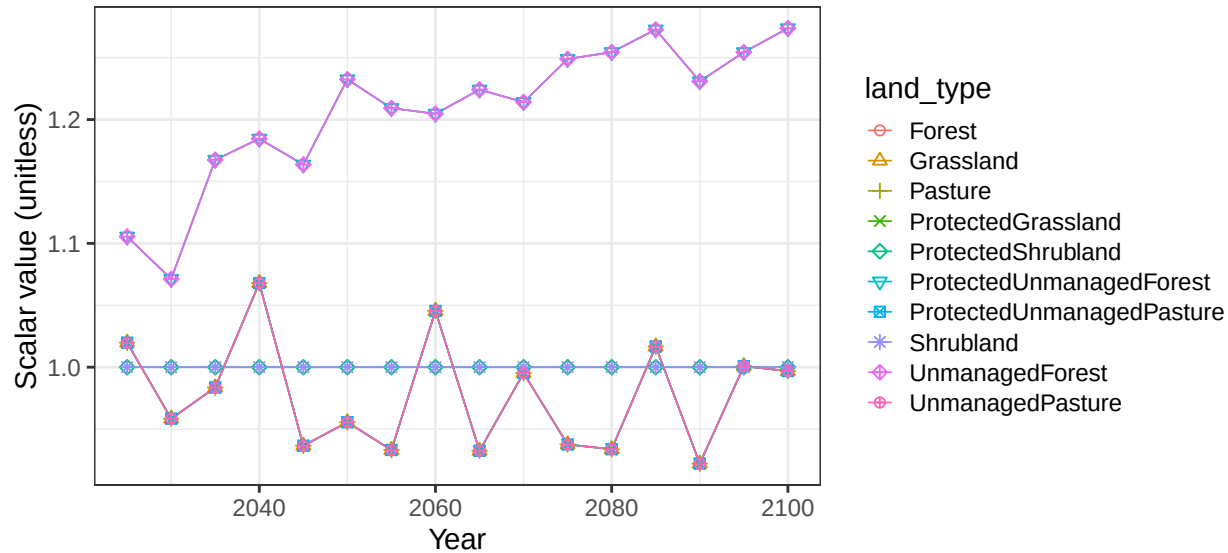
Region Brazil basin ParnaibaR non-crop soil scalars
