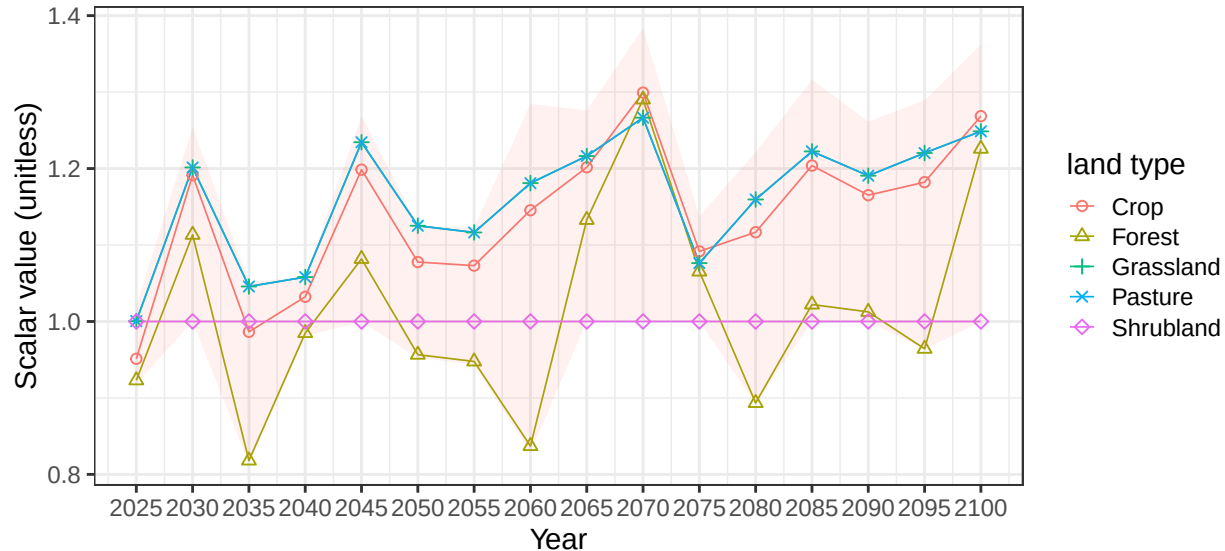
Region India basin CauveryR average vegetation scalars
