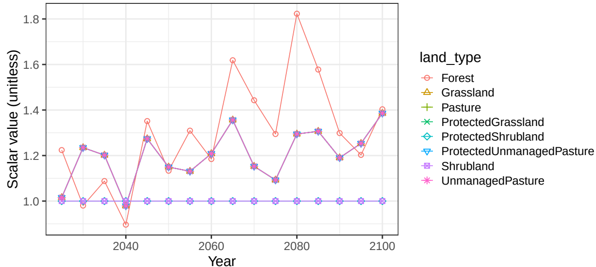
Region India basin MahanadiR non-crop vegetation scalars
