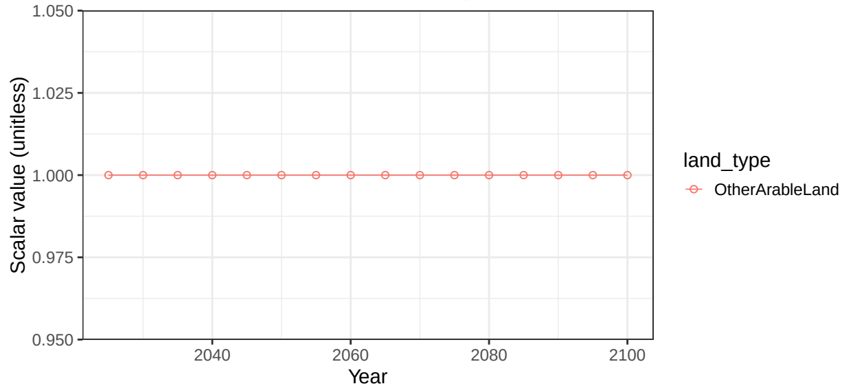
Region Russia basin BlackSeaS crop vegetation scalars
