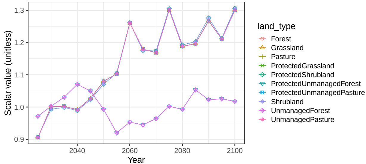
Region Russia basin Finland non-crop soil scalars
