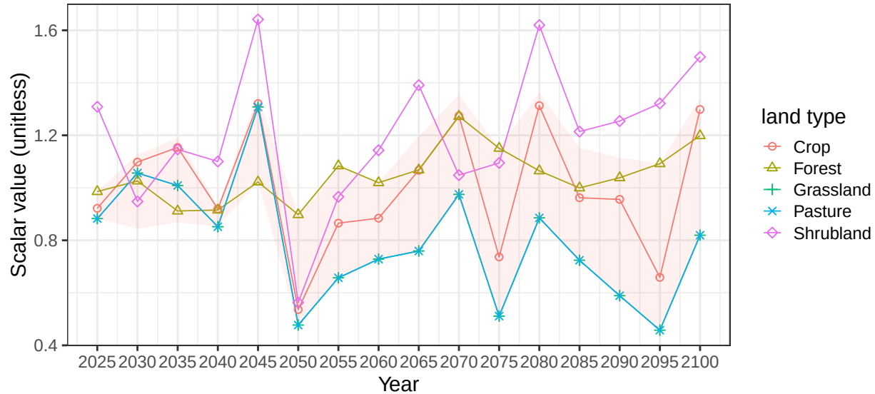
Region Russia basin DonR average vegetation scalars
