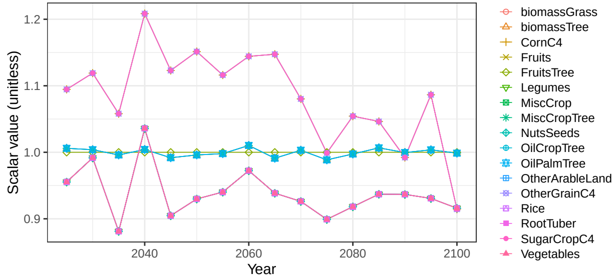
Region South America_Northern basin AmazonR crop soil scalars
