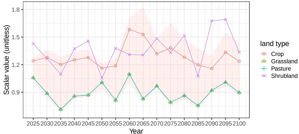
Region Pakistan basin ArabianSea average vegetation scalars
