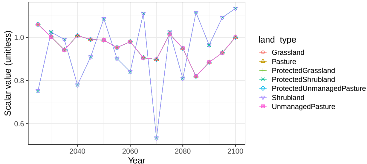
Region Middle East basin RedSeaE non-crop soil scalars
