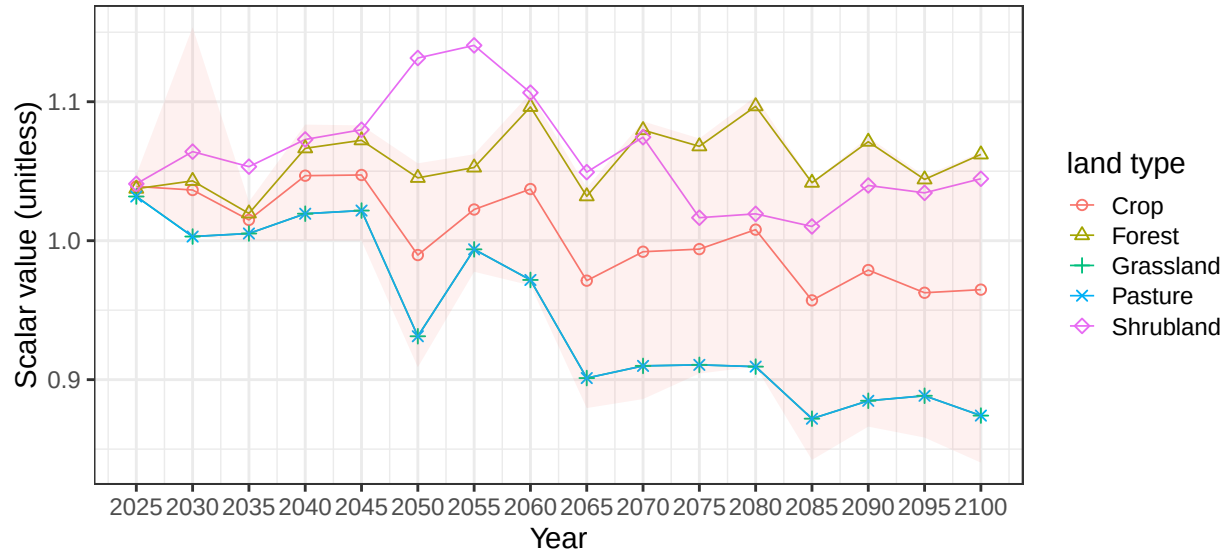
Region EU-15 basin DanubeR average soil scalars
