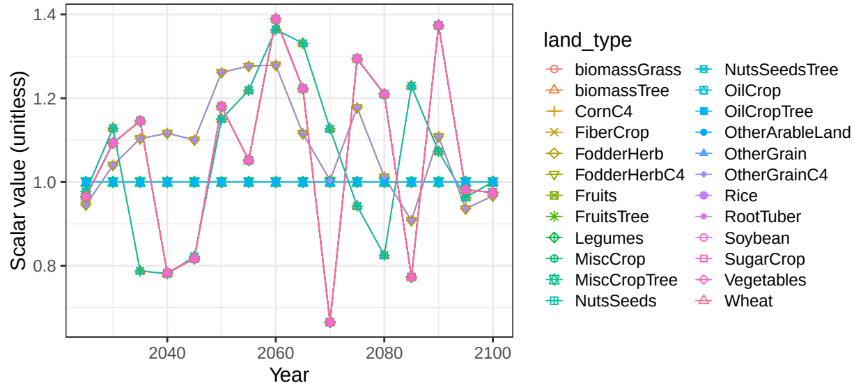
Region Europe_Non_EU basin CaspianSW crop vegetation scalars
