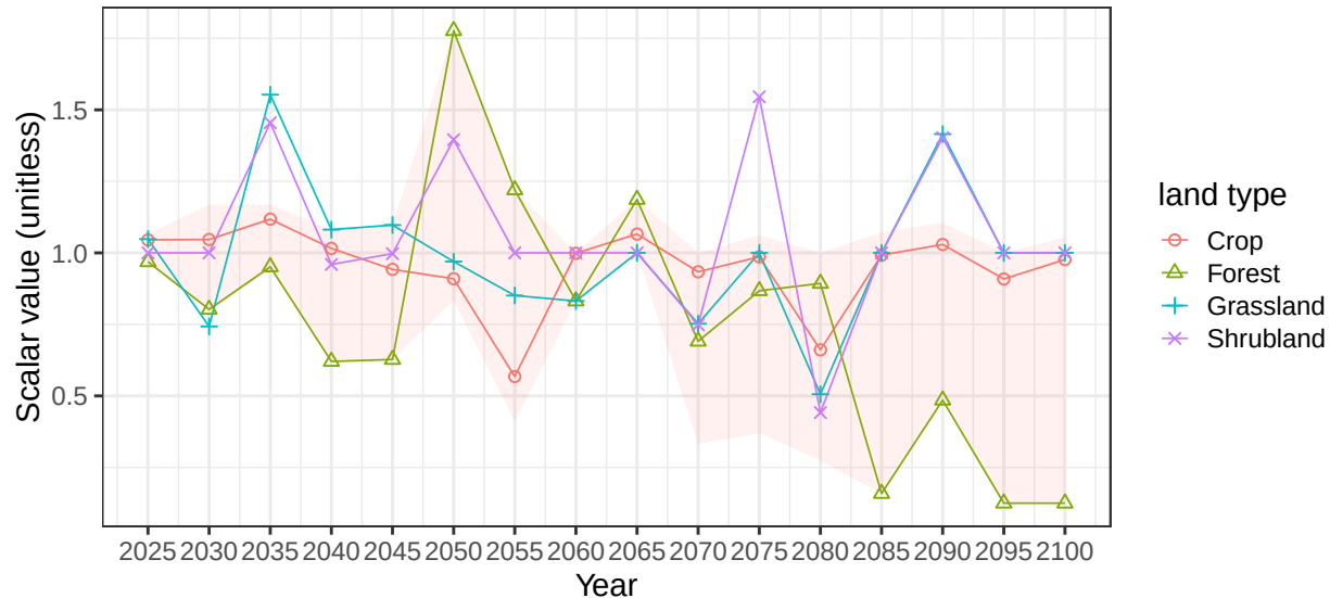
Region Africa_Northern basin NileR average soil scalars
