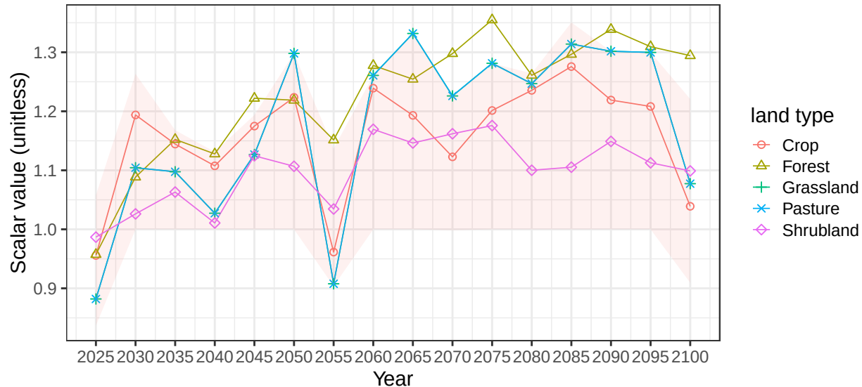
Region China basin AmurR average vegetation scalars
