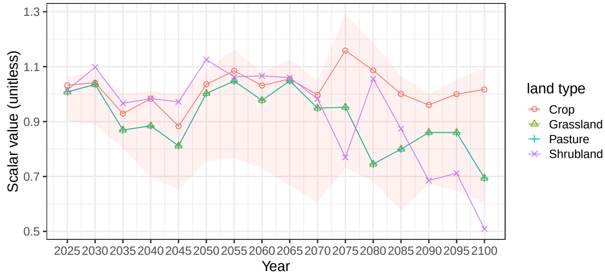
Region Middle East basin MeditE average vegetation scalars
