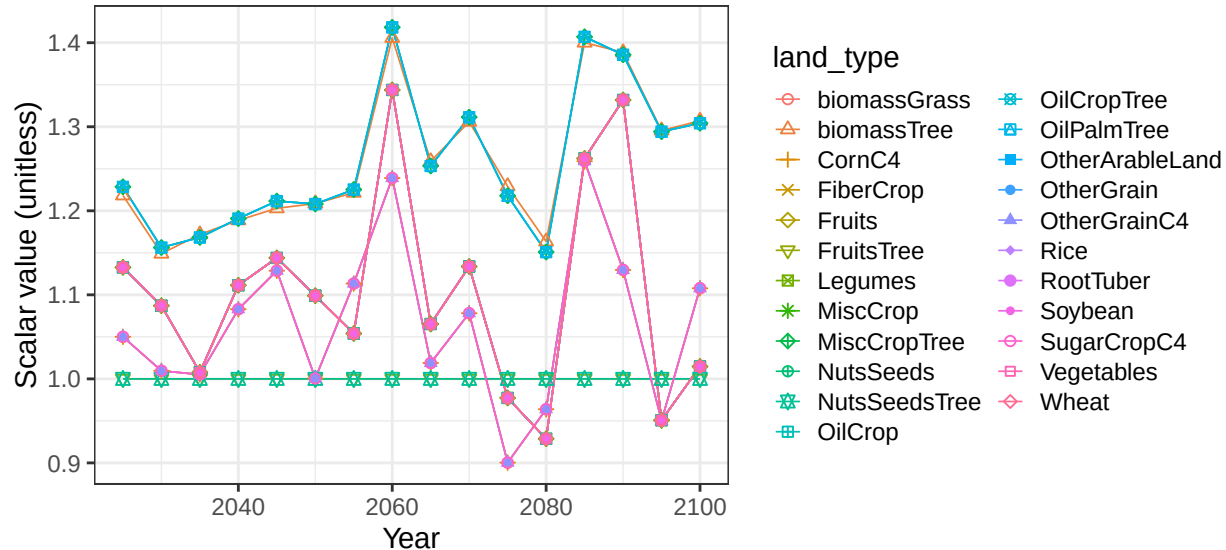
Region Africa_Southern basin ZambeziR crop vegetation scalars
