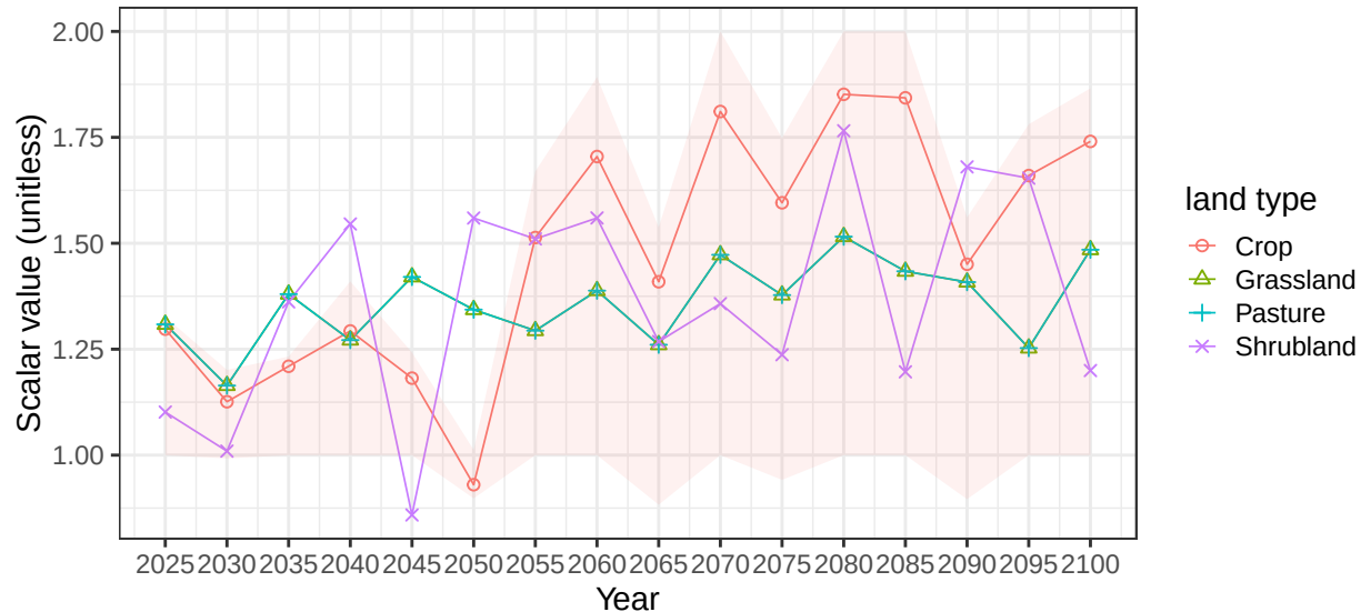
Region Africa_Southern basin AfrCstSW average vegetation scalars
