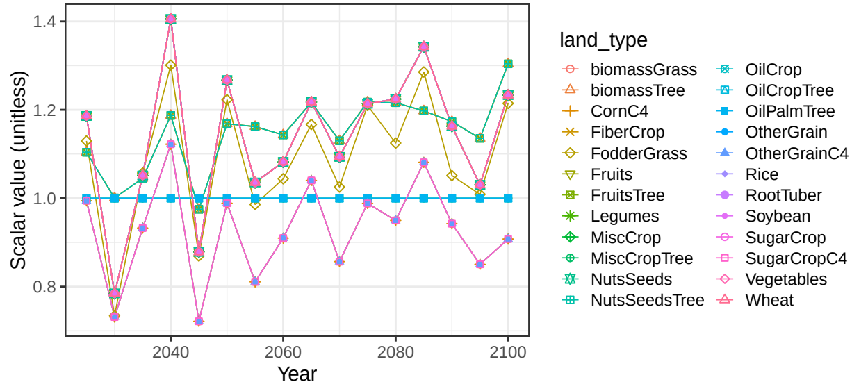
Region China basin ZiyaHe crop vegetation scalars
