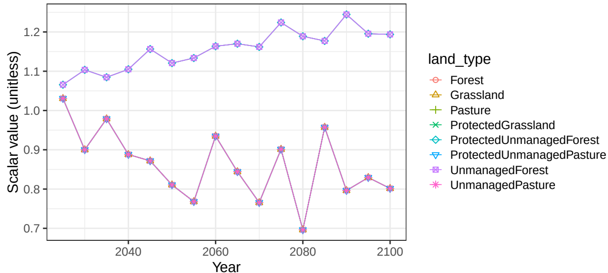
Region Indonesia basin JavaTimor non-crop vegetation scalars
