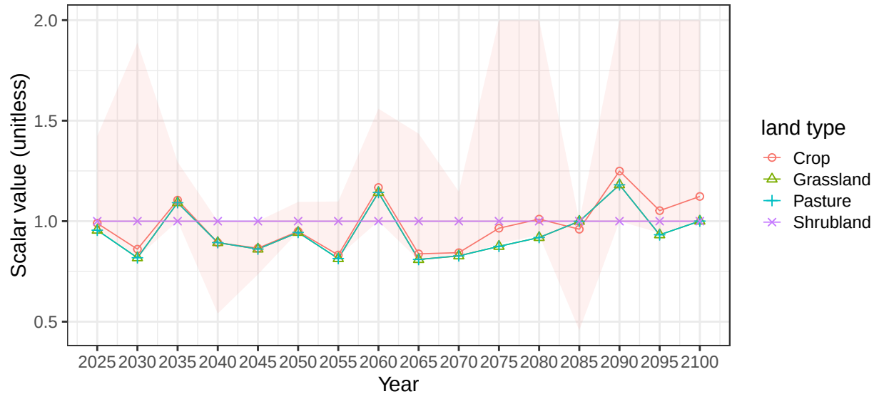
Region Africa_Western basin AfrCstNW average vegetation scalars
