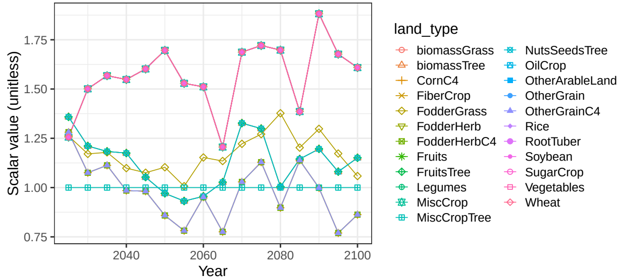
Region USA basin MissppRN crop vegetation scalars
