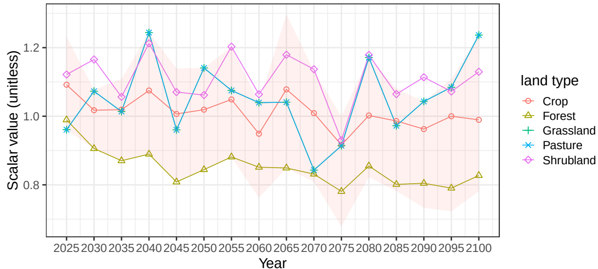
Region EU-15 basin GuadalqR average soil scalars
