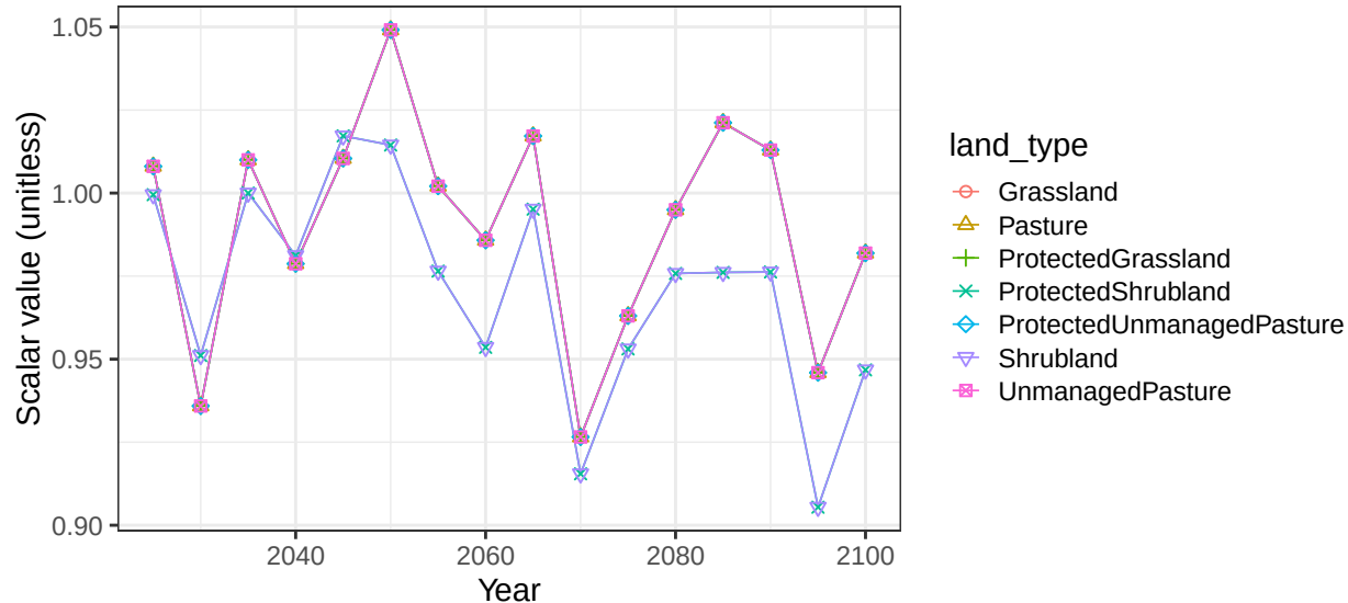
Region Central Asia basin Tarim non-crop soil scalars
