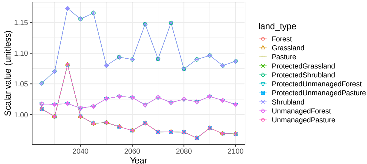
Region Colombia basin MagdalenaR non-crop soil scalars
