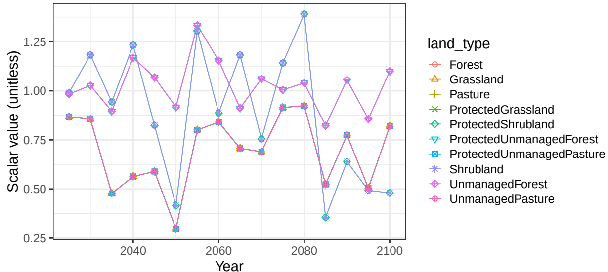
Region Europe_Eastern basin DanubeR non-crop vegetation scalars
