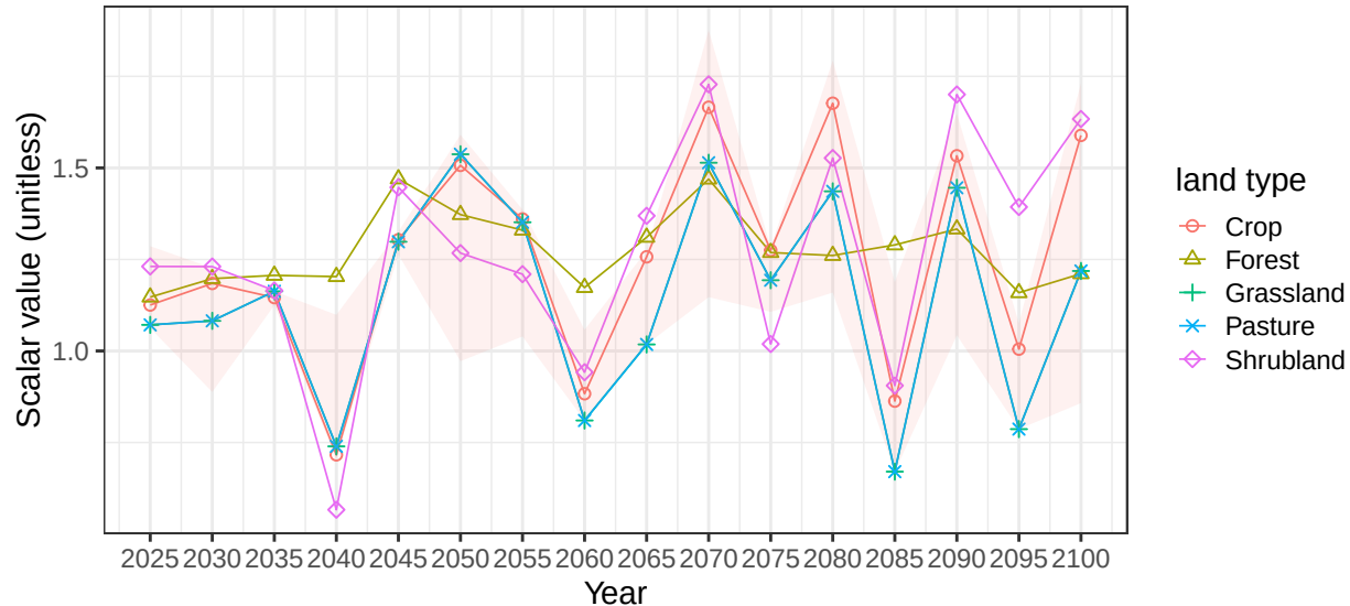
Region Russia basin UralR average vegetation scalars
