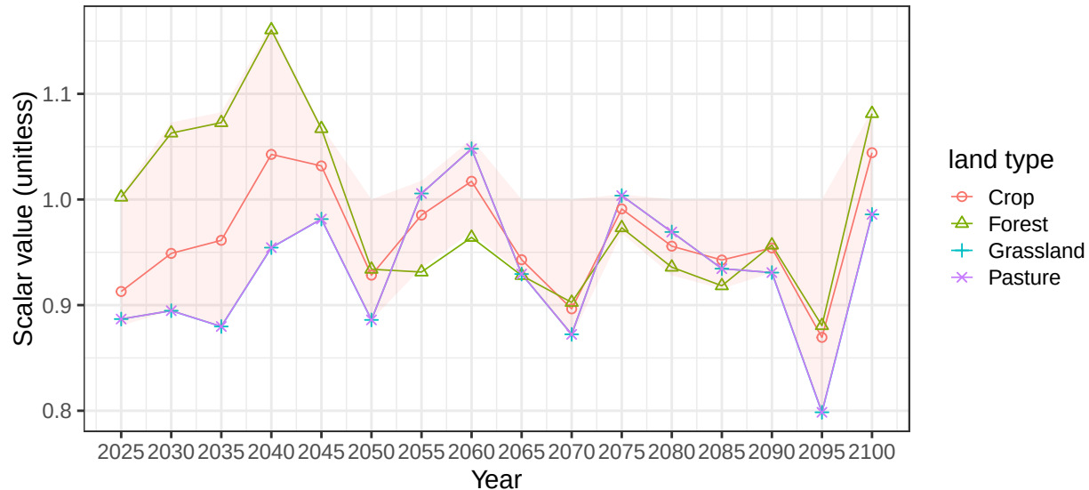
Region EU-12 basin OderR average soil scalars
