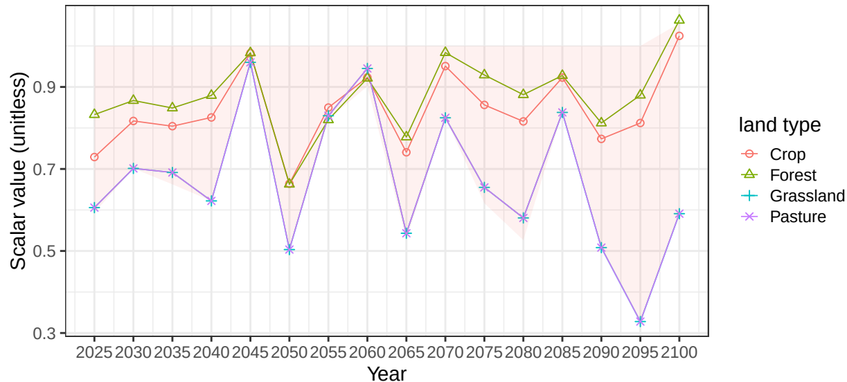
Region Europe_Eastern basin DaugavaR average vegetation scalars
