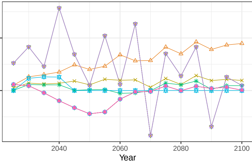
Region Argentina basin ChileCstS crop vegetation scalars land_type
