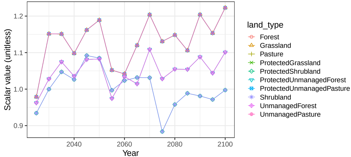
Region Canada basin GreatLakes non-crop vegetation scalars
