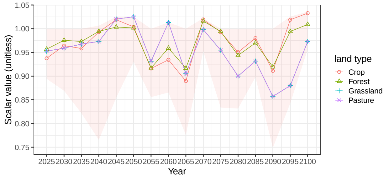
Region Russia basin NevaR average soil scalars
