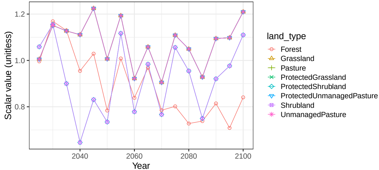
Region India basin IndusR non-crop vegetation scalars
