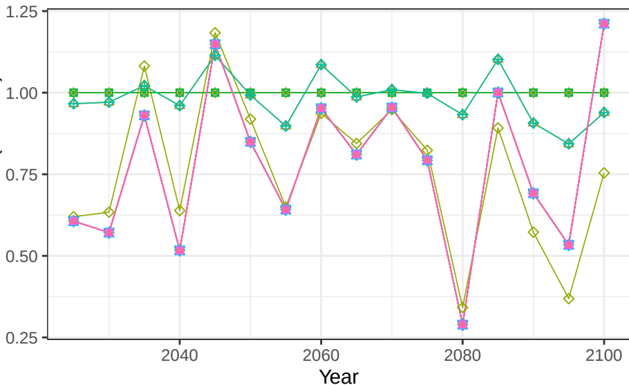
Region EU-12 basin BalticSea crop vegetation scalars
