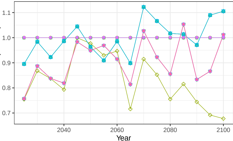
Region Europe_Eastern basin NevaR crop soil scalars
