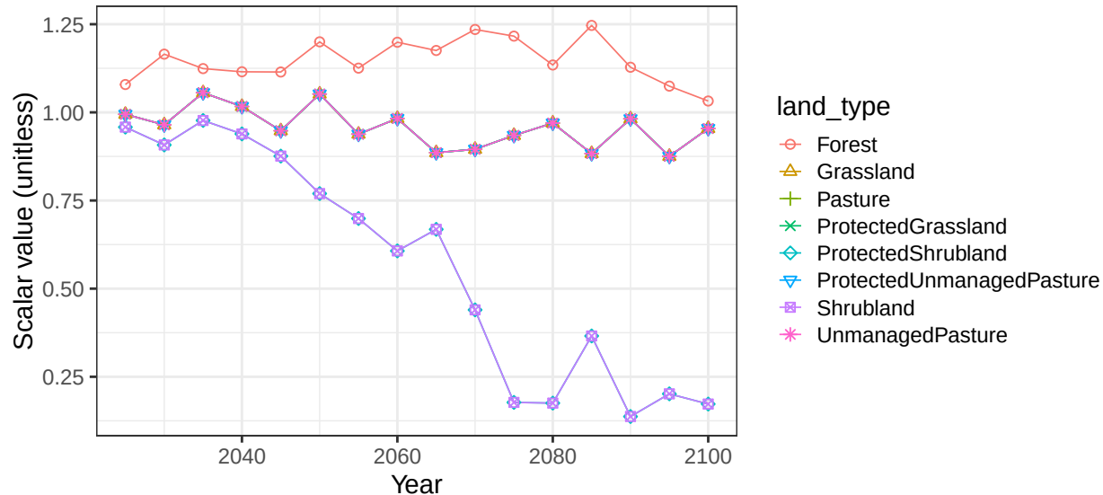
Region Africa_Eastern basin NileR non-crop soil scalars
