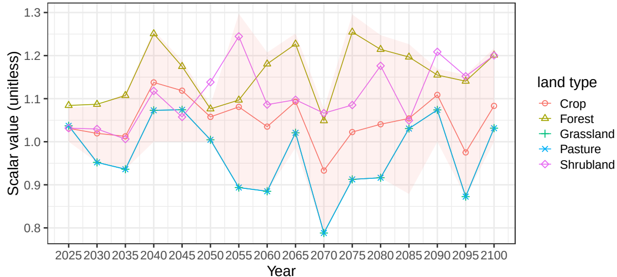
Region EU-15 basin FranceCstW average vegetation scalars
