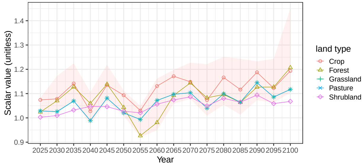
Region South Asia basin GangesR average soil scalars
