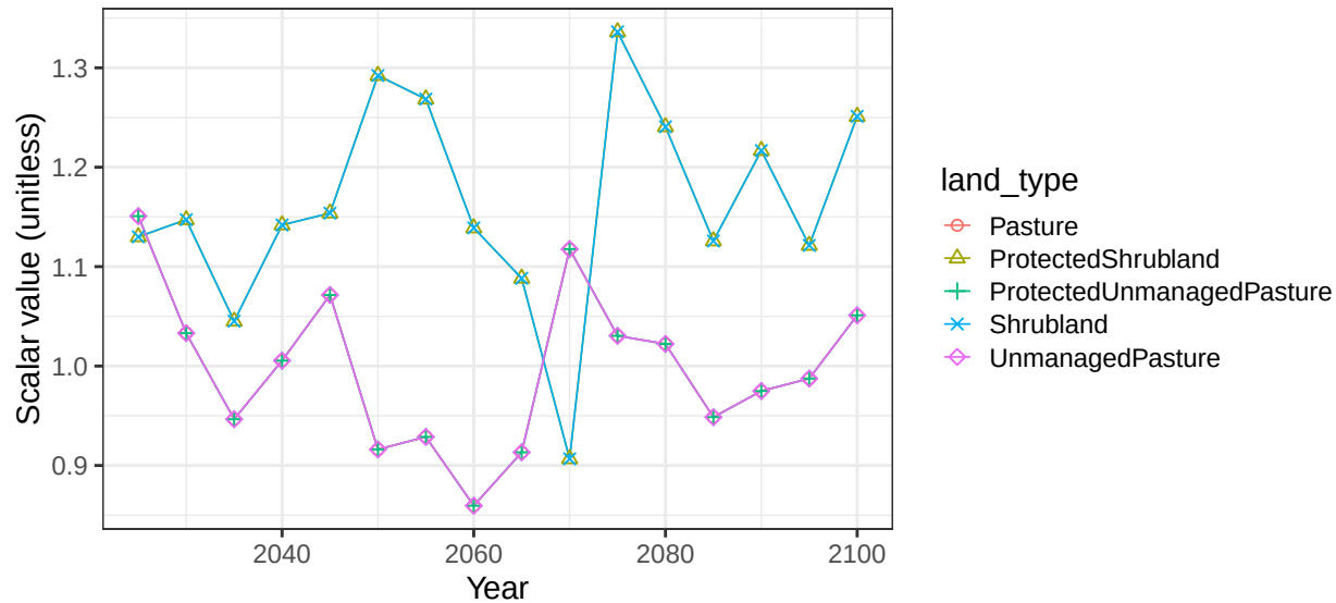
Region Pakistan basin Helmand non-crop soil scalars
