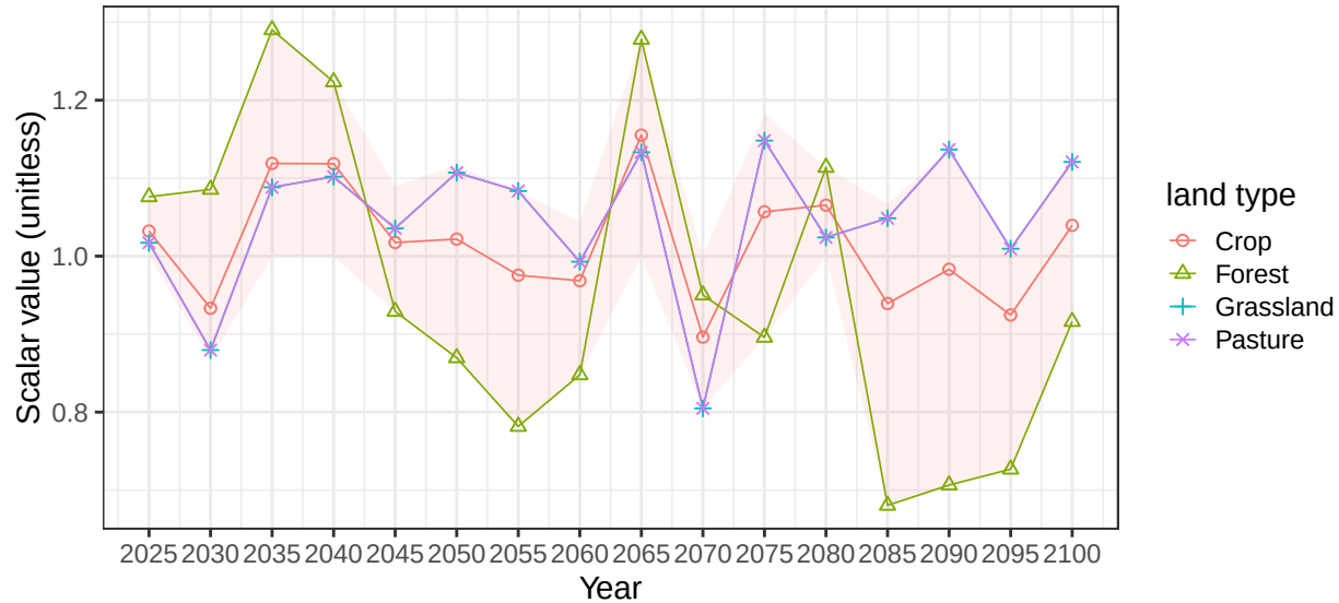
Region EU-15 basin ScheldtR average vegetation scalars
