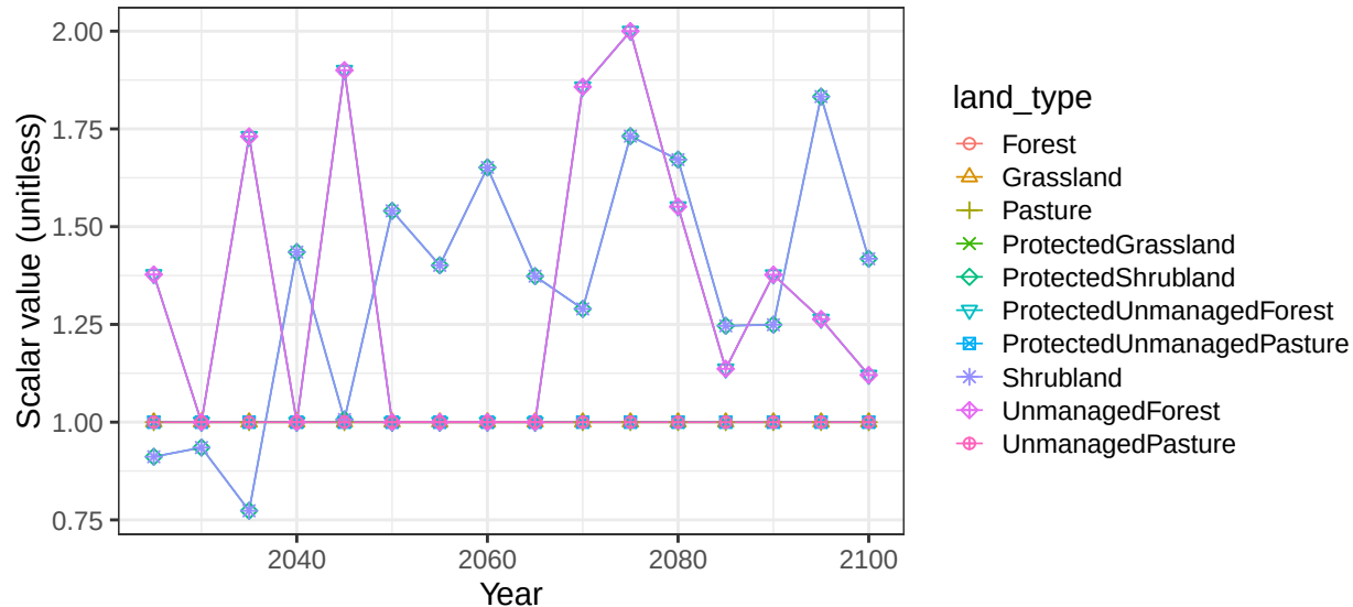
Region EU-12 basin MeditE non-crop vegetation scalars
