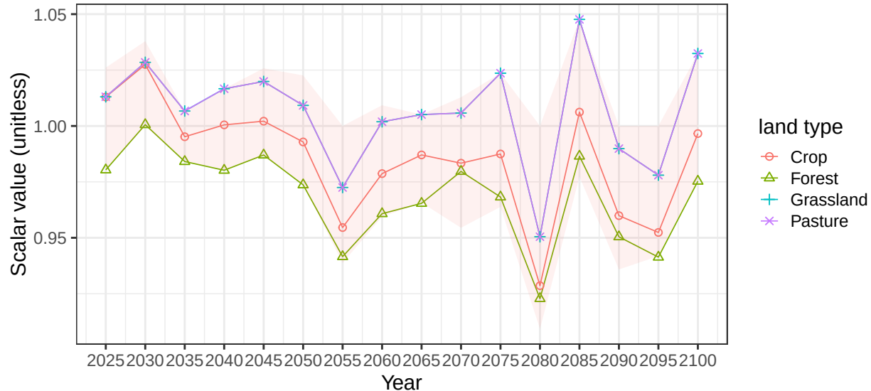
Region USA basin UsaCstE average soil scalars
