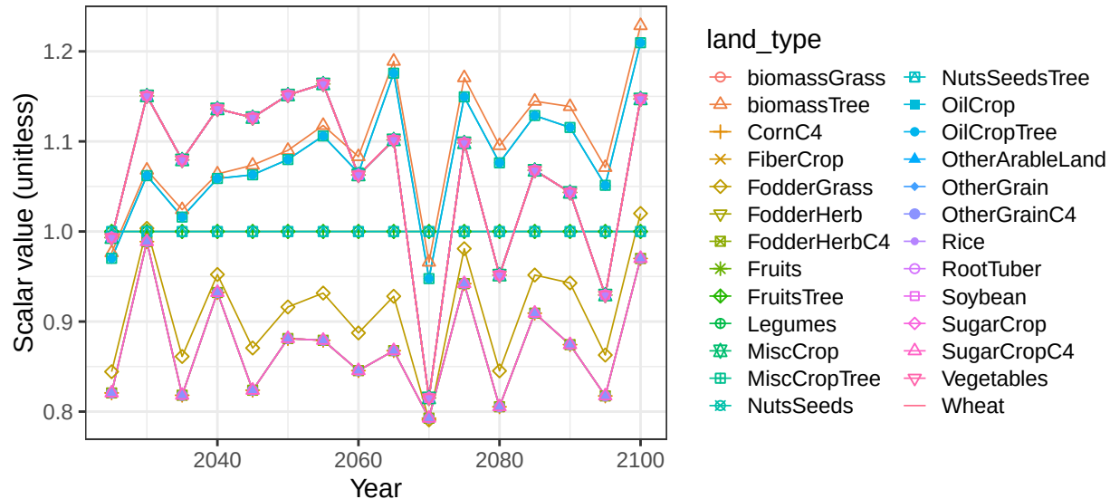
Region Mexico basin MexCstW crop vegetation scalars
