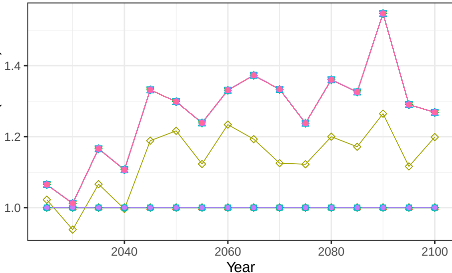
Region Russia basin Gobi crop vegetation scalars
