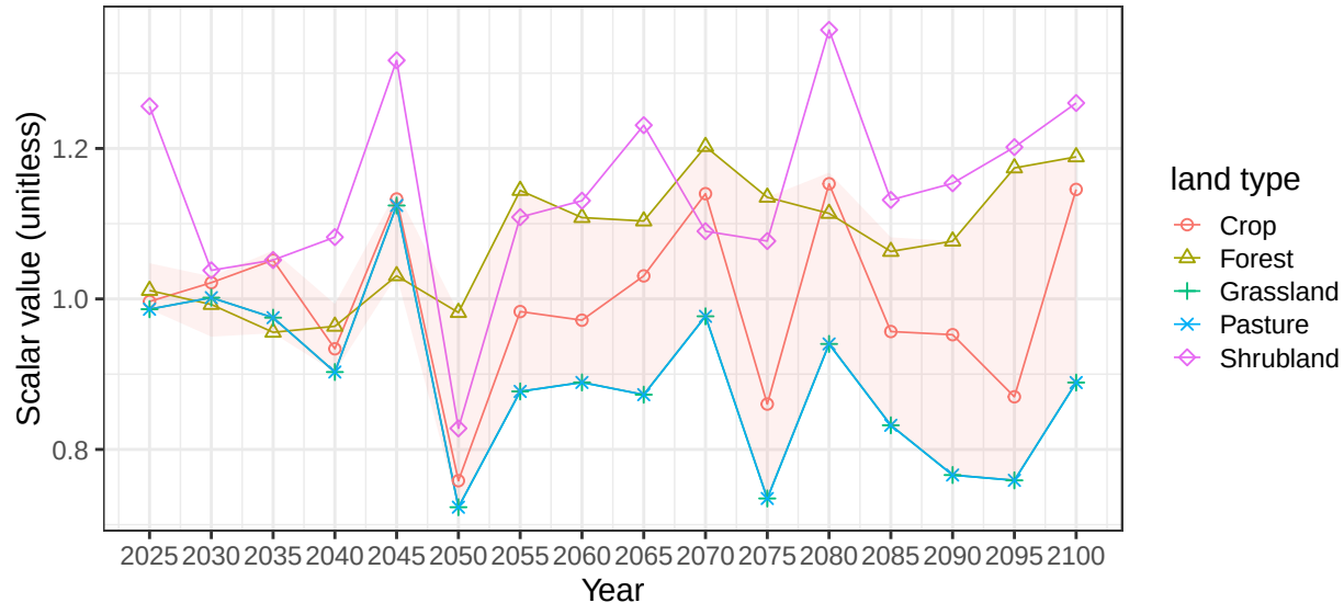
Region Russia basin DonR average soil scalars
