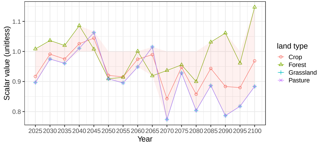
Region EU-15 basin OderR average soil scalars
