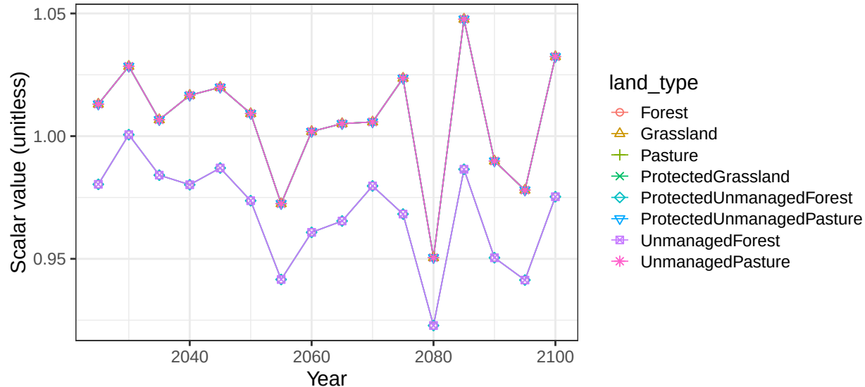
Region USA basin UsaCstE non-crop soil scalars
