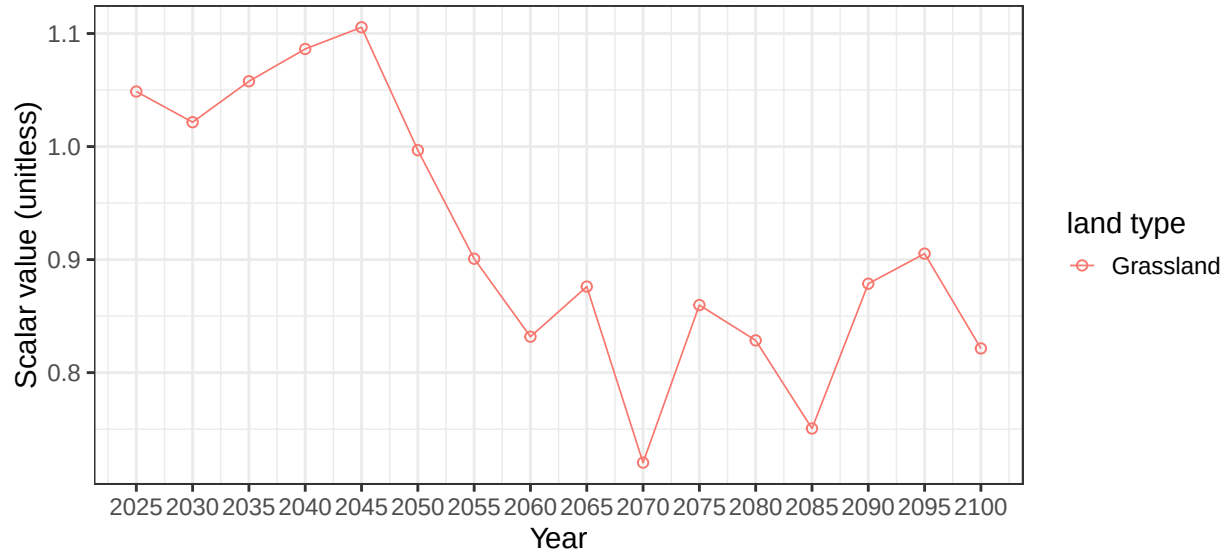
Region Africa_Northern basin AfrCstNE average soil scalars
