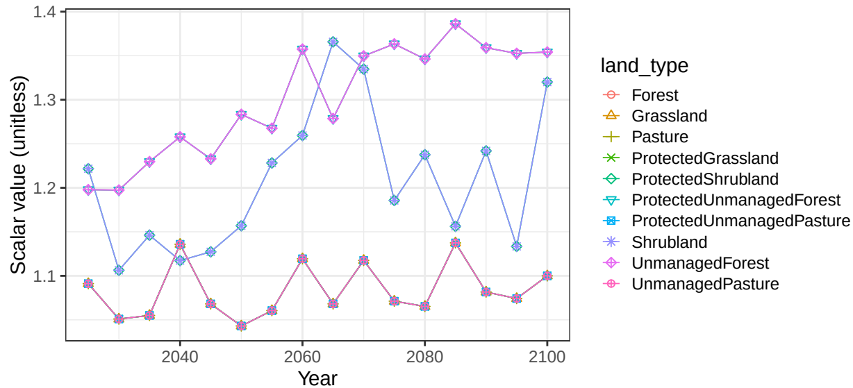
Region Brazil basin BrzCstE non-crop soil scalars
