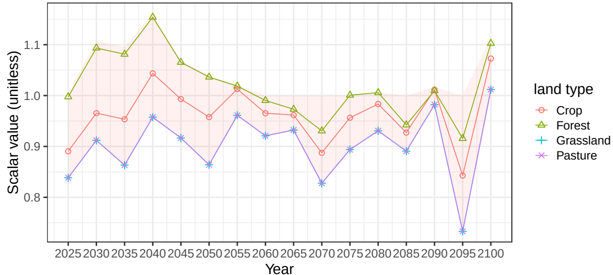
Region EU-12 basin WislaR average soil scalars
