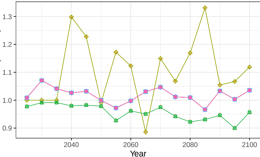
Region Canada basin GreatLakes crop soil scalars
