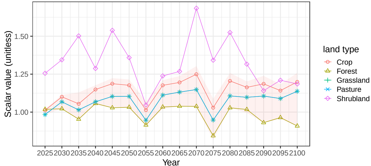
Region Southeast Asia basin Salween average vegetation scalars
