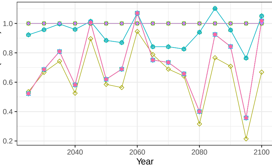
Region EU-12 basin NemanR crop vegetation scalars
