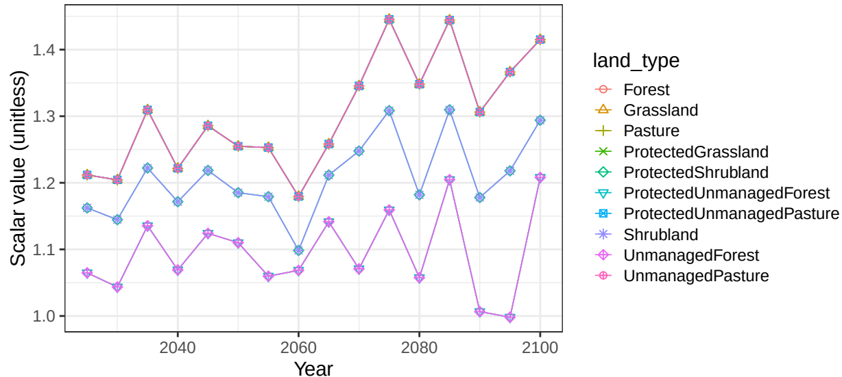
Region Canada basin PacArctic non-crop vegetation scalars
