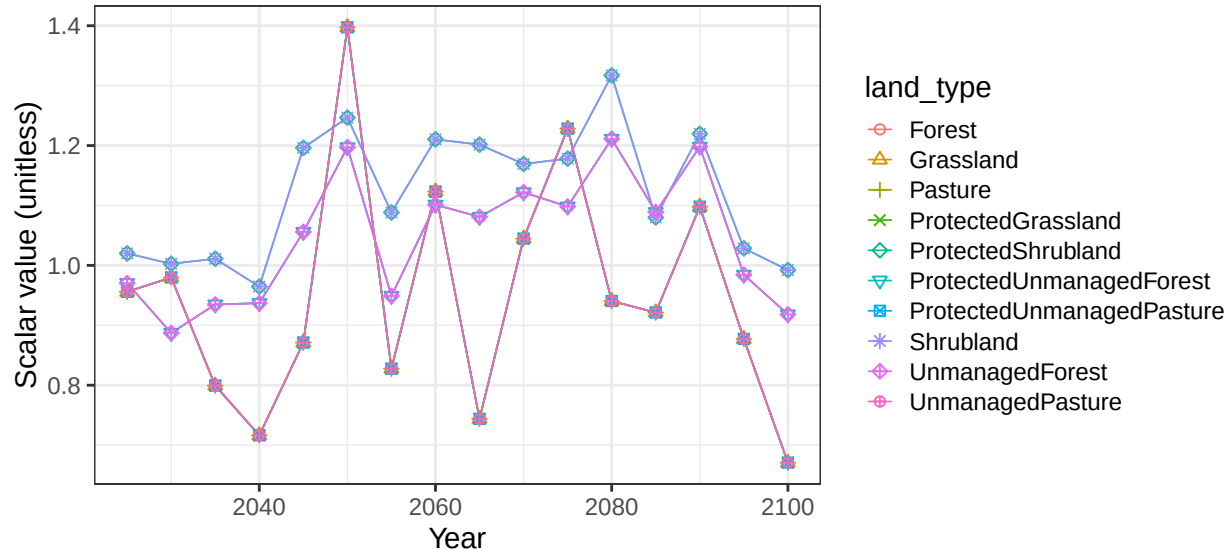
Region Central Asia basin ObR non-crop vegetation scalars
