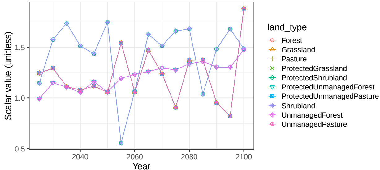
Region Central Asia basin VolgaR non-crop vegetation scalars
