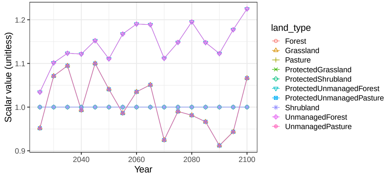
Region Mexico basin Tehuantpc non-crop vegetation scalars
