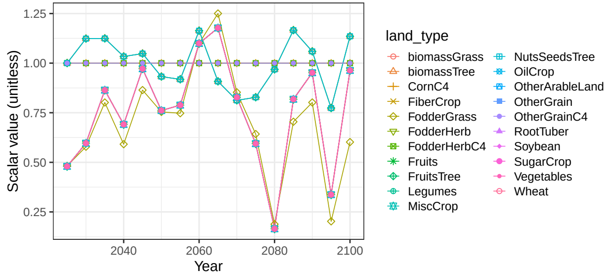
Region Russia basin NemanR crop vegetation scalars
