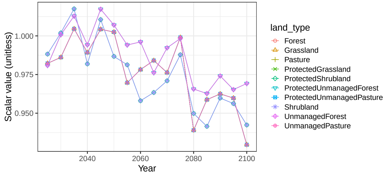
Region Russia basin AmurR non-crop soil scalars
