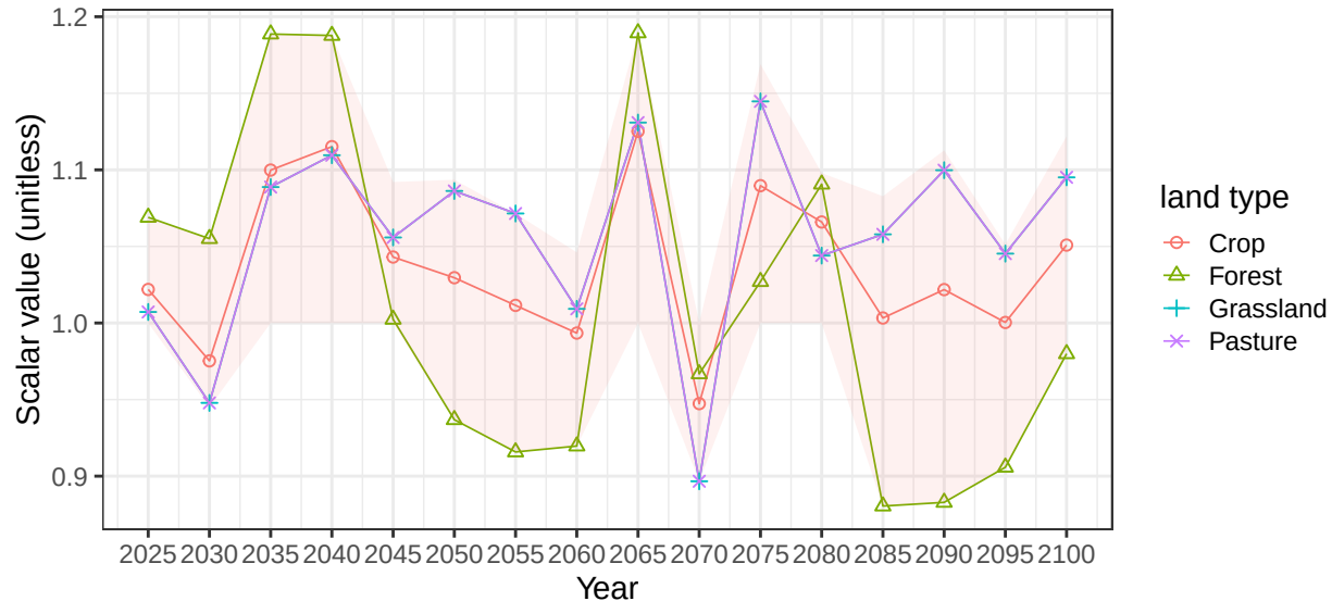
Region EU-15 basin ScheldtR average soil scalars
