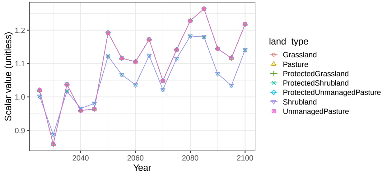
Region Central Asia basin Tarim non-crop vegetation scalars
