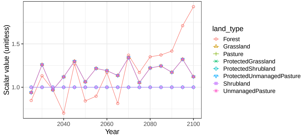
Region India basin IndCstE non-crop vegetation scalars
