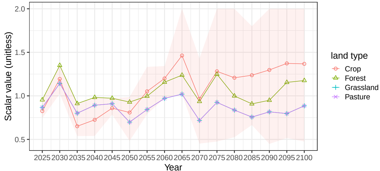
Region Central Asia basin BlackSeaS average vegetation scalars
