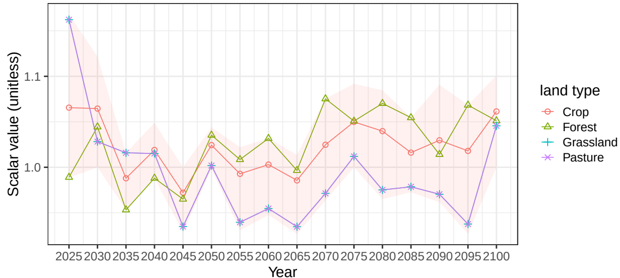
Region Southeast Asia basin Phlppns average vegetation scalars
