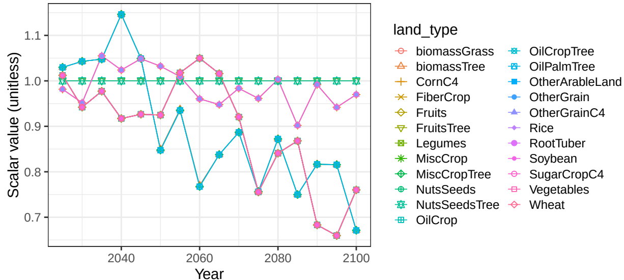
Region Africa_Western basin LChad crop soil scalars
