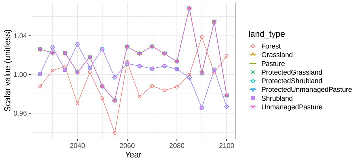
Region China basin IrrawaddyR non-crop soil scalars
