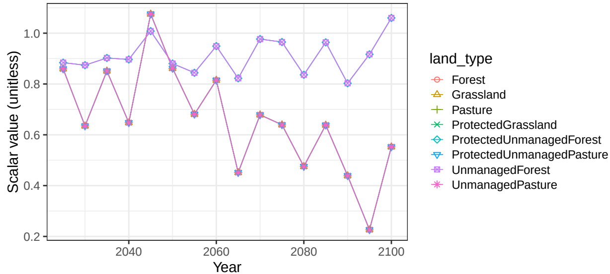
Region Russia basin NarvaR non-crop vegetation scalars
