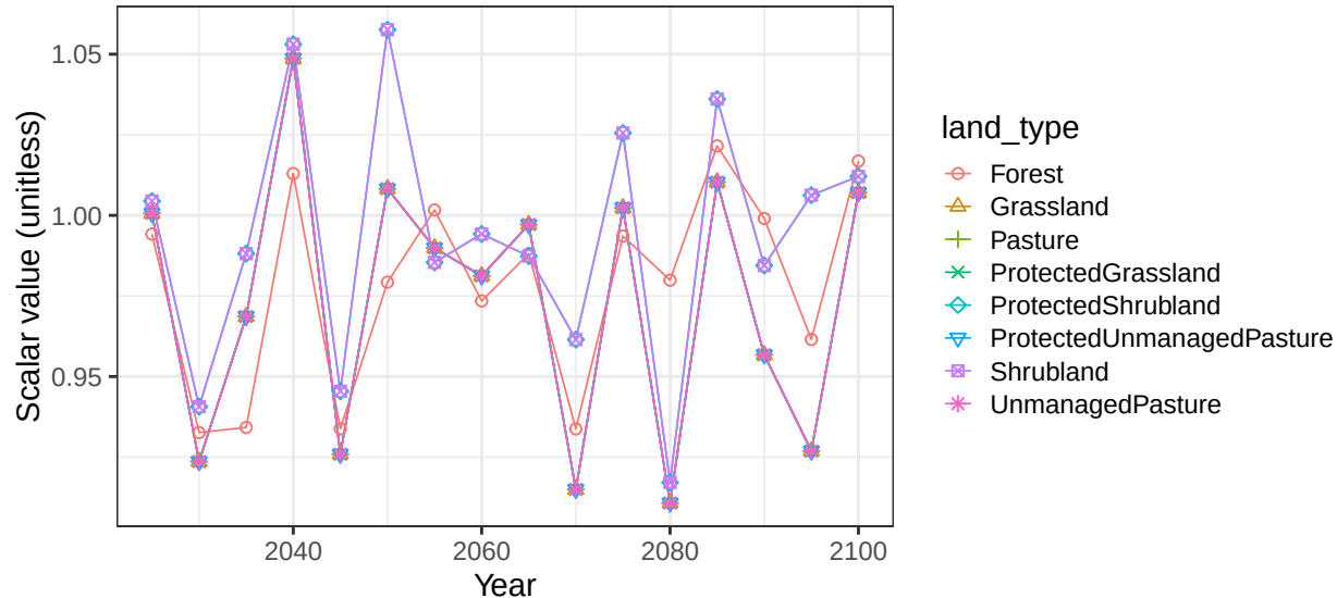
Region China basin HuangHeR non-crop soil scalars
