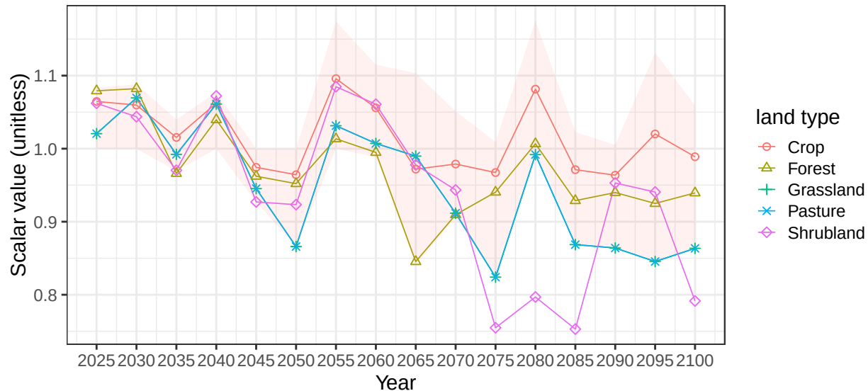
Region Europe_Non_EU basin AdrBlkSea average soil scalars
