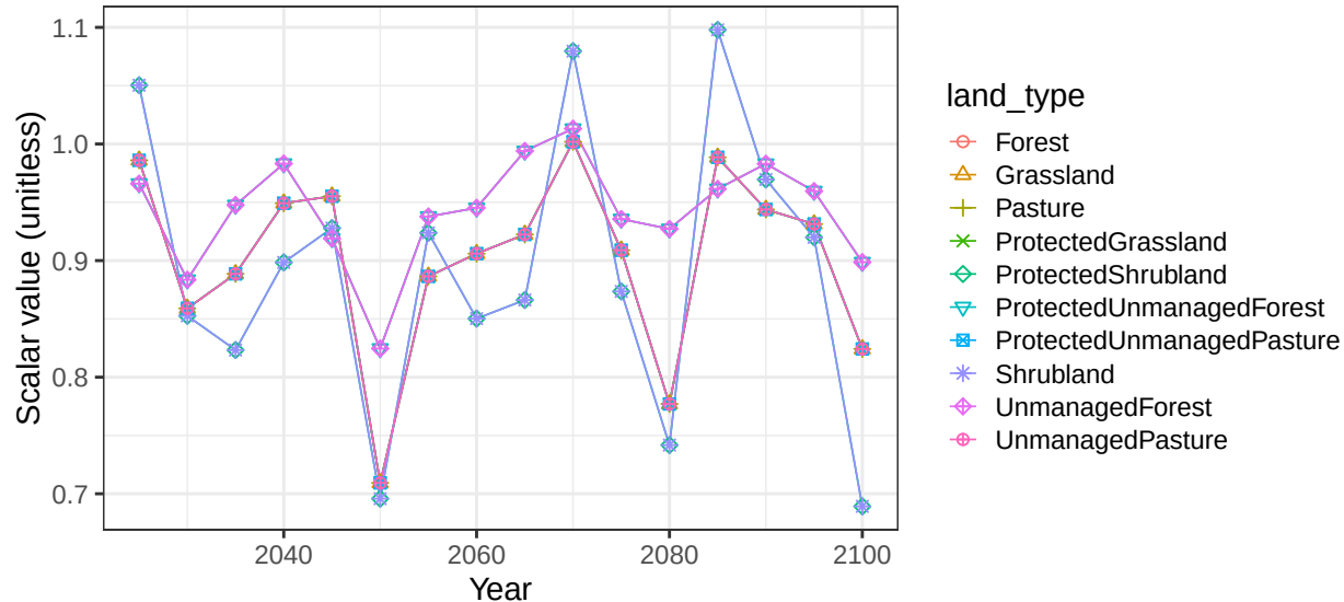
Region Australia_NZ basin MurrayDrlg non-crop soil scalars
