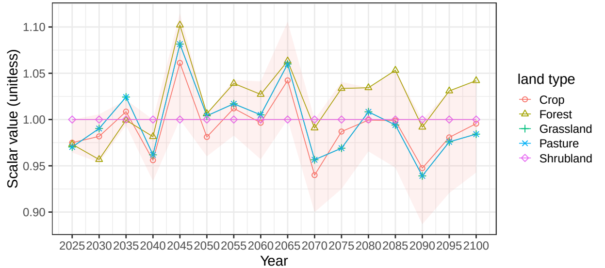
Region Central America and Caribbean basin GrijUsuR average vegetation
