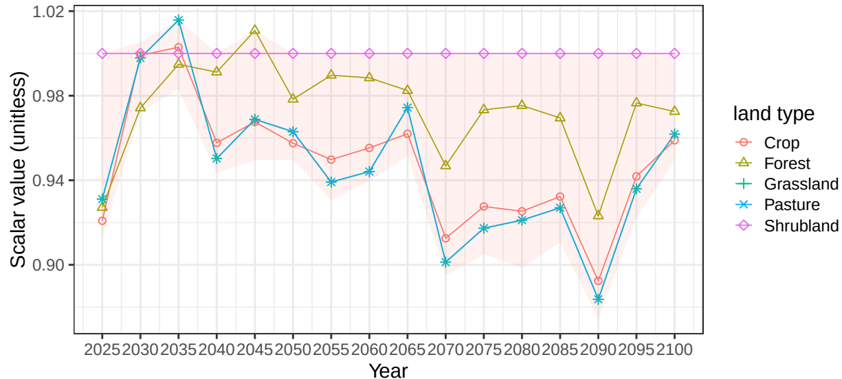
Region Mexico basin GrijUsuR average soil scalars
