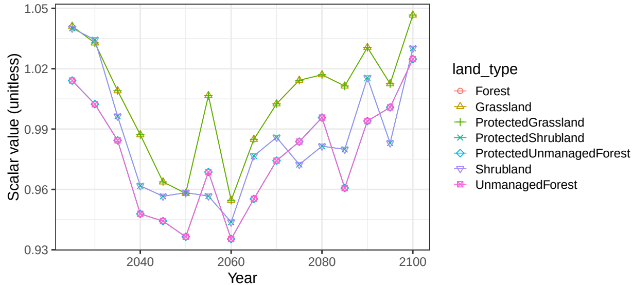
Region Japan basin Japan non-crop vegetation scalars
