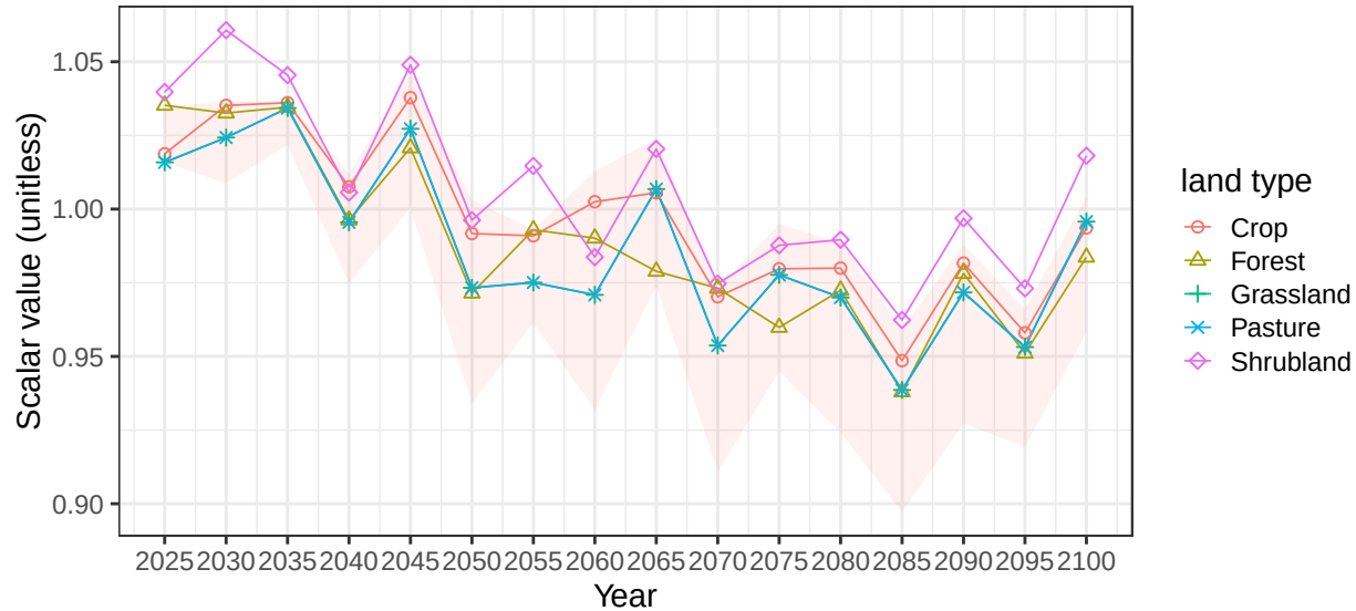
Region South Korea basin Korea average soil scalars
