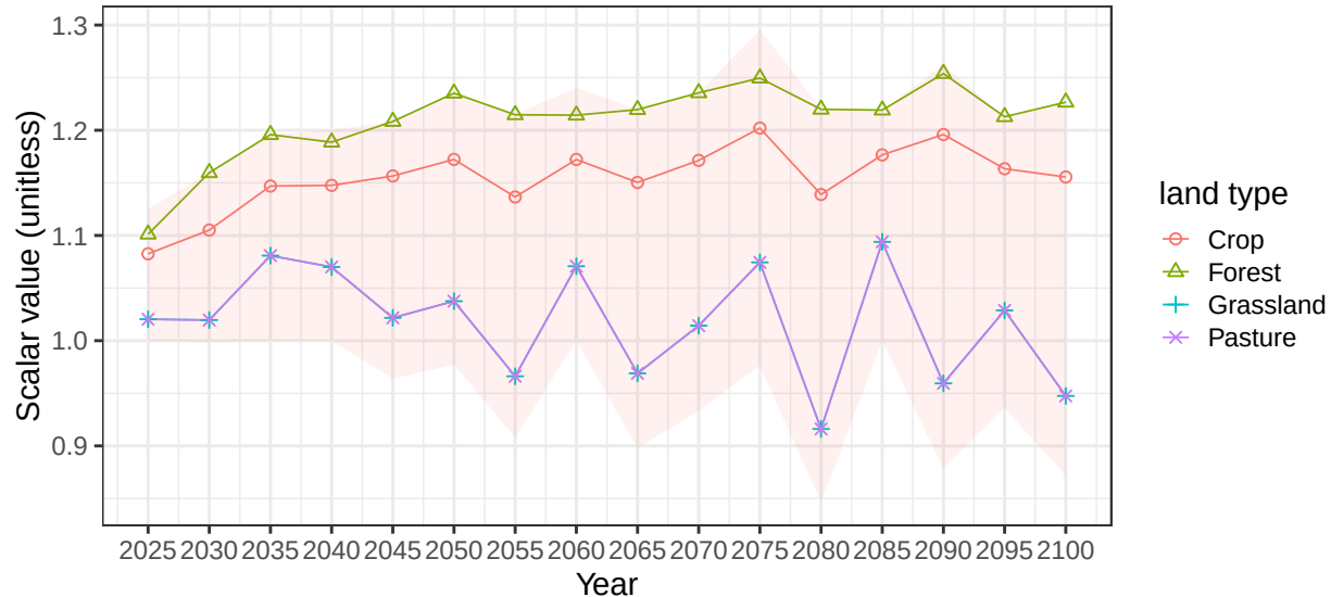
Region Indonesia basin IdnE average vegetation scalars
