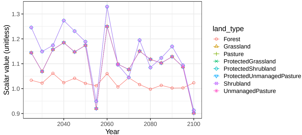
Region China basin BoHai non-crop soil scalars
