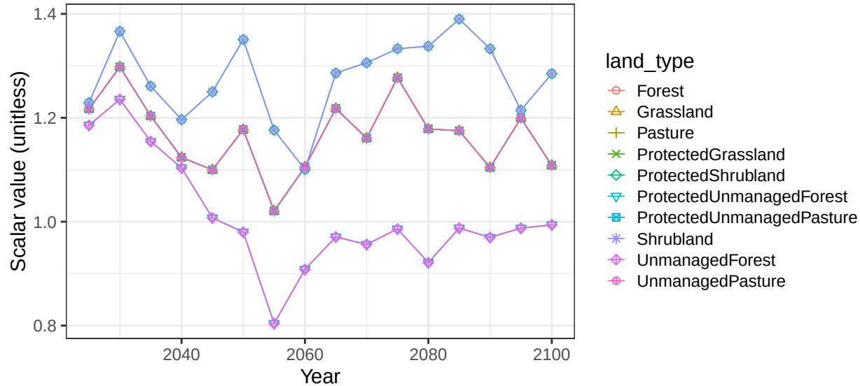
Region USA basin GreatBasin non-crop vegetation scalars
