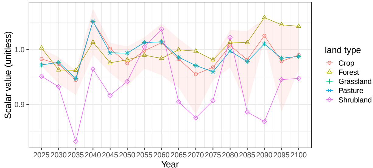
Region South Africa basin AfrCstS average soil scalars
