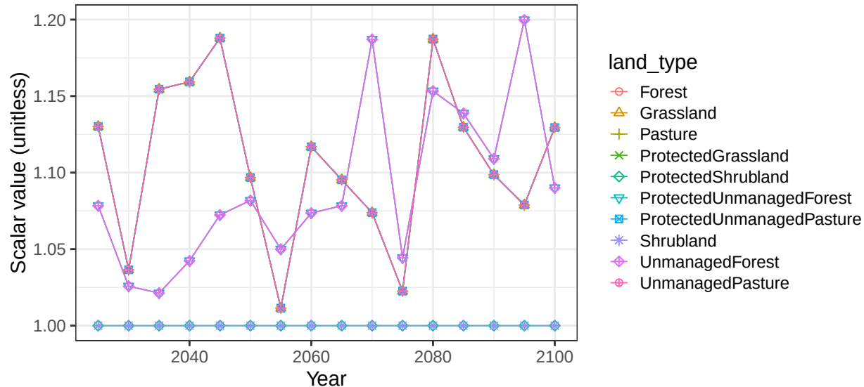
Region Southeast Asia basin ThaiGulf non-crop vegetation scalars
