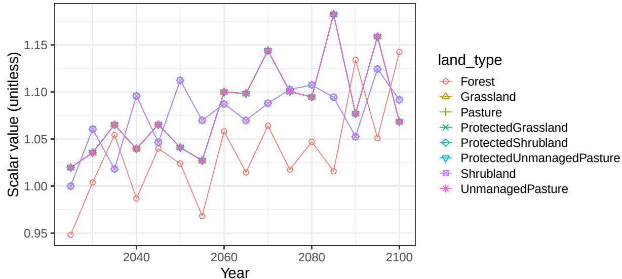
Region China basin IrrawaddyR non-crop vegetation scalars
