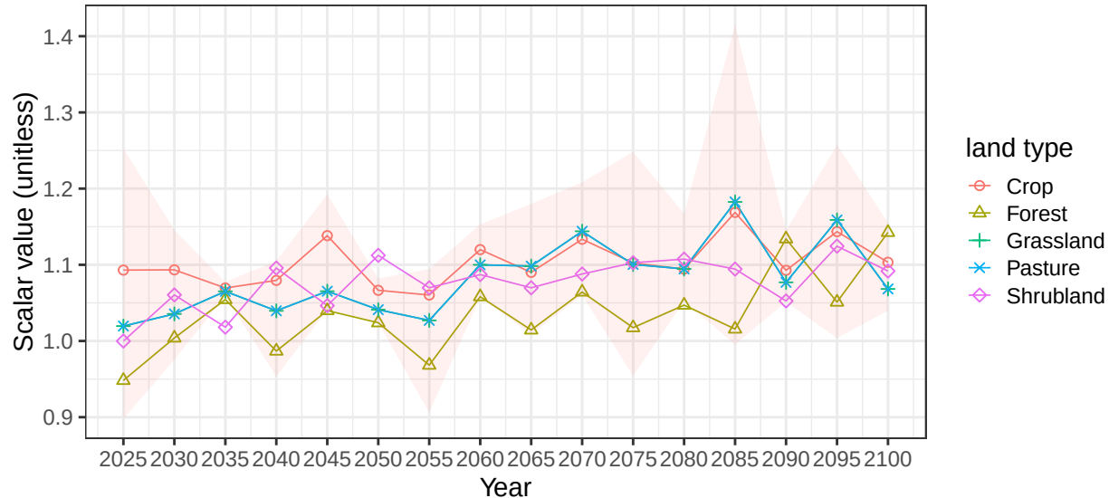
Region China basin IrrawaddyR average vegetation scalars
