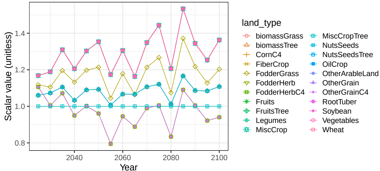
Region USA basin OhioR crop vegetation scalars
