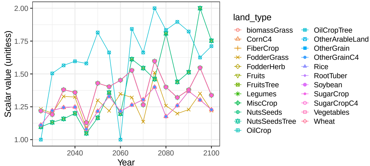
Region Middle East basin Iran crop vegetation scalars
