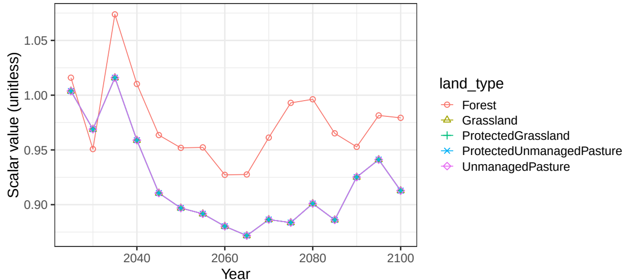
Region EU-15 basin Ireland non-crop vegetation scalars
