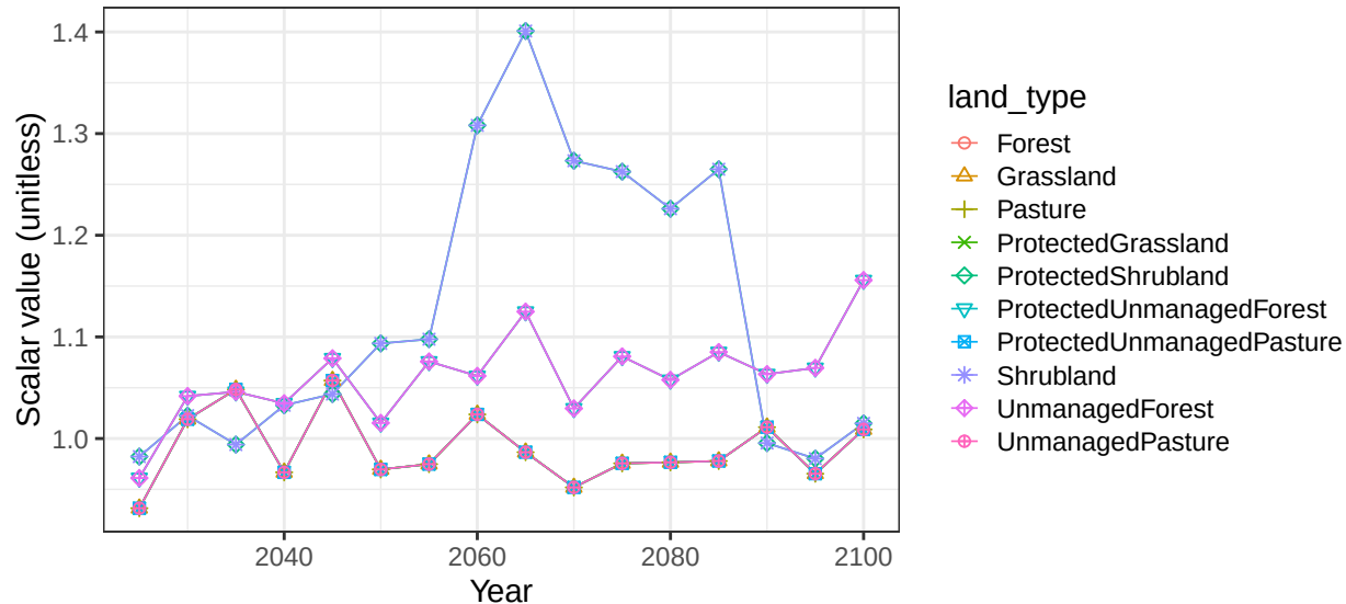
Region Mexico basin Papaloapan non-crop vegetation scalars
