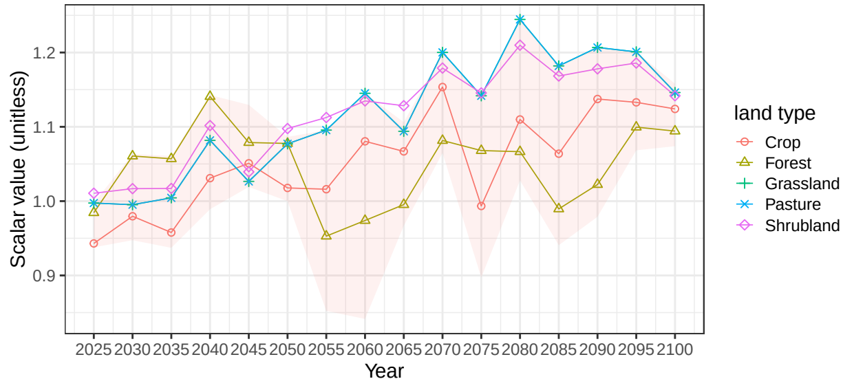
Region China basin GangesR average vegetation scalars
