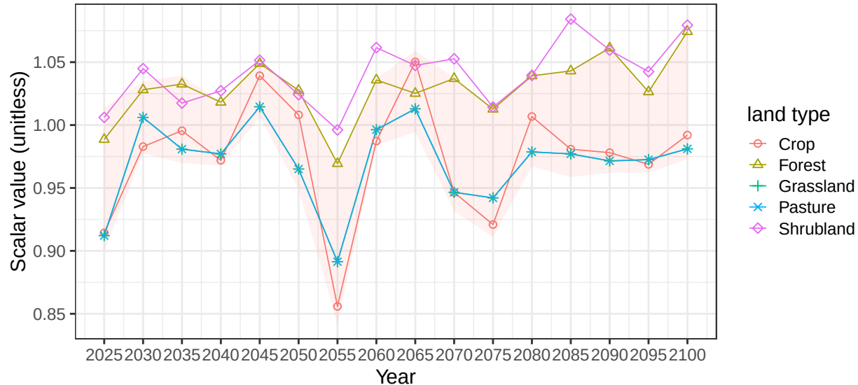
Region Southeast Asia basin IrrawaddyR average soil scalars
