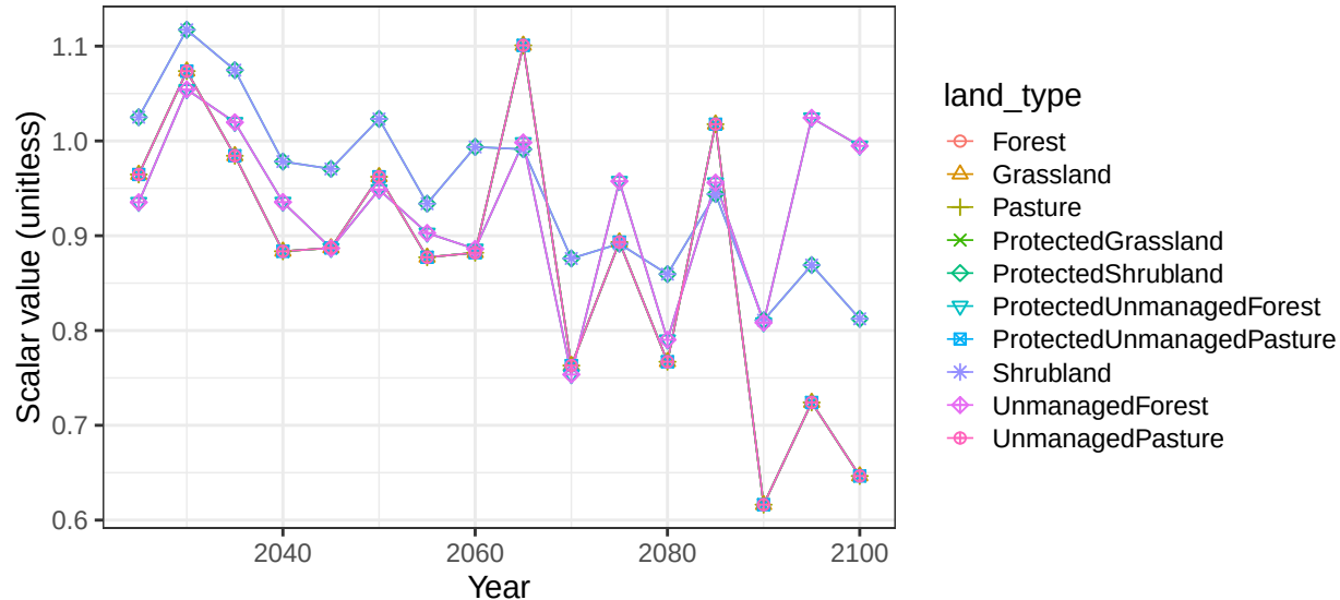
Region Argentina basin MarChiq non-crop soil scalars
