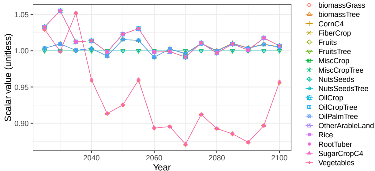
Region Southeast Asia basin BorneoCstN crop soil scalarsland_type
