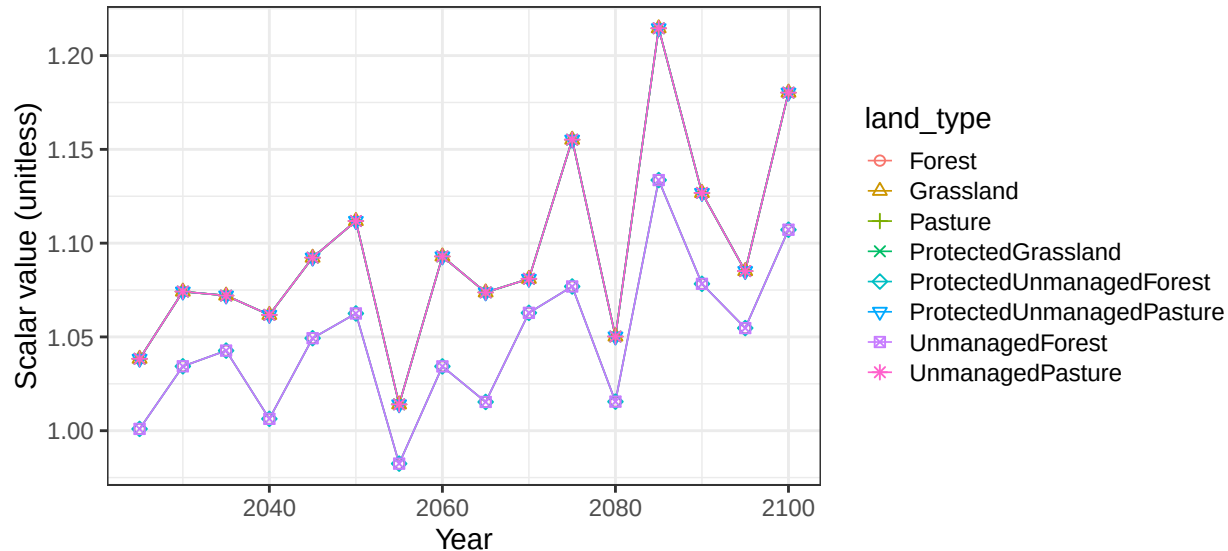
Region USA basin UsaCstE non-crop vegetation scalars
