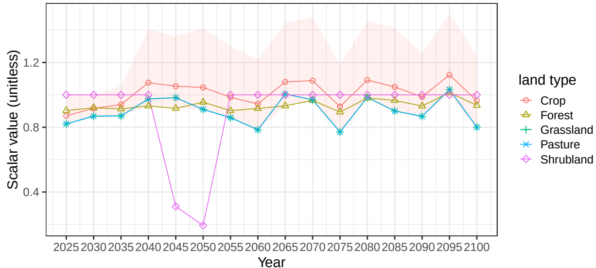
Region South America_Northern basin OrinocoR average vegetation scalar
