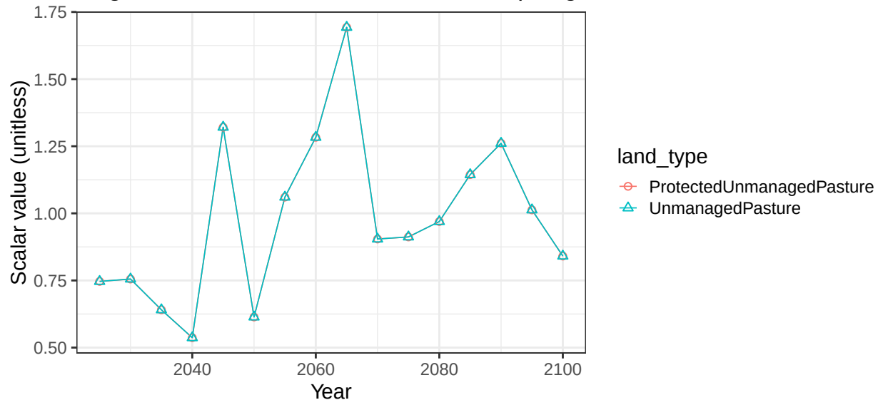
Region EU-15 basin AfrCstNW non-crop vegetation scalars
