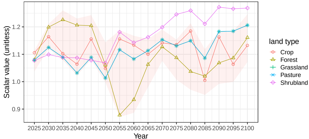
Region India basin GangesR average soil scalars
