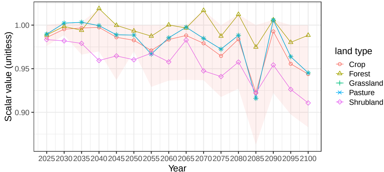
Region Australia_NZ basin Tasmania average soil scalars
