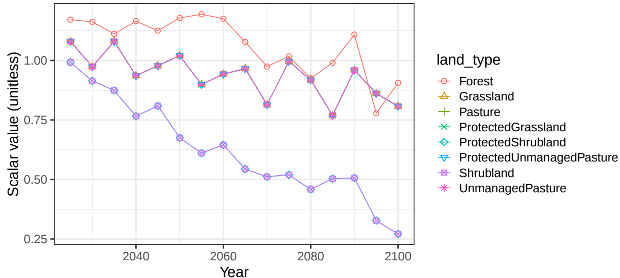
Region Africa_Eastern basin ShebJubR non-crop soil scalars
