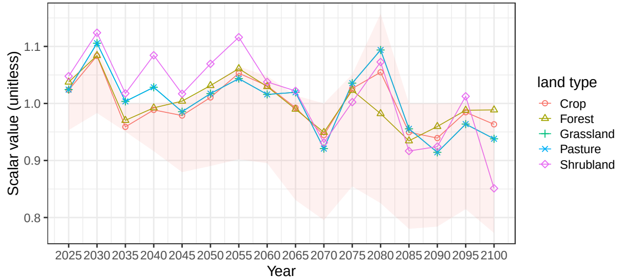
Region Europe_Non_EU basin MeditE average soil scalars
