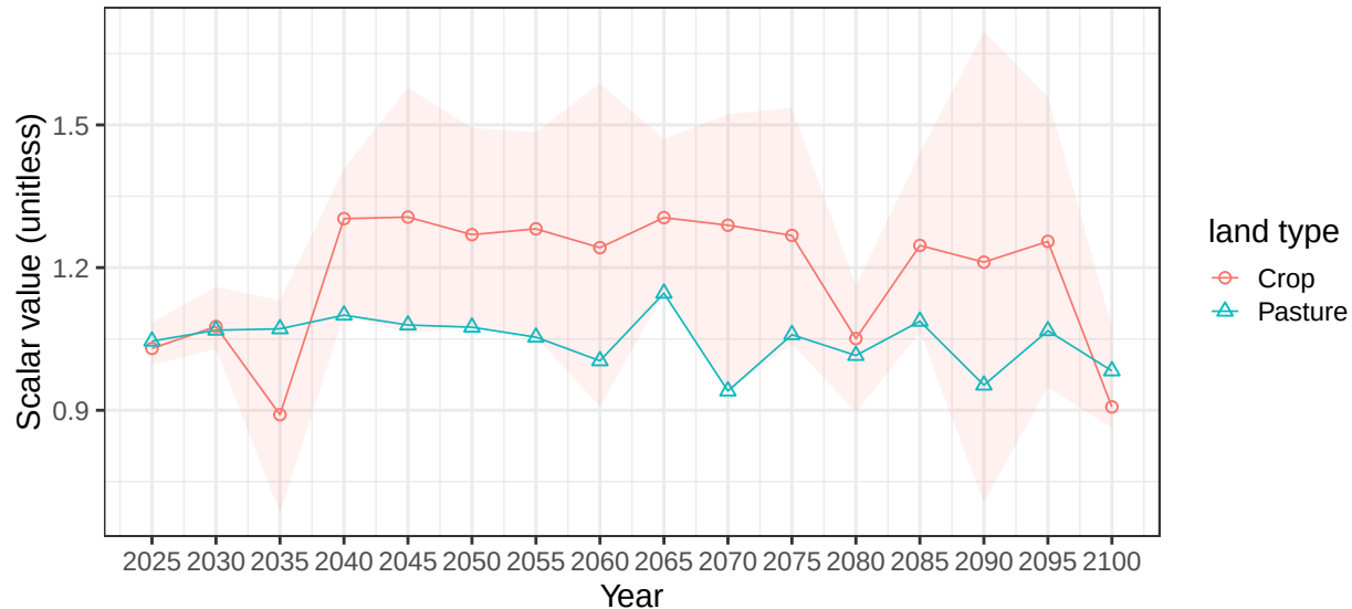
Region South America_Southern basin ArgColoR average soil scalars
