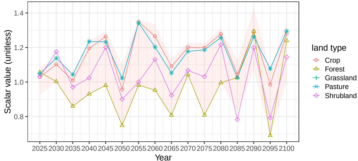
Region India basin MahiR average soil scalars
