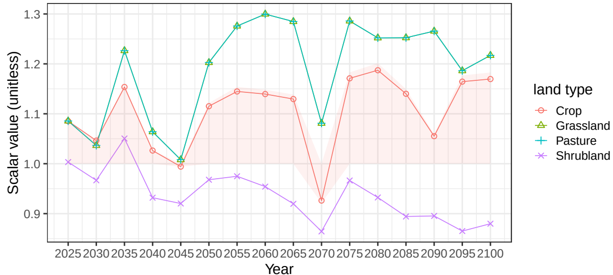
Region South Asia basin FarahrudR average soil scalars
