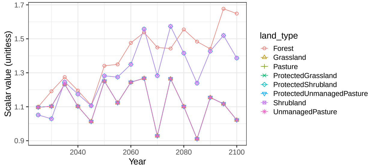
Region Middle East basin CaspianSW non-crop vegetation scalars
