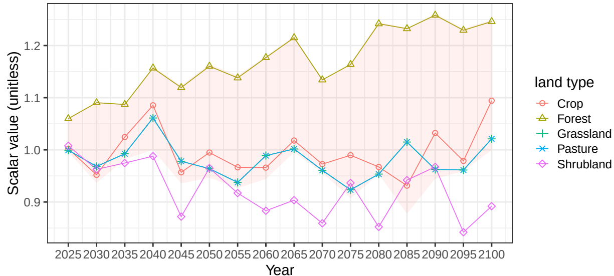
Region Africa_Southern basin AfrCstE average soil scalars
