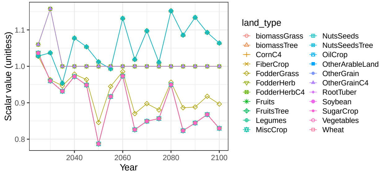
Region EU-15 basin DanubeR crop vegetation scalars
