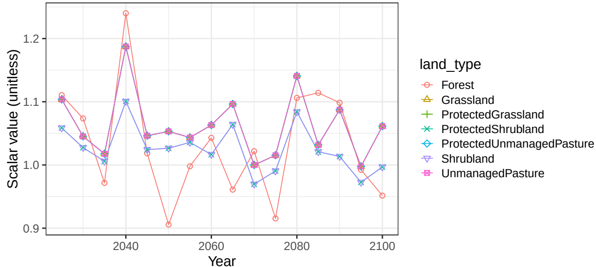
Region EU-15 basin FranceCstS non-crop soil scalars
