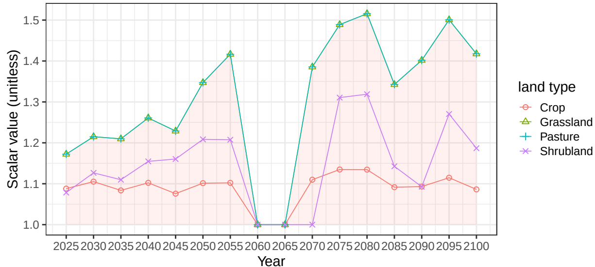
Region Middle East basin HamuMashR average vegetation scalars
