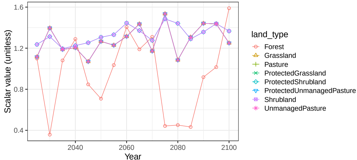
Region Middle East basin TigrEuphR non-crop vegetation scalars
