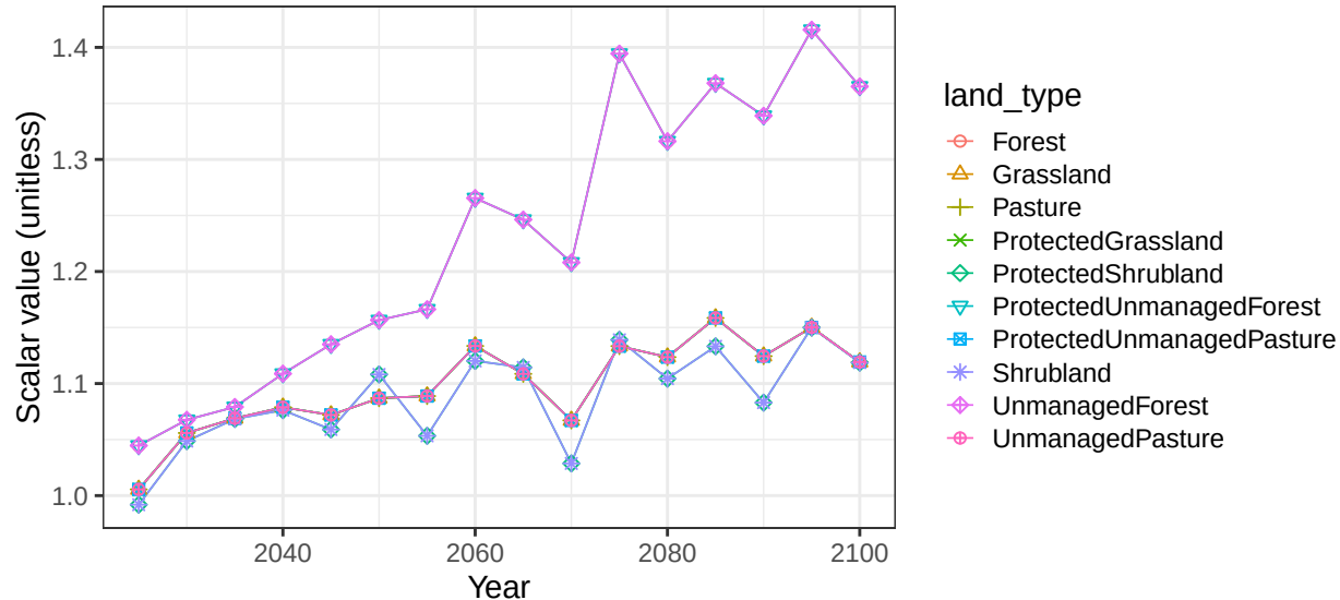
Region Argentina basin ArgCstS non-crop vegetation scalars
