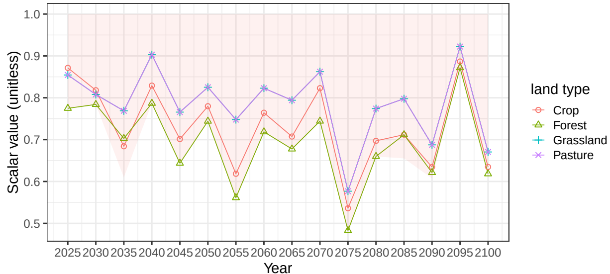
Region South America_Northern basin SAmersCstNE average vegetation so
