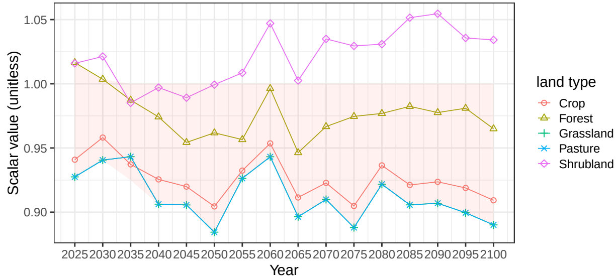
Region Brazil basin SAmerCstNE average soil scalars
