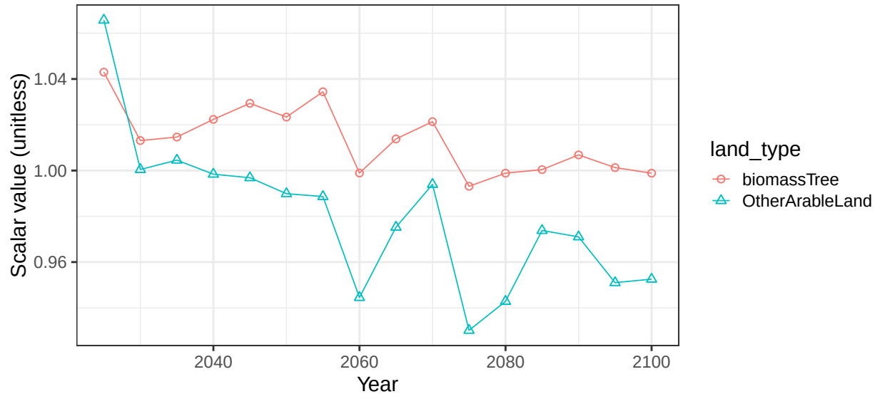
Region India basin AdnNiclsl crop soil scalars
