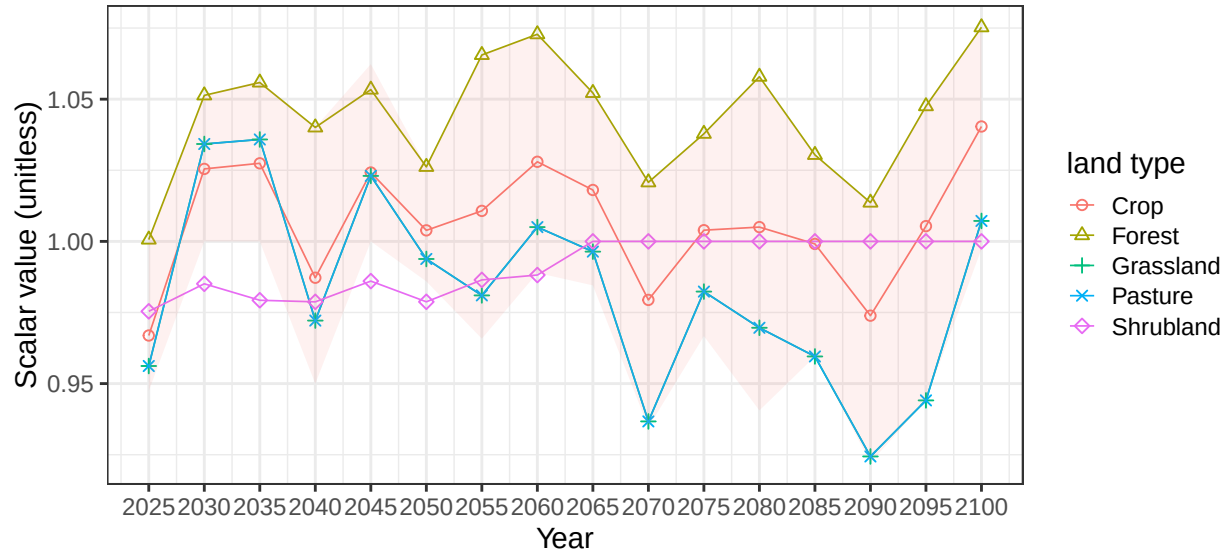
Region Mexico basin Tehuantepec average soil scalars
