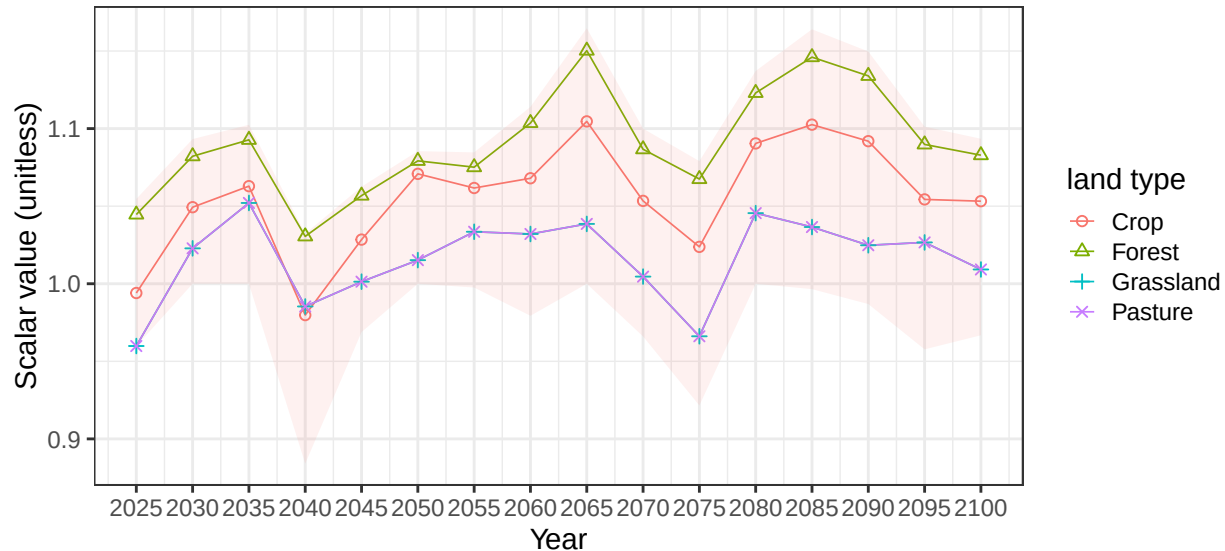
Region Australia_NZ basin NewZealand average vegetation scalars
