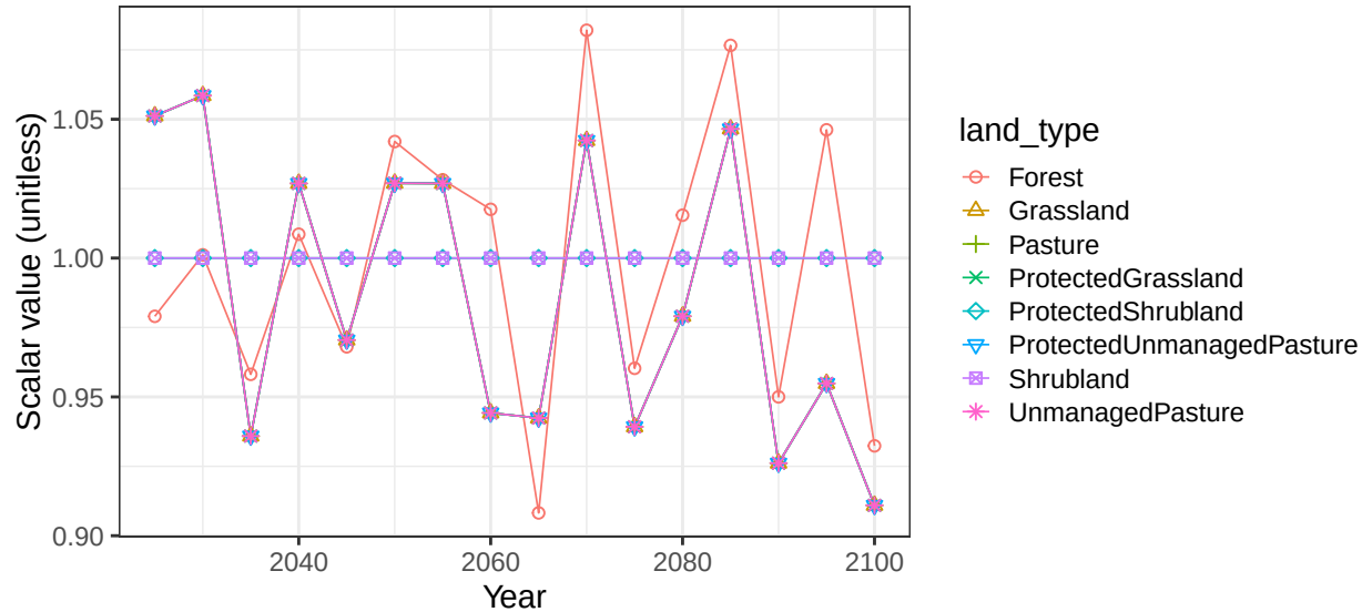
Region China basin Hainan non-crop soil scalars
