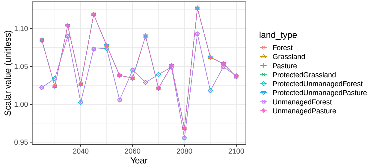
Region USA basin TennR non-crop vegetation scalars
