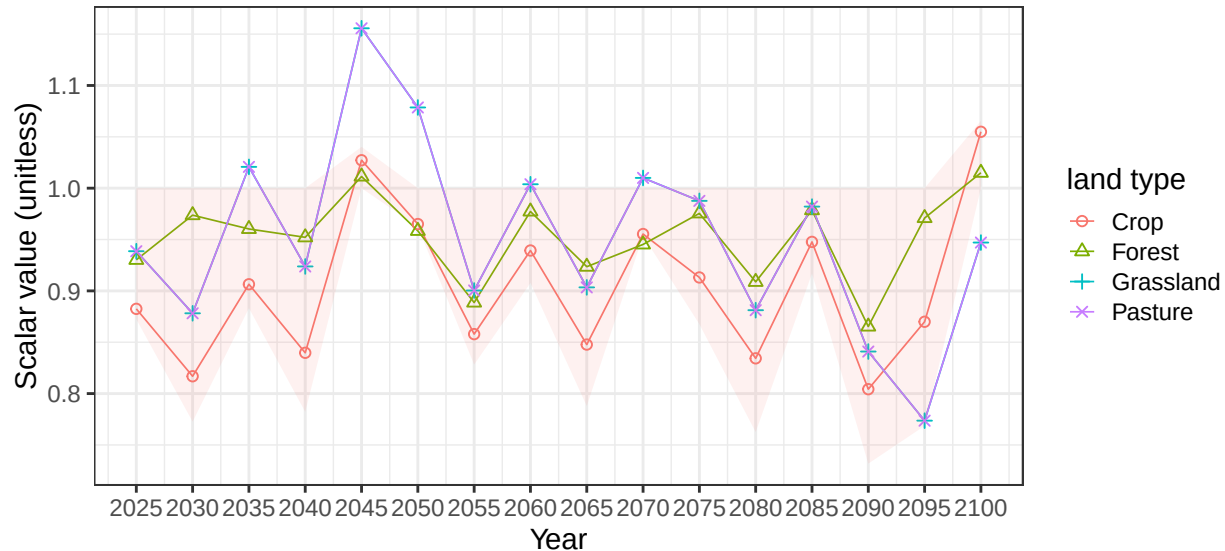
Region EU-12 basin NarvaR average soil scalars
