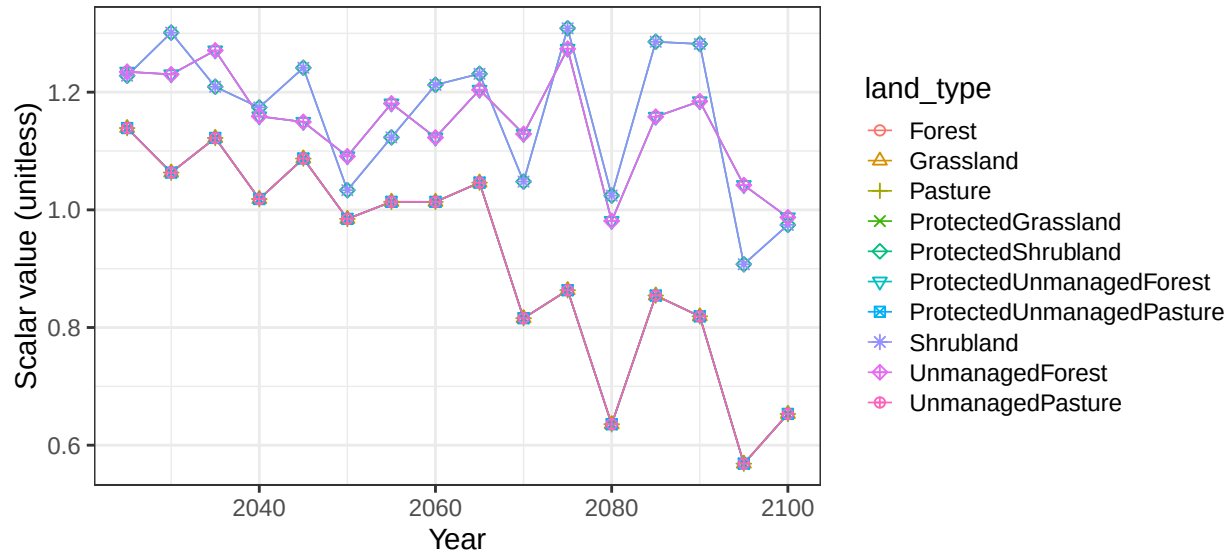
Region USA basin ArkWhtRedR non-crop vegetation scalars
