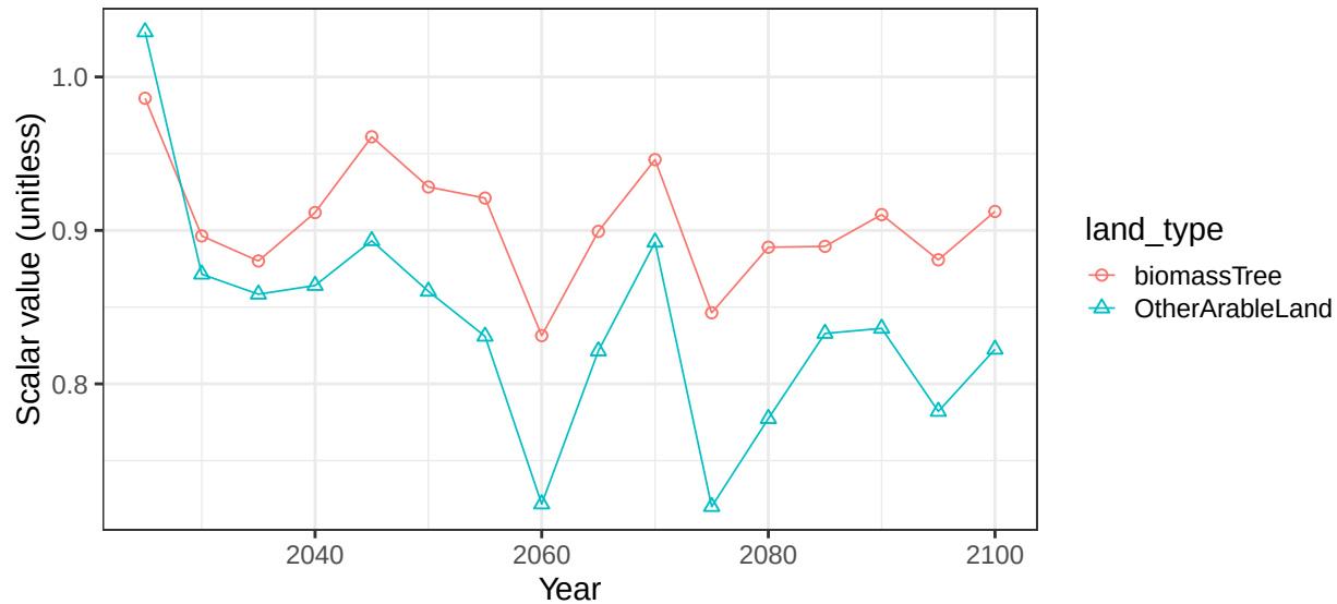
Region India basin AdnNicIsl crop vegetation scalars
