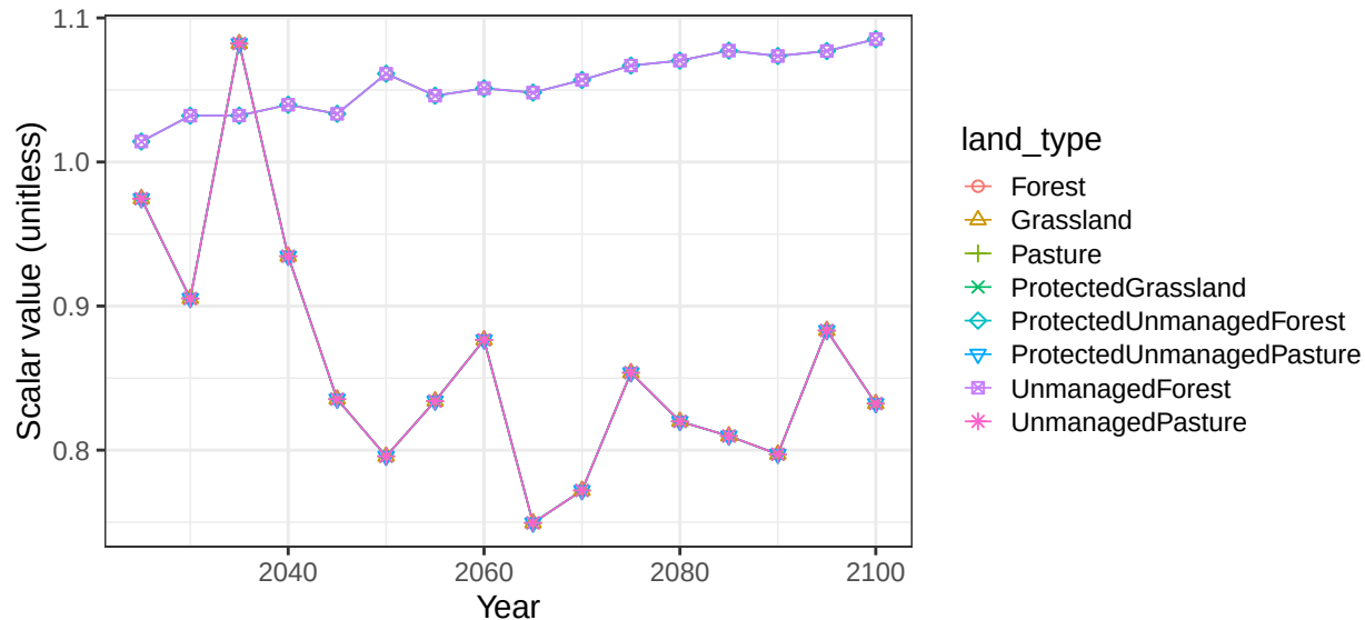
Region Indonesia basin Kalimantan non-crop vegetation scalars
