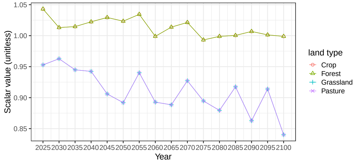
Region India basin AdnNiclsl average soil scalars
