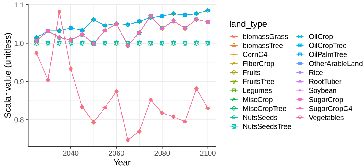
Region Indonesia basin Kalimantan crop vegetation scalars
