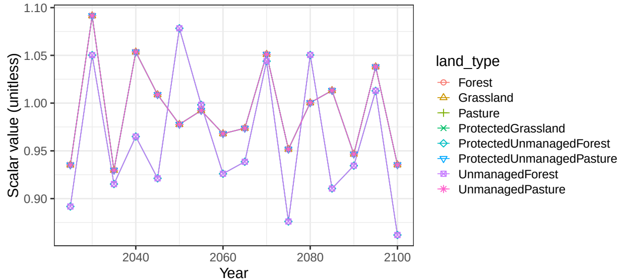
Region USA basin Caribbean non-crop soil scalars
