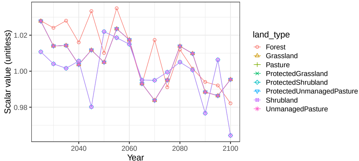
Region China basin Yangtze non-crop soil scalars
