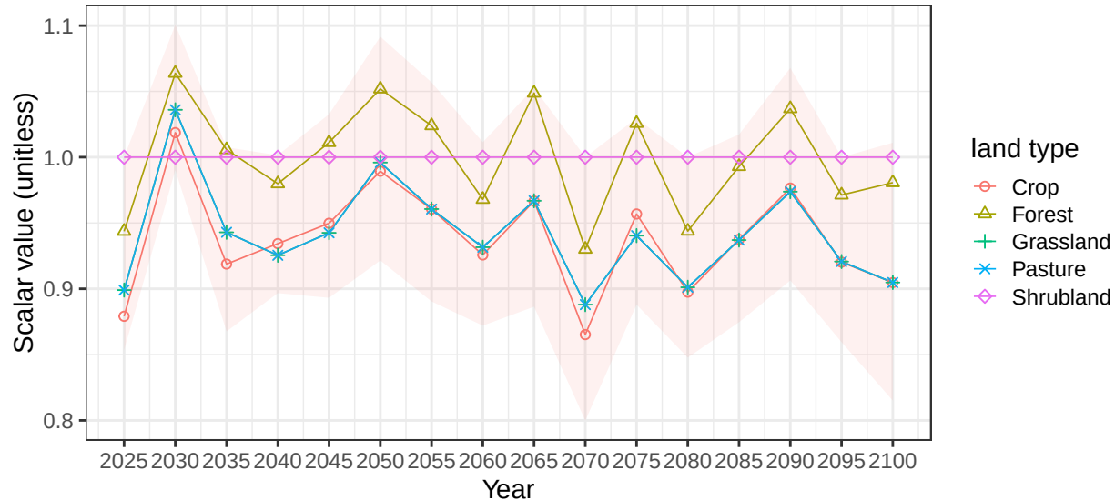
Region Mexico basin RioLerma average soil scalars
