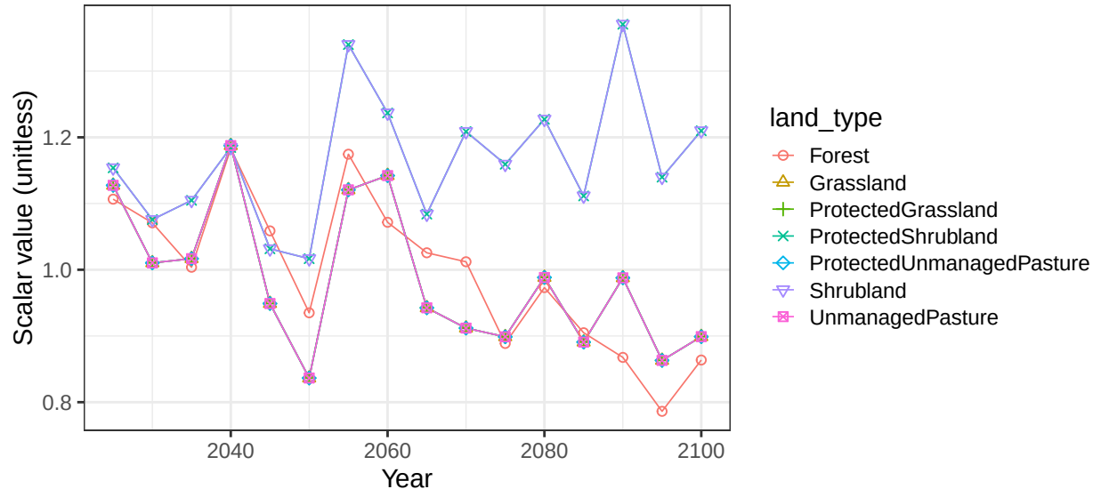
Region EU-15 basin ItalyCstW non-crop vegetation scalars
