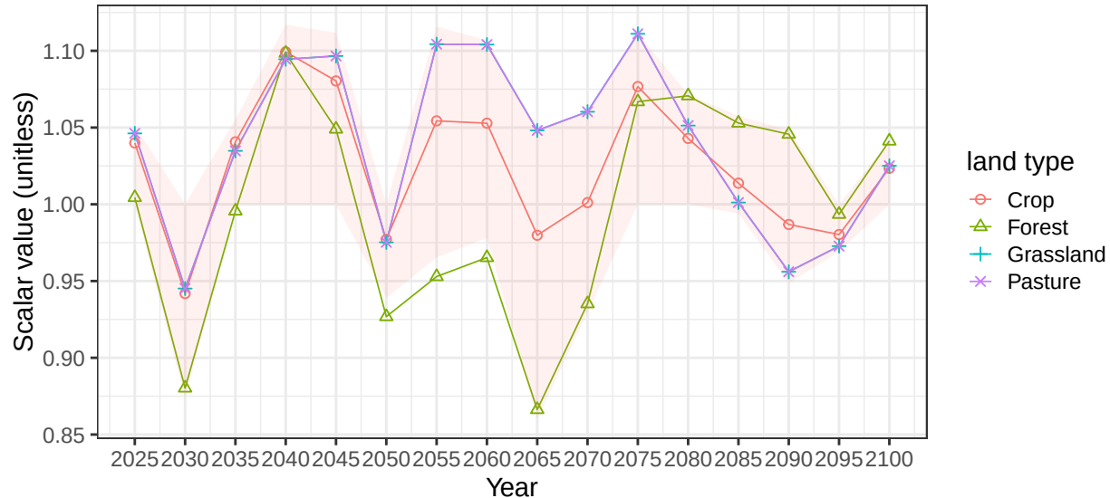
Region EU-12 basin ElbeR average soil scalars
