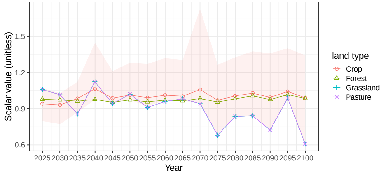
Region South America_Northern basin AmazonR average vegetation scalar
