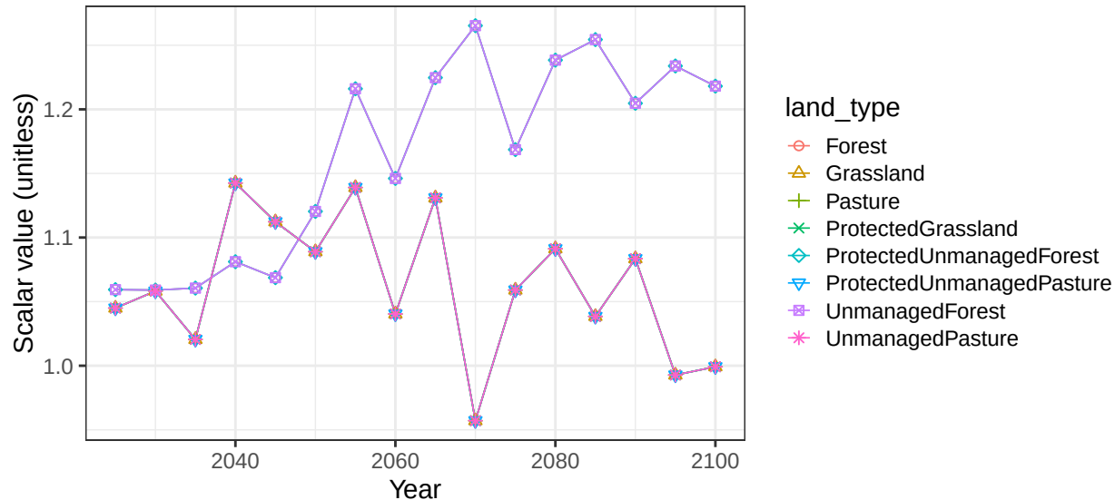
Region Africa_Southern basin AfrCstS non-crop soil scalars
