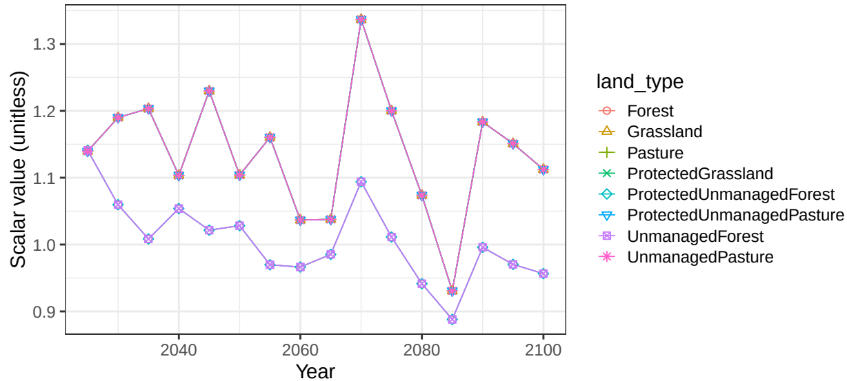
Region USA basin NelsonR non-crop soil scalars
