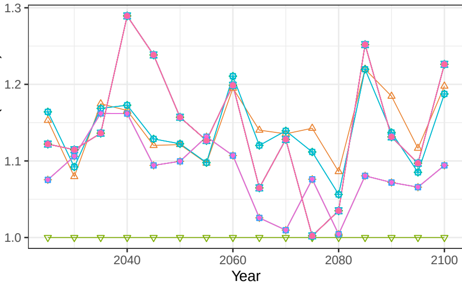
Region Africa_Western basin ZambeziR crop vegetation scalars
