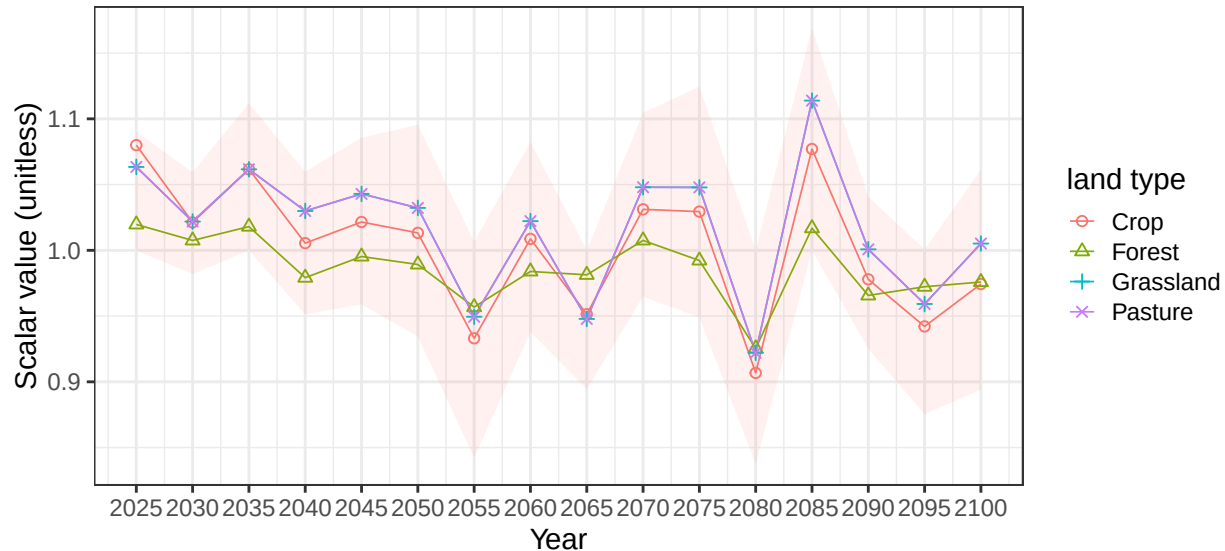
Region USA basin OhioR average soil scalars
