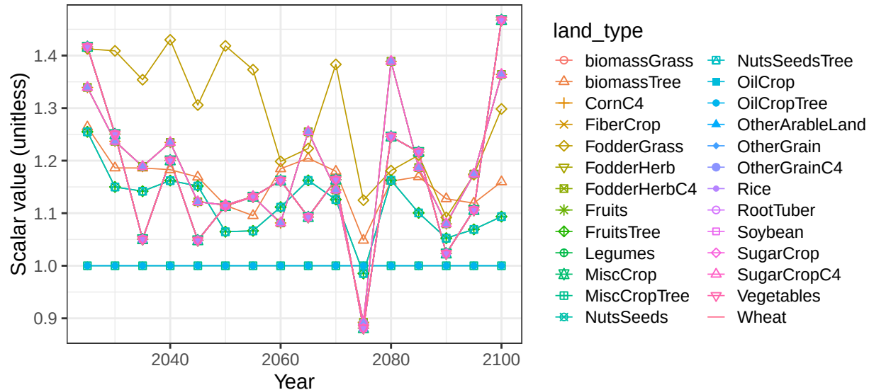
Region EU-15 basin TagusR crop vegetation scalars
