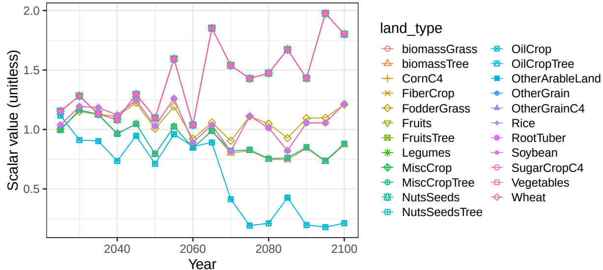
Region India basin IndusR crop vegetation scalars
