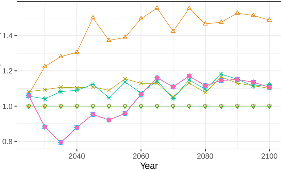
Region South America_Southern basin ArgCstS crop vegetation scalars
