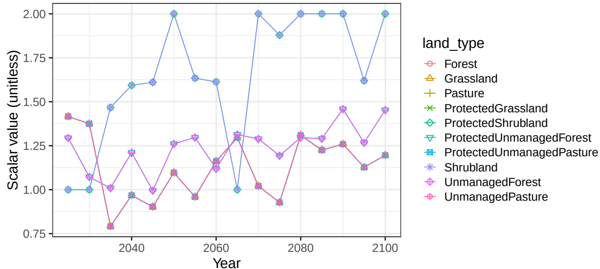
Region USA basin MexCstNW non-crop vegetation scalars
