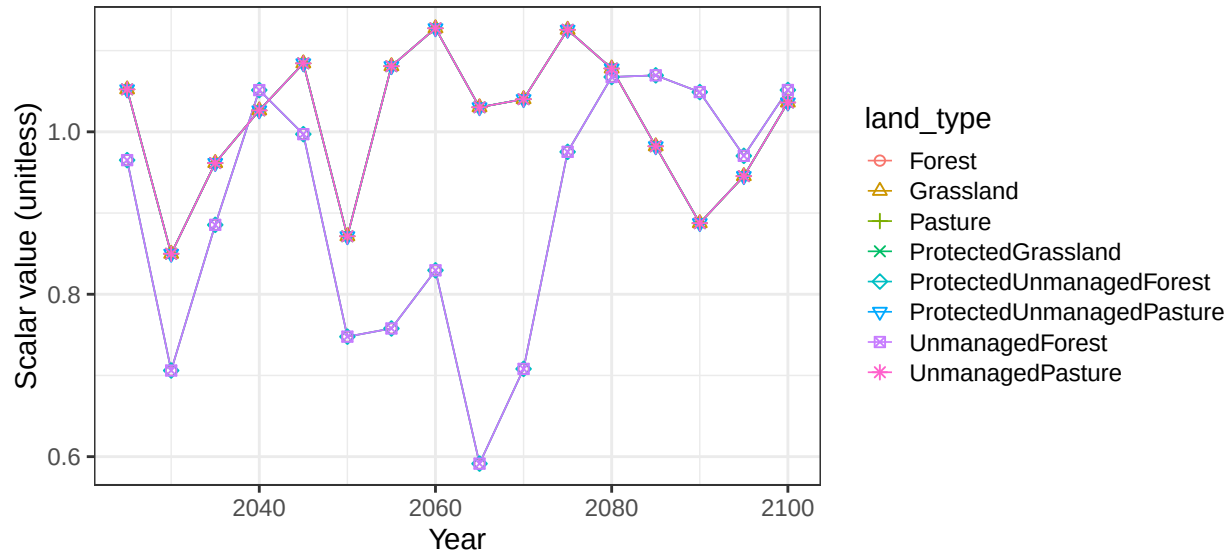
Region EU-12 basin ElbeR non-crop vegetation scalars
