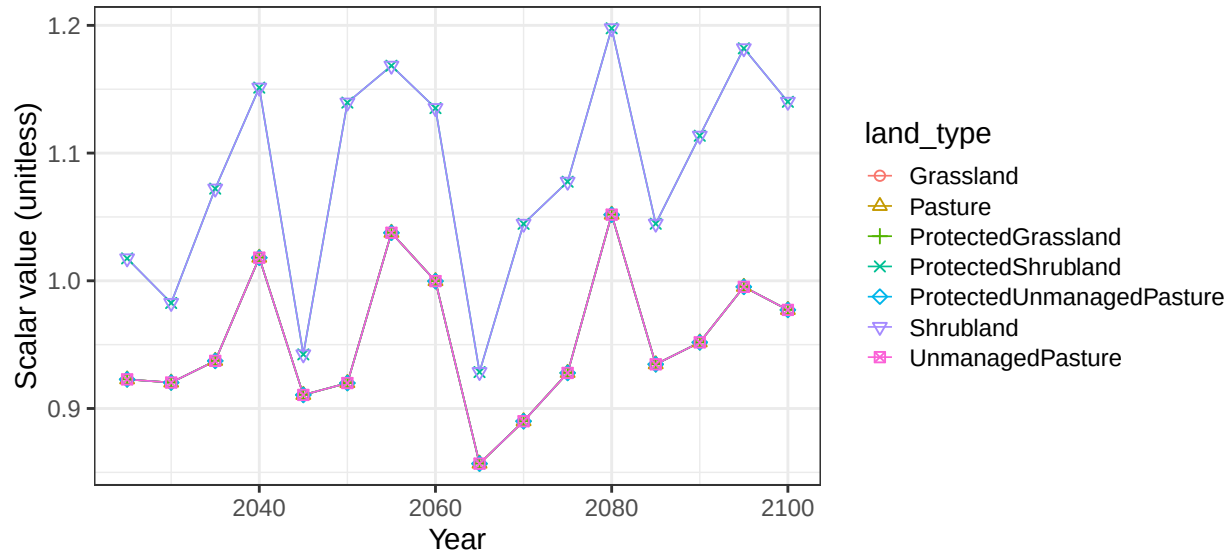
Region Africa_Southern basin OrangeR non-crop soil scalars
