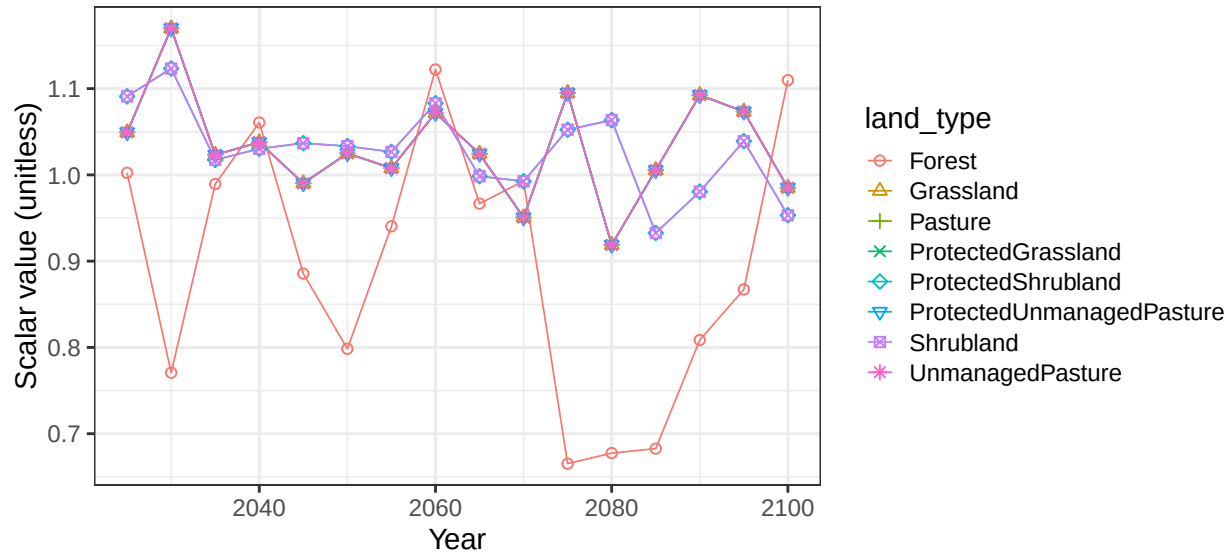
Region Middle East basin TigrEuphR non-crop soil scalars
