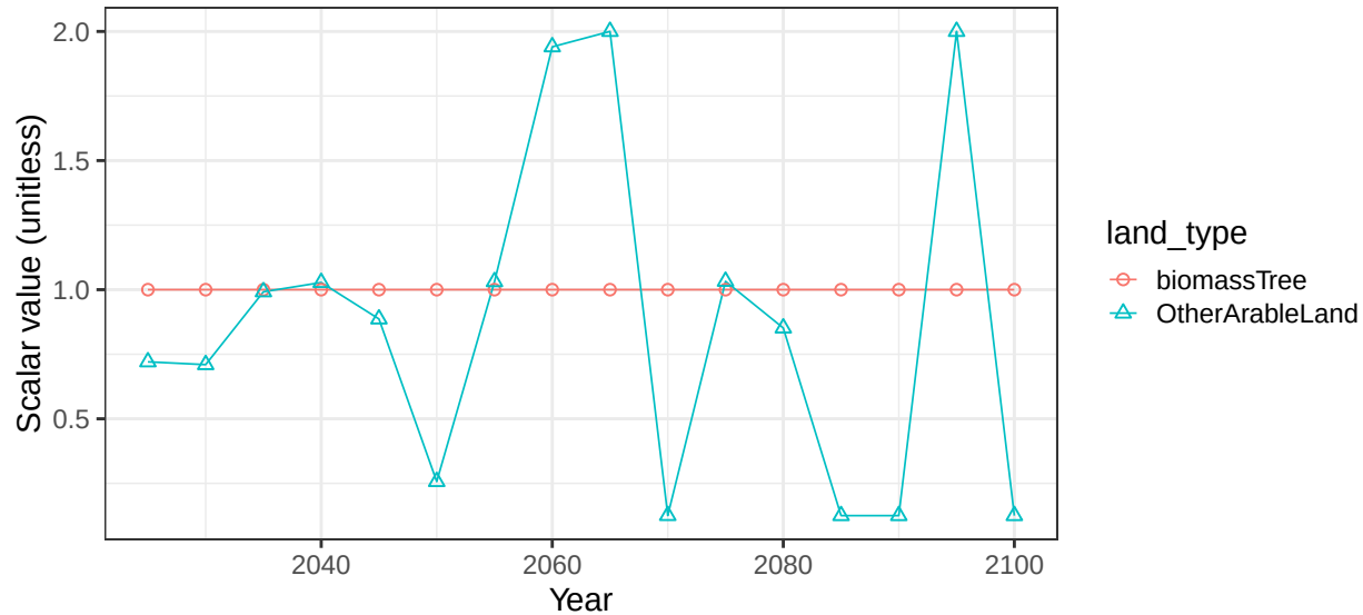
Region Russia basin ScndnvN crop vegetation scalars
