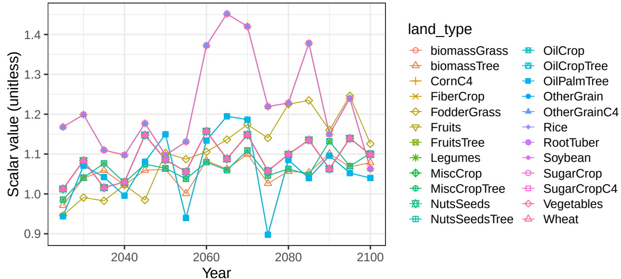
Region China basin Salween crop vegetation scalars
