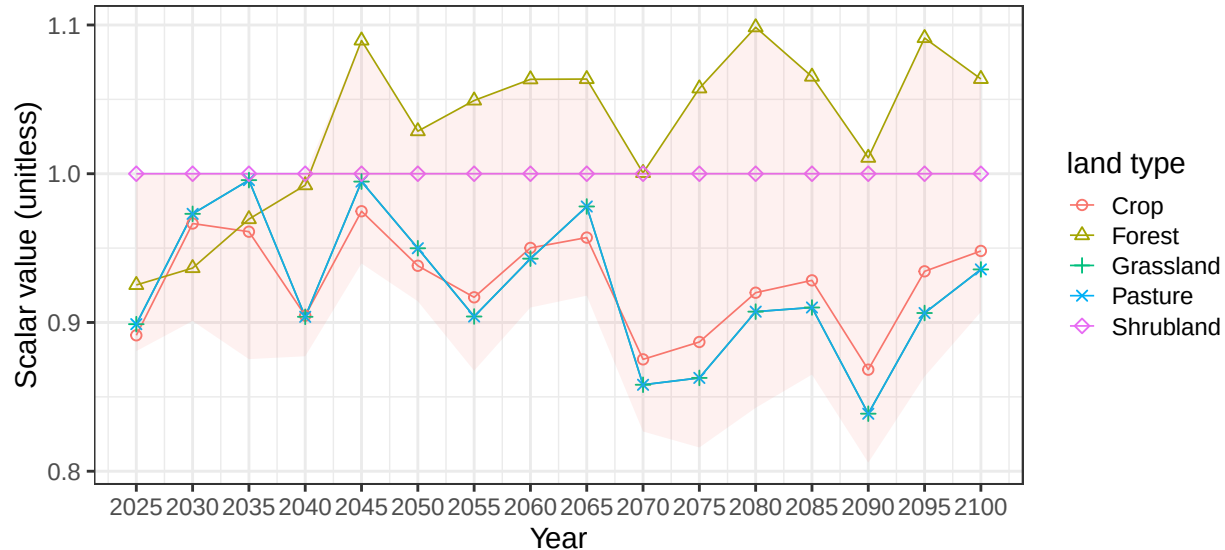
Region Mexico basin GrijUsuR average vegetation scalars
