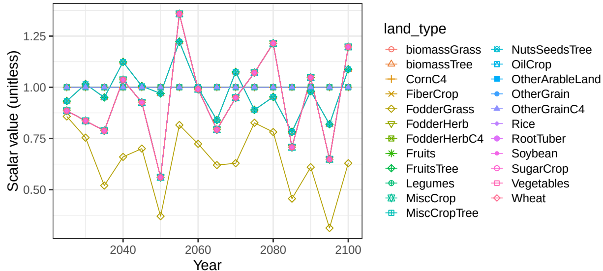
Region Europe_Eastern basin DniesterR crop vegetation scalars
