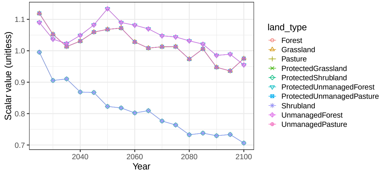
Region Africa_Southern basin AngolaCst non-crop soil scalars
