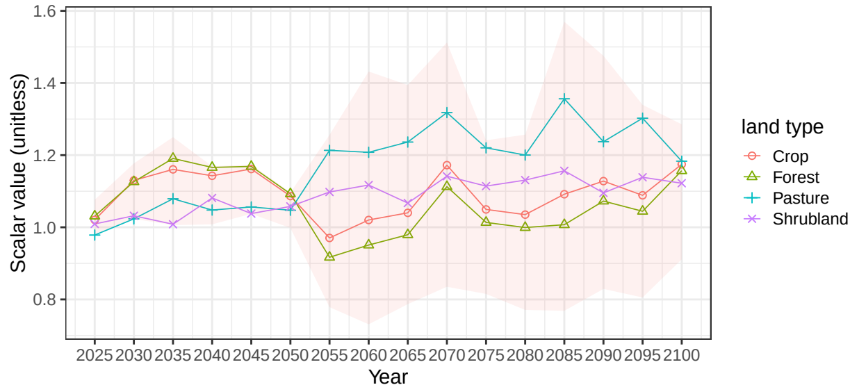
Region Southeast Asia basin GangesR average vegetation scalars
