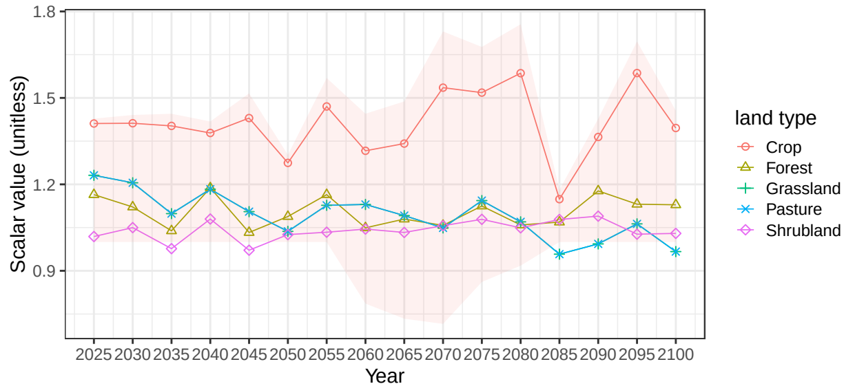
Region Canada basin NelsonR average vegetation scalars
