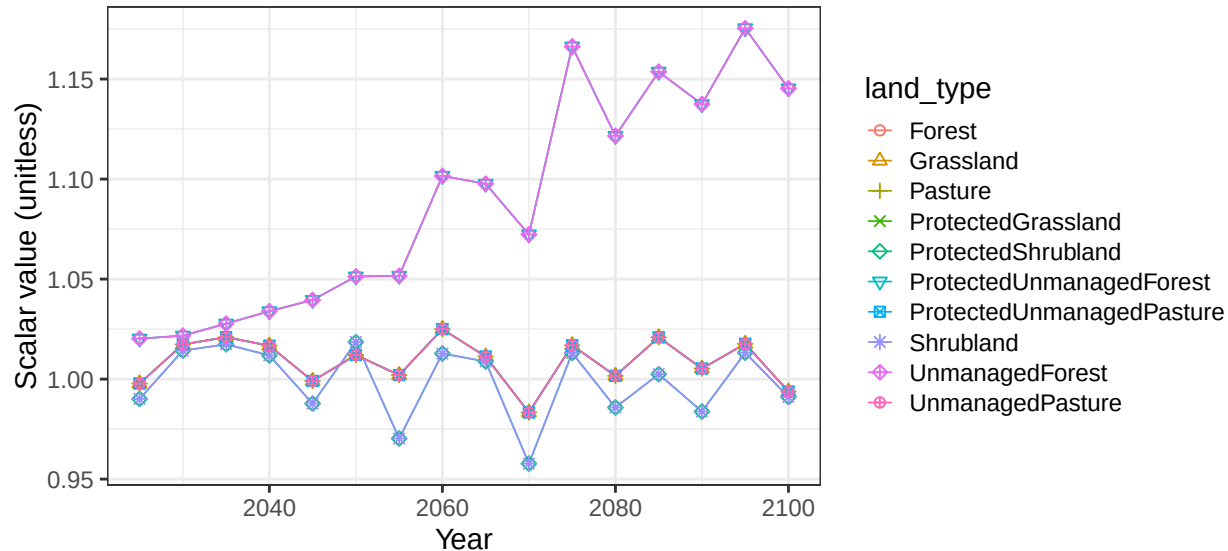
Region Argentina basin ArgCstS non-crop soil scalars
