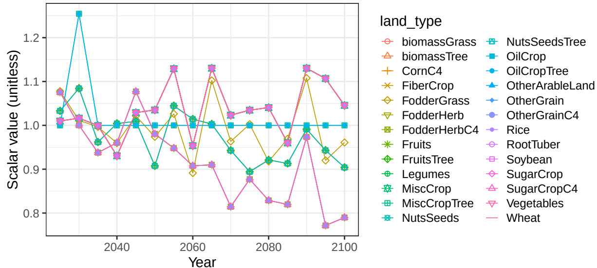
Region Africa_Northern basin AfrIntN crop soil scalars
