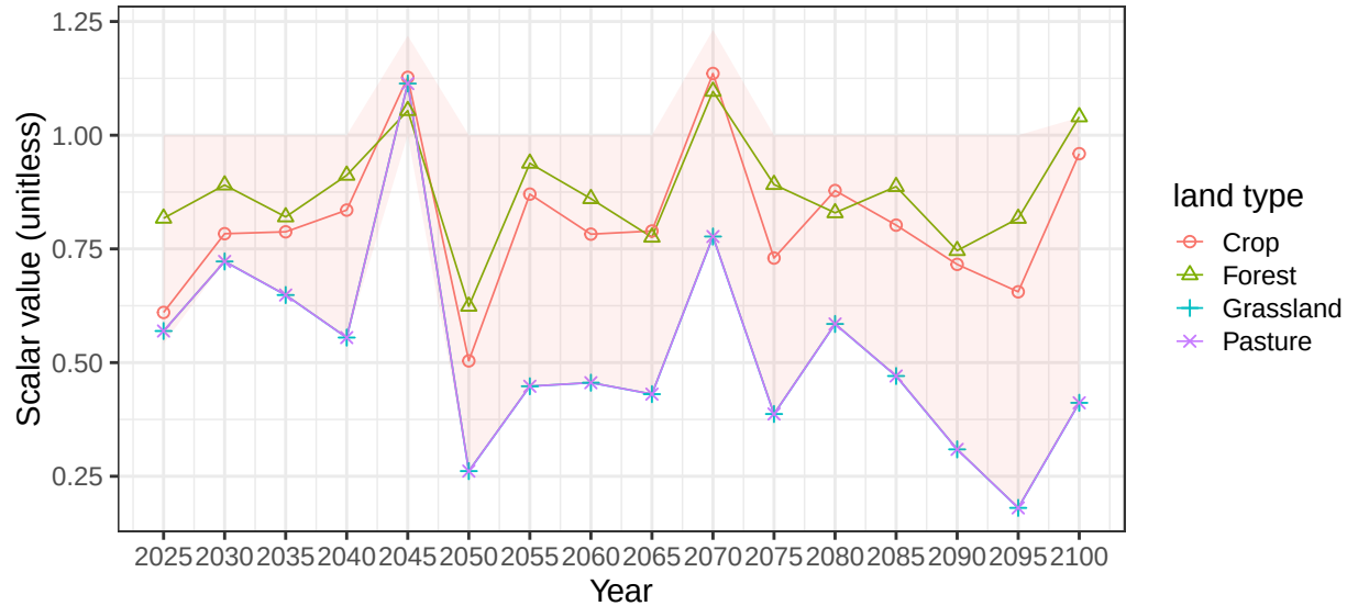
Region Russia basin DnieperR average vegetation scalars
