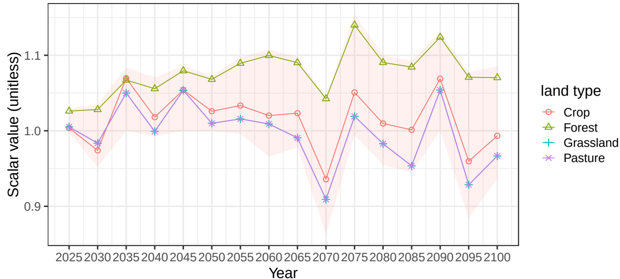
Region EU-15 basin EngWales average soil scalars
