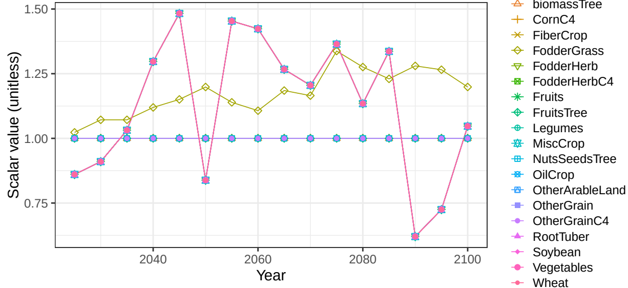
Region Russia basin LenaR crop vegetation scalars
