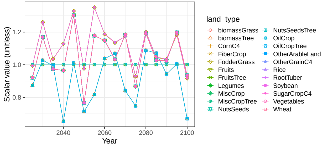
Region India basin PennarR crop soil scalars
