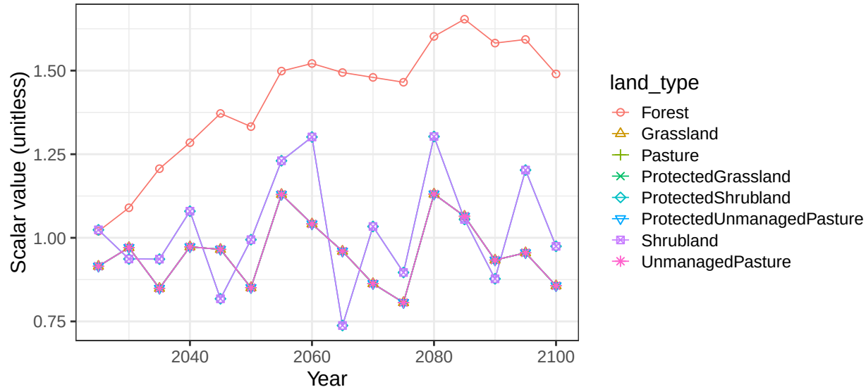
Region South Africa basin OrangeR non-crop vegetation scalars
