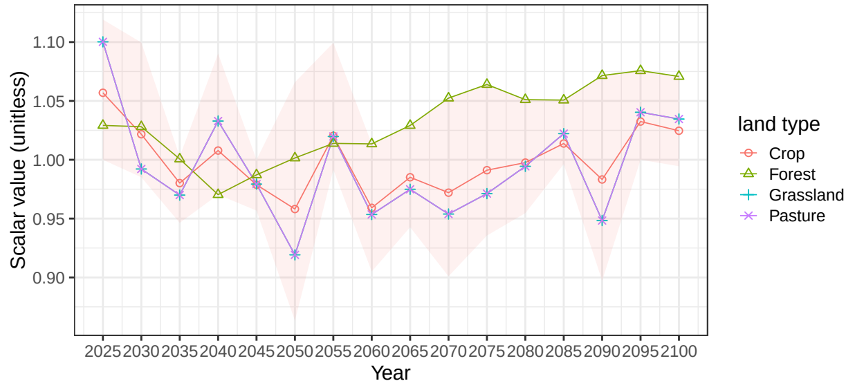
Region Southeast Asia basin PapuaCst average vegetation scalars
