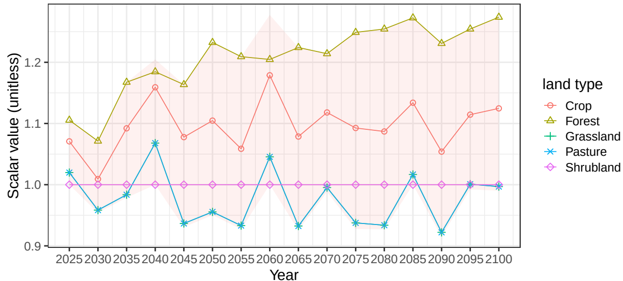
Region Brazil basin ParnaibaR average soil scalars
