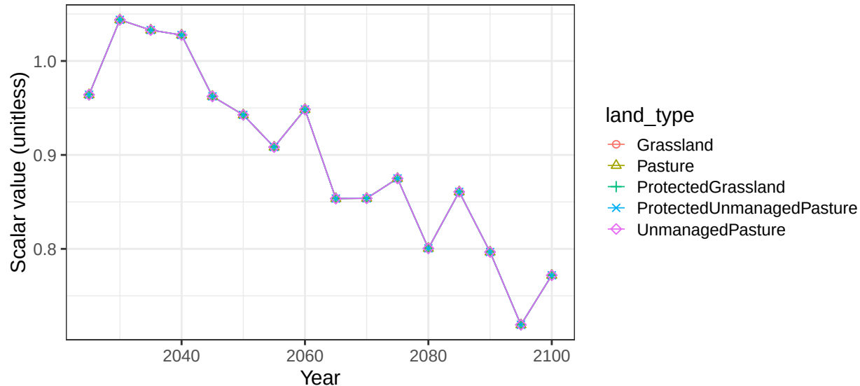
Region Argentina basin LaPuna non-crop vegetation scalars
