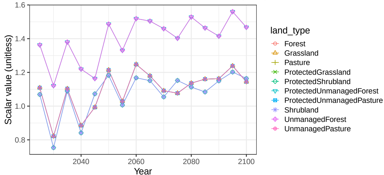
Region Central Asia basin YeniseiR non-crop vegetation scalars
