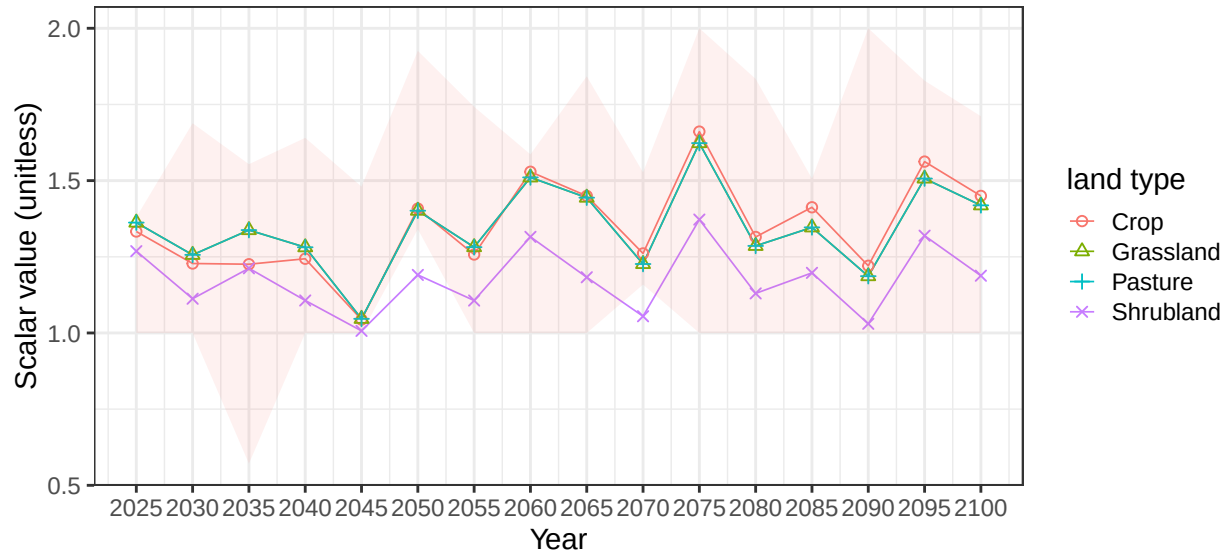
Region Middle East basin PersianGulf average vegetation scalars
