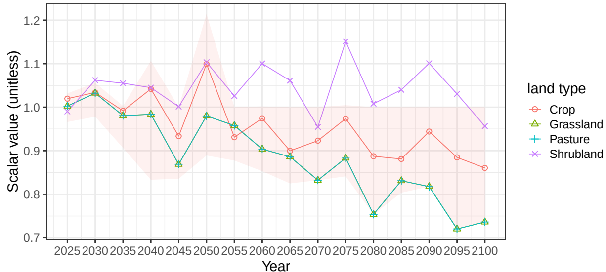
Region Middle East basin DeadSea average soil scalars
