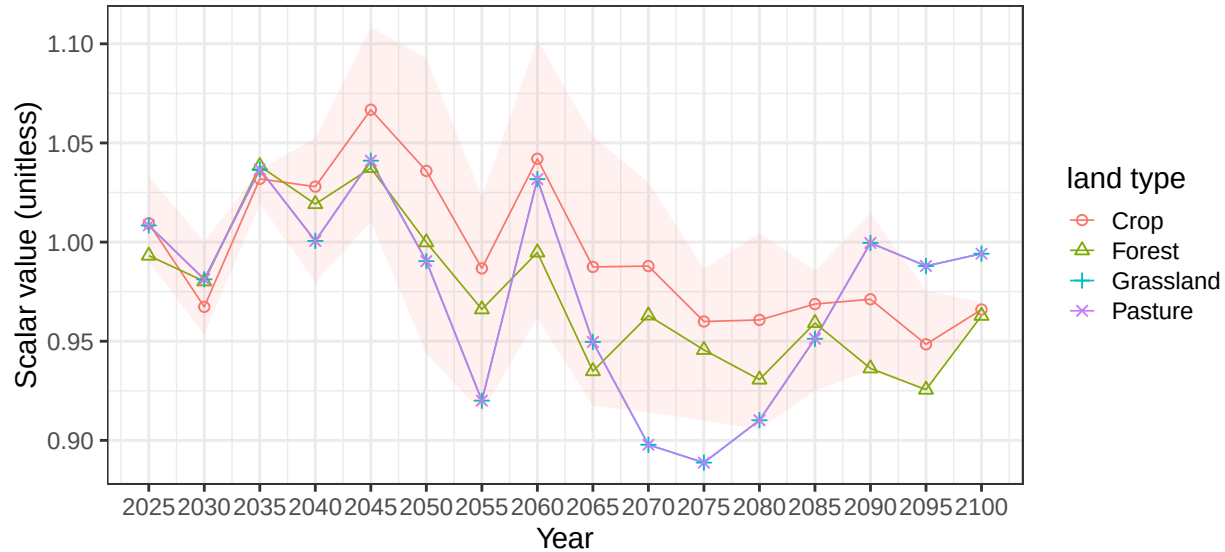
Region Southeast Asia basin RusCstSE average soil scalars
