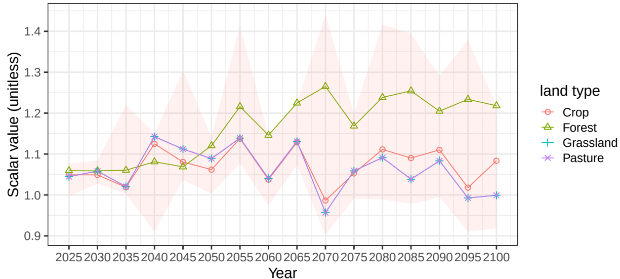
Region Africa_Southern basin AfrCstS average soil scalars
