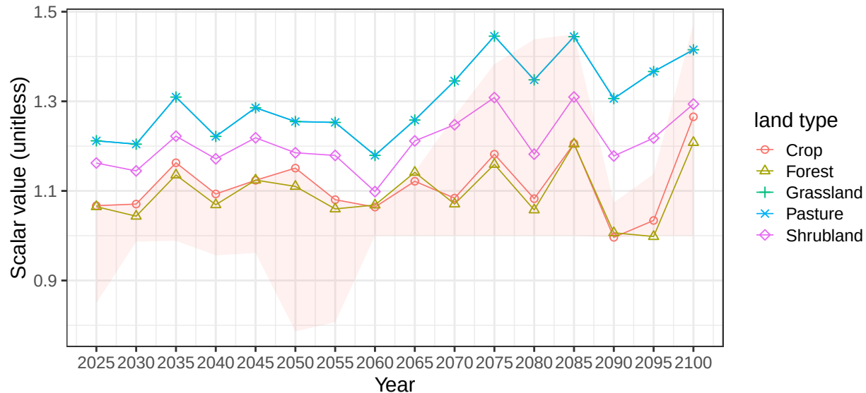
Region Canada basin PacArctic average vegetation scalars
