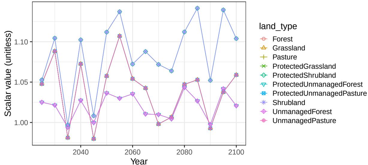
Region Taiwan basin Taiwan non-crop soil scalars
