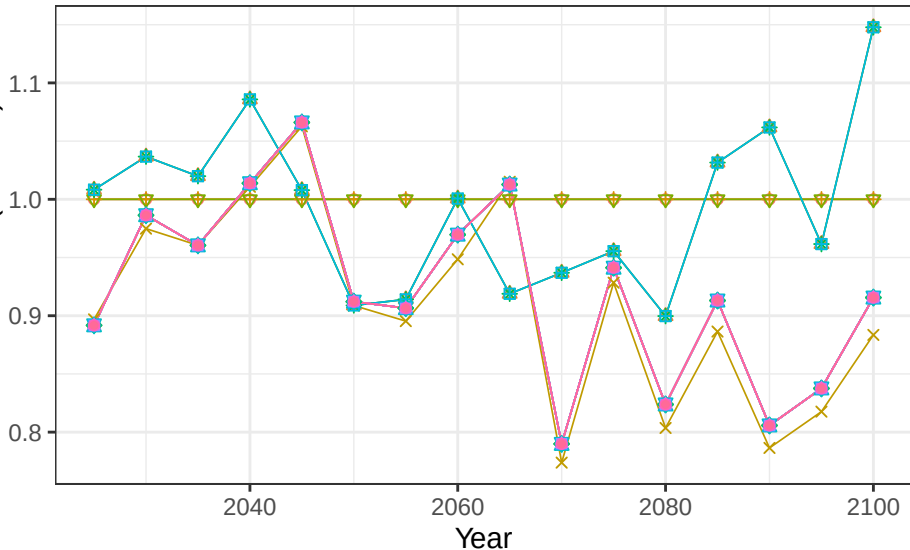
Region EU-15 basin OderR crop soil scalars
