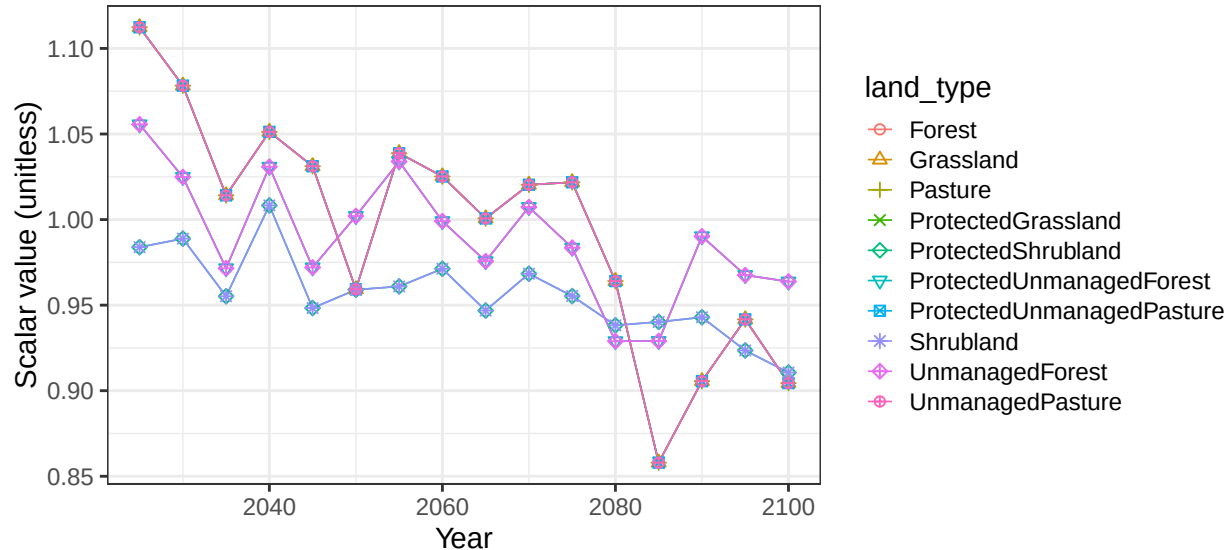
Region Canada basin NelsonR non-crop soil scalars
