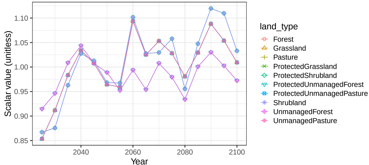
Region Canada basin HudsonBay non-crop vegetation scalars
