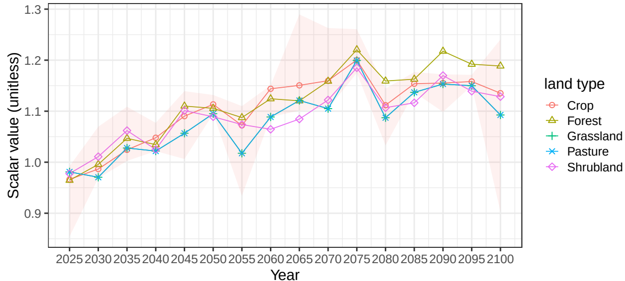
Region Russia basin AmurR average vegetation scalars
