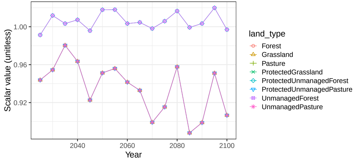
Region Indonesia basin Sumatra non-crop soil scalars
