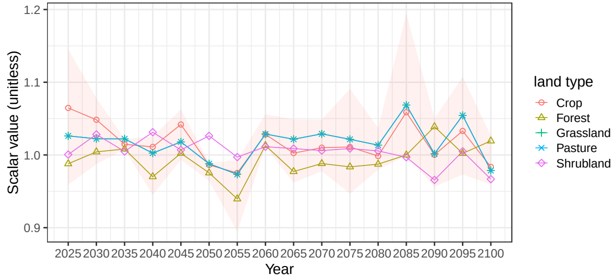
Region China basin IrrawaddyR average soil scalars
