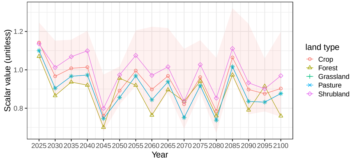
Region Mexico basin RioGrande average soil scalars
