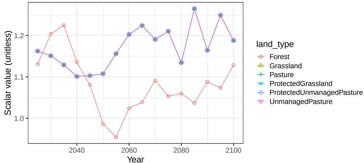
Region India basin IrrawaddyR non-crop soil scalars
