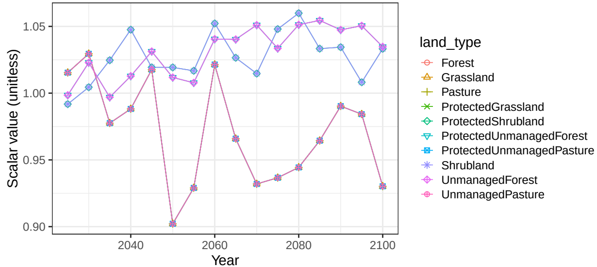
Region South America_Southern basin AmazonR non-crop vegetation sca
