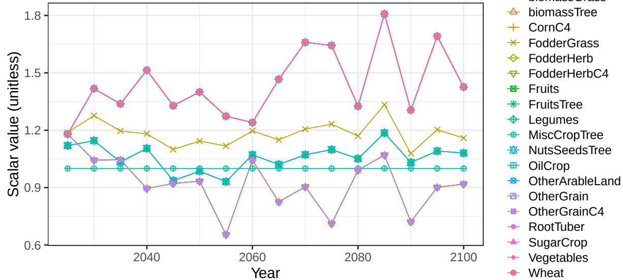
Region USA basin UsaColoRN crop vegetation scalars
