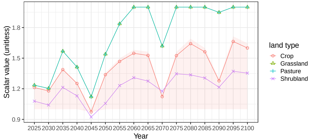
Region South Asia basin FarahrudR average vegetation scalars
