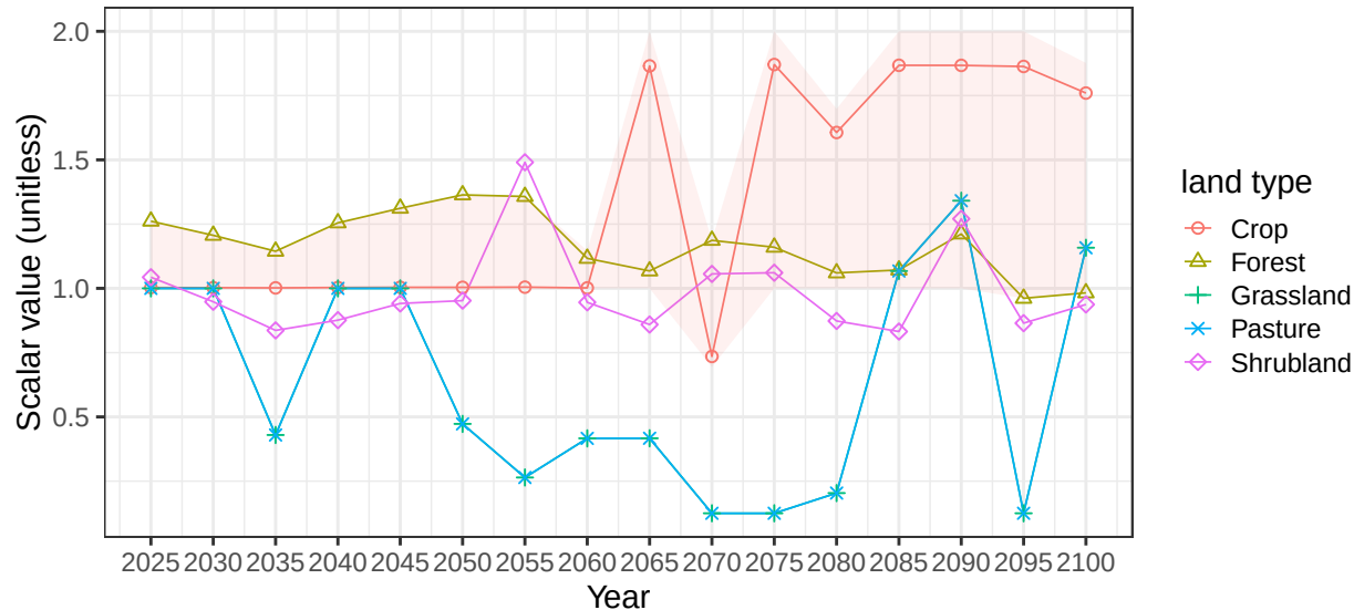
Region South Africa basin AfrCstSSW average vegetation scalars
