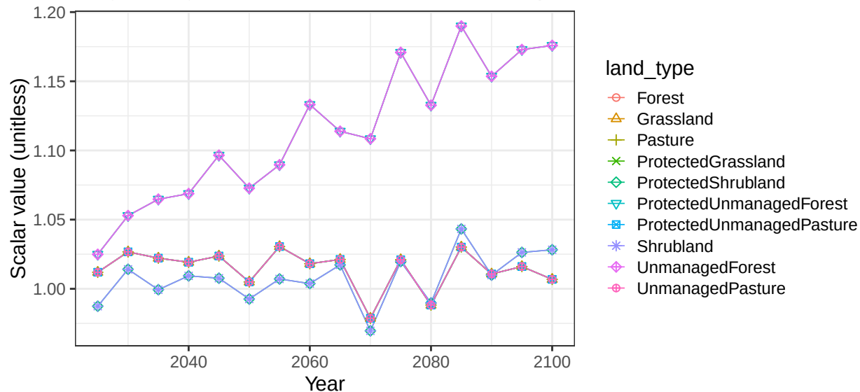
Region Argentina basin ChileCstS non-crop soil scalars
