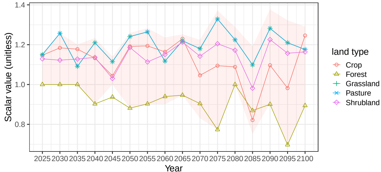
Region Middle East basin CaspianE average soil scalars
