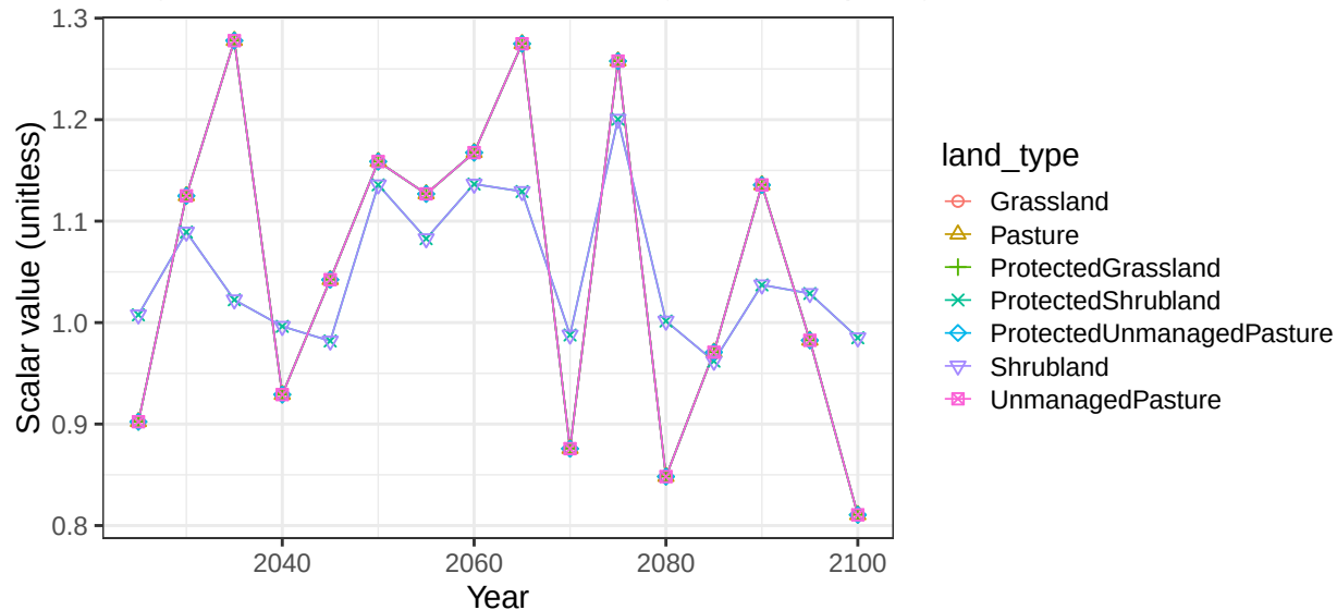
Region Middle East basin EJrdnSyr non-crop vegetation scalars
