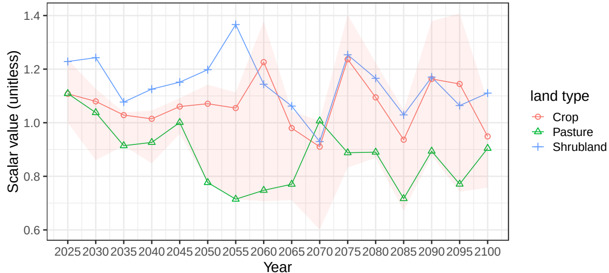
Region Pakistan basin HamuMashR average soil scalars
