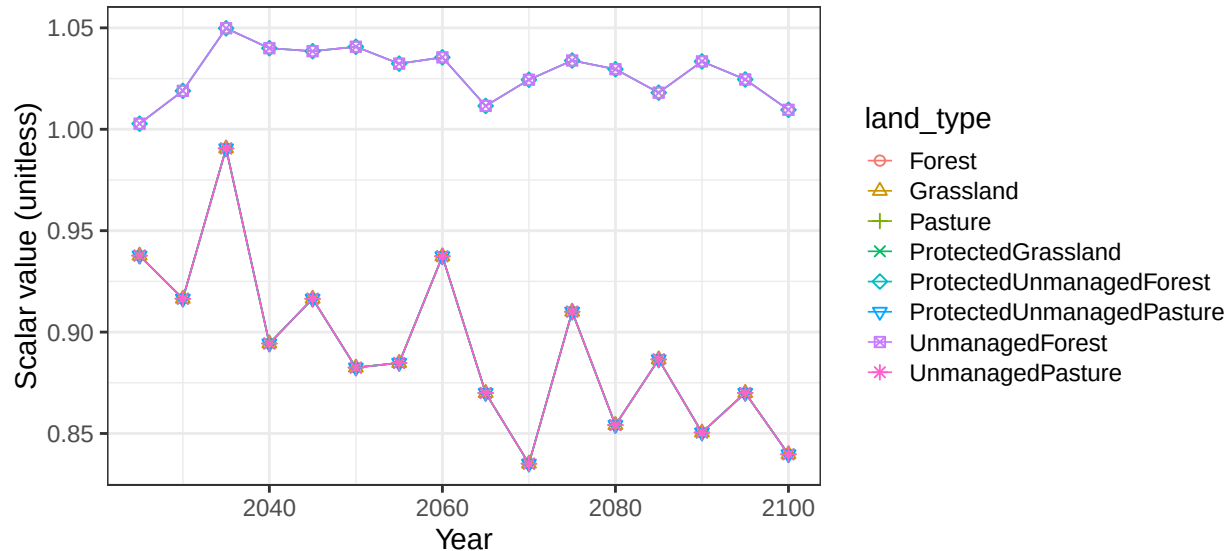
Region Indonesia basin Sulawesi non-crop soil scalars
