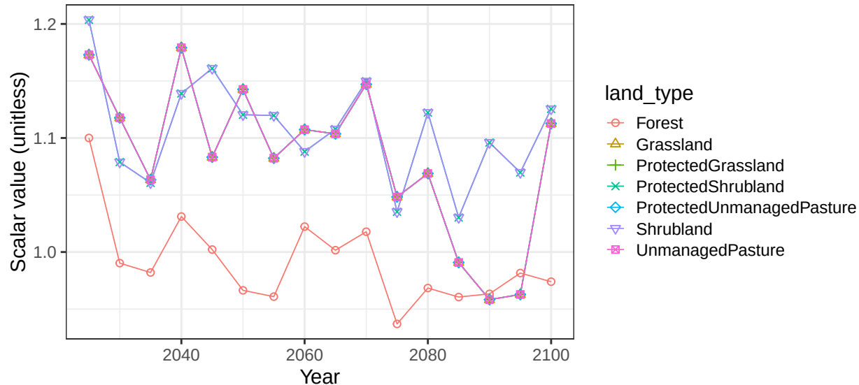
Region EU-15 basin DouroR non-crop soil scalars
