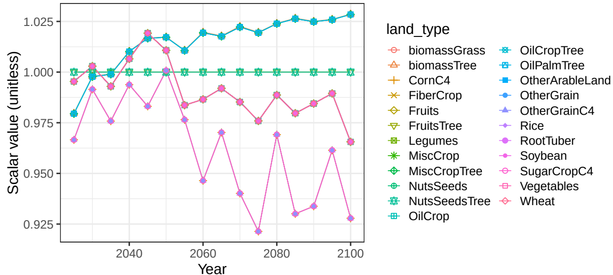
Region Africa_Western basin GuineaGulf crop soil scalars
