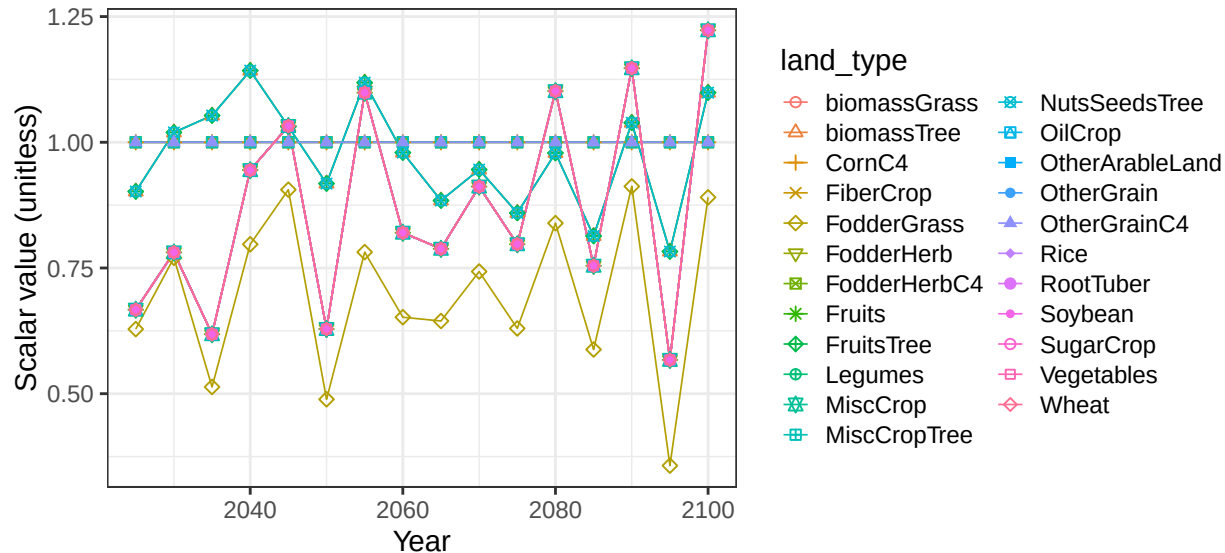
Region Europe_Eastern basin WislaR crop vegetation scalars
