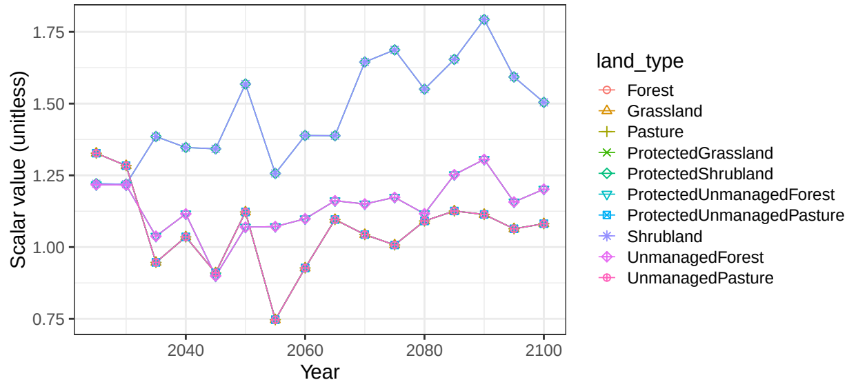
Region USA basin UsaColoRS non-crop vegetation scalars
