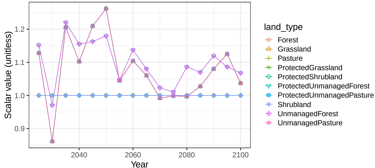
Region Africa_Southern basin NileR non-crop soil scalars
