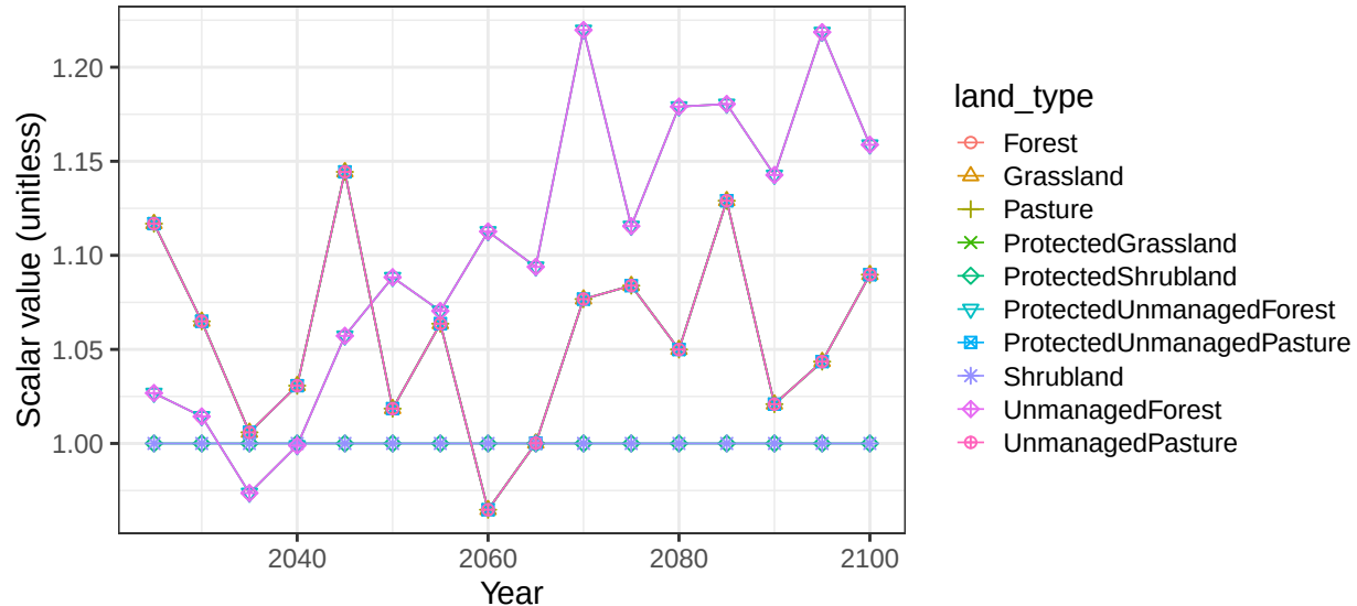
Region Southeast Asia basin VietnamCst non-crop vegetation scalars
