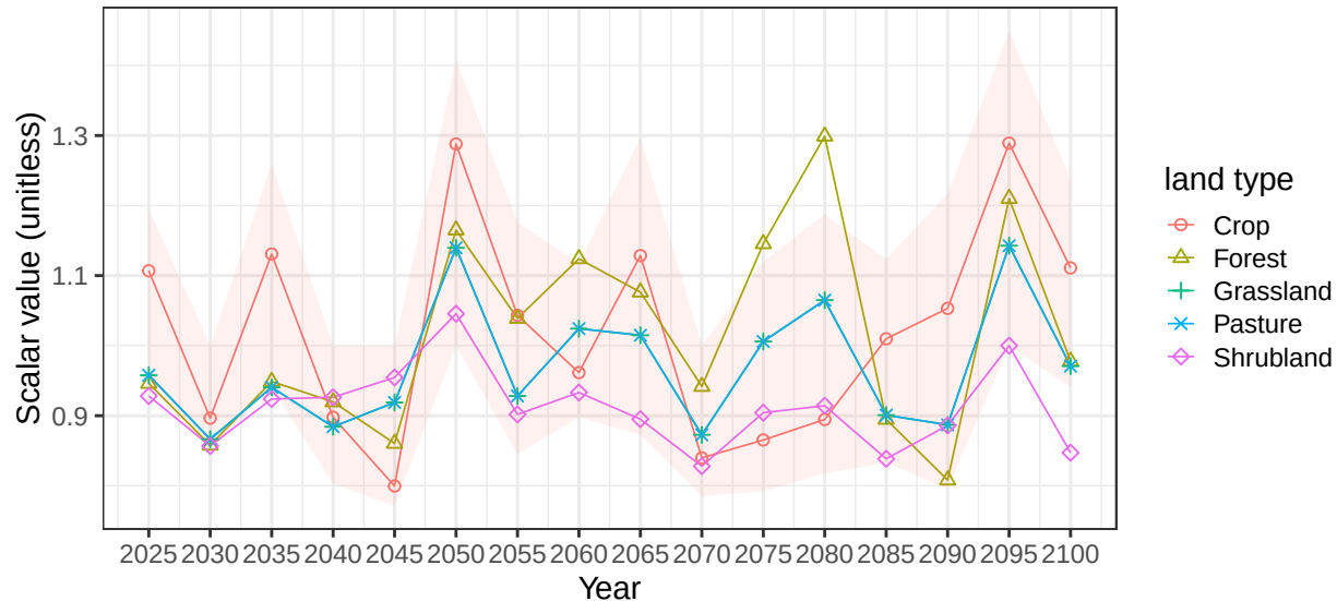
Region China basin LBalkash average soil scalars
