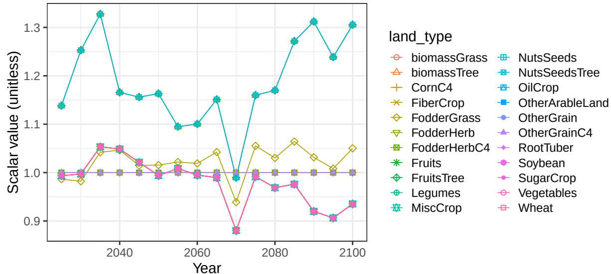
Region EU-15 basin RhineR crop soil scalars
