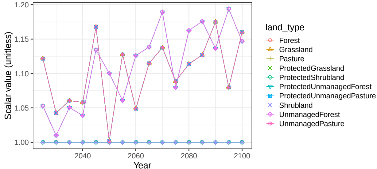
Region Southeast Asia basin Mekong non-crop vegetation scalars
