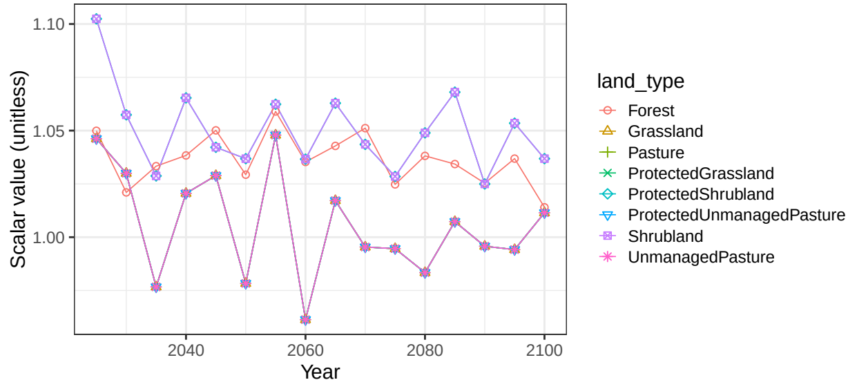
Region China basin XunJiang non-crop soil scalars
