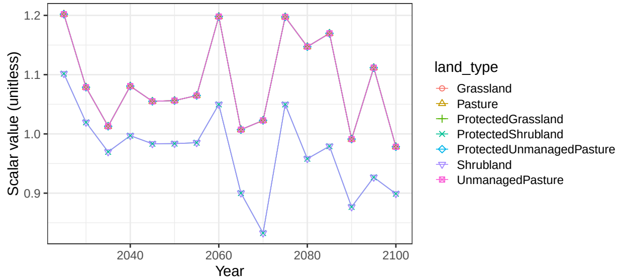
Region Middle East basin Helmand non-crop soil scalars
