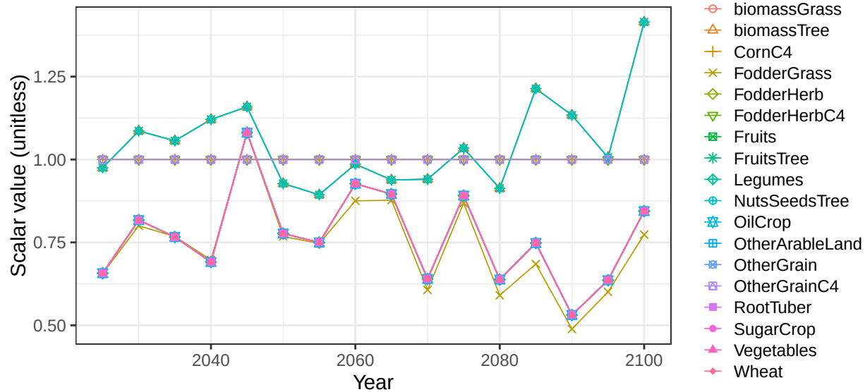
Region EU-12 basin DnkGrnCst crop vegetation scalars land_type
