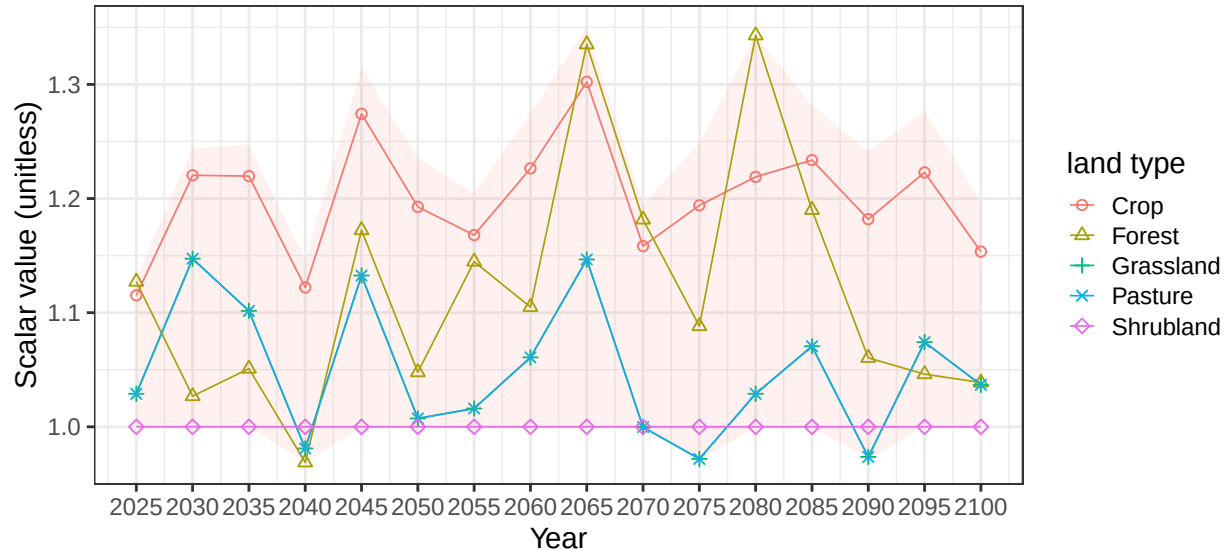
Region India basin MahanadiR average soil scalars
