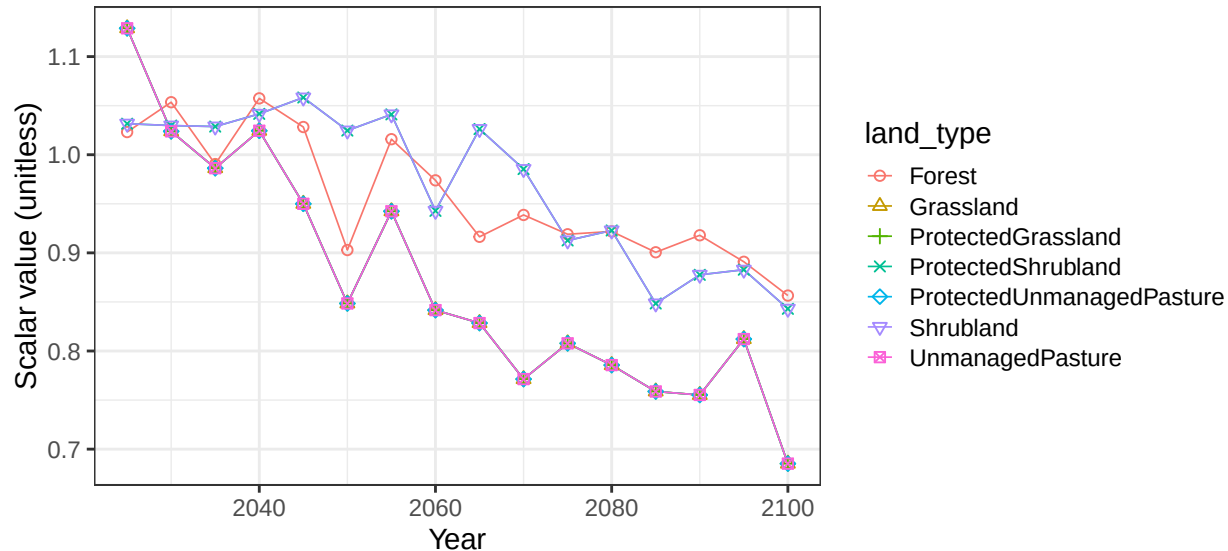
Region EU-15 basin Meditlsl non-crop soil scalars
