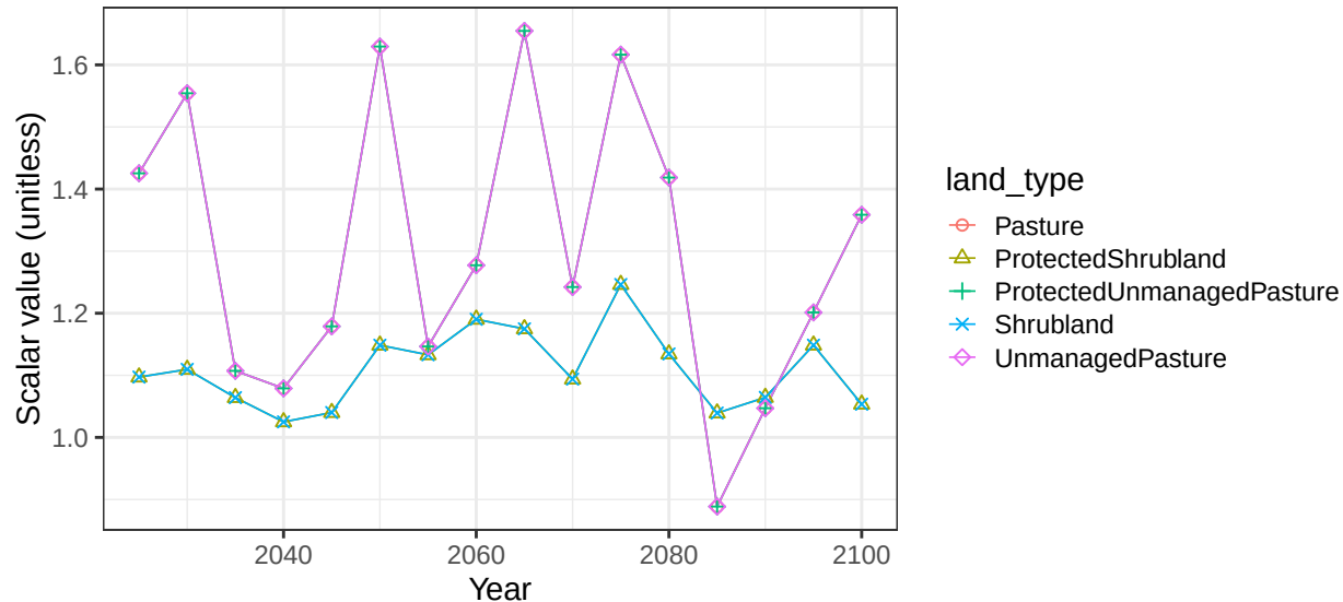
Region Europe_Non_EU basin EJrdnSyr non-crop vegetation scalars
