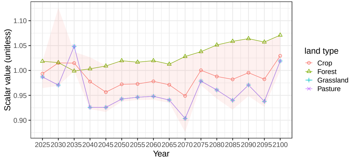
Region Colombia basin AmazonR average vegetation scalars
