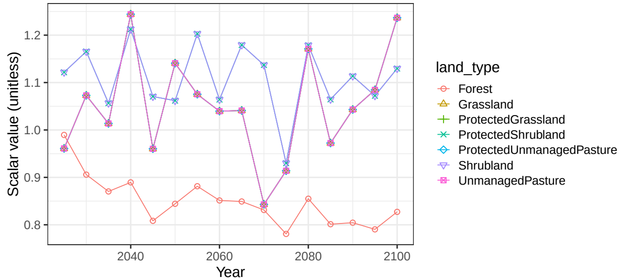
Region EU-15 basin GuadalqR non-crop soil scalars
