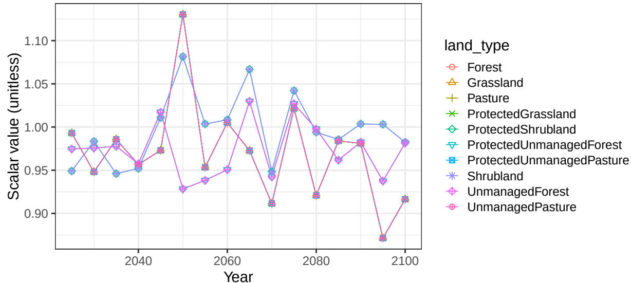
Region Central Asia basin SyrDaryaR non-crop soil scalars
