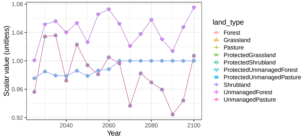
Region Mexico basin Tehuantepec non-crop soil scalars
