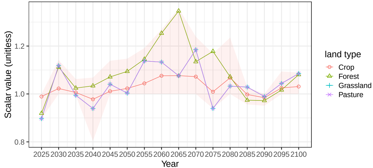
Region Russia basin CaspianSW average vegetation scalars
