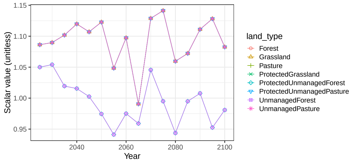
Region USA basin GreatLakes non-crop soil scalars
