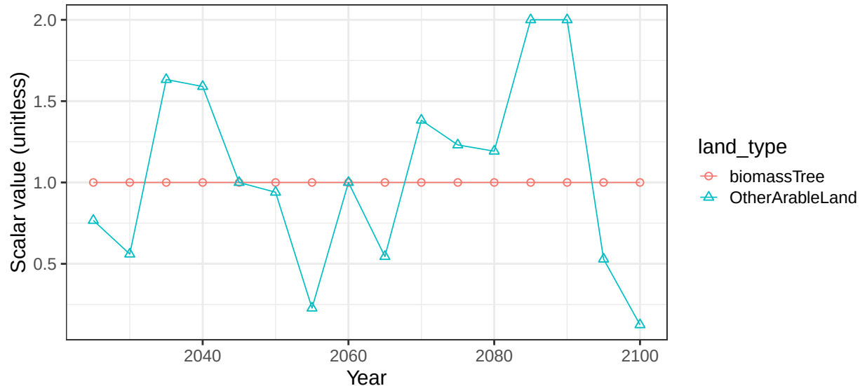
Region Canada basin ChurchillR crop vegetation scalars
