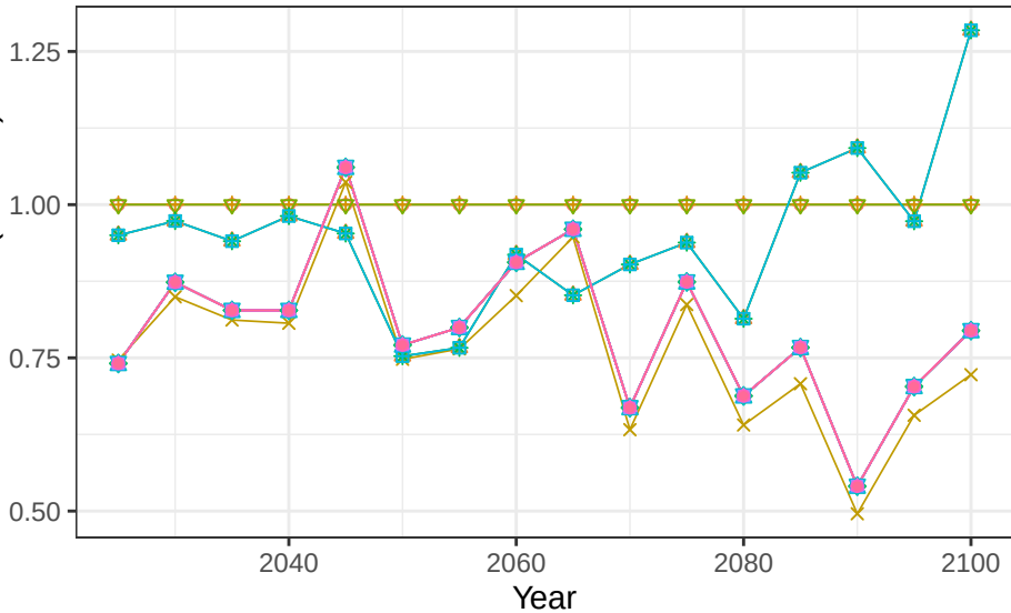
Region EU-15 basin OderR crop vegetation scalars
