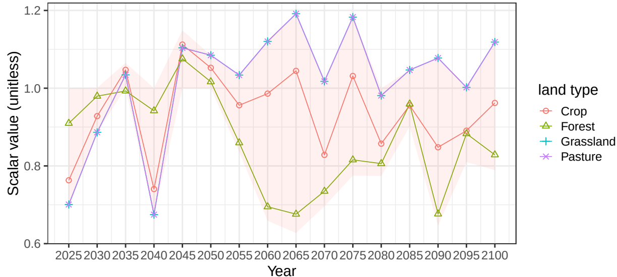
Region EU-15 basin DnkGrmCst average vegetation scalars
