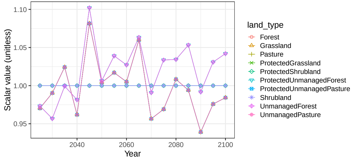
Region Central America and Caribbean basin GrijUsuR non-crop vegetati
