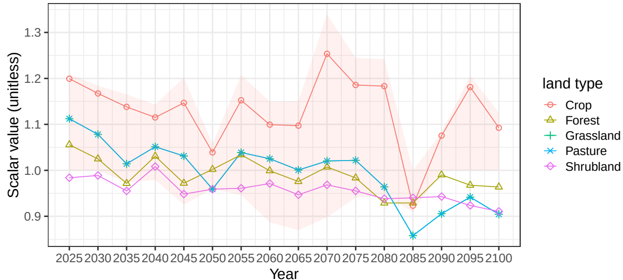
Region Canada basin NelsonR average soil scalars
