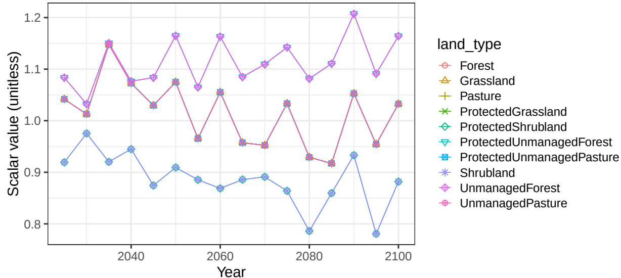
Region Africa_Southern basin RiftValley non-crop soil scalars
