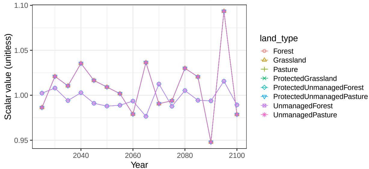
Region Brazil basin OrinocoR non-crop soil scalars
