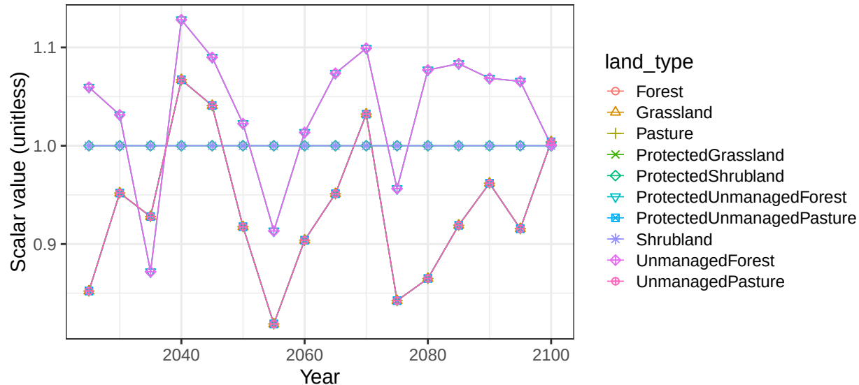
Region Southeast Asia basin SittaungR non-crop vegetation scalars
