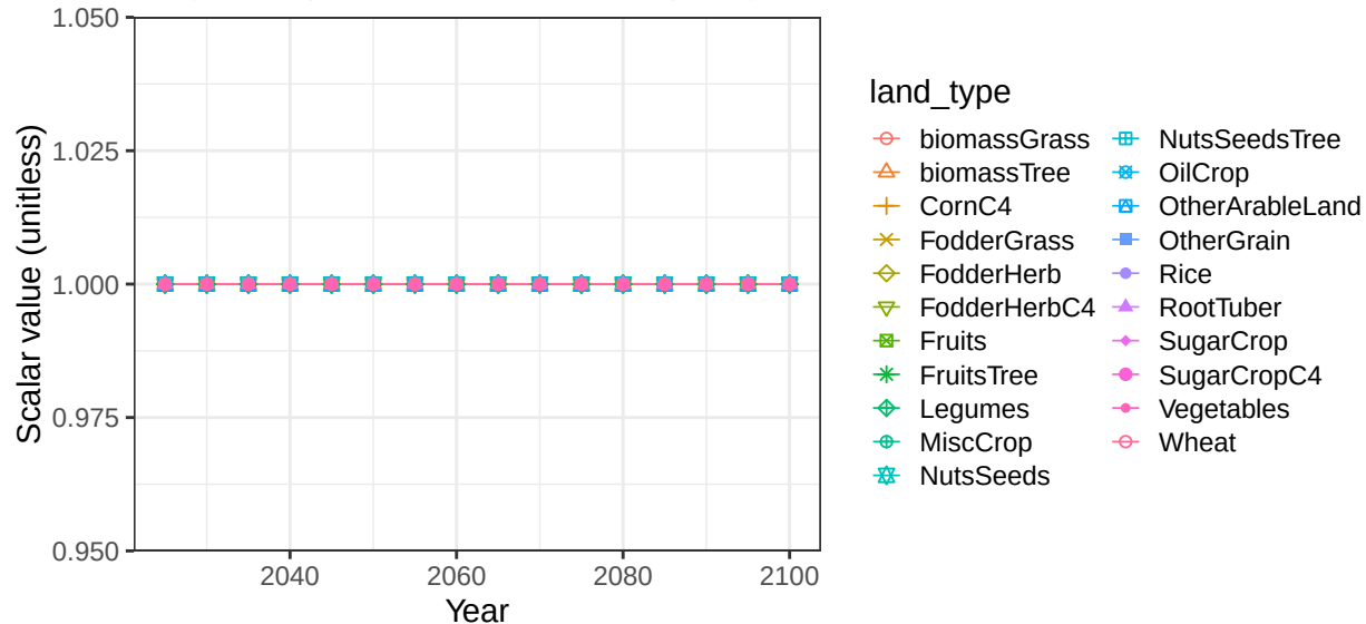
Region Japan basin Taiwan crop vegetation scalars
