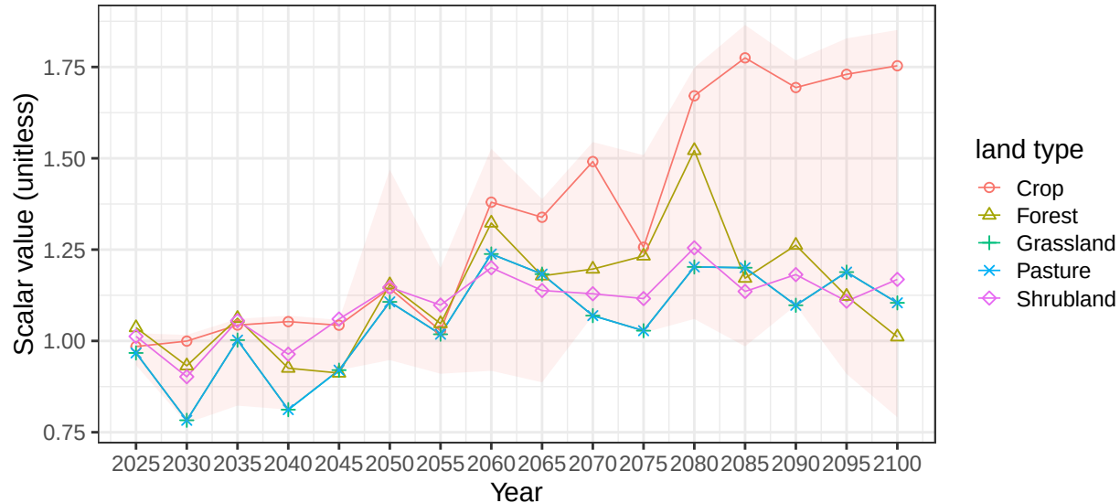
Region Central Asia basin Gobi average vegetation scalars
