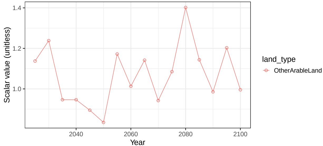
Region EU-15 basin MeditE crop vegetation scalars
