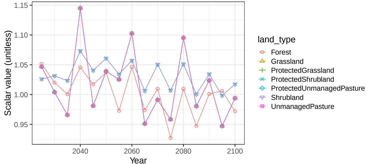
Region EU-15 basin PoR non-crop soil scalars
