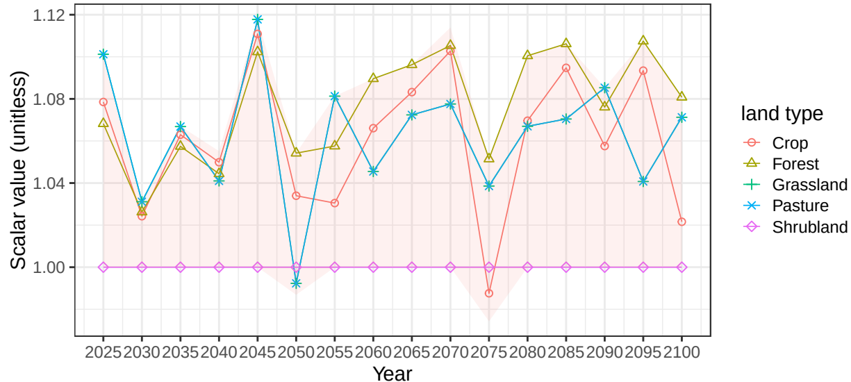
Region Southeast Asia basin Mekong average soil scalars
