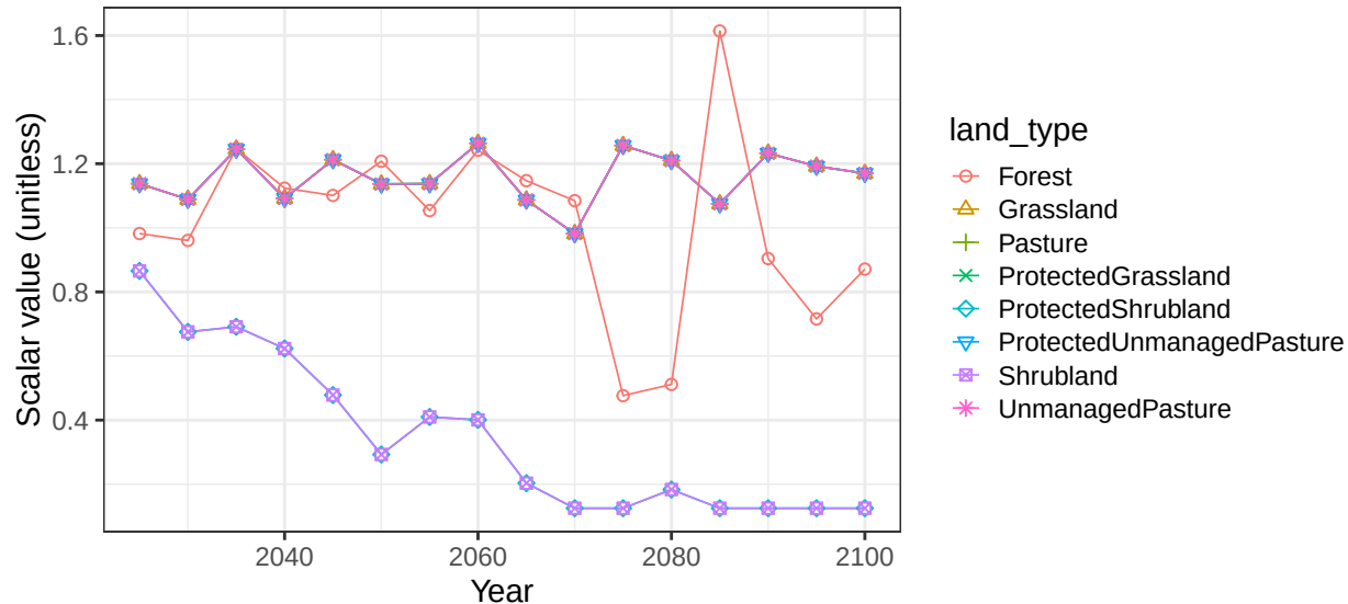
Region Africa_Eastern basin RiftValley non-crop vegetation scalars
