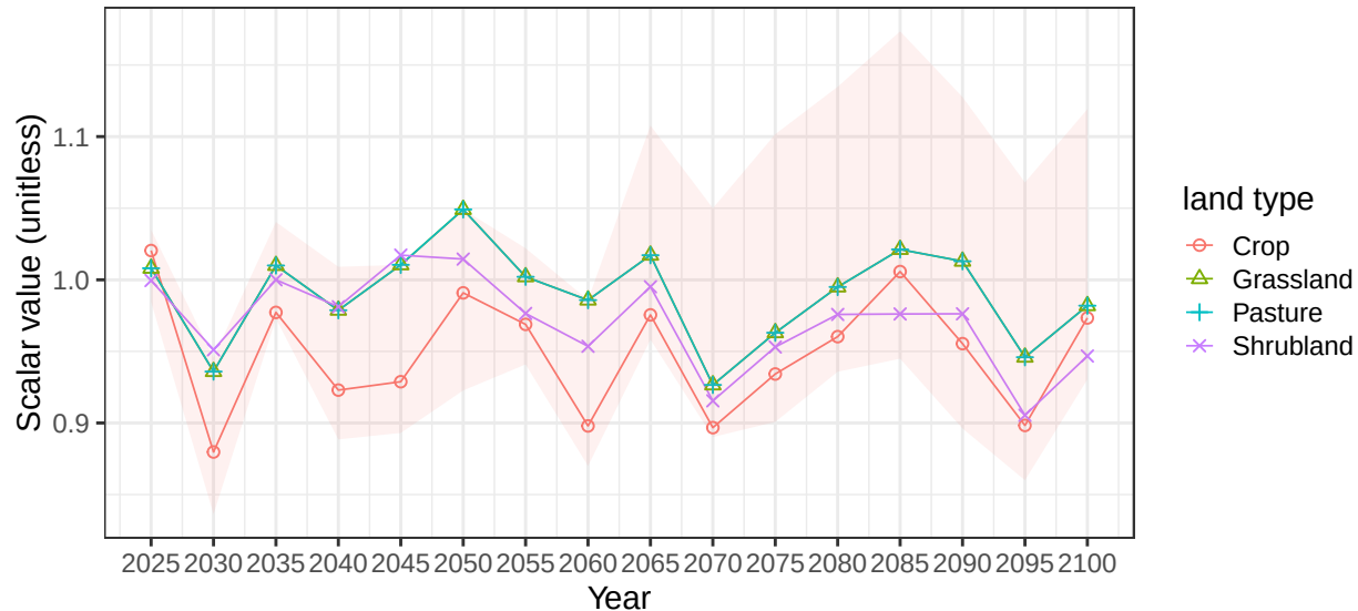
Region Central Asia basin Tarim average soil scalars
