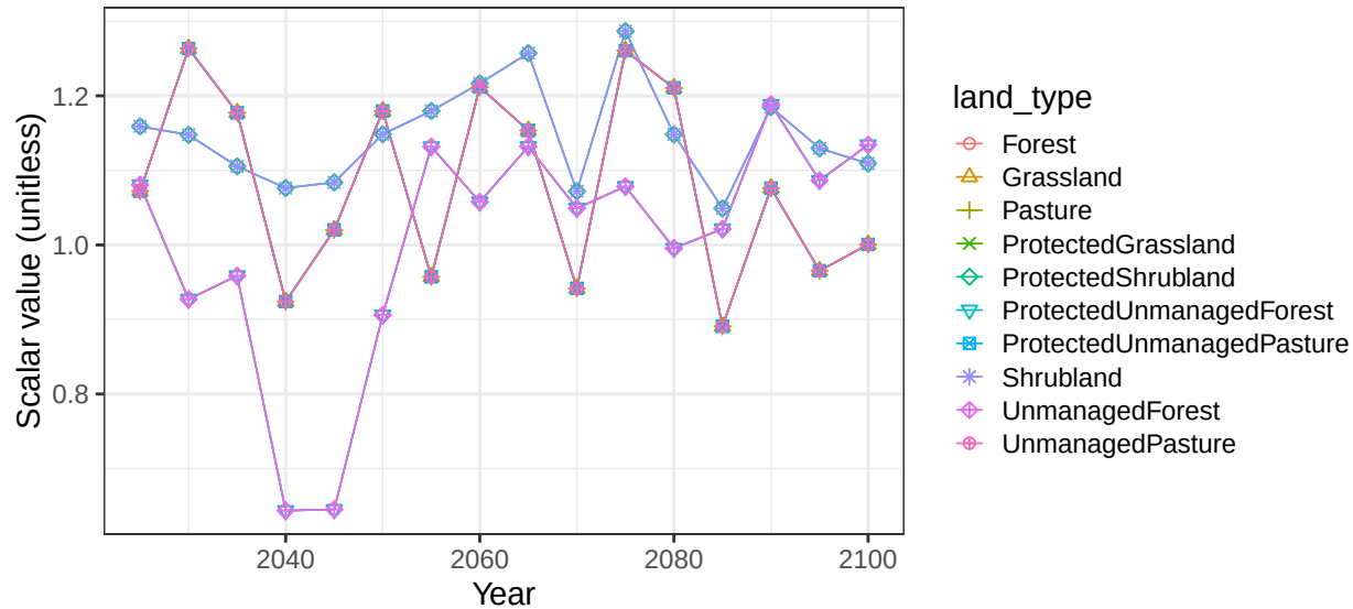
Region Europe_Non_EU basin TigrEuphR non-crop vegetation scalars
