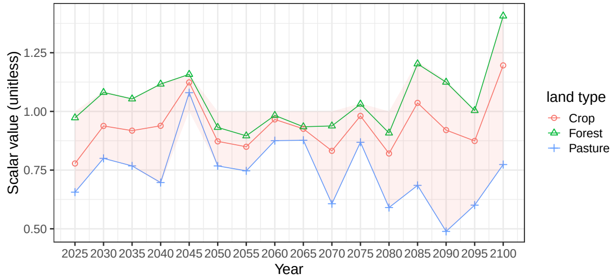
Region EU-12 basin DnkGrnCst average vegetation scalars
