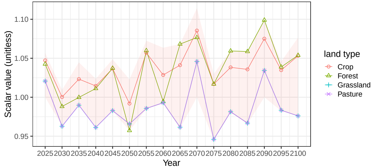
Region South Asia basin SriLanka average soil scalars
