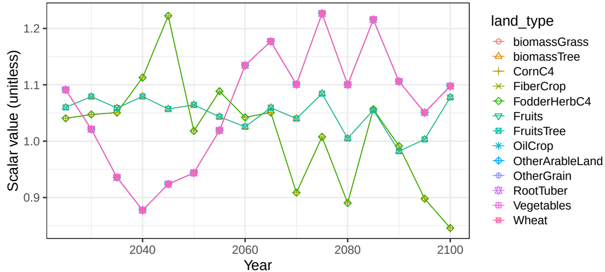
Region Canada basin FraserR crop soil scalars
