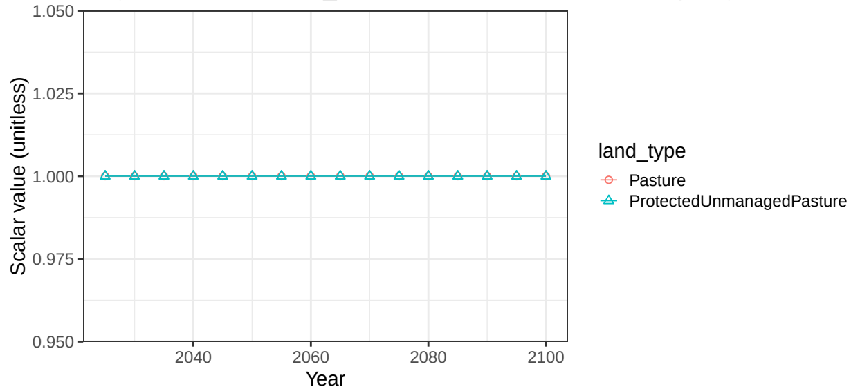
Region South America_Southern basin Salinas non-crop vegetation scalar
