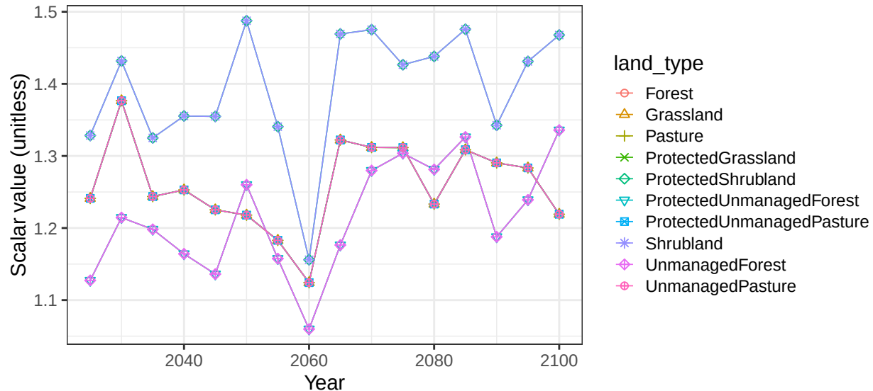
Region USA basin UsaPacNW non-crop vegetation scalars
