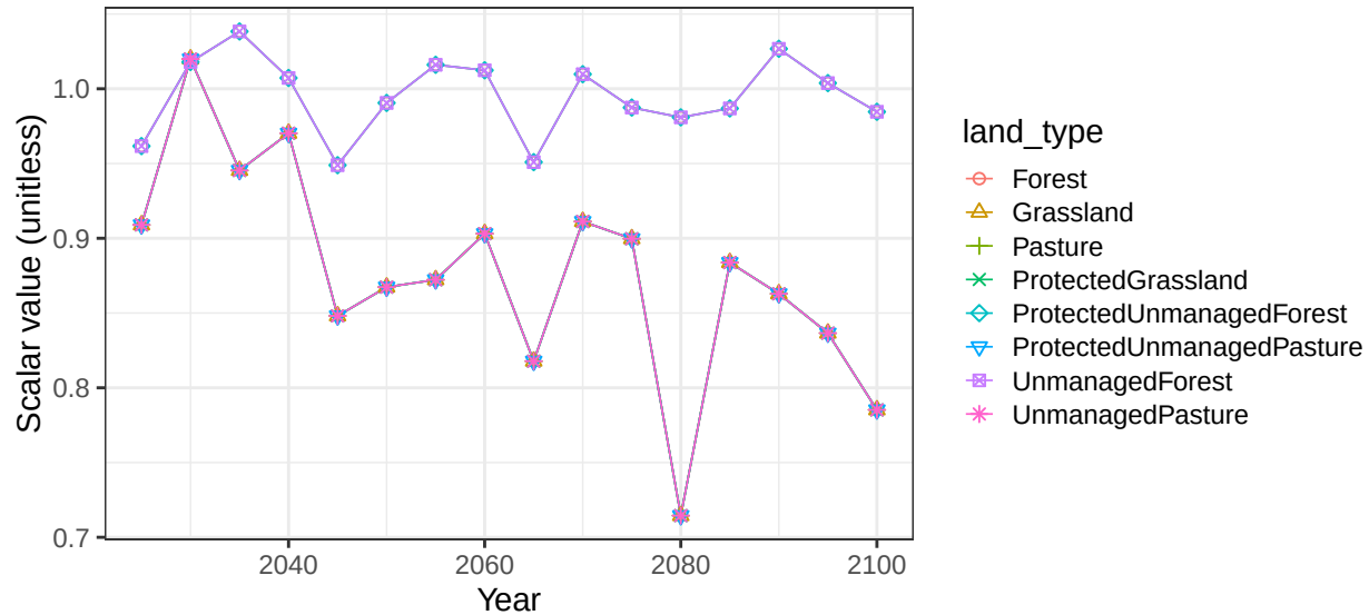
Region Southeast Asia basin JavaTimor non-crop soil scalars
