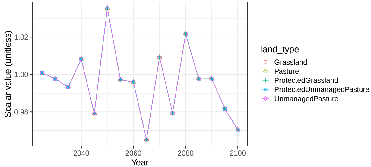
Region China basin Tibet non-crop soil scalars
