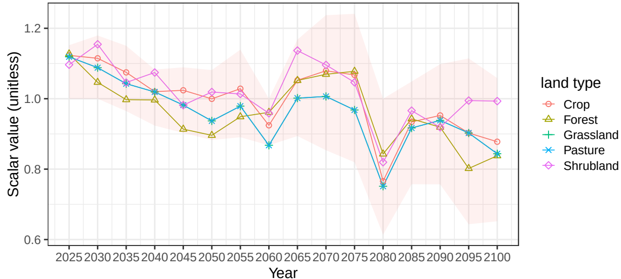
Region USA basin MissouriR average soil scalars
