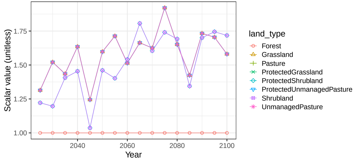
Region Middle East basin CaspianE non-crop vegetation scalars
