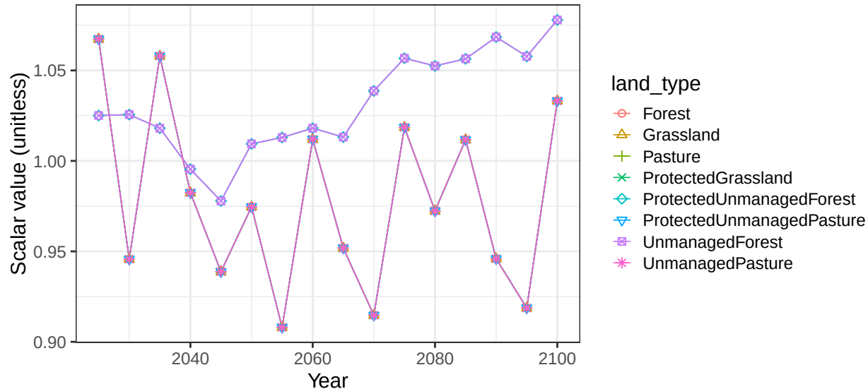
Region Southeast Asia basin FlyR non-crop vegetation scalars
