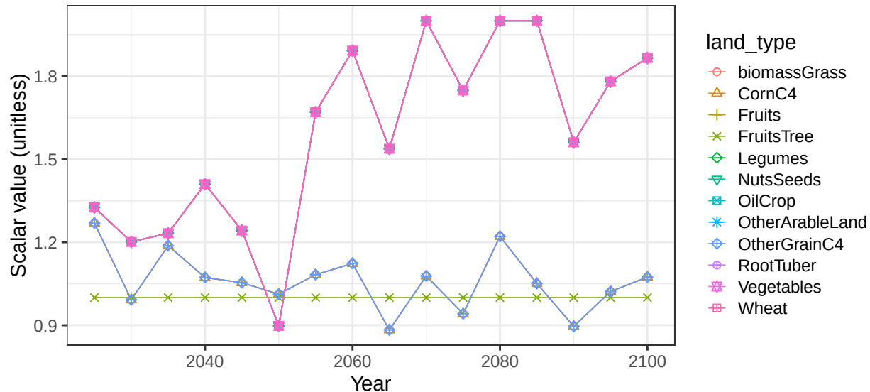
Region Africa_Southern basin AfrCstSW crop vegetation scalars
