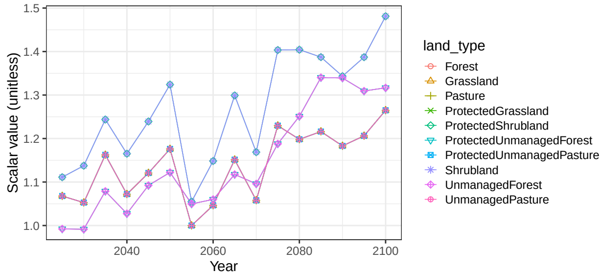
Region Russia basin SiberiaW non-crop vegetation scalars
