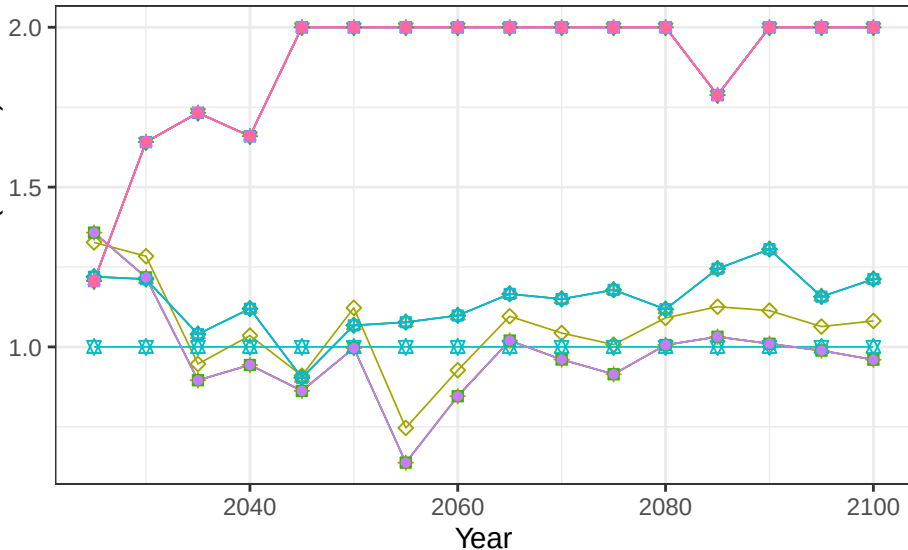
Region USA basin UsaColoRS crop vegetation scalars
