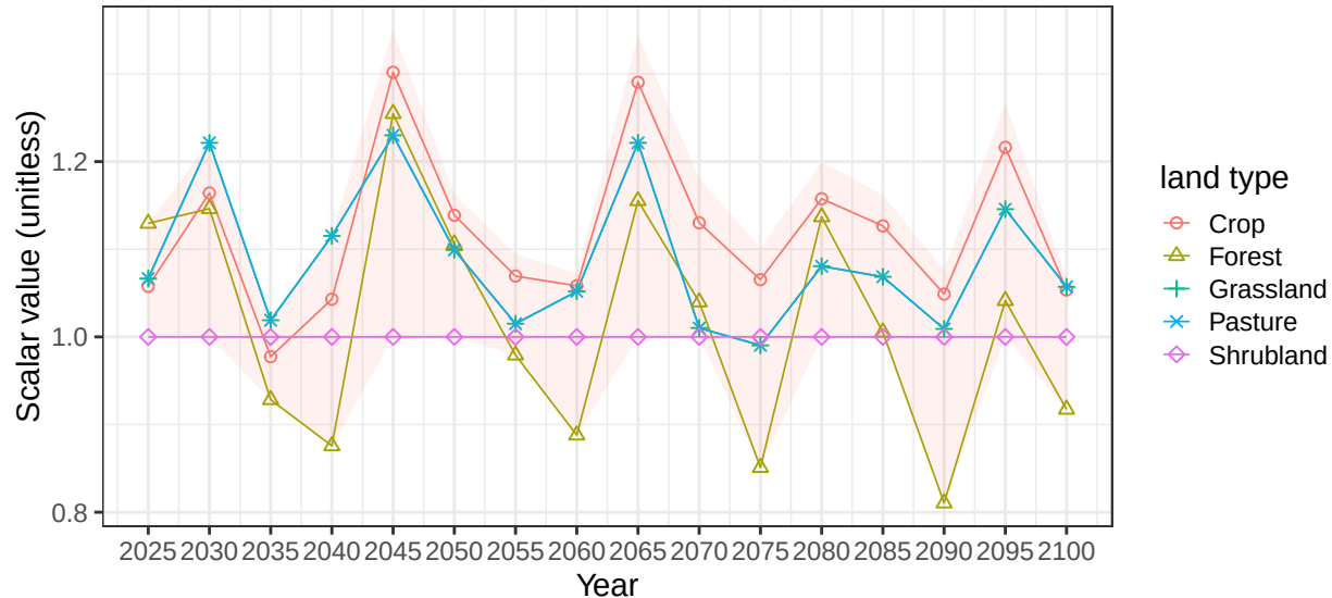
Region India basin IndCstNE average soil scalars
