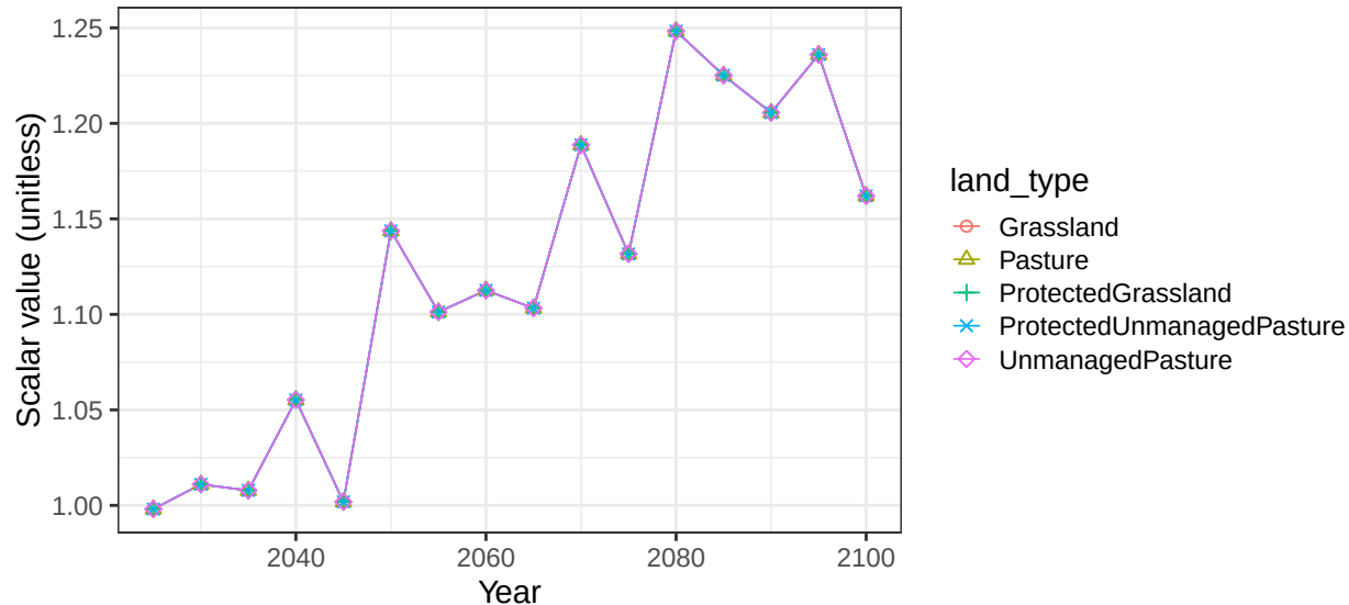
Region China basin Tibet non-crop vegetation scalars
