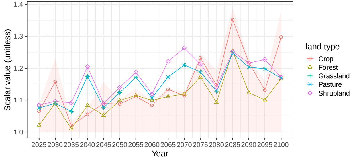
Region Canada basin Mackenzie average vegetation scalars
