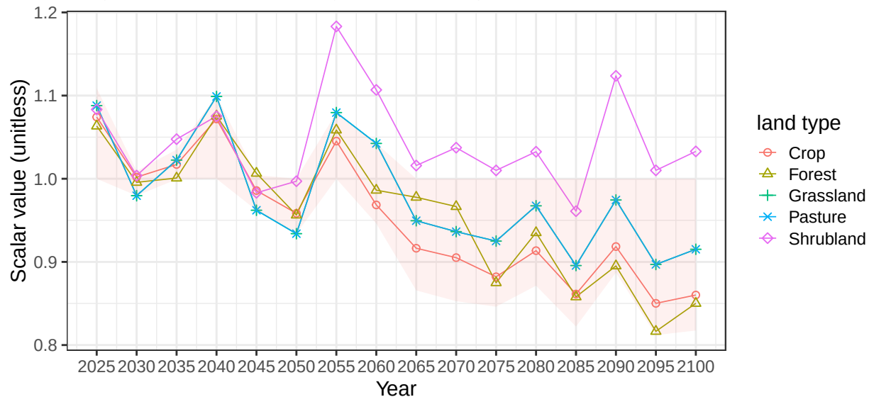
Region EU-15 basin ItalyCstW average soil scalars
