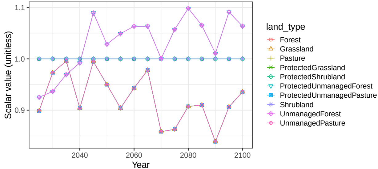
Region Mexico basin GrijUsuR non-crop vegetation scalars
