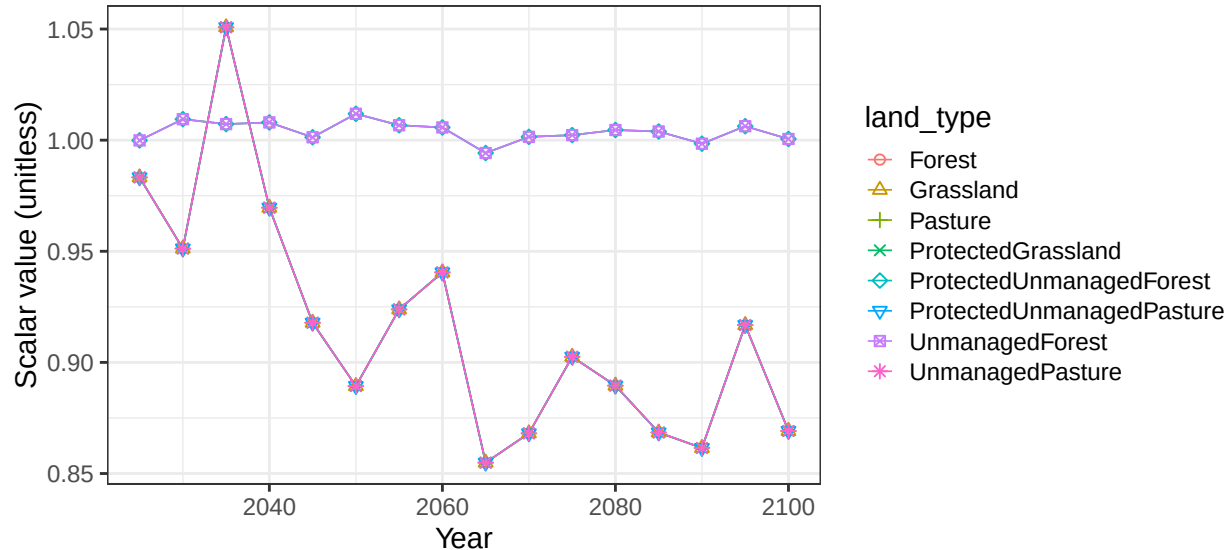
Region Indonesia basin Kalimantan non-crop soil scalars
