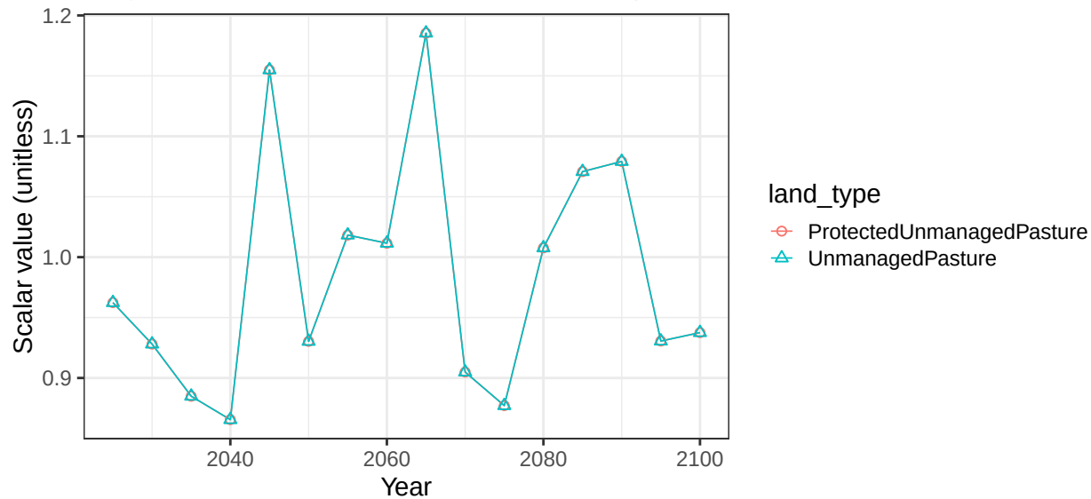
Region EU-15 basin AfrCstNW non-crop soil scalars
