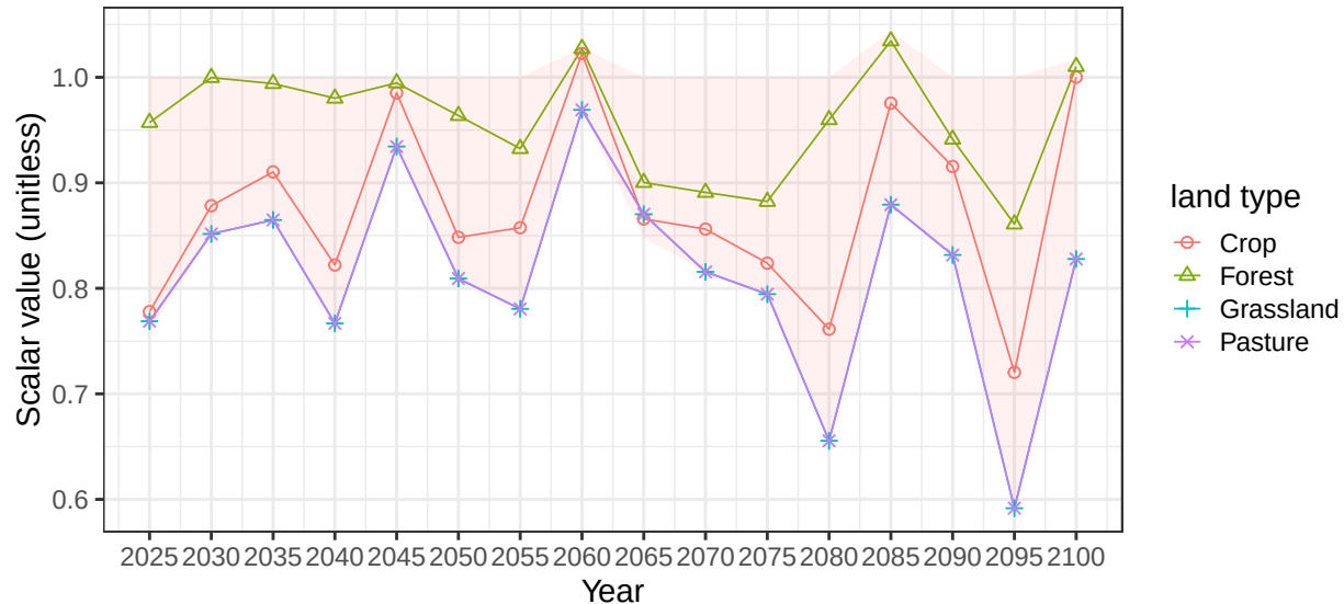
Region EU-12 basin NemanR average soil scalars
