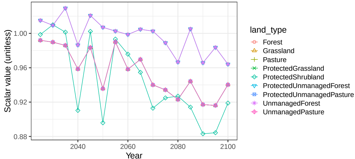
Region USA basin UsaCstSE non-crop soil scalars
