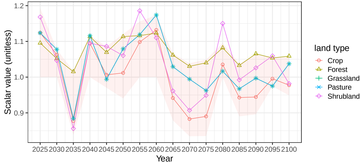
Region EU-15 basin EbroR average soil scalars
