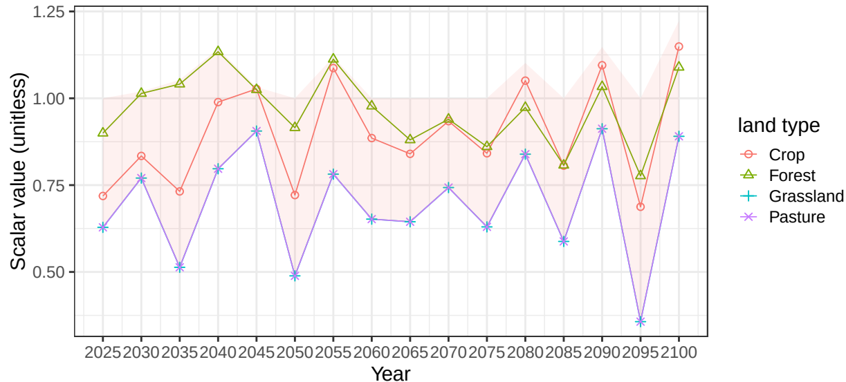
Region Europe_Eastern basin WislaR average vegetation scalars
