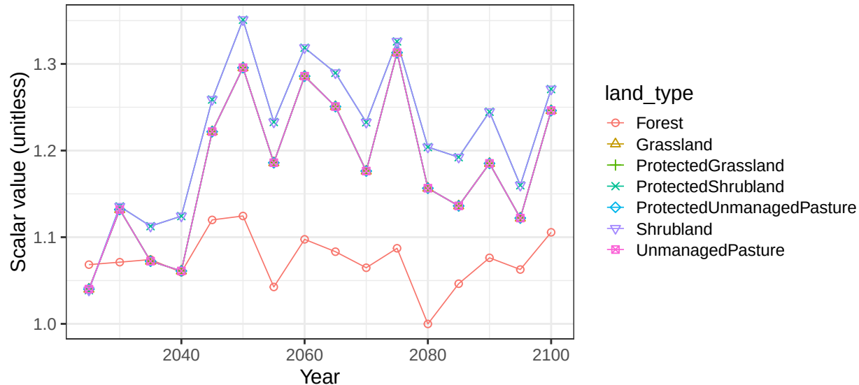
Region EU-15 basin Sweden non-crop soil scalars
