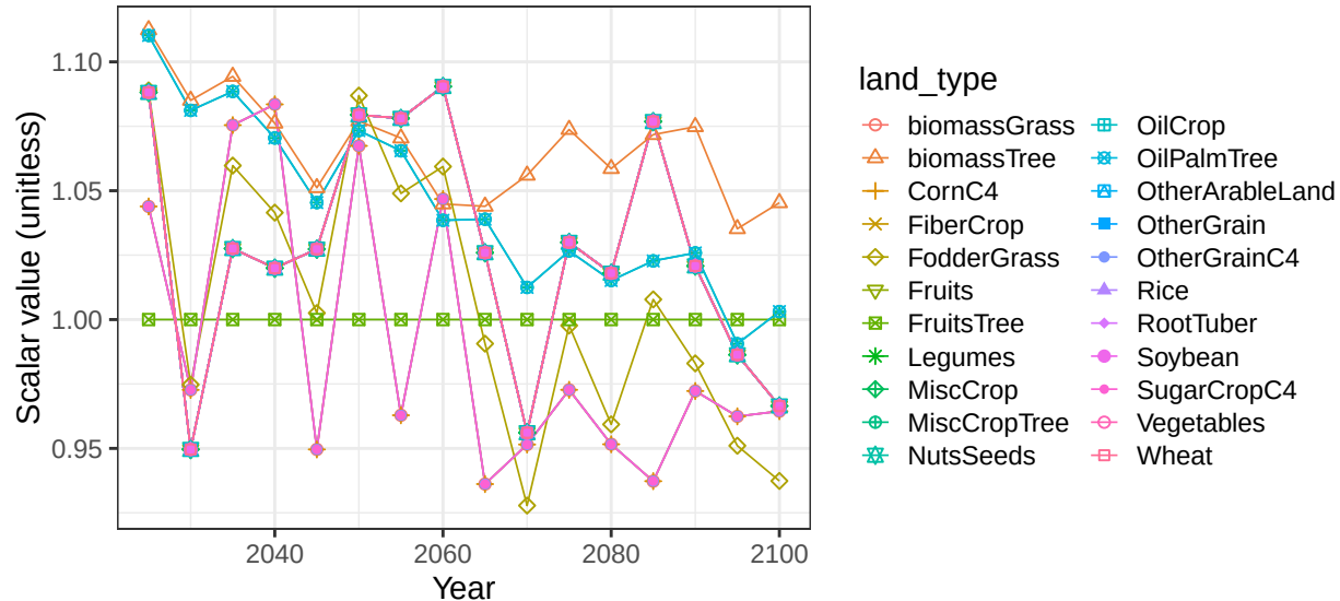
Region Africa_Eastern basin CongoR crop soil scalars
