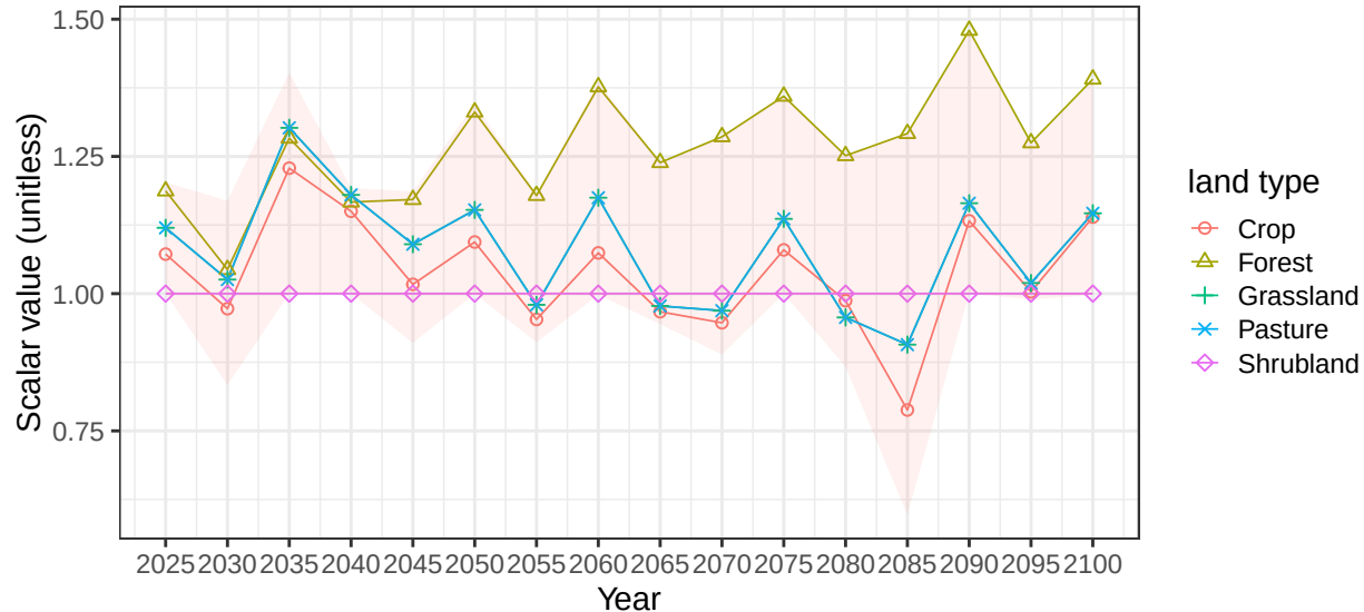
Region Africa_Southern basin RiftValley average vegetation scalars
