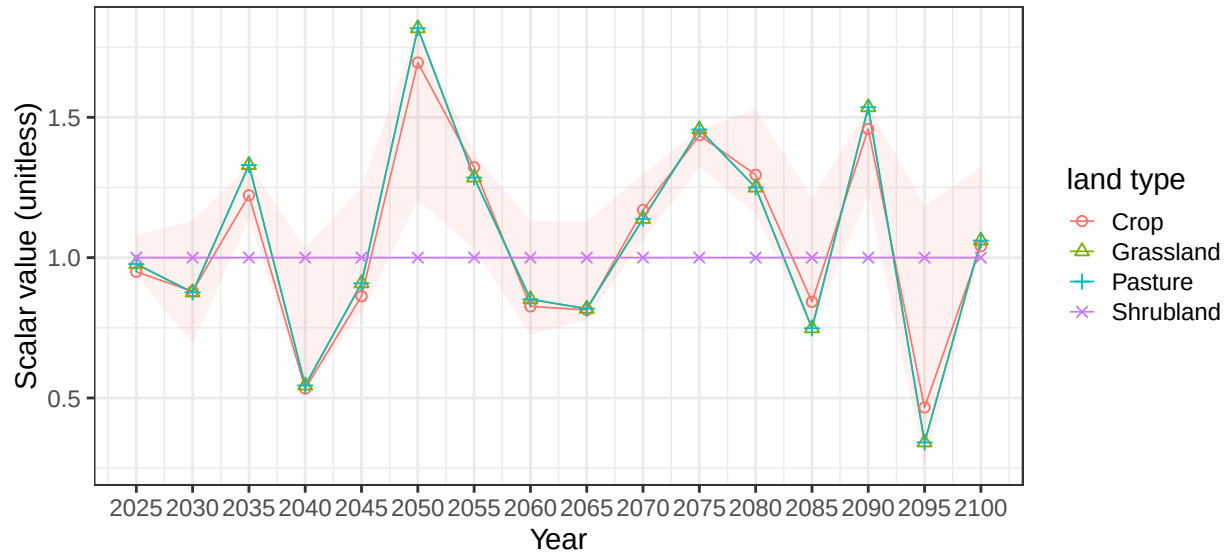
Region Russia basin SyrDaryaR average vegetation scalars
