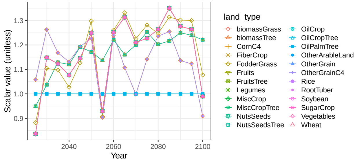
Region China basin AmurR crop vegetation scalars
