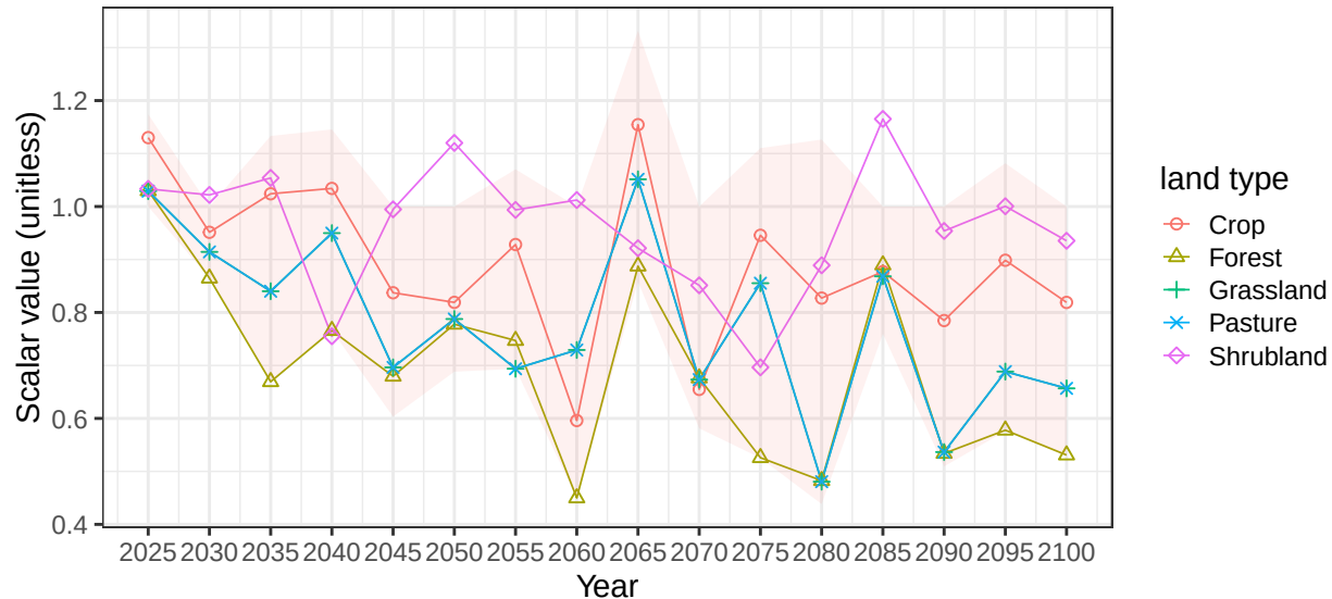
Region Argentina basin Pampas average soil scalars
