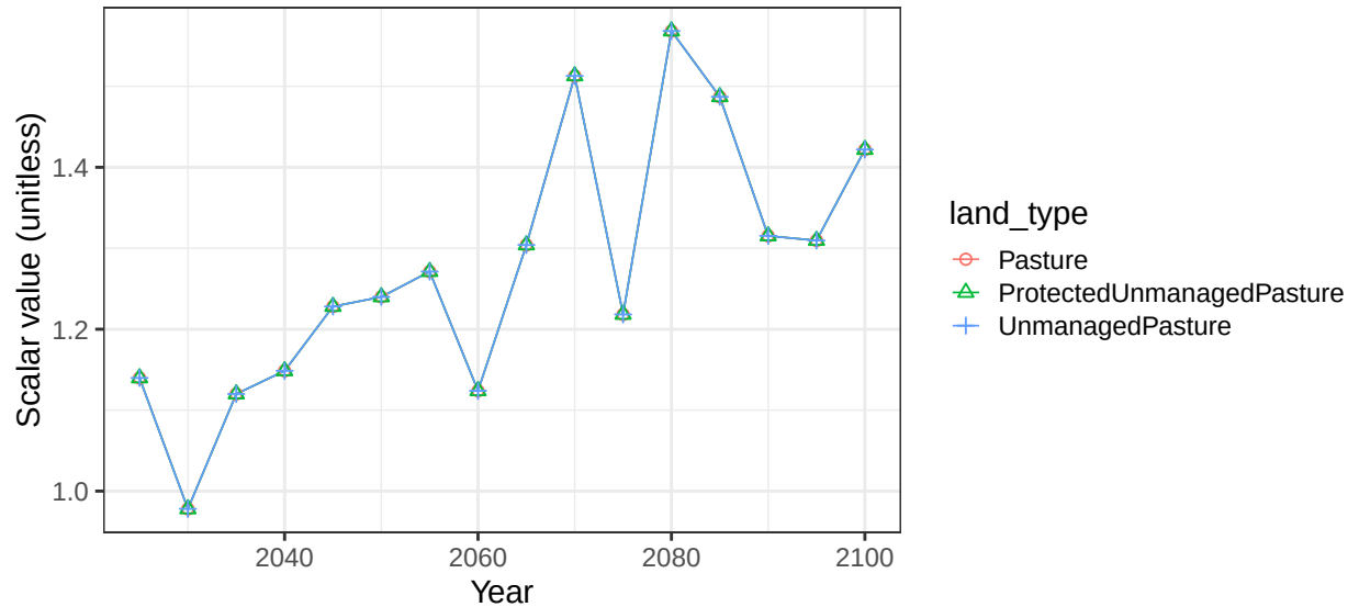
Region Pakistan basin Tarim non-crop vegetation scalars
