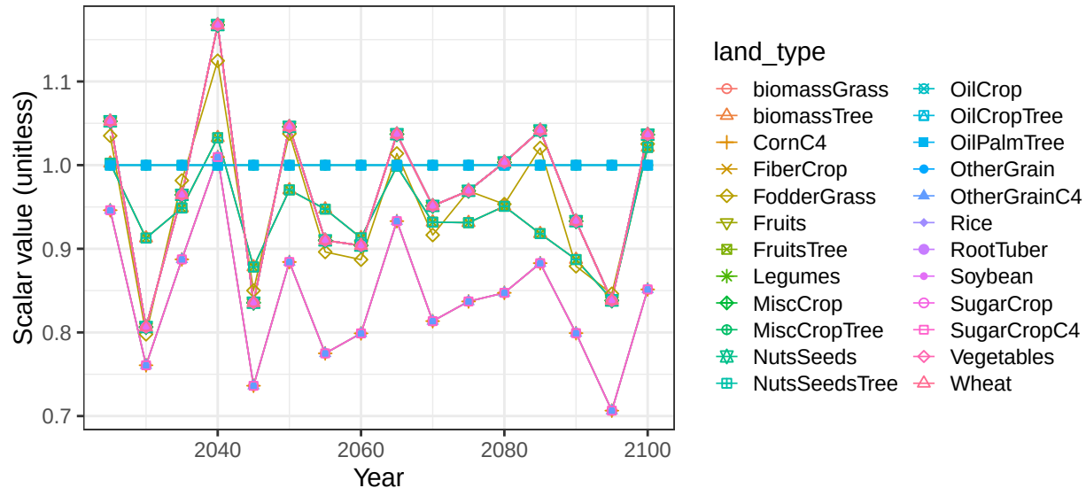
Region China basin ZiyaHe crop soil scalars
