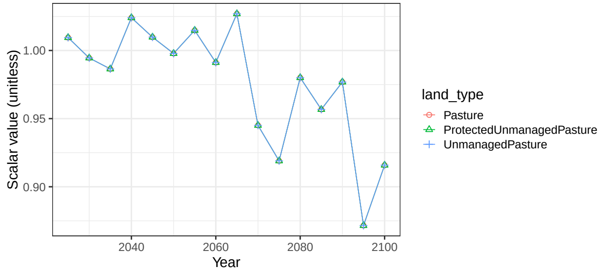
Region China basin AmuDaryaR non-crop soil scalars
