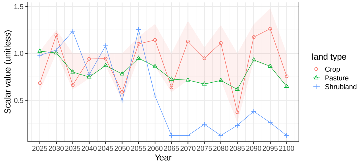
Region Pakistan basin SabarmatiR average vegetation scalars
