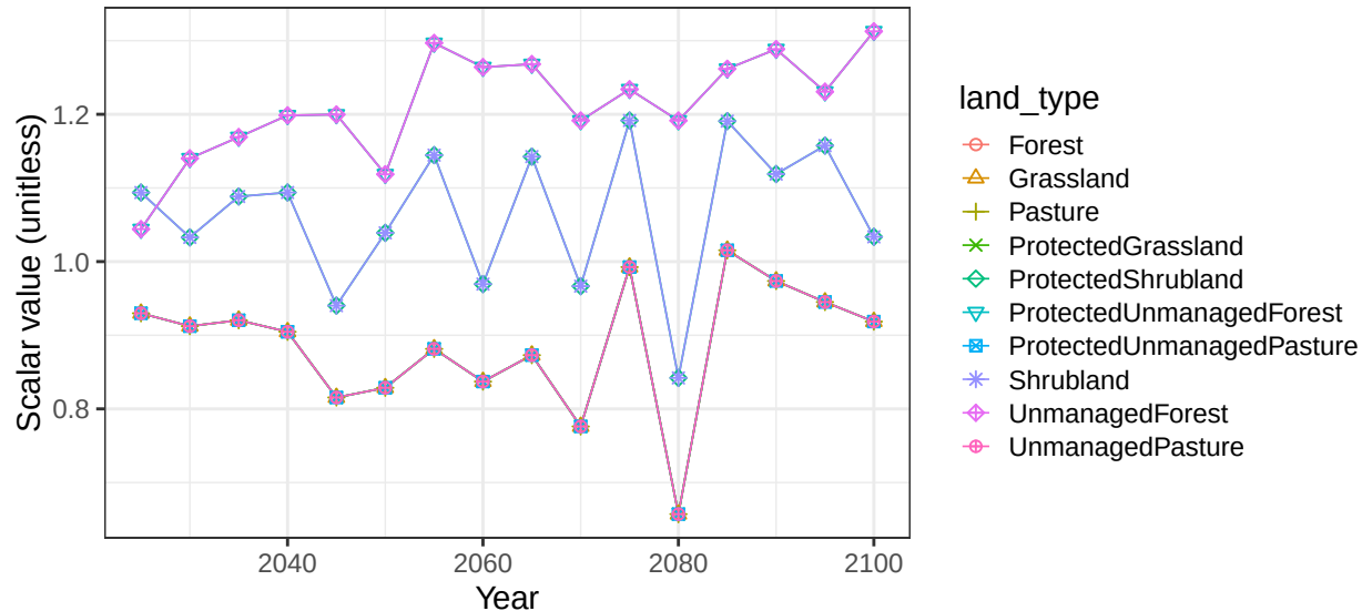
Region Mexico basin MexGulf non-crop vegetation scalars
