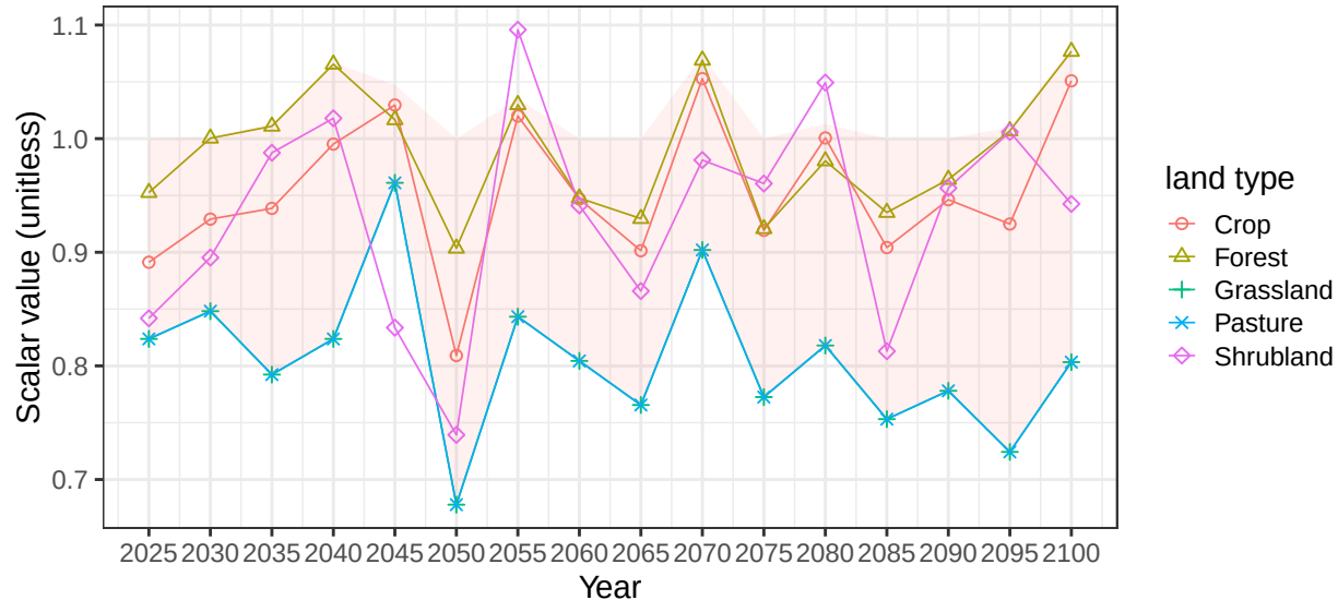
Region Europe_Eastern basin DnieperR average soil scalars
