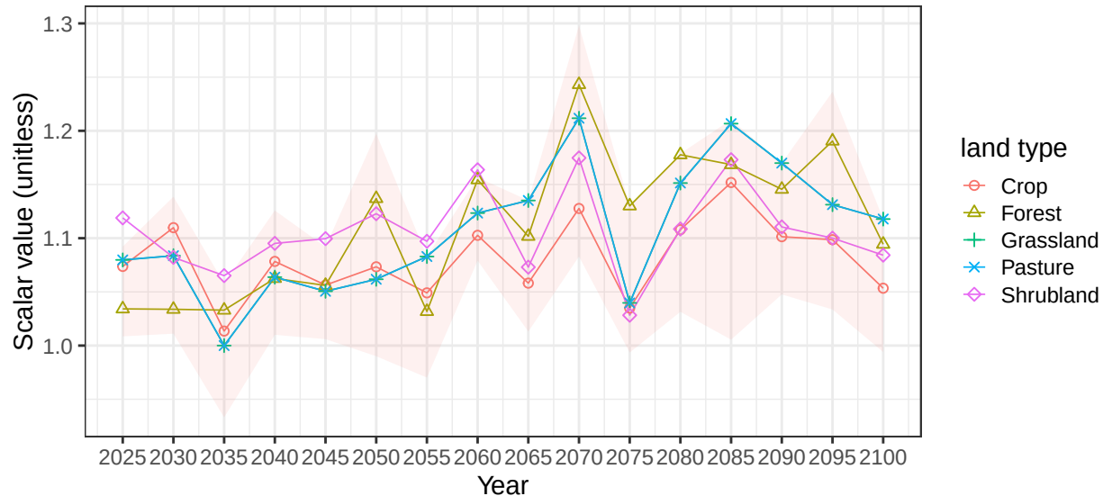
Region China basin Hong average vegetation scalars
