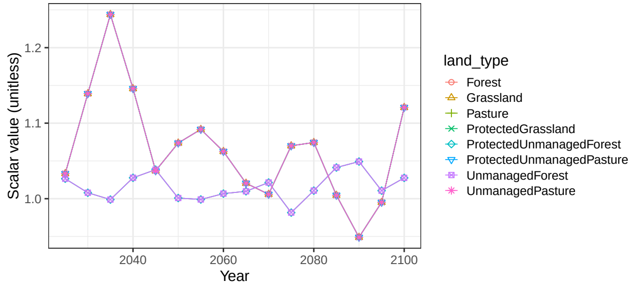
Region Indonesia basin BorneoCstN non-crop vegetation scalars
