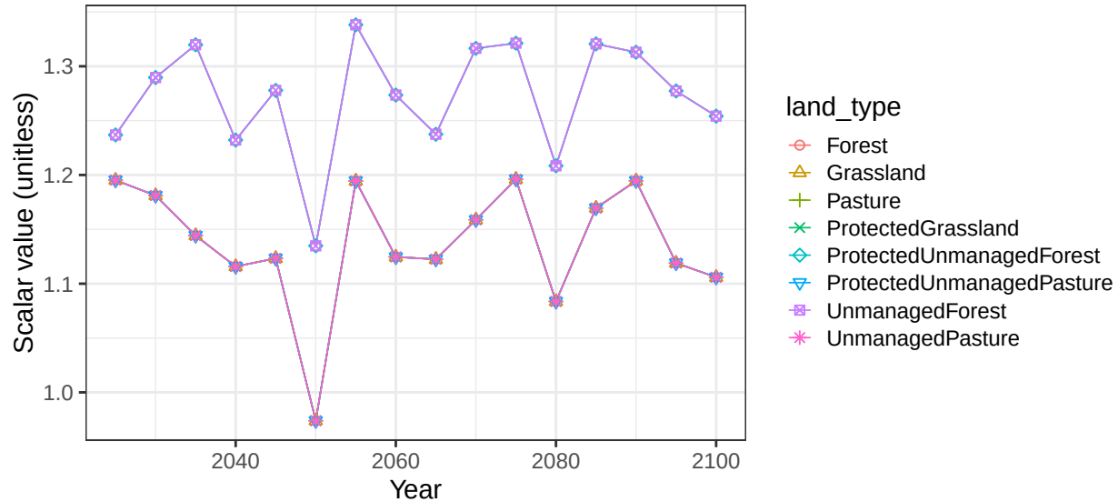
Region USA basin MisspppRS non-crop vegetation scalars
