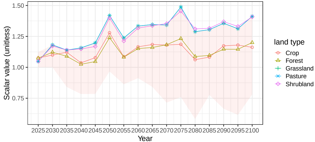
Region European Free Trade Association basin ScndnvN average vegetati
