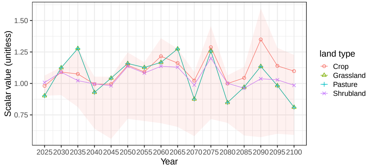
Region Middle East basin EJrdnSyr average vegetation scalars
