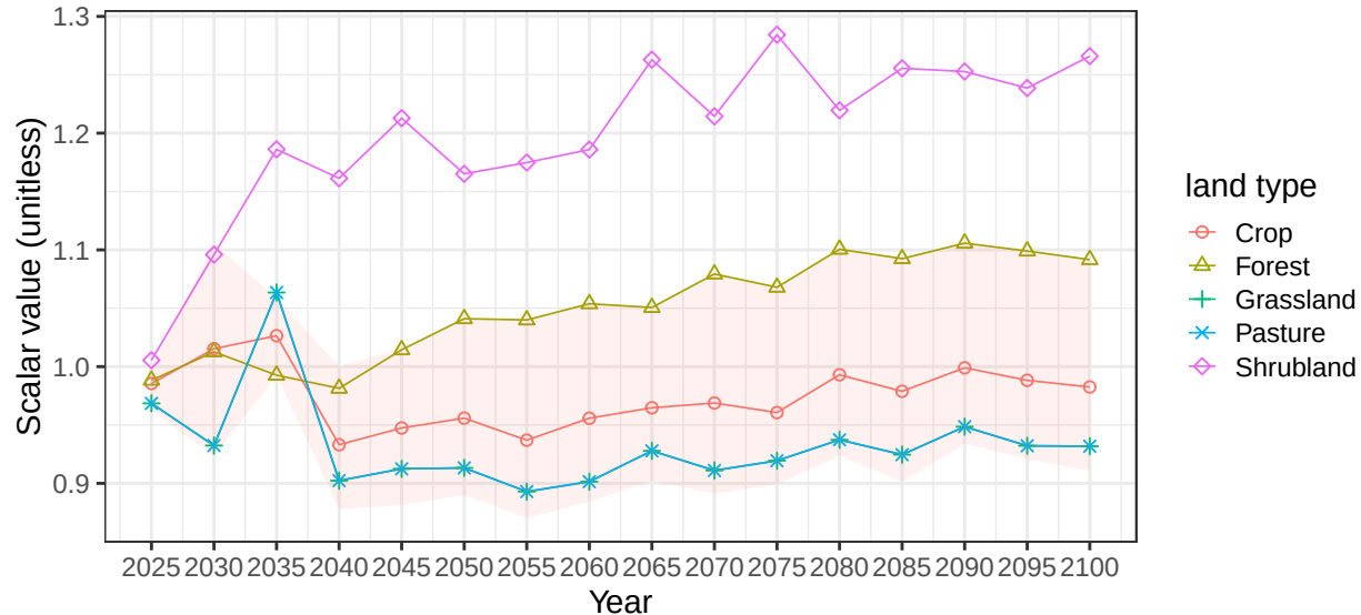
Region Colombia basin MagdalenaR average vegetation scalars
