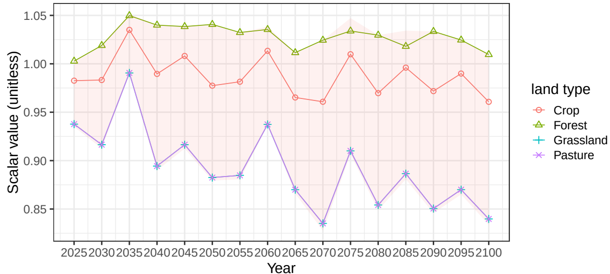
Region Indonesia basin Sulawesi average soil scalars
