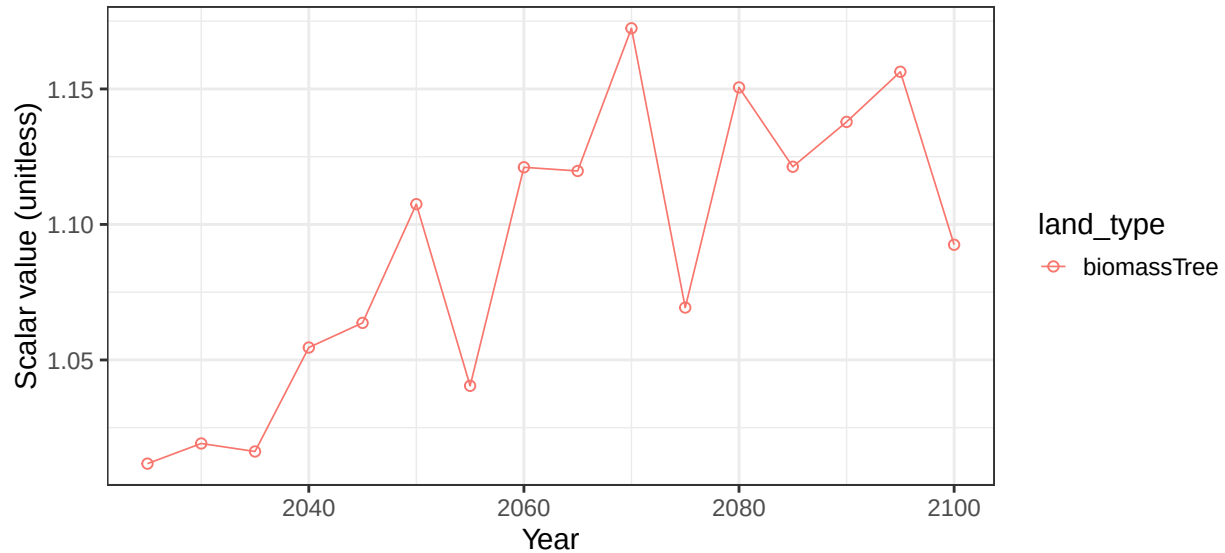
Region South America_Northern basin MagdalenaR crop vegetation scala
