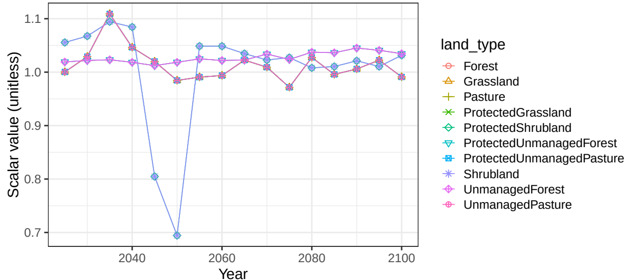
Region Colombia basin SAmerCstN non-crop soil scalars
