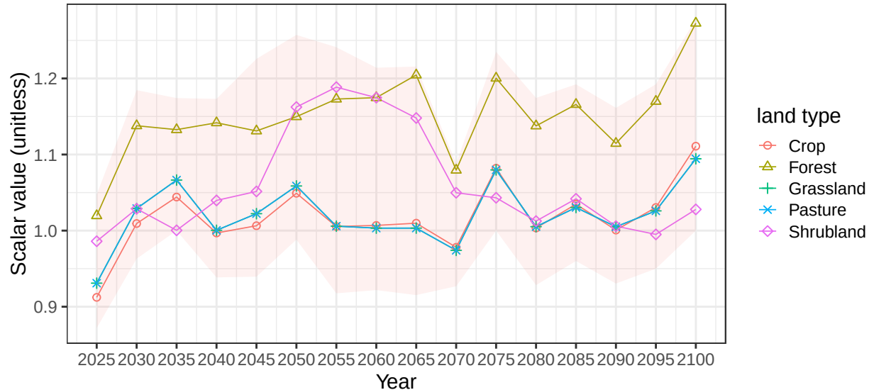
Region Mexico basin RioBalsas average vegetation scalars
