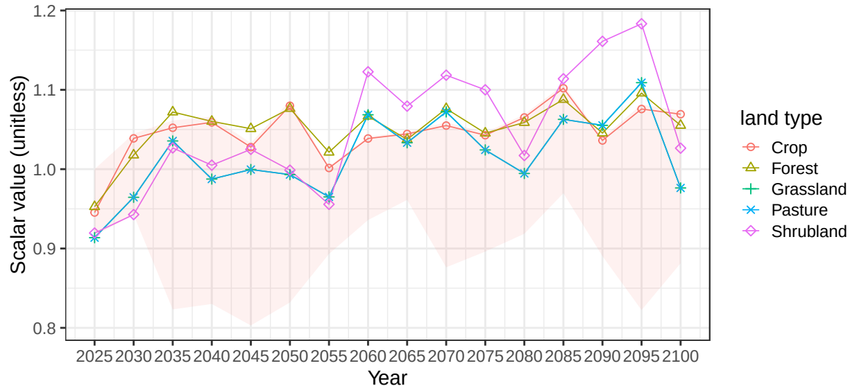
Region Canada basin CanAtl average vegetation scalars
