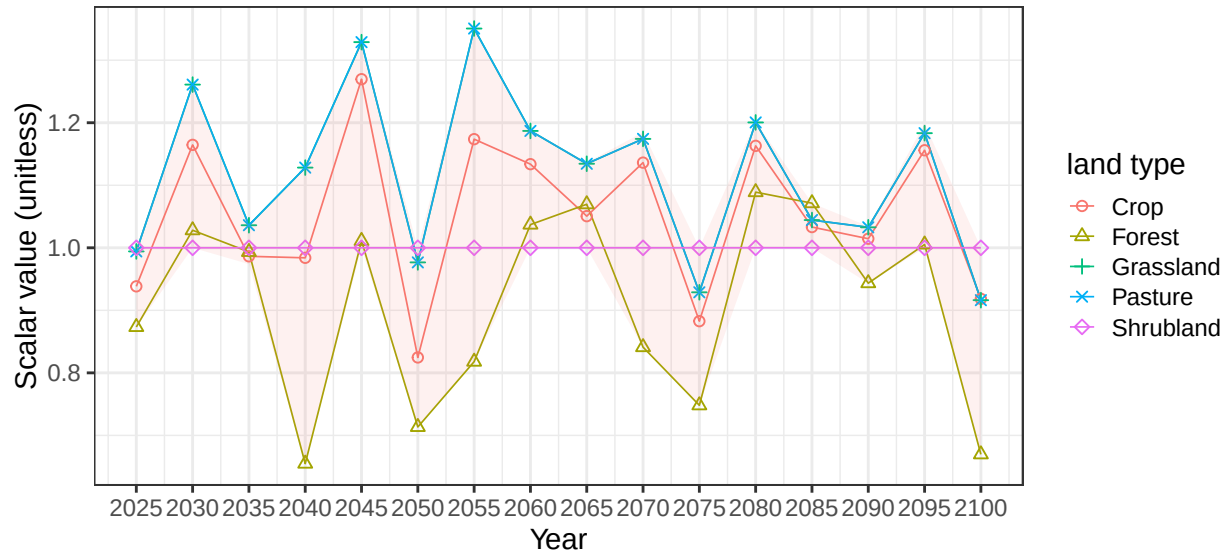
Region India basin PennarR average soil scalars
