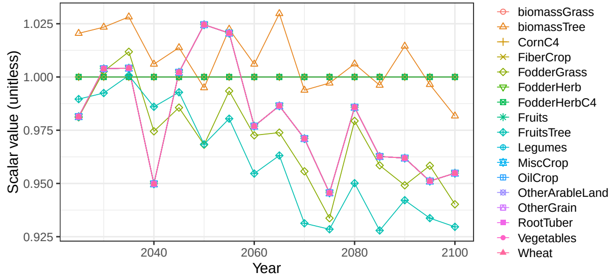
Region Australia_NZ basin NewZealand crop soil scalars land_type
