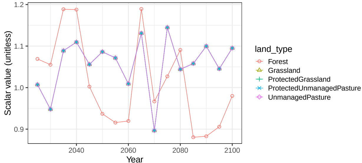
Region EU-15 basin ScheldtR non-crop soil scalars
