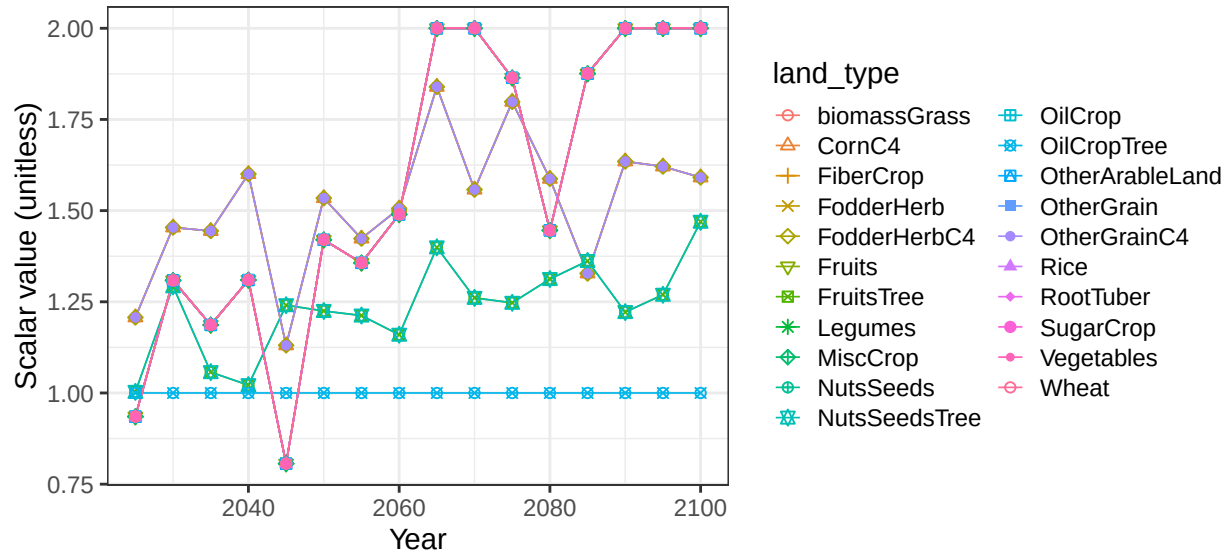
Region Central Asia basin CaspianE crop vegetation scalars
