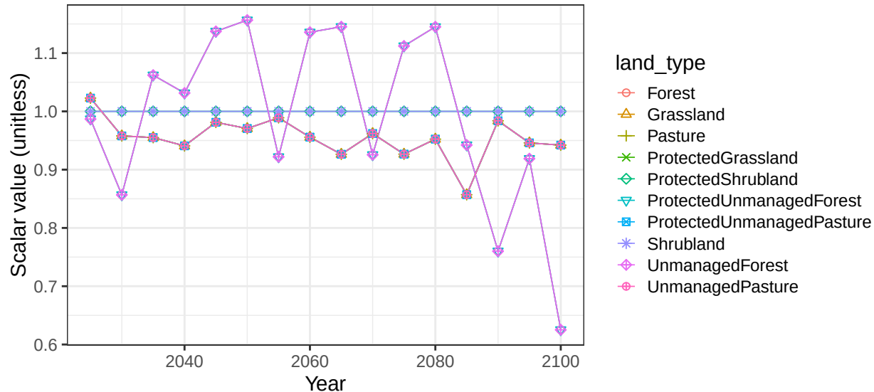
Region Africa_Western basin VoltaR non-crop soil scalars
