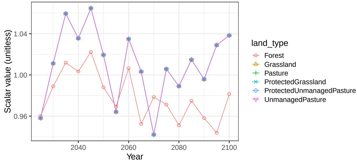
Region China basin RusCstSE non-crop soil scalars
