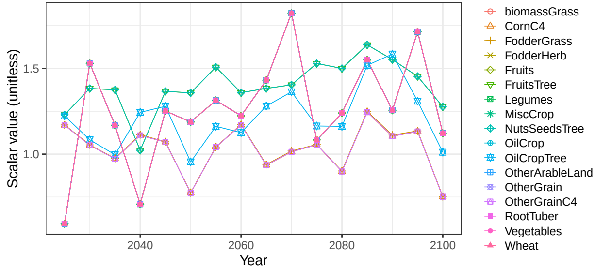
Region Australia_NZ basin AusInt crop vegetation scalars land_type
