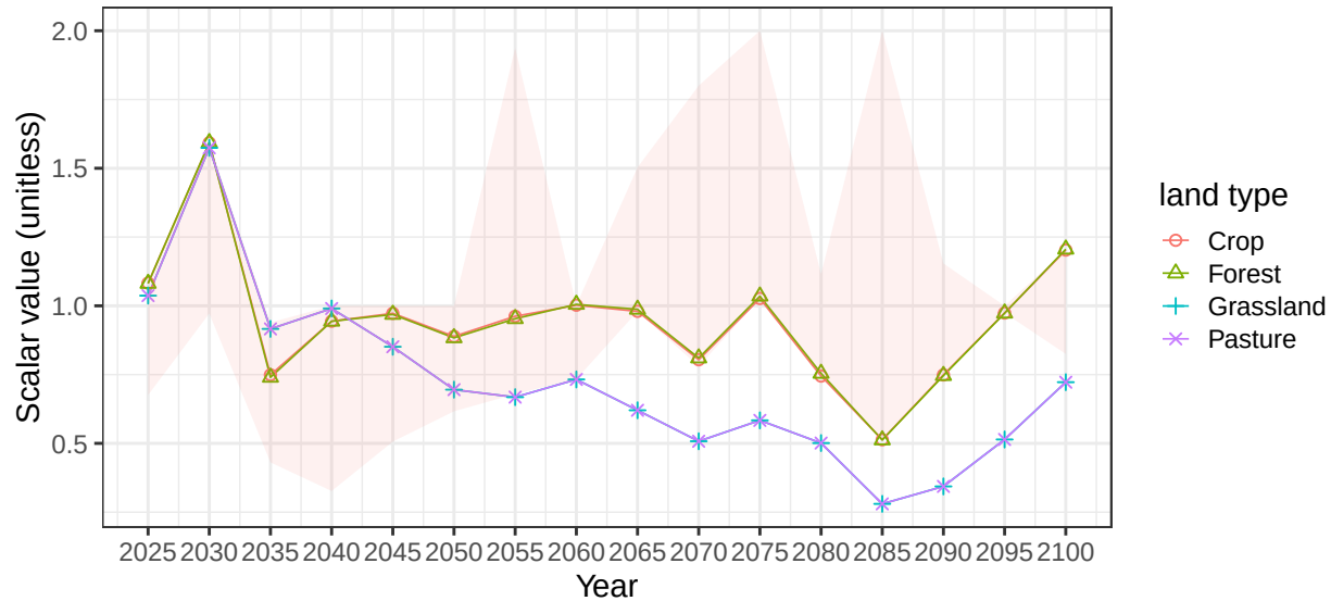
Region Central Asia basin BlackSeaN average vegetation scalars
