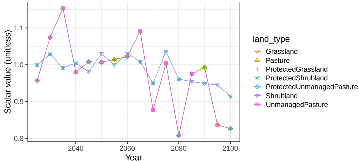
Region Middle East basin EJrdnSyr non-crop soil scalars
