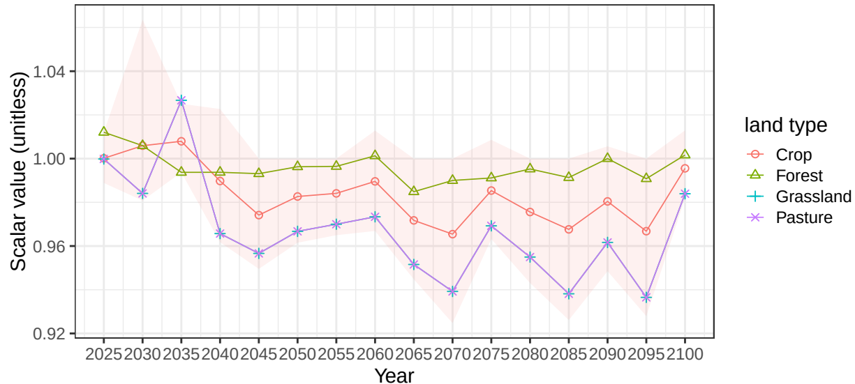
Region Colombia basin AmazonR average soil scalars
