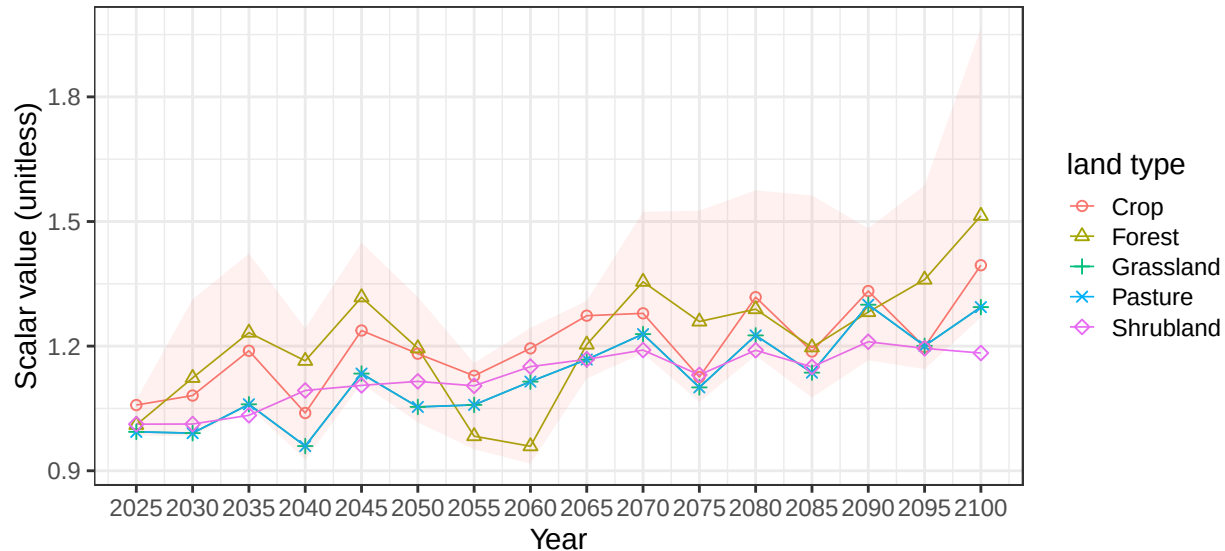
Region South Asia basin GangesR average vegetation scalars
