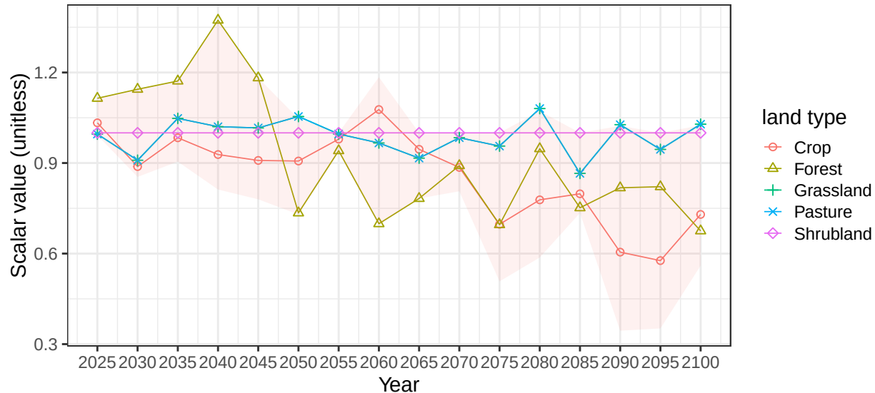
Region Africa_Western basin LChad average vegetation scalars
