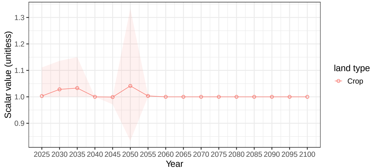
Region Africa_Northern basin SinaiP average soil scalars
