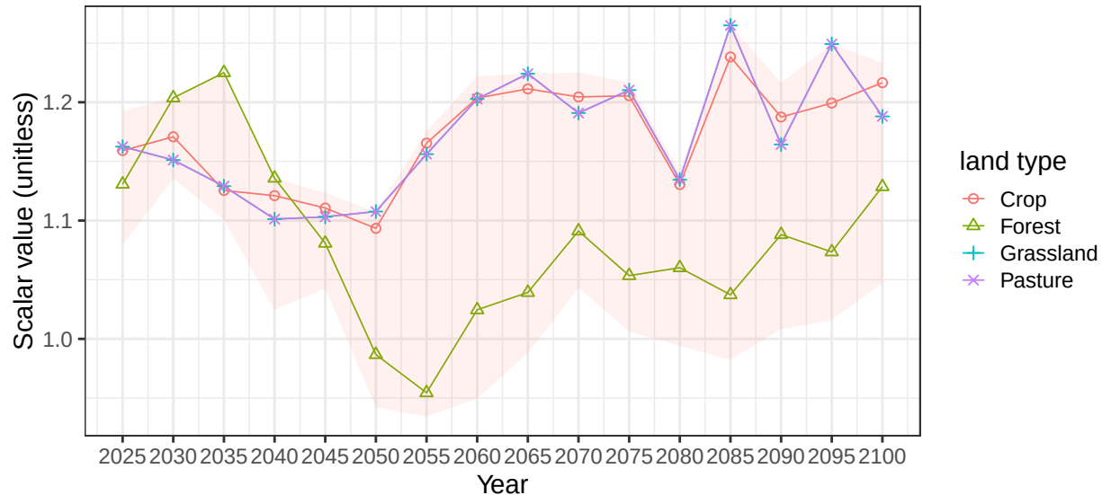
Region India basin IrrawaddyR average soil scalars
