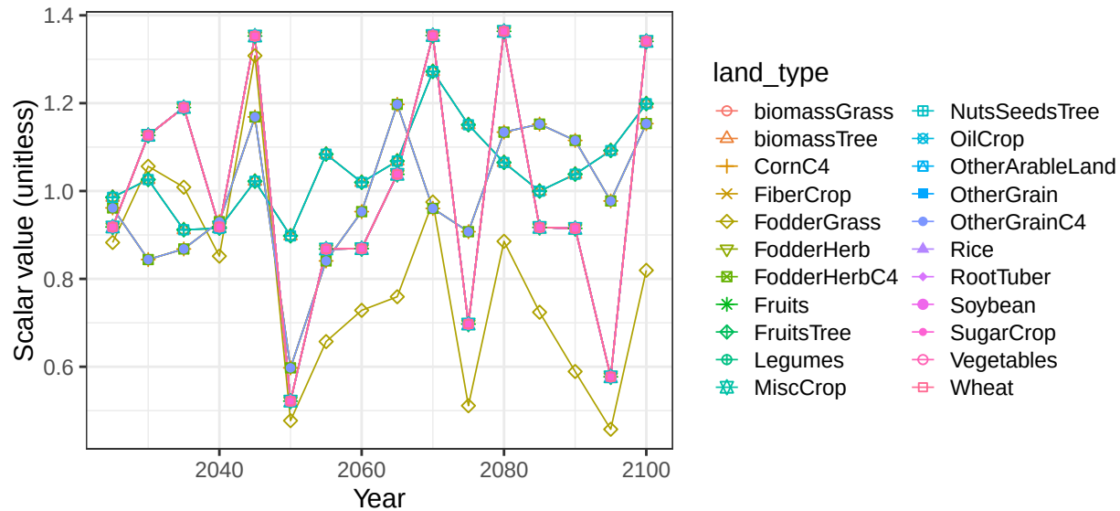
Region Russia basin DonR crop vegetation scalars
