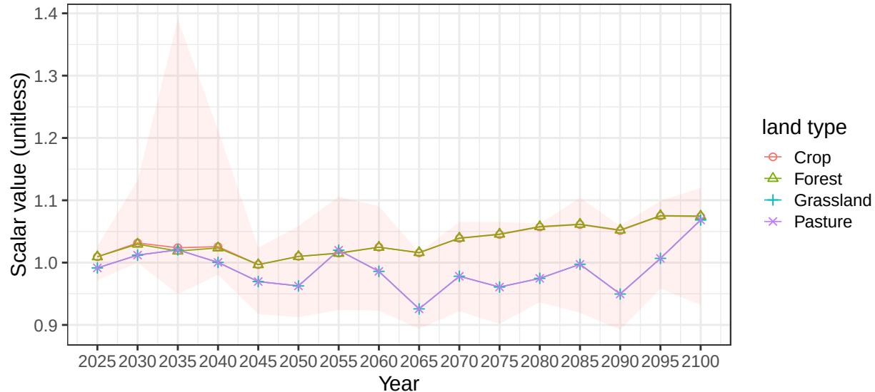
Region Indonesia basin SepikR average vegetation scalars
