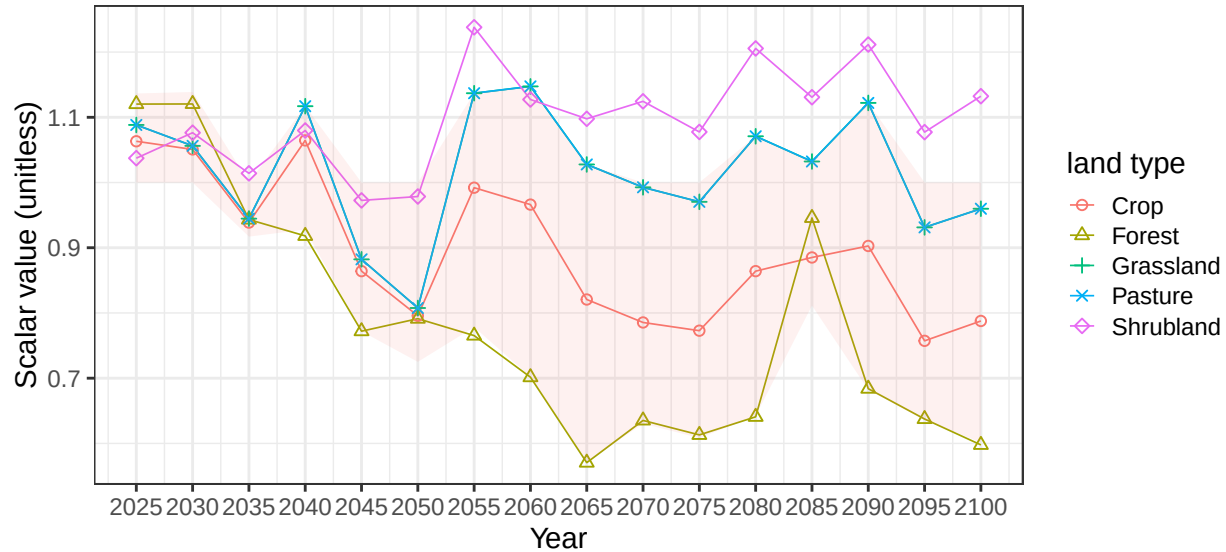
Region EU-15 basin ItalyCstE average vegetation scalars
