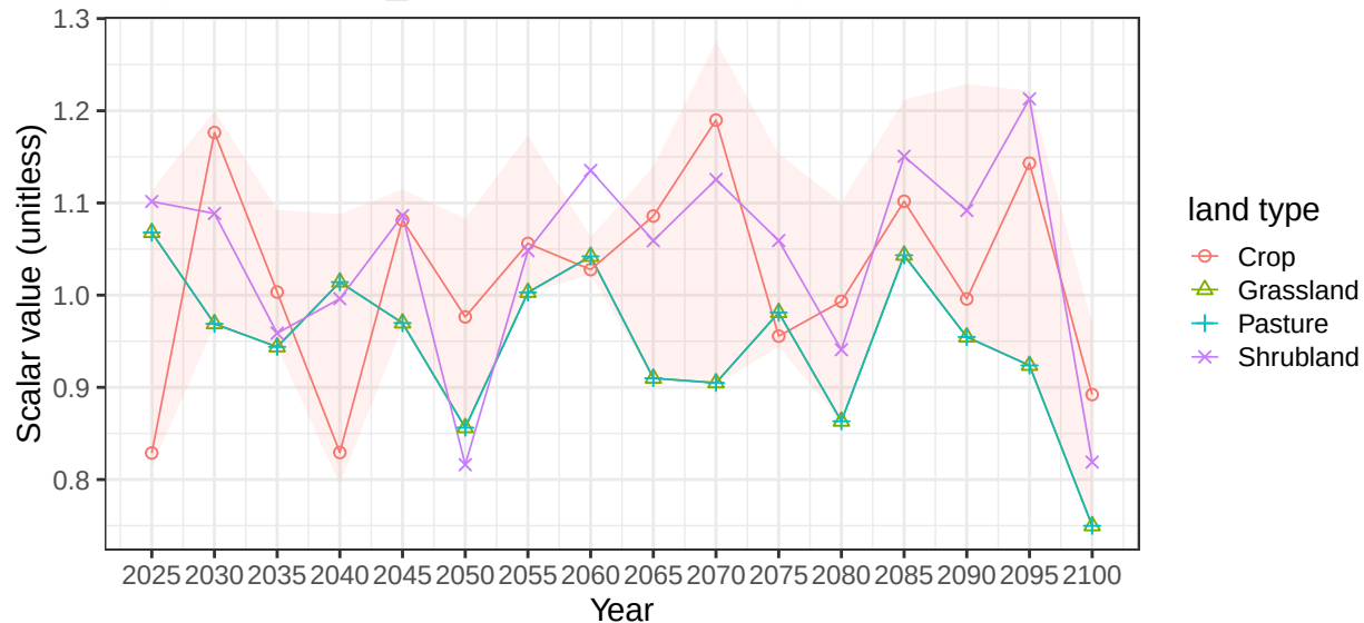
Region Australia_NZ basin AusInt average soil scalars
