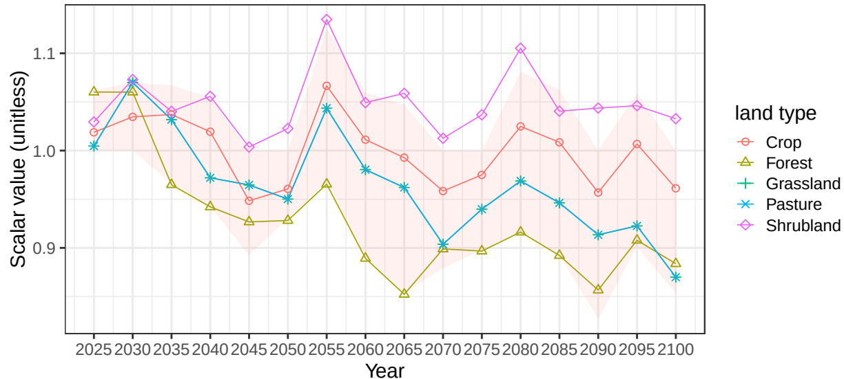
Region EU-15 basin AdrBlkSea average soil scalars
