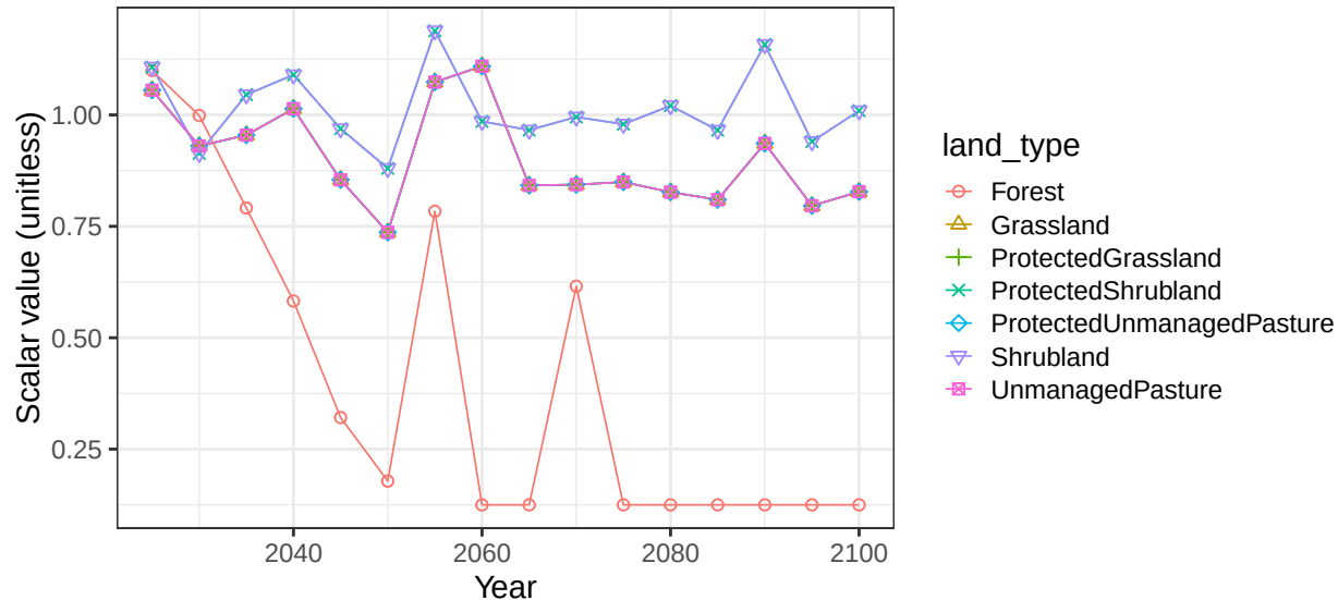
Region EU-15 basin TiberR non-crop vegetation scalars
