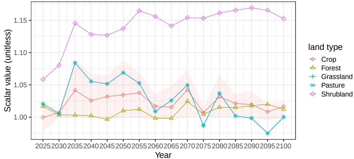
Region Colombia basin OrinocoR average soil scalars
