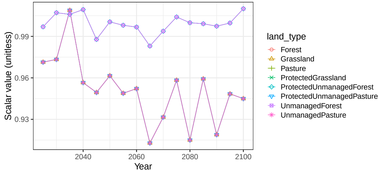
Region Indonesia basin IrianJaya non-crop soil scalars
