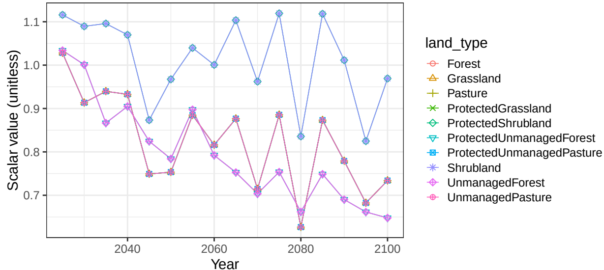
Region USA basin RioGrande non-crop soil scalars
