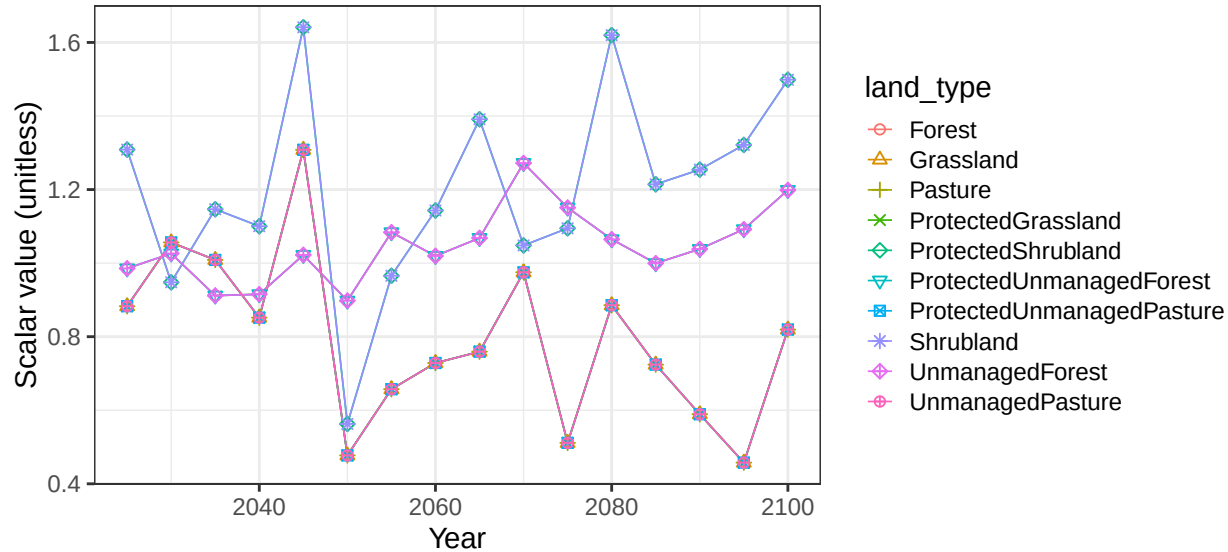
Region Russia basin DonR non-crop vegetation scalars
