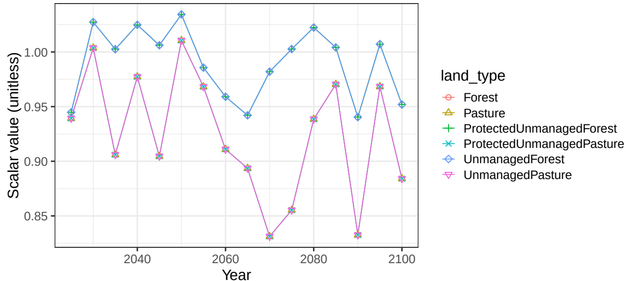
Region Taiwan basin ChinaCst non-crop soil scalars
