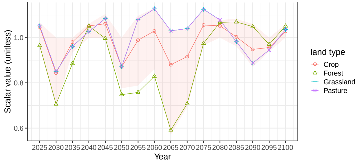
Region EU-12 basin ElbeR average vegetation scalars
