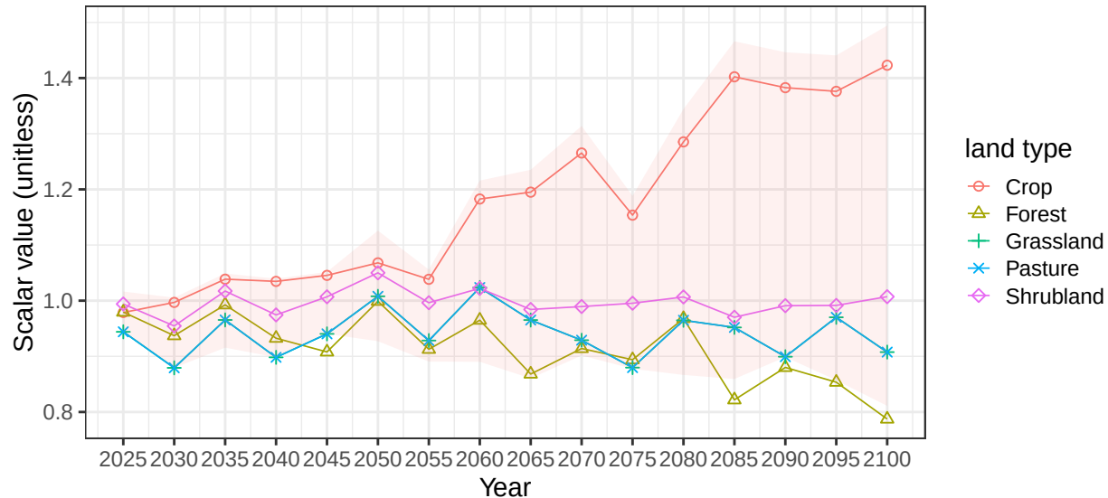
Region Central Asia basin Gobi average soil scalars
