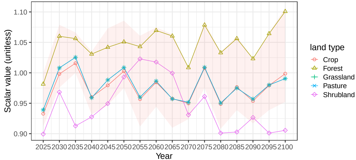
Region Mexico basin RioBalsas average soil scalars
