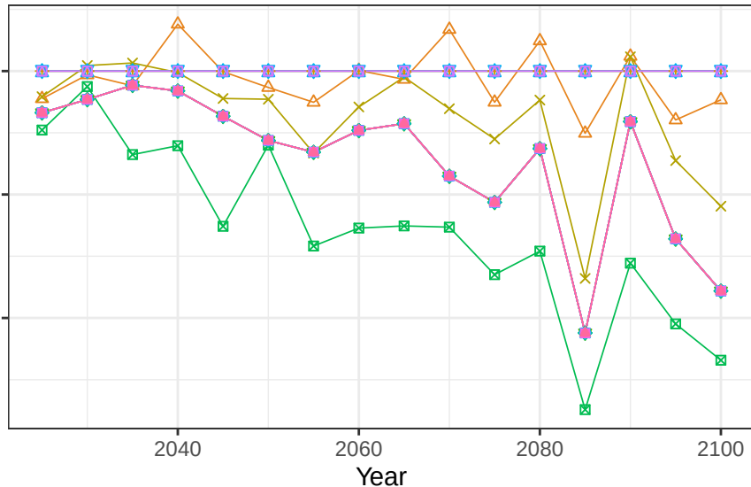
Region Australia_NZ basin Tasmania crop soil scalars
