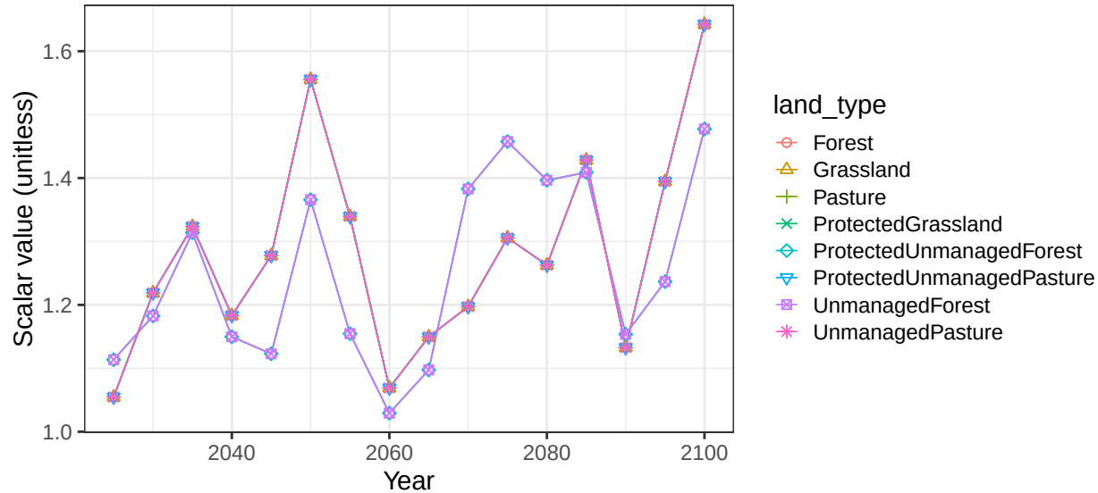
Region USA basin FraserR non-crop vegetation scalars
