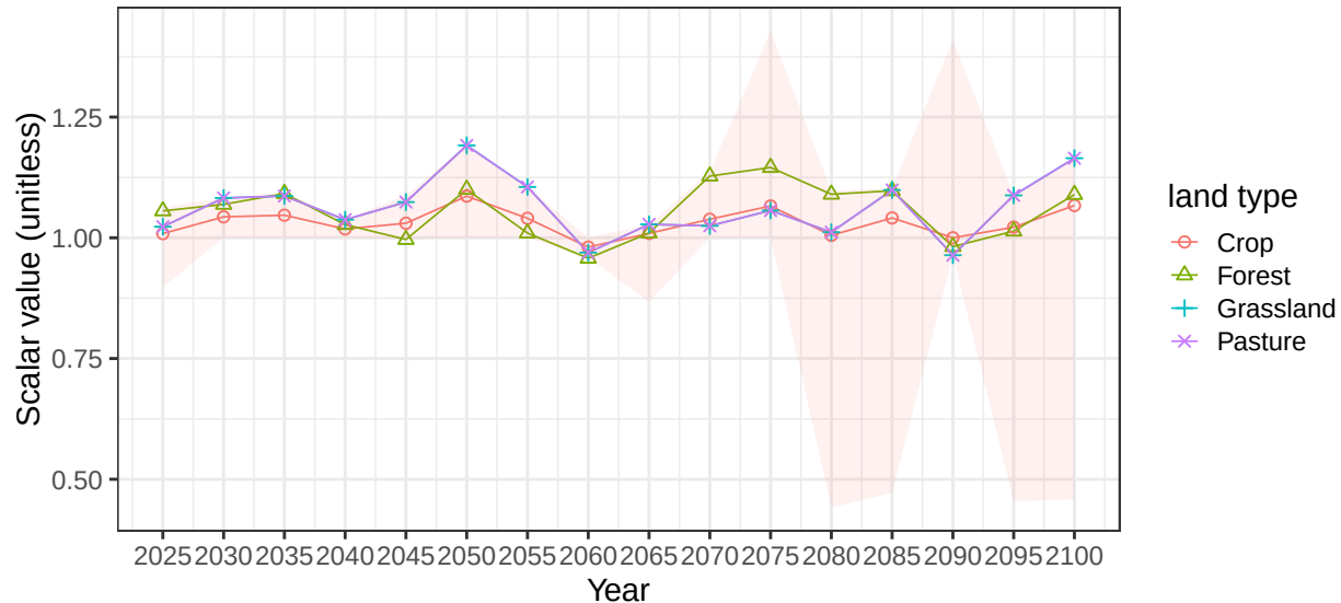
Region USA basin FraserR average soil scalars
