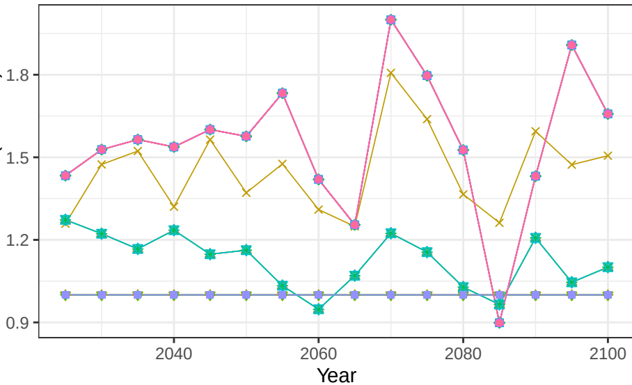
Region USA basin NelsonR crop vegetation scalars
