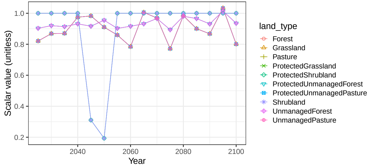
Region South America_Northern basin OrinocoR non-crop vegetation scalar
