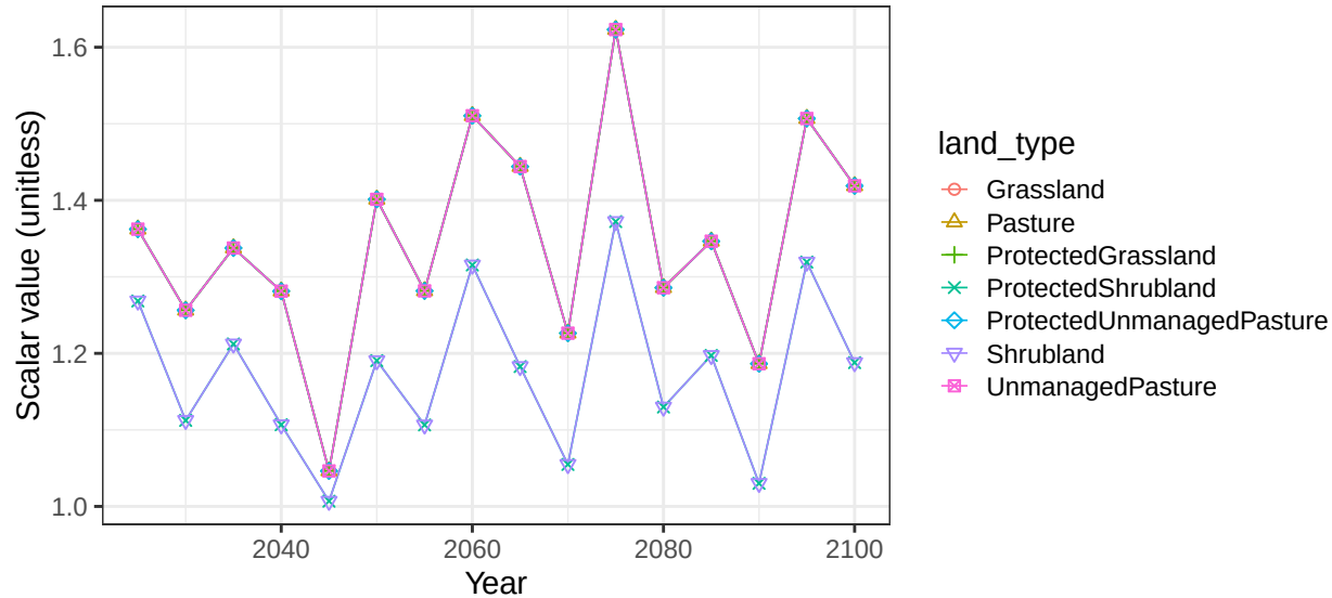
Region Middle East basin PersianGulf non-crop vegetation scalars
