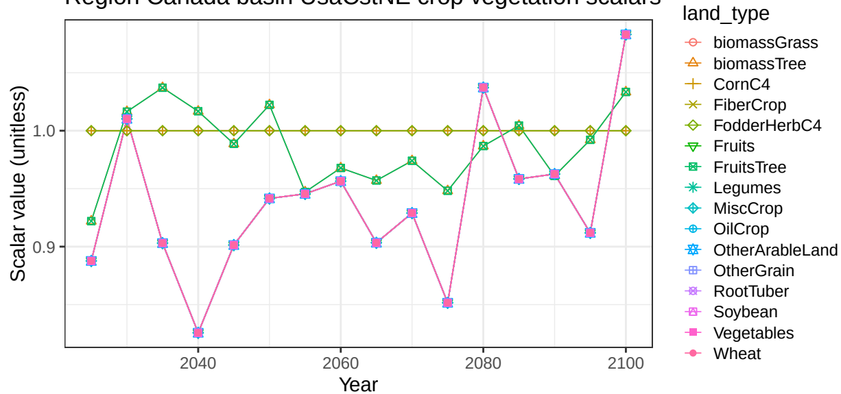
Region Canada basin UsaCstNE crop vegetation scalars
