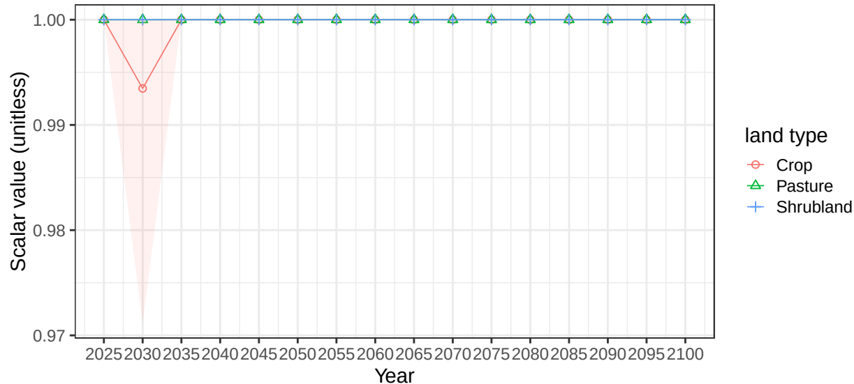
Region Middle East basin AfrCstNE average vegetation scalars
