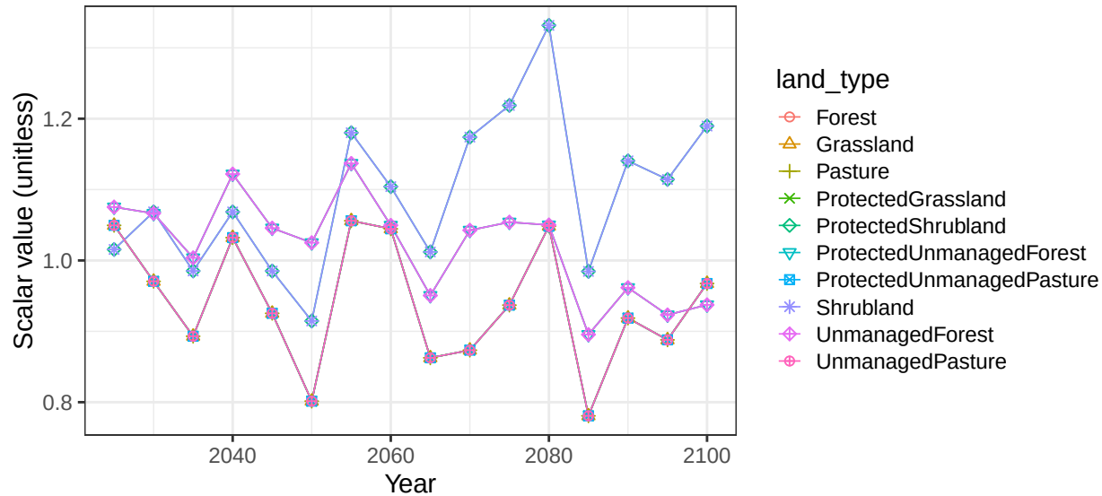
Region EU-12 basin DanubeR non-crop soil scalars
