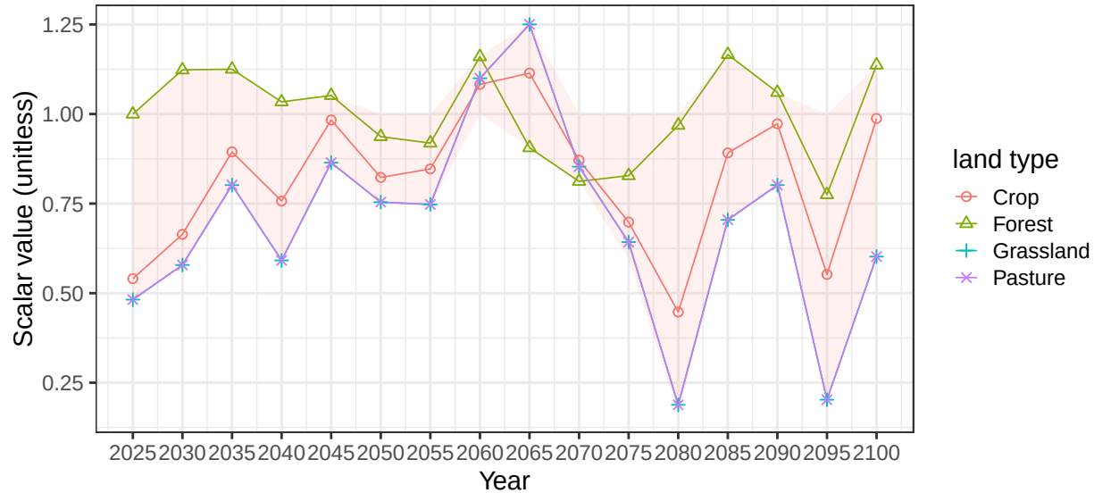
Region Russia basin NemanR average vegetation scalars
