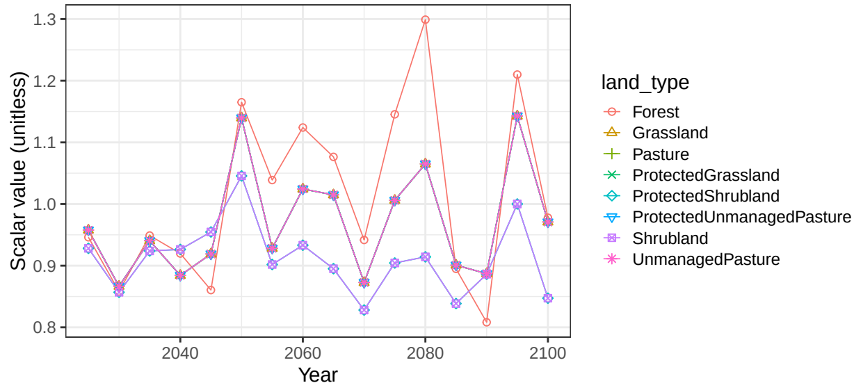
Region China basin LBalkash non-crop soil scalars
