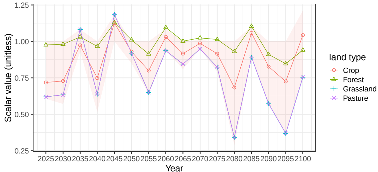
Region EU-12 basin BalticSea average vegetation scalars
