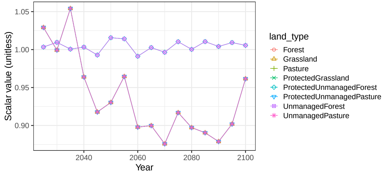
Region Southeast Asia basin BorneoCstN non-crop soil scalars
