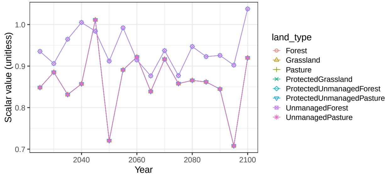
Region Europe_Eastern basin NemanR non-crop soil scalars
