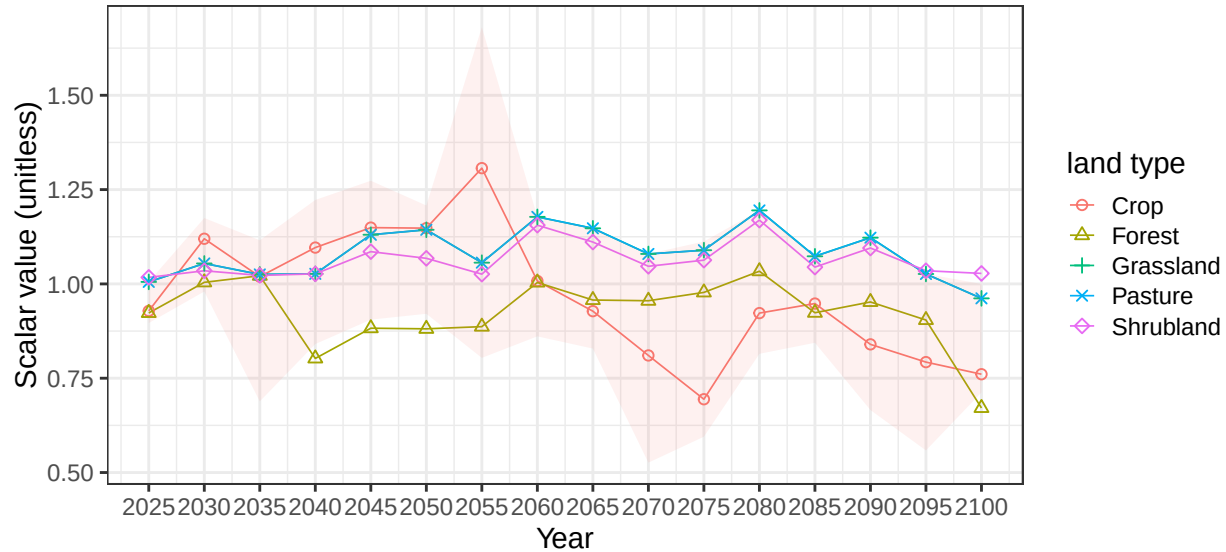
Region China basin ObR average soil scalars
