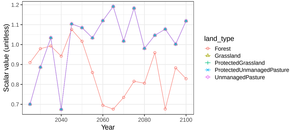
Region EU-15 basin DnkGrmCst non-crop vegetation scalars
