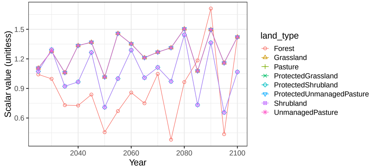
Region India basin MahiR non-crop vegetation scalars
