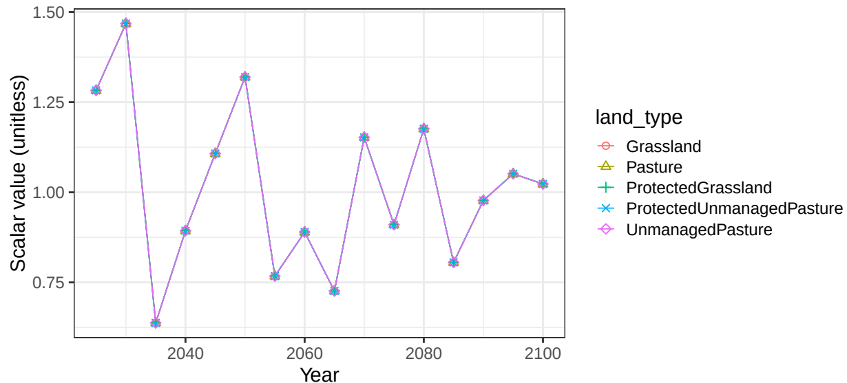
Region USA basin Hawaii non-crop vegetation scalars
