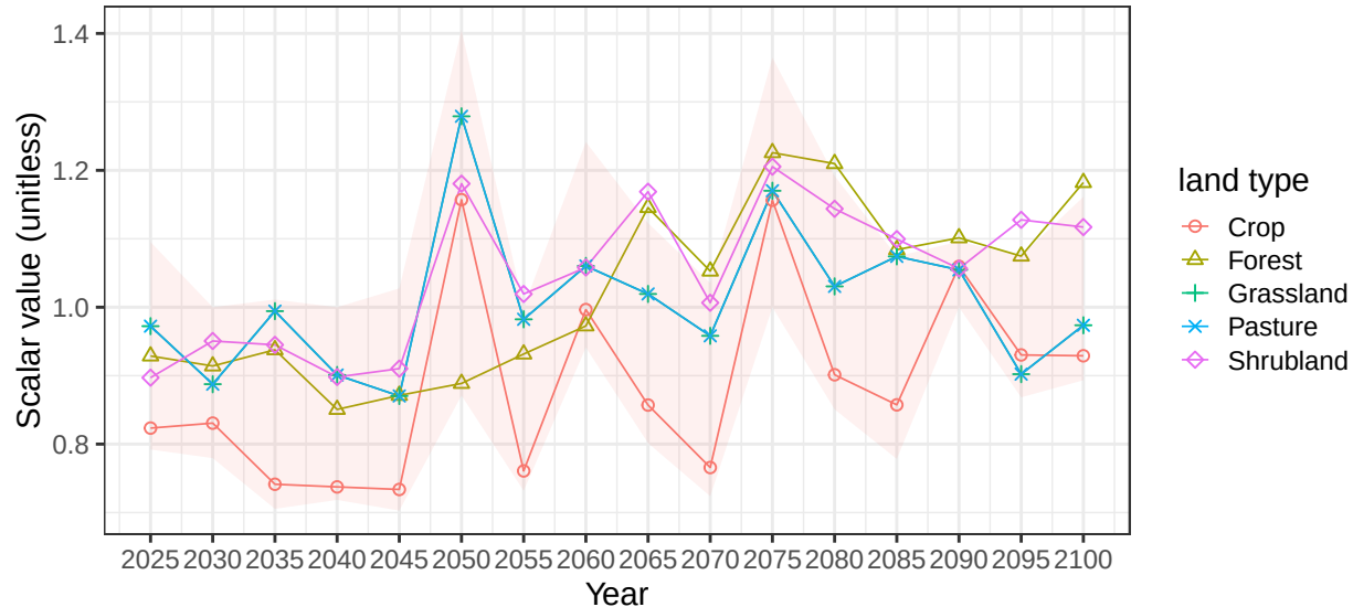
Region Central Asia basin SyrDaryaR average vegetation scalars
