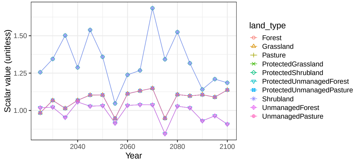
Region Southeast Asia basin Salween non-crop vegetation scalars
