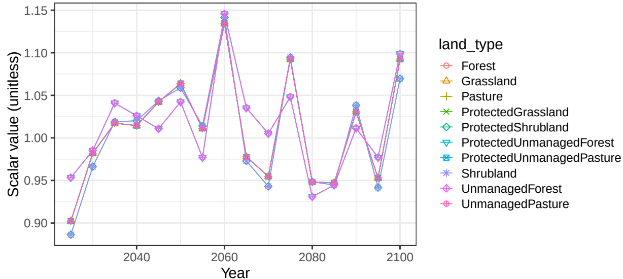
Region Russia basin ScndnvN non-crop soil scalars
