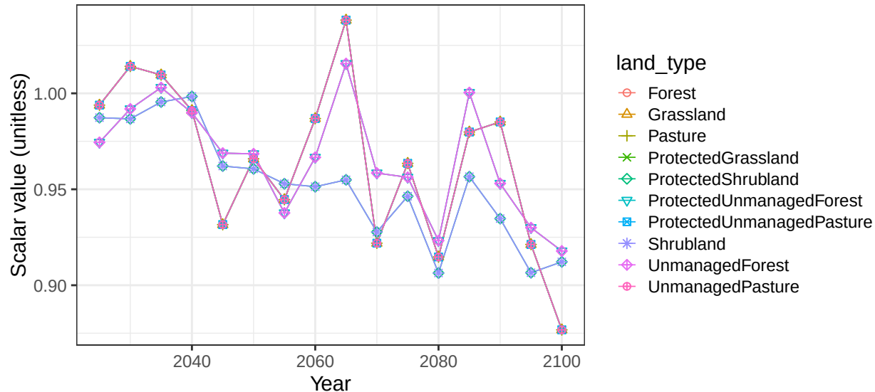
Region South America_Southern basin RioLaPlata non-crop soil scalars
