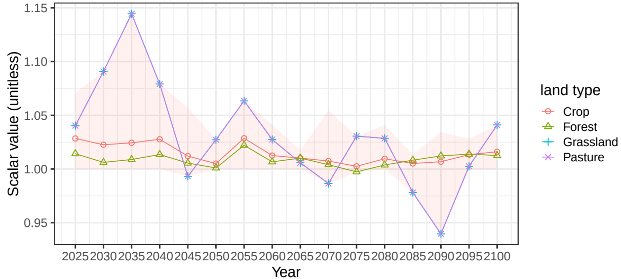
Region Indonesia basin BorneoCstN average soil scalars
