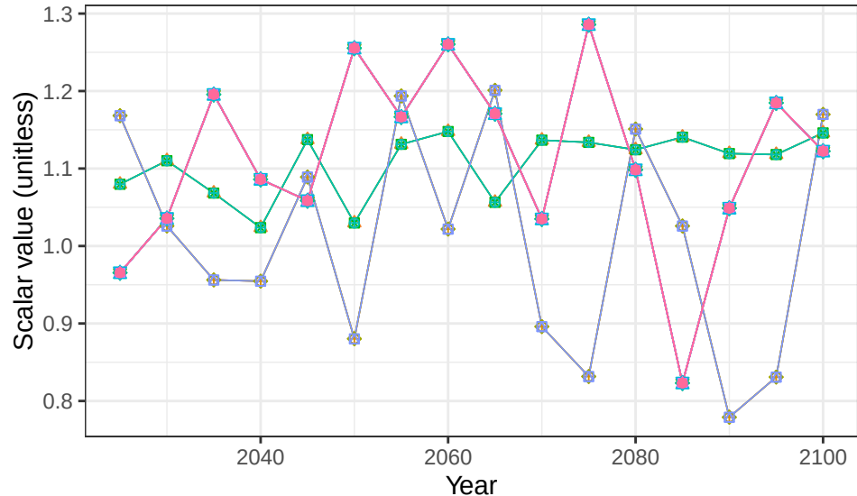
Region Central Asia basin VolgaR crop soil scalars
