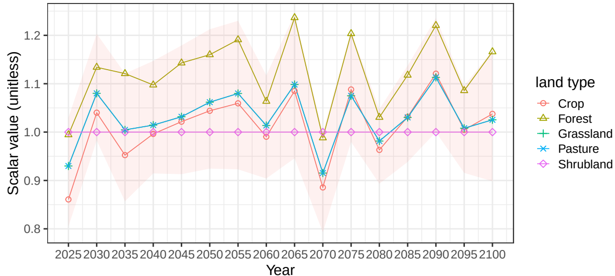
Region Mexico basin RioLerma average vegetation scalars
