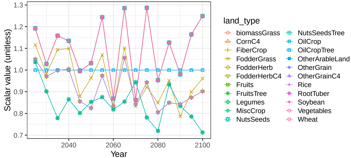
Region Argentina basin ArgCstN crop soil scalars
