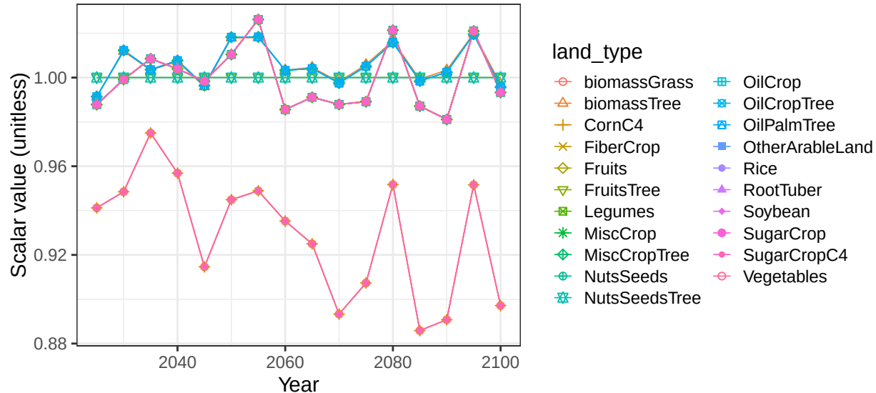
Region Indonesia basin Sumatra crop soil scalars
