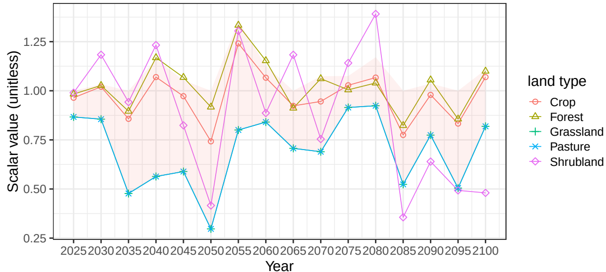
Region Europe_Eastern basin DanubeR average vegetation scalars
