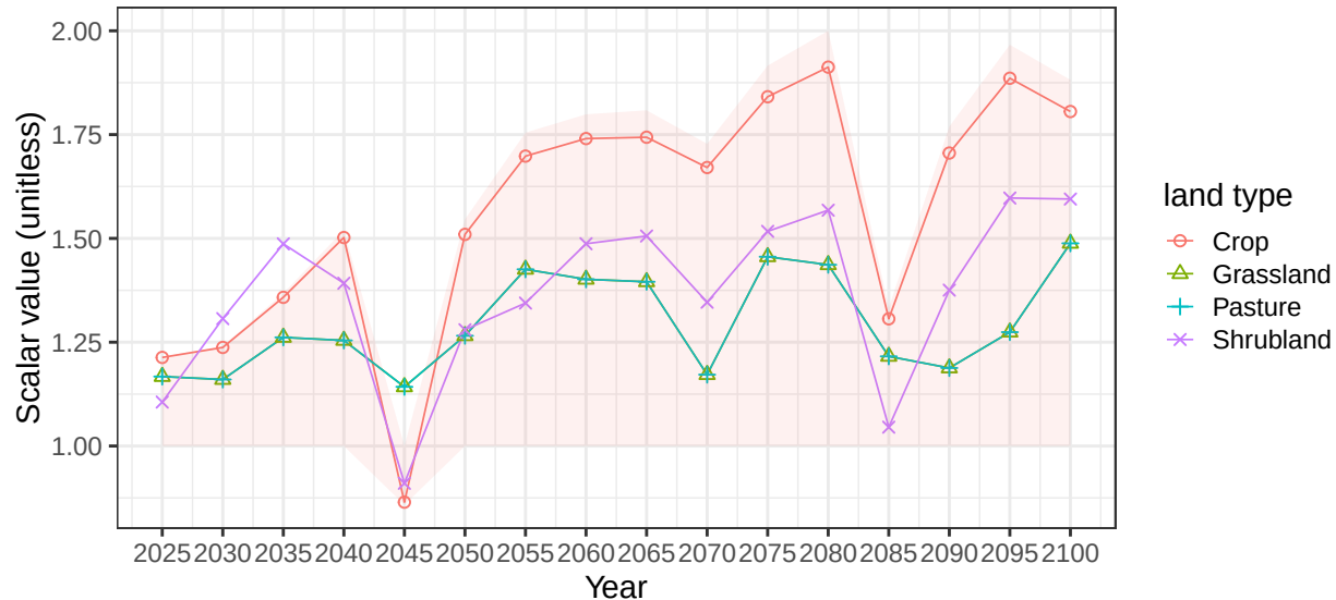
Region South Asia basin CaspianE average vegetation scalars
