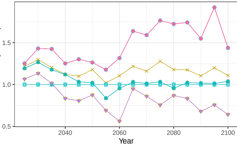
Region USA basin GreatBasin crop vegetation scalars
