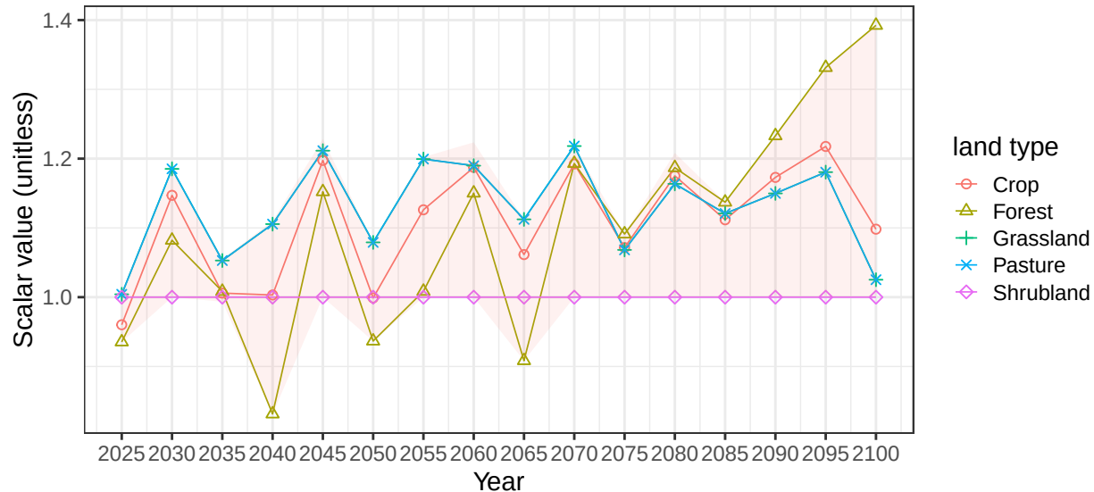
Region India basin IndCstE average soil scalars
