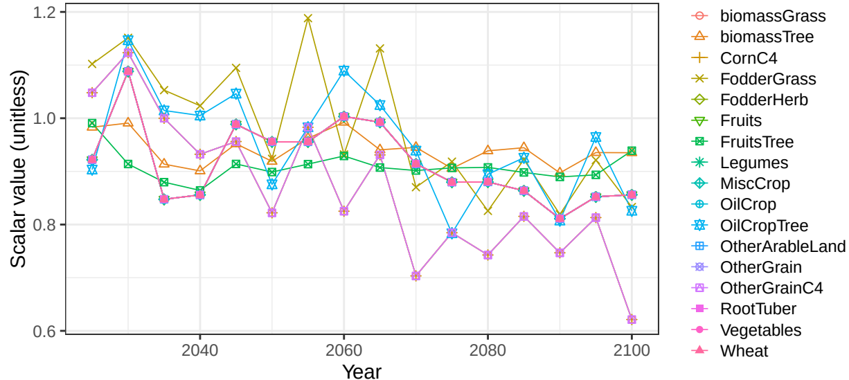
Region Australia_NZ basin AusCstW crop soil scalars
