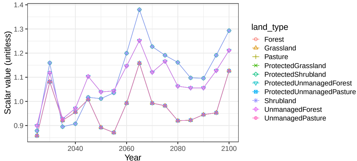
Region Russia basin CaspianNE non-crop vegetation scalars
