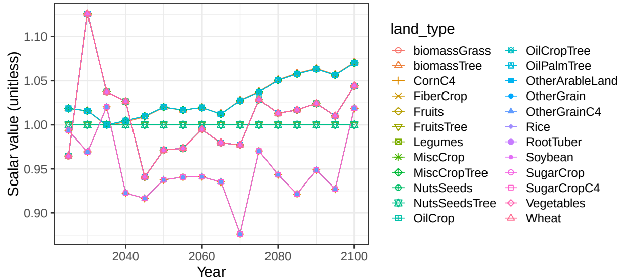
Region Colombia basin AmazonR crop vegetation scalars
