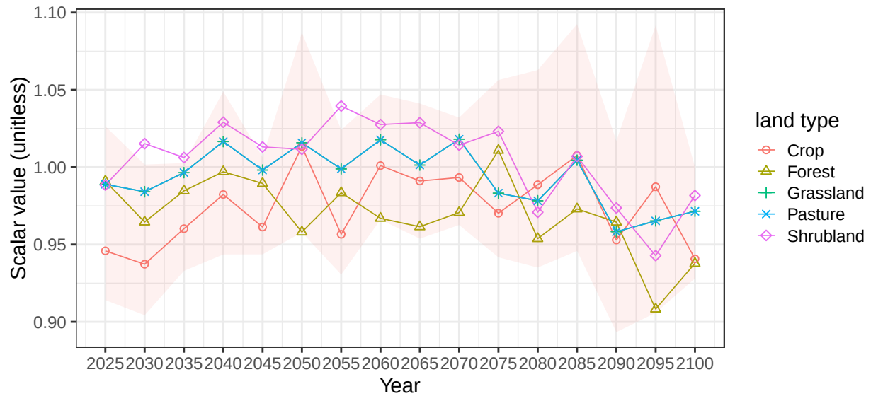
Region South America_Southern basin LaPuna average vegetation scalars
