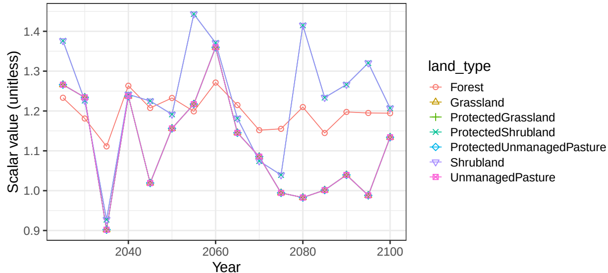
Region EU-15 basin EbroR non-crop vegetation scalars
