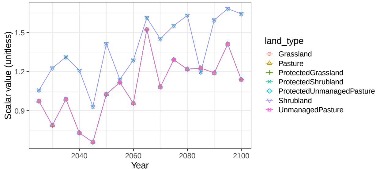
Region Central Asia basin CaspianE non-crop vegetation scalars
