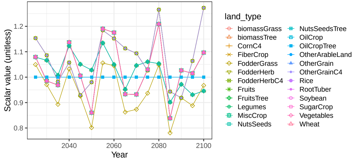
Region EU-12 basin DanubeR crop soil scalars
