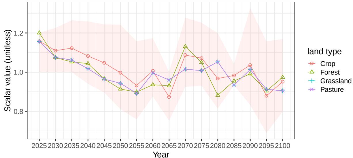
Region USA basin MisspppRN average soil scalars
