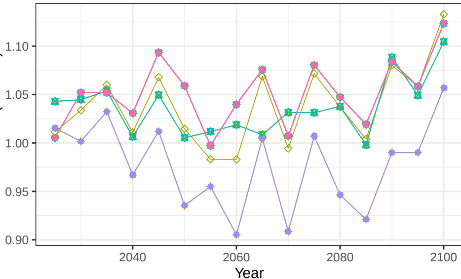
Region South Korea basin Korea crop vegetation scalars
