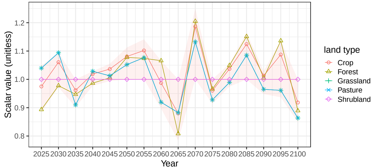
Region China basin Hainan average vegetation scalars
