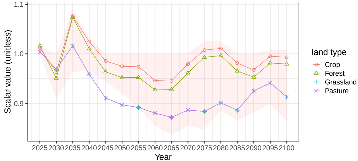
Region EU-15 basin Ireland average vegetation scalars
