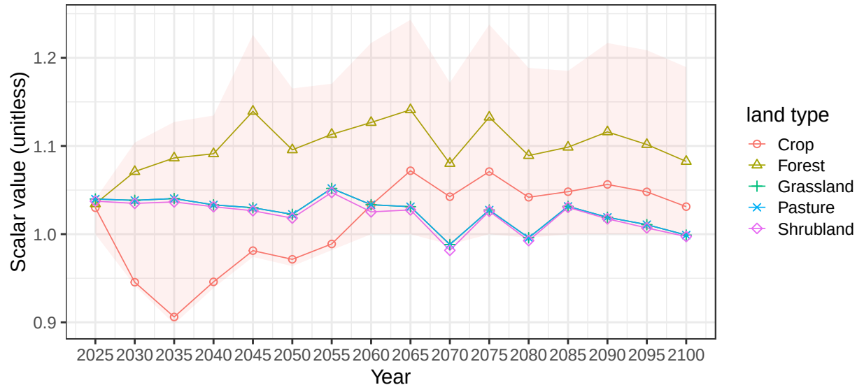
Region South America_Southern basin ArgCstS average soil scalars
