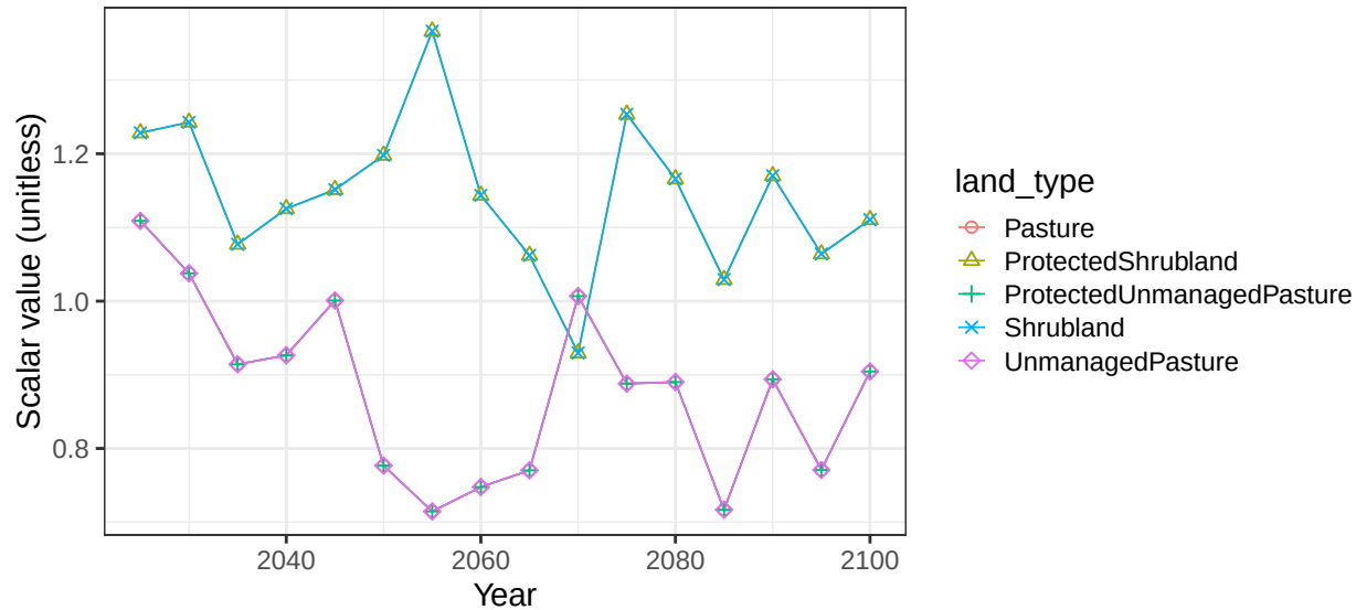
Region Pakistan basin HamuMashR non-crop soil scalars
