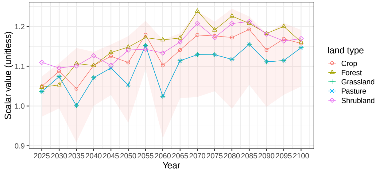
Region China basin XunJiang average vegetation scalars
