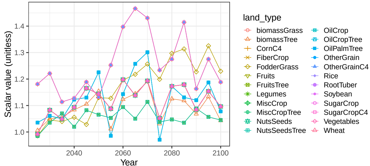
Region China basin Mekong crop vegetation scalars
