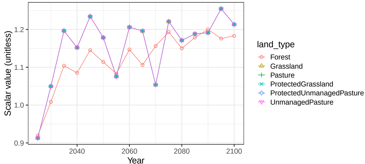
Region China basin RusCstSE non-crop vegetation scalars
