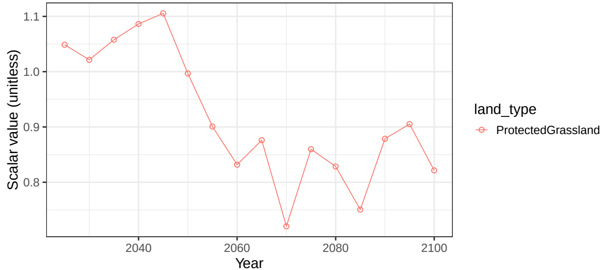
Region Africa_Northern basin AfrCstNE non-crop soil scalars
