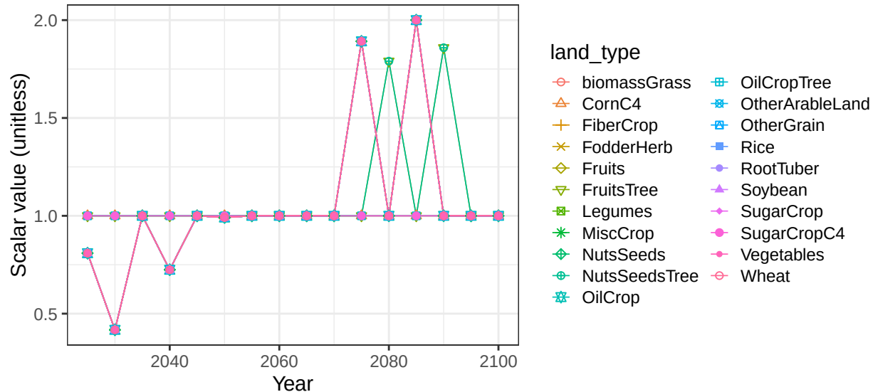
Region Africa_Northern basin MeditE crop vegetation scalars
