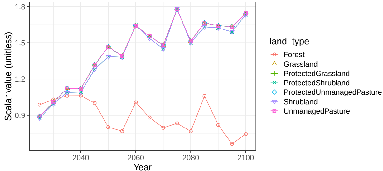
Region EU-15 basin Finland non-crop vegetation scalars
