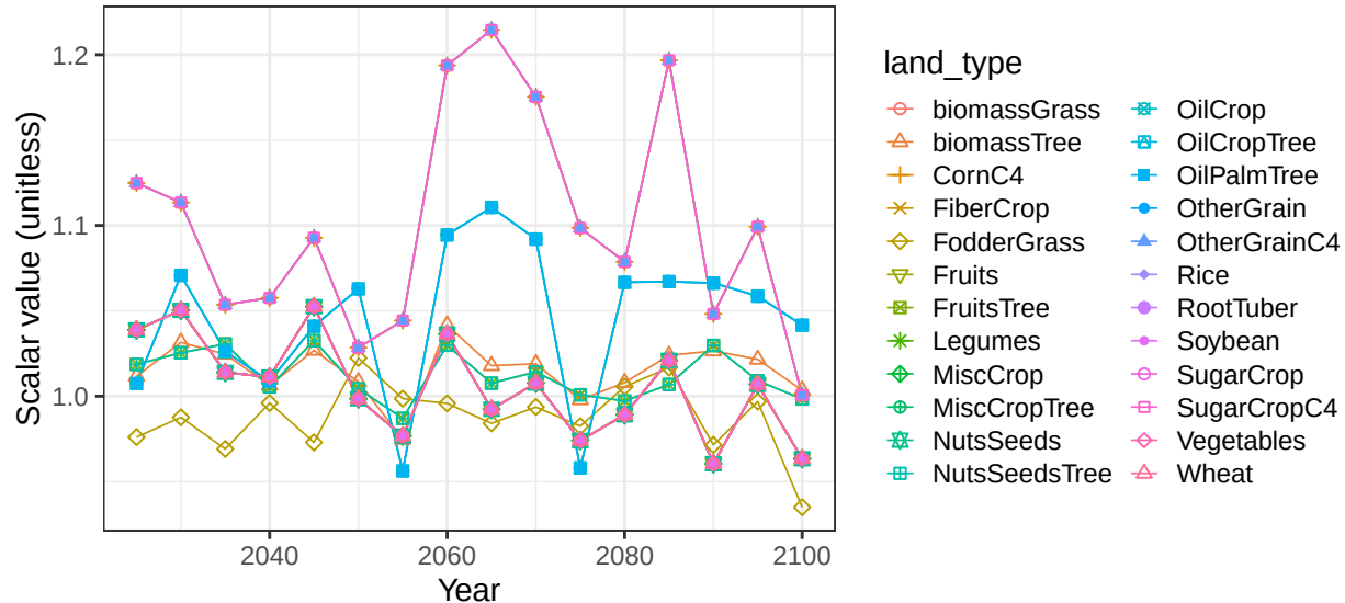
Region China basin Salween crop soil scalars
