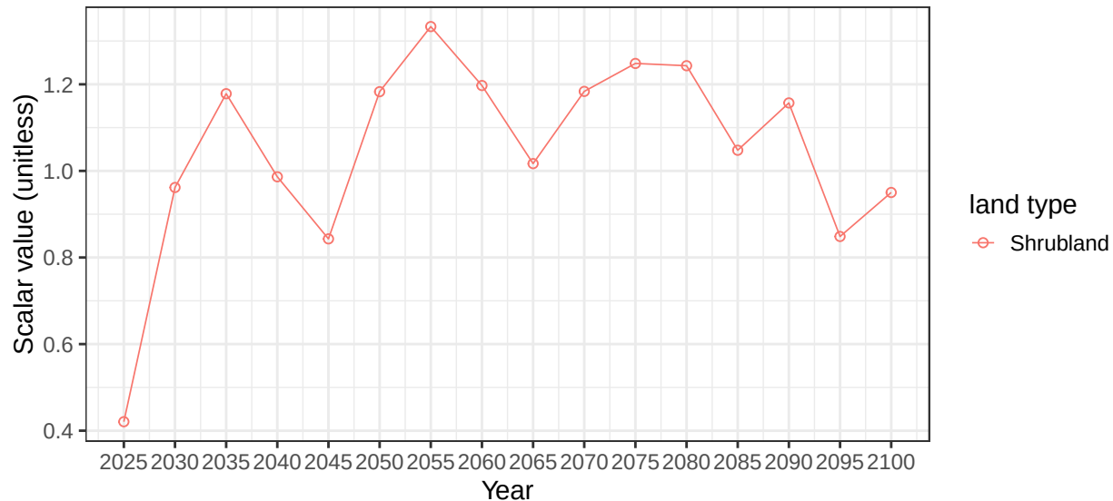
Region Russia basin ArcticIsl average vegetation scalars
