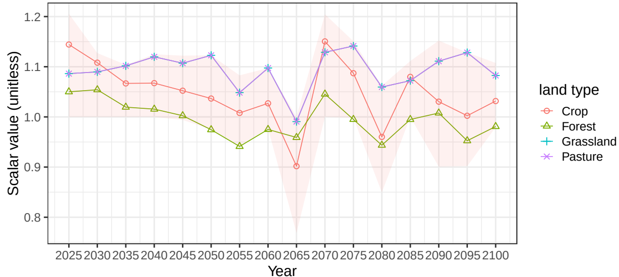
Region USA basin GreatLakes average soil scalars
