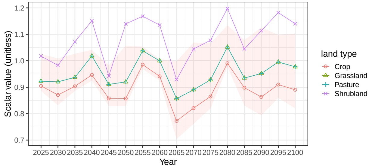
Region Africa_Southern basin OrangeR average soil scalars
