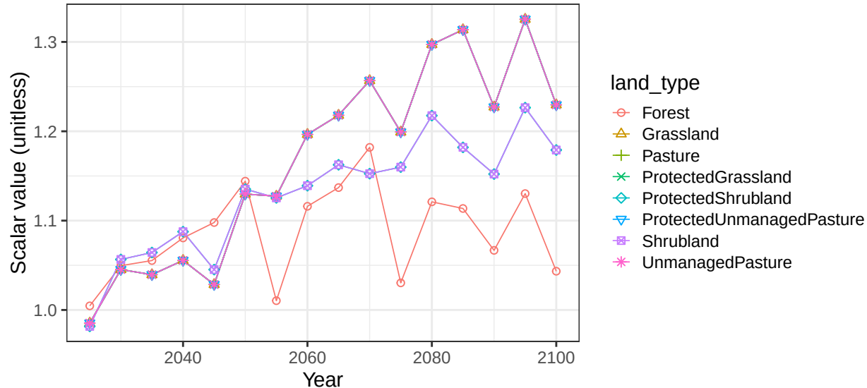
Region China basin Mekong non-crop vegetation scalars
