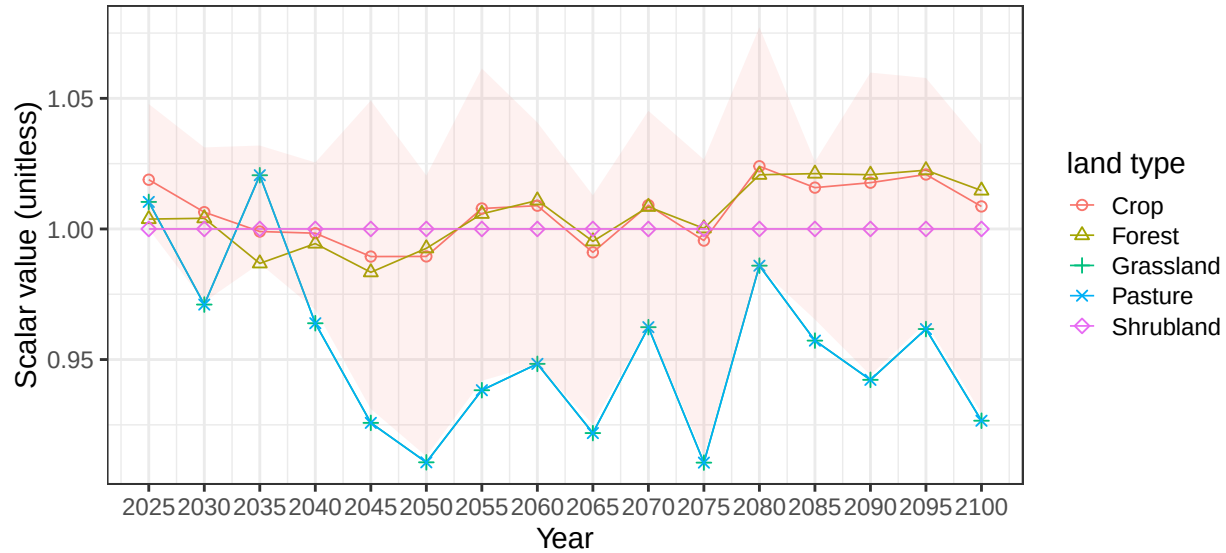
Region Central America and Caribbean basin ColEcuacSt average soil sca
