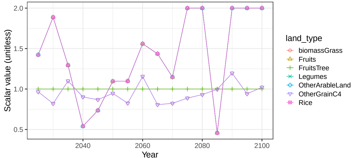
Region Africa_Western basin AfrCstNW crop vegetation scalars
