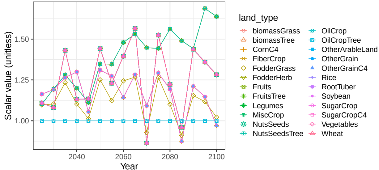
Region Middle East basin CaspianSW crop vegetation scalars
