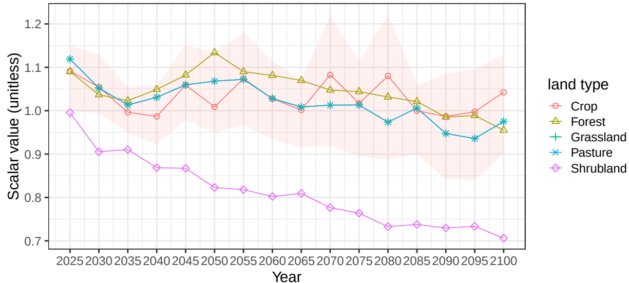
Region Africa_Southern basin AngolaCst average soil scalars
