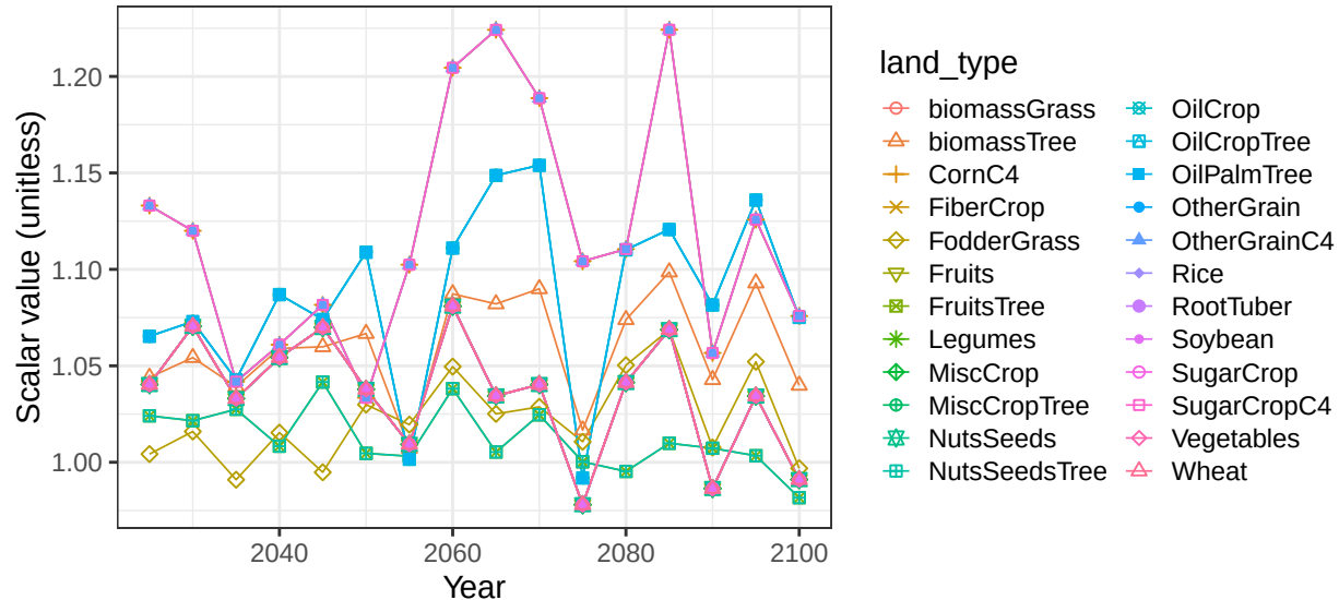
Region China basin Mekong crop soil scalars
