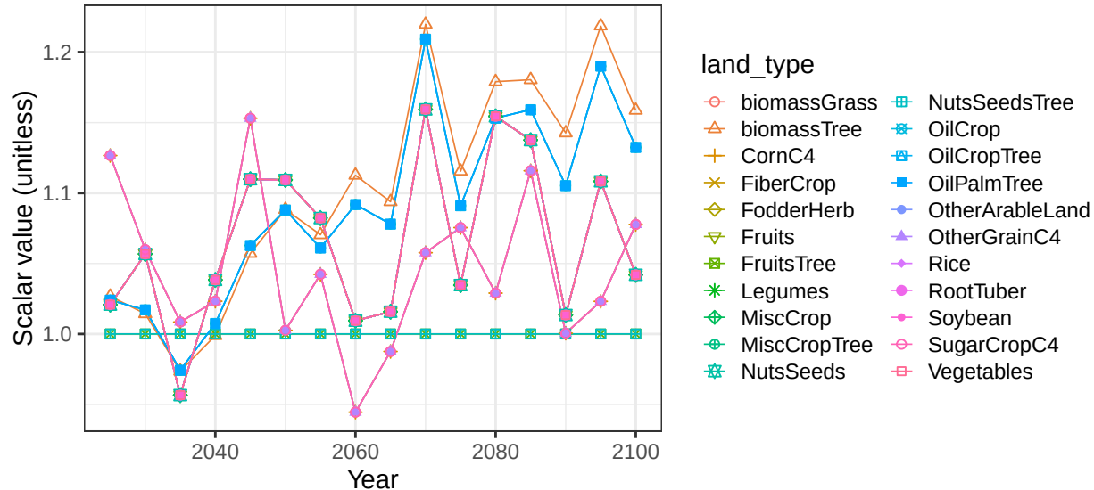
Region Southeast Asia basin VietnamCst crop vegetation scalars
