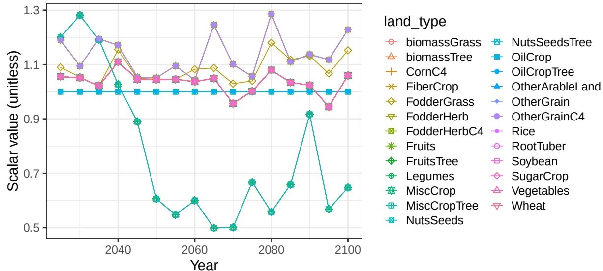
Region EU-15 basin RhoneR crop vegetation scalars
