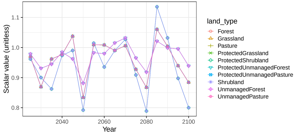
Region Australia_NZ basin AusCstE non-crop soil scalars
