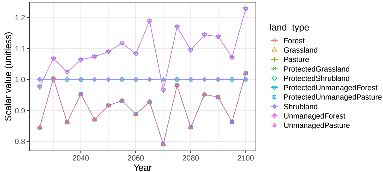
Region Mexico basin MexCstW non-crop vegetation scalars
