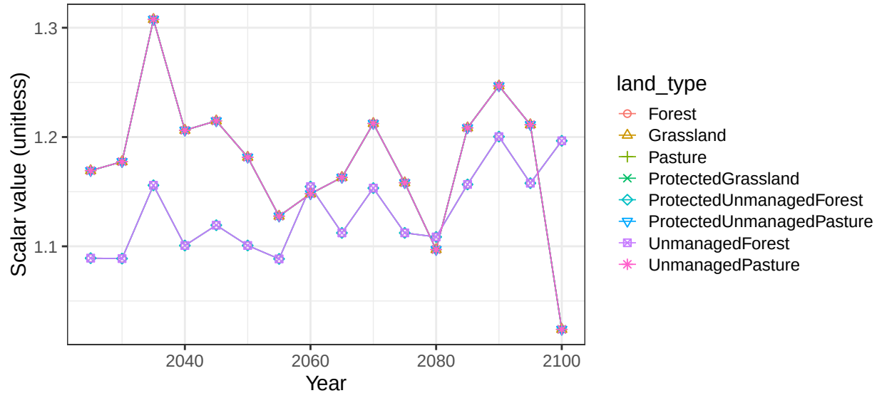
Region Southeast Asia basin Korea non-crop vegetation scalars
