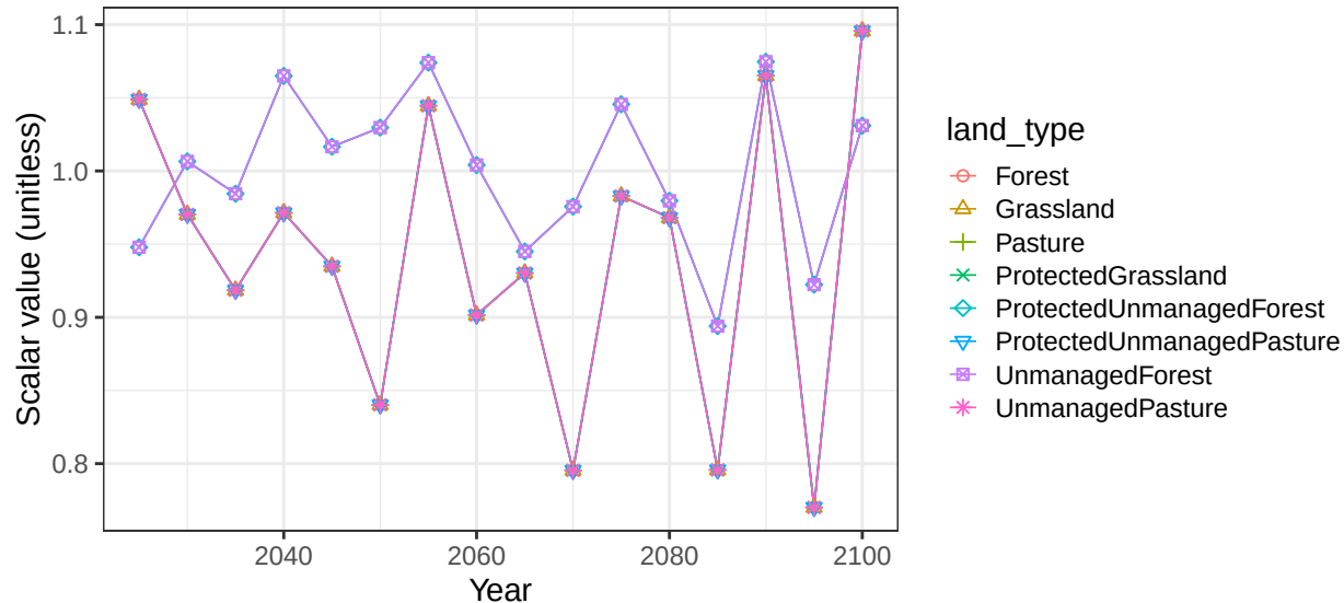
Region EU-12 basin DniesterR non-crop soil scalars
