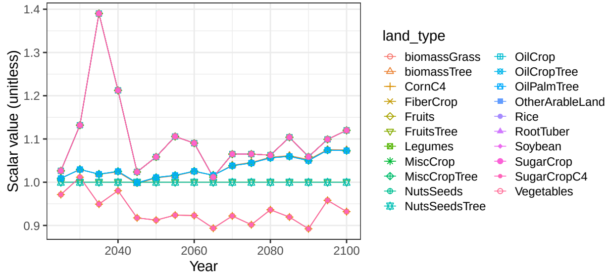
Region Indonesia basin SepikR crop vegetation scalars
