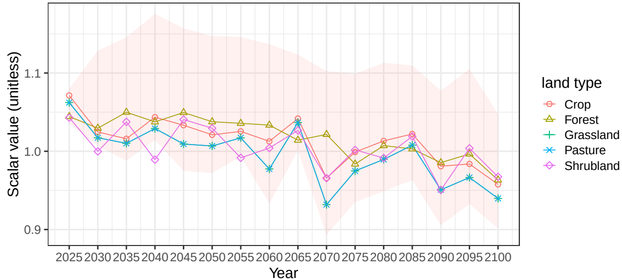
Region China basin ChinaCst average soil scalars
