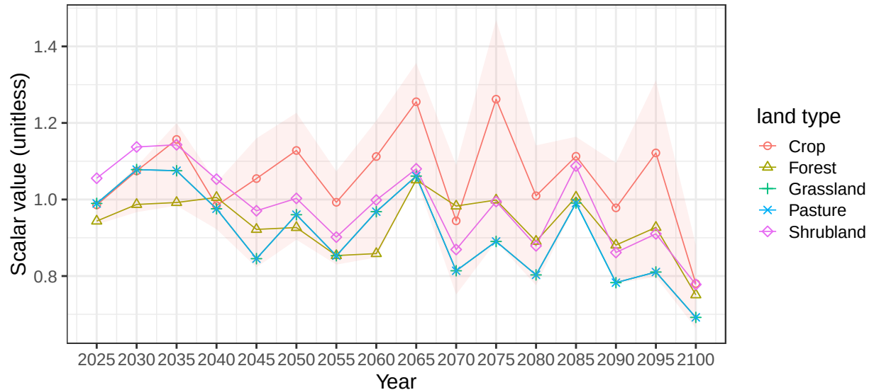
Region Argentina basin RioLaPlata average vegetation scalars
