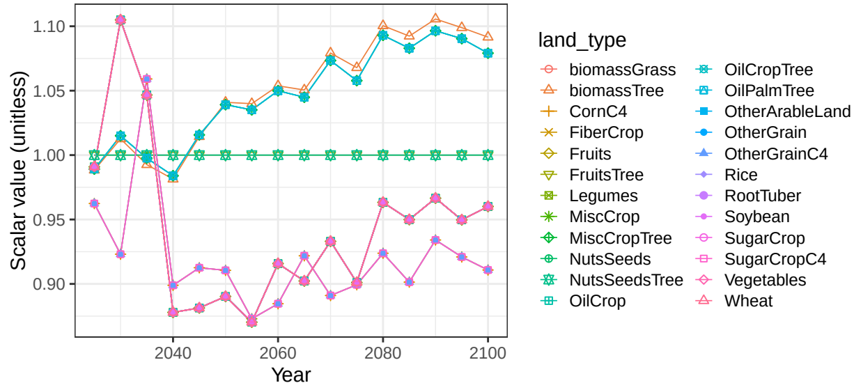
Region Colombia basin MagdalenaR crop vegetation scalars
