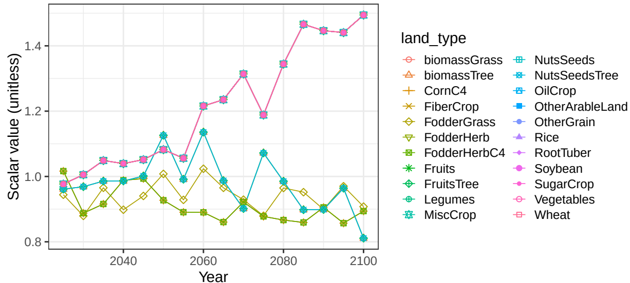
Region Central Asia basin Gobi crop soil scalars
