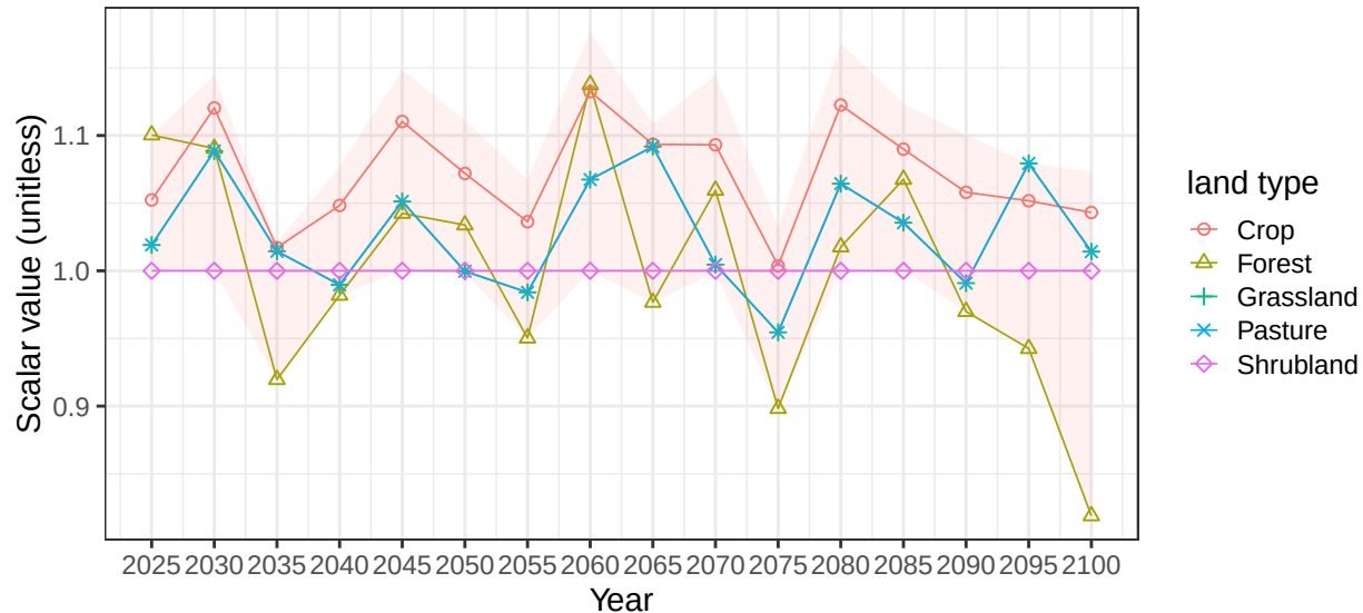
Region India basin GodavariR average soil scalars
