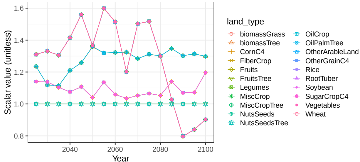
Region Africa_Southern basin AngolaCst crop vegetation scalars
