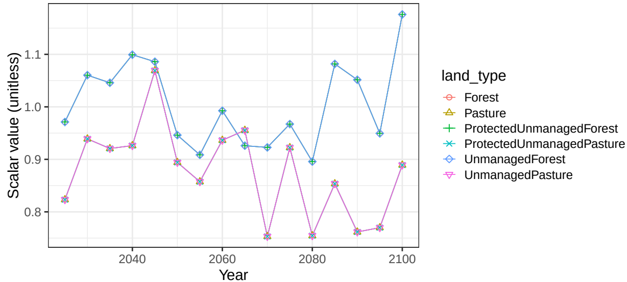
Region EU-12 basin DnkGrmCst non-crop soil scalars
