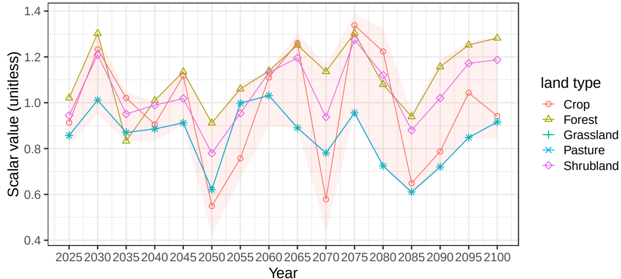
Region Russia basin BlackSeaN average vegetation scalars
