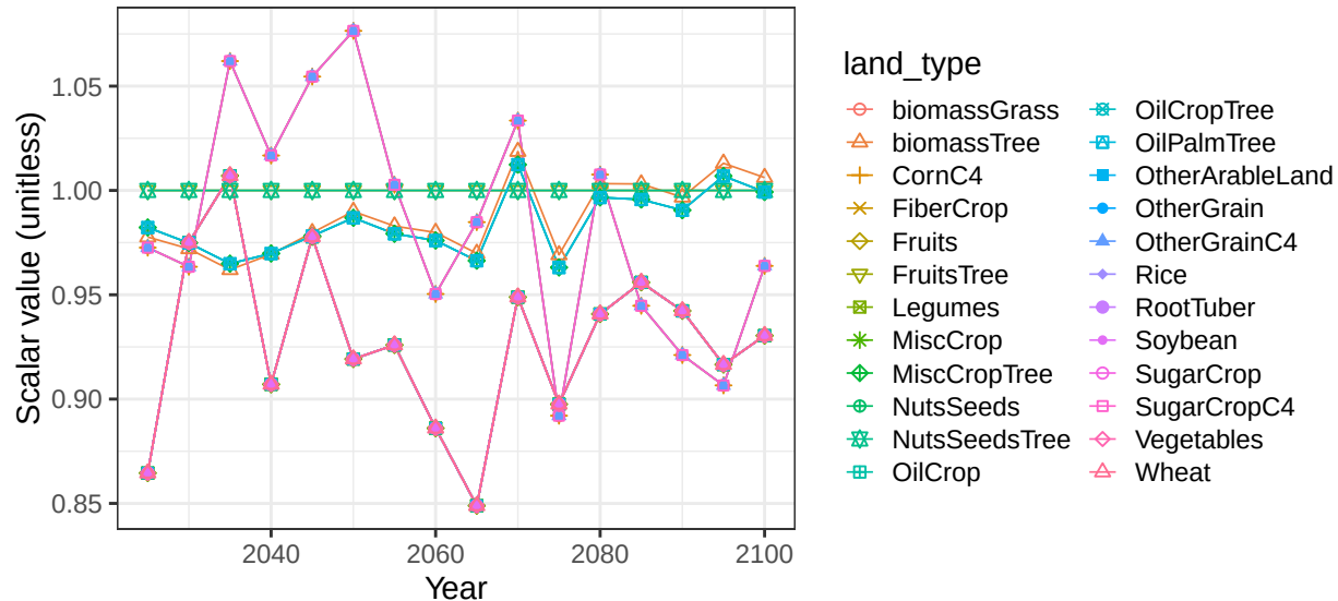
Region Colombia basin OrinocoR crop vegetation scalars
