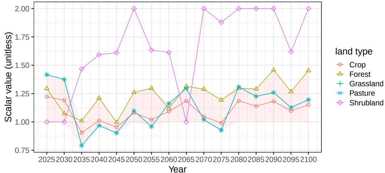
Region USA basin MexCstNW average vegetation scalars
