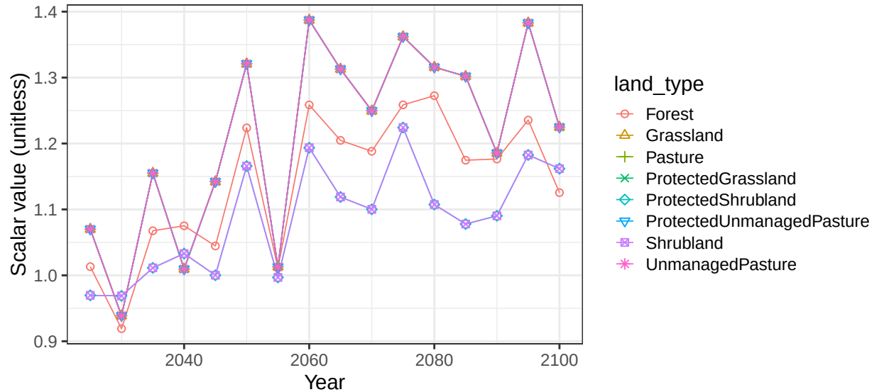
Region China basin Gobi non-crop vegetation scalars
