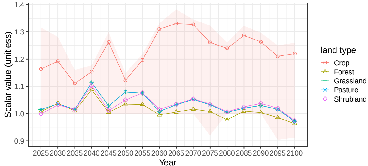
Region Canada basin NWTerr average soil scalars
