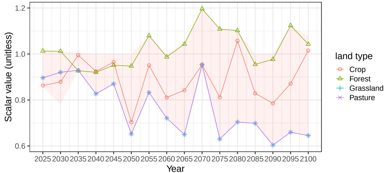
Region Europe_Eastern basin DonR average soil scalars
