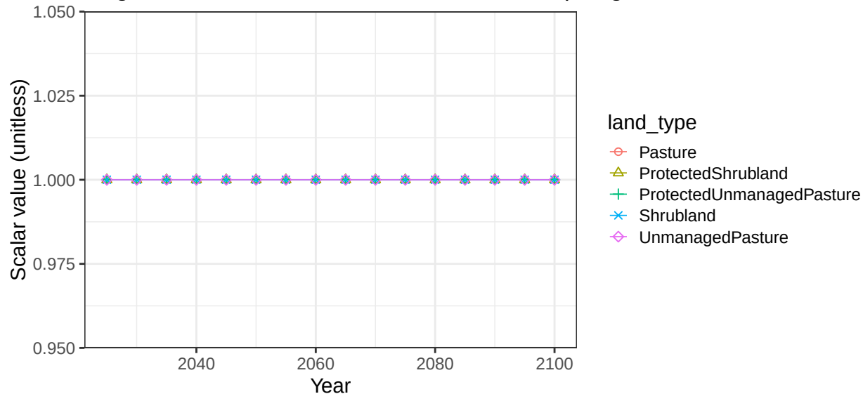
Region Middle East basin AfrCstNE non-crop vegetation scalars
