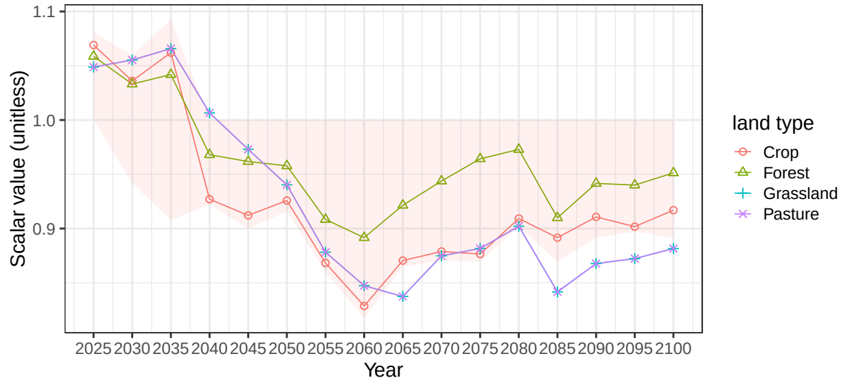
Region EU-15 basin Scotland average vegetation scalars
