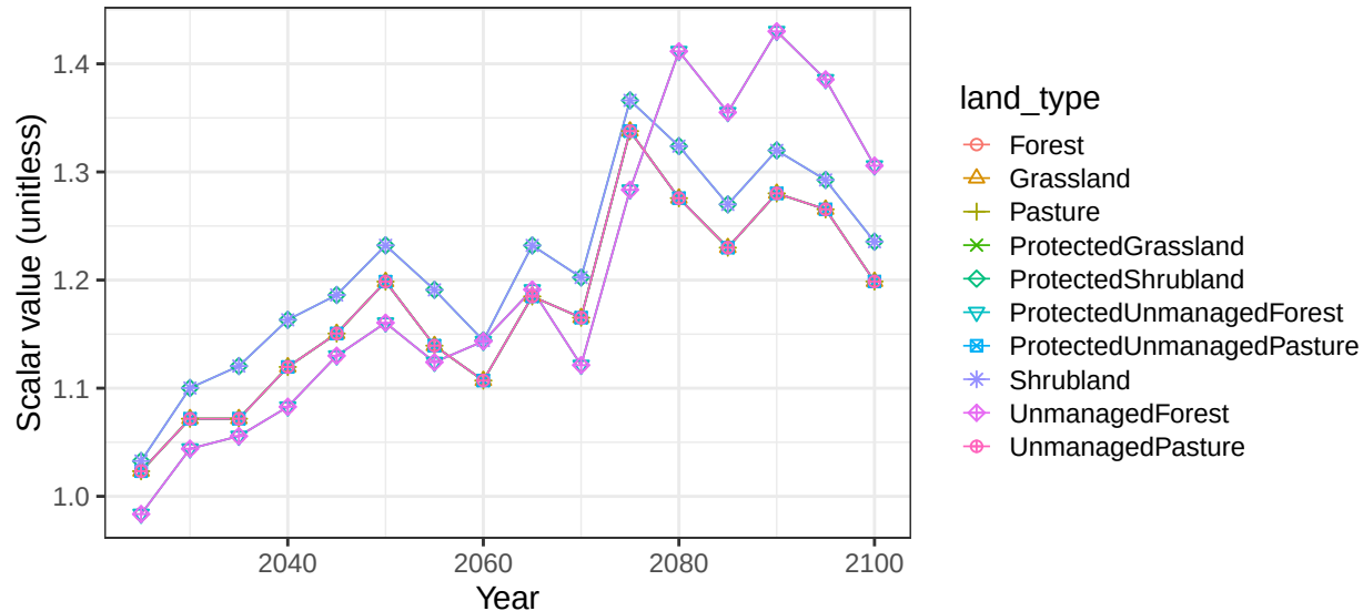
Region Russia basin LenaR non-crop vegetation scalars
