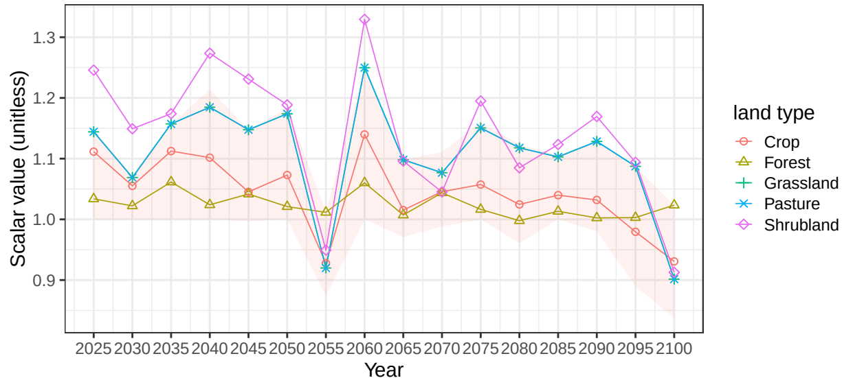
Region China basin BoHai average soil scalars
