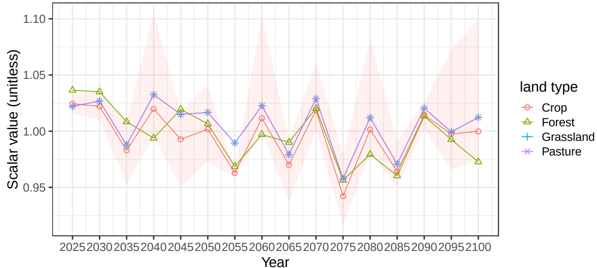
Region European Free Trade Association basin PoR average soil scalars
