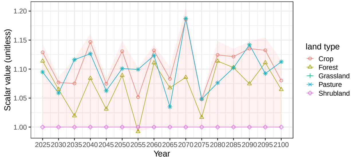
Region Southeast Asia basin ChaoPhrR average soil scalars
