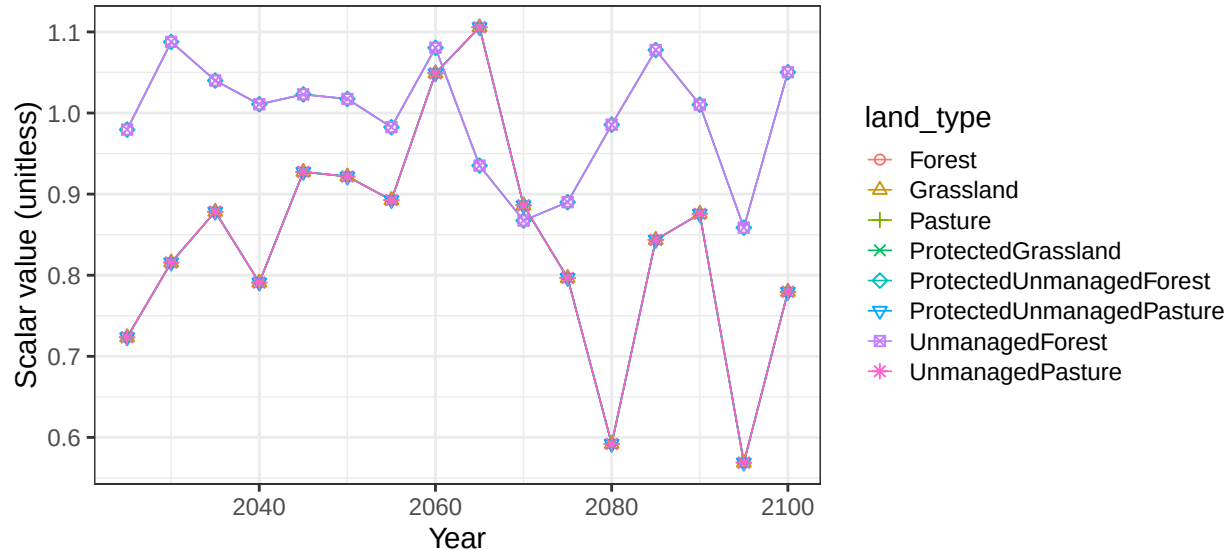
Region Russia basin NemanR non-crop soil scalars
