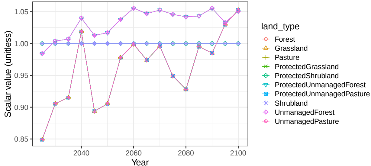
Region Brazil basin TocantinsR non-crop soil scalars
