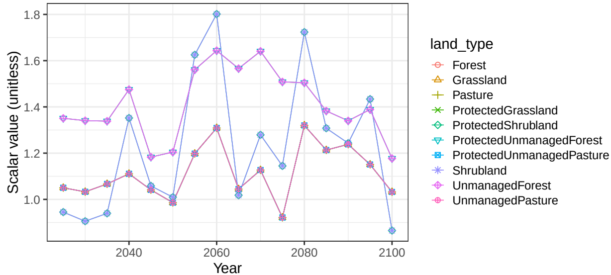
Region Africa_Southern basin AfrIntS non-crop vegetation scalars
