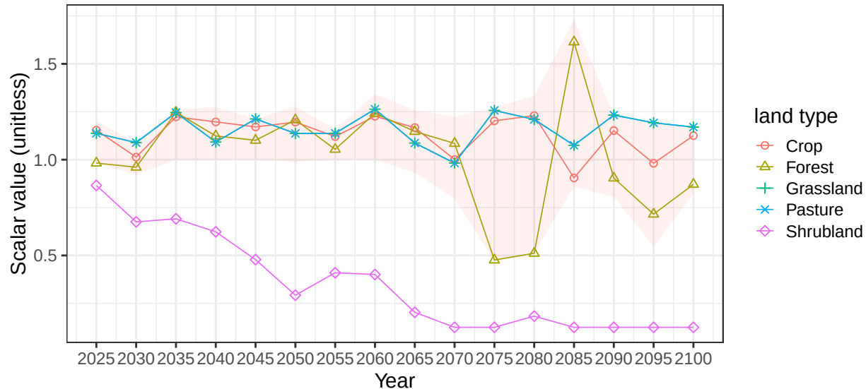
Region Africa_Eastern basin RiftValley average vegetation scalars
