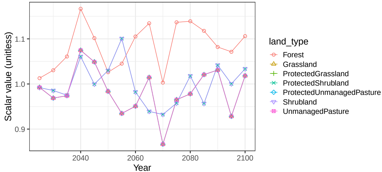
Region EU-15 basin FranceCstW non-crop soil scalars
