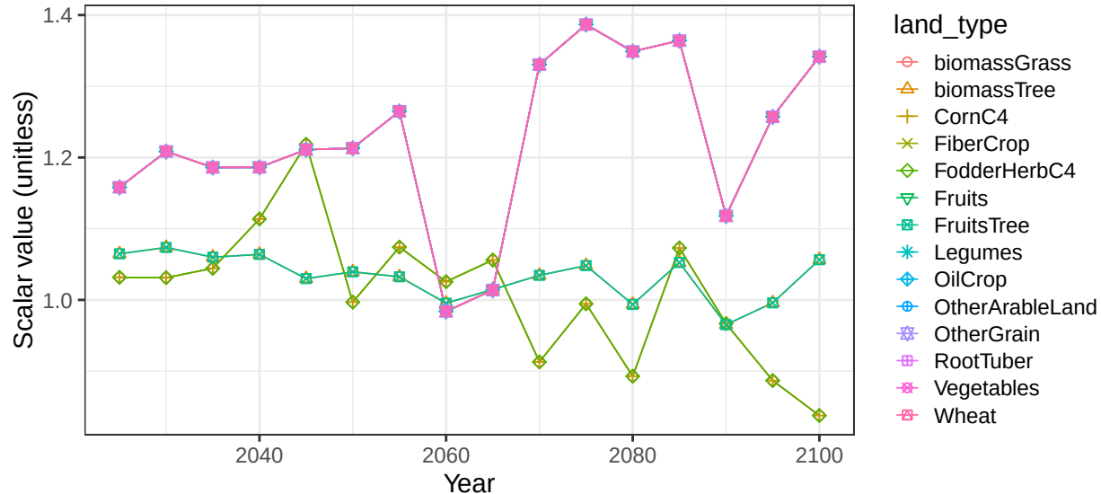
Region Canada basin UsaPacNW crop soil scalars
