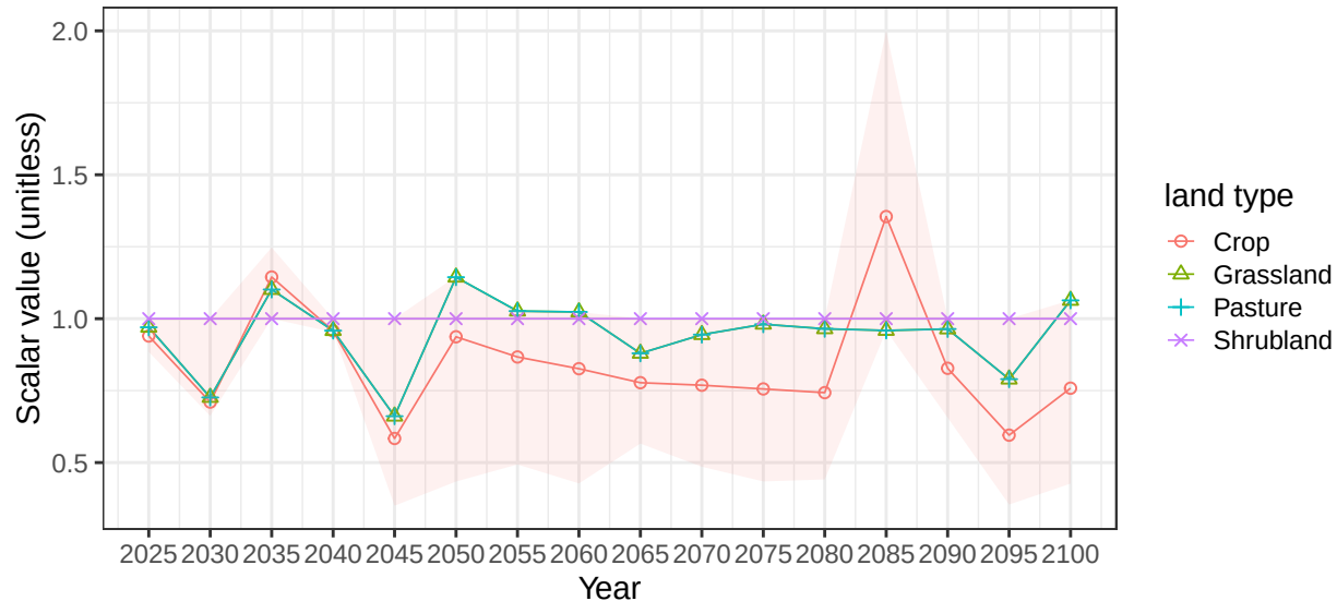
Region Africa_Eastern basin LChad average vegetation scalars
