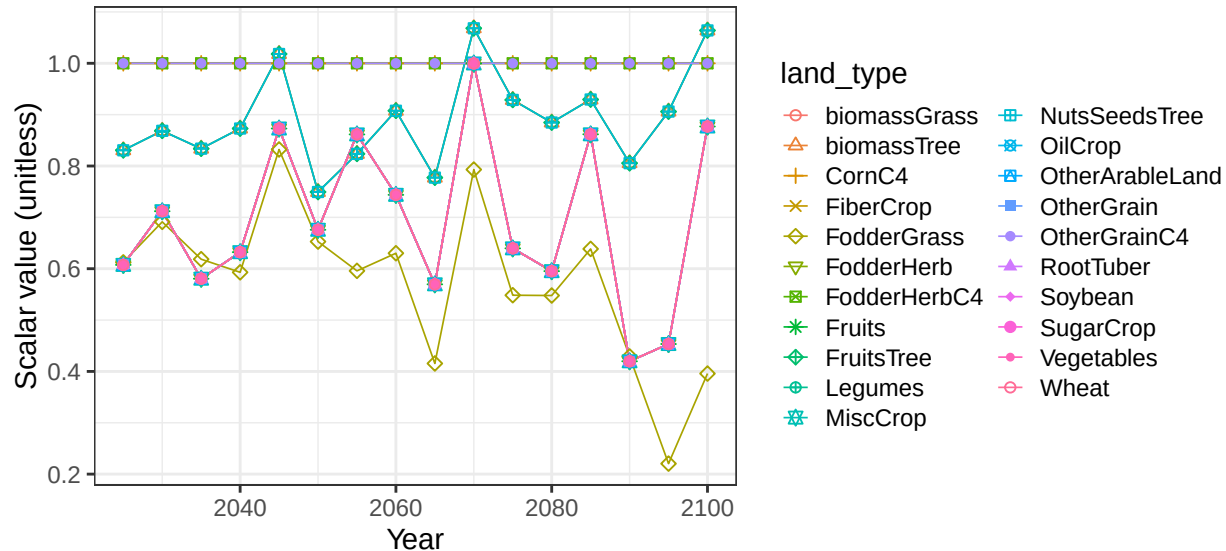
Region Russia basin DaugavaR crop vegetation scalars
