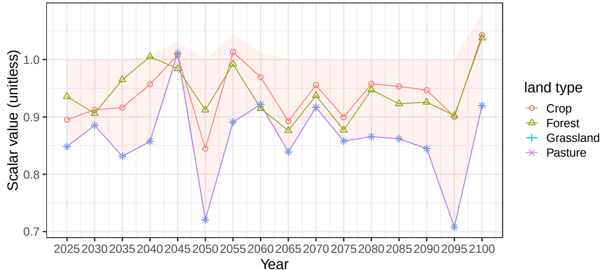
Region Europe_Eastern basin NemanR average soil scalars
