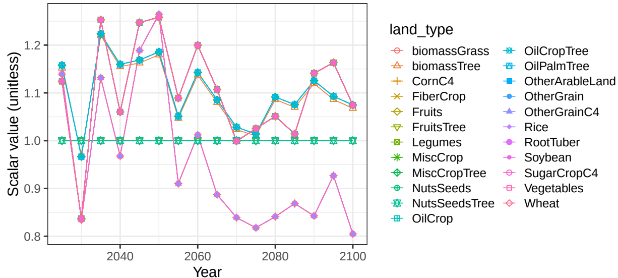
Region Africa_Southern basin NileR crop soil scalars
