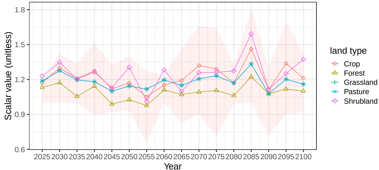
Region USA basin UsaColoRN average vegetation scalars
