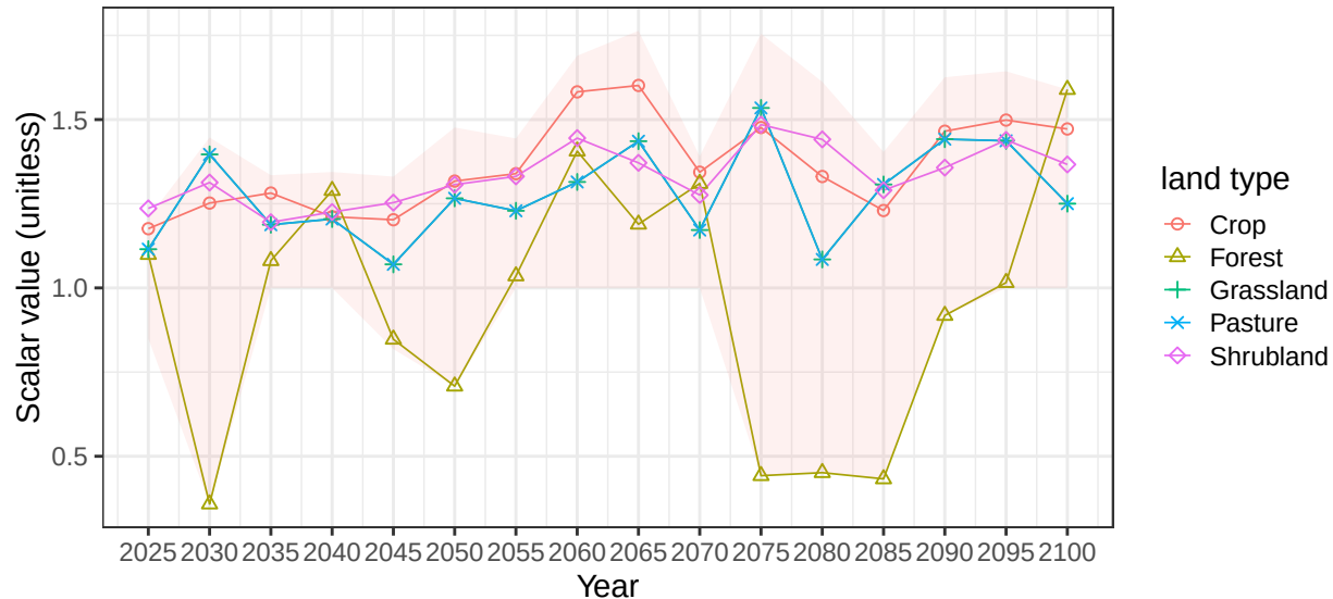
Region Middle East basin TigrEuphR average vegetation scalars
