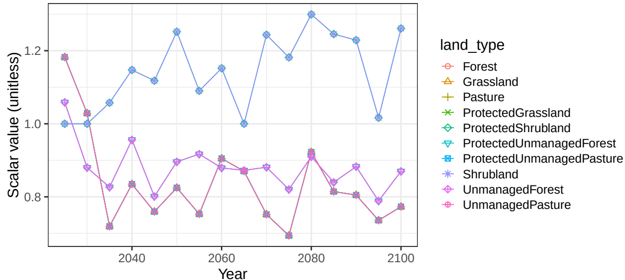
Region USA basin MexCstNW non-crop soil scalars
