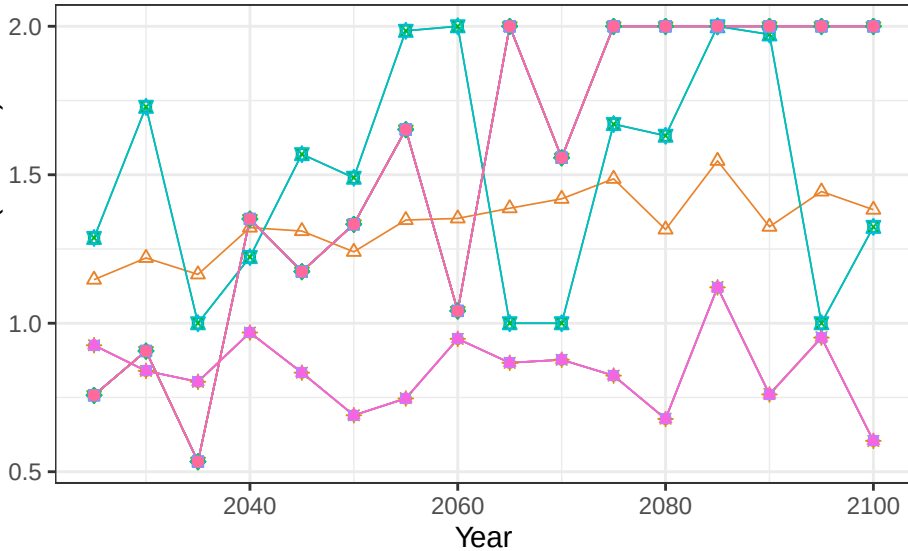
Region Australia_NZ basin AusCstN crop vegetation scalars
