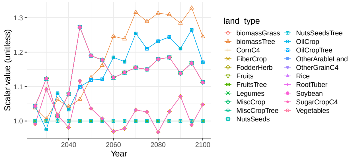
Region Southeast Asia basin Hong crop vegetation scalars
