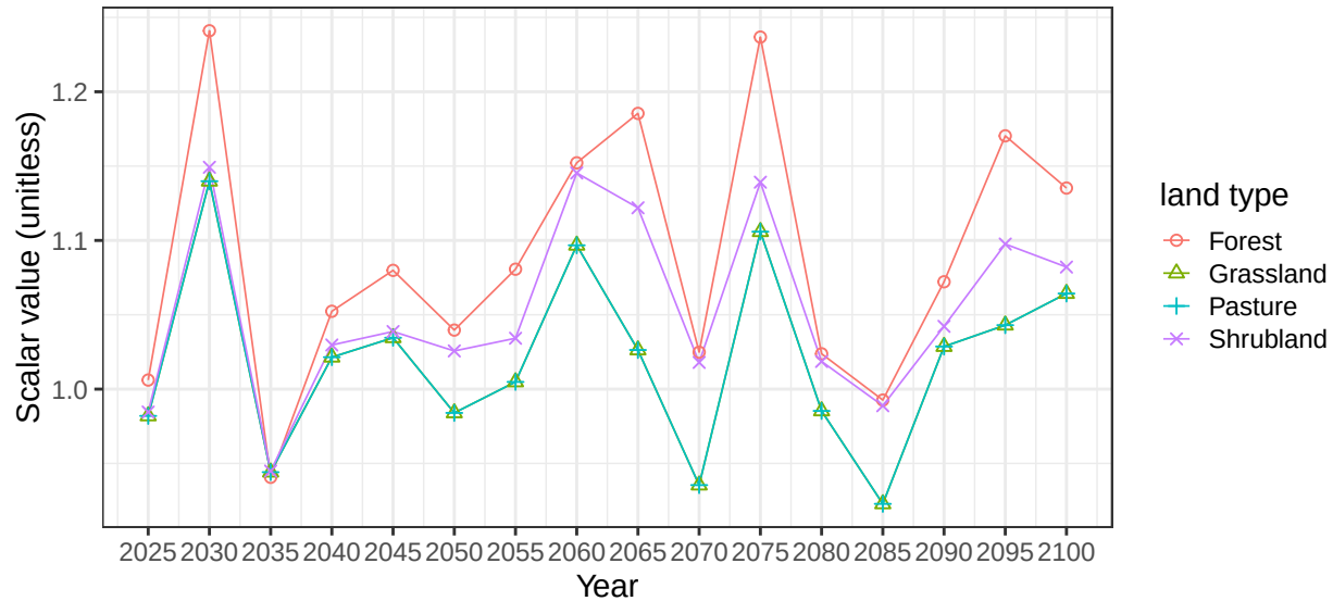
Region Russia basin BlackSeaS average soil scalars
