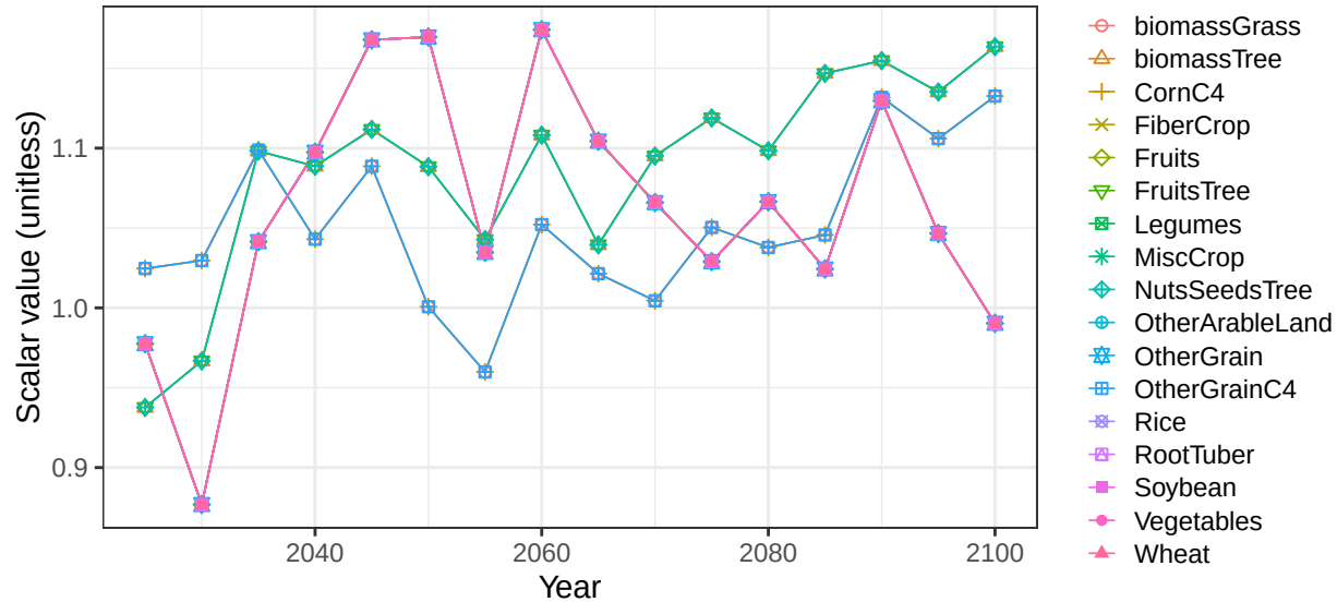
Region Southeast Asia basin RusCstSE crop vegetation scalars
