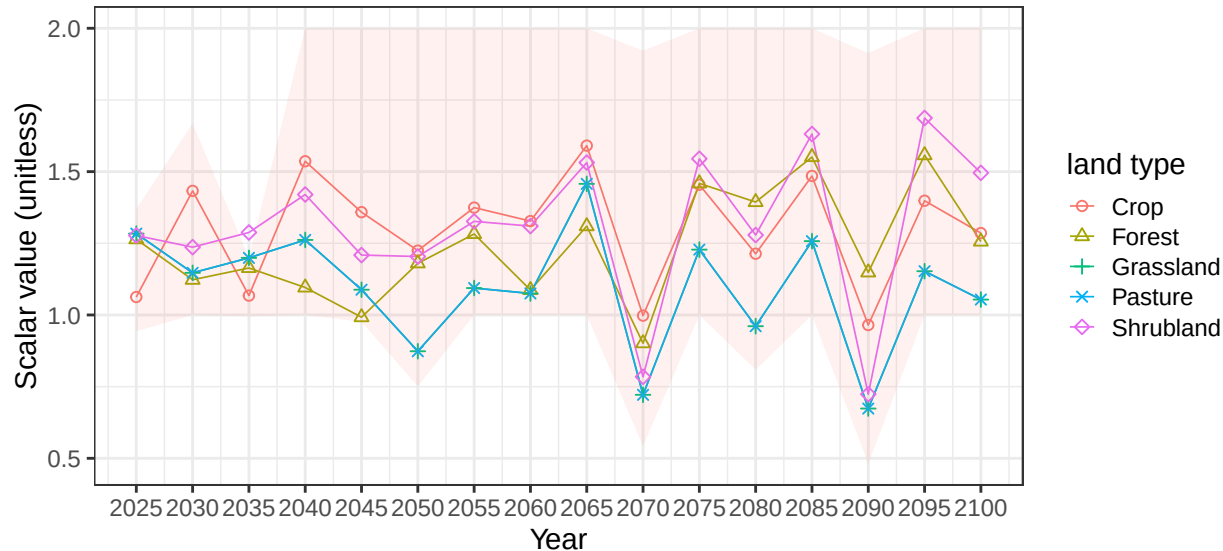
Region Argentina basin ArgColoR average vegetation scalars
