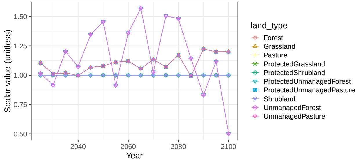
Region Africa_Western basin VoltaR non-crop vegetation scalars
