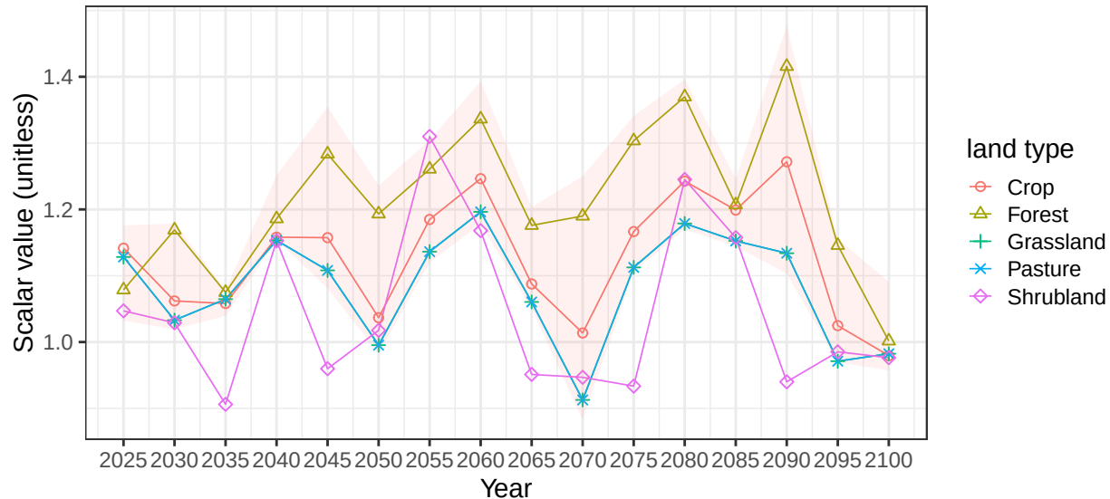
Region Africa_Southern basin LimpopoR average soil scalars
