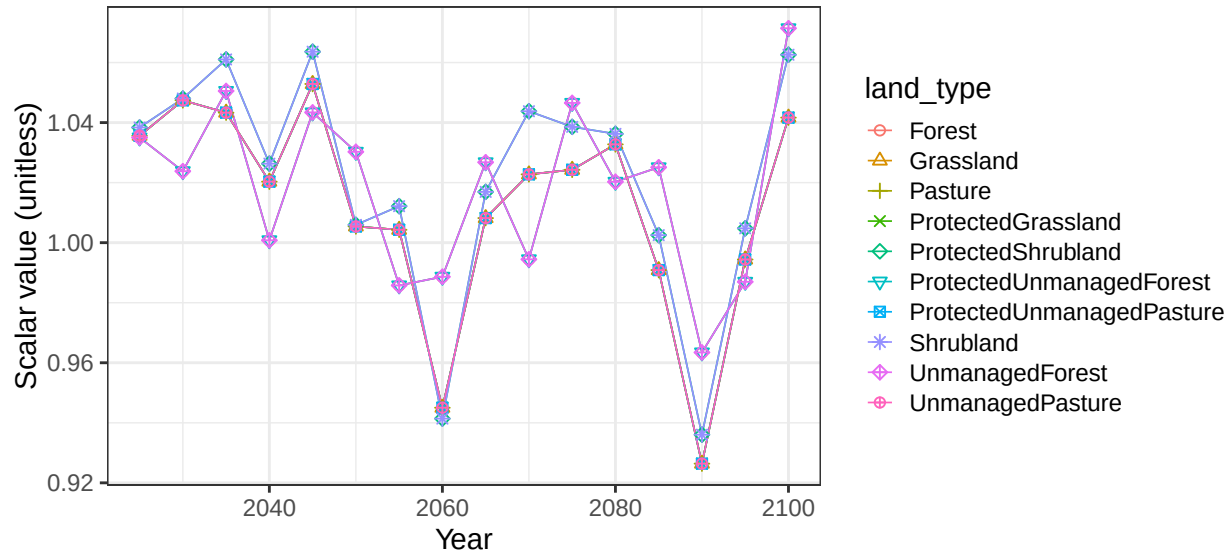
Region USA basin PacArctic non-crop soil scalars
