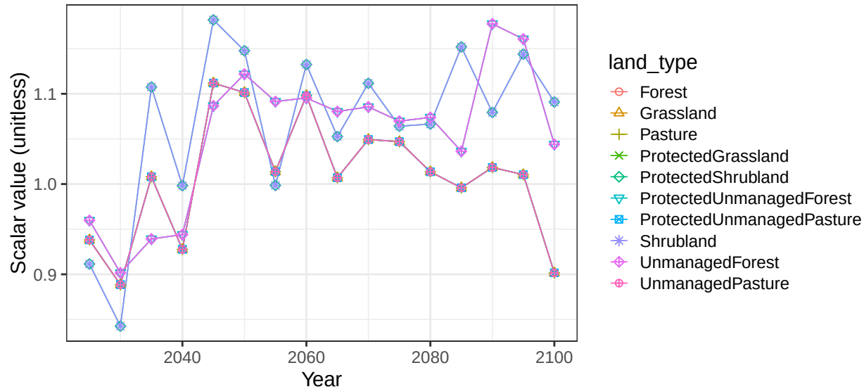
Region Russia basin ObR non-crop vegetation scalars
