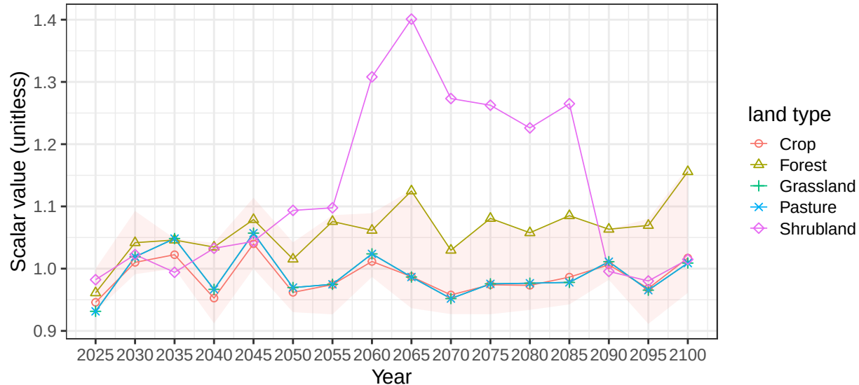
Region Mexico basin Papaloapan average vegetation scalars
