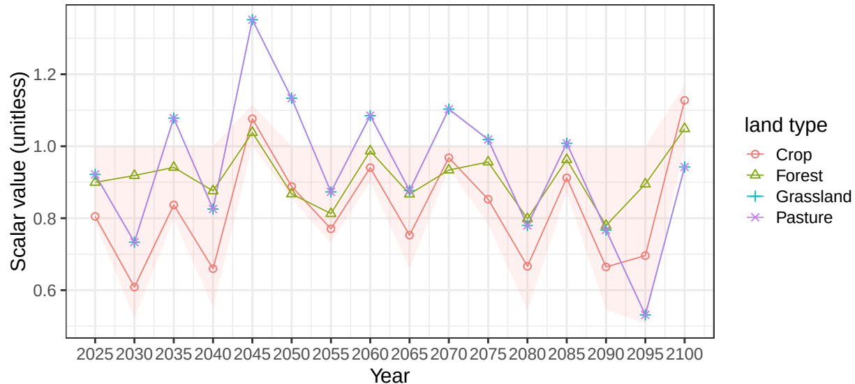
Region EU-12 basin NarvaR average vegetation scalars
