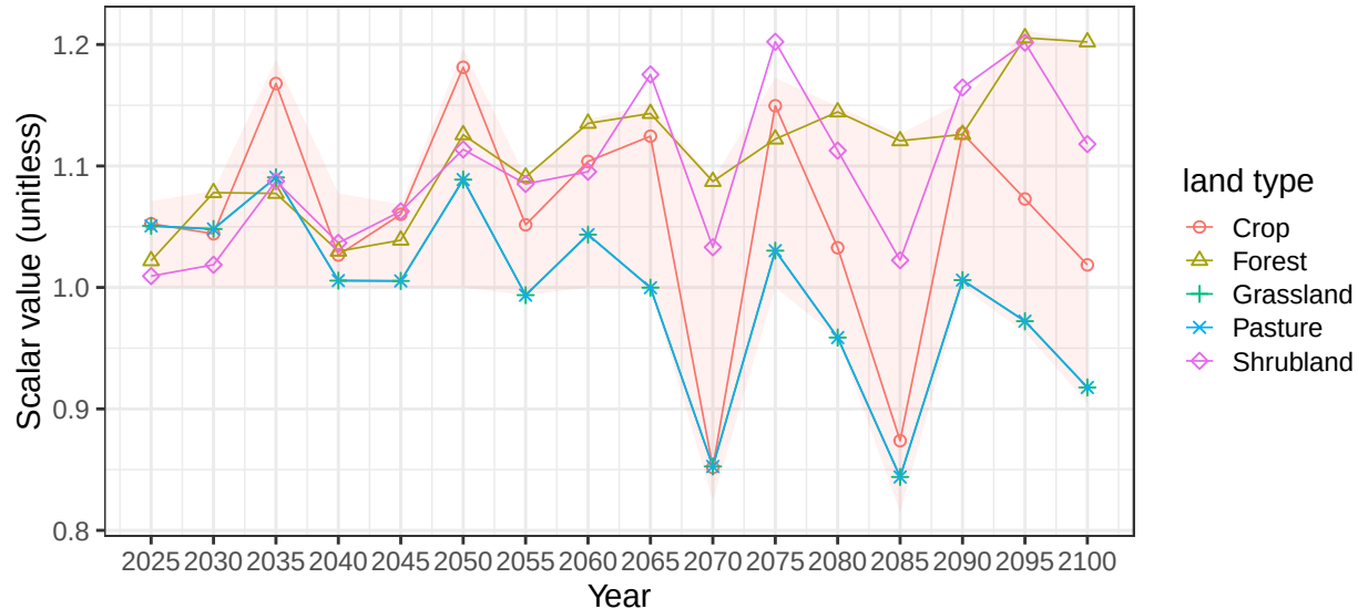
Region Middle East basin CaspianSW average soil scalars
