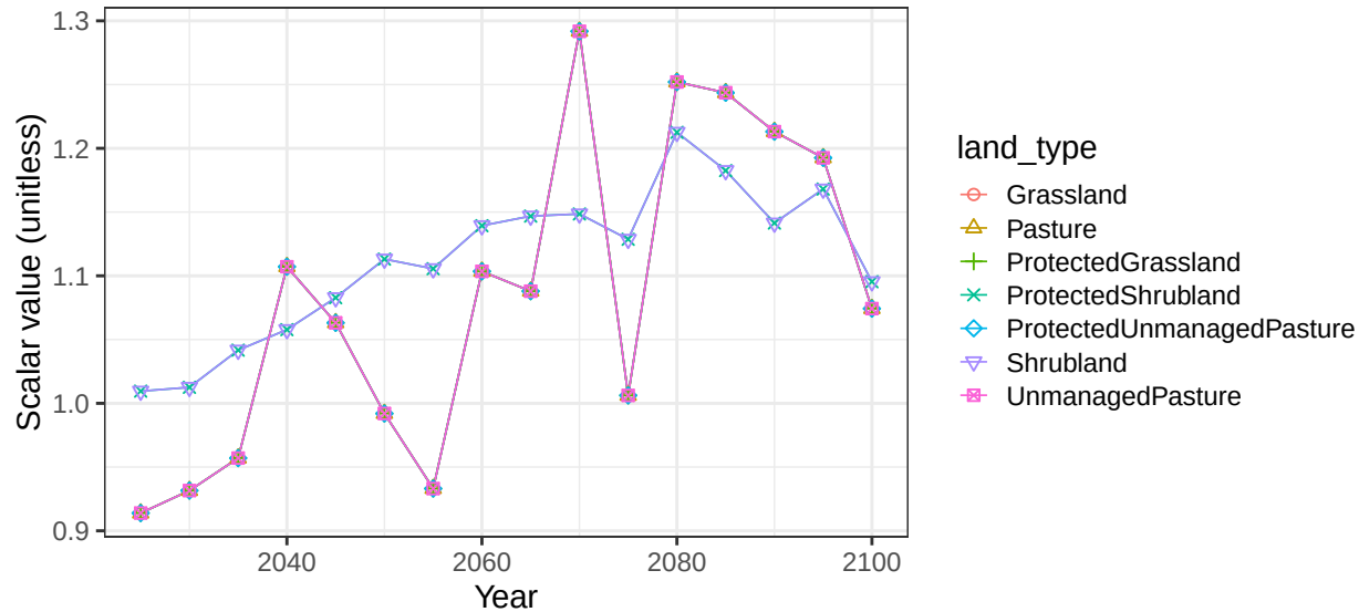
Region China basin IndusR non-crop vegetation scalars
