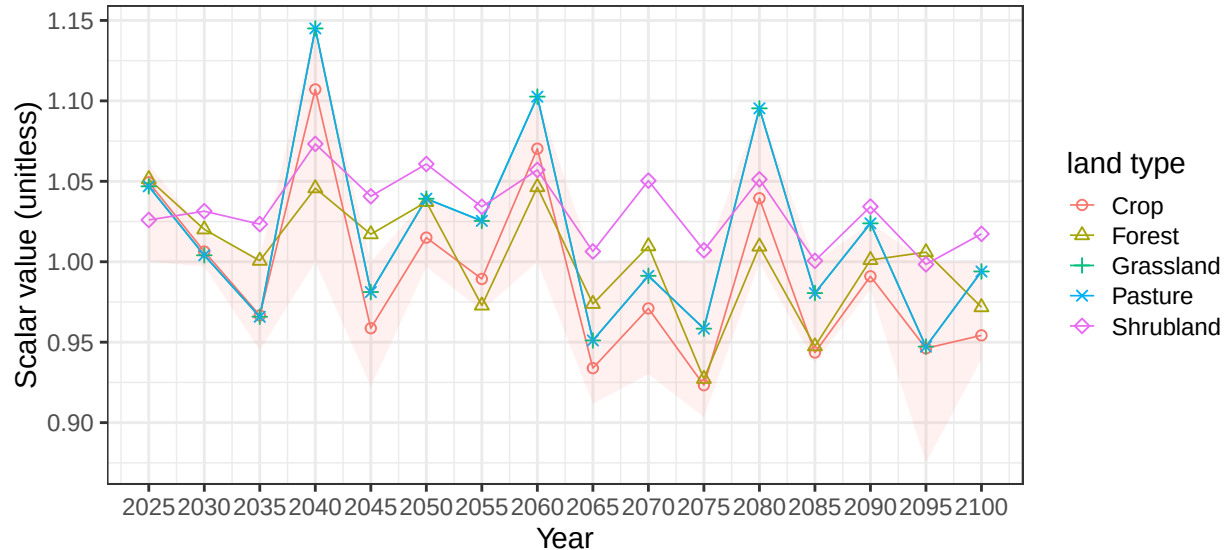
Region EU-15 basin PoR average soil scalars
