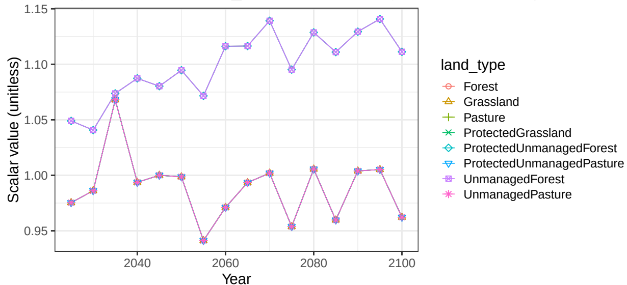
Region South America_Northern basin MagdalenaR non-crop soil scalars
