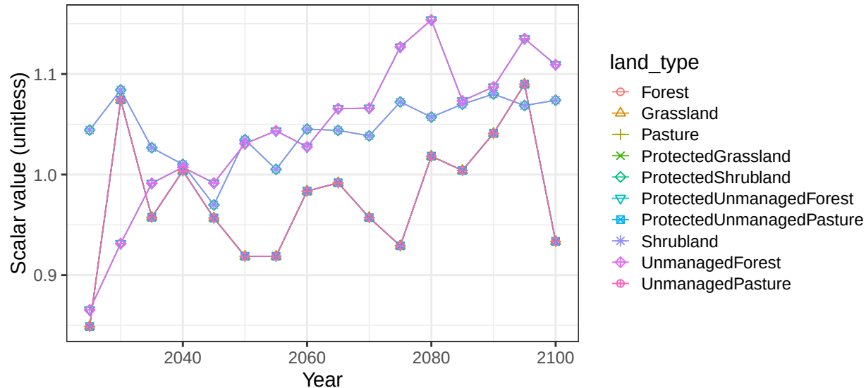
Region Brazil basin RioLaPlata non-crop vegetation scalars
