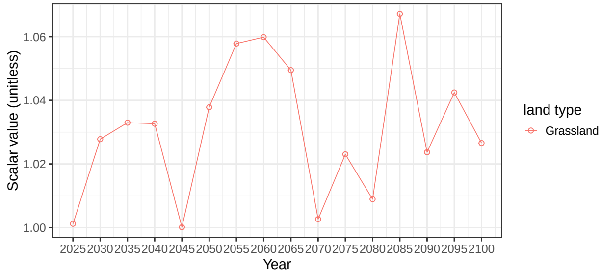
Region EU-15 basin ArgCstS average vegetation scalars
