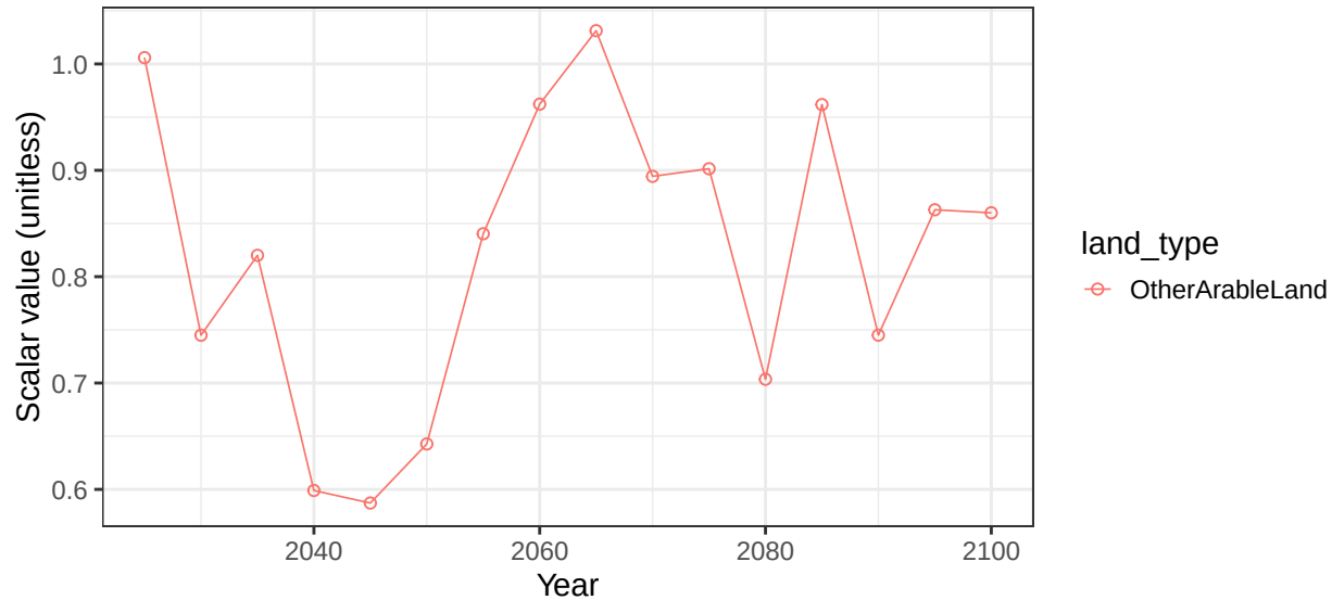
Region Pakistan basin Tarim crop soil scalars
