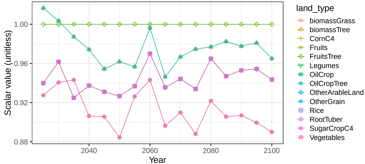
Region Brazil basin SAmerCstNE crop soil scalars
