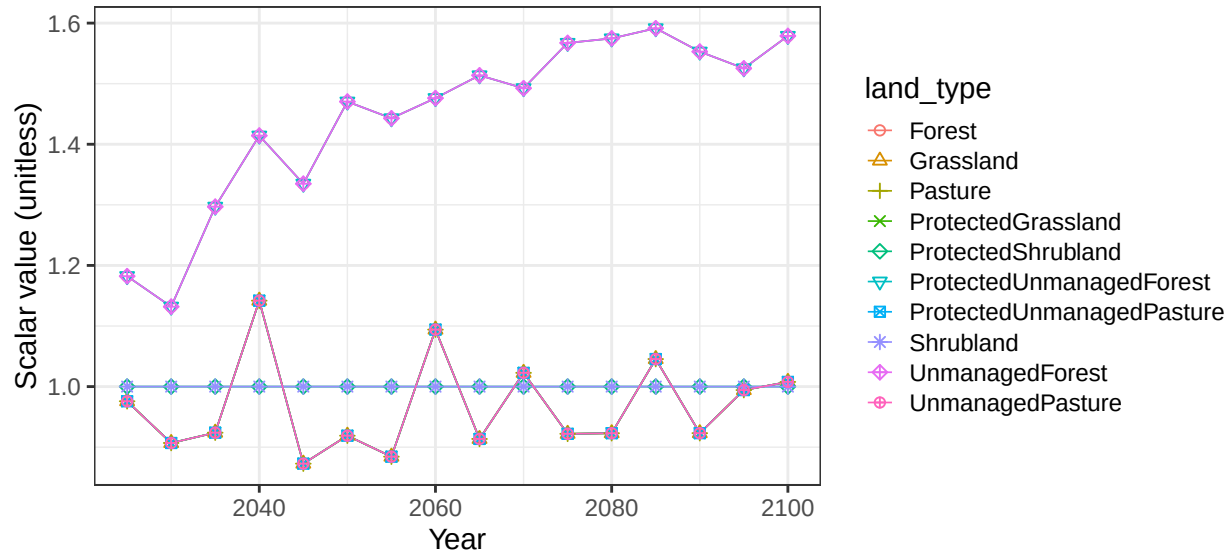
Region Brazil basin ParnaibaR non-crop vegetation scalars
