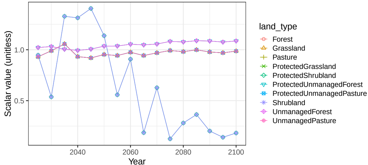
Region Colombia basin ColEcuacSt non-crop vegetation scalars
