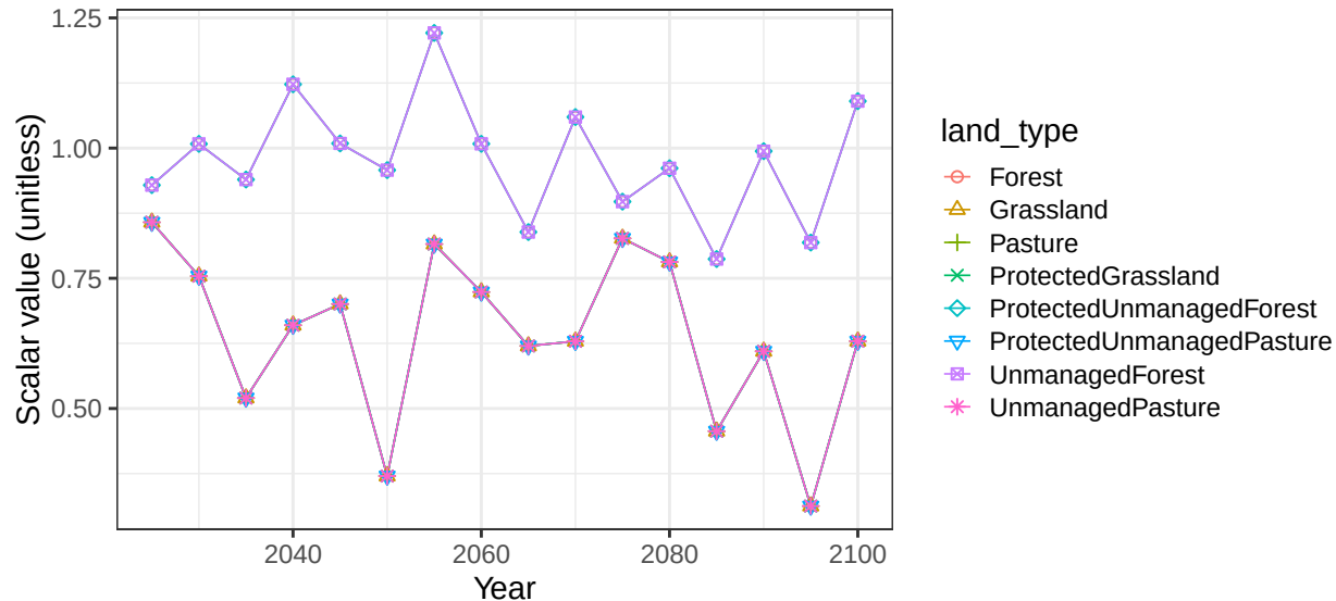
Region Europe_Eastern basin DniesterR non-crop vegetation scalars
