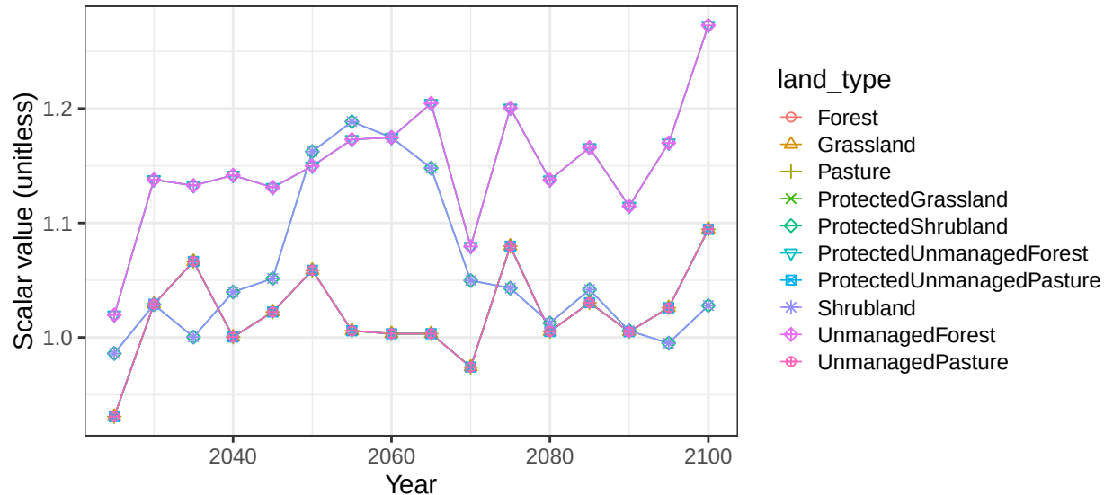
Region Mexico basin RioBalsas non-crop vegetation scalars
