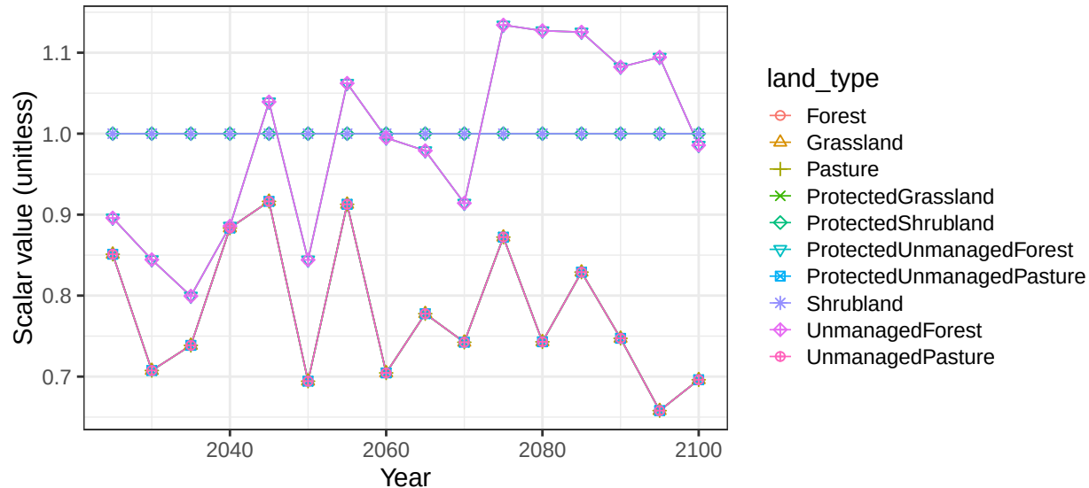
Region Mexico basin YucatanP non-crop vegetation scalars
