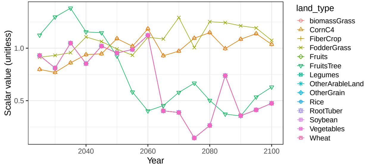
Region China basin IndusR crop vegetation scalars
