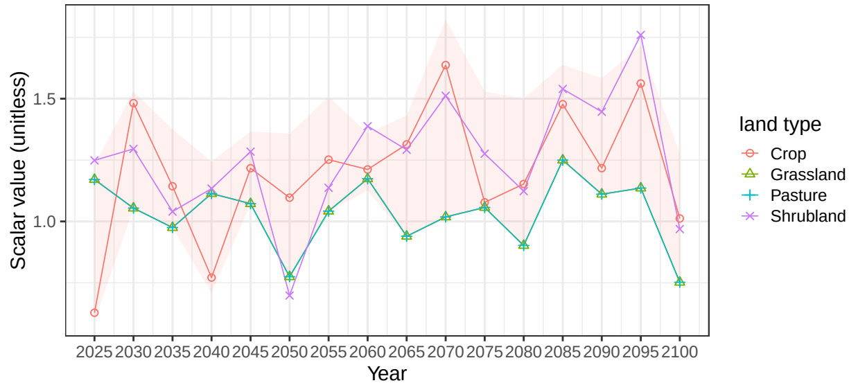
Region Australia_NZ basin AusInt average vegetation scalars
