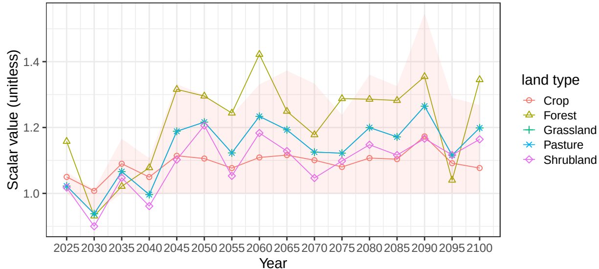
Region Russia basin Gobi average vegetation scalars
