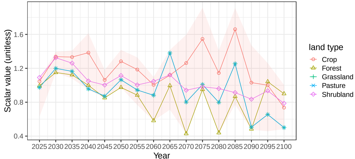
Region Argentina basin MarChiq average vegetation scalars
