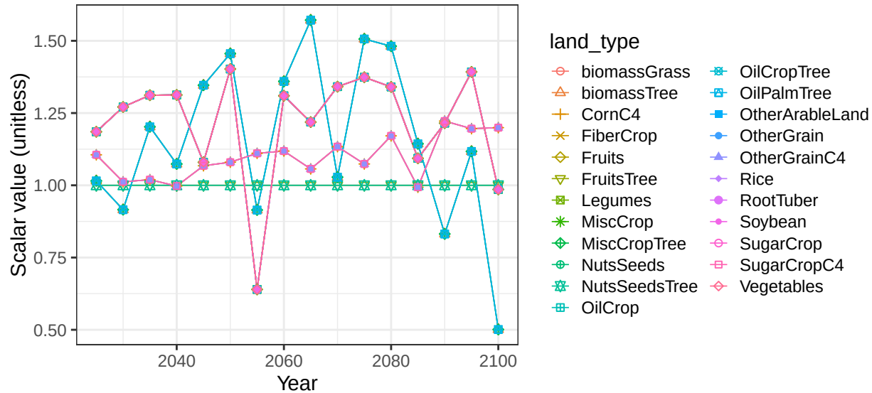
Region Africa_Western basin VoltaR crop vegetation scalars
