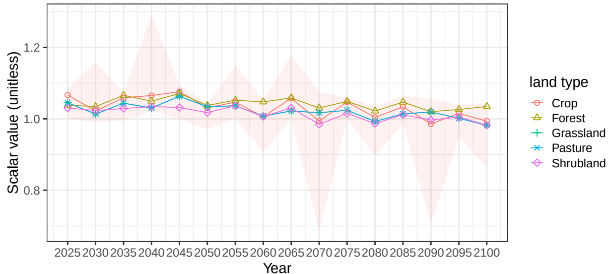
Region South America_Southern basin ChileCstS average soil scalars
