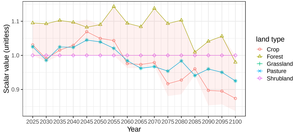
Region Africa_Western basin NigerR average soil scalars
