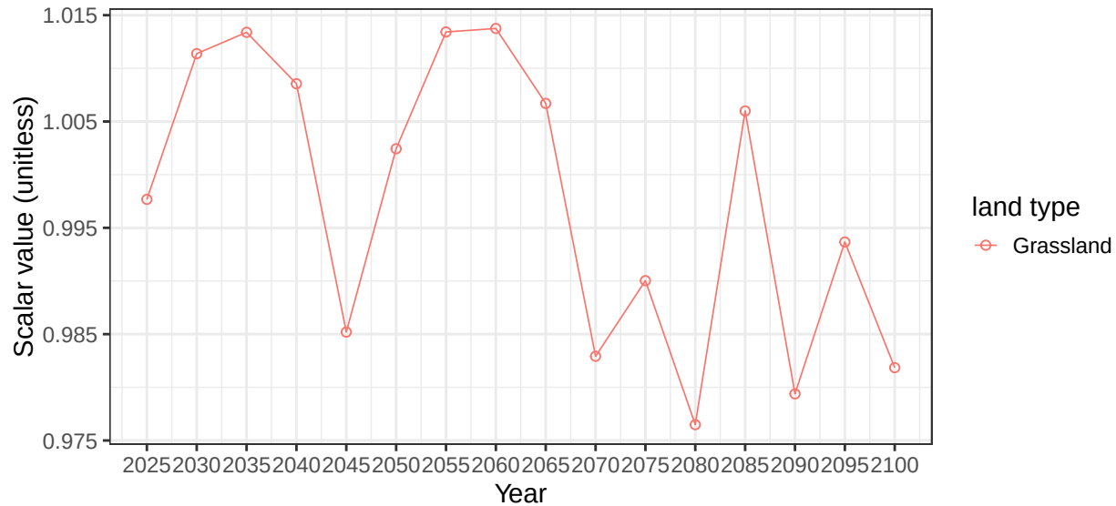
Region EU-15 basin ArgCstS average soil scalars
