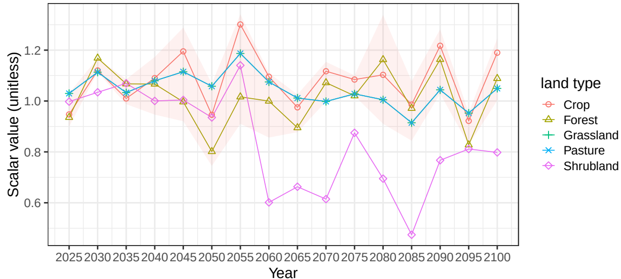
Region India basin SabarmatiR average soil scalars
