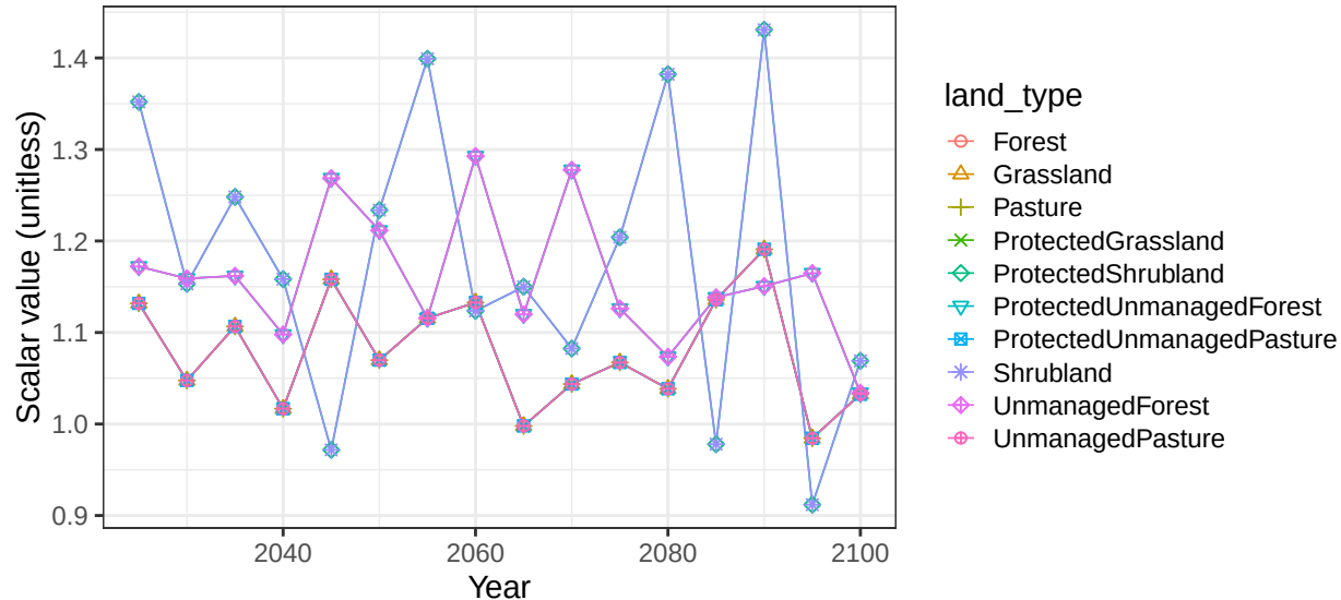
Region Africa_Southern basin AfrCstSE non-crop soil scalars
