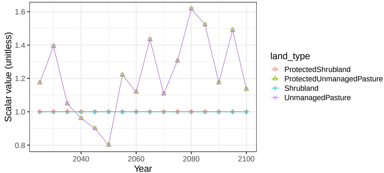
Region EU-15 basin MeditE non-crop vegetation scalars
