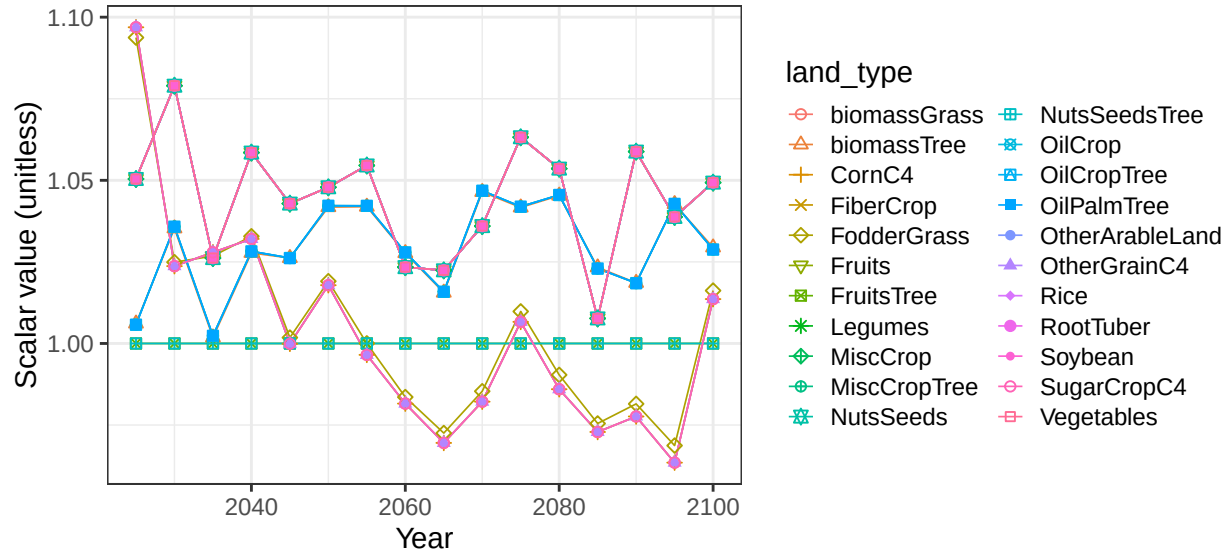
Region Southeast Asia basin Phlppns crop soil scalars
