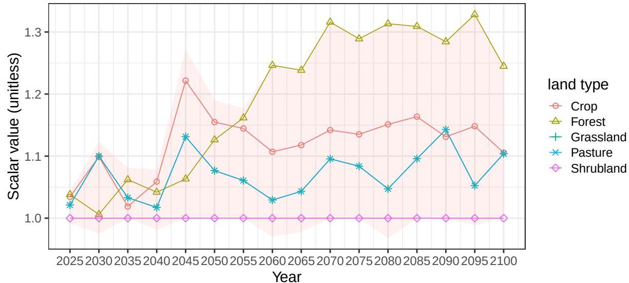
Region Southeast Asia basin Hong average vegetation scalars
