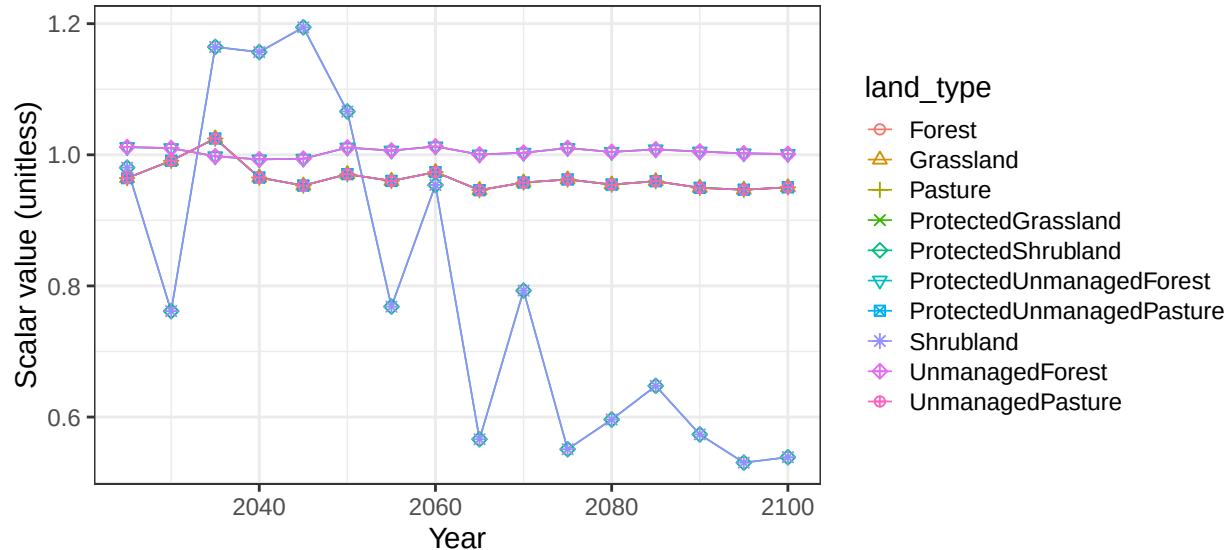
Region Colombia basin ColEcuacSt non-crop soil scalars
