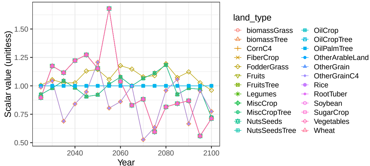
Region China basin ObR crop soil scalars
