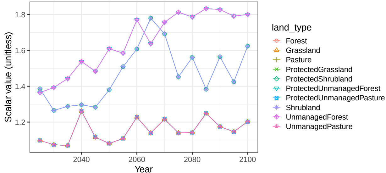
Region Brazil basin BrzCstE non-crop vegetation scalars
