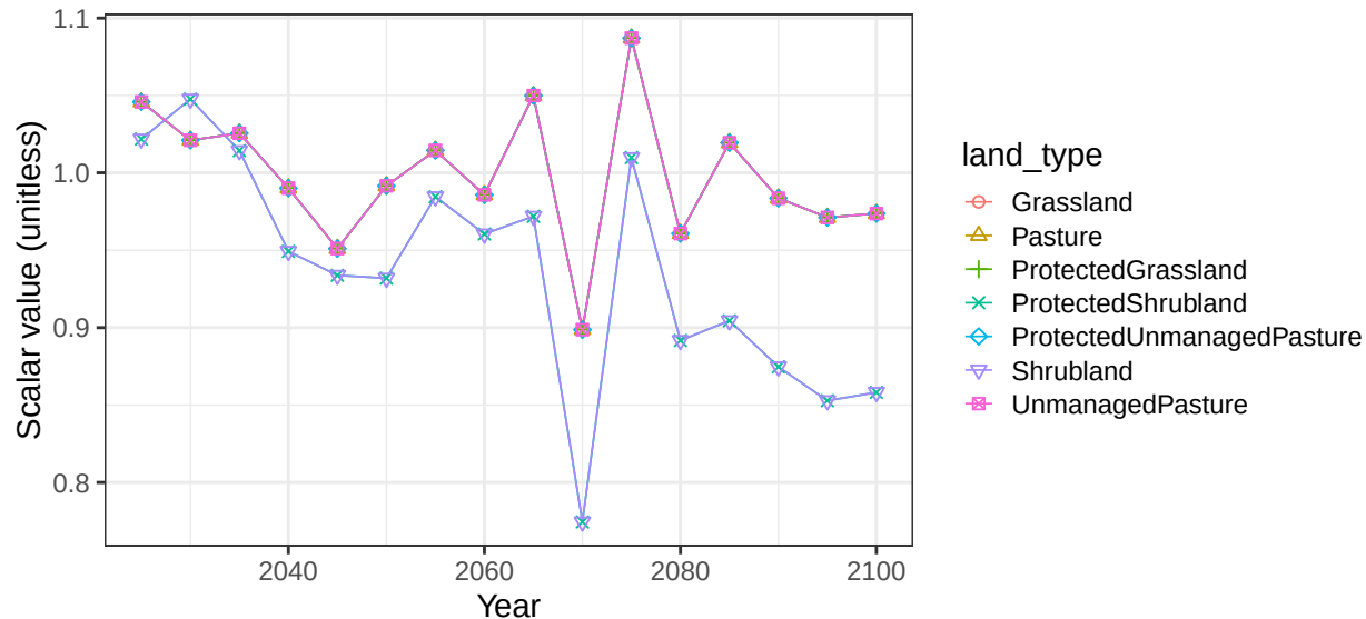
Region South Asia basin IndusR non-crop soil scalars
