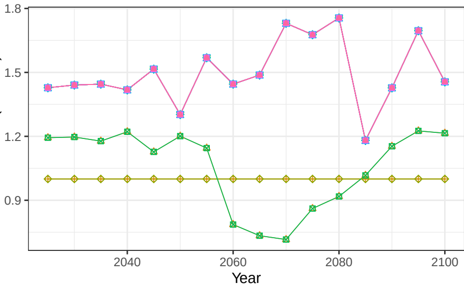
Region Canada basin NelsonR crop vegetation scalars
