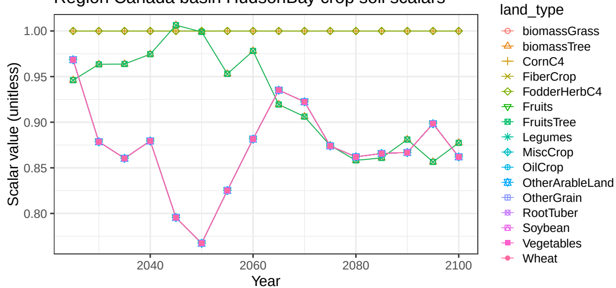
Region Canada basin HudsonBay crop soil scalars
