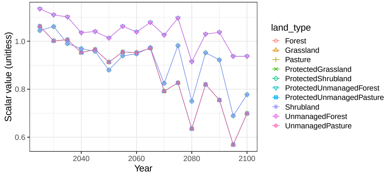
Region USA basin ArkWhtRedR non-crop soil scalars
