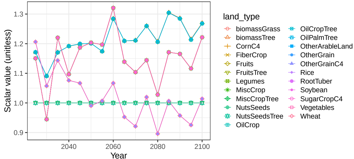
Region Africa_Southern basin CongoR crop vegetation scalars
