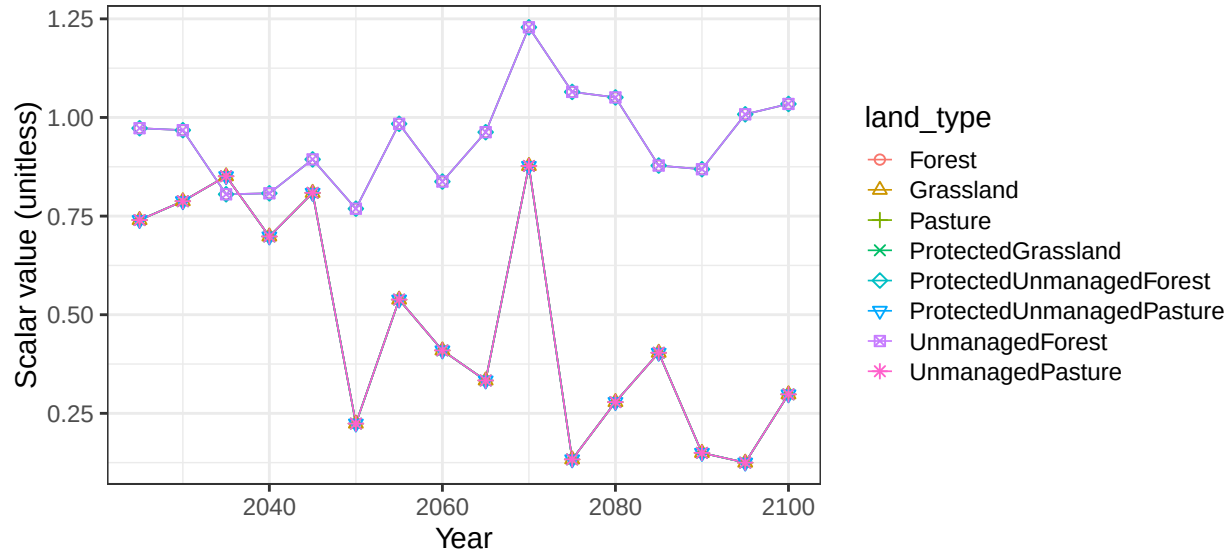
Region Europe_Eastern basin DonR non-crop vegetation scalars
