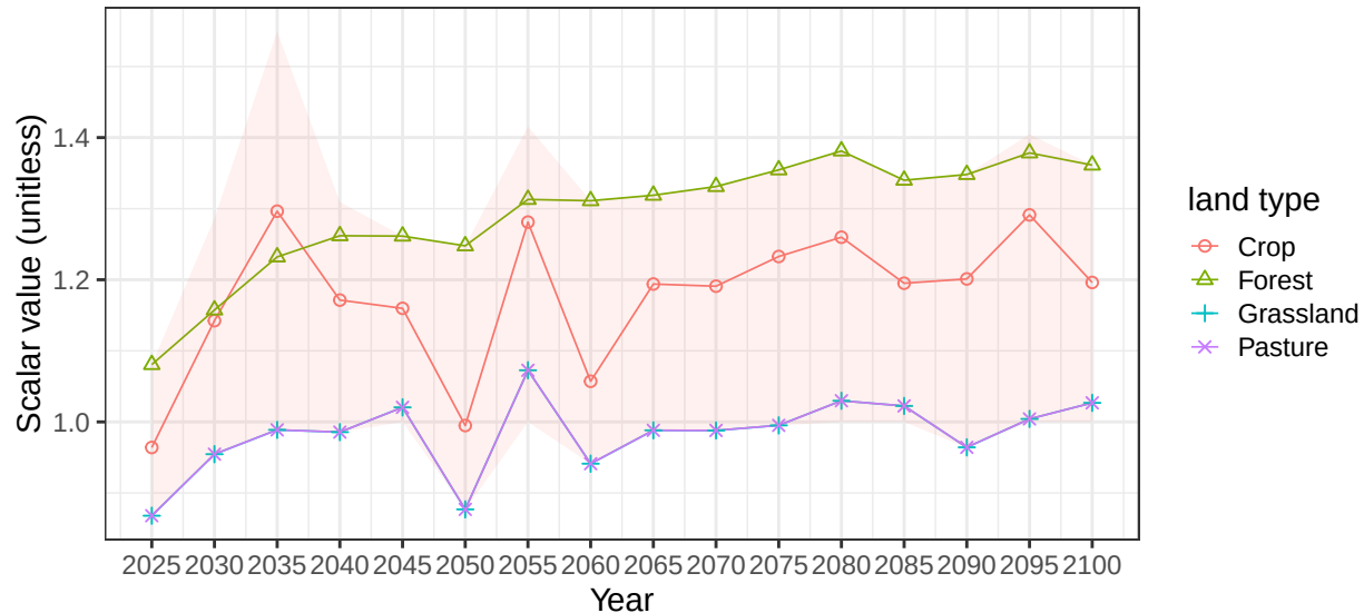
Region Africa_Southern basin GuineaGulf average vegetation scalars
