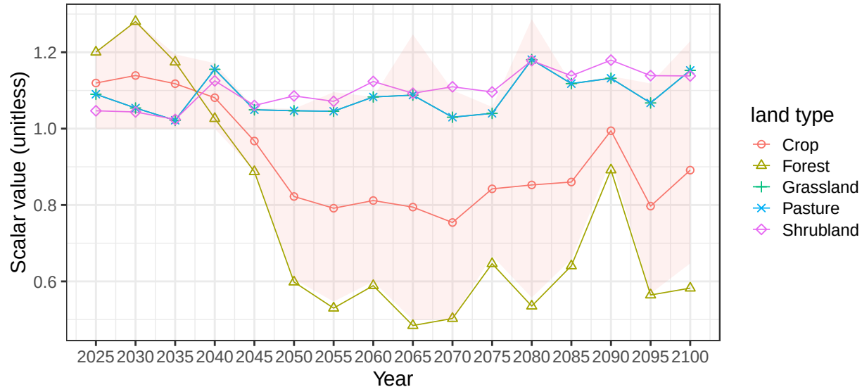
Region EU-15 basin RhoneR average vegetation scalars
