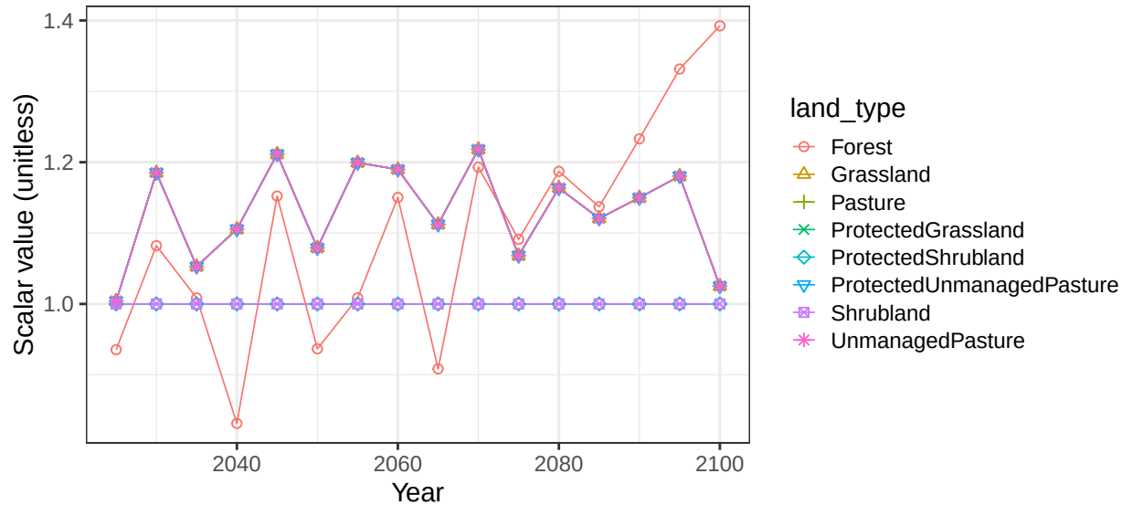
Region India basin IndCstE non-crop soil scalars
