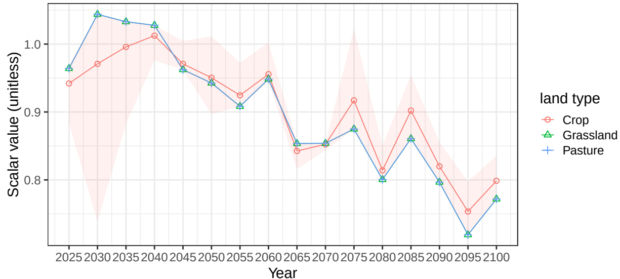
Region Argentina basin LaPuna average vegetation scalars
