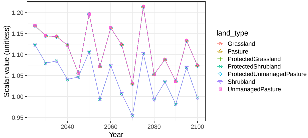
Region Middle East basin PersianGulf non-crop soil scalars
