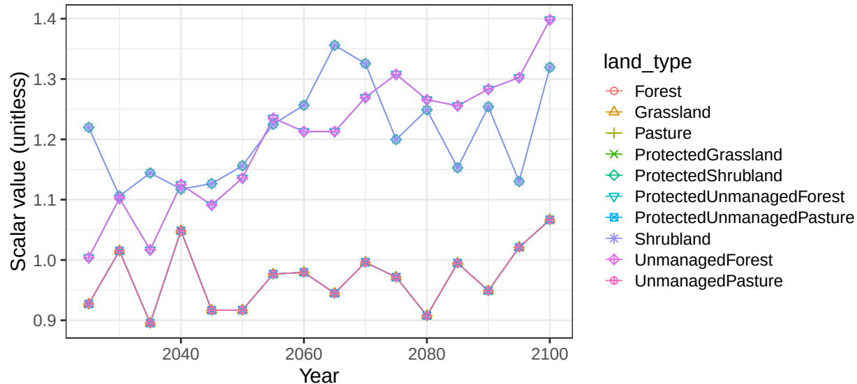
Region Brazil basin SaoFrancR non-crop soil scalars
