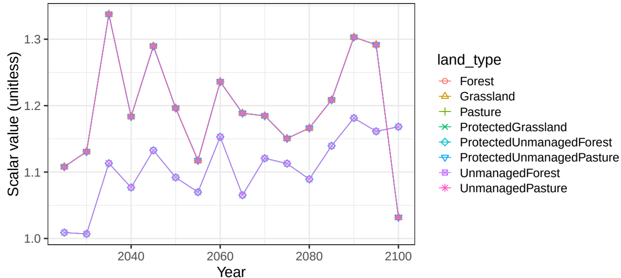
Region Southeast Asia basin BoHai non-crop vegetation scalars
