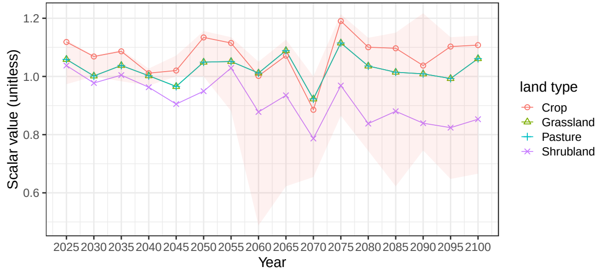
Region South Asia basin Helmand average soil scalars
