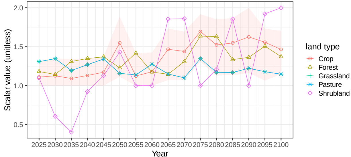
Region Mexico basin MexBaja average vegetation scalars
