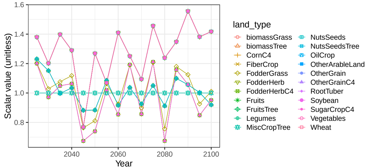
Region USA basin RioGrande crop vegetation scalars
