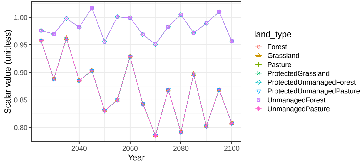
Region Indonesia basin JavaTimor non-crop soil scalars
