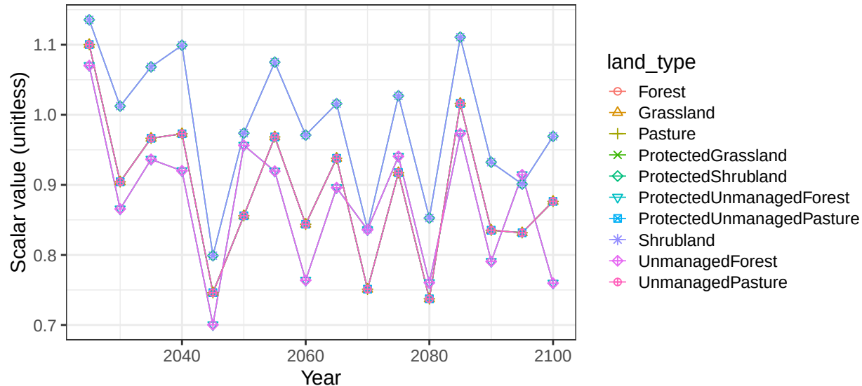
Region Mexico basin RioGrande non-crop soil scalars
