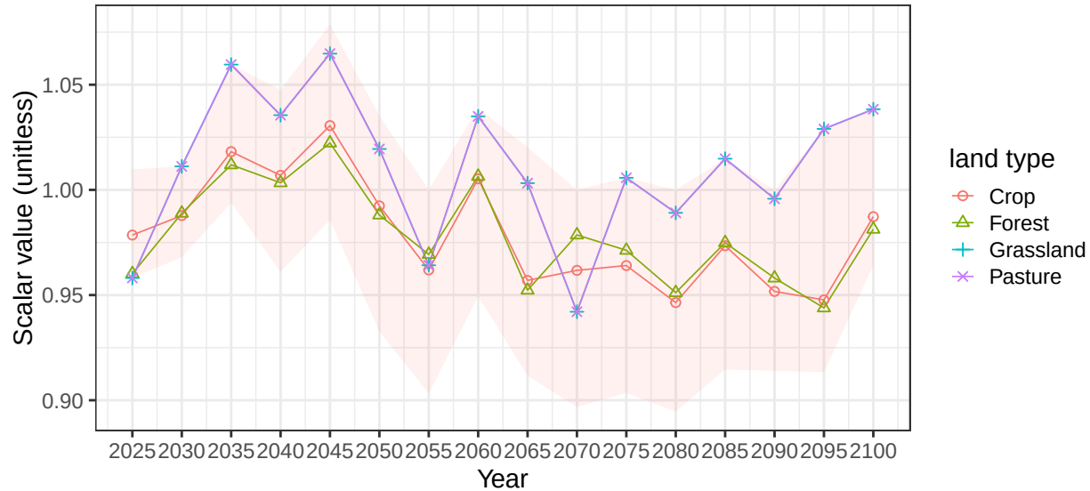
Region China basin RusCstSE average soil scalars
