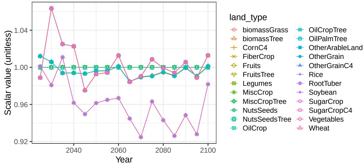
Region Colombia basin AmazonR crop soil scalars
