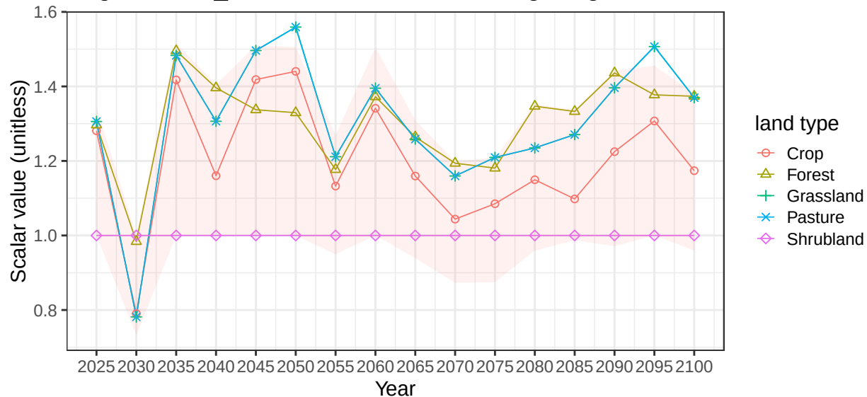
Region Africa_Southern basin NileR average vegetation scalars
