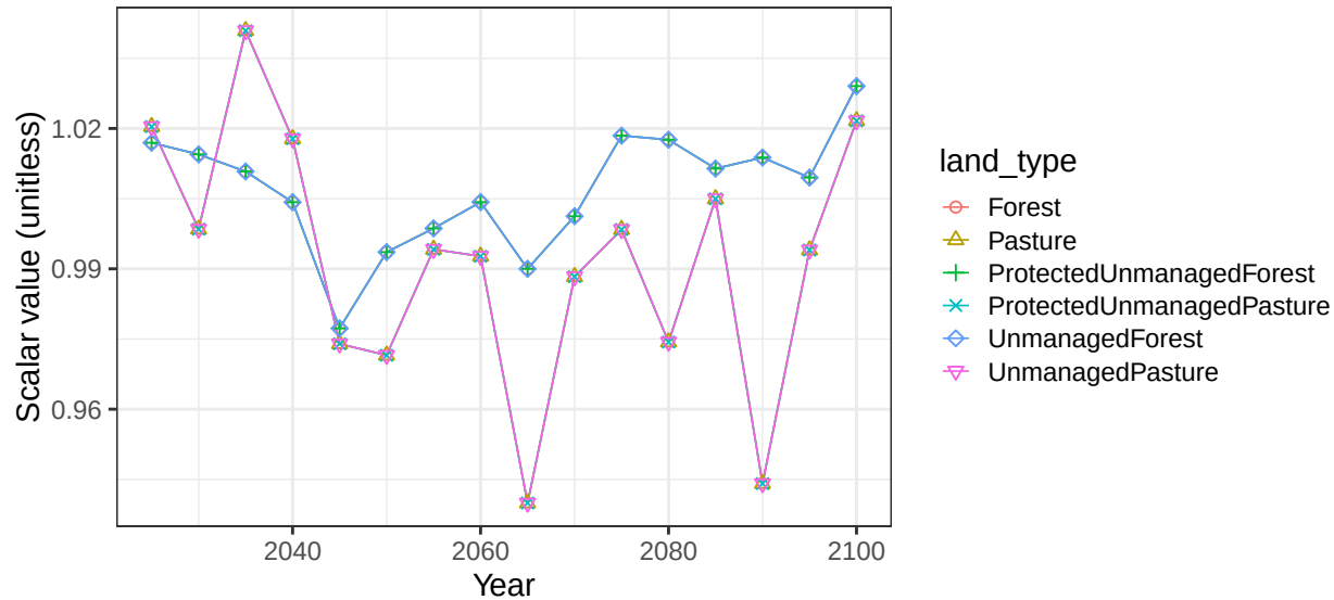
Region Indonesia basin FlyR non-crop soil scalars
