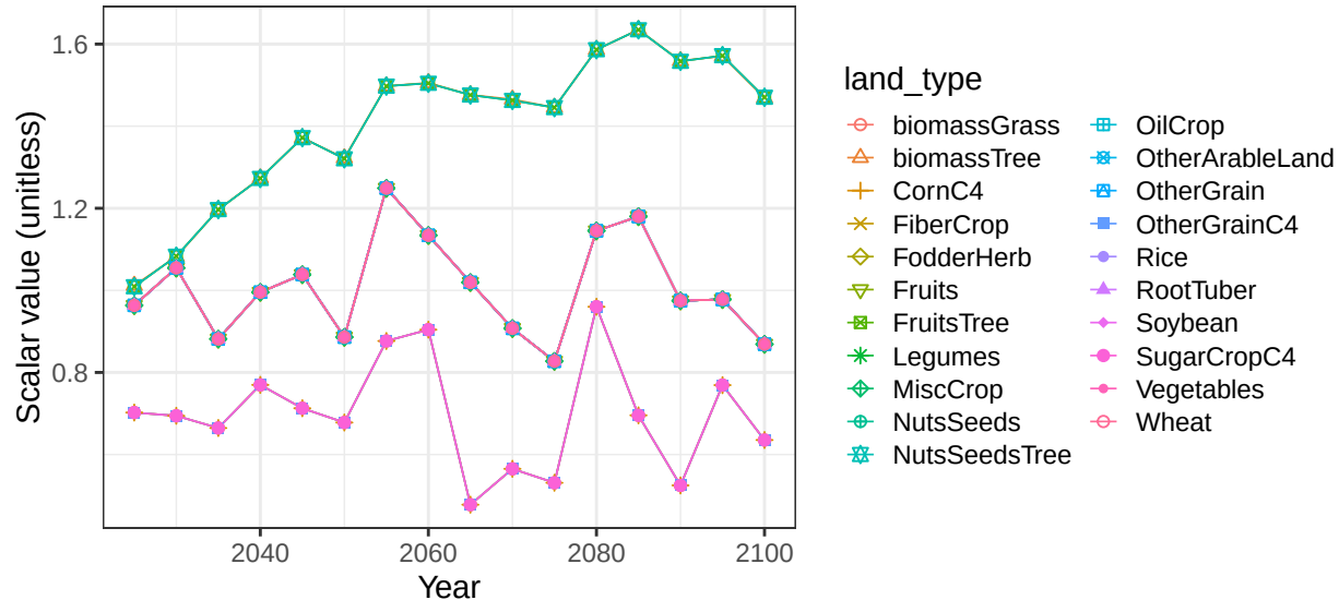
Region South Africa basin OrangeR crop vegetation scalars
