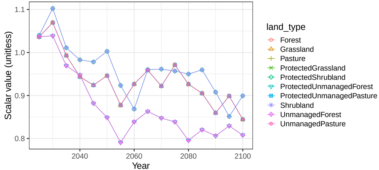
Region USA basin GreatBasin non-crop soil scalars
