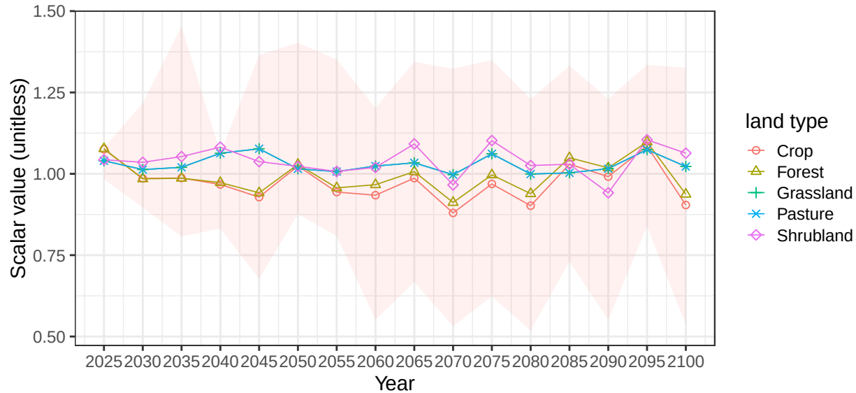
Region Argentina basin Patagonia average soil scalars
