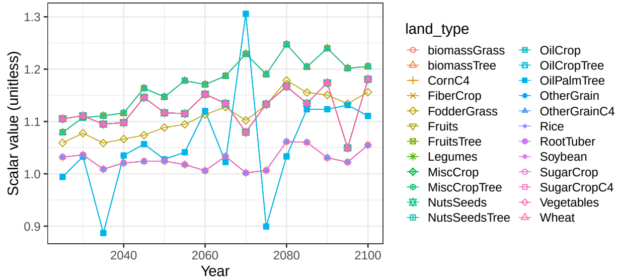
Region China basin Yangtze crop vegetation scalars
