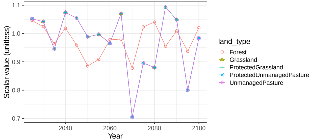
Region EU-15 basin LoireR non-crop vegetation scalars
