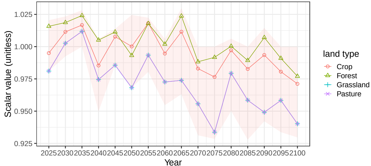
Region Australia_NZ basin NewZealand average soil scalars
