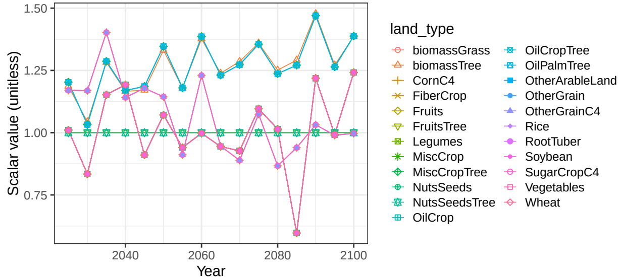
Region Africa_Southern basin RiftValley crop vegetation scalars
