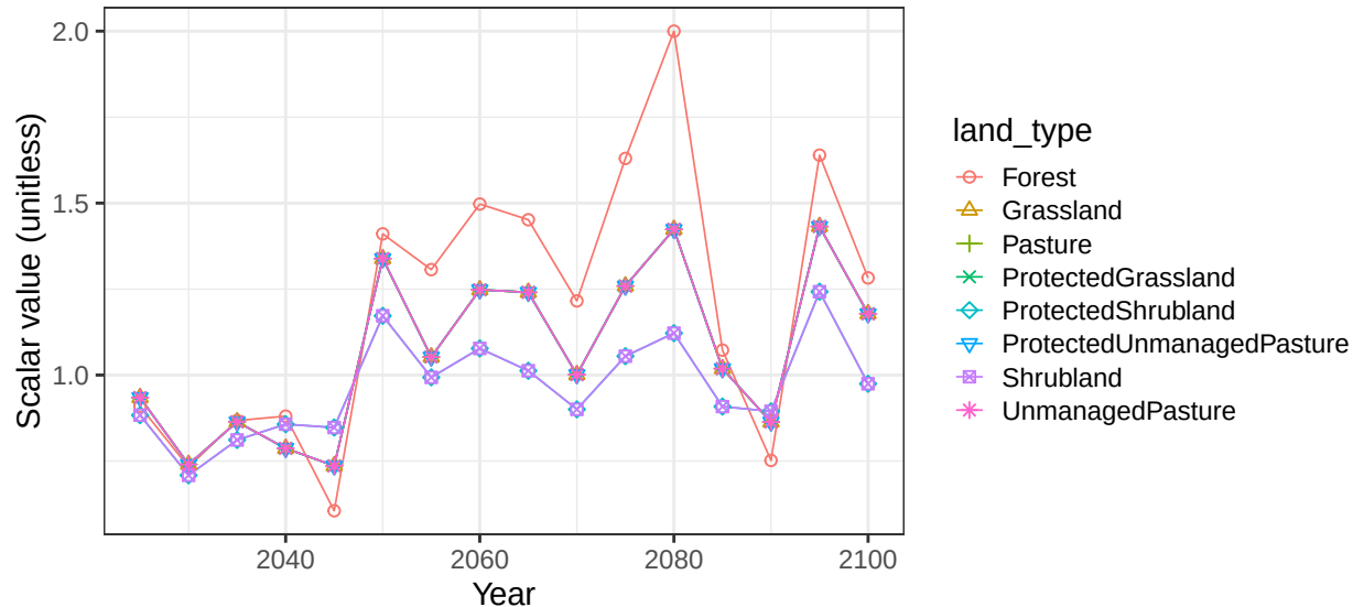
Region China basin LBalkash non-crop vegetation scalars
