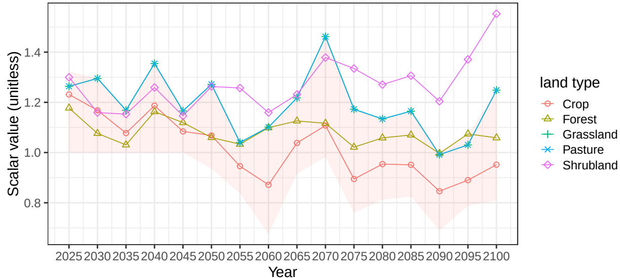
Region EU-15 basin IberiaCst average vegetation scalars
