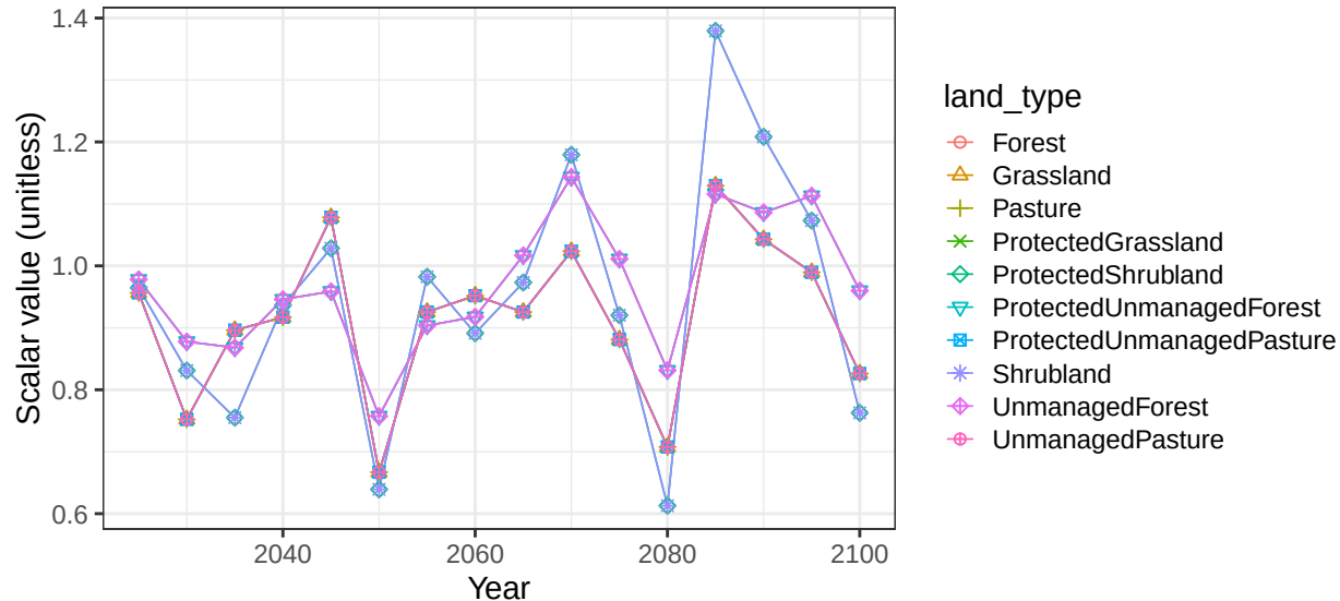
Region Australia_NZ basin AusCstE non-crop vegetation scalars
