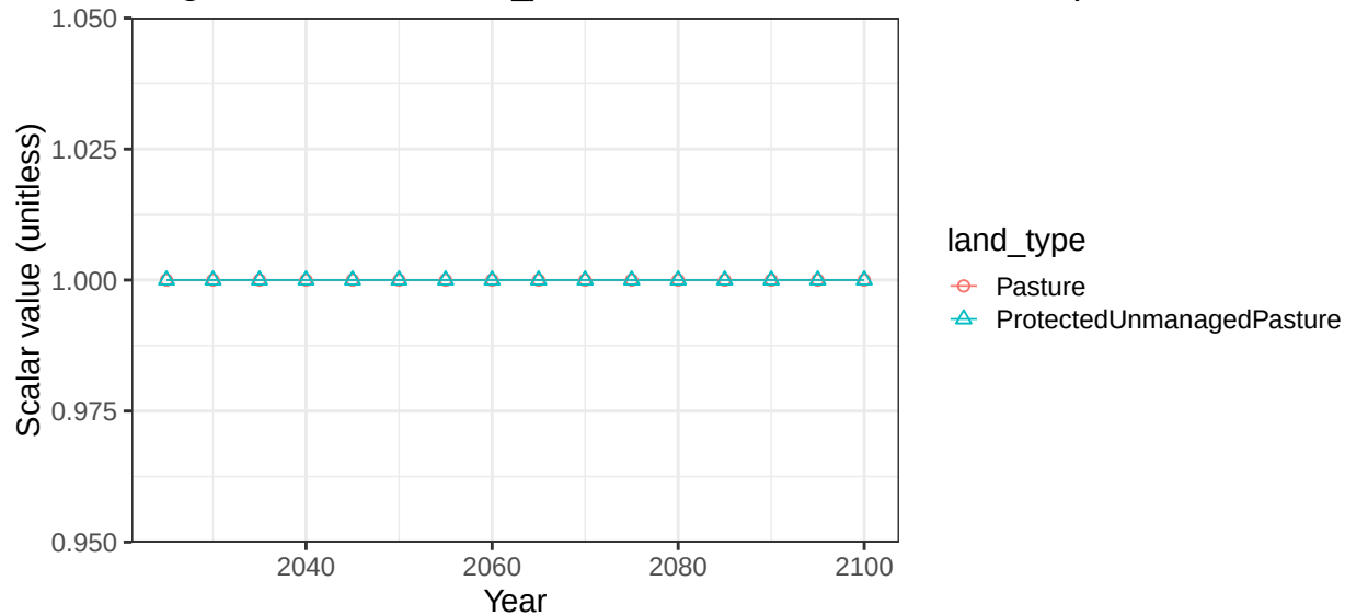
Region South America_Southern basin Salinas non-crop soil scalars
