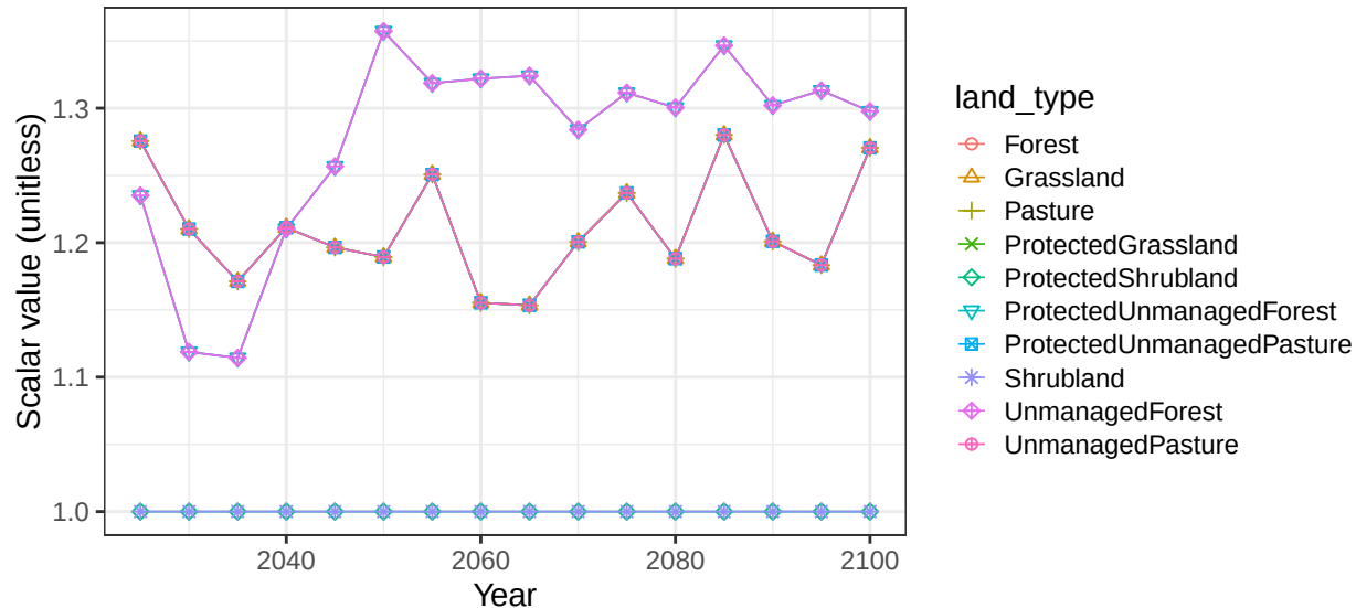
Region Africa_Southern basin AngolaCst non-crop vegetation scalars
