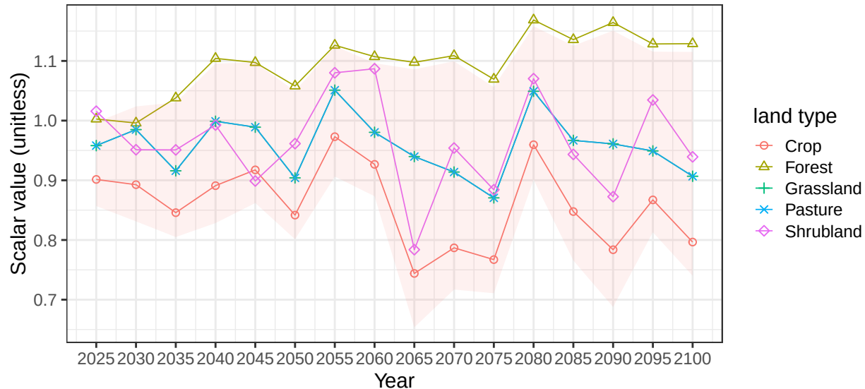
Region South Africa basin OrangeR average soil scalars
