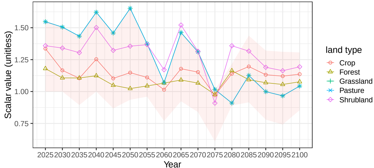
Region EU-15 basin GuadianaR average vegetation scalars
