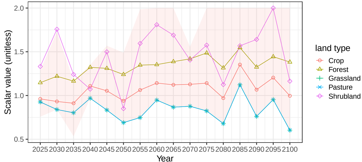
Region Australia_NZ basin AusCstN average vegetation scalars
