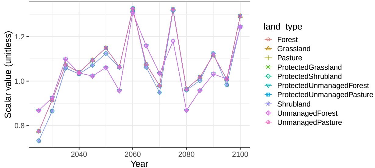
Region Russia basin ScndnvN non-crop vegetation scalars
