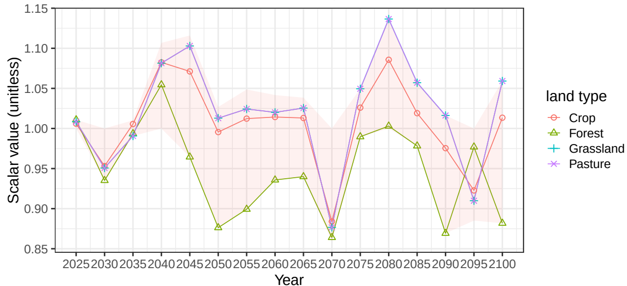
Region EU-15 basin SeineR average soil scalars
