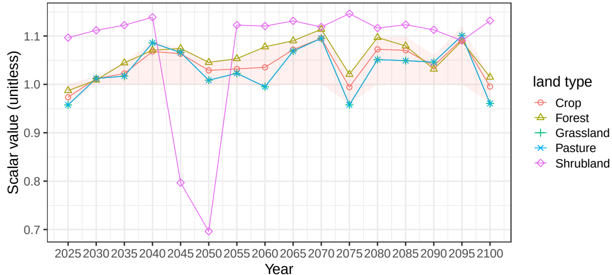
Region South America_Northern basin SAmersCstN average soil scalars
