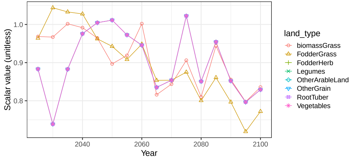
Region Argentina basin LaPuna crop vegetation scalars
