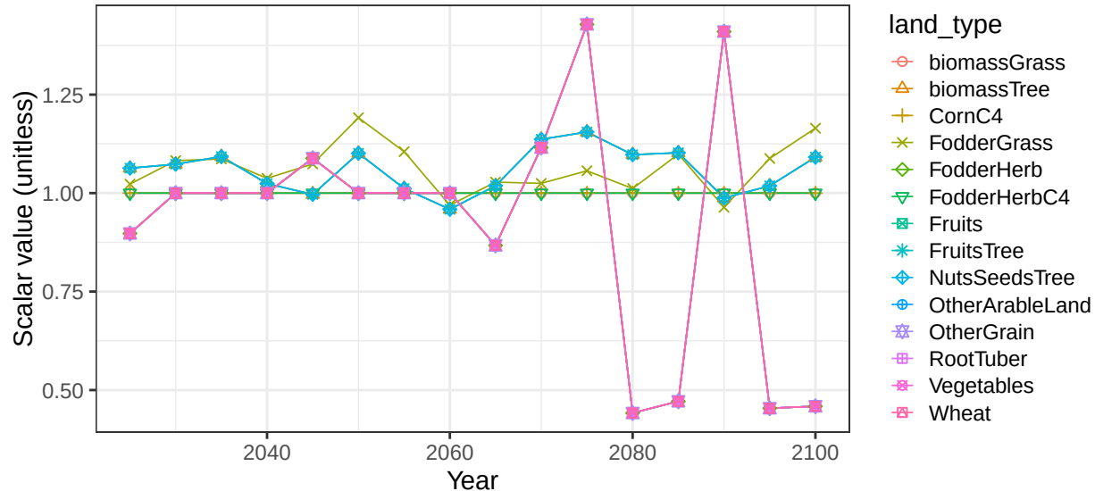
Region USA basin FraserR crop soil scalars
