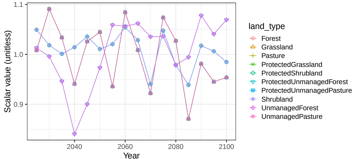
Region Europe_Non_EU basin TigrEuphR non-crop soil scalars
