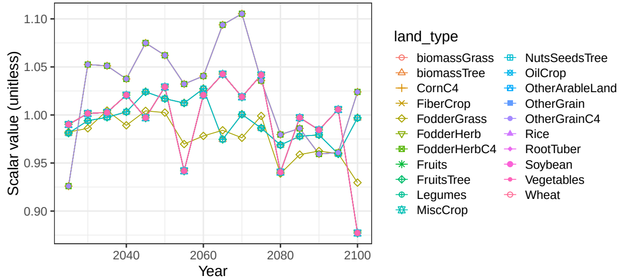
Region Russia basin AmurR crop soil scalars
