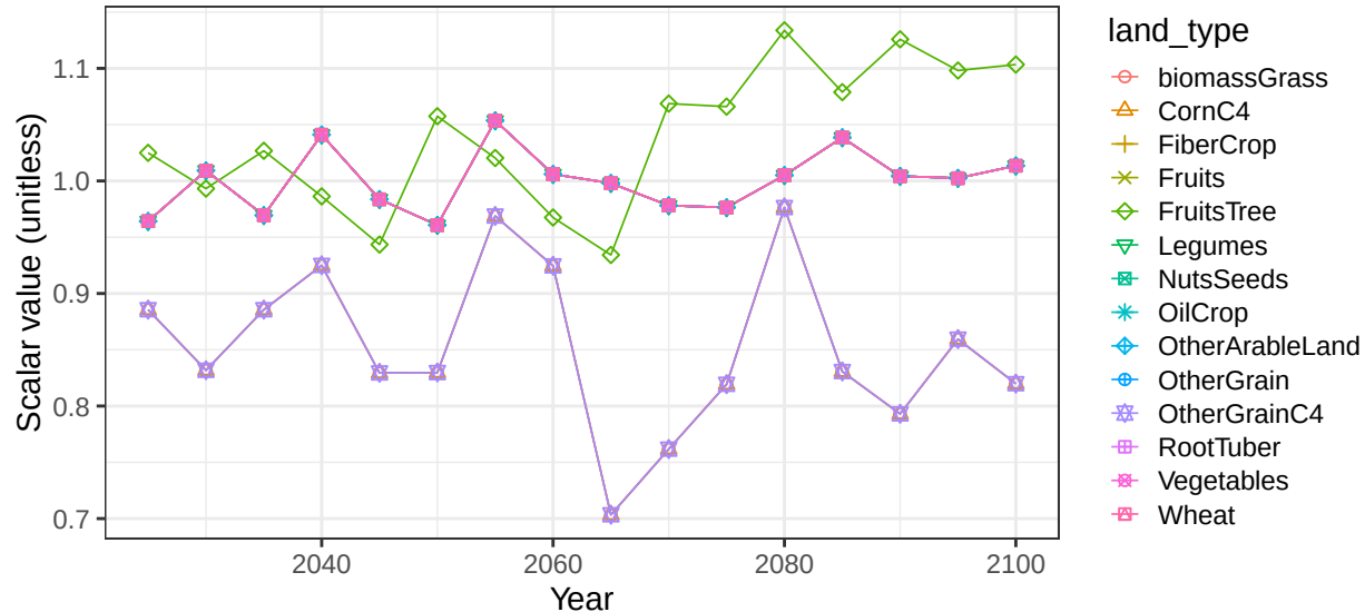
Region Africa_Southern basin OrangeR crop soil scalars
