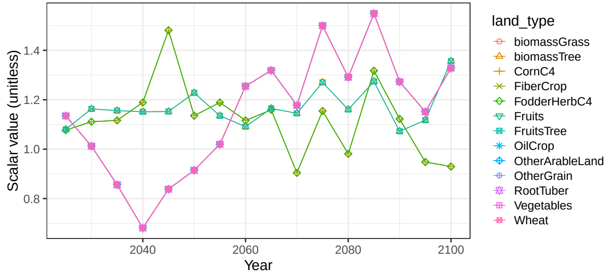
Region Canada basin FraserR crop vegetation scalars
