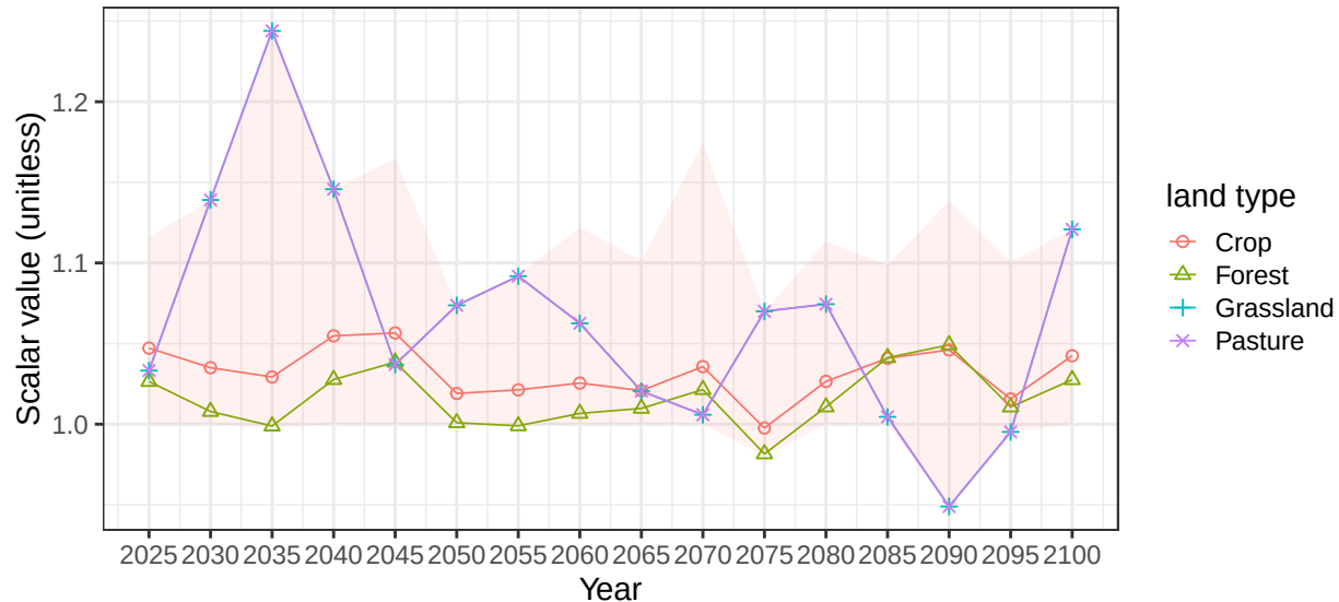
Region Indonesia basin BorneoCstN average vegetation scalars
