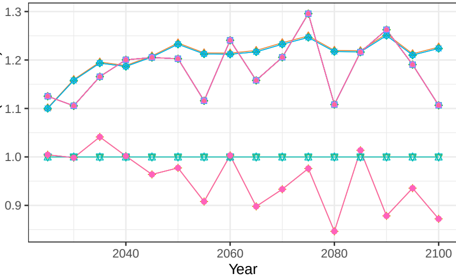
Region Indonesia basin IdnE crop vegetation scalars
