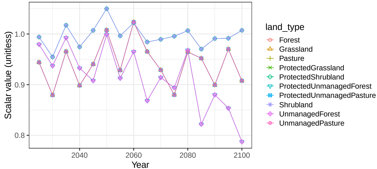
Region Central Asia basin Gobi non-crop soil scalars
