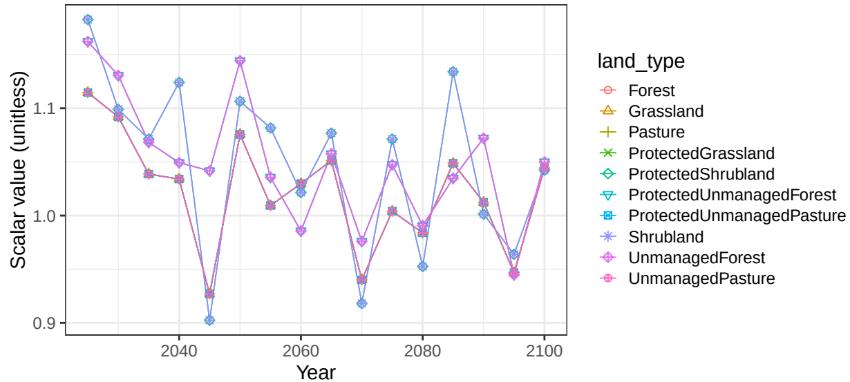
Region Mexico basin MexInt non-crop soil scalars
