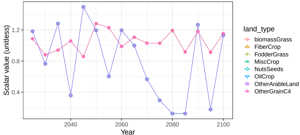
Region Africa_Eastern basin AfrIntN crop vegetation scalars
