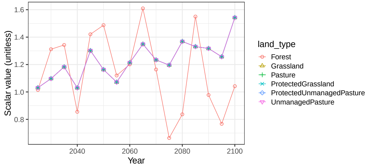
Region India basin BengalW non-crop vegetation scalars
