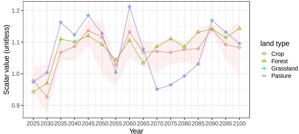
Region Southeast Asia basin RusCstSE average vegetation scalars
