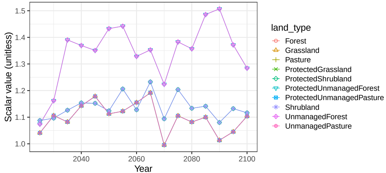
Region South America_Southern basin ChileCstN non-crop vegetation sca
