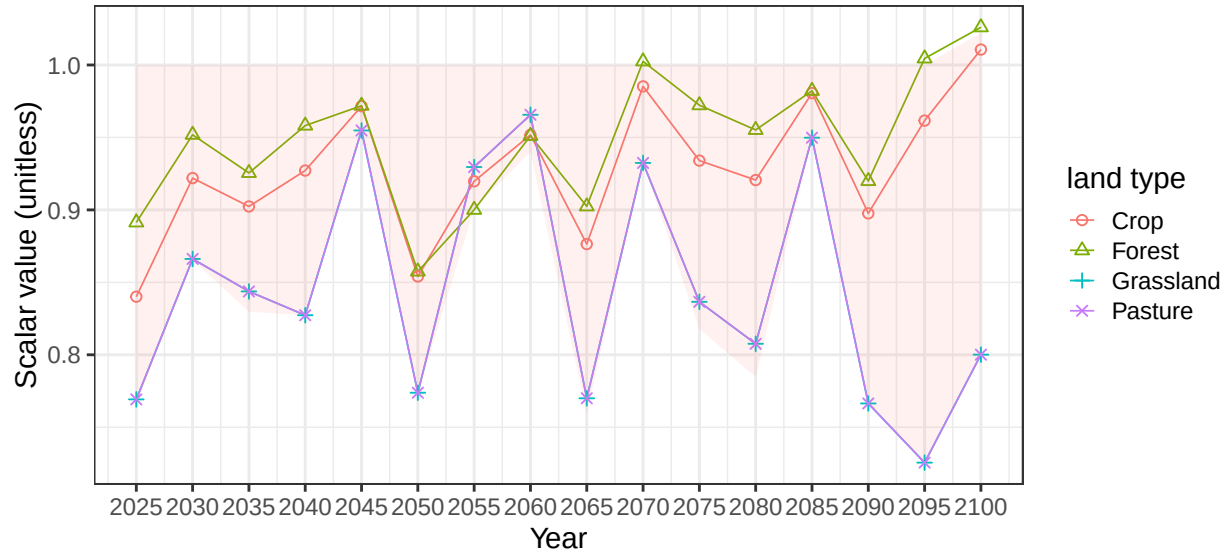
Region Europe_Eastern basin DaugavaR average soil scalars
