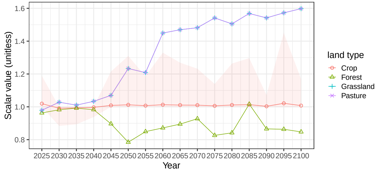
Region EU-15 basin NevaR average soil scalars
