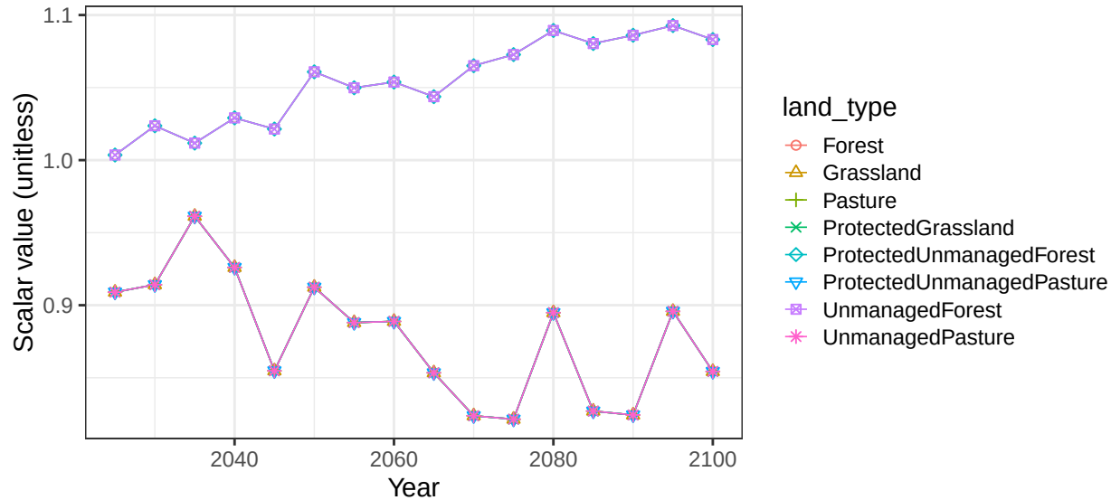
Region Indonesia basin Sumatra non-crop vegetation scalars
