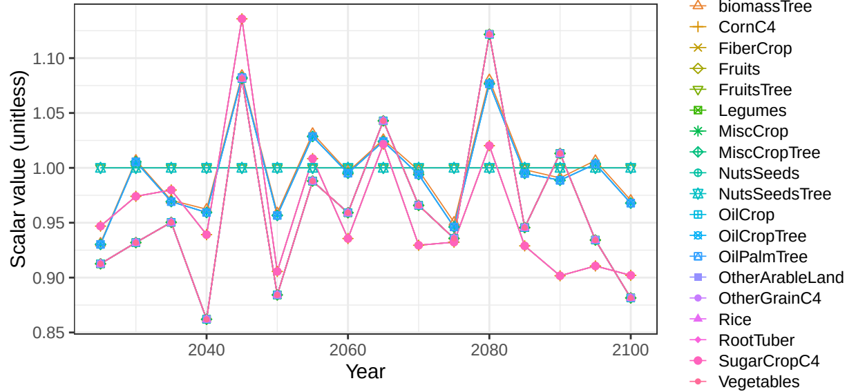
Region Central America and Caribbean basin Caribbean crop soil scalars
