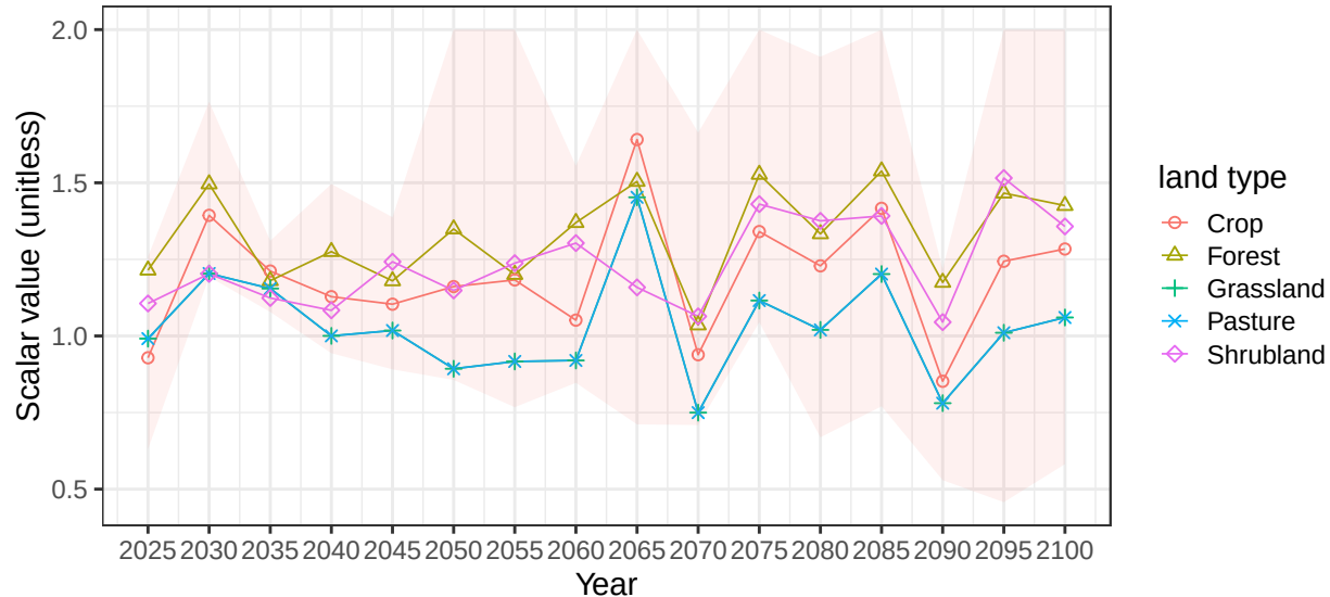
Region Argentina basin Salinas average vegetation scalars
