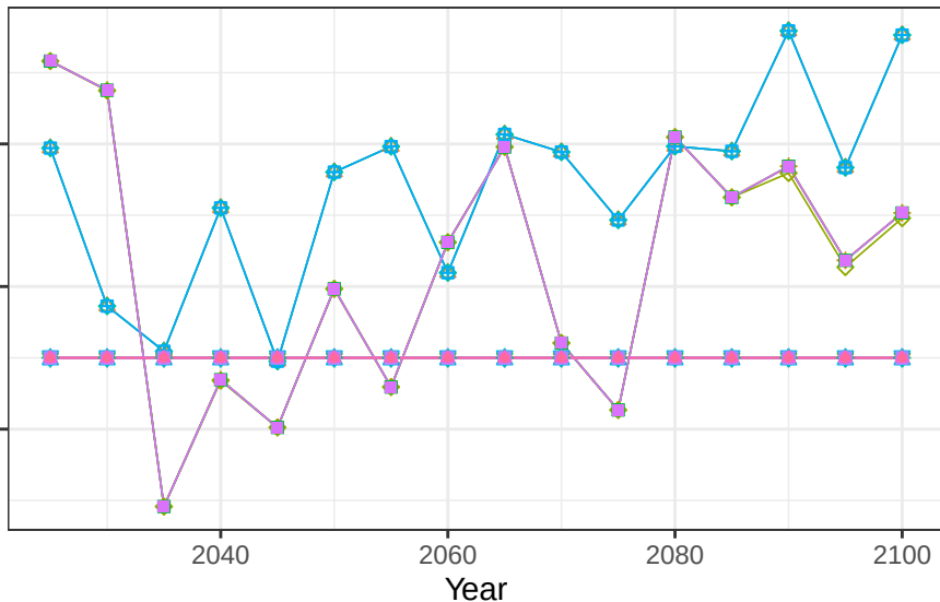
Region USA basin MexCstNW crop vegetation scalars
