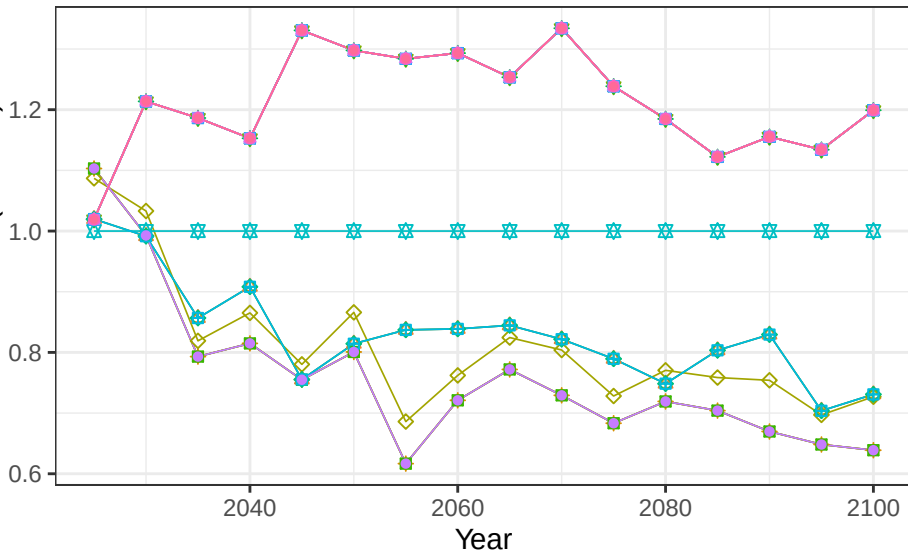
Region USA basin UsaColoRS crop soil scalars
