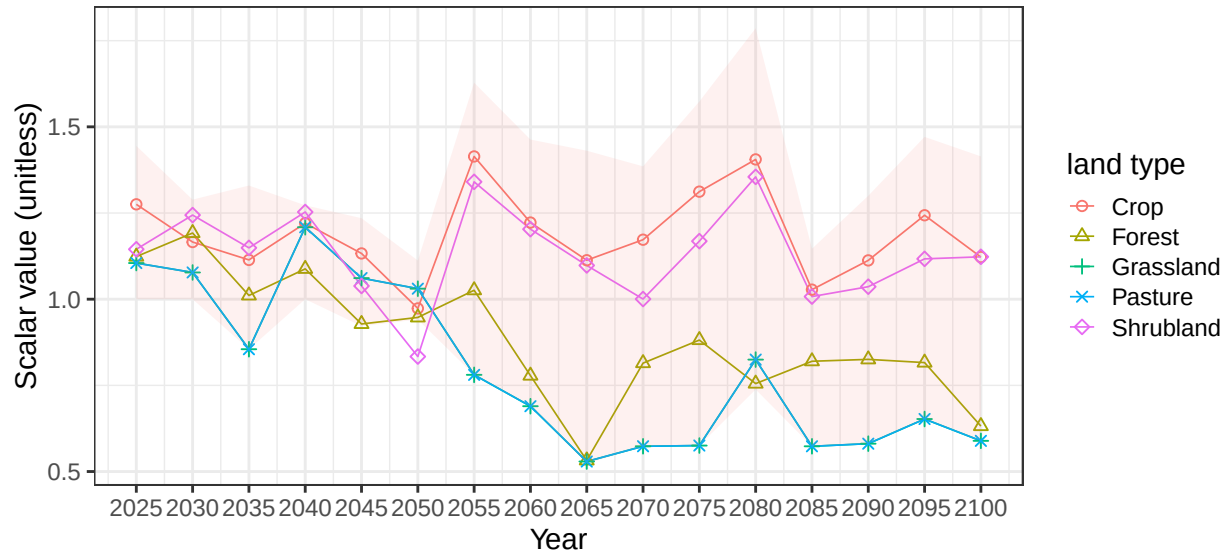
Region EU-12 basin AdrBlkSea average vegetation scalars
