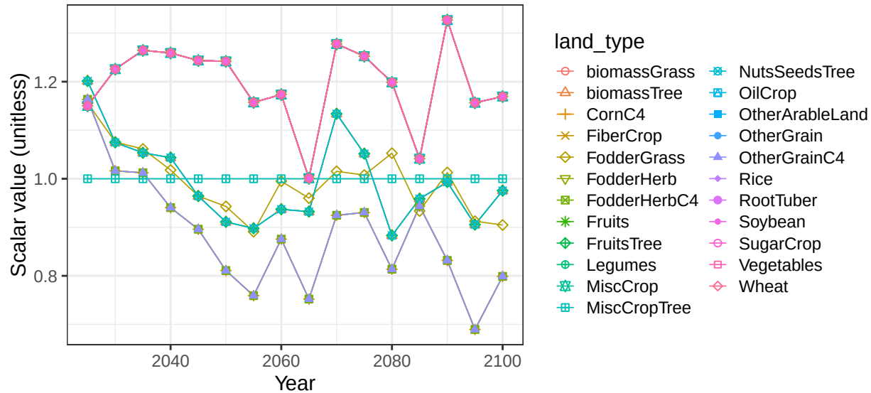
Region USA basin MissppRN crop soil scalars
