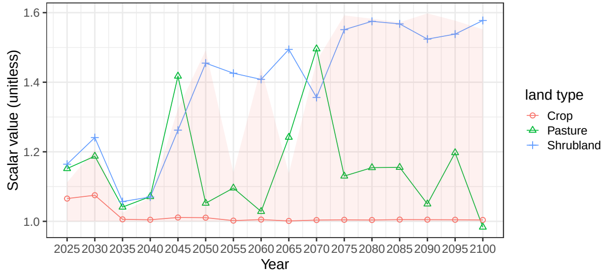
Region South Asia basin HamuMashR average soil scalars
