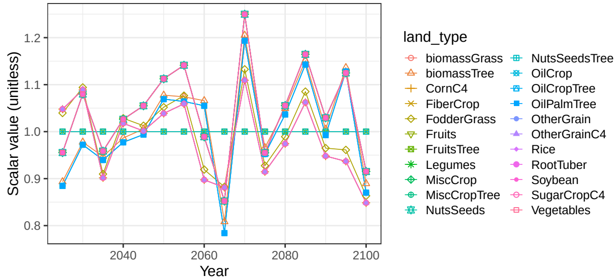
Region China basin Hainan crop vegetation scalars
