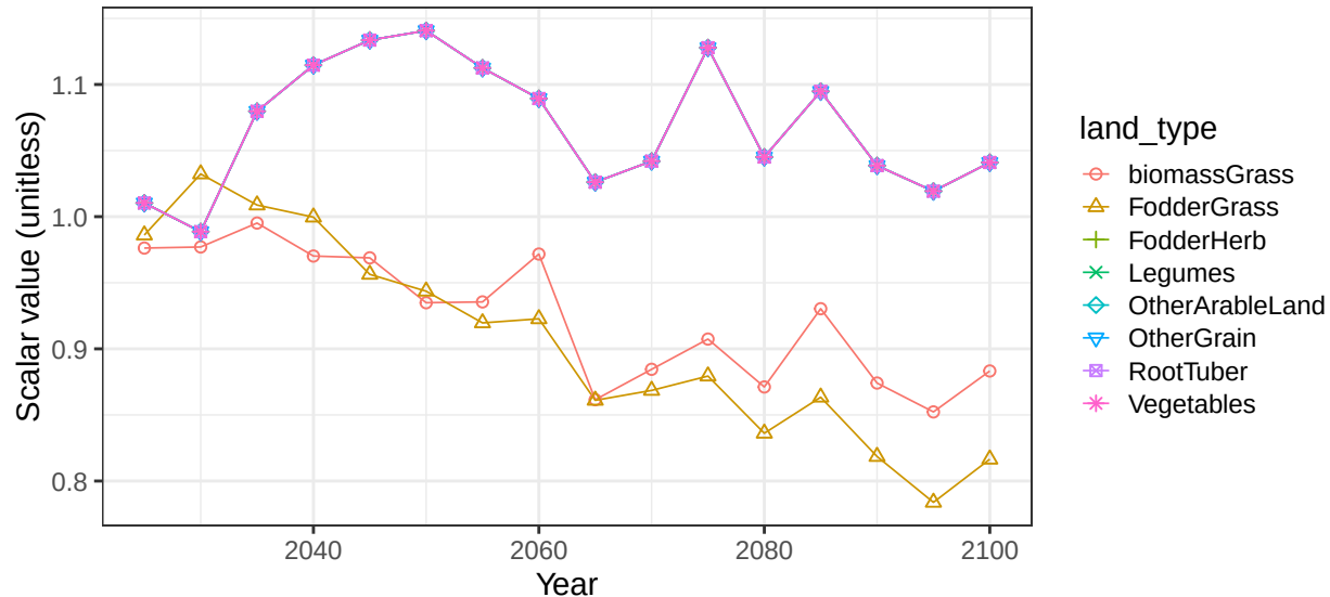
Region Argentina basin LaPuna crop soil scalars
