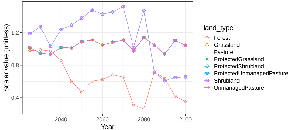
Region Africa_Eastern basin Madagascar non-crop vegetation scalars
