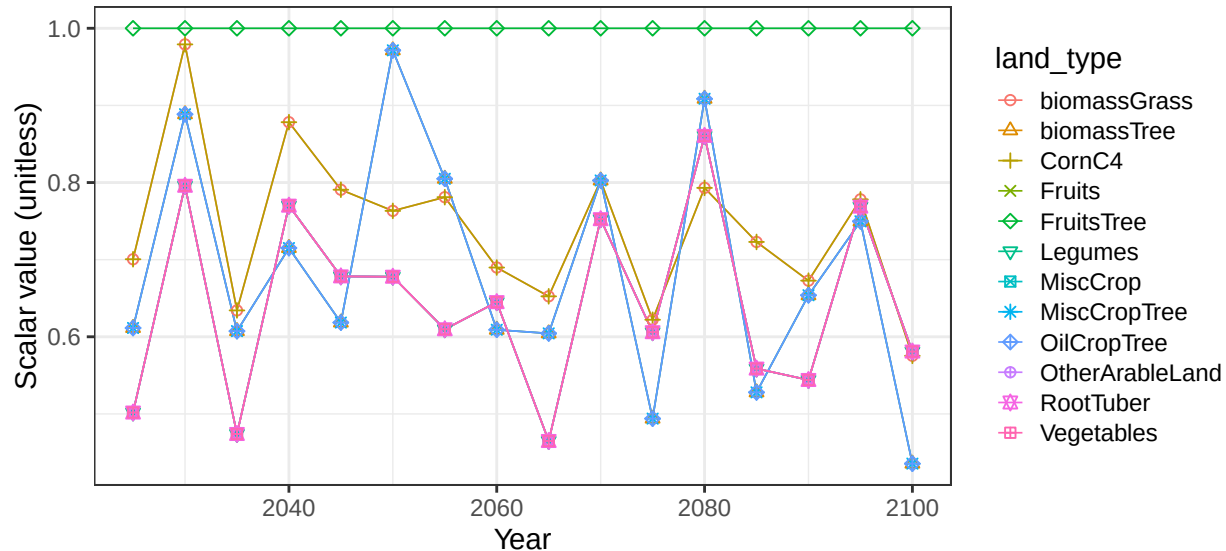
Region USA basin Caribbean crop vegetation scalars
