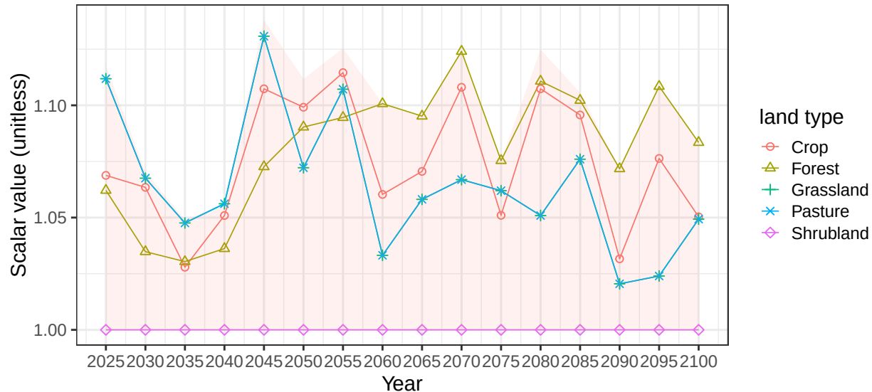
Region Southeast Asia basin VietnamCst average soil scalars
