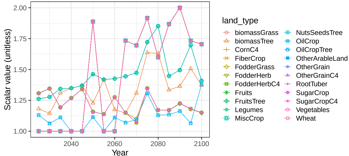
Region Mexico basin MexBaja crop vegetation scalars
