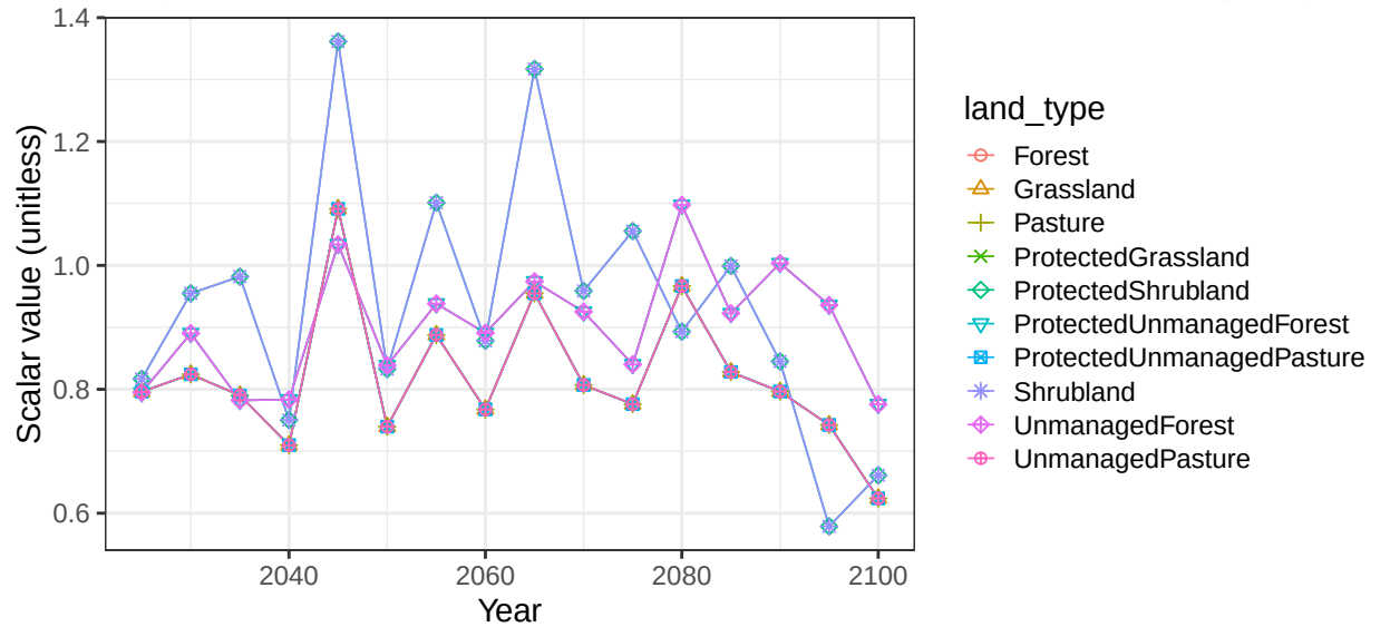
Region Central America and Caribbean basin Caribbean non-crop vegetati
