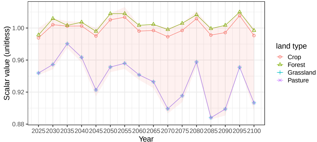
Region Indonesia basin Sumatra average soil scalars
