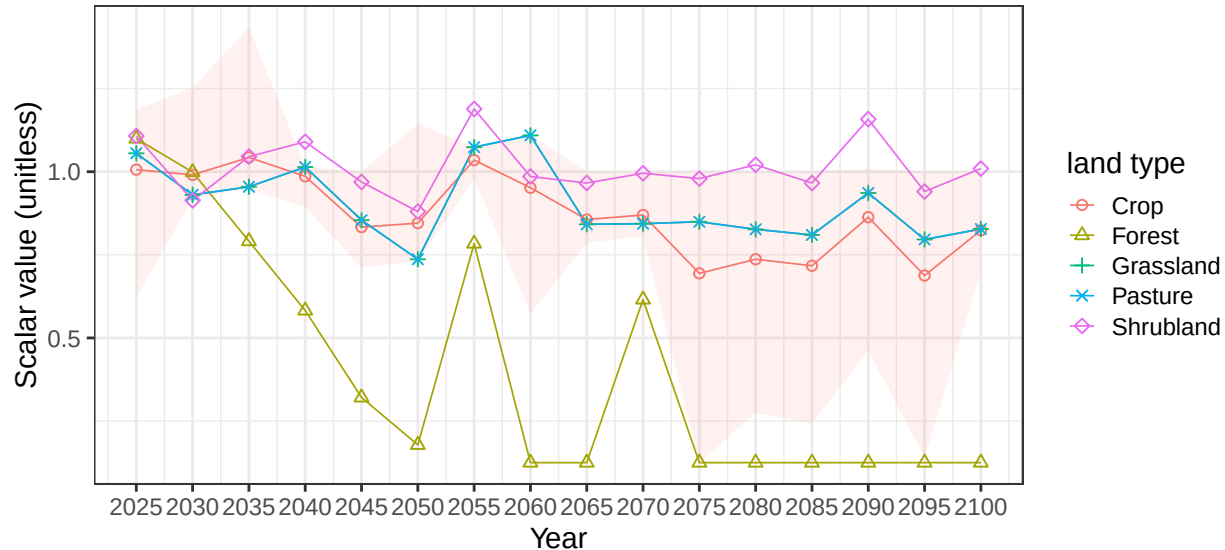
Region EU-15 basin TiberR average vegetation scalars
