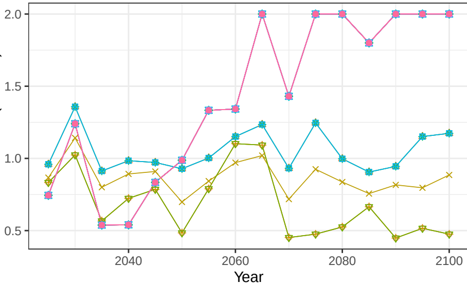
Region Central Asia basin BlackSeaS crop vegetation scalars
