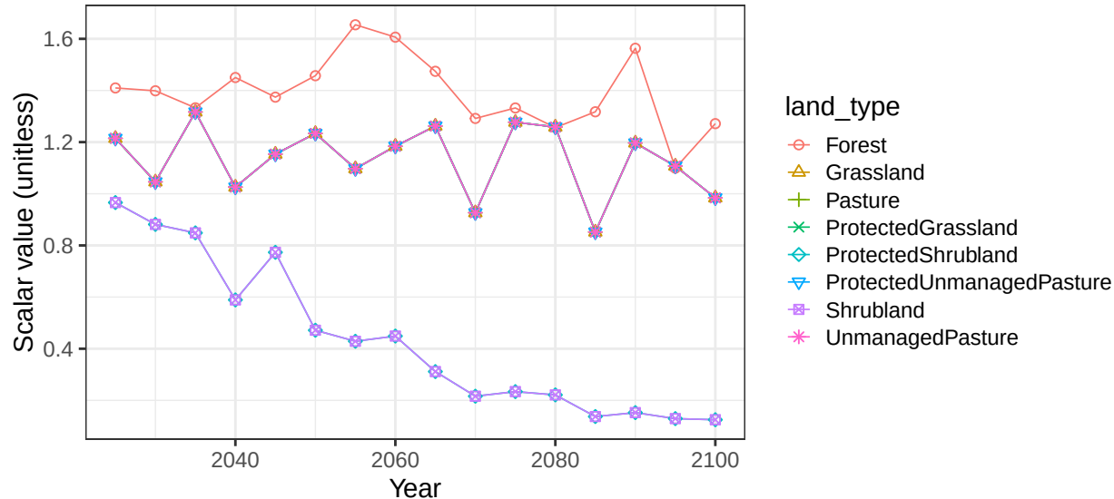
Region Africa_Eastern basin ShebJubR non-crop vegetation scalars
