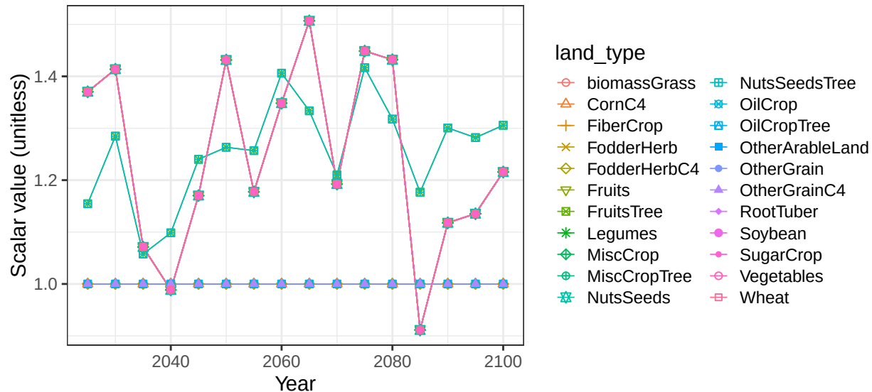
Region Europe_Non_EU basin EJrdrnSyr crop vegetation scalars
