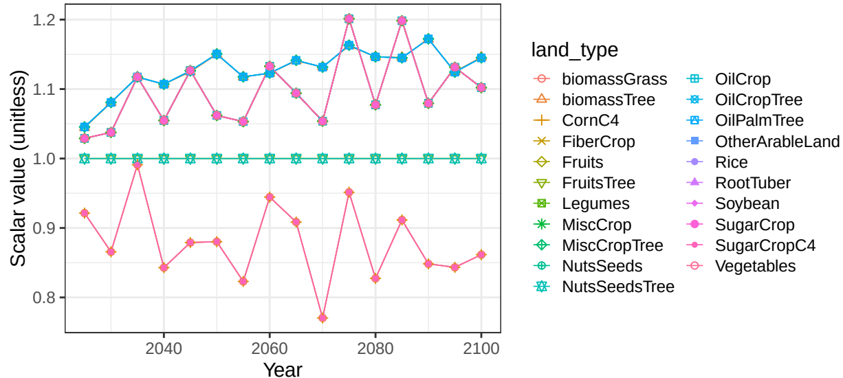
Region Indonesia basin Sulawesi crop vegetation scalars
