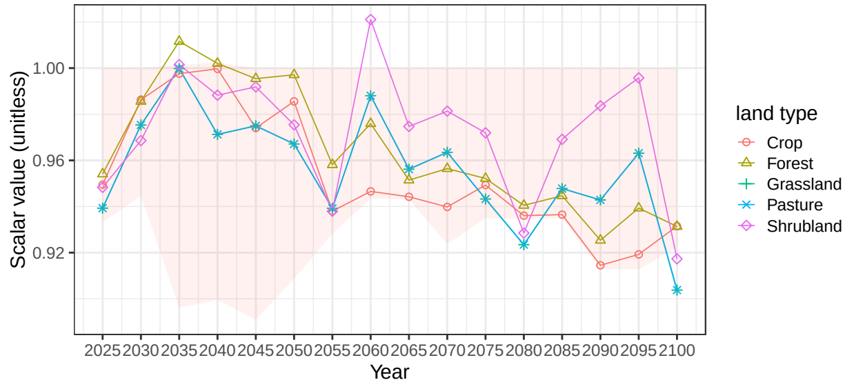
Region Canada basin CanAtl average soil scalars
