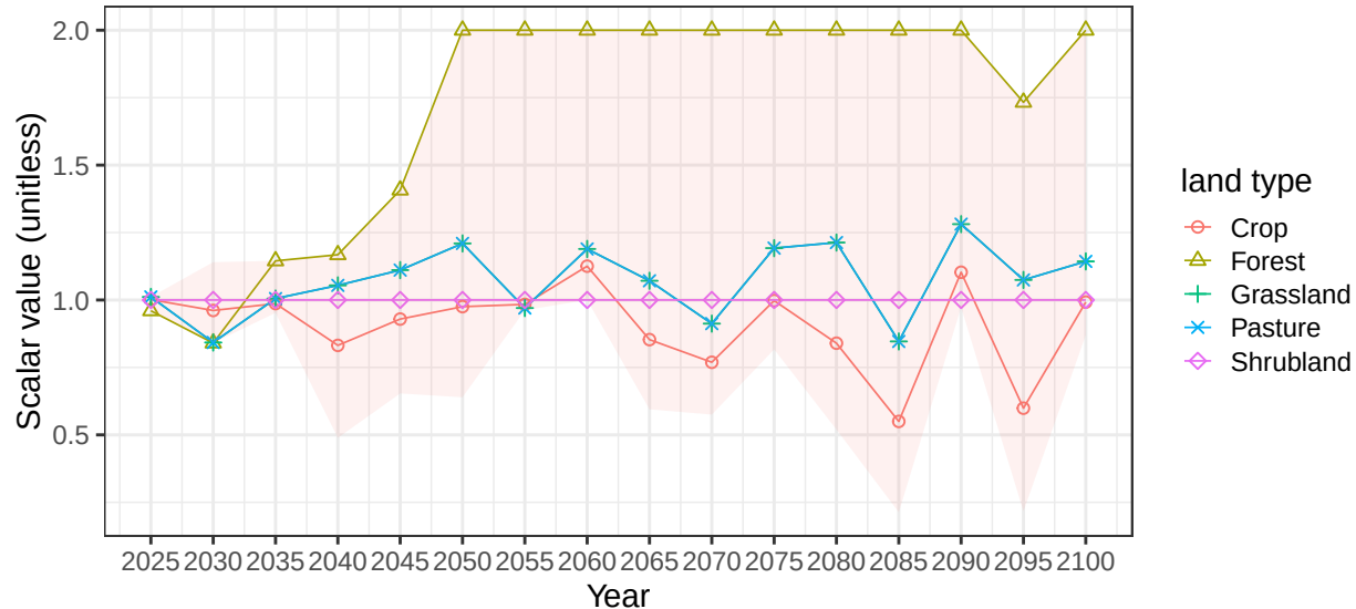
Region Africa_Western basin SenegalR average vegetation scalars
