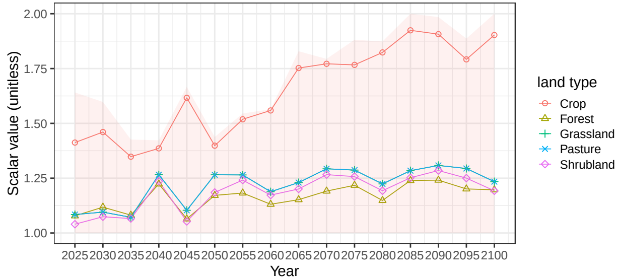
Region Canada basin NWTerr average vegetation scalars
