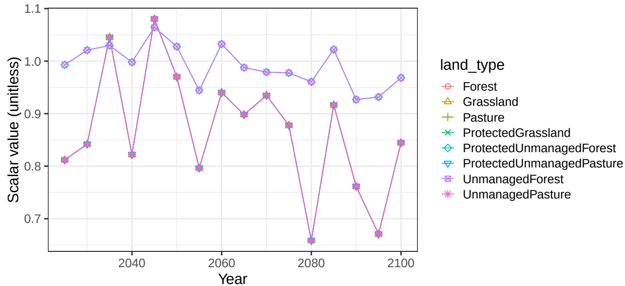
Region EU-12 basin BalticSea non-crop soil scalars
