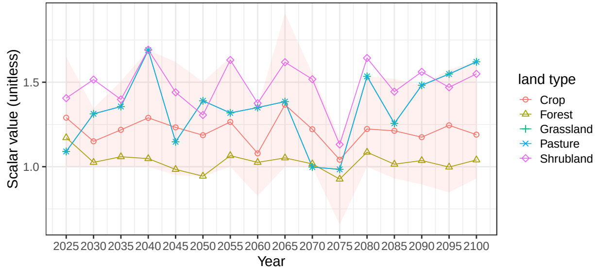
Region EU-15 basin GuadalqR average vegetation scalars
