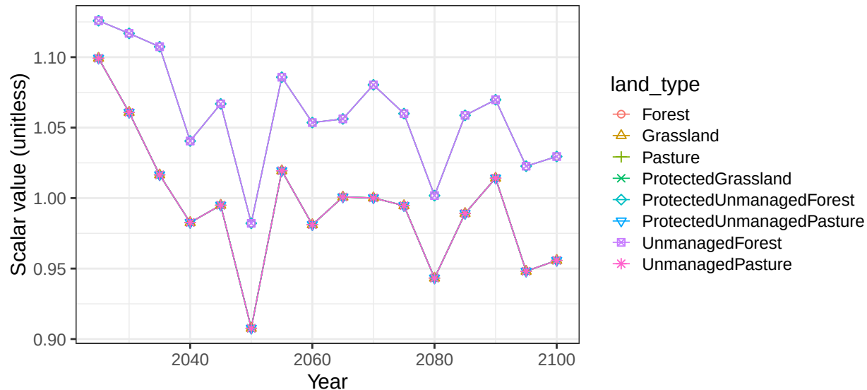
Region USA basin MissppRS non-crop soil scalars
