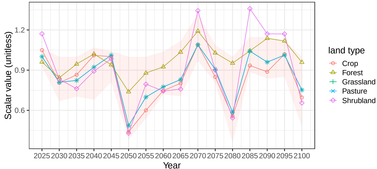
Region Australia_NZ basin MurrayDrlg average vegetation scalars
