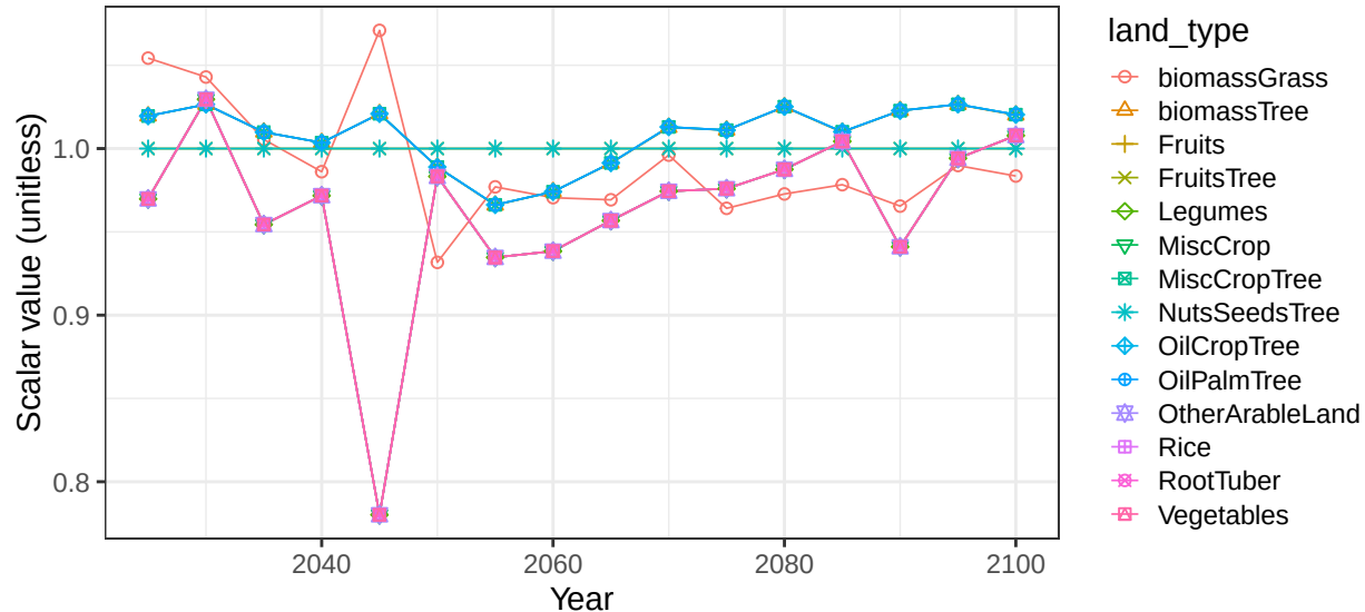
Region Southeast Asia basin SolomonIsI crop soil scalars
