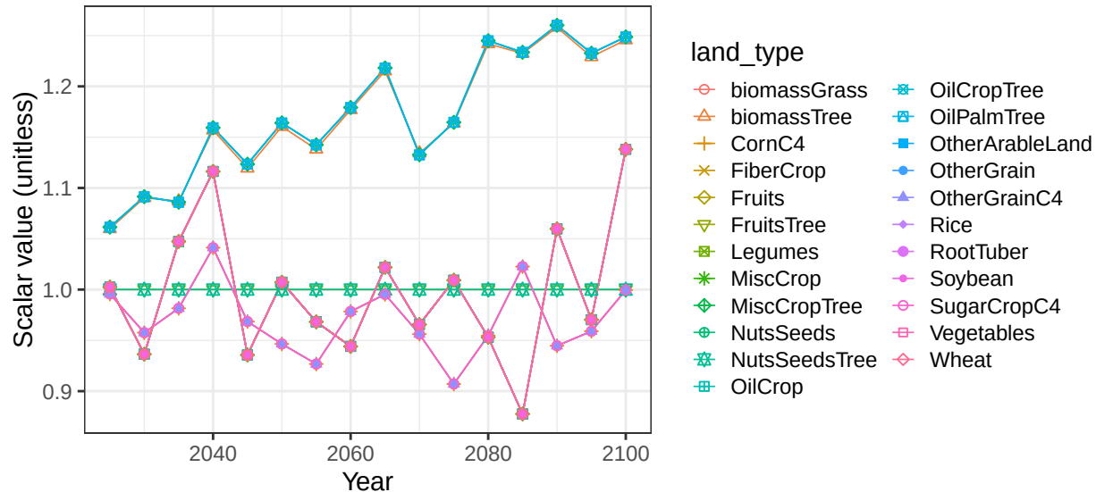
Region Africa_Southern basin AfrCstE crop soil scalars
