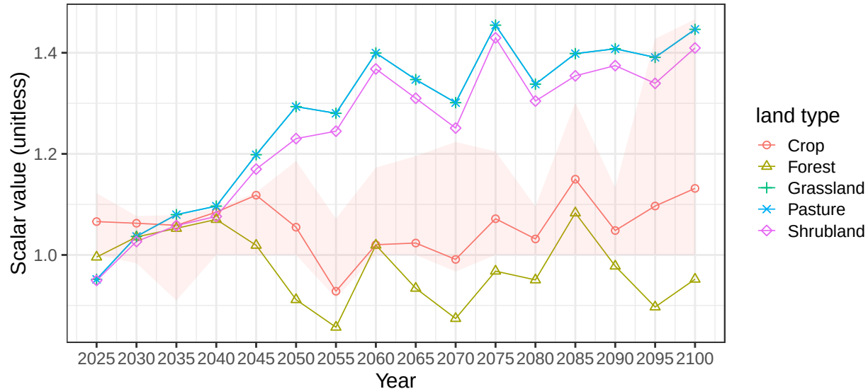
Region EU-15 basin Finland average soil scalars
