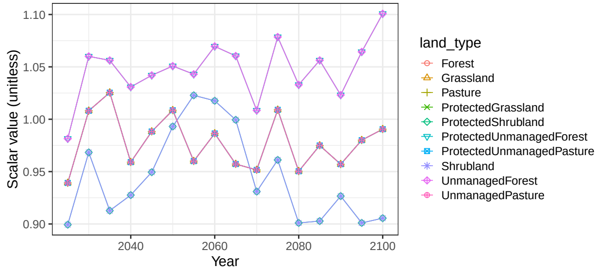
Region Mexico basin RioBalsas non-crop soil scalars
