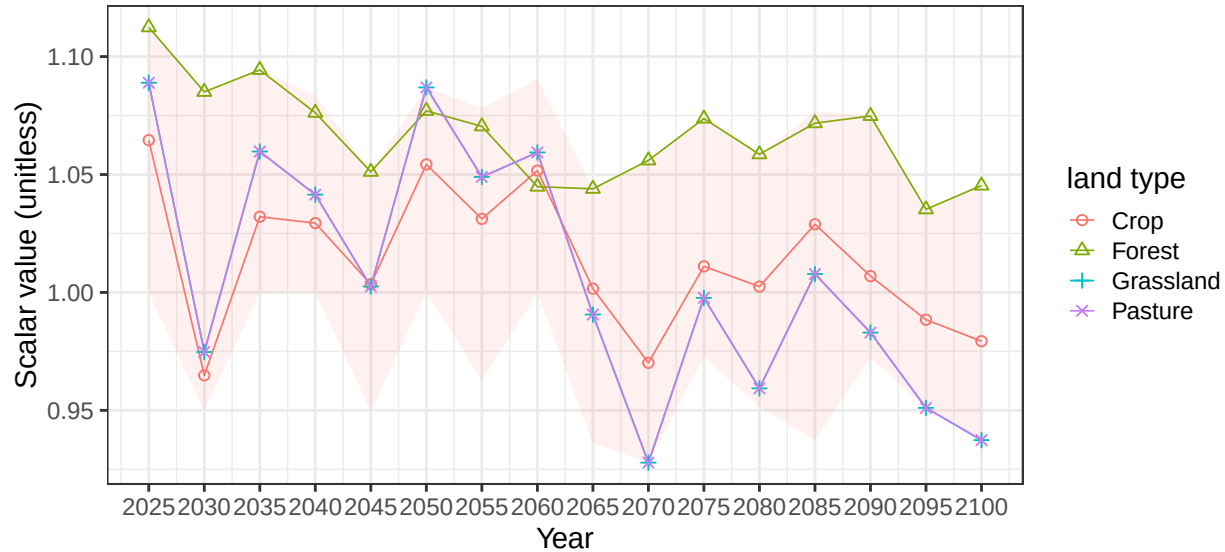
Region Africa_Eastern basin CongoR average soil scalars
