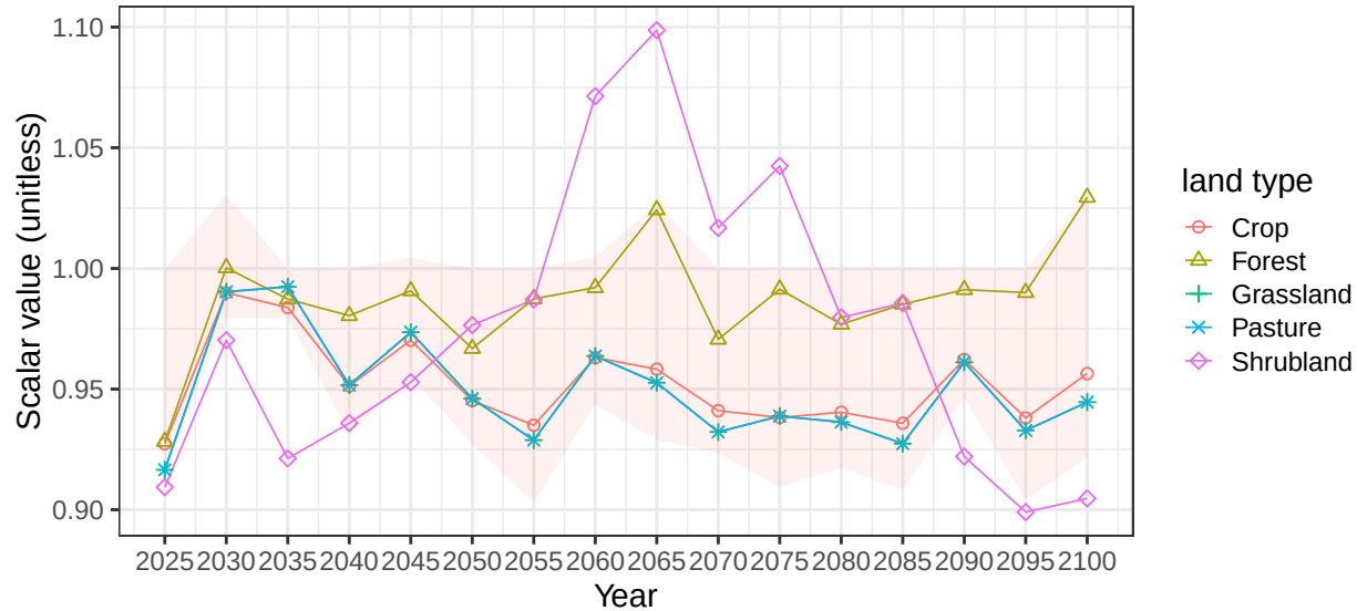
Region Mexico basin Papaloapan average soil scalars
