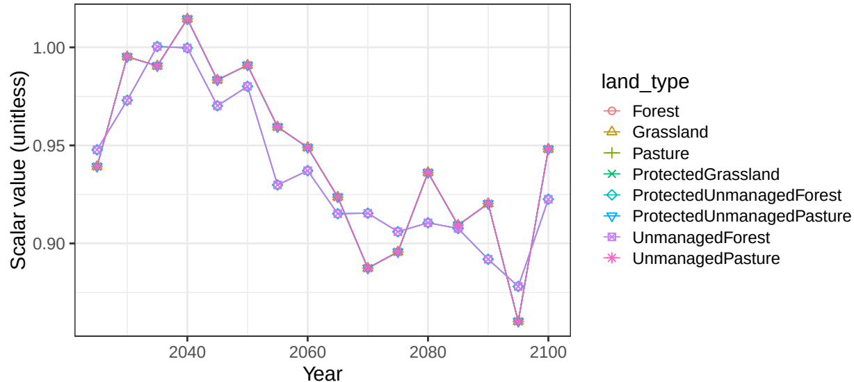
Region Canada basin UsaCstNE non-crop soil scalars
