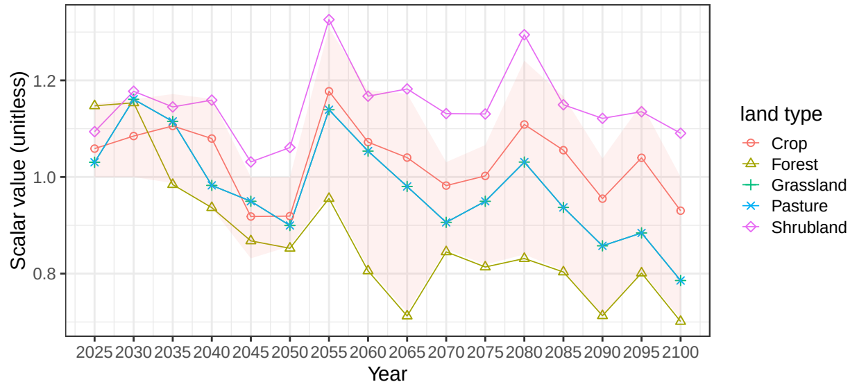
Region EU-15 basin AdrBlkSea average vegetation scalars
