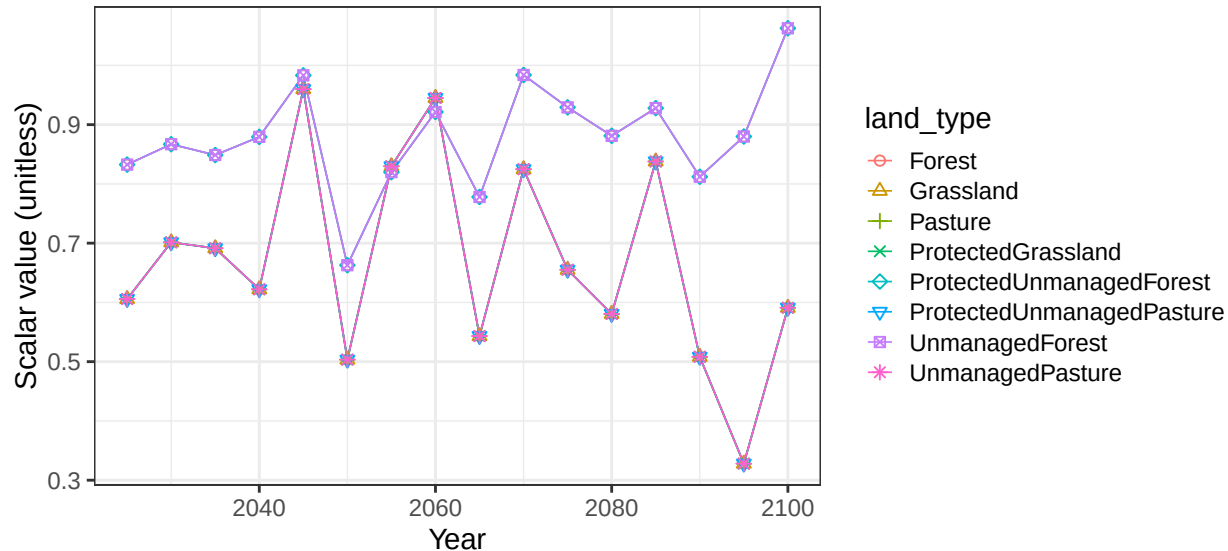
Region Europe_Eastern basin DaugavaR non-crop vegetation scalars
