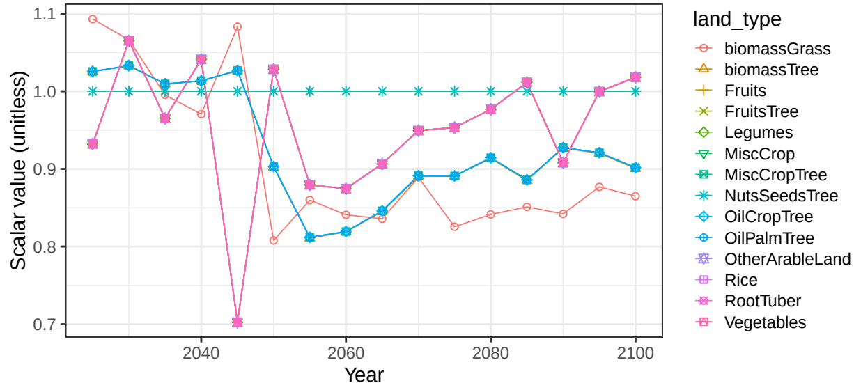
Region Southeast Asia basin SolomonIsI crop vegetation scalars
