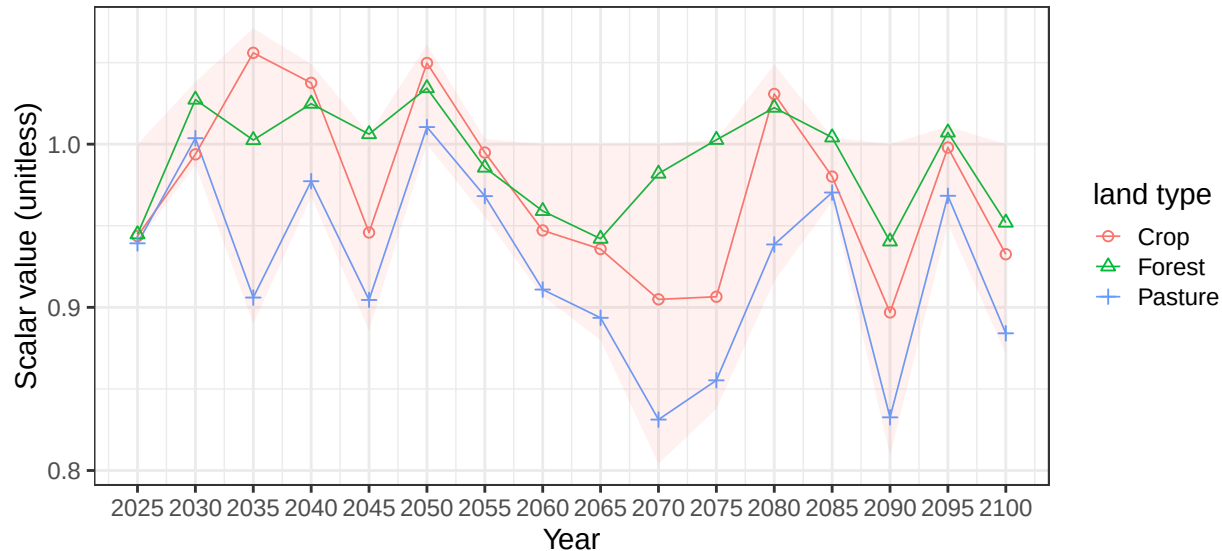
Region Taiwan basin ChinaCst average soil scalars
