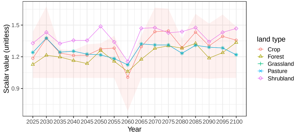
Region USA basin UsaPacNW average vegetation scalars
