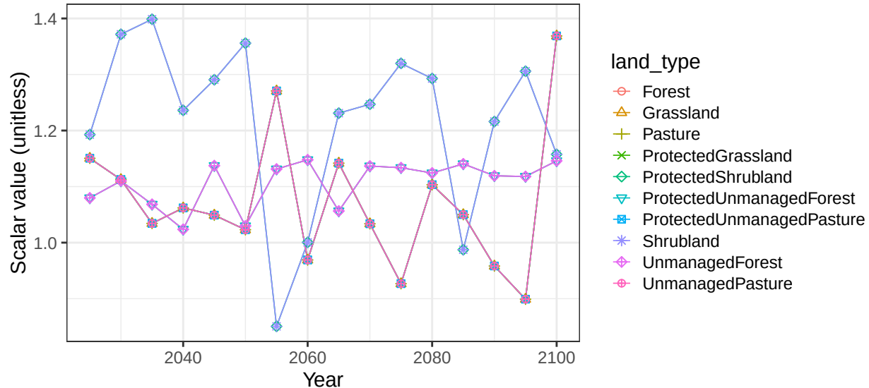
Region Central Asia basin VolgaR non-crop soil scalars
