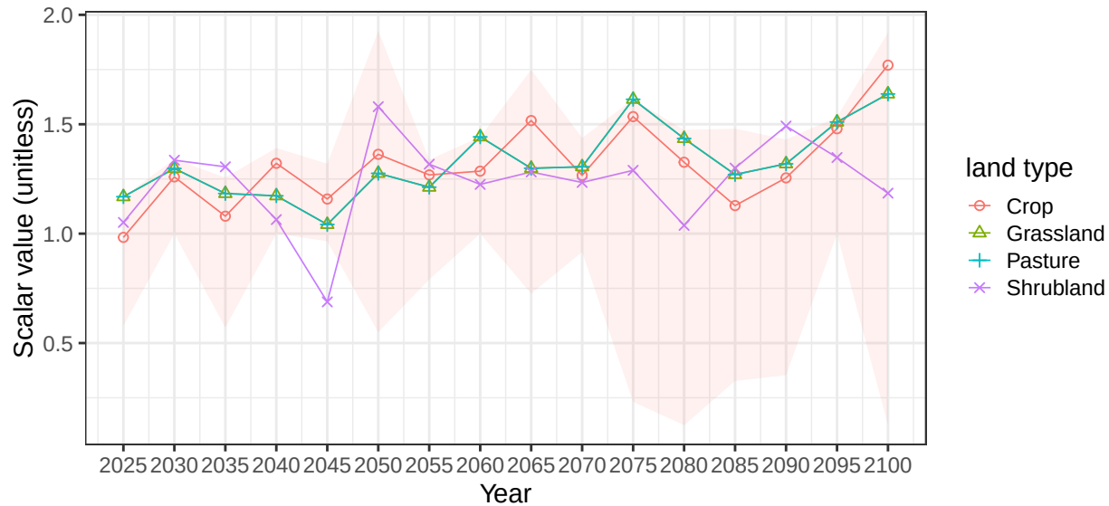
Region Middle East basin ArabianP average vegetation scalars
