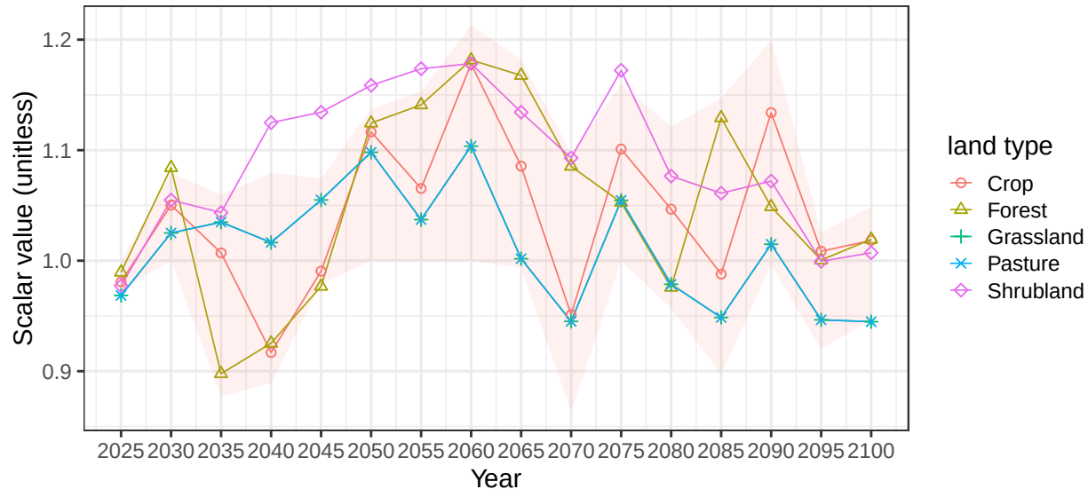
Region Europe_Non_EU basin CaspianSW average soil scalars
