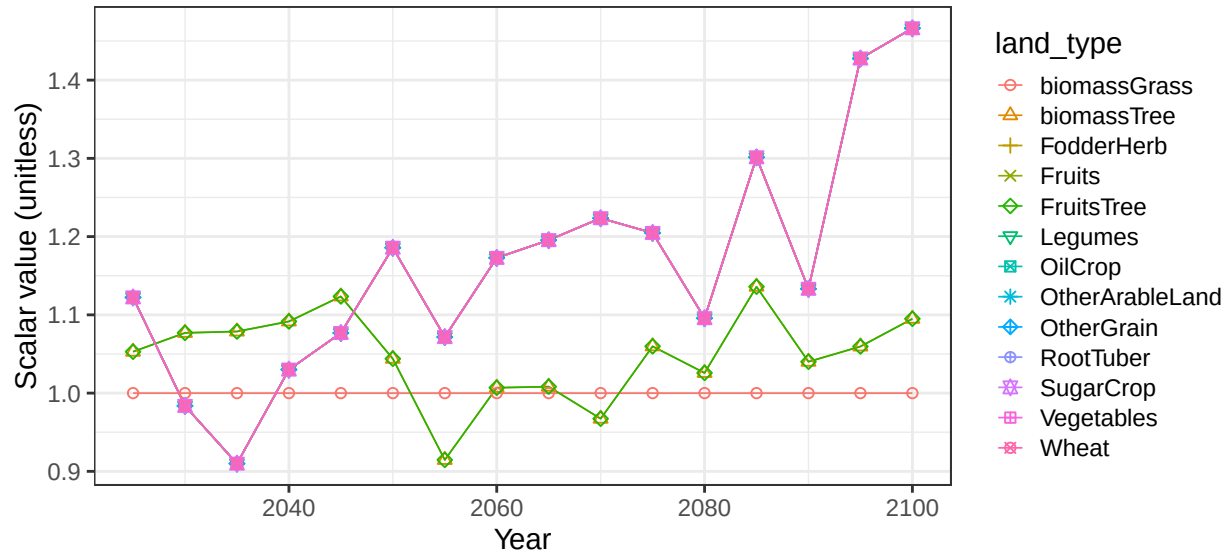
Region EU-15 basin Finland crop soil scalars
