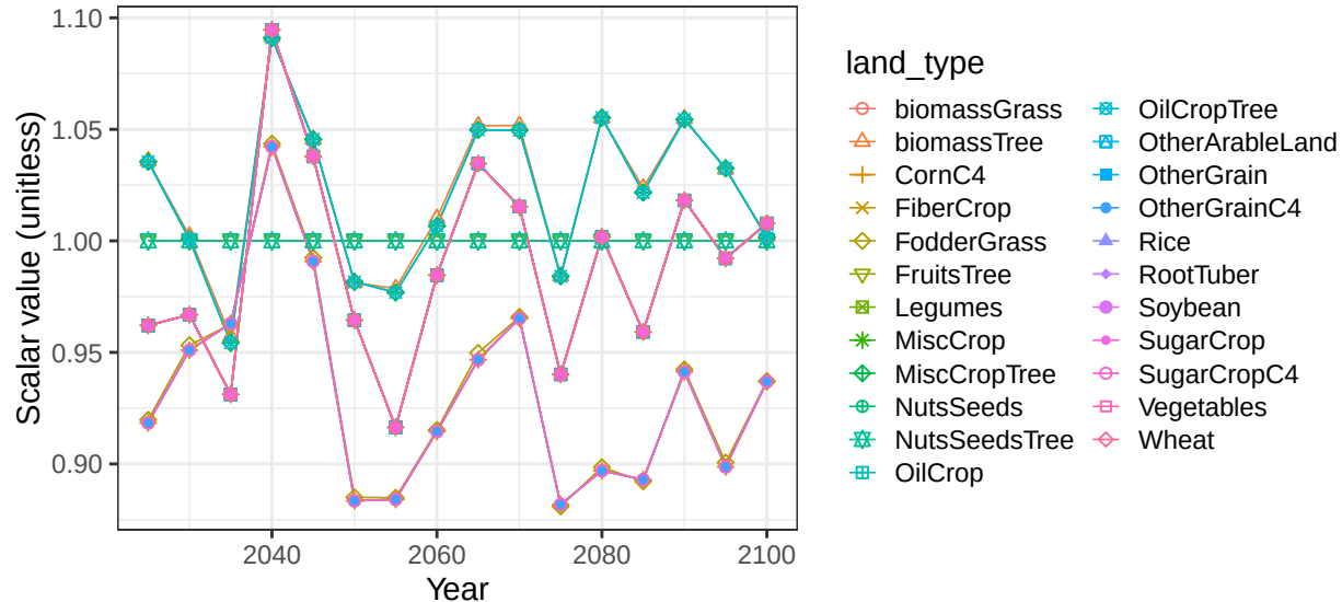
Region Southeast Asia basin SittaungR crop soil scalars
