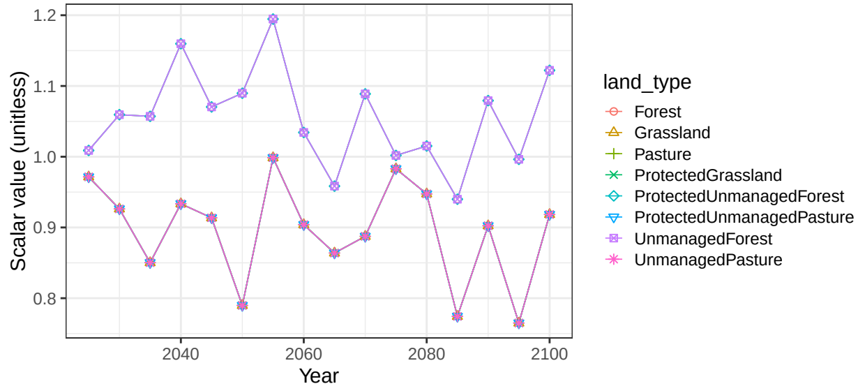
Region Europe_Eastern basin DniesterR non-crop soil scalars
