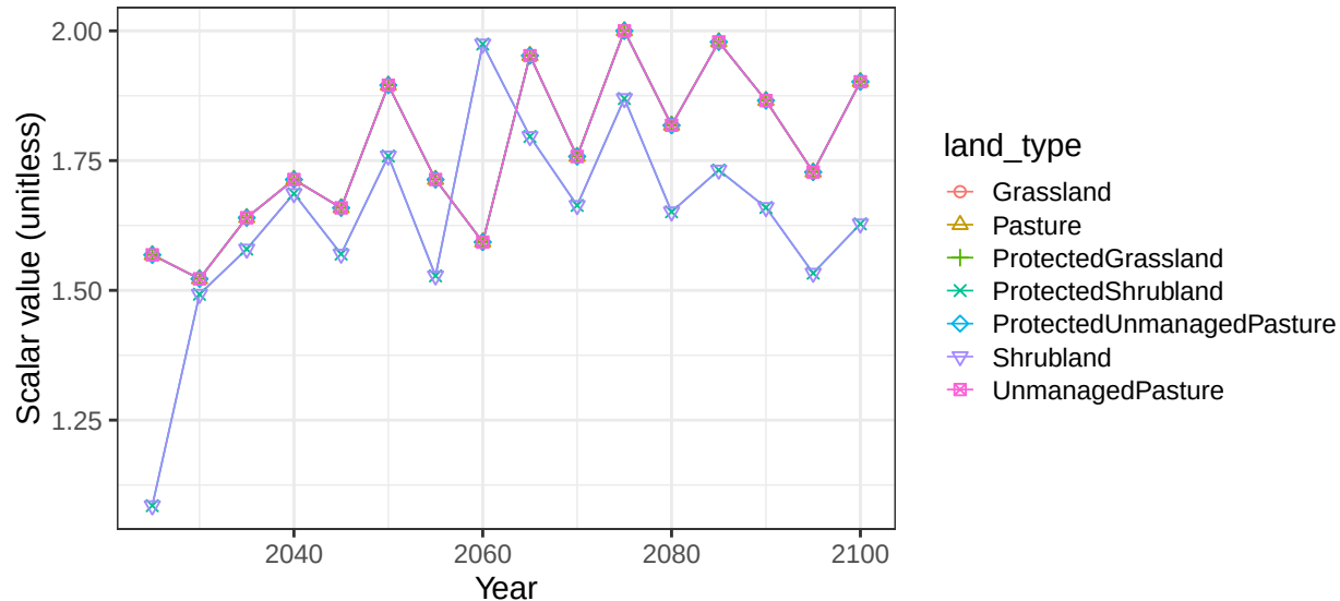
Region Middle East basin ArabianSea non-crop vegetation scalars
