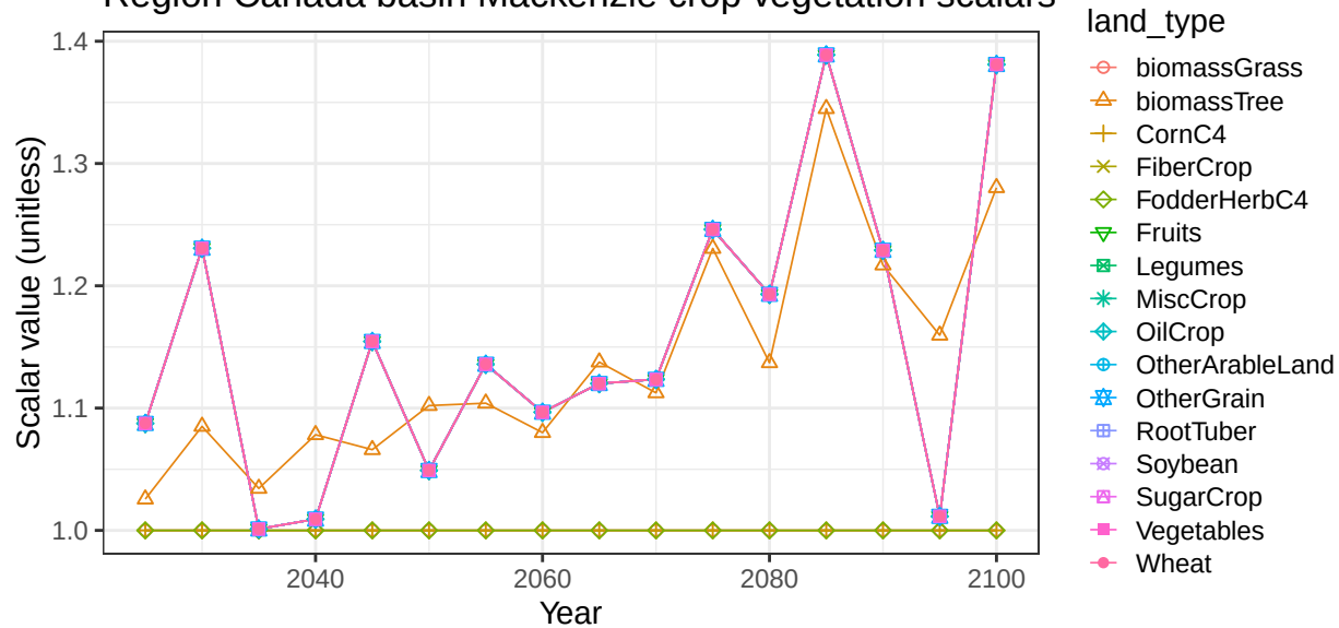
Region Canada basin Mackenzie crop vegetation scalars
