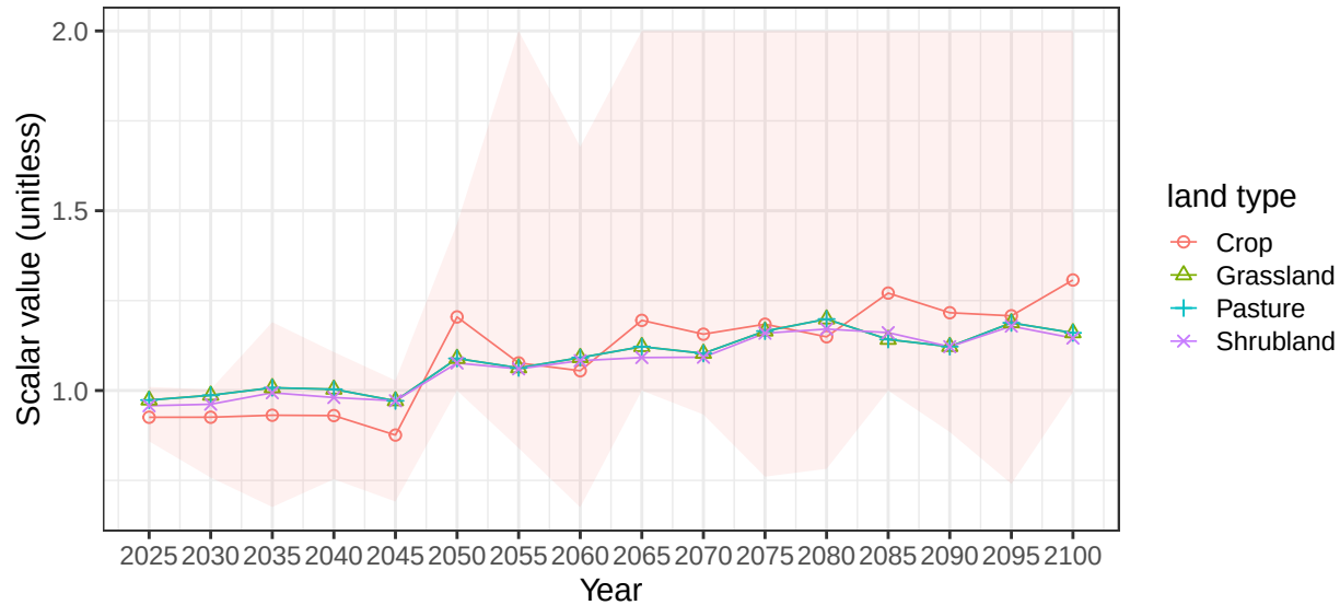
Region China basin Tarim average vegetation scalars
