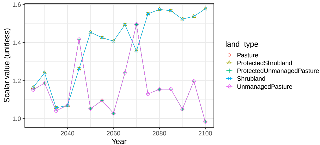
Region South Asia basin HamuMashR non-crop soil scalars
