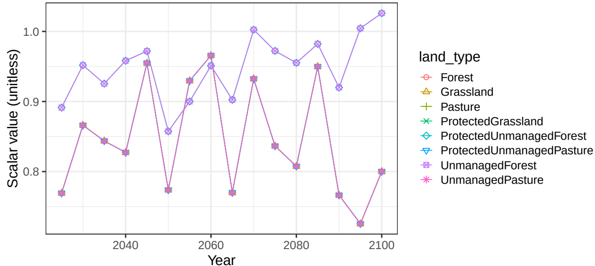
Region Europe_Eastern basin DaugavaR non-crop soil scalars
