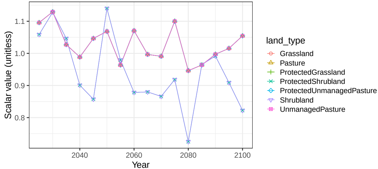
Region Middle East basin ArabianP non-crop soil scalars
