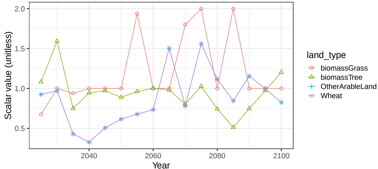
Region Central Asia basin BlackSeaN crop vegetation scalars
