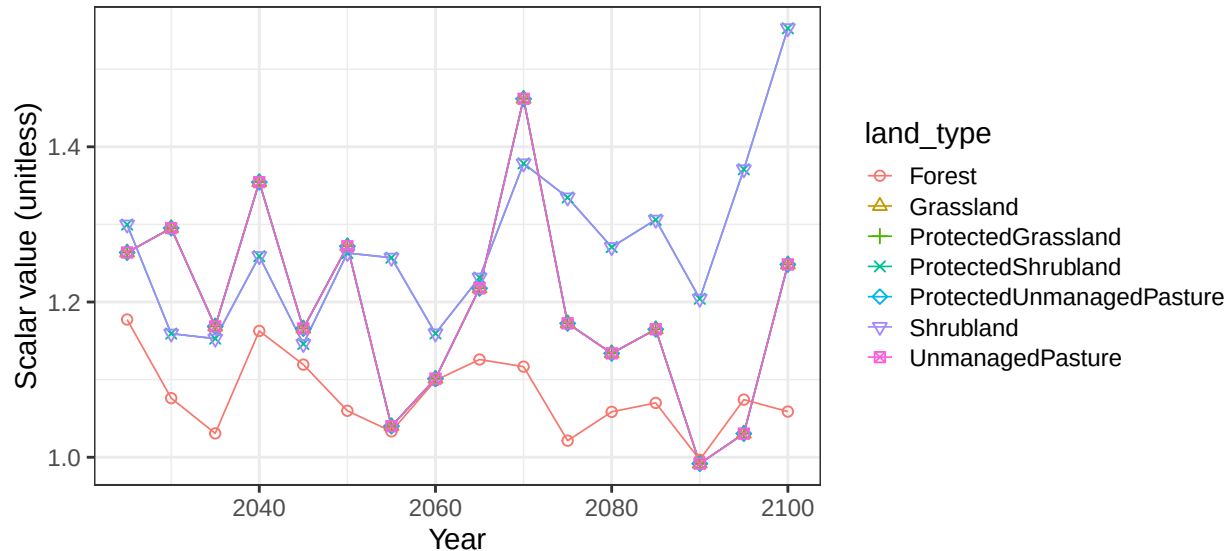
Region EU-15 basin IberiaCst non-crop vegetation scalars
