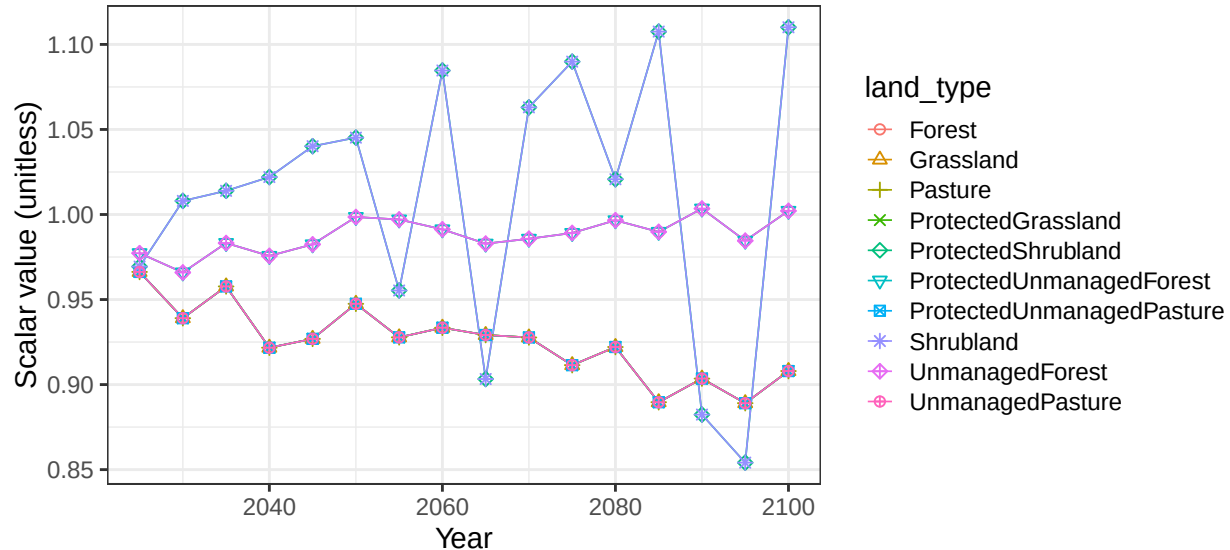
Region South America_Southern basin PeruCst non-crop soil scalars
