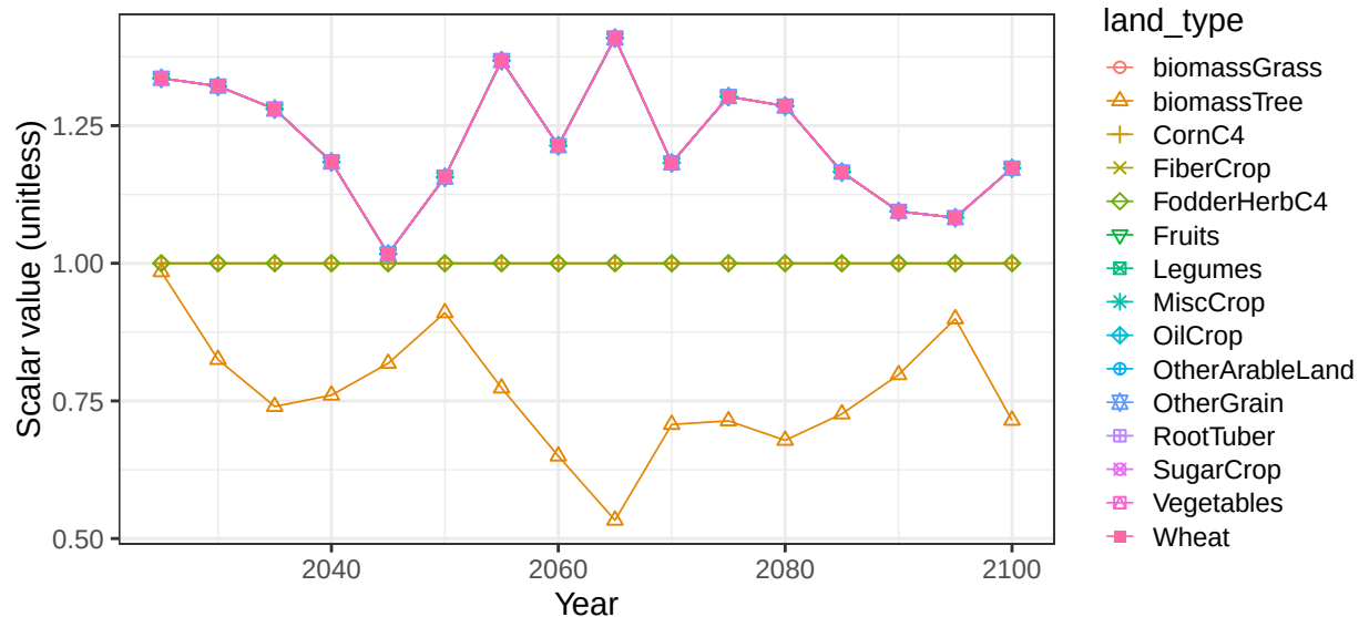
Region Canada basin MissouriR crop soil scalars
