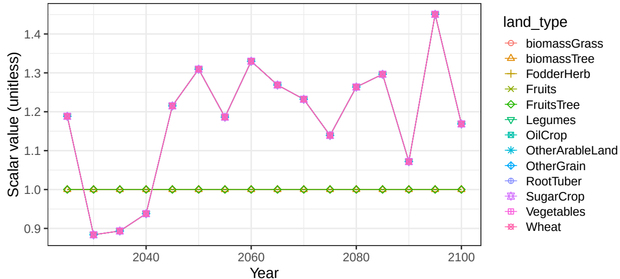
Region EU-15 basin NevaR crop soil scalars
