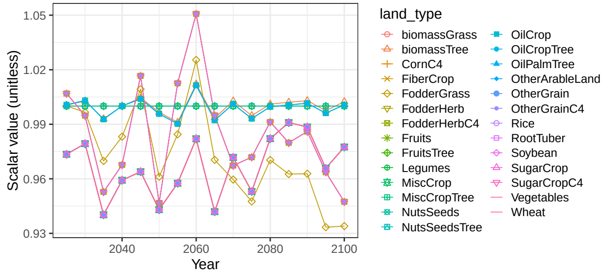
Region South America_Southern basin AmazonR crop soil scalars
