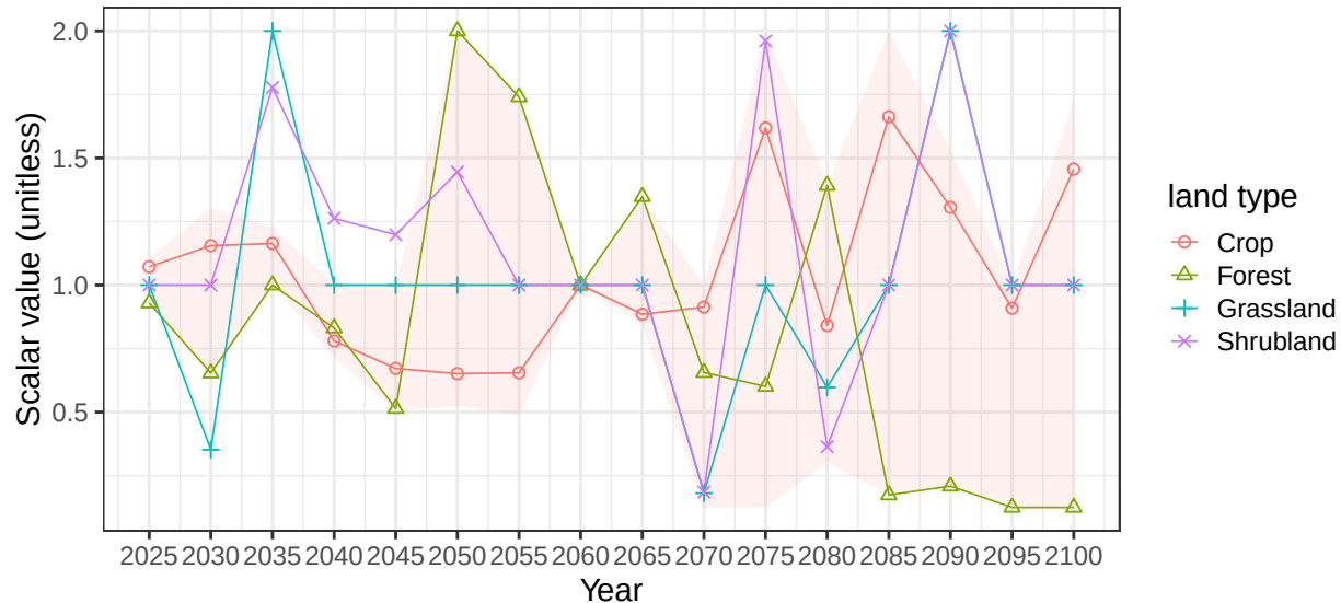
Region Africa_Northern basin NileR average vegetation scalars
