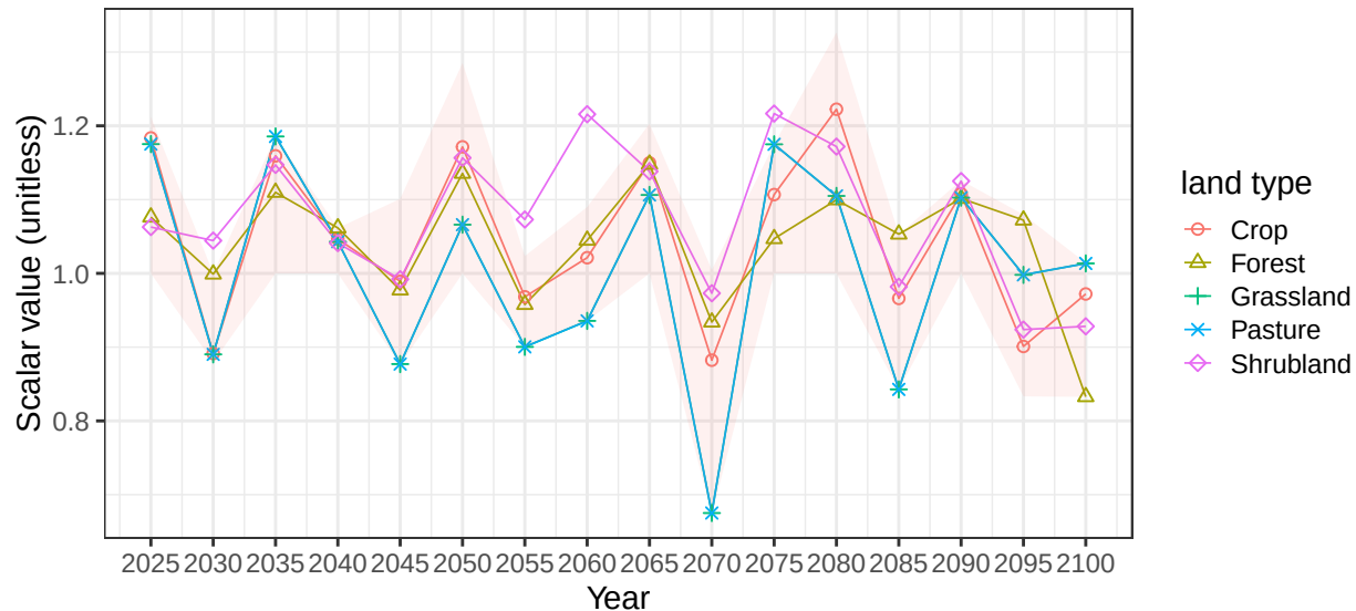
Region Africa_Eastern basin AfrCstE average soil scalars
