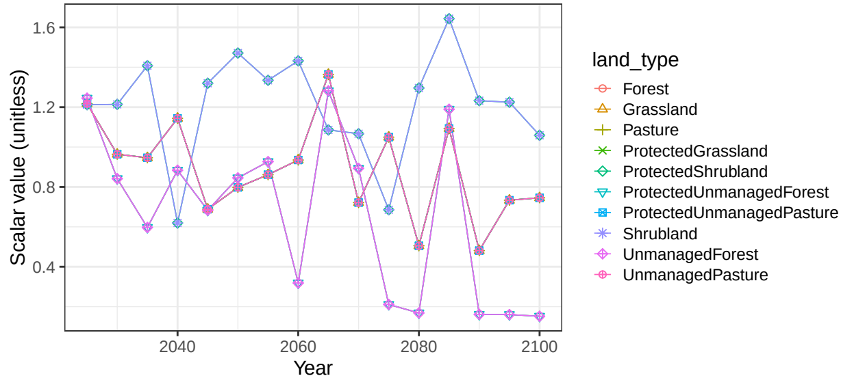
Region Argentina basin Pampas non-crop vegetation scalars
