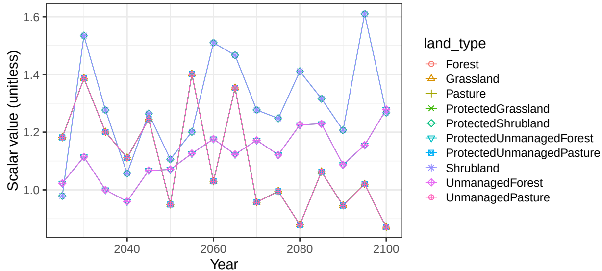
Region Australia_NZ basin AusCstW non-crop vegetation scalars
