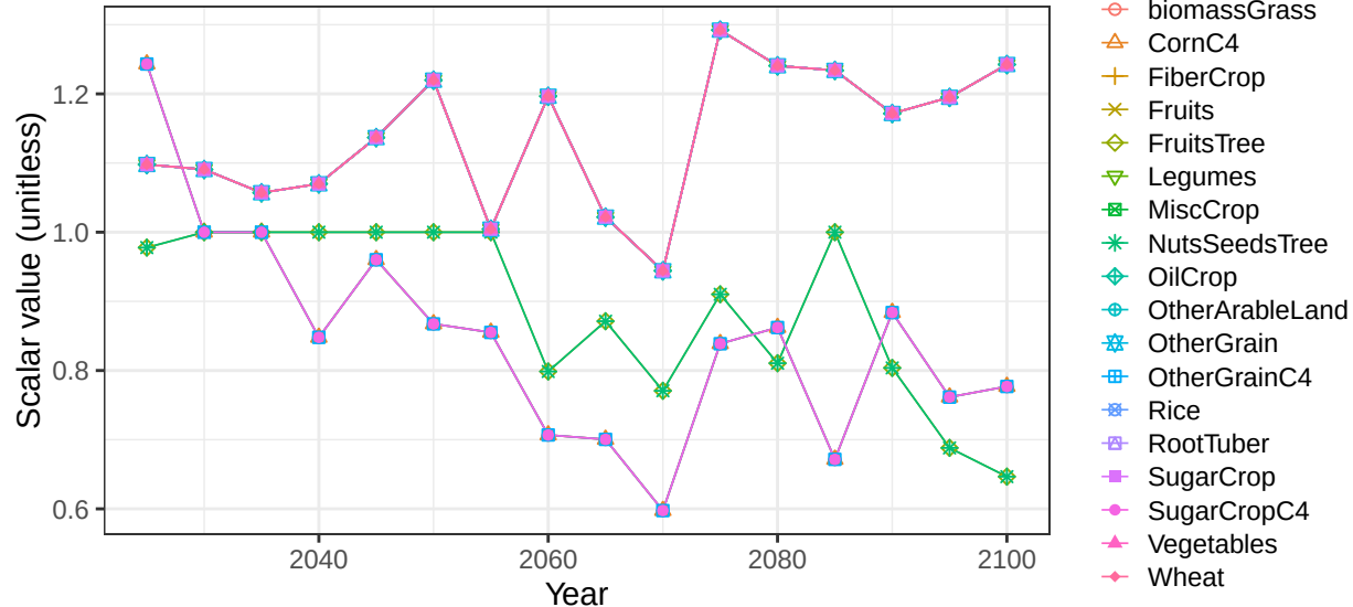
Region Pakistan basin Helmand crop soil scalars
