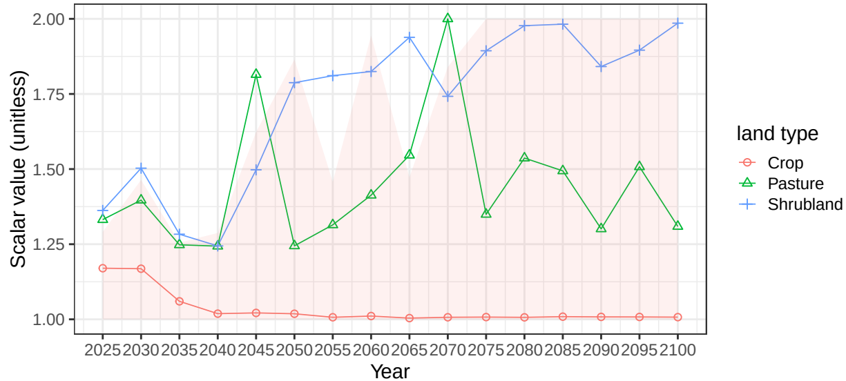
Region South Asia basin HamuMashR average vegetation scalars
