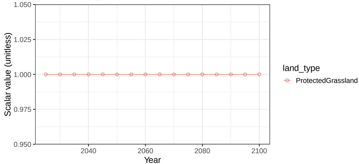
Region Africa_Northern basin AfrCstNE non-crop vegetation scalars
