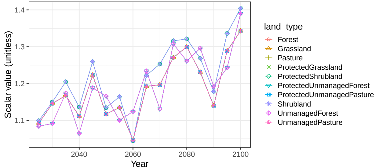
Region USA basin PacArctic non-crop vegetation scalars
