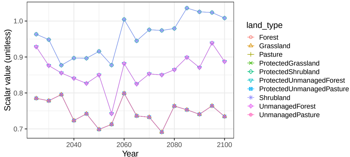
Region Brazil basin SAmerCstNE non-crop vegetation scalars
