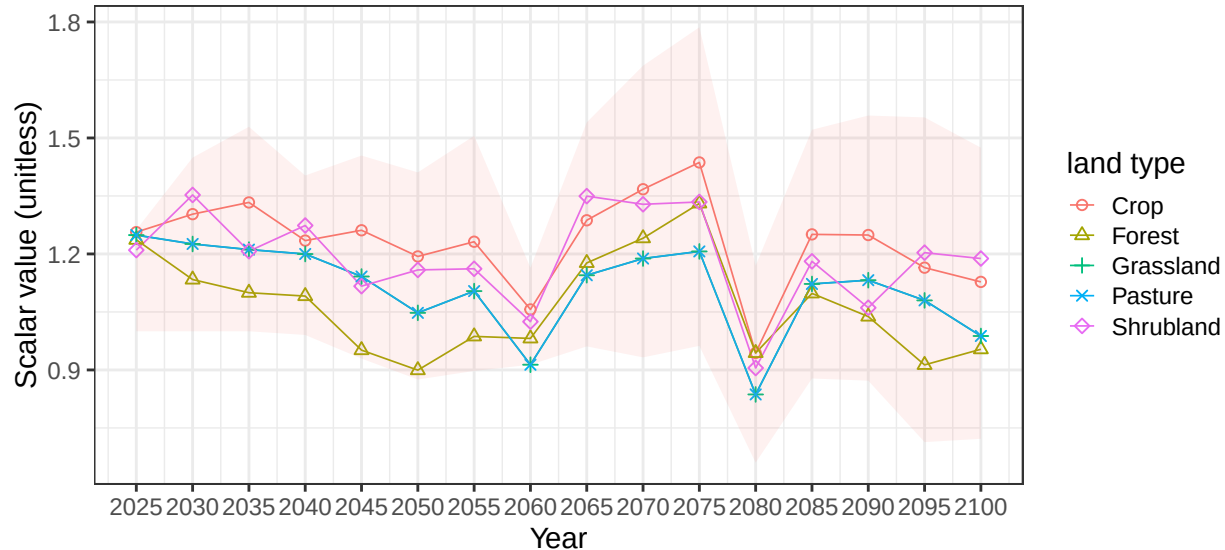
Region USA basin MissouriR average vegetation scalars
