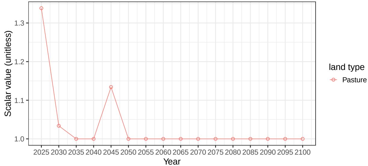
Region Pakistan basin AmuDaryaR average vegetation scalars
