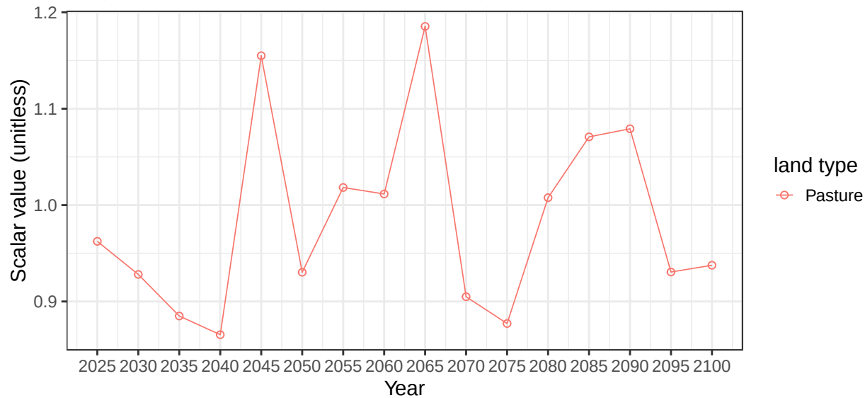
Region EU-15 basin AfrCstNW average soil scalars
