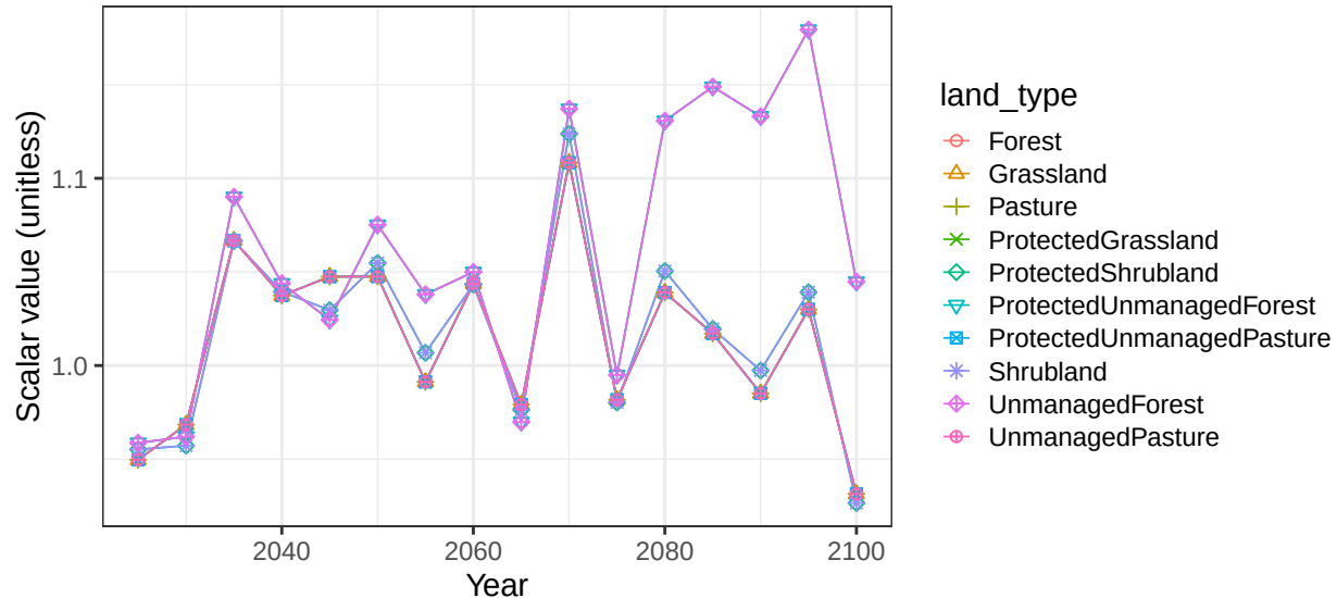
Region Russia basin KaraSea non-crop soil scalars
