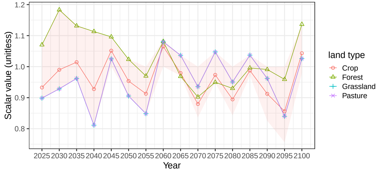
Region EU-12 basin PolandCst average soil scalars
