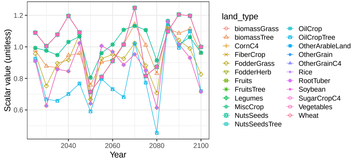
Region Australia_NZ basin AusCstE crop vegetation scalars
