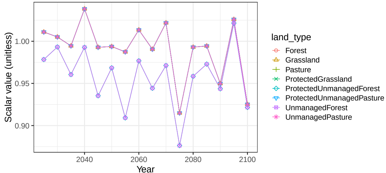
Region South America_Northern basin SAmerCstNE non-crop soil scalars
