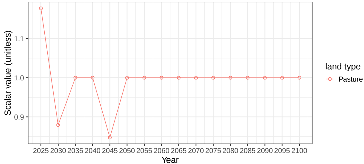
Region Pakistan basin AmuDaryaR average soil scalars
