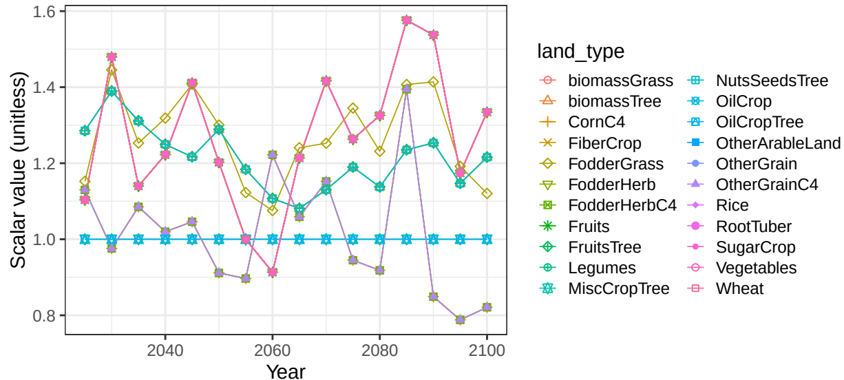
Region USA basin California crop vegetation scalars
