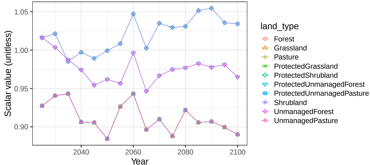
Region Brazil basin SAmerCstNE non-crop soil scalars
