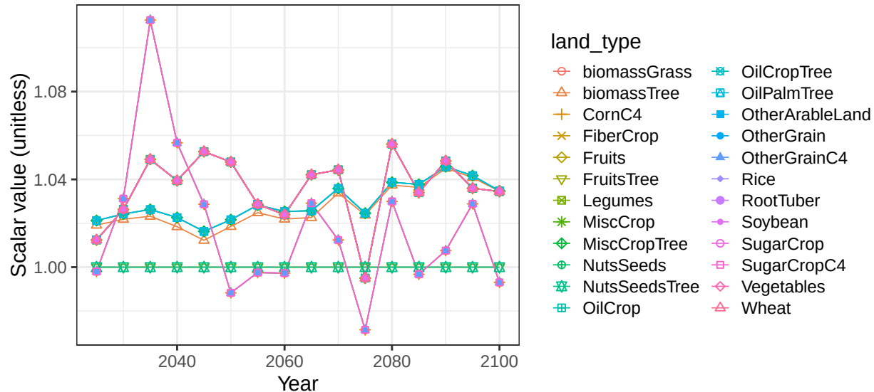
Region Colombia basin SAmerCstN crop soil scalars
