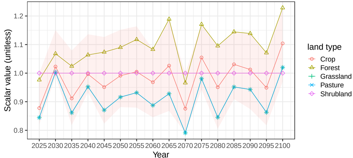
Region Mexico basin MexCstW average vegetation scalars
