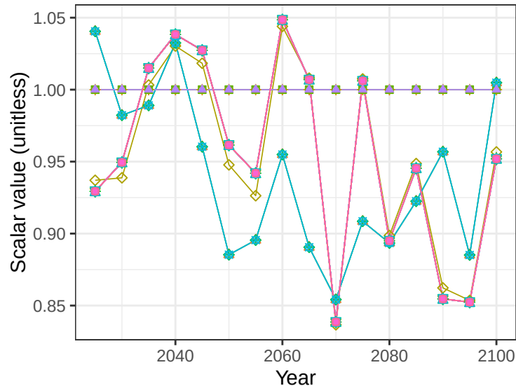
Region EU-15 basin ElbeR crop soil scalars
