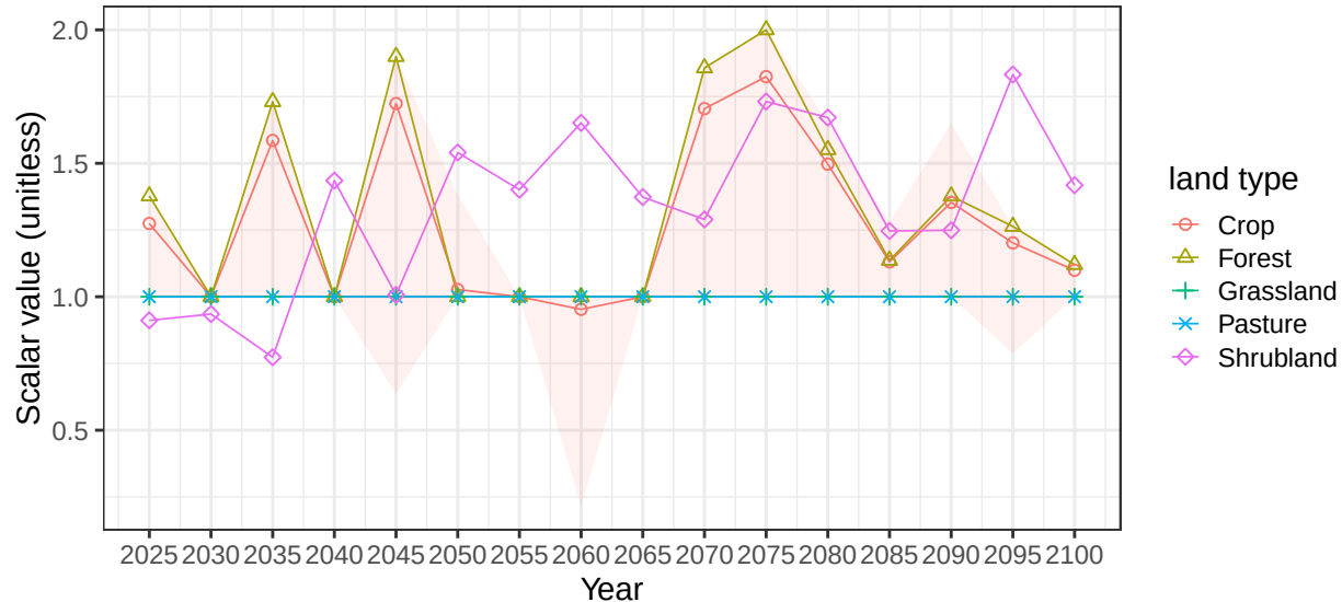
Region EU-12 basin MeditE average vegetation scalars
