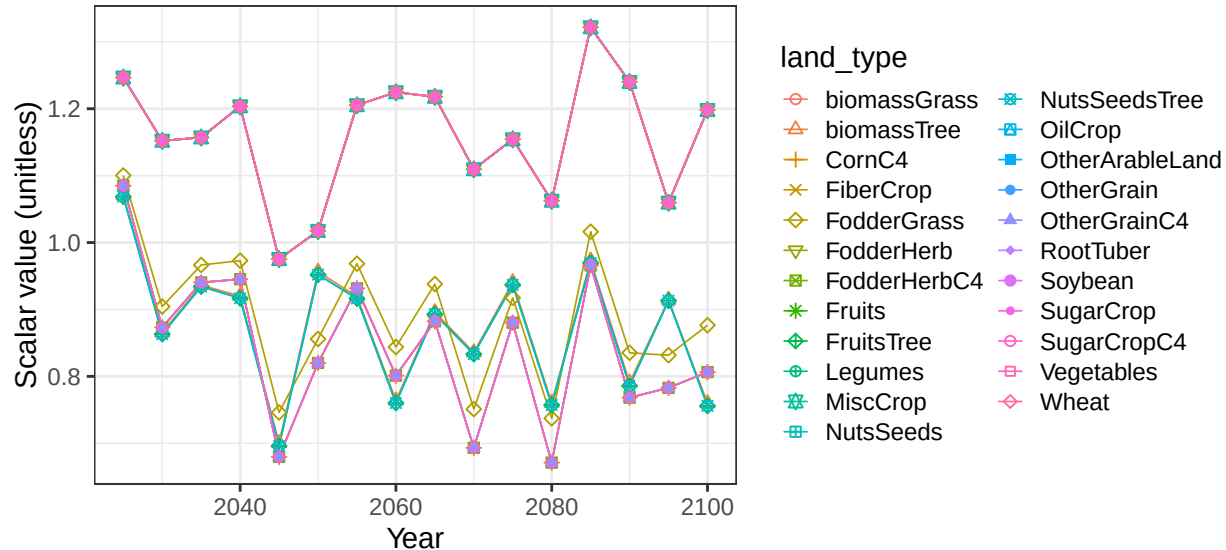
Region Mexico basin RioGrande crop soil scalars
