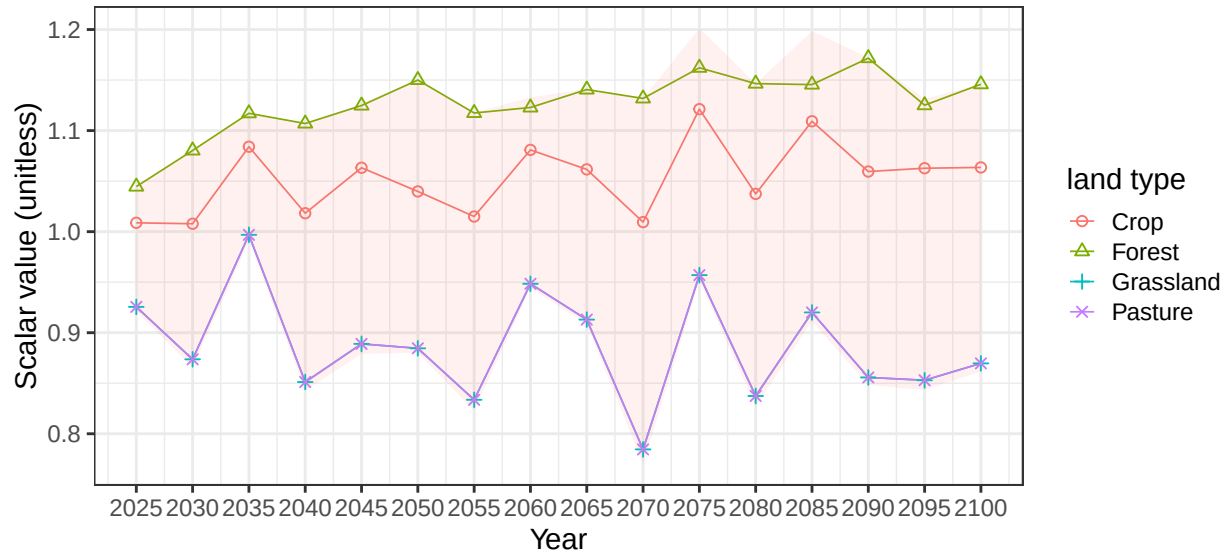
Region Indonesia basin Sulawesi average vegetation scalars
