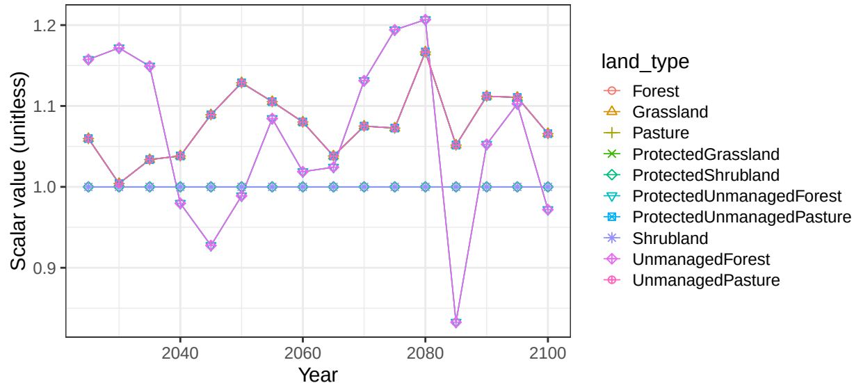
Region Africa_Western basin NigerR non-crop vegetation scalars
