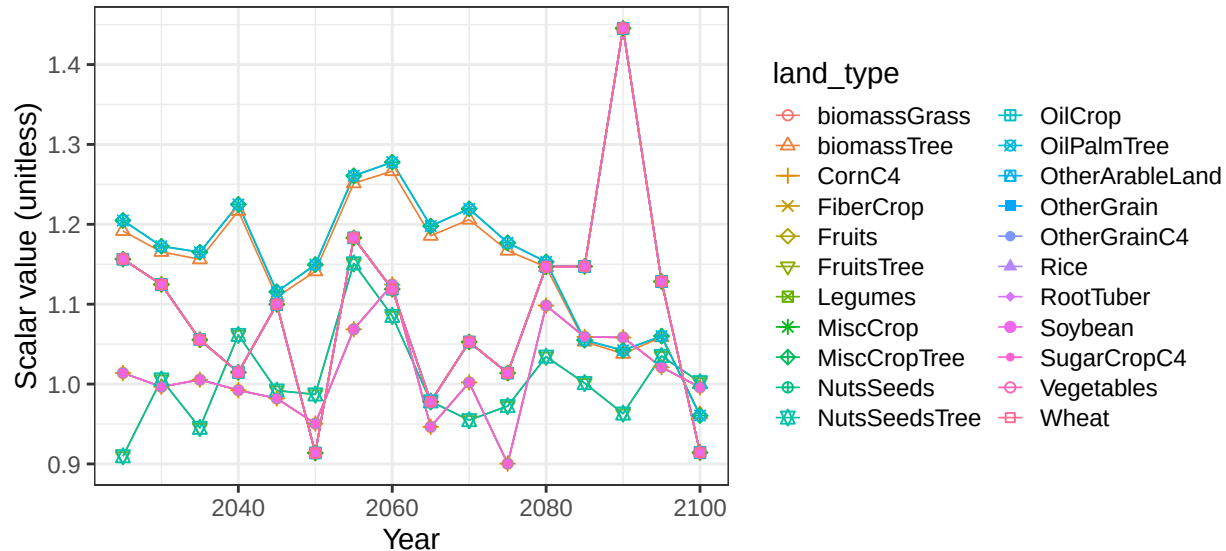
Region Africa_Southern basin AfrIntS crop soil scalars
