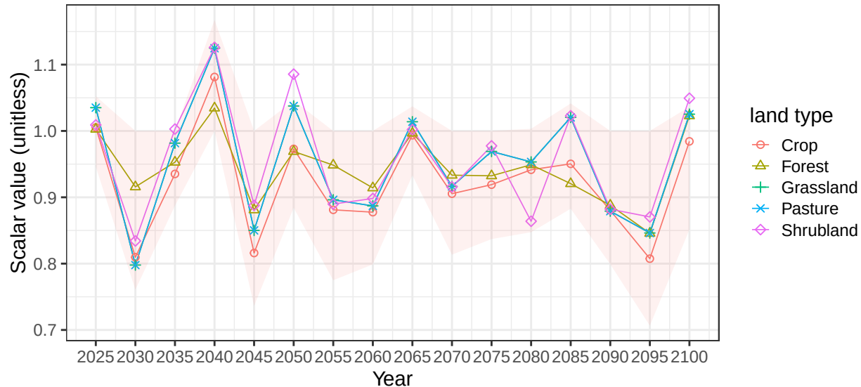
Region China basin ZiyaHe average soil scalars
