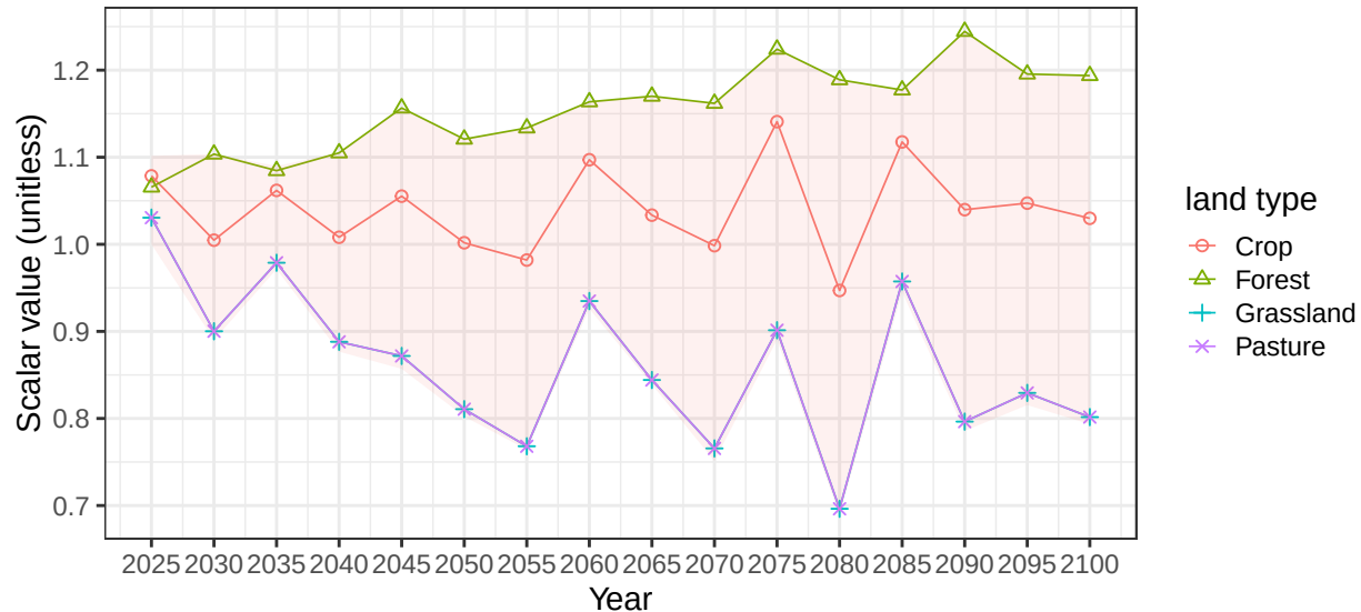
Region Indonesia basin JavaTimor average vegetation scalars
