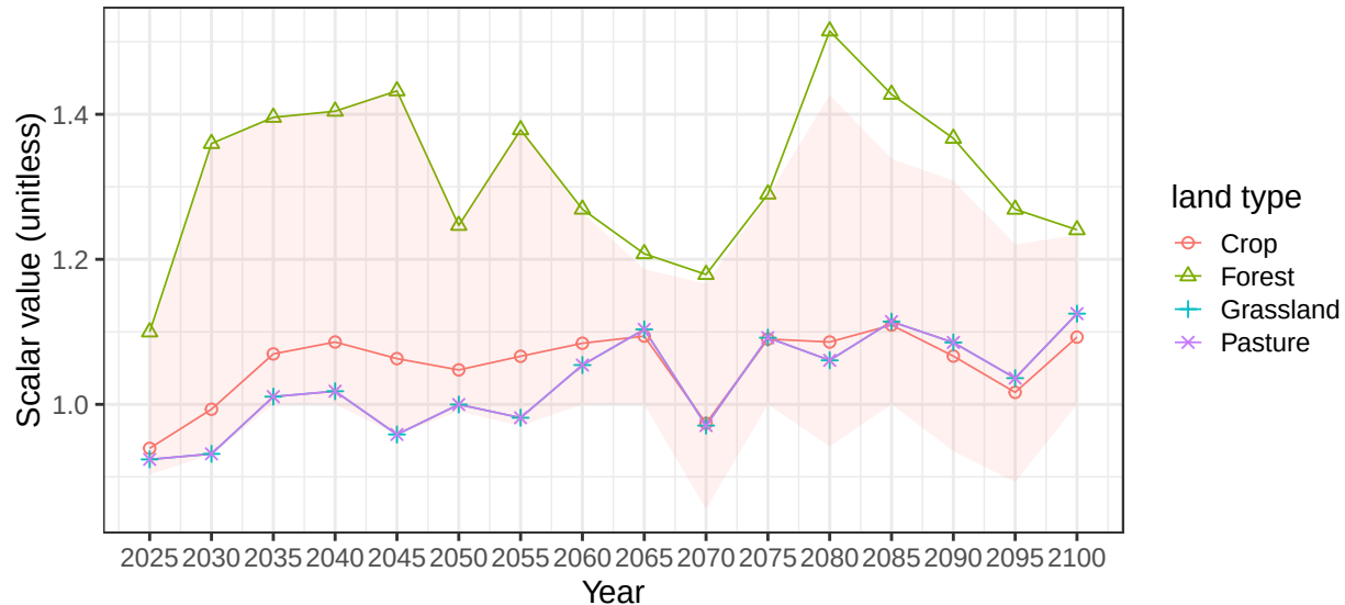
Region EU-15 basin EmsWeserR average soil scalars
