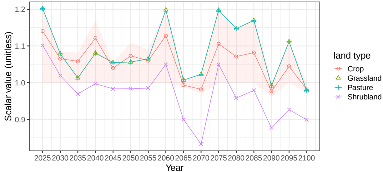
Region Middle East basin Helmand average soil scalars
