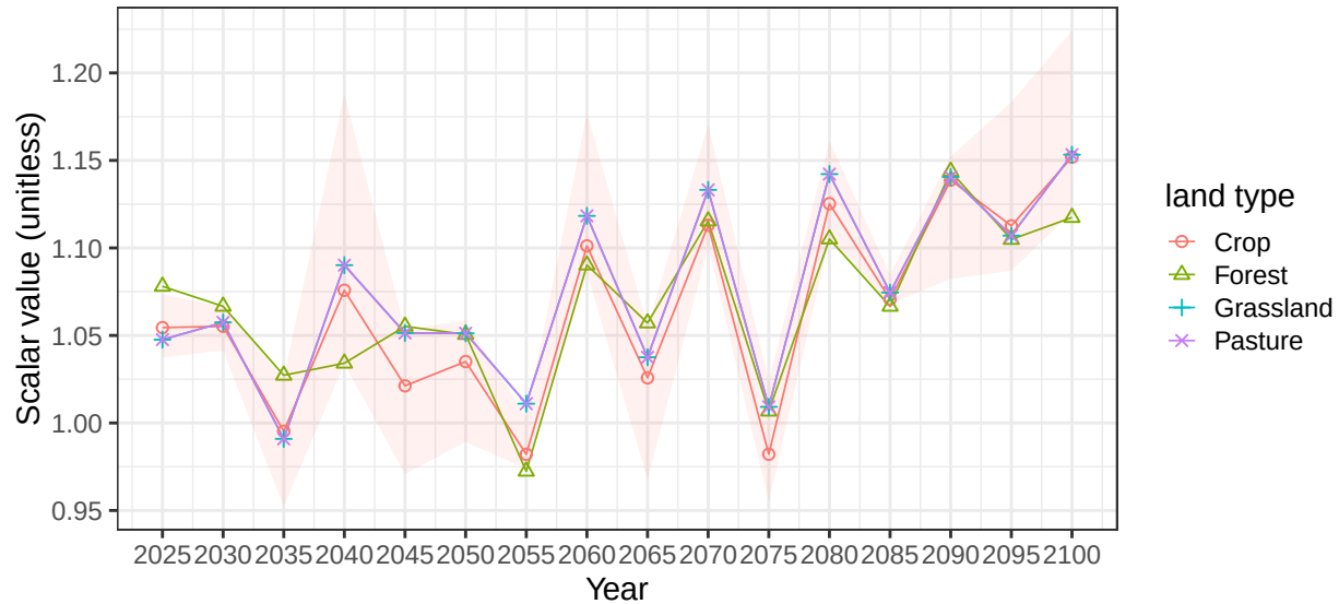
Region European Free Trade Association basin PoR average vegetation so
