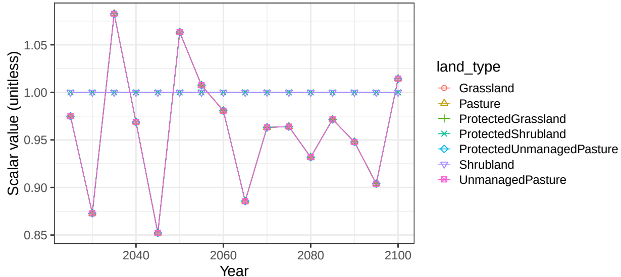
Region Africa_Eastern basin LChad non-crop soil scalars
