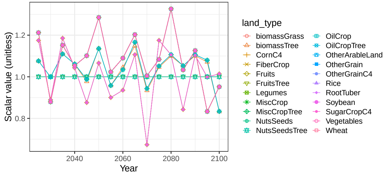
Region Africa_Eastern basin AfrCstE crop soil scalars
