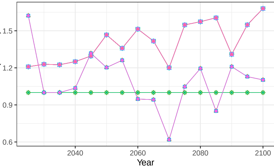
Region Pakistan basin Helmand crop vegetation scalars
