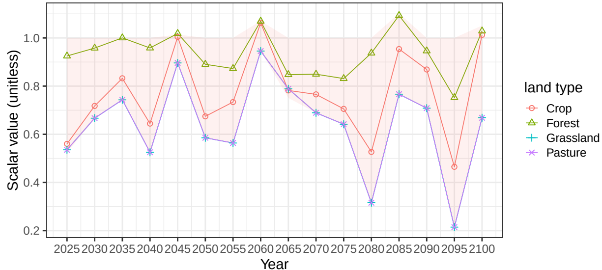
Region EU-12 basin NemanR average vegetation scalars
