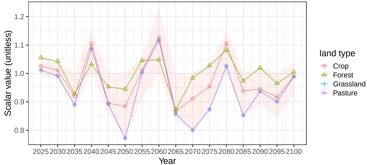
Region Europe_Non_EU basin DanubeR average soil scalars
