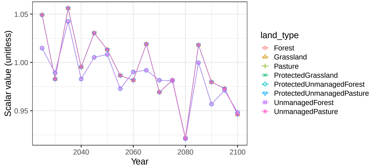
Region USA basin TennR non-crop soil scalars
