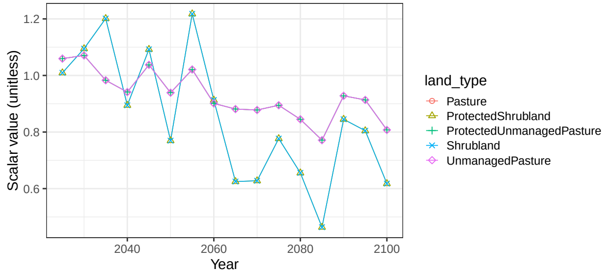
Region Pakistan basin SabarmatiR non-crop soil scalars
