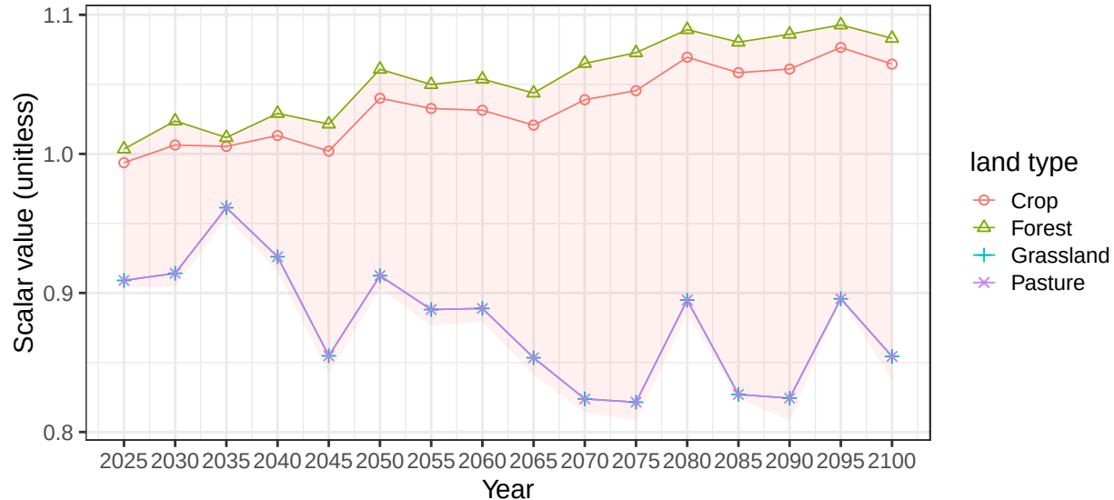
Region Indonesia basin Sumatra average vegetation scalars
