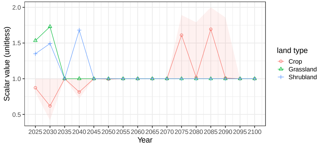
Region Africa_Northern basin MeditE average vegetation scalars
