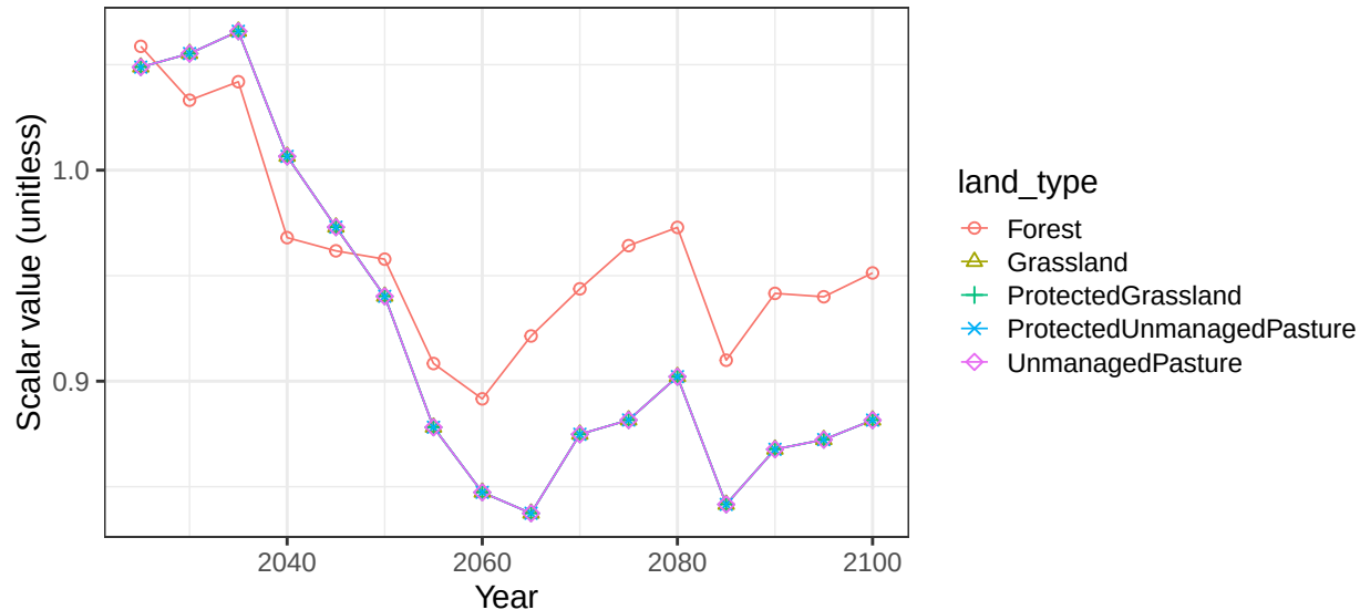
Region EU-15 basin Scotland non-crop vegetation scalars
