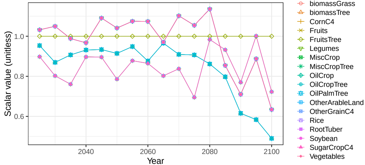
Region Central America and Caribbean basin SAMerCstN land use Vegetation s
