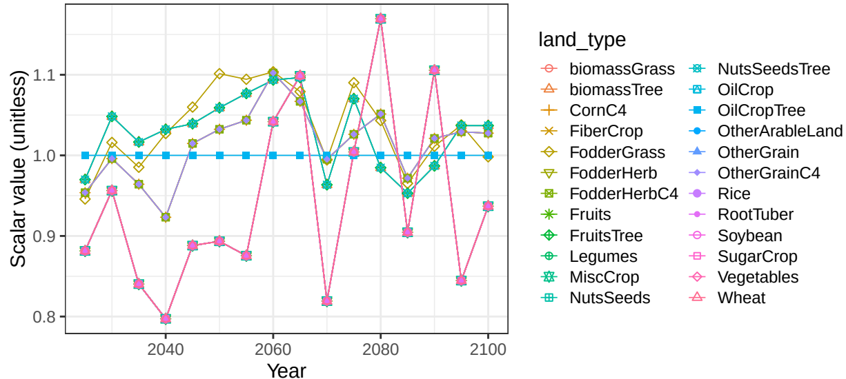
Region Central Asia basin CaspianSW crop soil scalars
