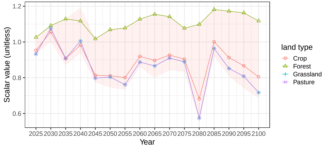
Region Southeast Asia basin JavaTimor average vegetation scalars
