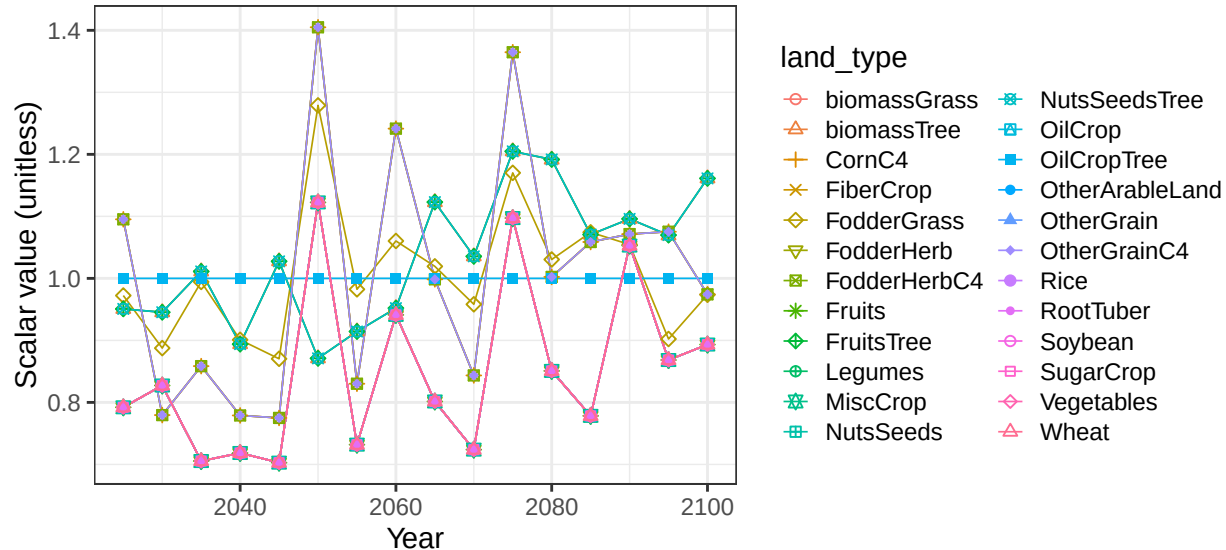
Region Central Asia basin SyrDaryaR crop vegetation scalars
