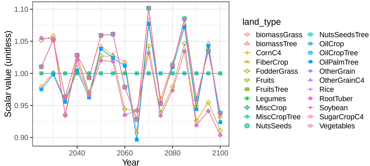
Region China basin Hainan crop soil scalars
