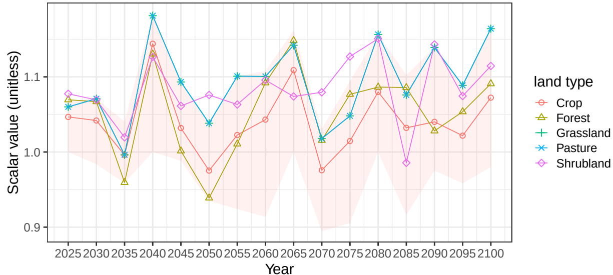
Region EU-15 basin Gironde average vegetation scalars
