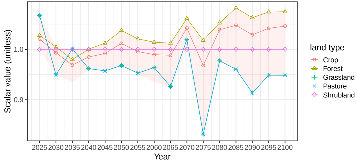
Region Southeast Asia basin MalaysiaP average vegetation scalars
