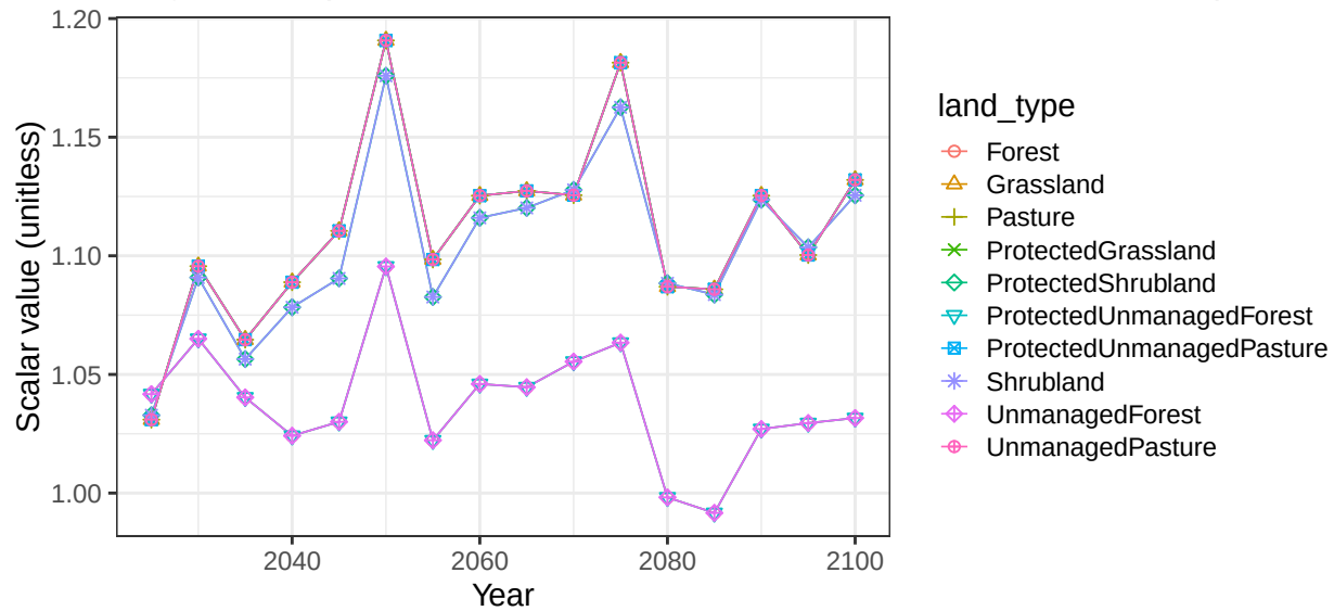
Region European Free Trade Association basin ScndnvN non-crop soil sca
