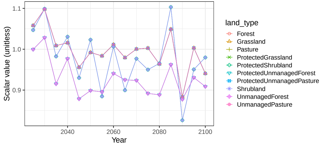
Region USA basin UsaColoRN non-crop soil scalars
