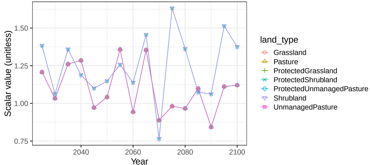
Region Argentina basin ArgCstN non-crop vegetation scalars
