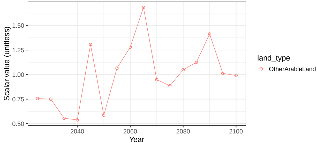
Region EU-15 basin AfrCstNW crop vegetation scalars
