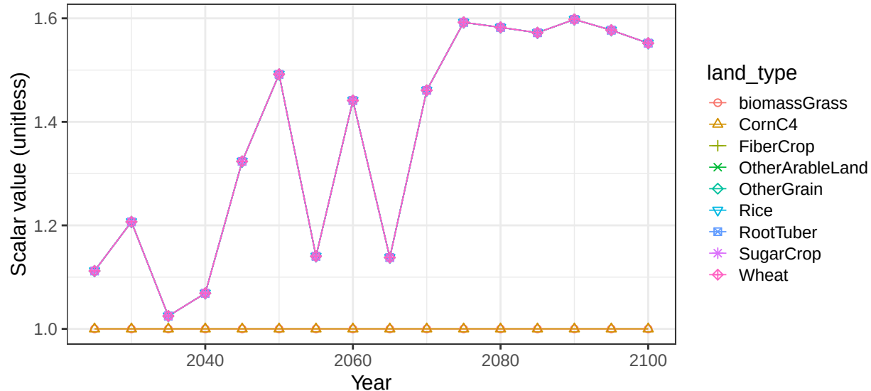
Region South Asia basin HamuMashR crop soil scalars
