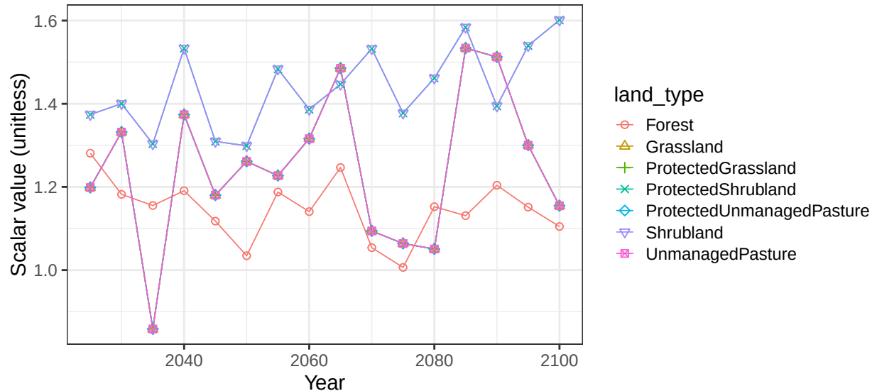
Region EU-15 basin SpainCstSE non-crop vegetation scalars
