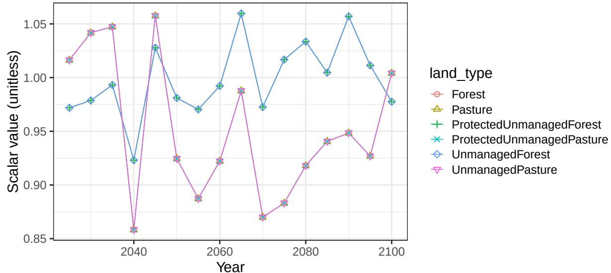
Region Mexico basin CntAmer non-crop vegetation scalars
