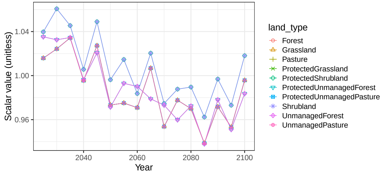
Region South Korea basin Korea non-crop soil scalars
