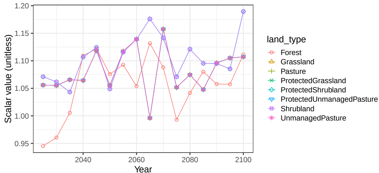
Region India basin IndCstS non-crop soil scalars
