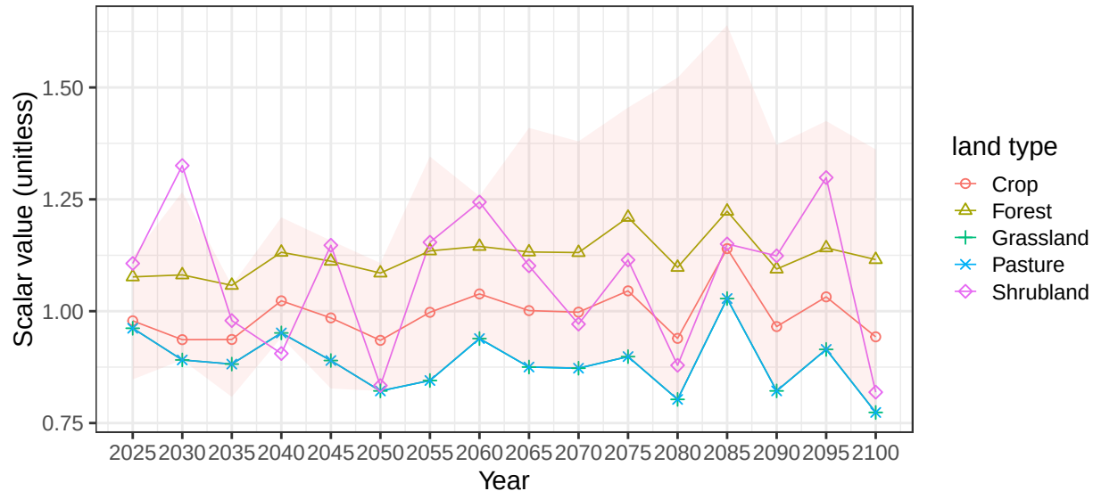
Region Australia_NZ basin AusCstN average soil scalars
