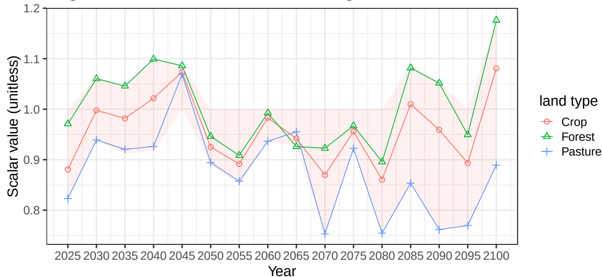
Region EU-12 basin DnkGrmCst average soil scalars
