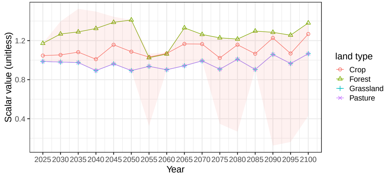
Region South Asia basin BengalBay average vegetation scalars
