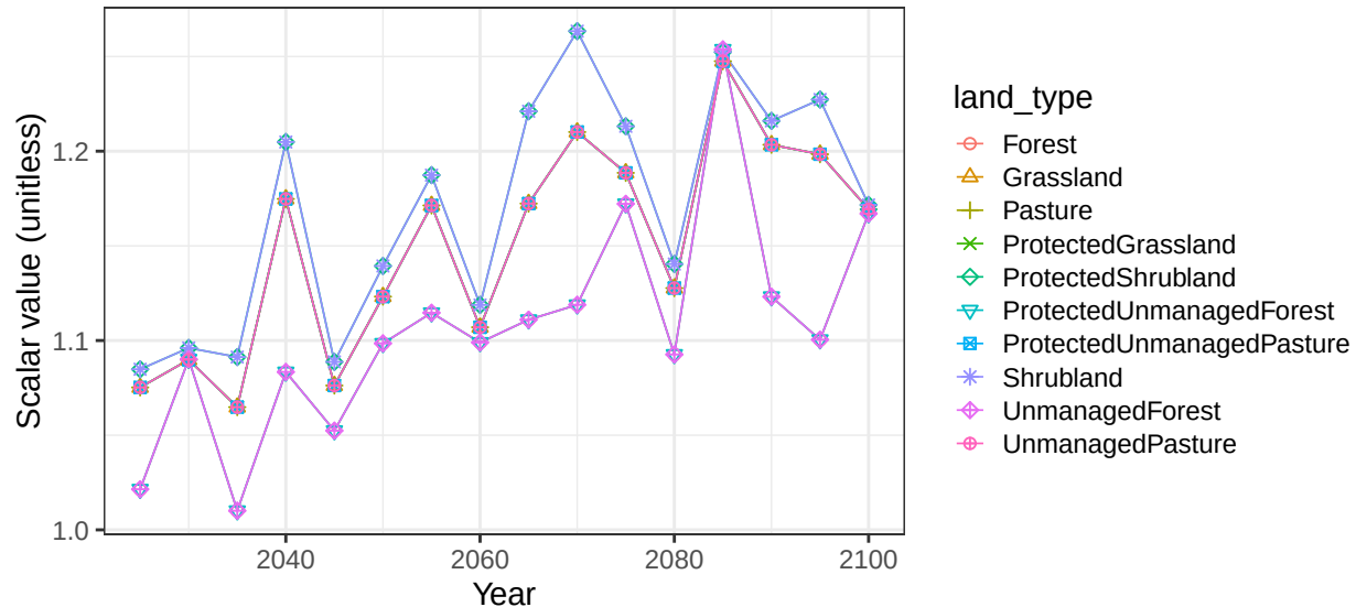
Region Canada basin Mackenzie non-crop vegetation scalars
