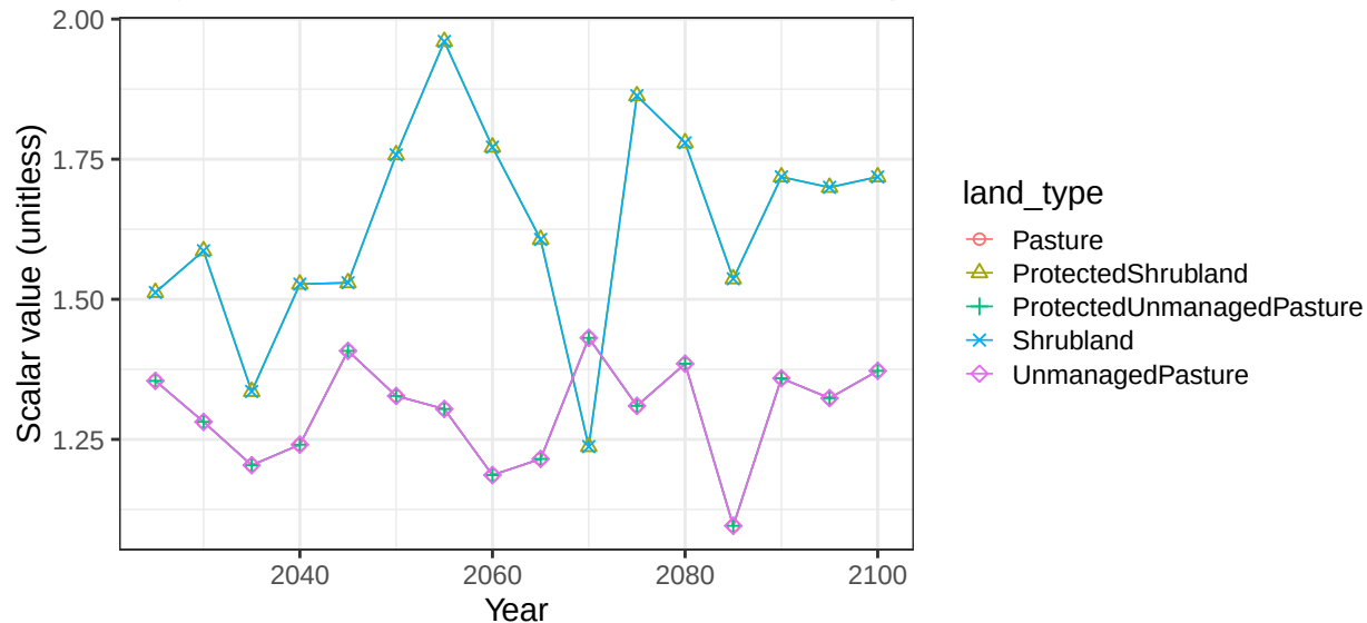
Region Pakistan basin HamuMashR non-crop vegetation scalars
