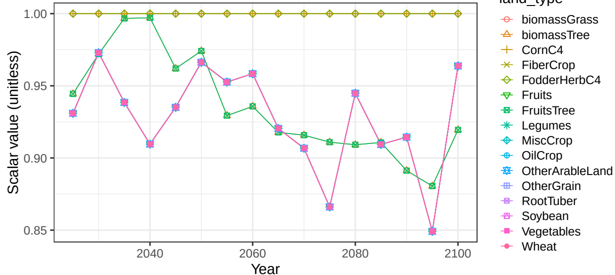
Region Canada basin UsaCstNE crop soil scalars
