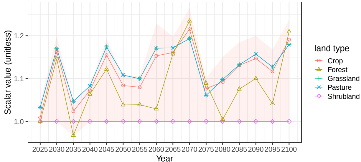
Region India basin CauveryR average soil scalars
