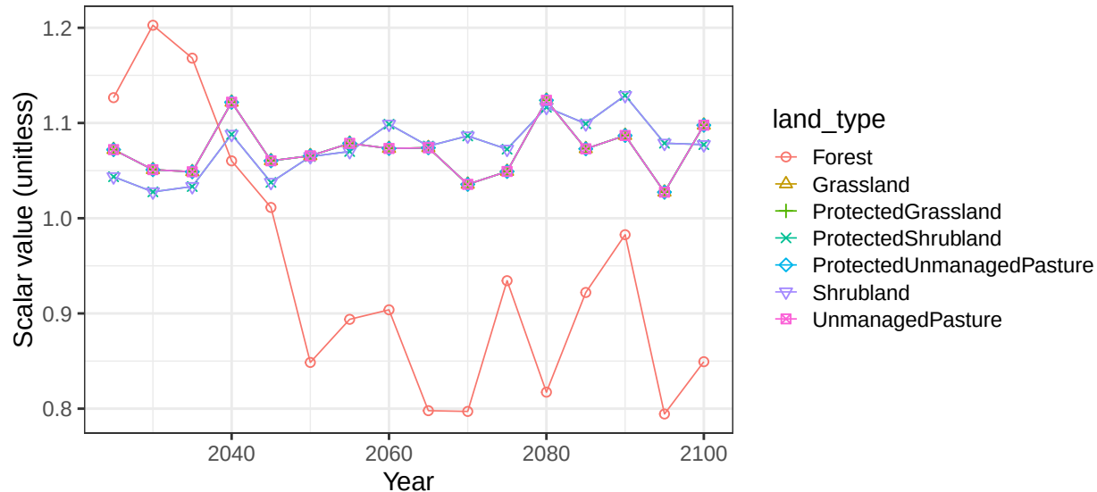
Region EU-15 basin RhoneR non-crop soil scalars
