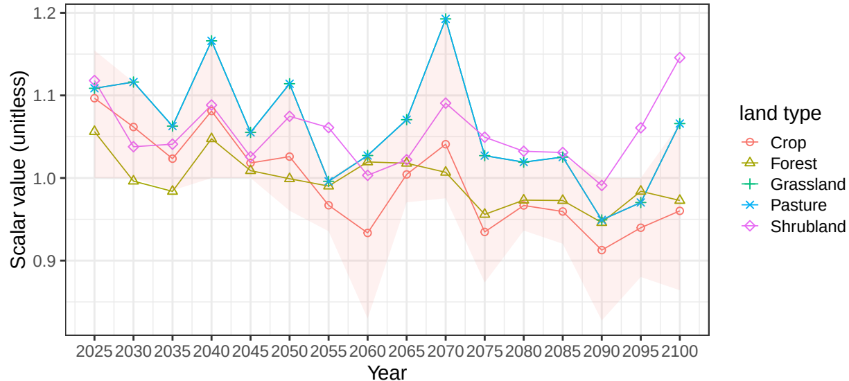
Region EU-15 basin IberiaCst average soil scalars
