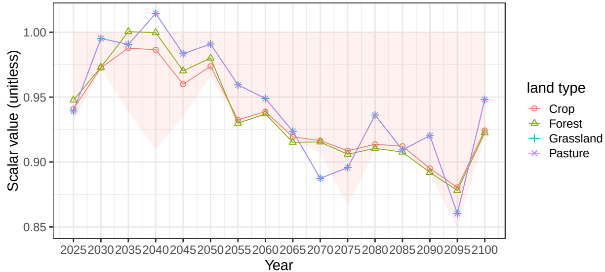
Region Canada basin UsaCstNE average soil scalars
