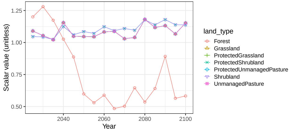
Region EU-15 basin RhoneR non-crop vegetation scalars
