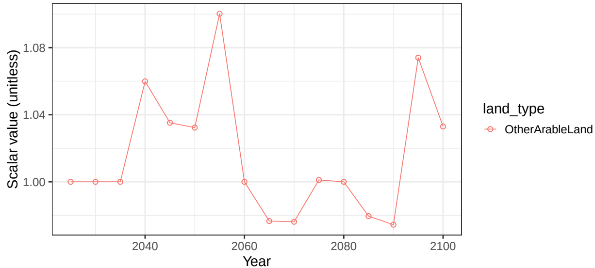
Region Russia basin BlackSeaS crop soil scalars
