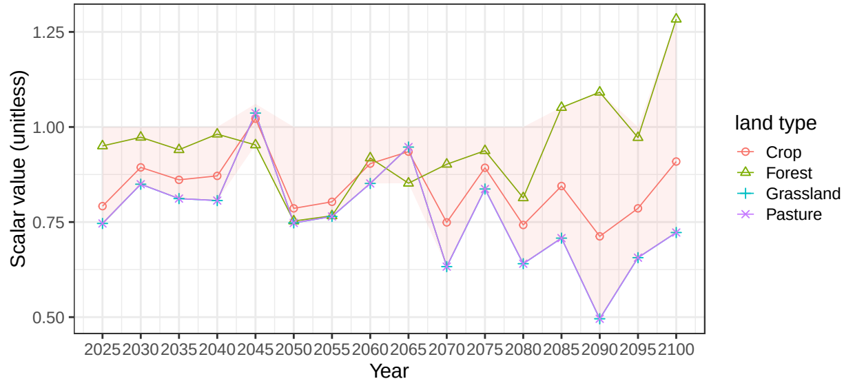
Region EU-15 basin OderR average vegetation scalars
