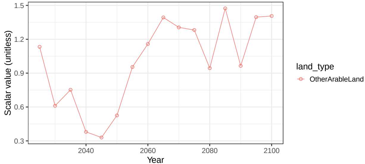
Region Pakistan basin Tarim crop vegetation scalars
