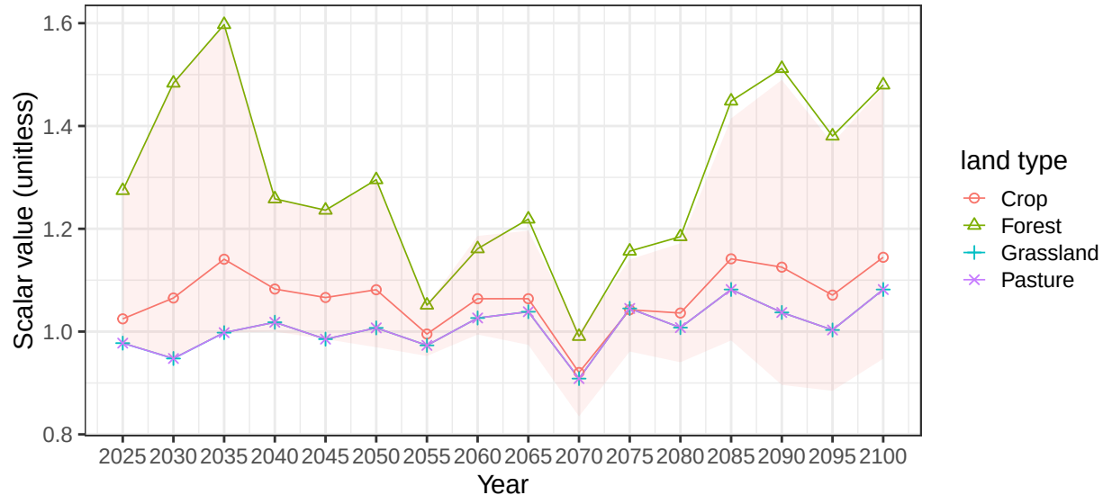
Region EU-15 basin RhineR average vegetation scalars
