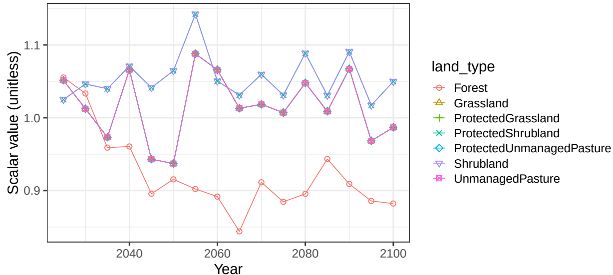
Region EU-15 basin ItalyCstE non-crop soil scalars
