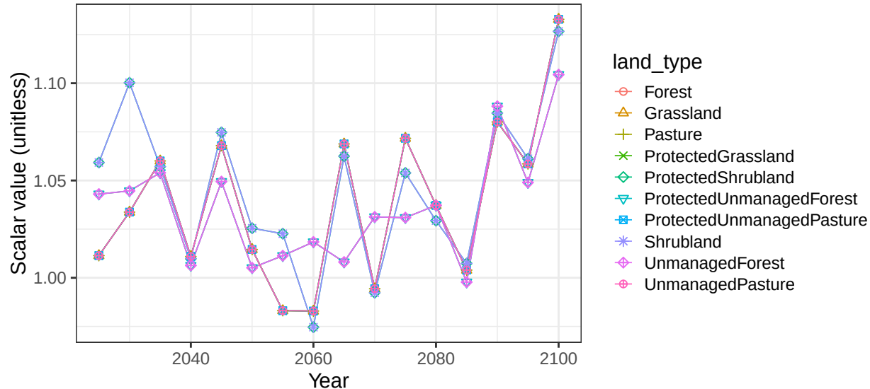
Region South Korea basin Korea non-crop vegetation scalars
