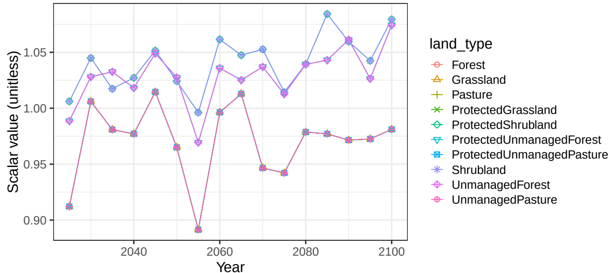
Region Southeast Asia basin IrrawaddyR non-crop soil scalars
