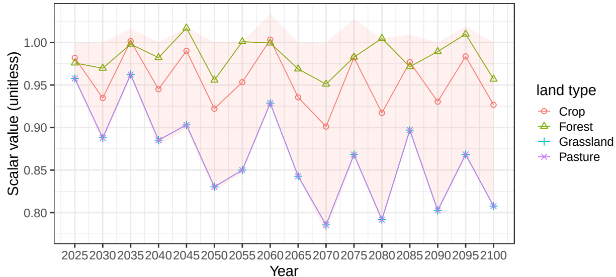
Region Indonesia basin JavaTimor average soil scalars
