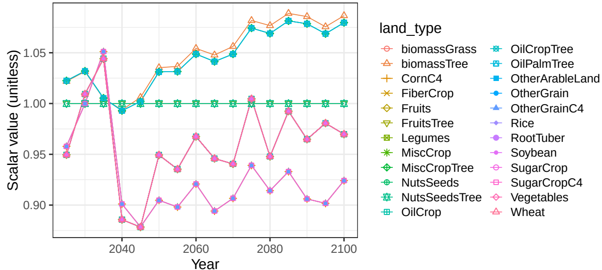
Region Colombia basin ColEcuacst crop vegetation scalars
