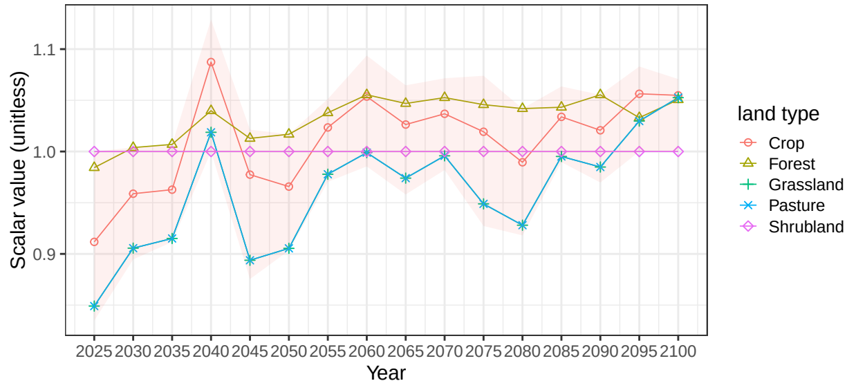
Region Brazil basin TocantinsR average soil scalars
