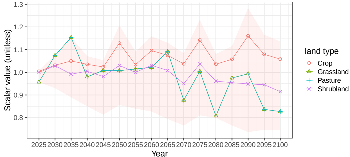
Region Middle East basin EJrdnSyr average soil scalars
