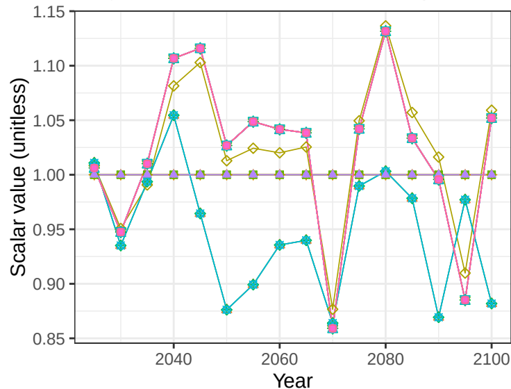
Region EU-15 basin SeineR crop soil scalars
