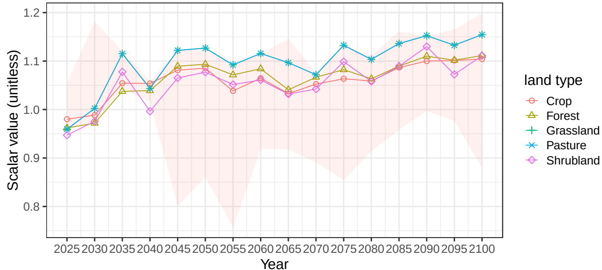
Region Russia basin RusCstSE average vegetation scalars
