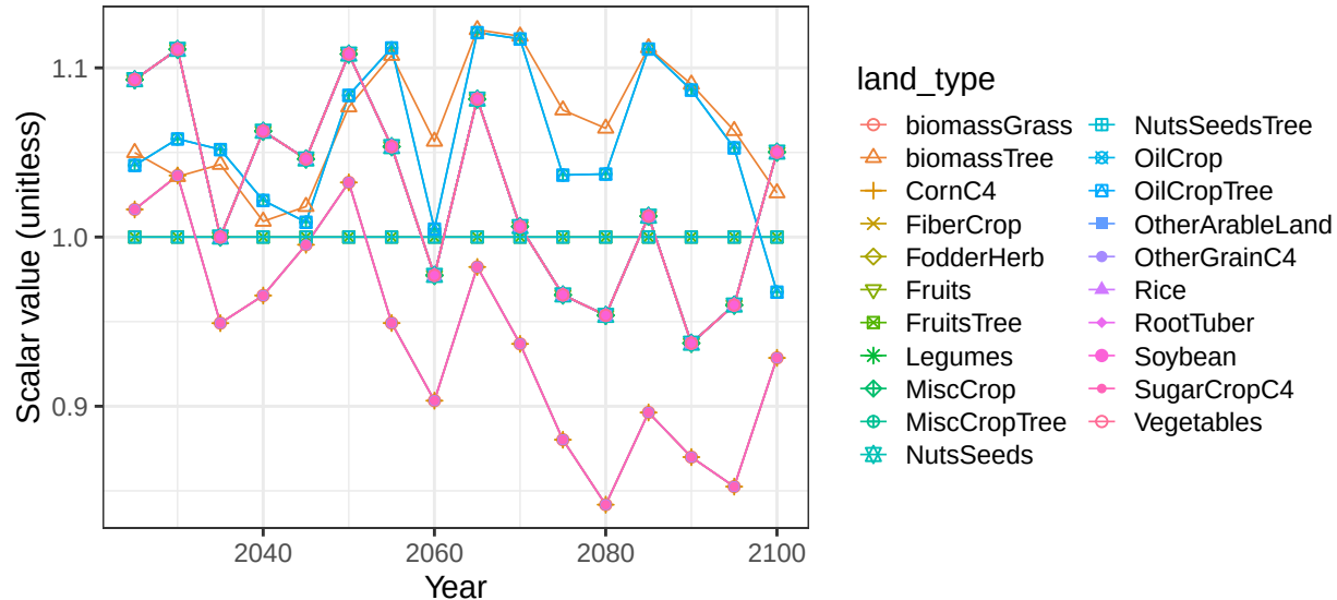
Region Southeast Asia basin SChinaSea crop soil scalars
