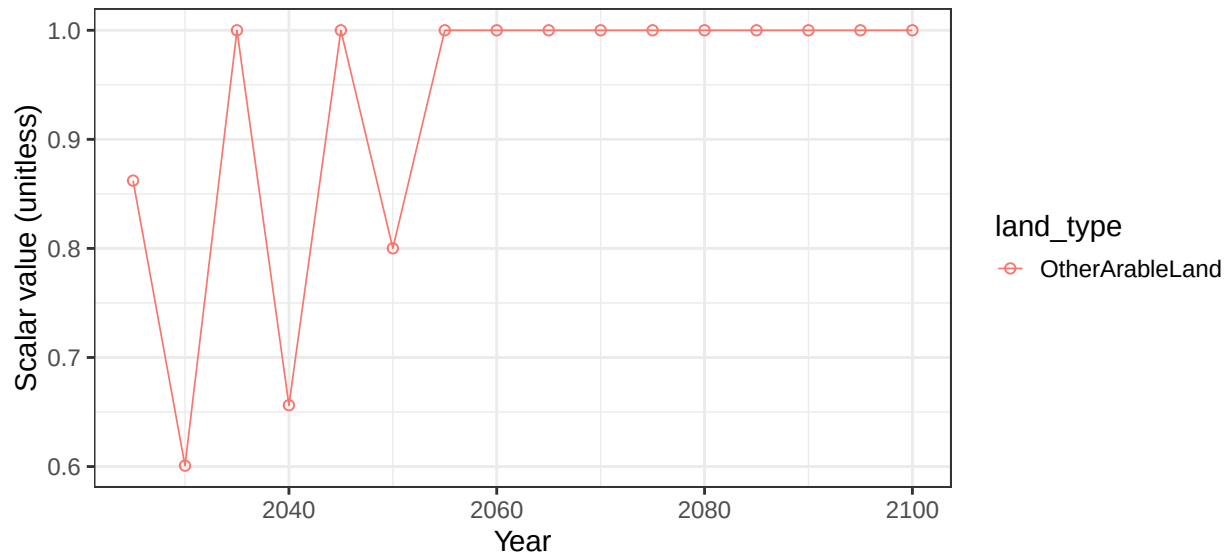
Region Africa_Northern basin DeadSea crop soil scalars
