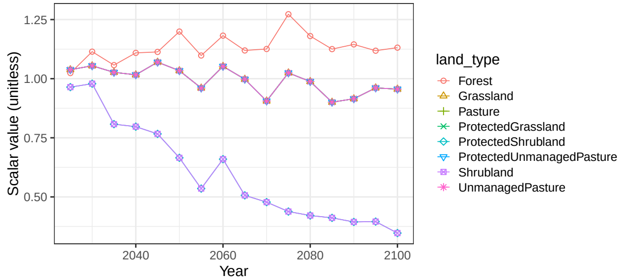
Region Africa_Eastern basin AfrCstNE non-crop soil scalars
