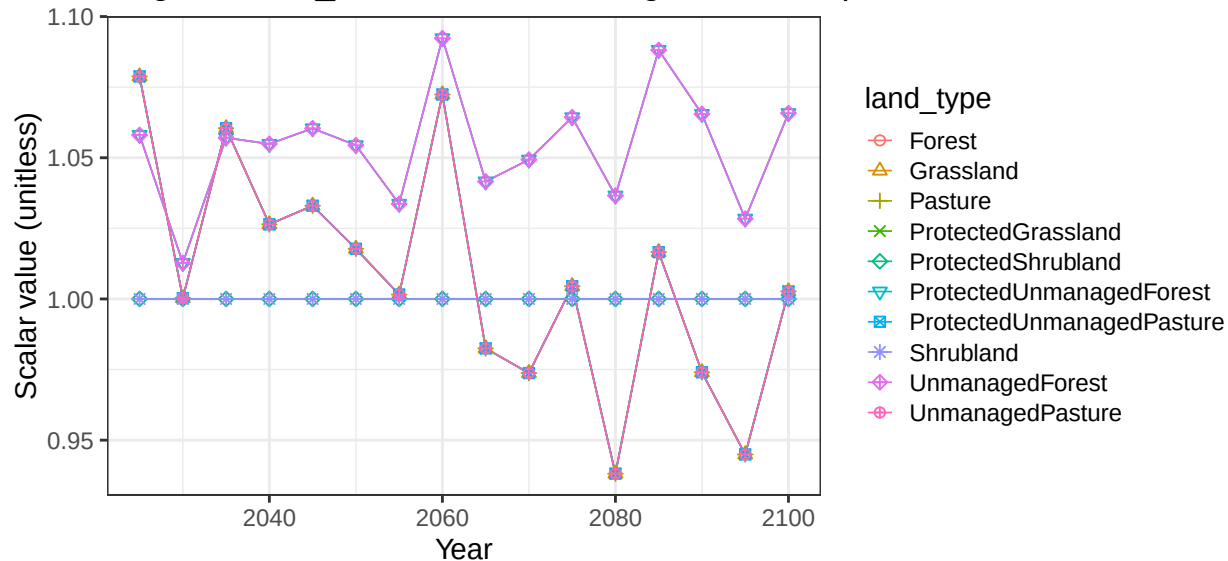
Region Africa_Southern basin CongoR non-crop soil scalars
