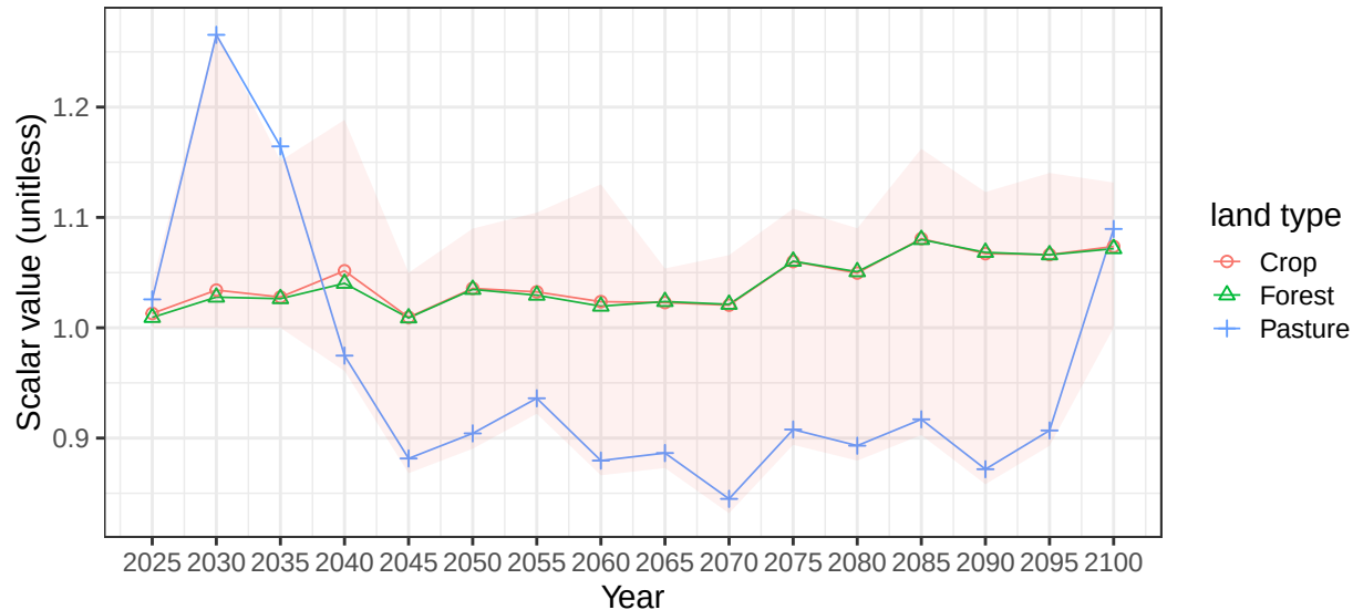
Region Southeast Asia basin Kalimantan average vegetation scalars
