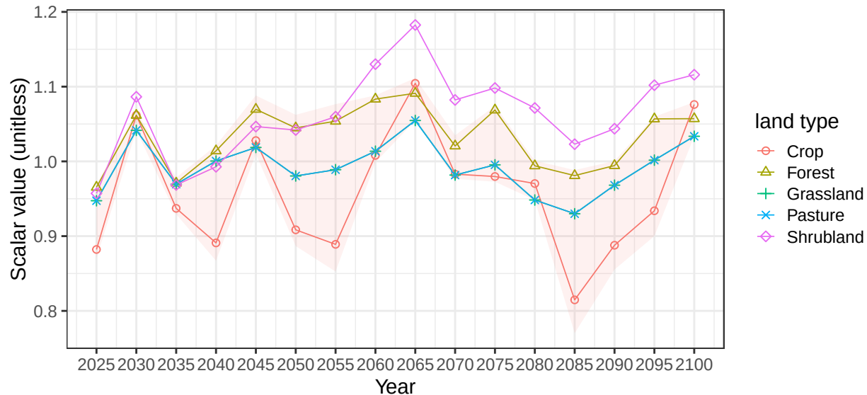
Region Russia basin CaspianNE average soil scalars
