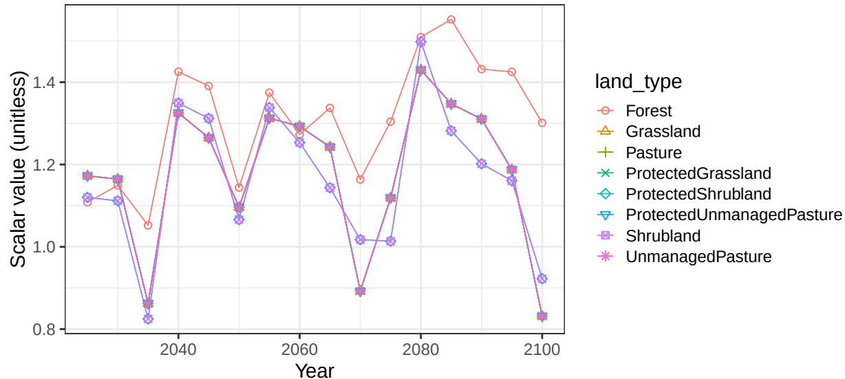
Region South Africa basin LimpopoR non-crop vegetation scalars
