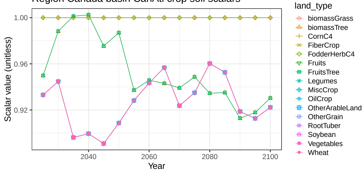
Region Canada basin CanAtl crop soil scalars
