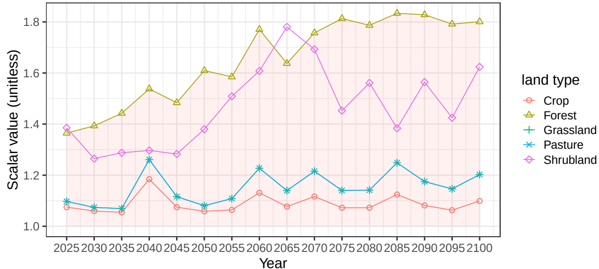
Region Brazil basin BrzCstE average vegetation scalars
