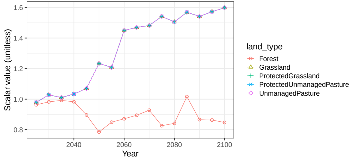
Region EU-15 basin NevaR non-crop soil scalars
