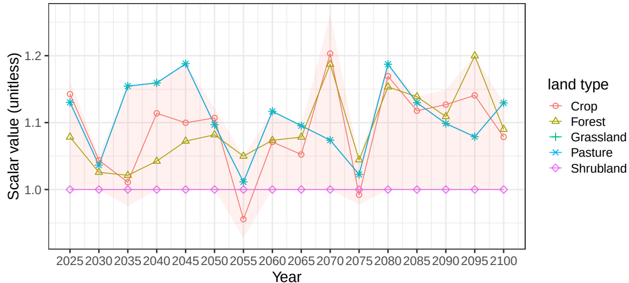
Region Southeast Asia basin ThaiGulf average vegetation scalars
