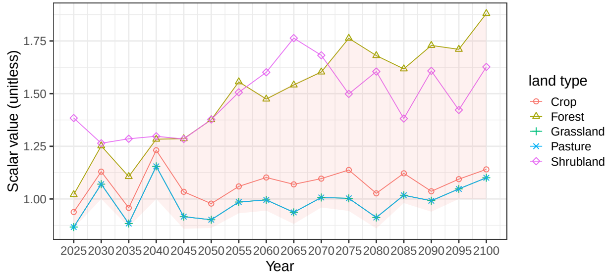
Region Brazil basin SaoFrancR average vegetation scalars
