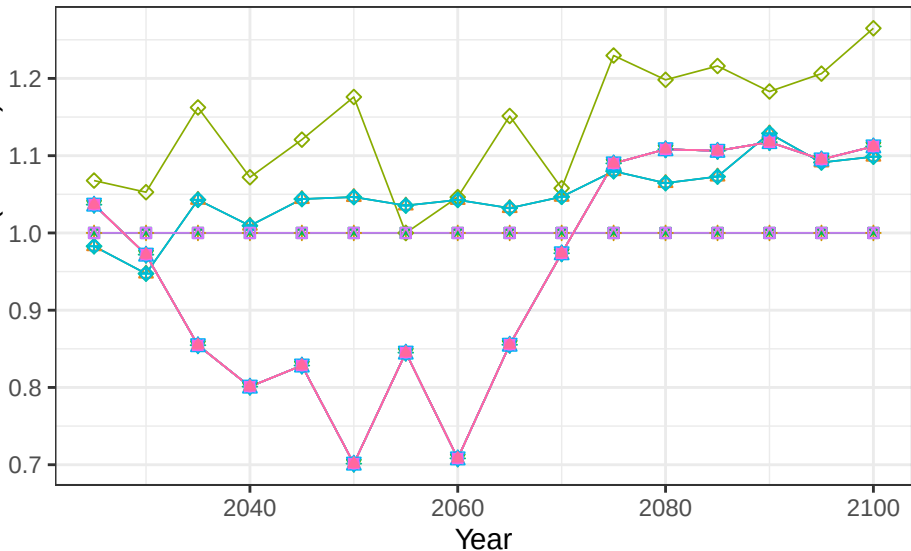
Region Russia basin SiberiaW crop vegetation scalars
