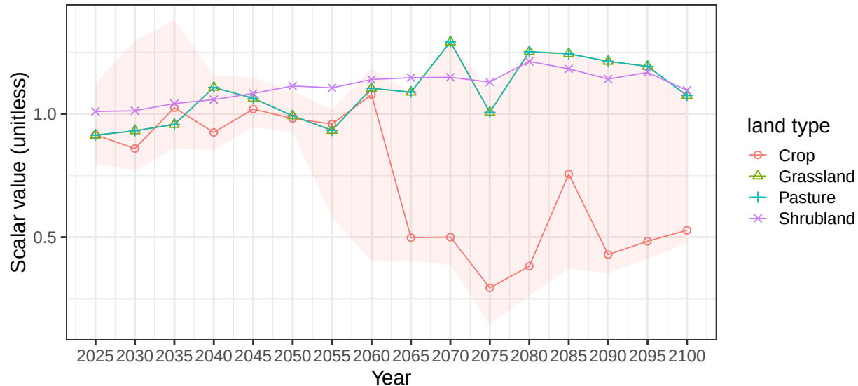
Region China basin IndusR average vegetation scalars
