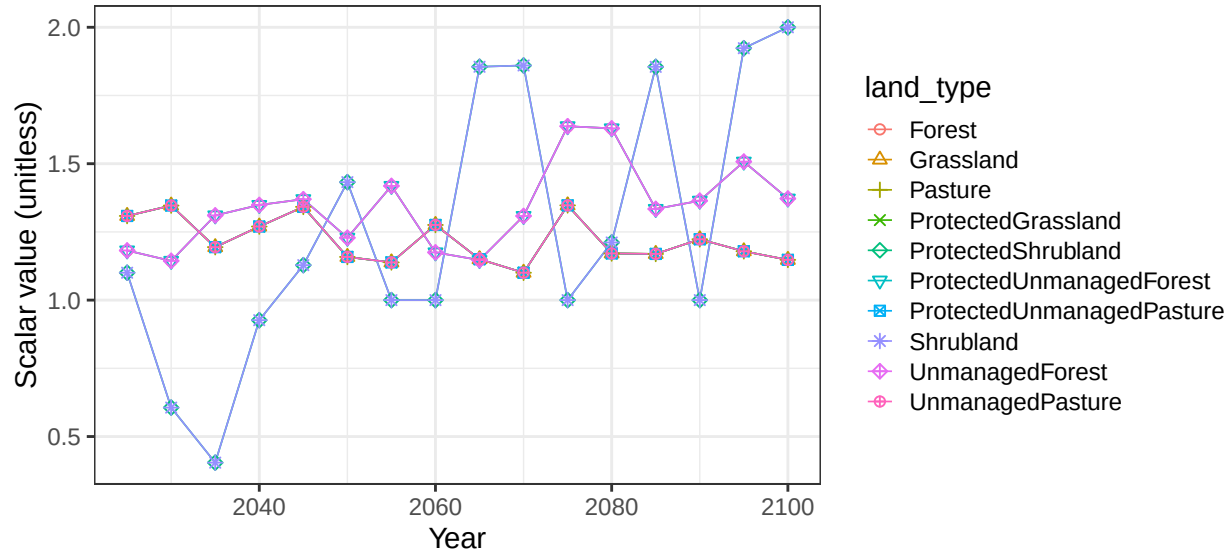
Region Mexico basin MexBaja non-crop vegetation scalars
