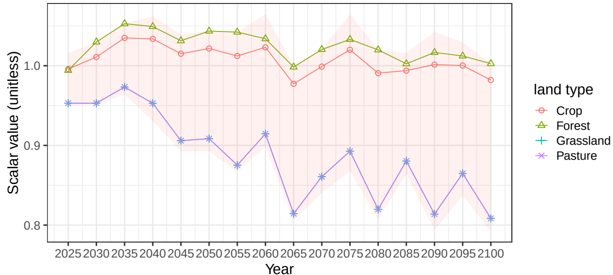
Region Indonesia basin IdnE average soil scalars
