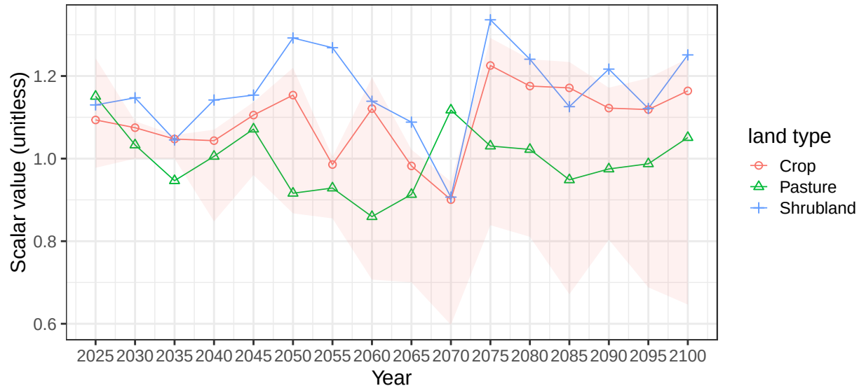
Region Pakistan basin Helmand average soil scalars
