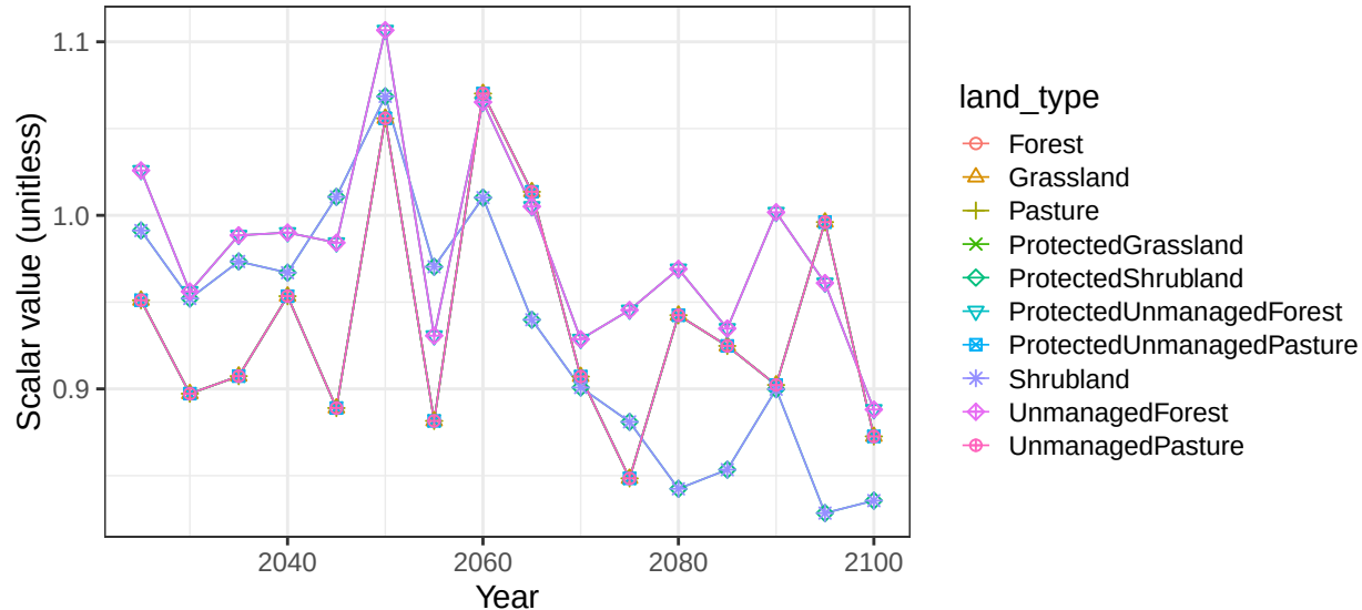
Region Central Asia basin AmurR non-crop soil scalars
