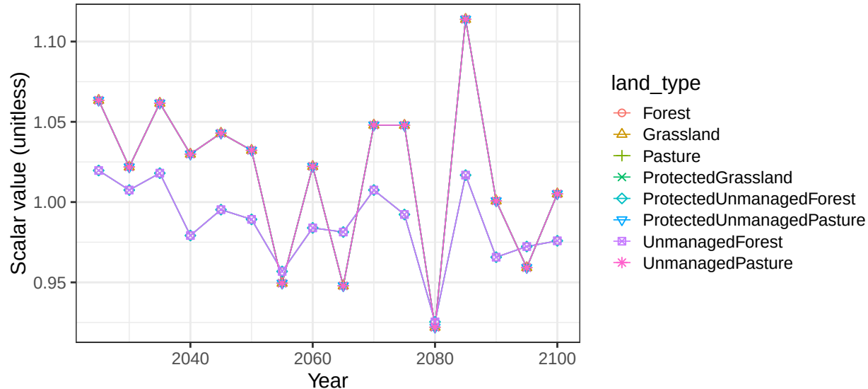
Region USA basin OhioR non-crop soil scalars
