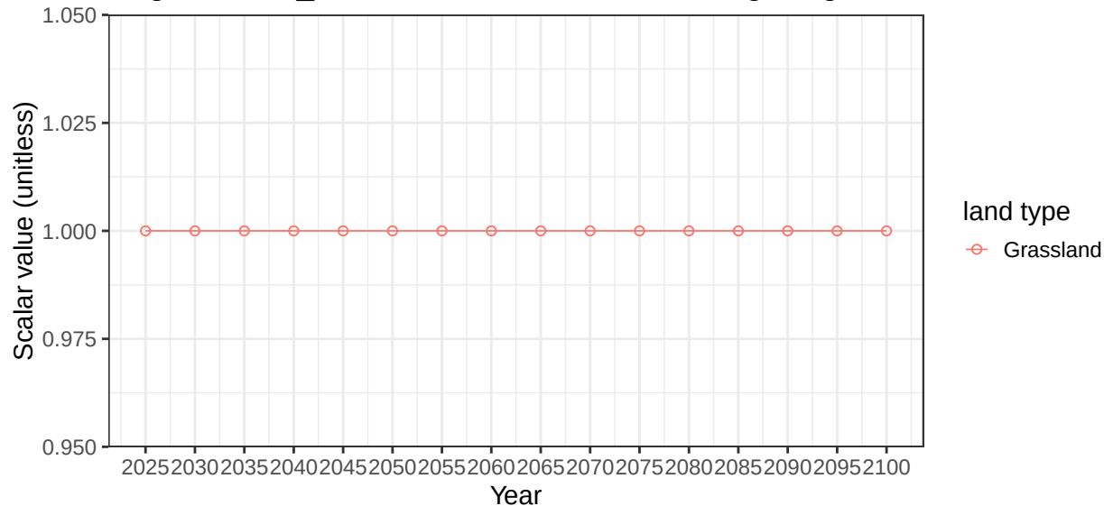
Region Africa_Northern basin AfrCstNE average vegetation scalars
