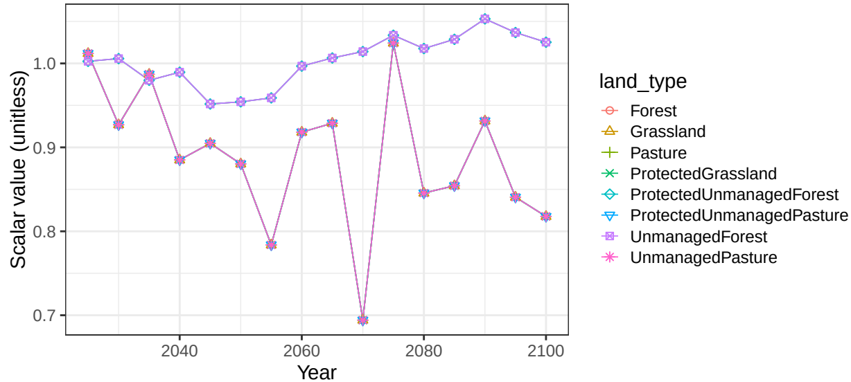
Region Southeast Asia basin IrianJaya non-crop vegetation scalars
