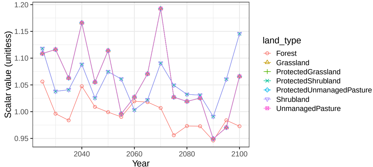
Region EU-15 basin IberiaCst non-crop soil scalars
