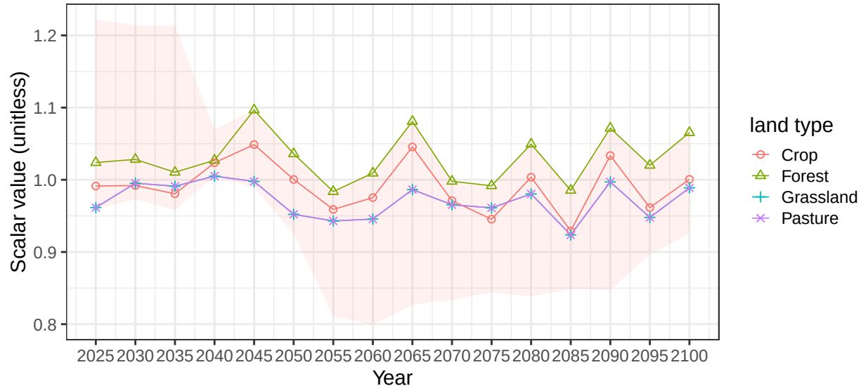
Region Southeast Asia basin BengalBay average soil scalars
