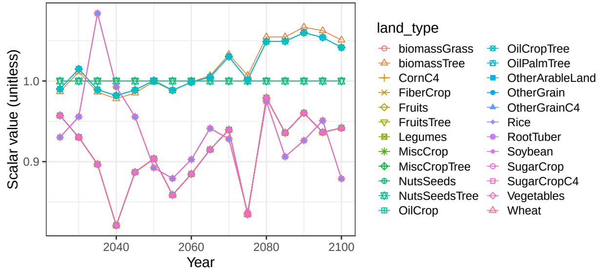
Region Colombia basin SAmerCstN crop vegetation scalars
