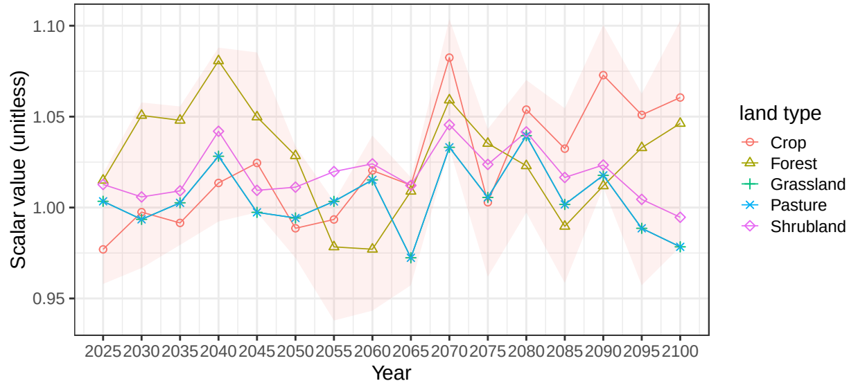
Region China basin GangesR average soil scalars
