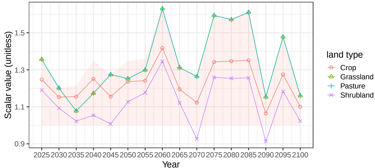
Region Middle East basin Helmand average vegetation scalars
