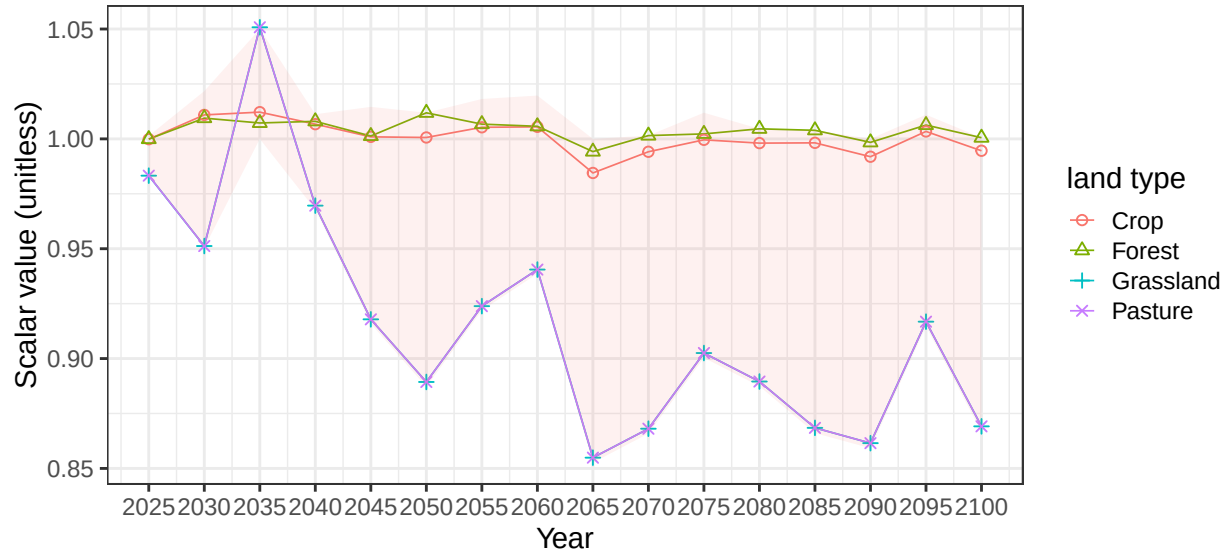
Region Indonesia basin Kalimantan average soil scalars
