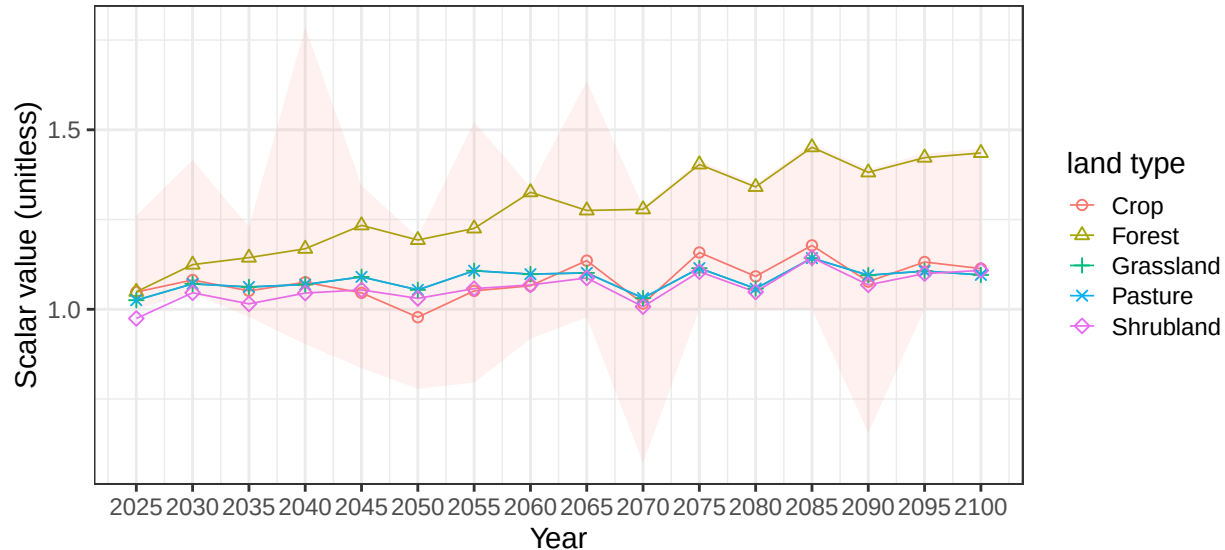
Region Argentina basin ChileCstS average vegetation scalars
