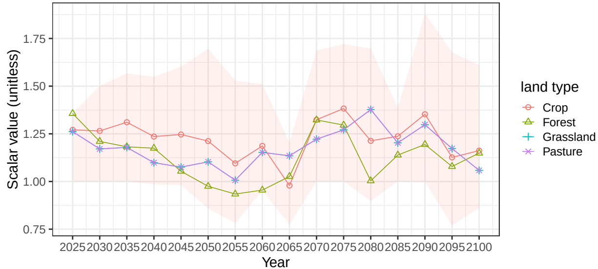
Region USA basin MissppRN average vegetation scalars
