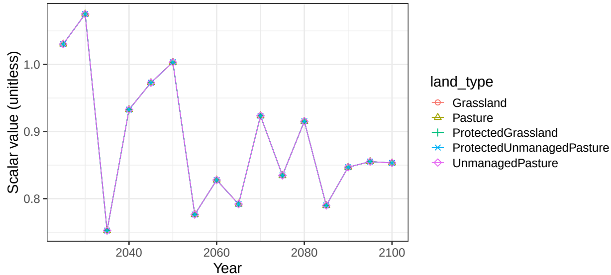
Region USA basin Hawaii non-crop soil scalars
