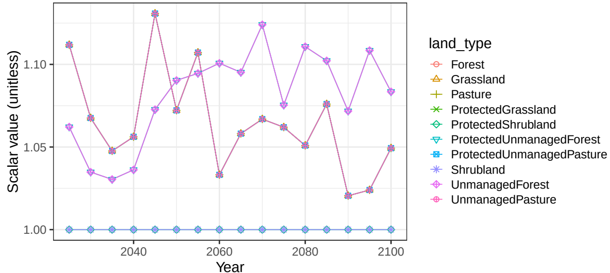
Region Southeast Asia basin VietnamCst non-crop soil scalars
