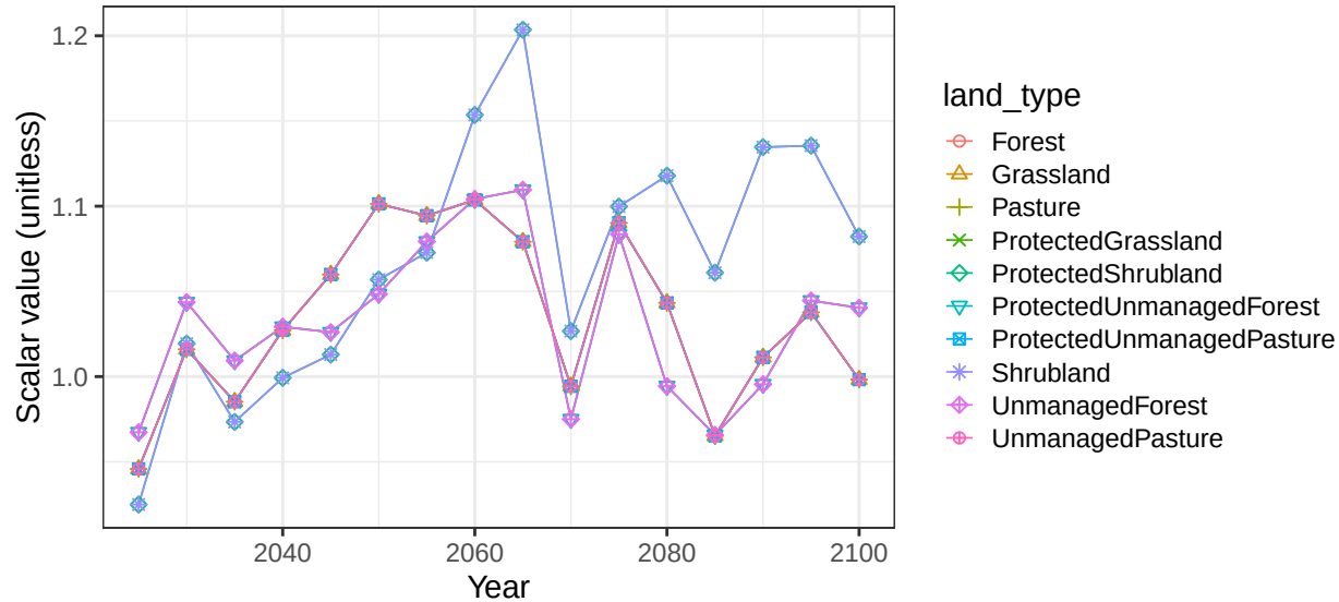
Region Central Asia basin CaspianSW non-crop soil scalars
