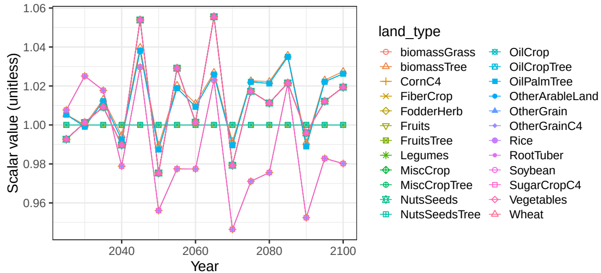
Region Central America and Caribbean basin YucatanP crop soil scalars
