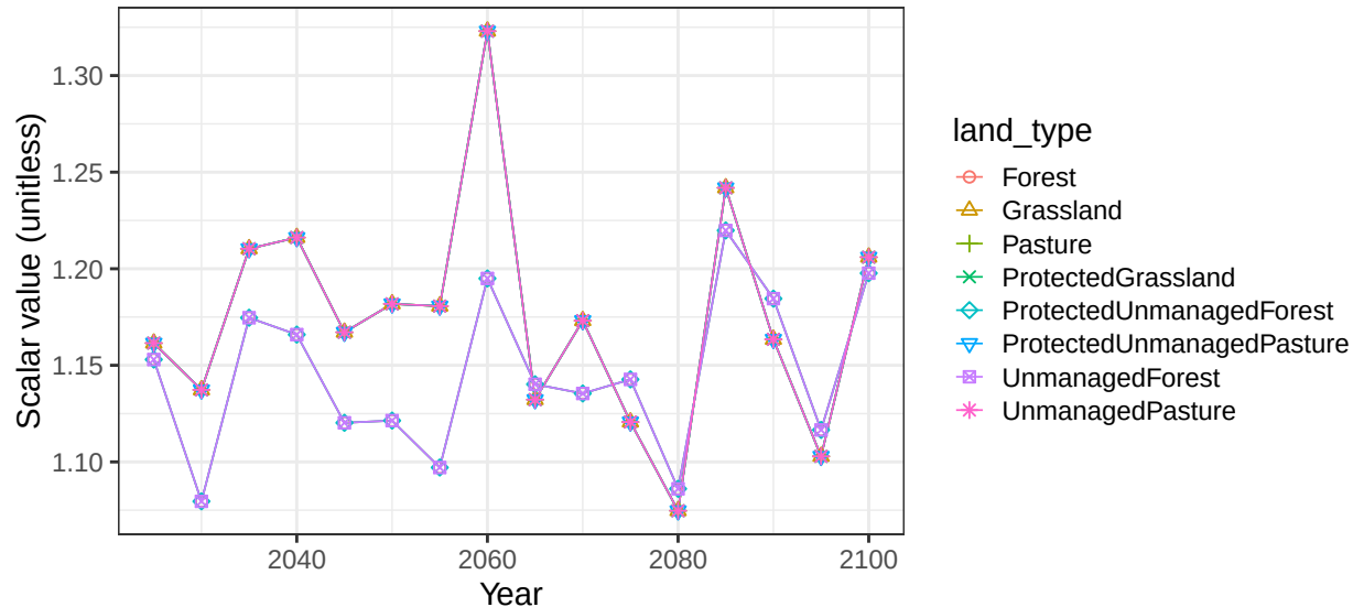
Region Africa_Western basin ZambeziR non-crop vegetation scalars
