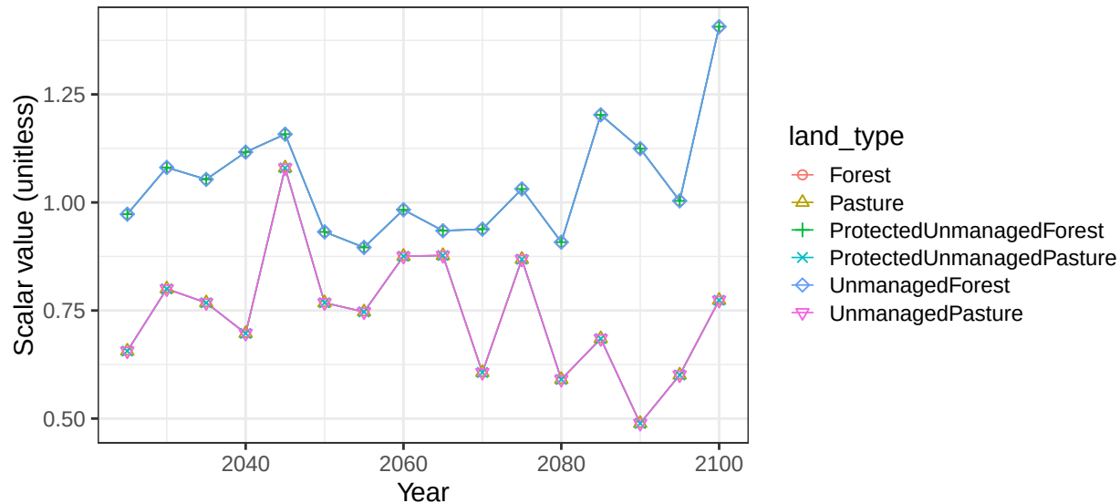
Region EU-12 basin DnkGrmCst non-crop vegetation scalars
