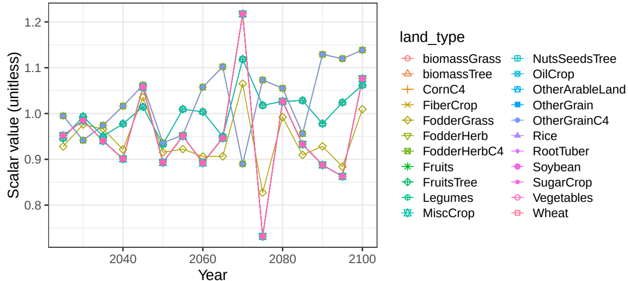
Region Russia basin VolgaR crop soil scalars
