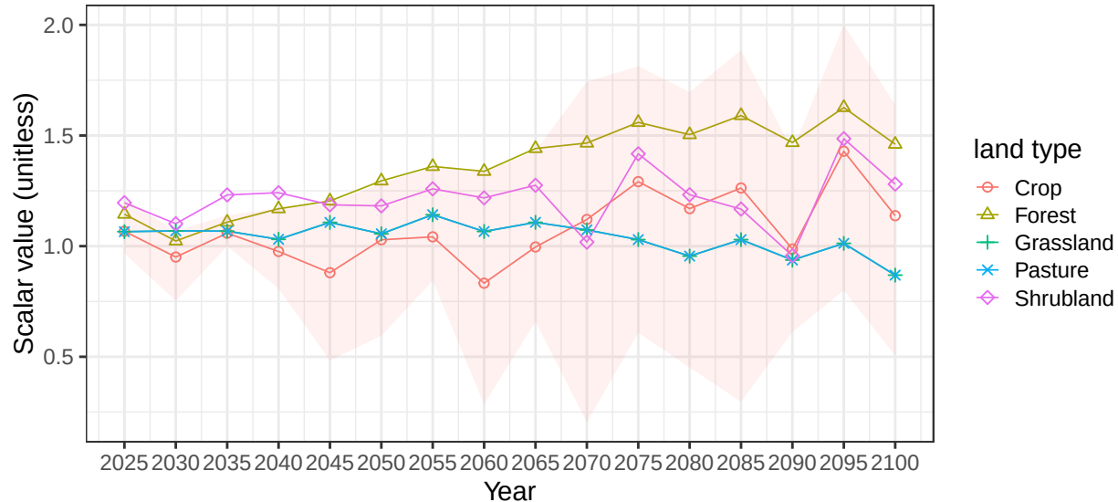
Region Argentina basin NegroR average vegetation scalars
