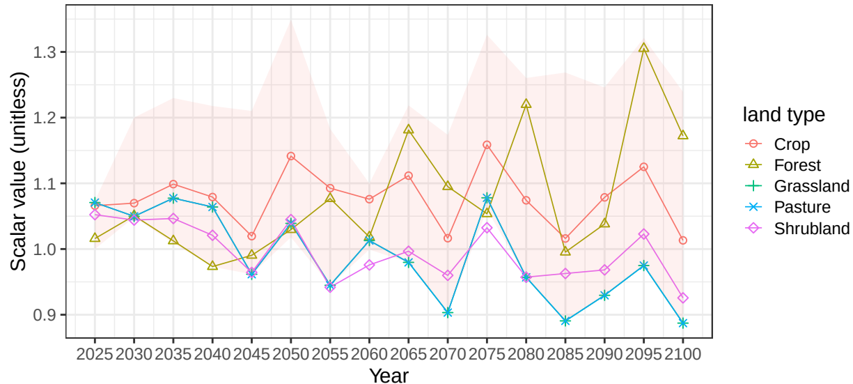
Region Middle East basin Iran average soil scalars
