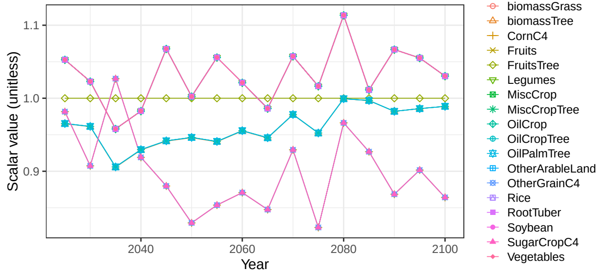
Region Central America and Caribbean basin ColEcuacSt land use Vegetation s
