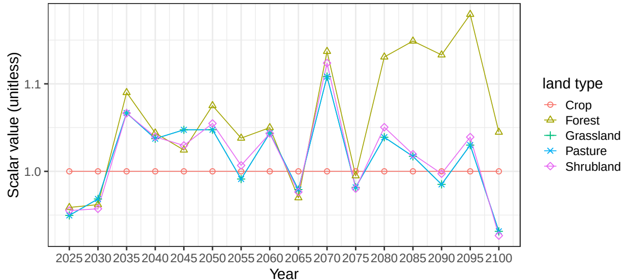
Region Russia basin KaraSea average soil scalars
