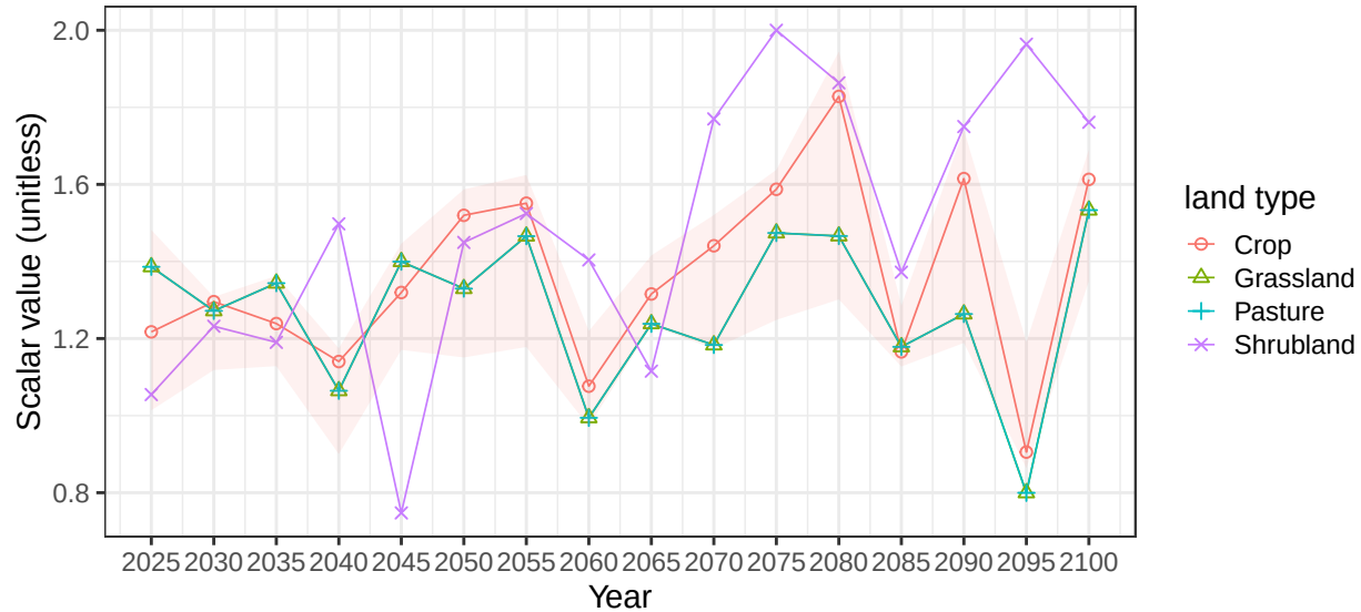
Region Central Asia basin UralR average vegetation scalars
