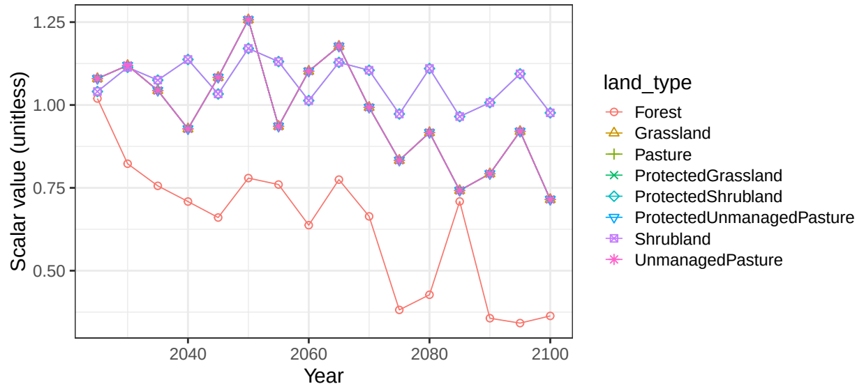
Region Africa_Northern basin AfrCstNW non-crop soil scalars
