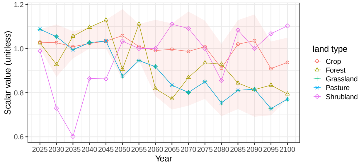
Region Mexico basin MexBaja average soil scalars
