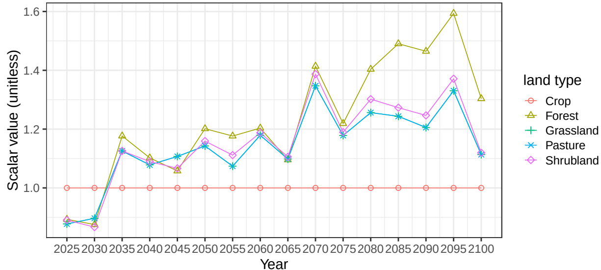
Region Russia basin KaraSea average vegetation scalars
