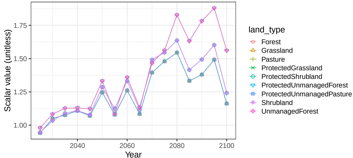
Region Russia basin SiberiaN non-crop vegetation scalars
