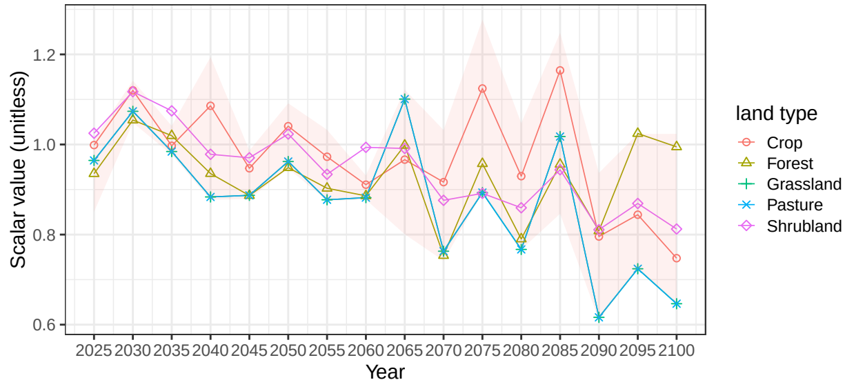
Region Argentina basin MarChiq average soil scalars
