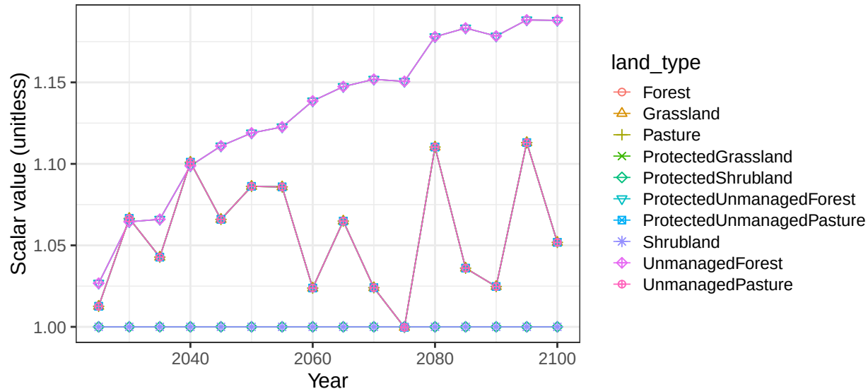
Region Africa_Western basin GuineaGulf non-crop vegetation scalars
