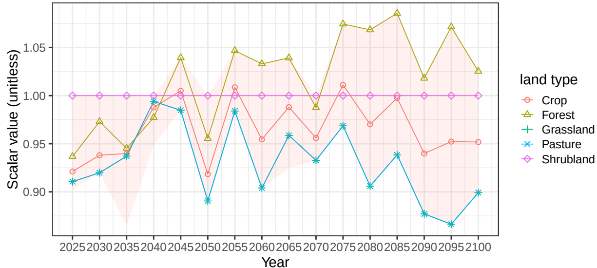
Region Mexico basin YucatanP average soil scalars
