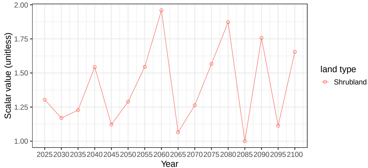
Region European Free Trade Association basin ArcticIsl average vegetation
