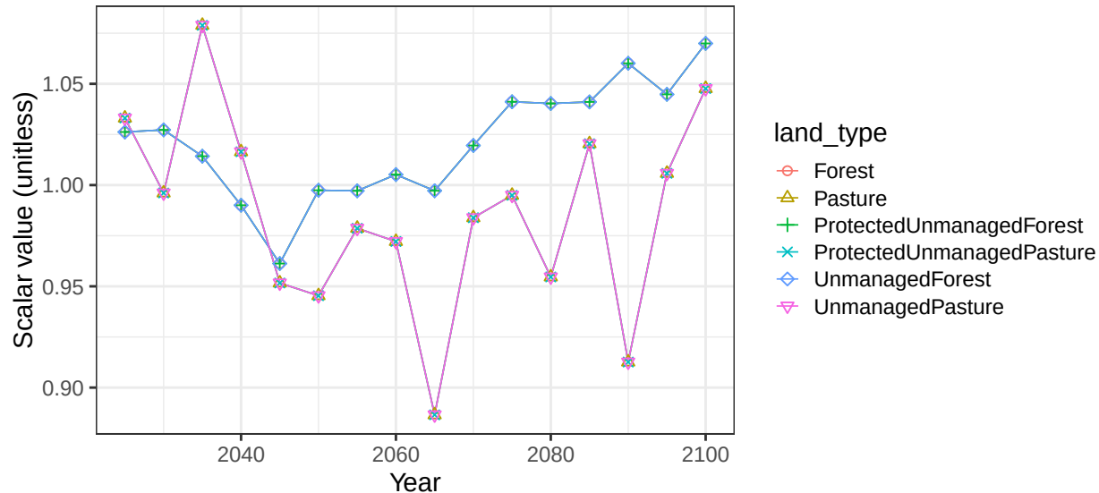
Region Indonesia basin FlyR non-crop vegetation scalars
