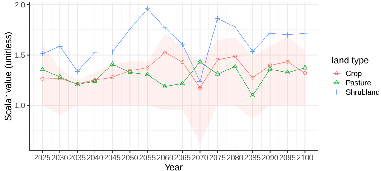
Region Pakistan basin HamuMashR average vegetation scalars
