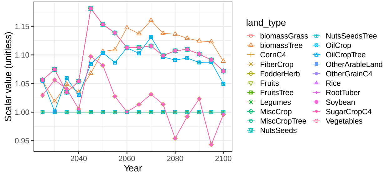
Region Southeast Asia basin Hong crop soil scalars
