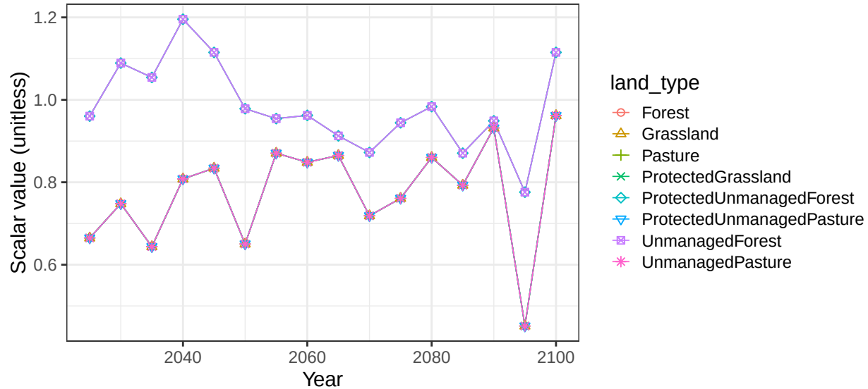
Region EU-12 basin WislaR non-crop vegetation scalars
