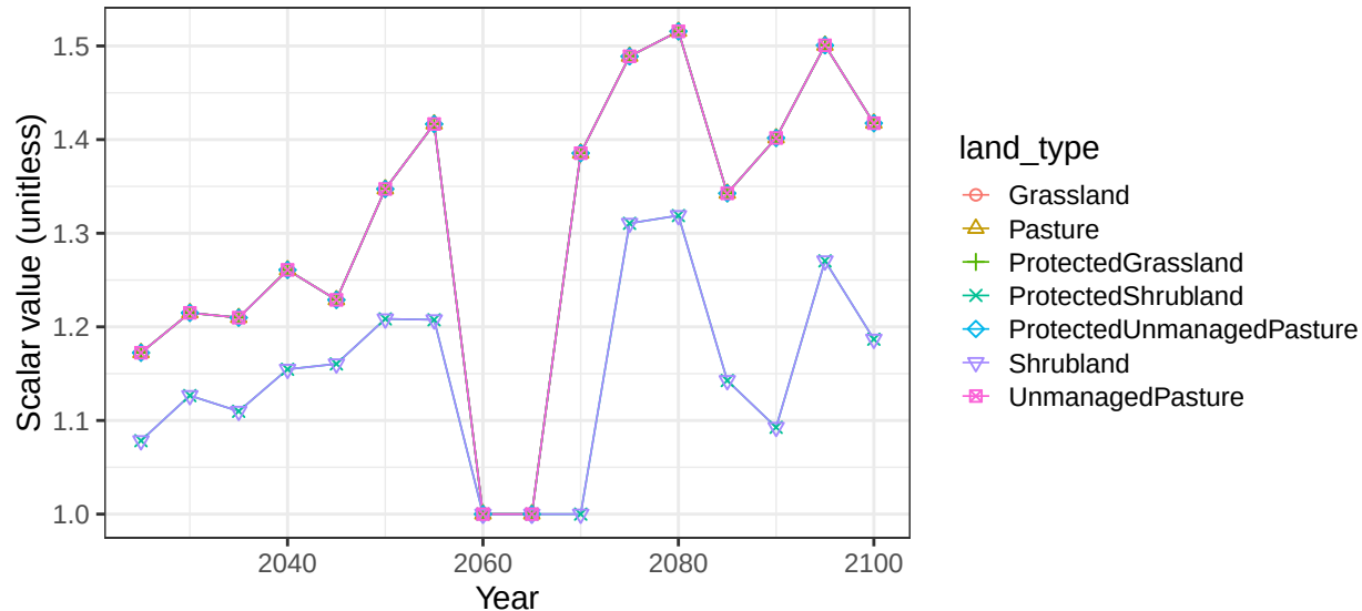
Region Middle East basin HamuMashR non-crop vegetation scalars
