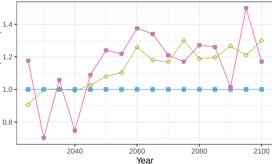
Region Russia basin Finland crop soil scalars
