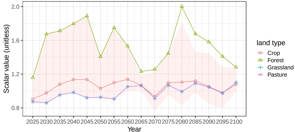
Region EU-15 basin EmsWeserR average vegetation scalars
