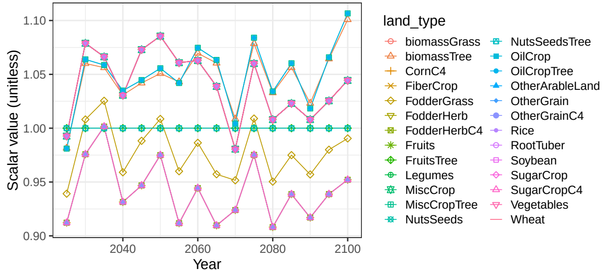
Region Mexico basin RioBalsas crop soil scalars
