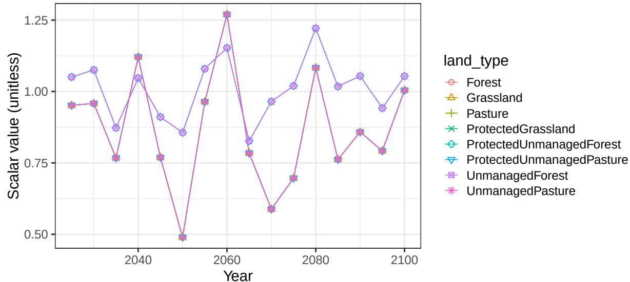
Region Europe_Non_EU basin DanubeR non-crop vegetation scalars
