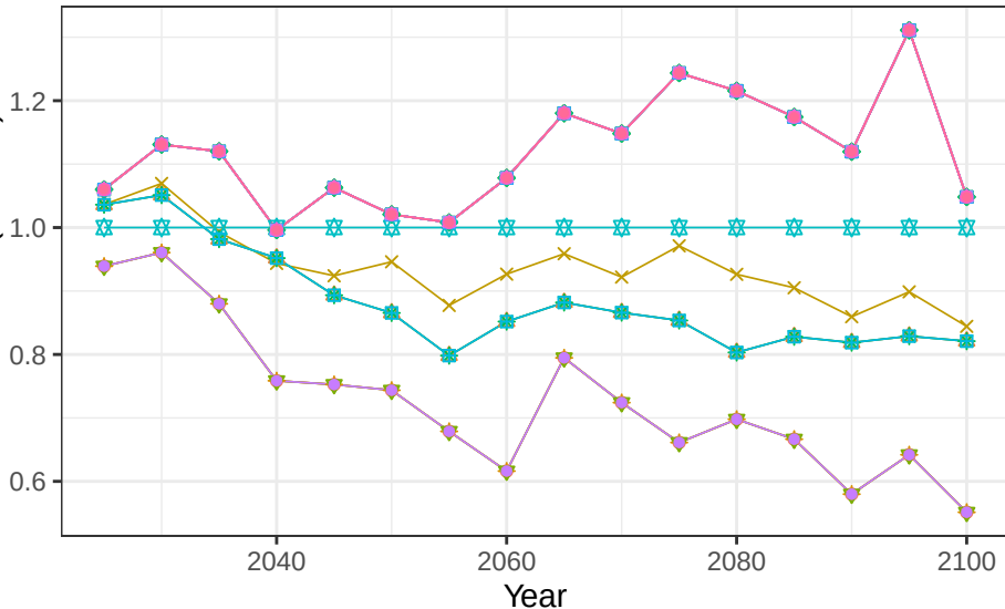
Region USA basin GreatBasin crop soil scalars
