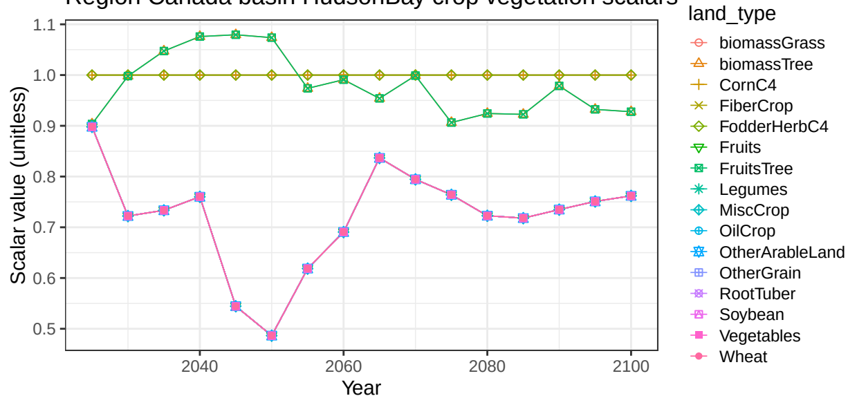
Region Canada basin HudsonBay crop vegetation scalars
