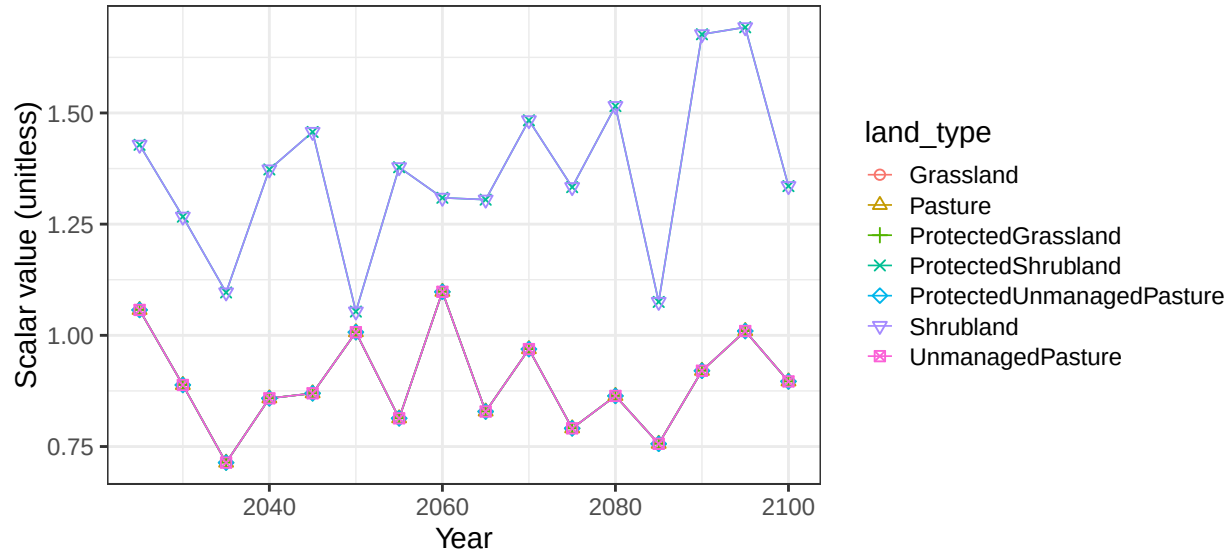
Region Pakistan basin ArabianSea non-crop vegetation scalars
