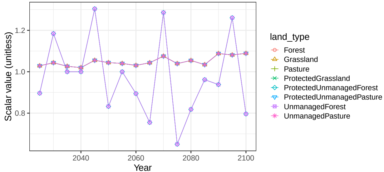
Region European Free Trade Association basin DanubeR non-crop soil sca
