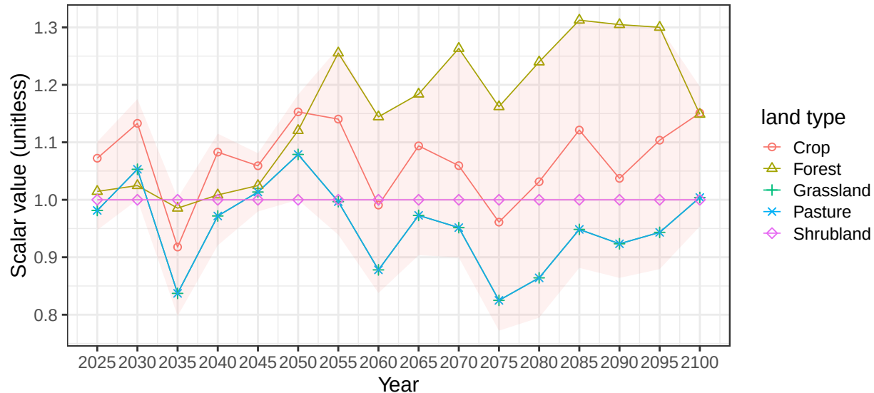
Region Southeast Asia basin SChinaSea average vegetation scalars
