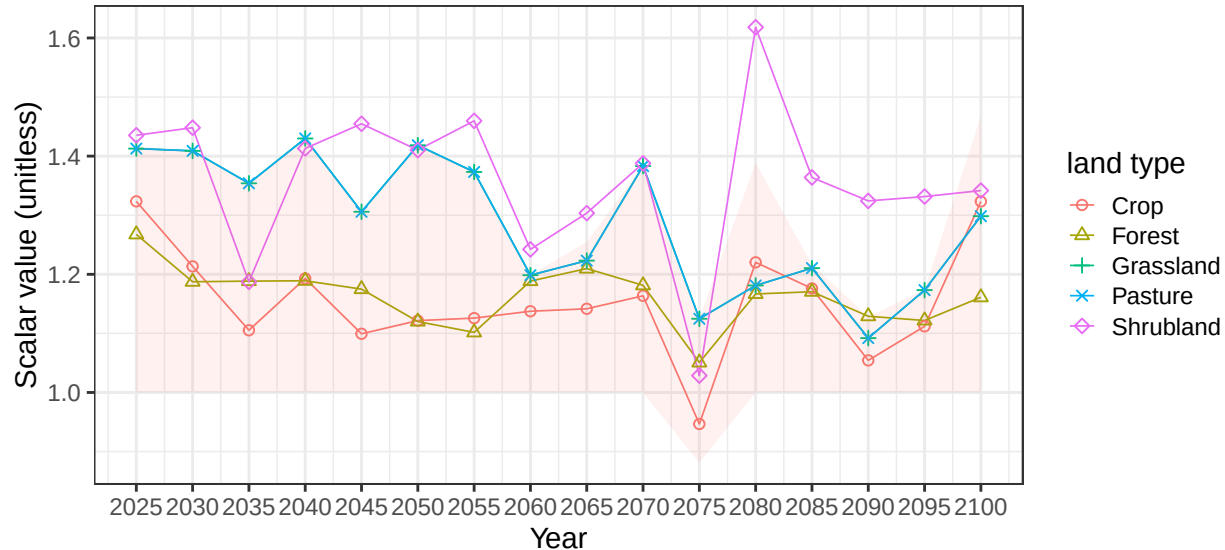
Region EU-15 basin TagusR average vegetation scalars
