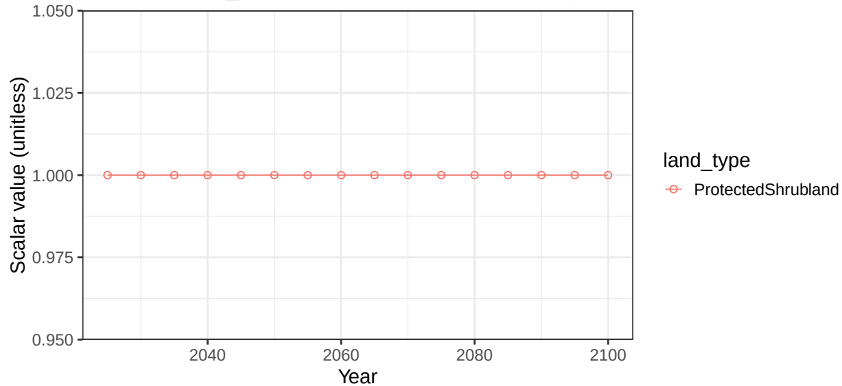
Region Africa_Northern basin LChad non-crop vegetation scalars
