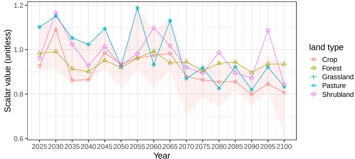
Region Australia_NZ basin AusCstW average soil scalars
