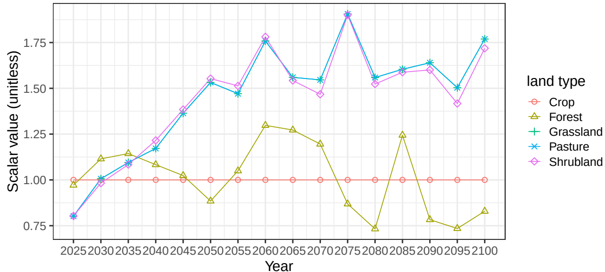
Region EU-15 basin ScndnvN average vegetation scalars
