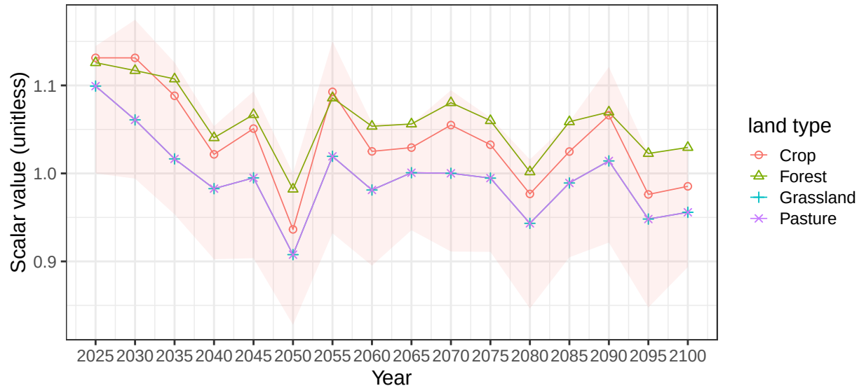
Region USA basin MissppRS average soil scalars
