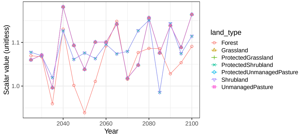
Region EU-15 basin Gironde non-crop vegetation scalars
