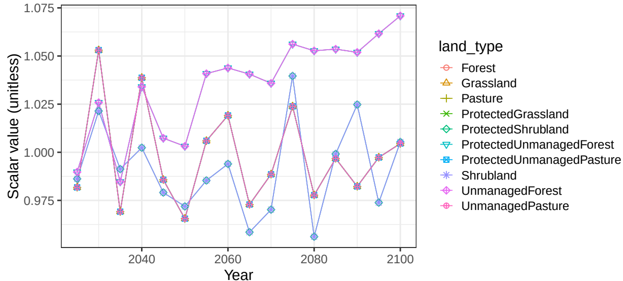
Region Brazil basin BrzCstS non-crop soil scalars
