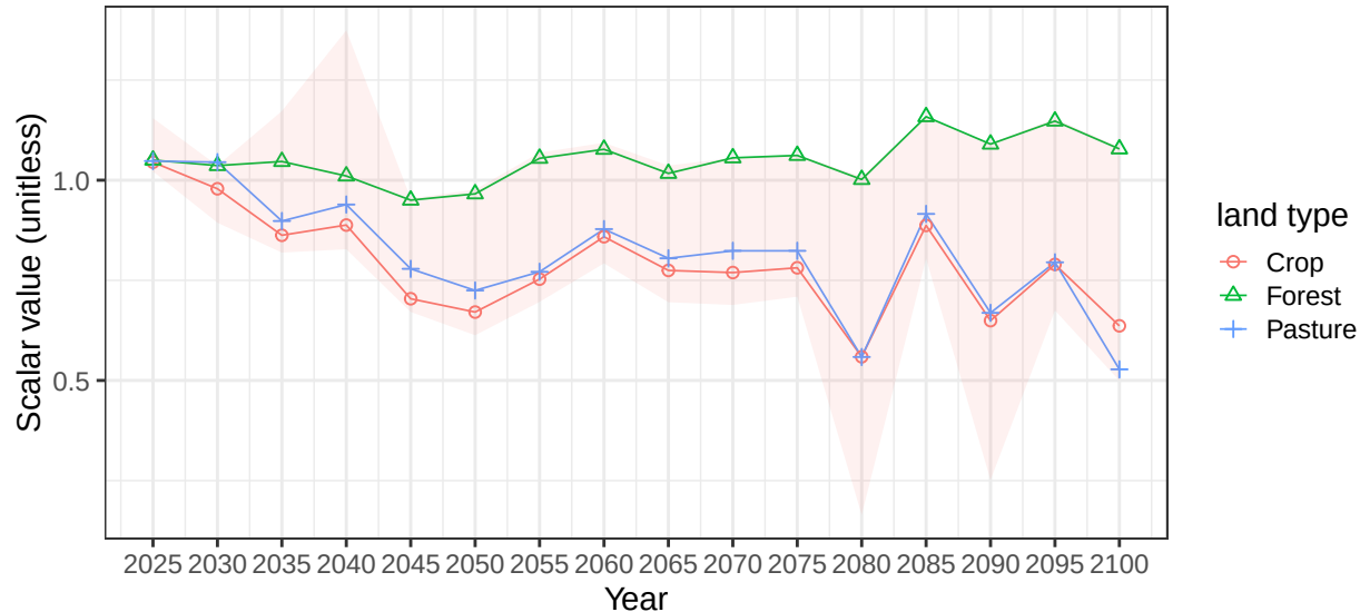
Region Southeast Asia basin IdnE average vegetation scalars
