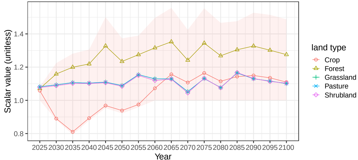
Region South America_Southern basin ArgCstS average vegetation scalars
