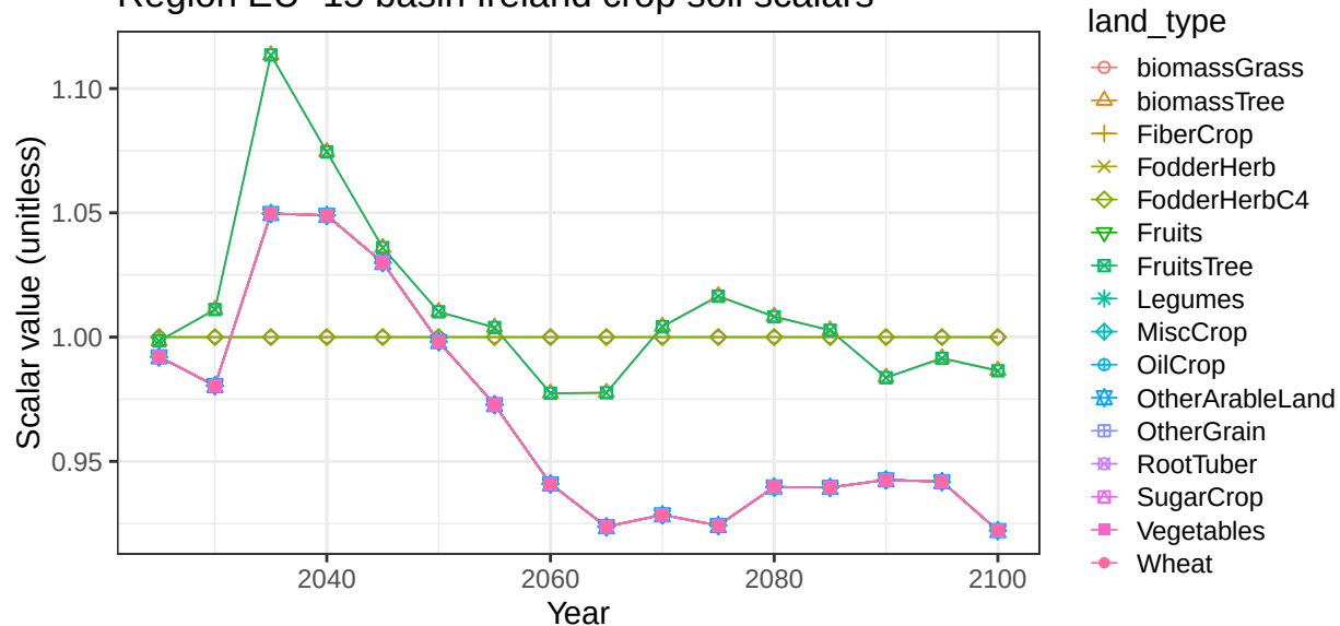
Region EU-15 basin Ireland crop soil scalars
