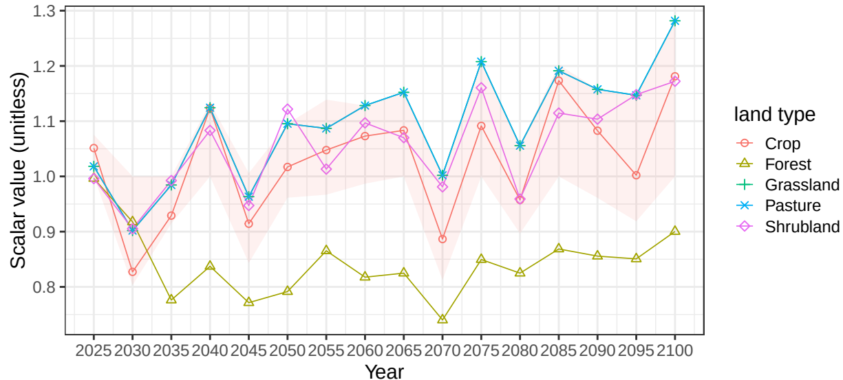
Region China basin HuangHeR average vegetation scalars
