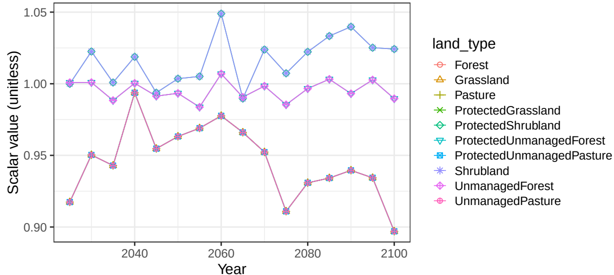
Region Brazil basin AmazonR non-crop soil scalars
