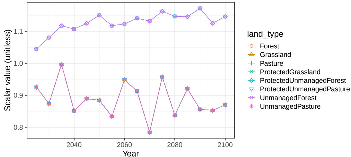
Region Indonesia basin Sulawesi non-crop vegetation scalars
