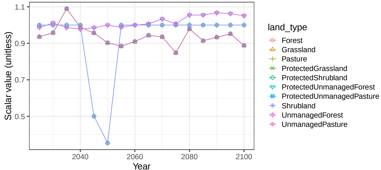
Region Colombia basin SAmerCstN non-crop vegetation scalars
