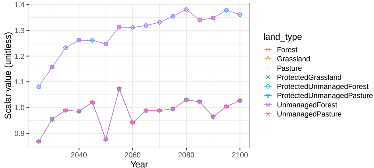
Region Africa_Southern basin GuineaGulf non-crop vegetation scalars
