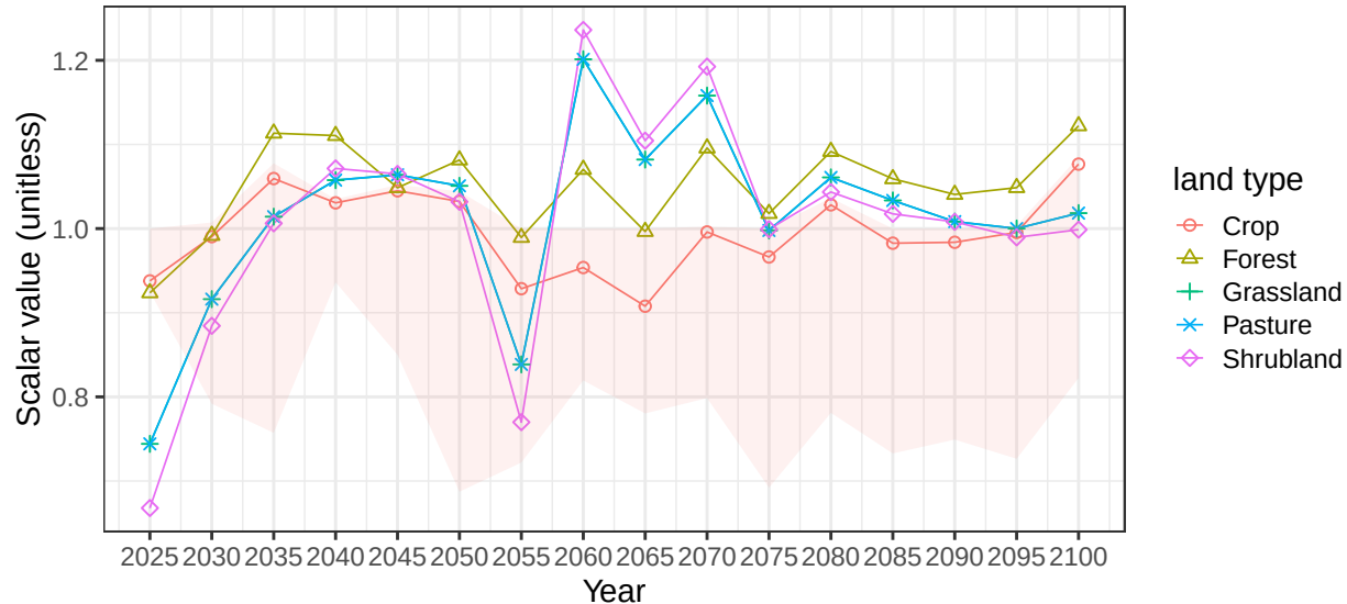
Region Canada basin StLwrncR average vegetation scalars
