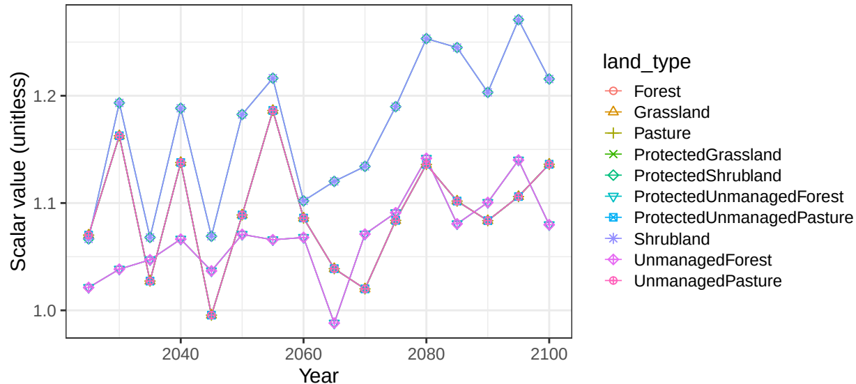
Region Taiwan basin Taiwan non-crop vegetation scalars
