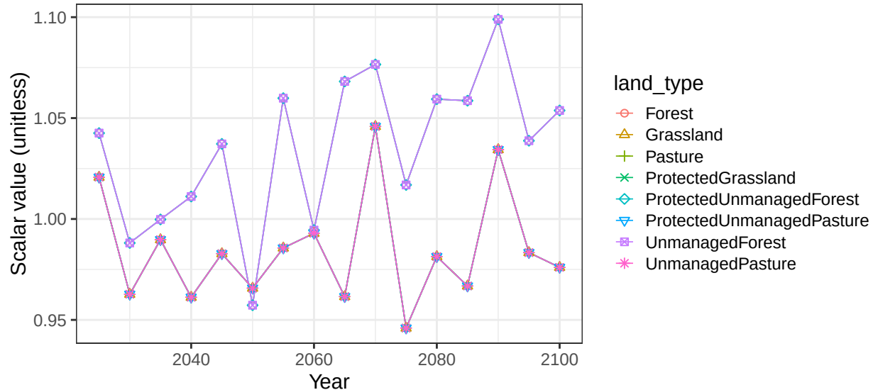
Region South Asia basin SriLanka non-crop soil scalars
