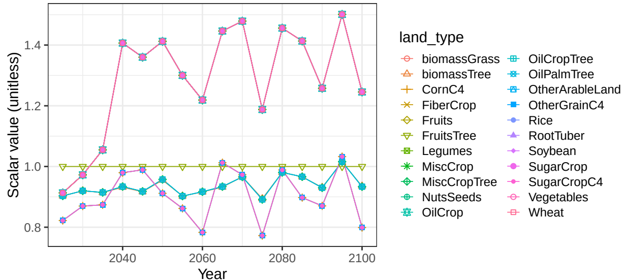
Region South America_Northern basin OrinocoR crop vegetation scalars
