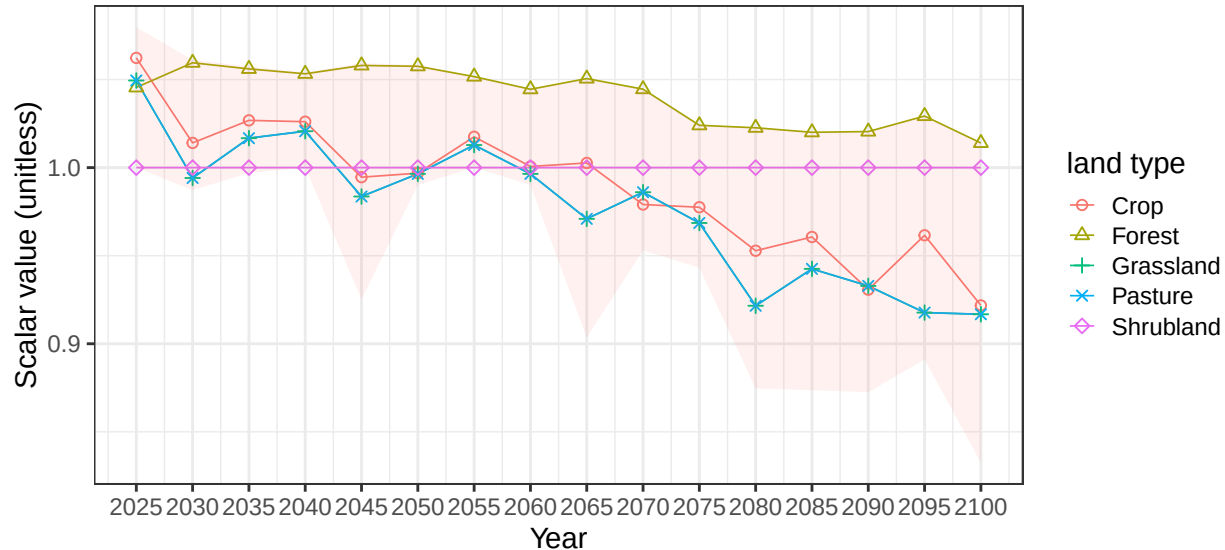
Region Africa_Western basin NileR average soil scalars
