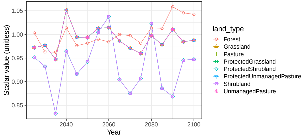
Region South Africa basin AfrCstS non-crop soil scalars
