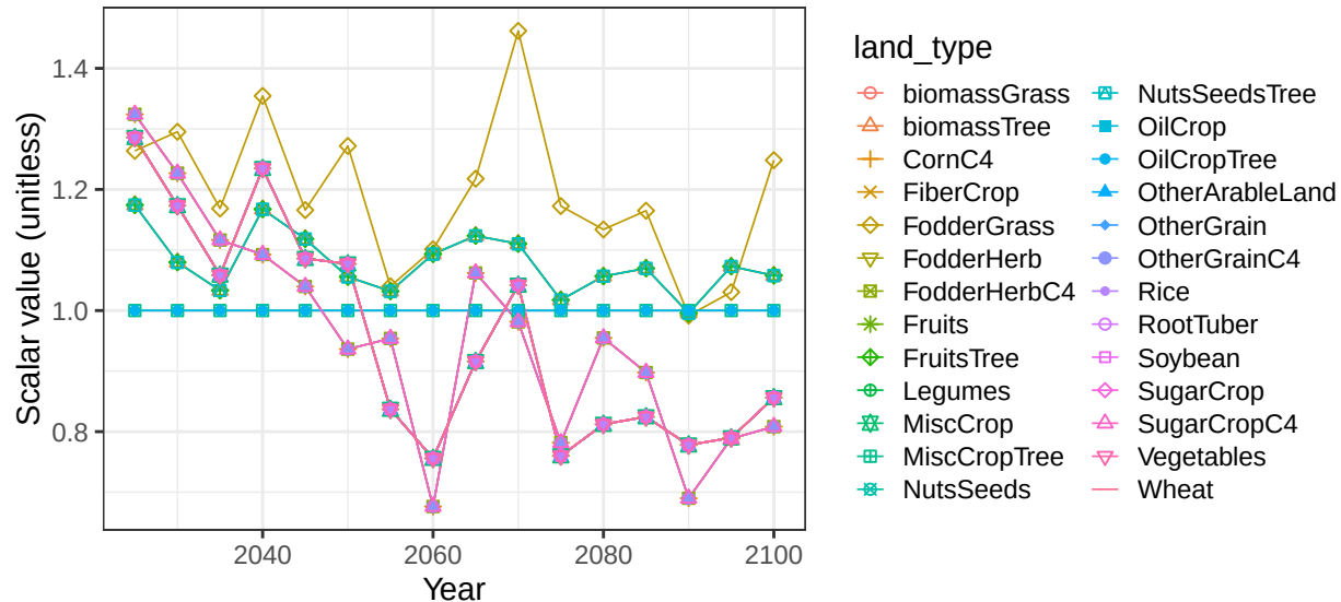
Region EU-15 basin IberiaCst crop vegetation scalars
