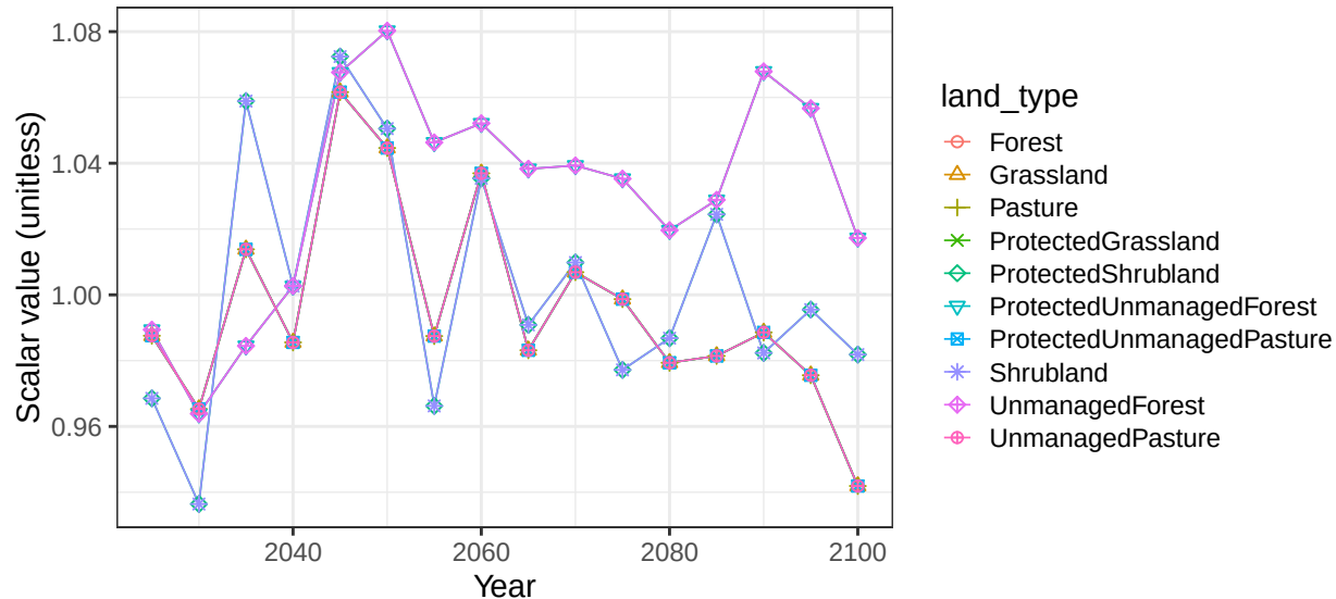
Region Russia basin ObR non-crop soil scalars
