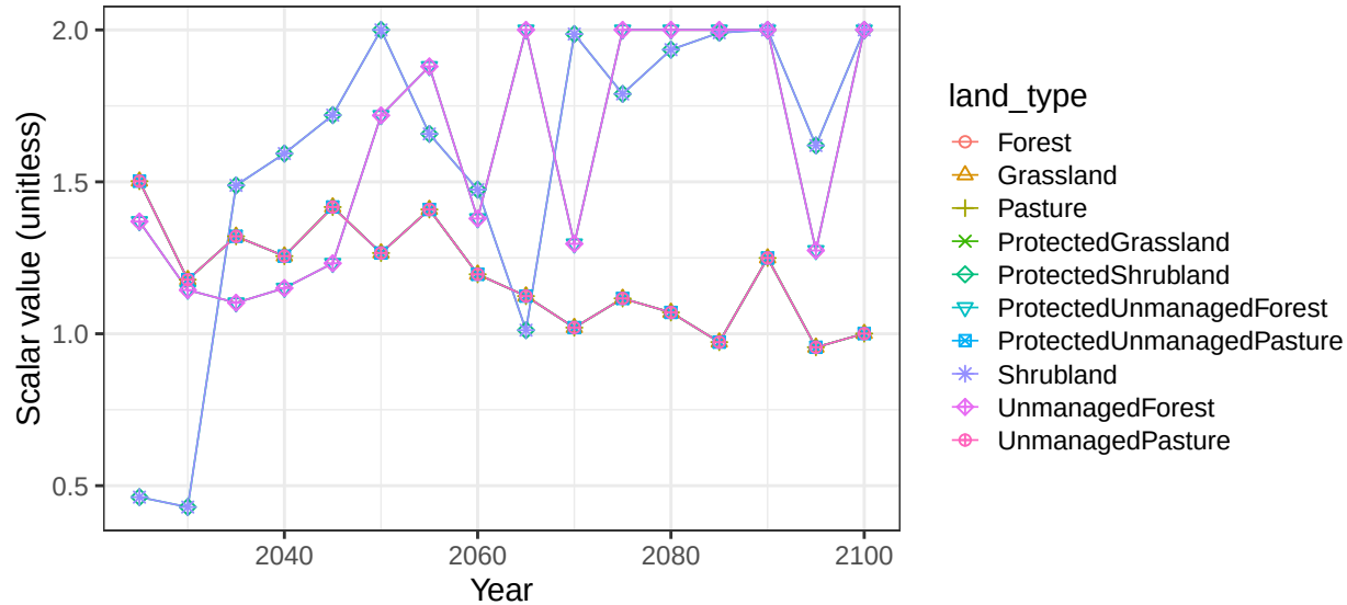
Region Mexico basin UsaColoRS non-crop vegetation scalars
