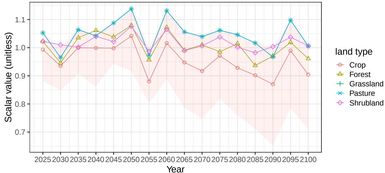
Region China basin Gobi average soil scalars
