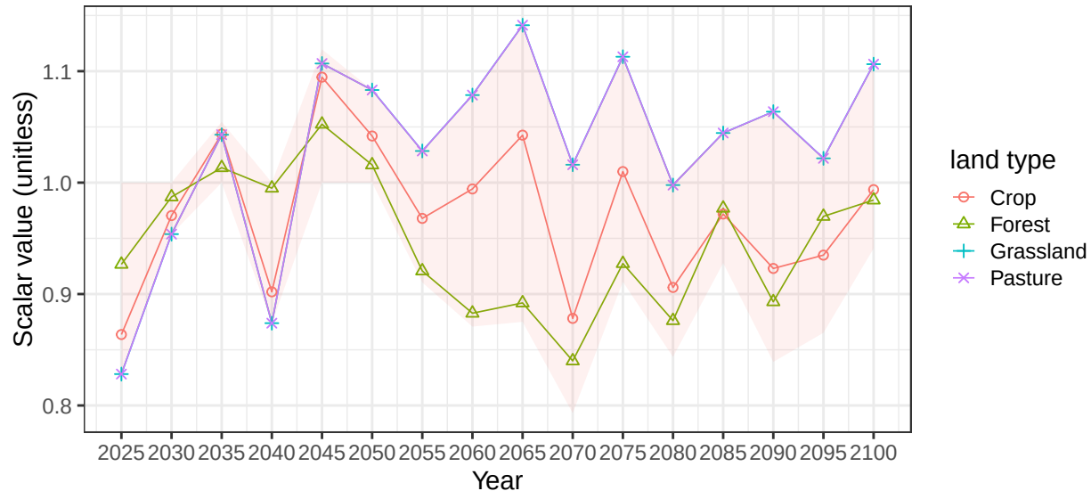
Region EU-15 basin DnkGrmCst average soil scalars
