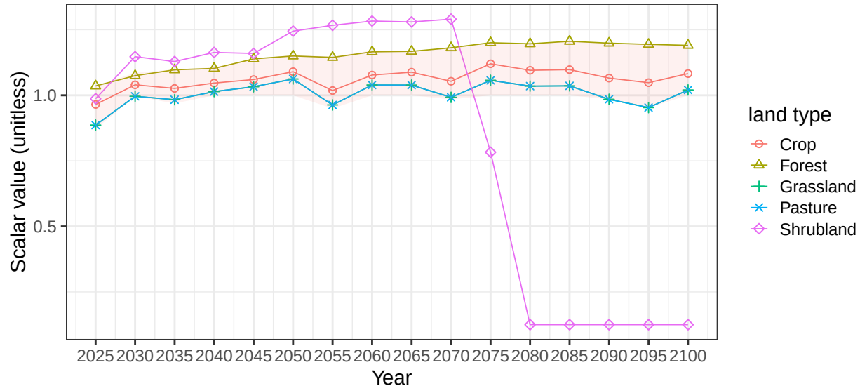
Region South America_Southern basin ColEcuacSt average vegetation sca
