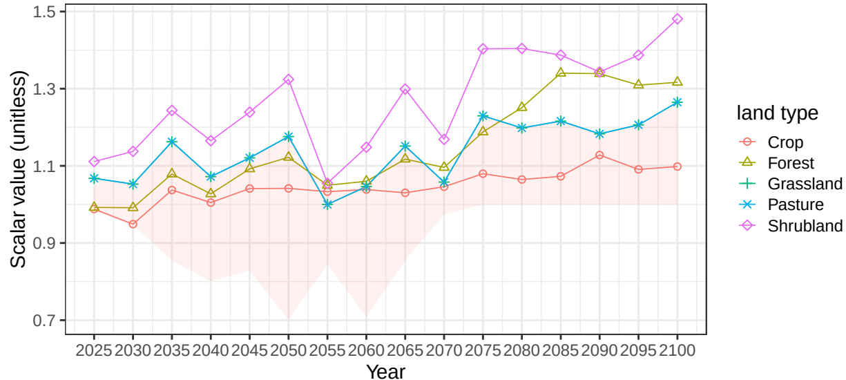
Region Russia basin SiberiaW average vegetation scalars
