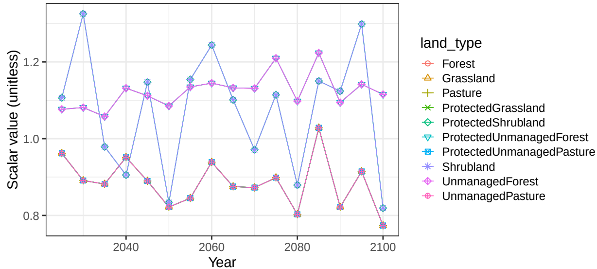
Region Australia_NZ basin AusCstN non-crop soil scalars
