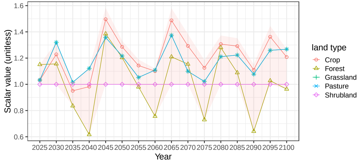
Region India basin IndCstNE average vegetation scalars
