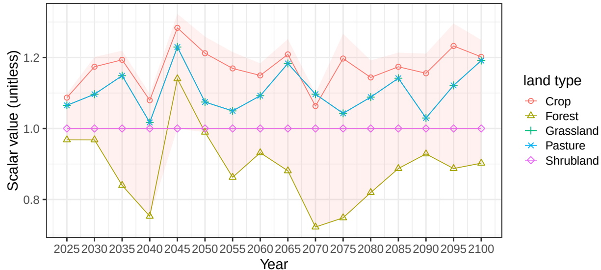
Region India basin BrahmaniR average soil scalars
