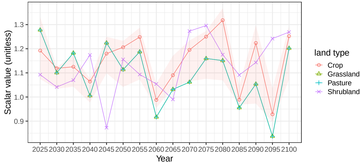
Region Central Asia basin UralR average soil scalars
