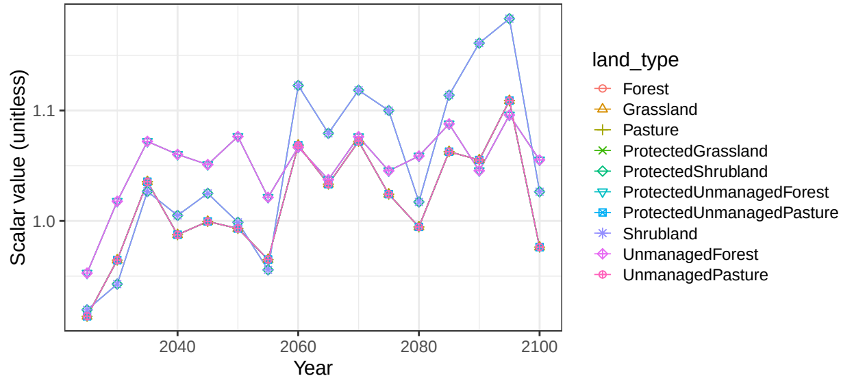
Region Canada basin CanAtl non-crop vegetation scalars
