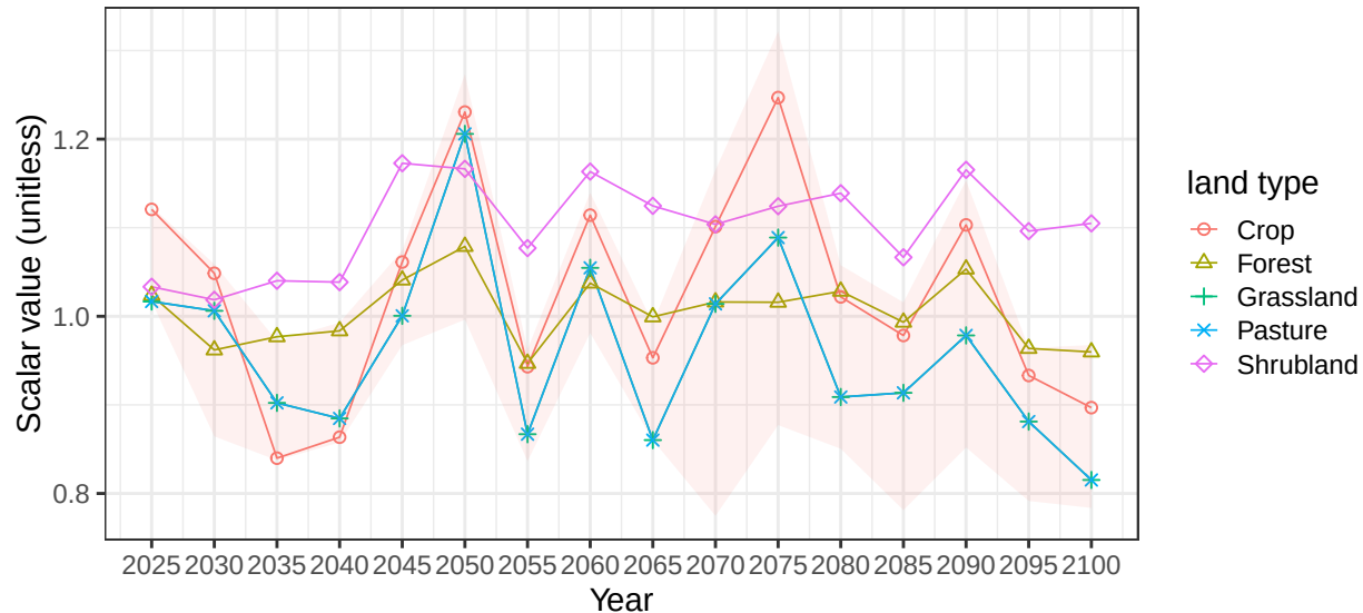
Region Central Asia basin ObR average soil scalars
