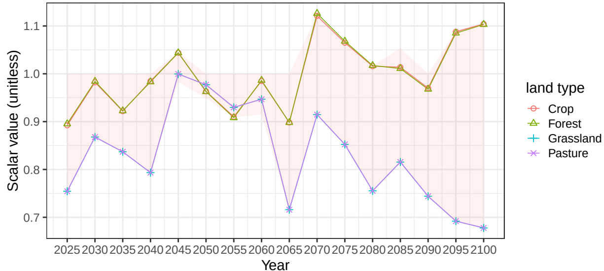
Region Europe_Eastern basin NevaR average soil scalars
