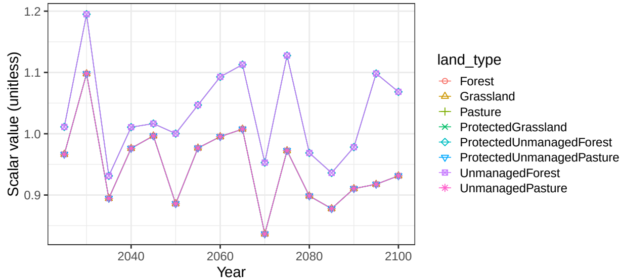
Region Central Asia basin BlackSeaS non-crop soil scalars
