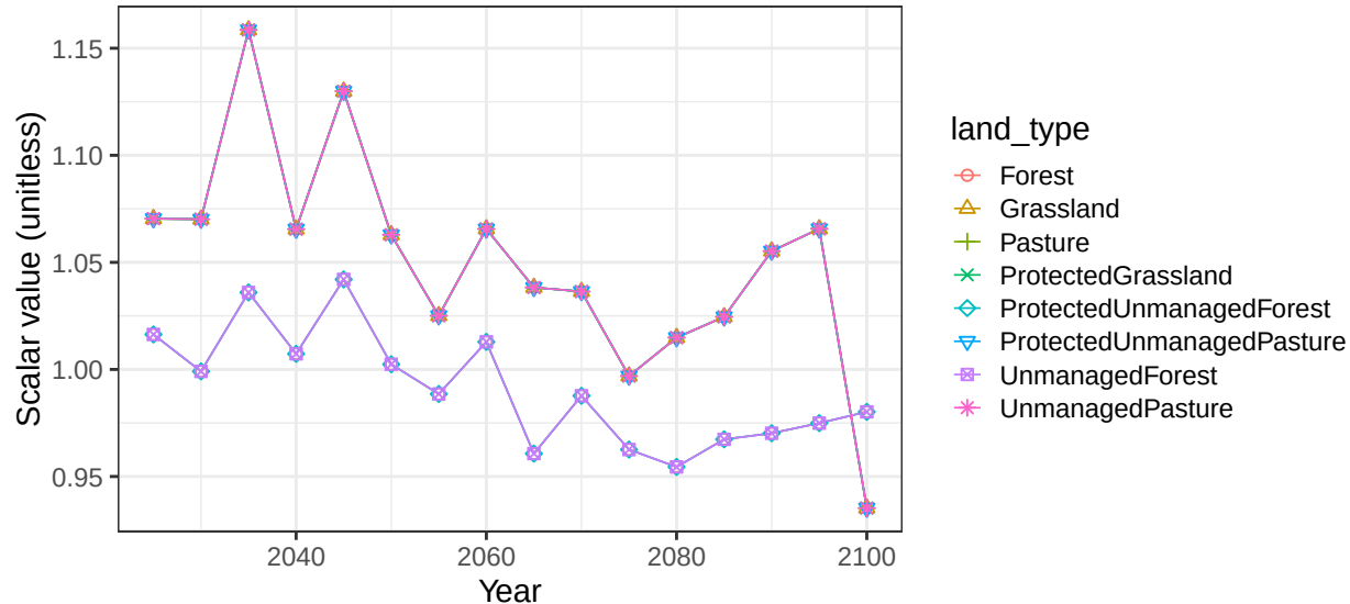
Region Southeast Asia basin BoHai non-crop soil scalars
