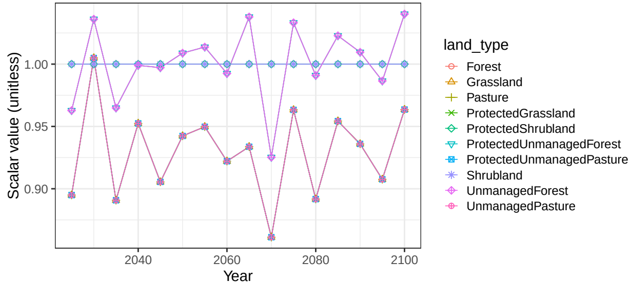
Region Mexico basin MexCstW non-crop soil scalars
