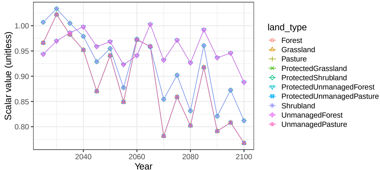
Region Argentina basin RioLaPlata non-crop soil scalars
