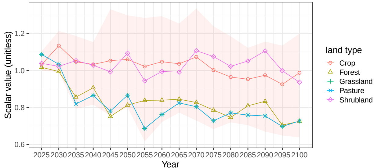
Region USA basin UsaColoRS average soil scalars
