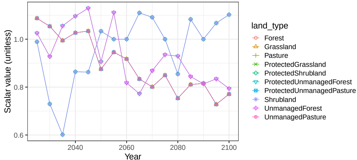
Region Mexico basin MexBaja non-crop soil scalars
