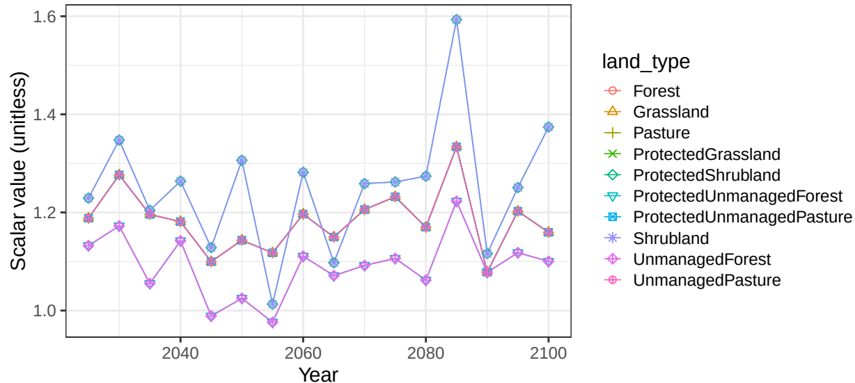
Region USA basin UsaColoRN non-crop vegetation scalars
