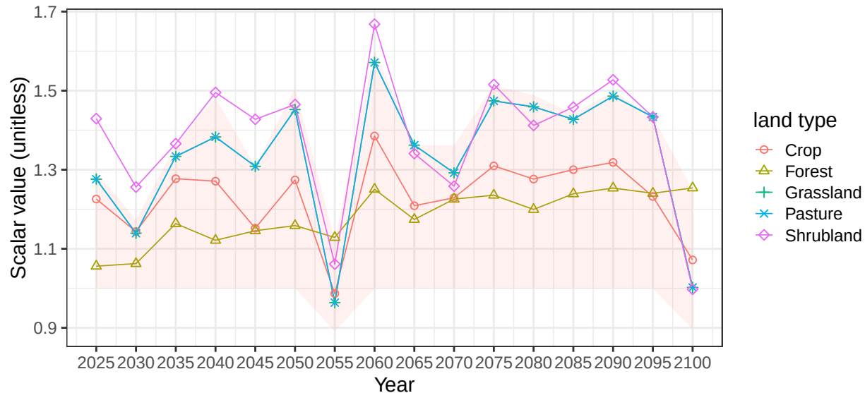
Region China basin BoHai average vegetation scalars
