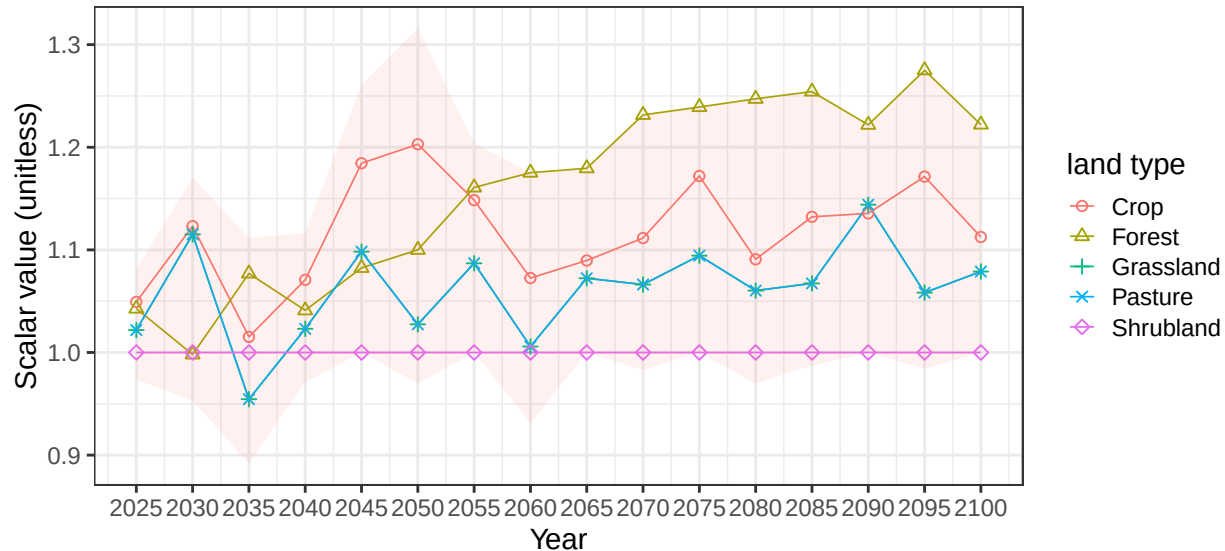
Region Southeast Asia basin XunJiang average vegetation scalars
