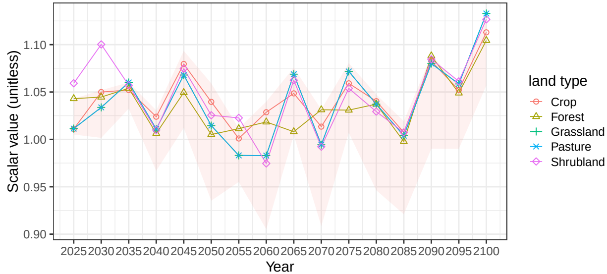
Region South Korea basin Korea average vegetation scalars
