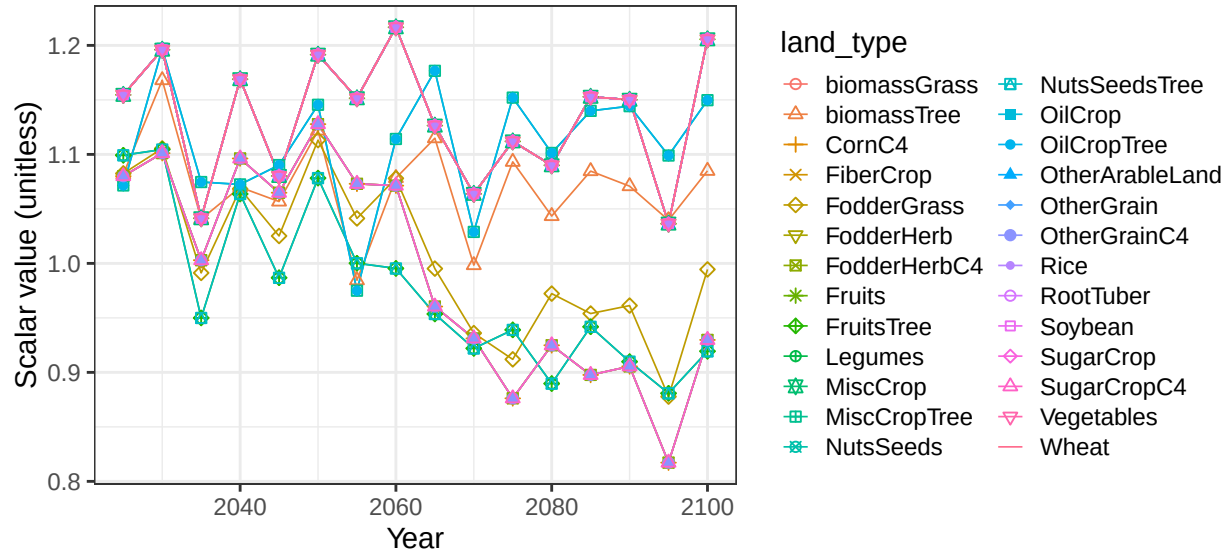
Region Mexico basin MexCstNW crop soil scalars
