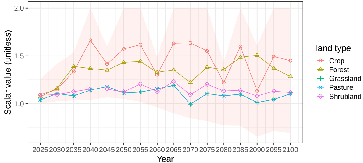
Region South America_Southern basin ChileCstN average vegetation scalar
