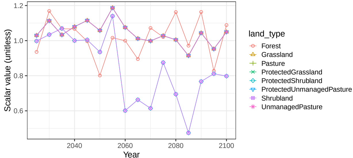
Region India basin SabarmatiR non-crop soil scalars
