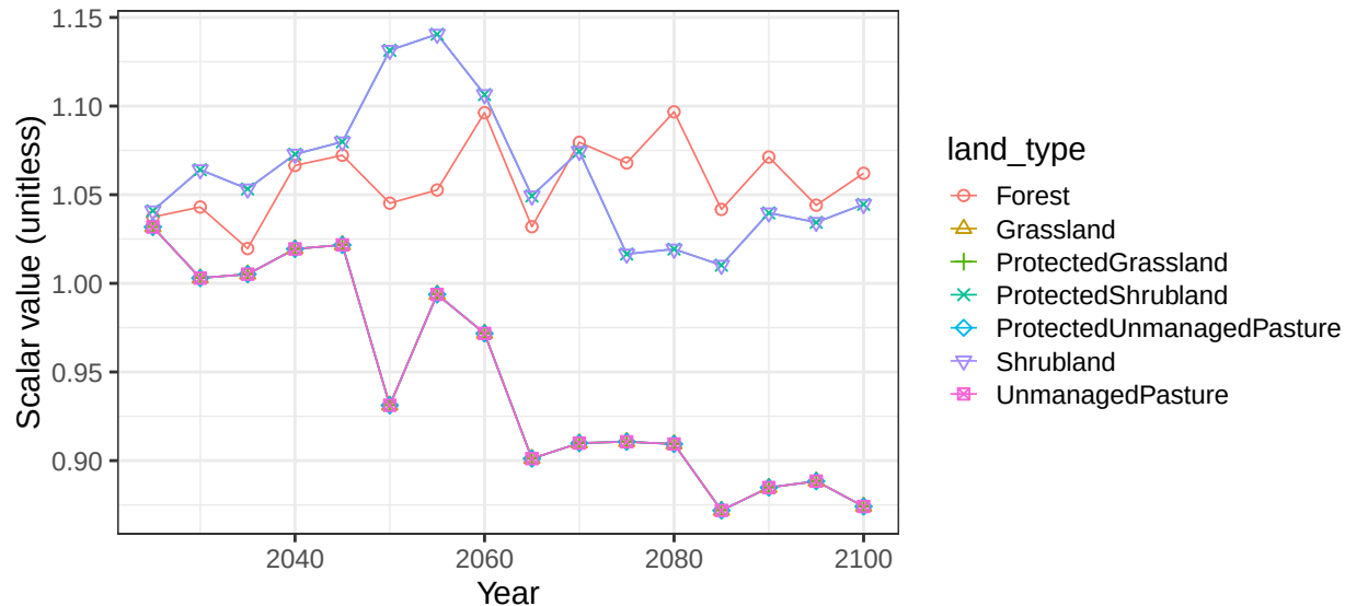
Region EU-15 basin DanubeR non-crop soil scalars
