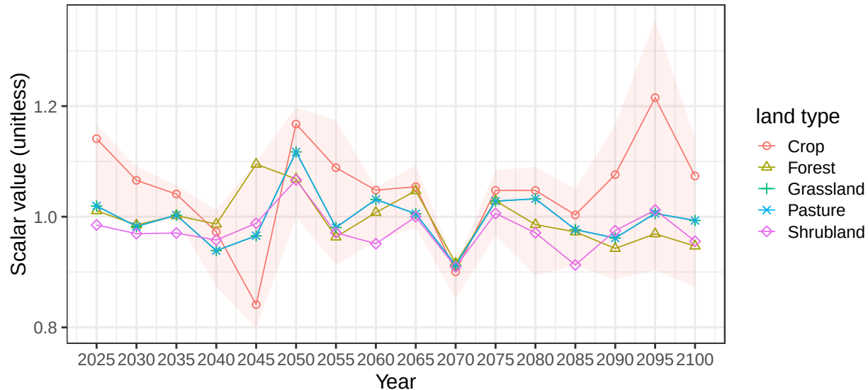
Region Central Asia basin LBalkash average soil scalars
