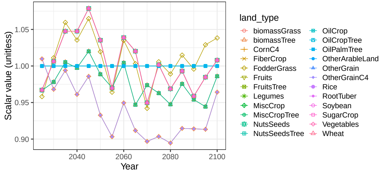
Region China basin RusCstSE crop soil scalars
