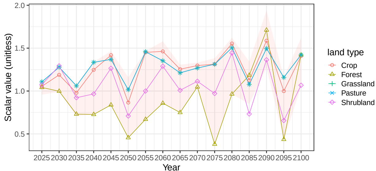
Region India basin MahiR average vegetation scalars
