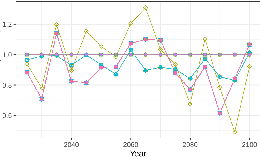
Region Russia basin BalticSea crop vegetation scalars
