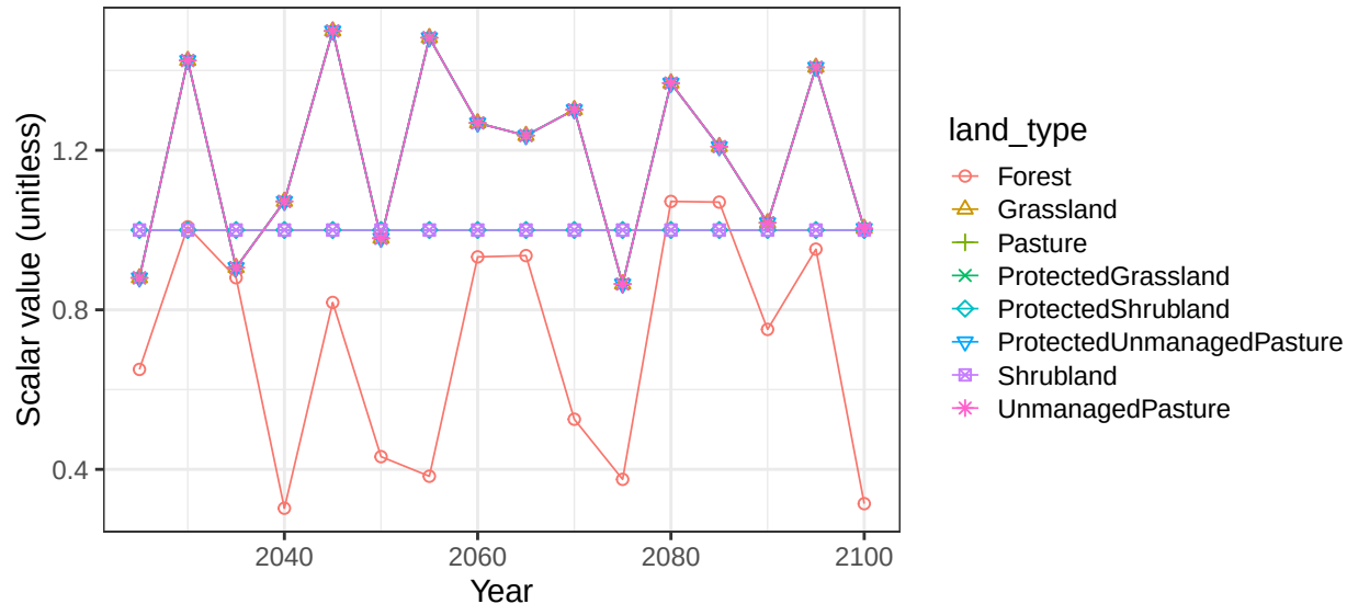
Region India basin PennarR non-crop vegetation scalars
