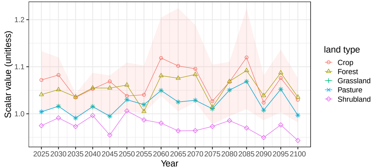
Region China basin Mekong average soil scalars
