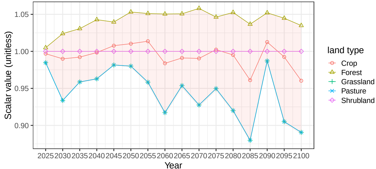
Region Africa_Western basin AfrCstW average soil scalars
