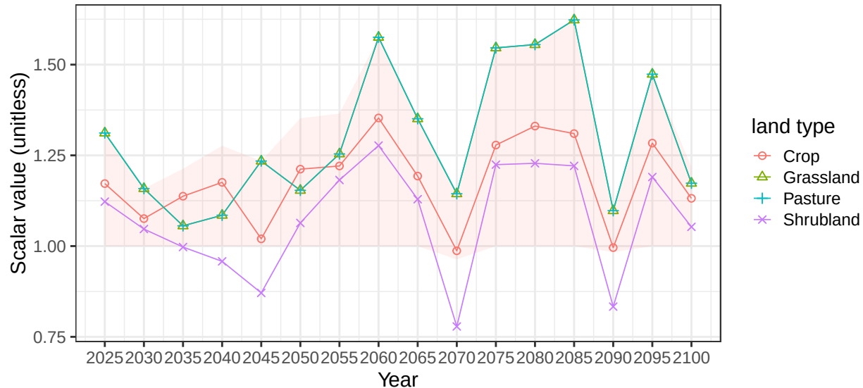
Region Middle East basin FarahrudR average vegetation scalars
