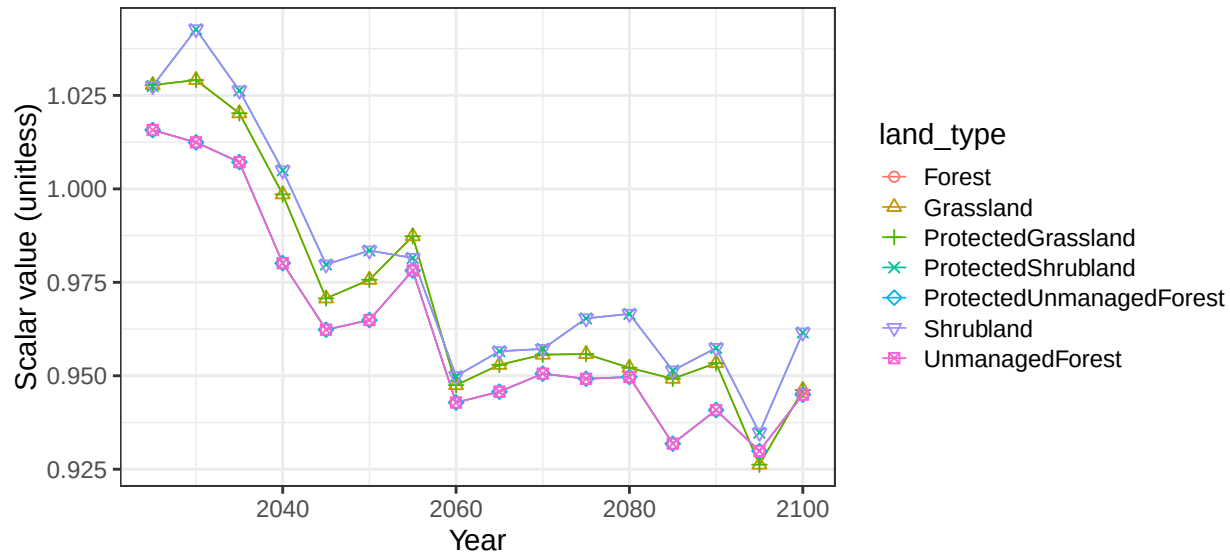
Region Japan basin Japan non-crop soil scalars
