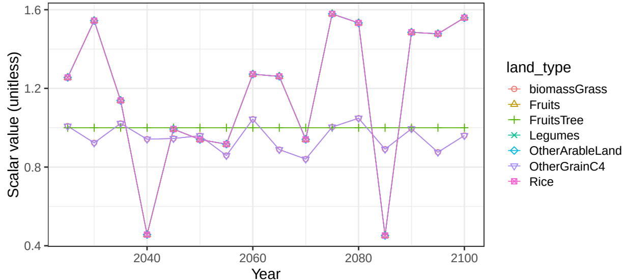
Region Africa_Western basin AfrCstNW crop soil scalars
