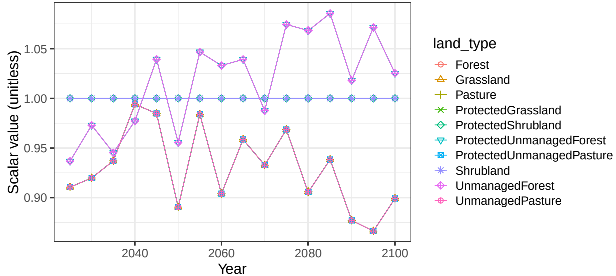
Region Mexico basin YucatanP non-crop soil scalars
