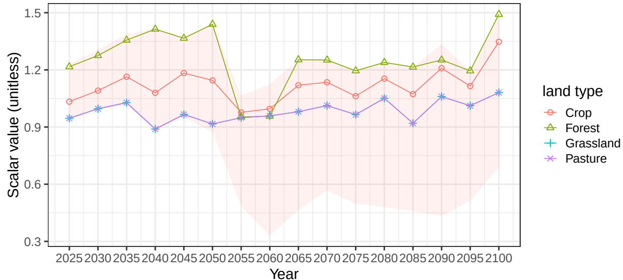
Region India basin BengalBay average vegetation scalars
