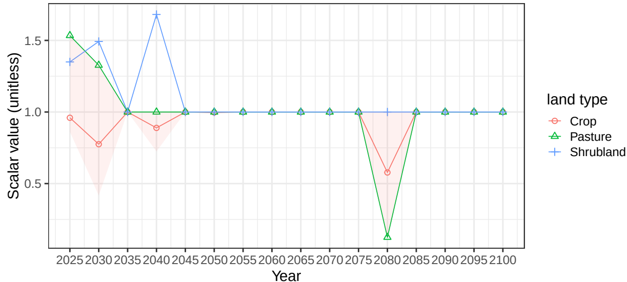
Region Middle East basin SinaiP average vegetation scalars
