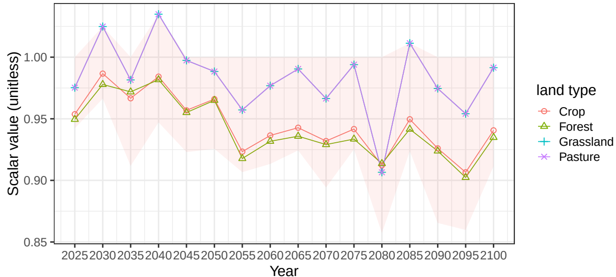
Region USA basin UsaCstNE average soil scalars
