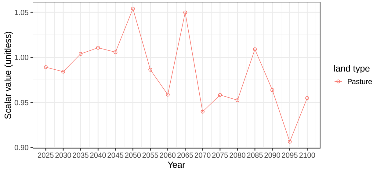
Region China basin SyrDaryaR average soil scalars
