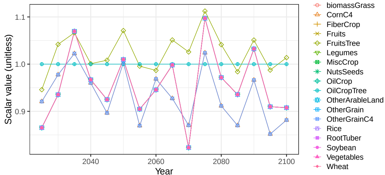
Region South America_Southern basin BrzCstS crop soil land type
