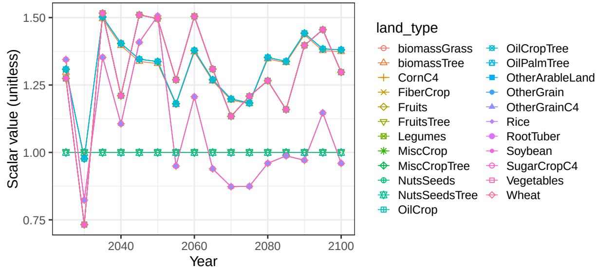
Region Africa_Southern basin NileR crop vegetation scalars
