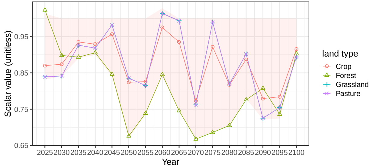
Region EU-15 basin ElbeR average vegetation scalars
