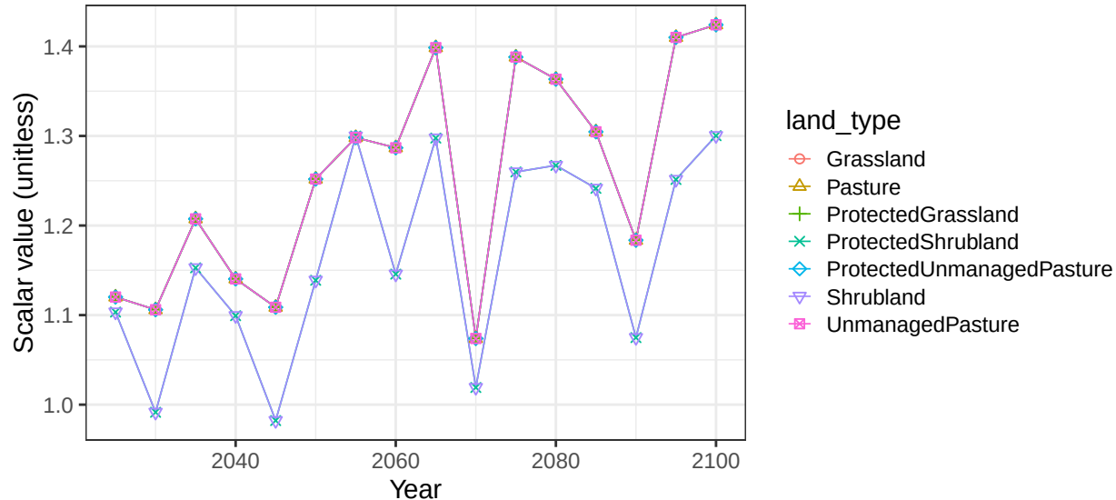
Region South Asia basin Helmand non-crop vegetation scalars
