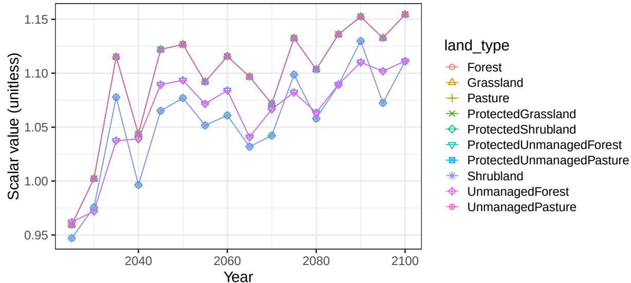
Region Russia basin RusCstSE non-crop vegetation scalars
