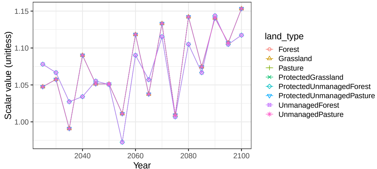
Region European Free Trade Association basin PoR non-crop vegetation s
