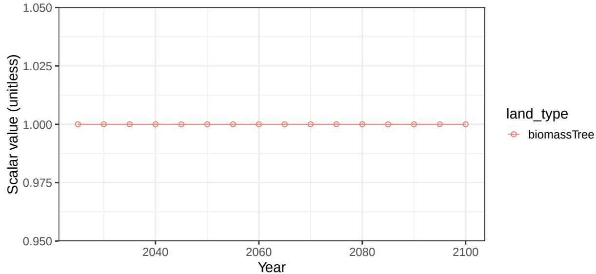
Region Russia basin KaraSea crop vegetation scalars
