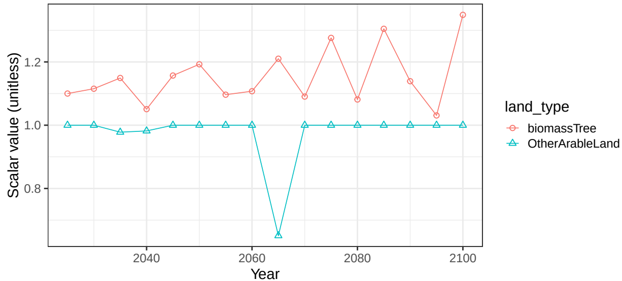
Region USA basin PacArctic crop vegetation scalars
