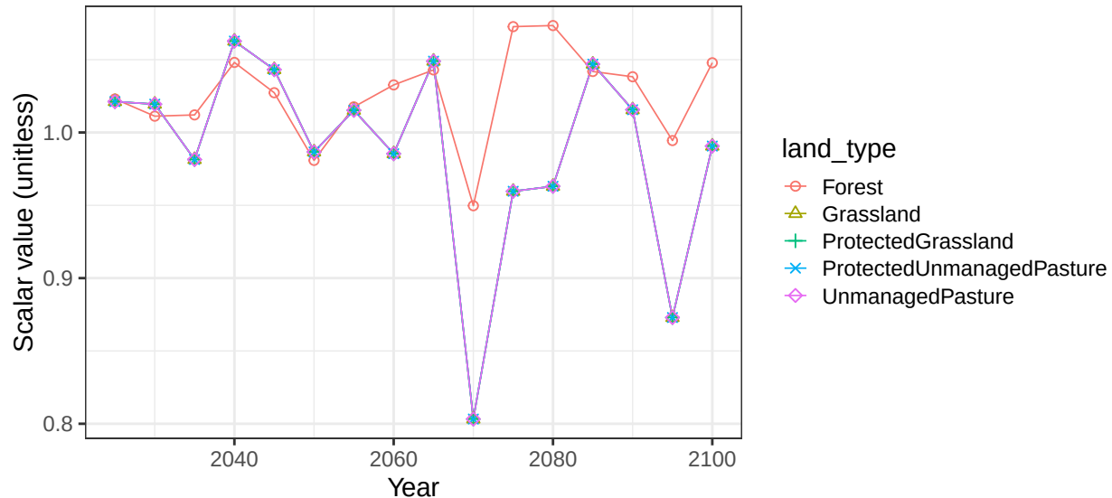
Region EU-15 basin LoireR non-crop soil scalars
