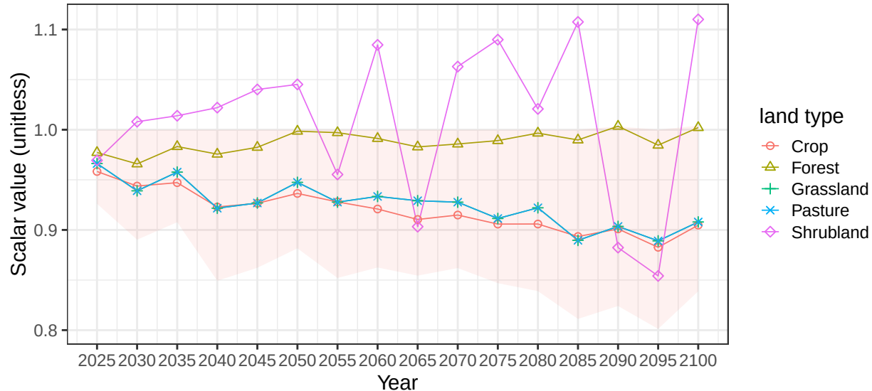
Region South America_Southern basin PeruCst average soil scalars
