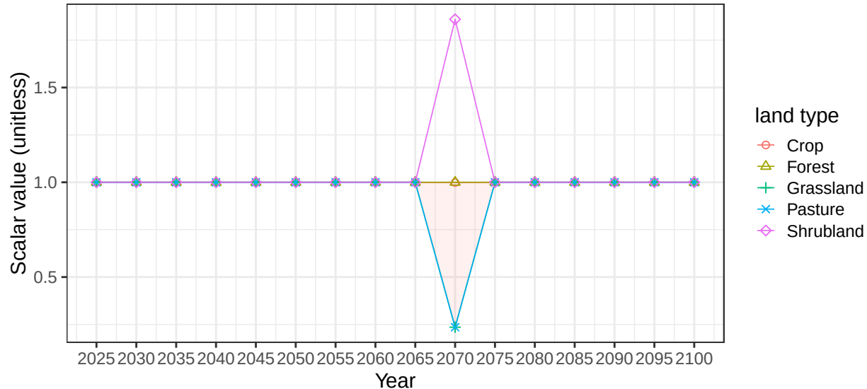
Region Mexico basin California average vegetation scalars
