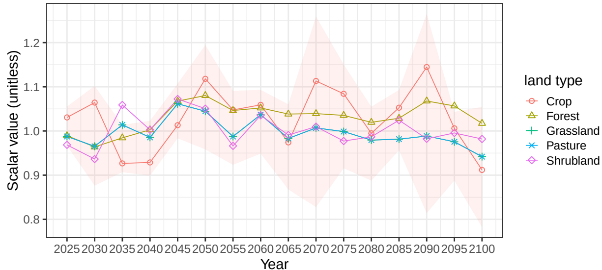
Region Russia basin ObR average soil scalars
