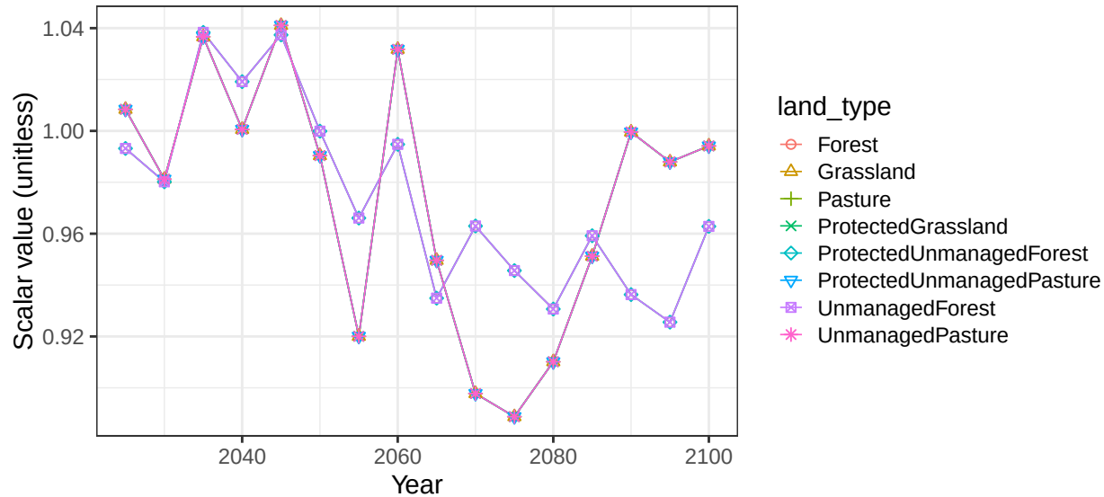
Region Southeast Asia basin RusCstSE non-crop soil scalars
