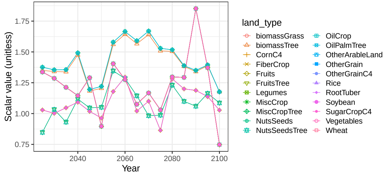
Region Africa_Southern basin AfrIntS crop vegetation scalars
