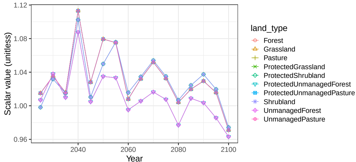
Region Canada basin NWTerr non-crop soil scalars
