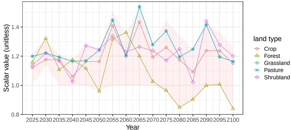
Region Africa_Northern basin AfrIntN average vegetation scalars
