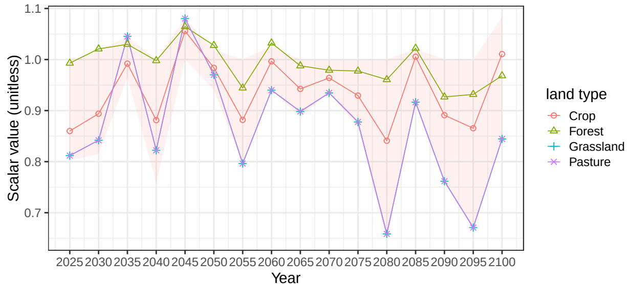
Region EU-12 basin BalticSea average soil scalars
