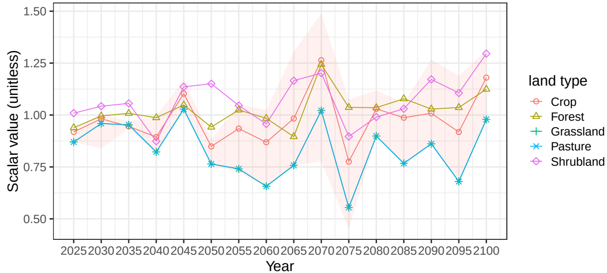
Region Russia basin VolgaR average vegetation scalars
