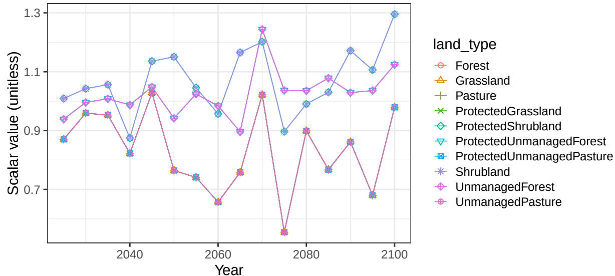
Region Russia basin VolgaR non-crop vegetation scalars
