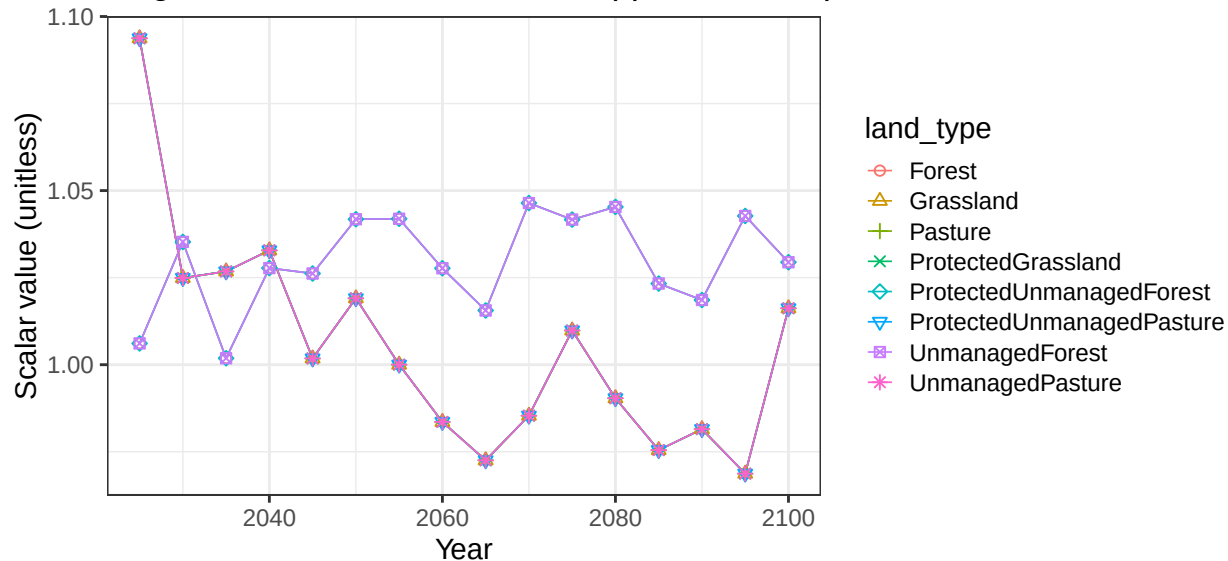
Region Southeast Asia basin Phlppns non-crop soil scalars
