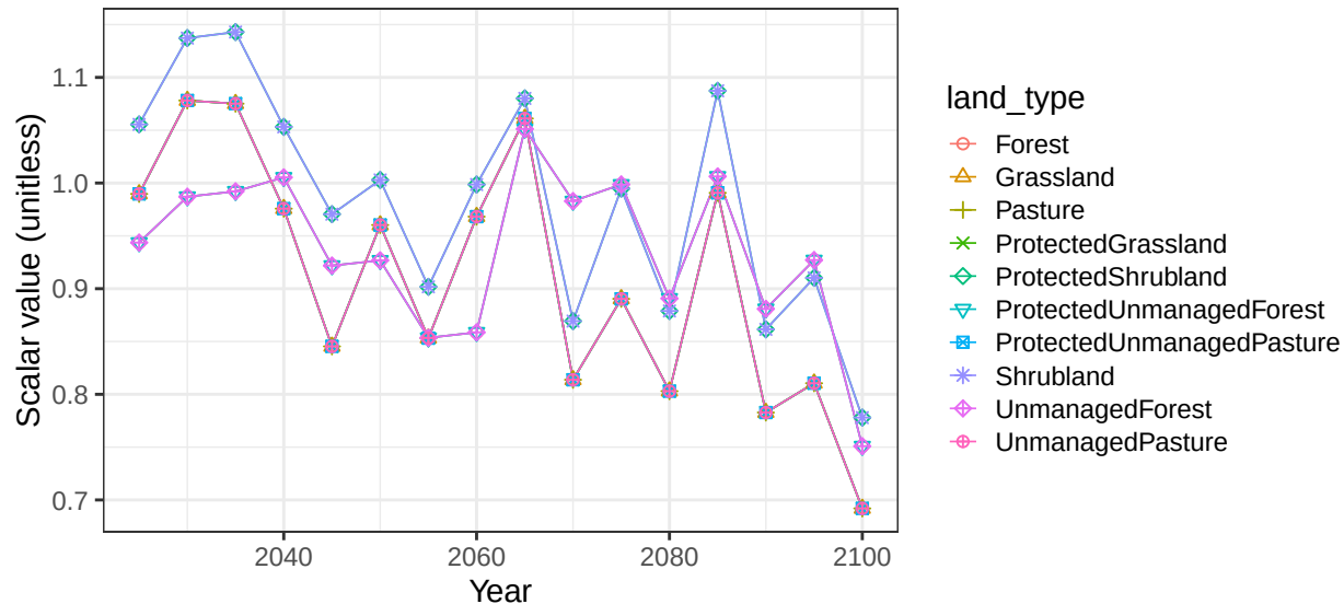
Region Argentina basin RioLaPlata non-crop vegetation scalars
