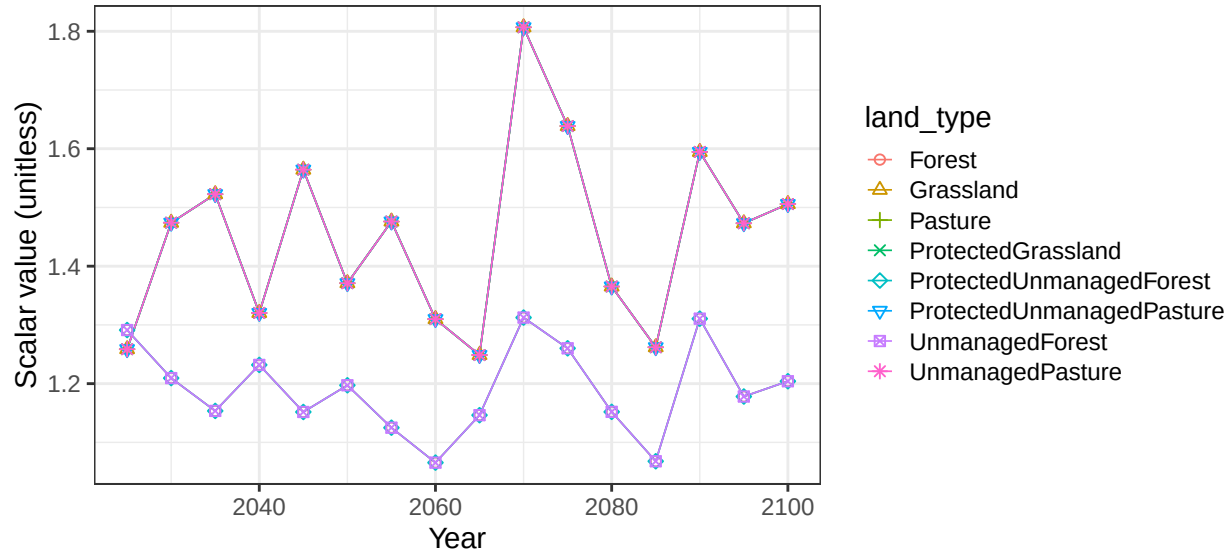
Region USA basin NelsonR non-crop vegetation scalars
