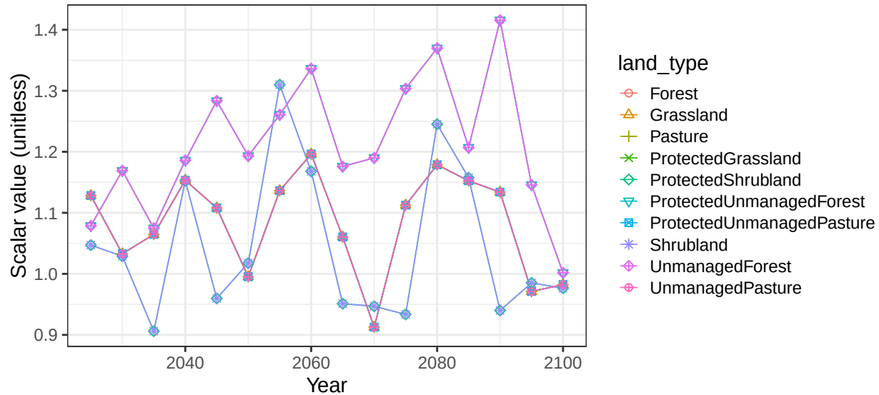
Region Africa_Southern basin LimpopoR non-crop soil scalars
