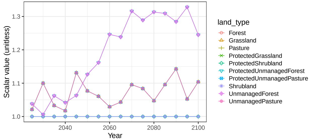
Region Southeast Asia basin Hong non-crop vegetation scalars
