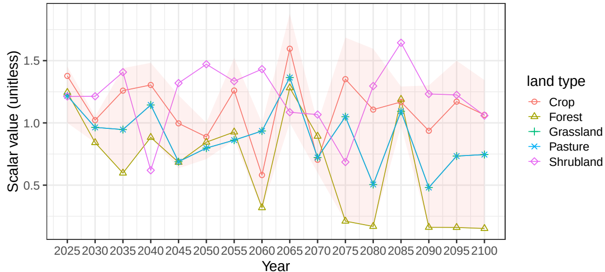
Region Argentina basin Pampas average vegetation scalars
