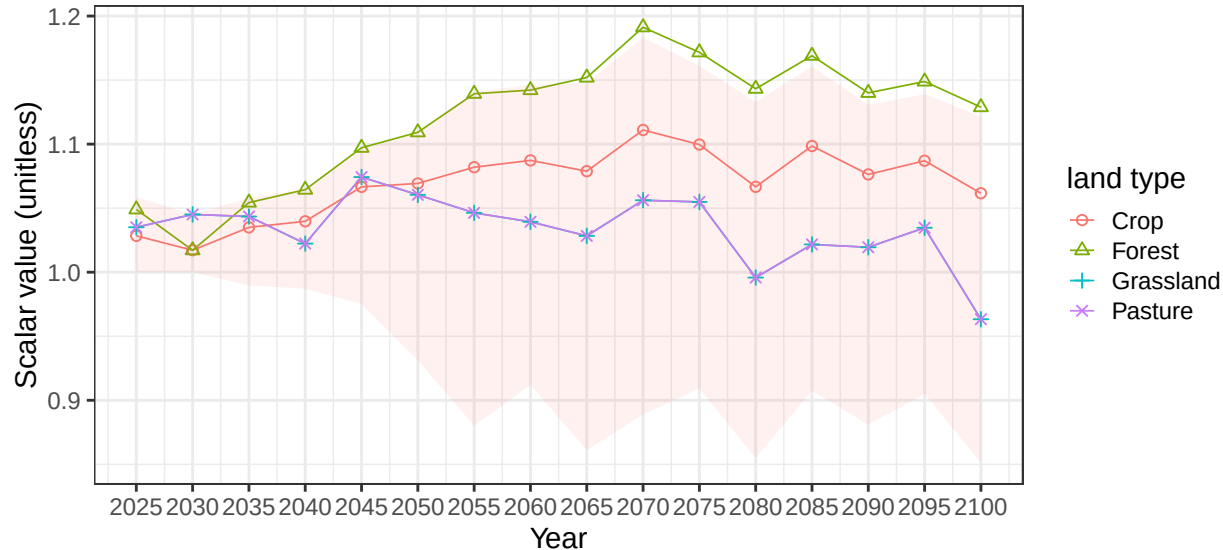
Region South America_Southern basin NegroR average soil scalars
