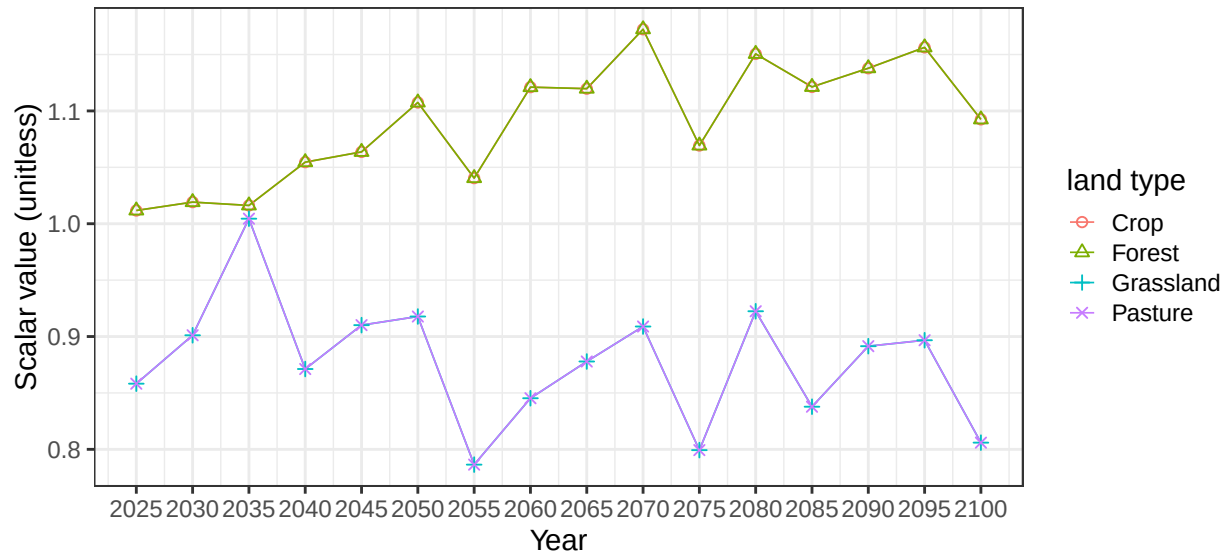
Region South America_Northern basin MagdalenaR average vegetation sca
