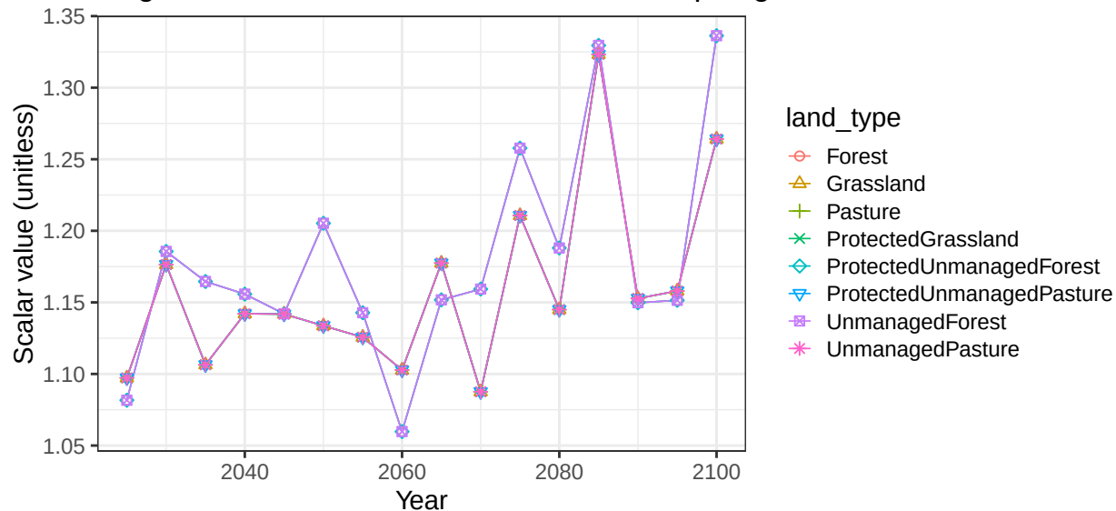
Region Canada basin UsaPacNW non-crop vegetation scalars
