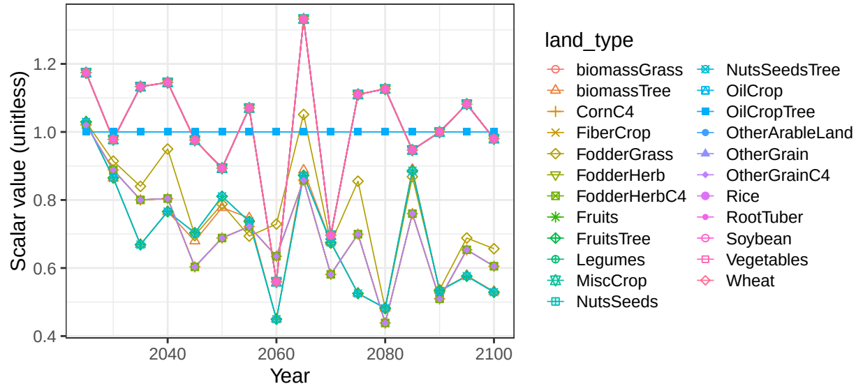
Region Argentina basin Pampas crop soil scalars
