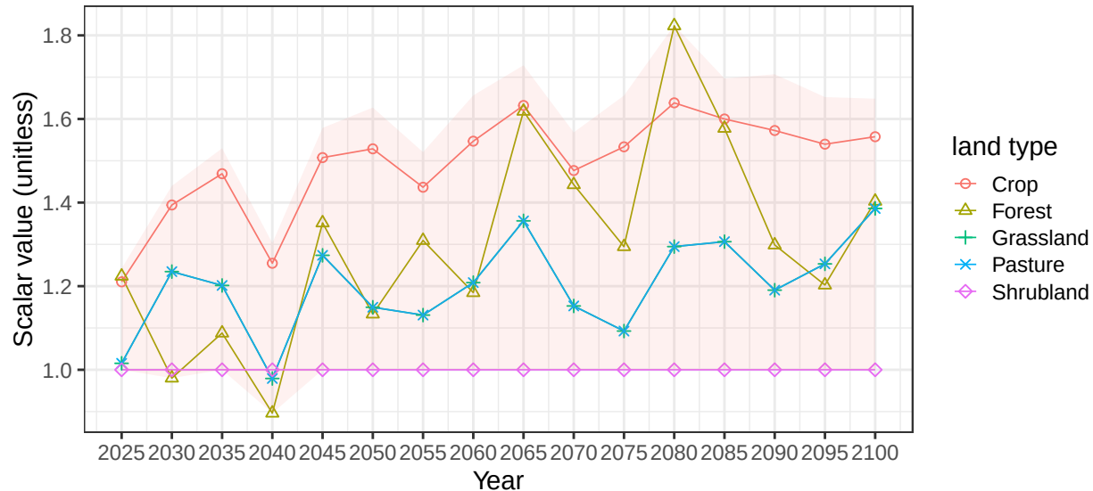
Region India basin MahanadiR average vegetation scalars
