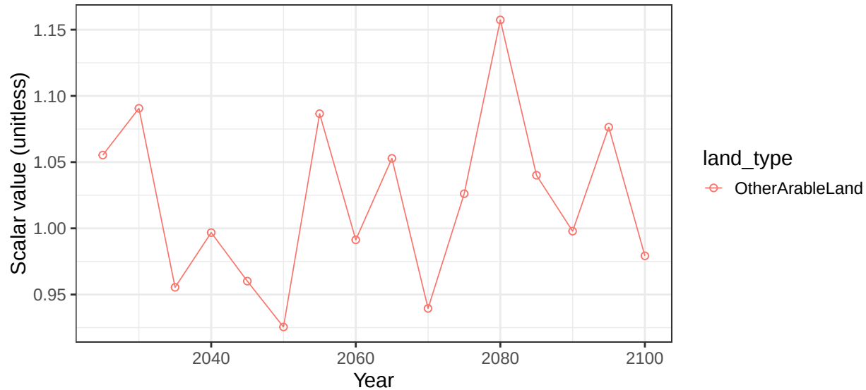
Region EU-15 basin MeditE crop soil scalars
