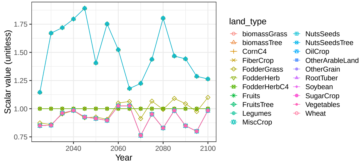
Region EU-15 basin EmsWeserR crop vegetation scalars
