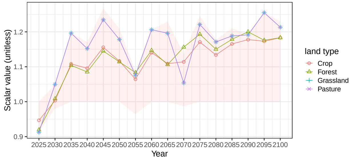
Region China basin RusCstSE average vegetation scalars
