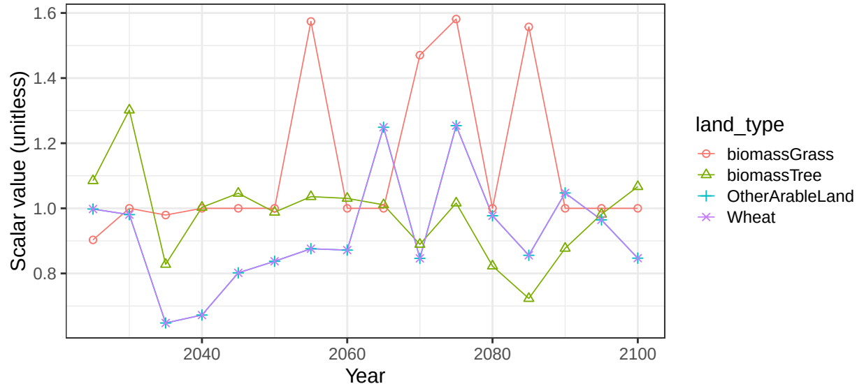
Region Central Asia basin BlackSeaN crop soil scalars
