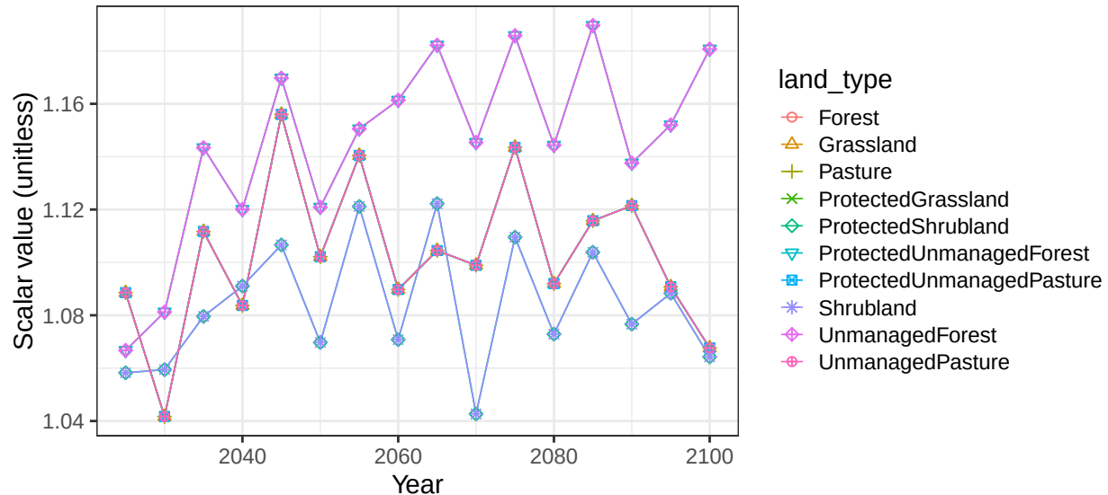
Region South America_Southern basin ChileCstS non-crop vegetation sca
