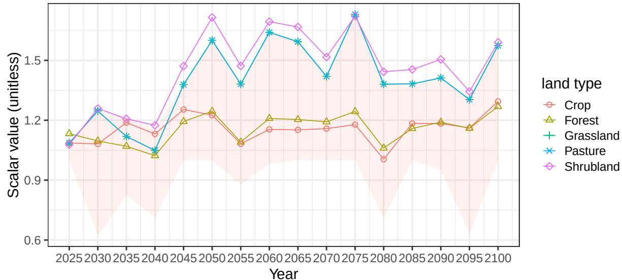
Region EU-15 basin Sweden average vegetation scalars
