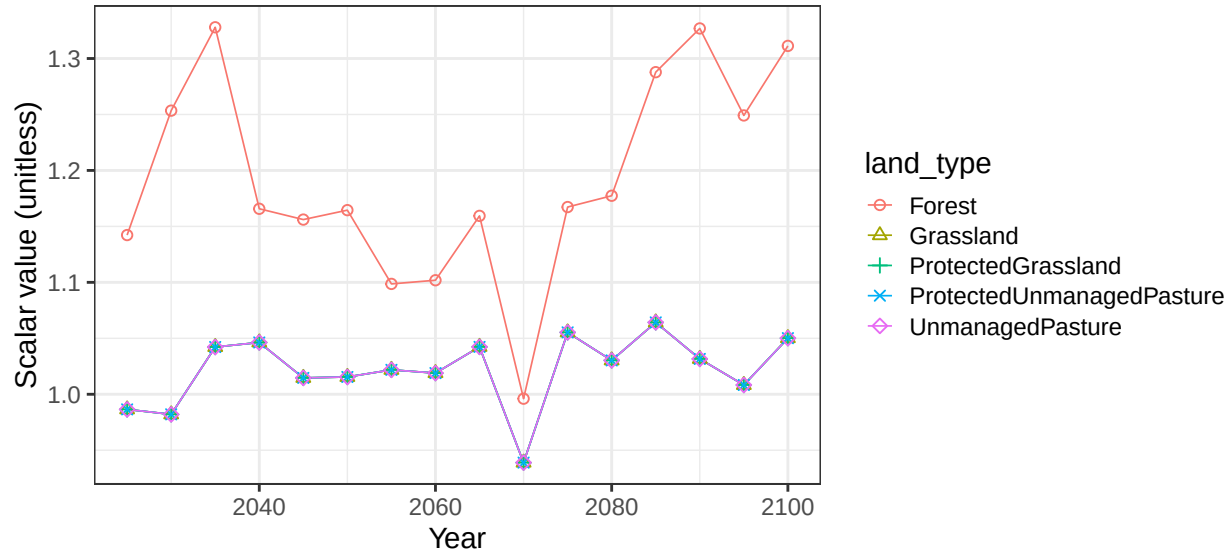
Region EU-15 basin RhineR non-crop soil scalars
