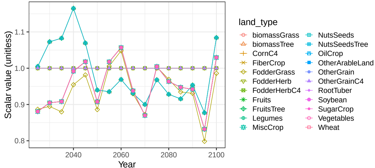
Region EU-12 basin OderR crop soil scalars
