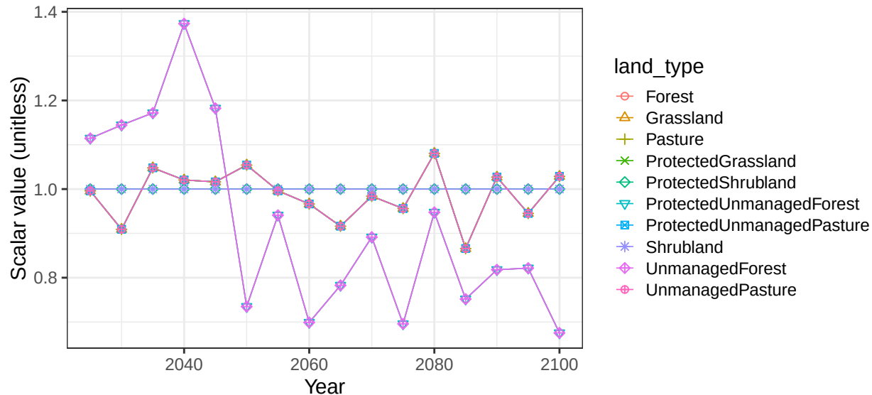
Region Africa_Western basin LChad non-crop vegetation scalars
