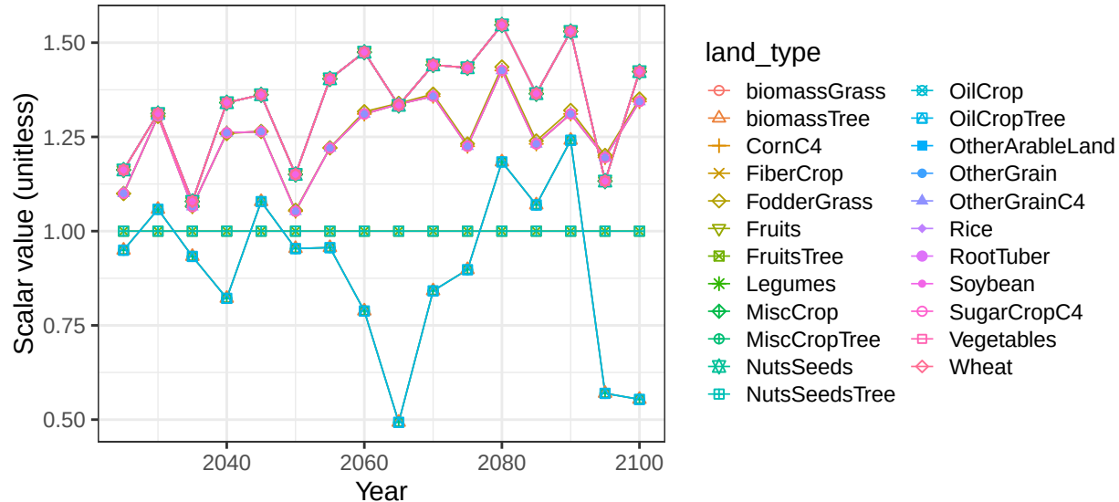
Region India basin NarmadaR crop vegetation scalars
