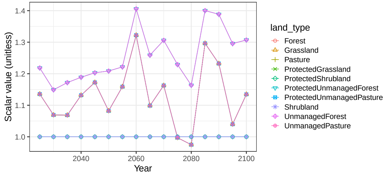
Region Africa_Southern basin ZambeziR non-crop vegetation scalars
