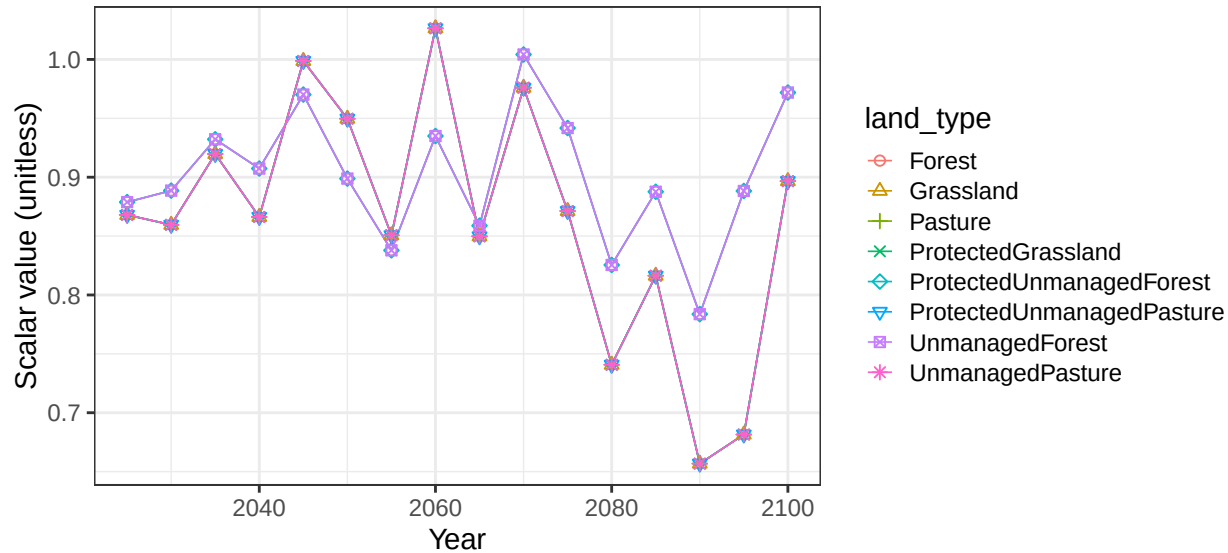
Region Russia basin NevaR non-crop vegetation scalars
