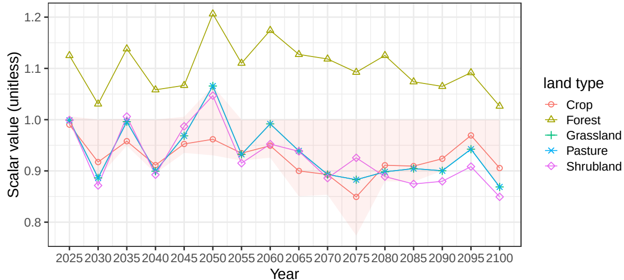
Region Central Asia basin YeniseiR average soil scalars
