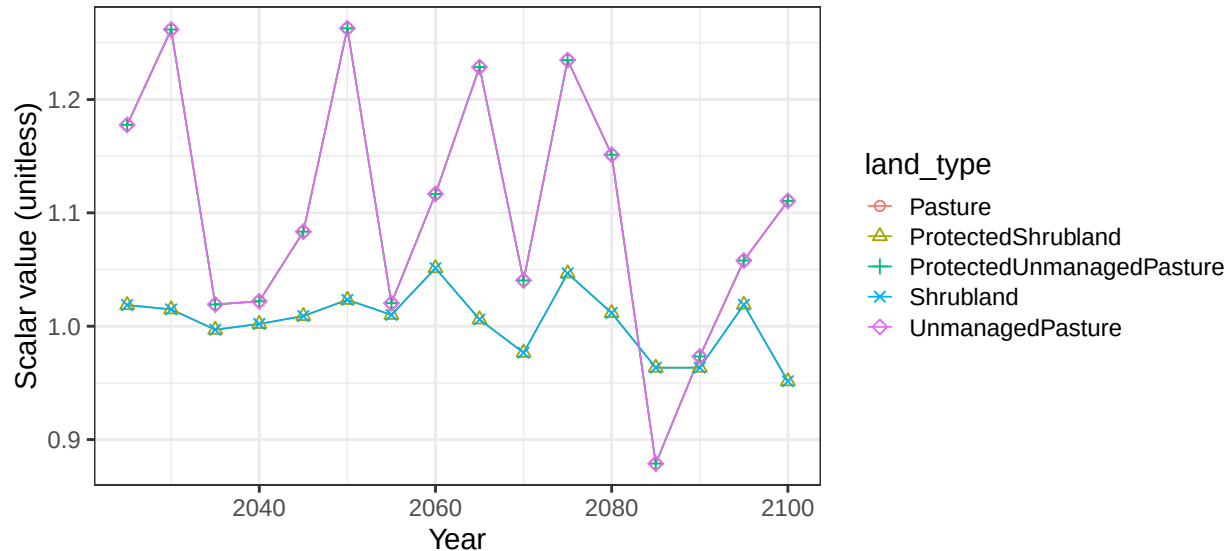
Region Europe_Non_EU basin EJrdnSyr non-crop soil scalars
