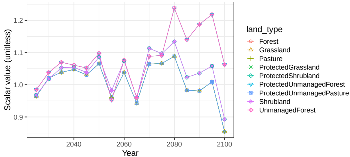
Region Russia basin SiberiaN non-crop soil scalars
