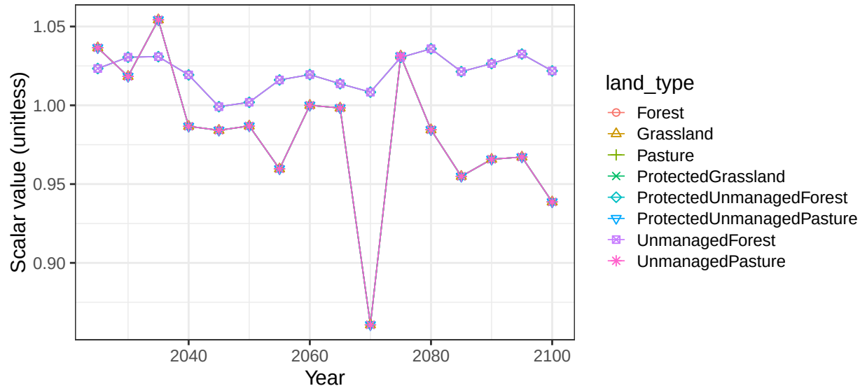
Region Southeast Asia basin IrianJaya non-crop soil scalars
