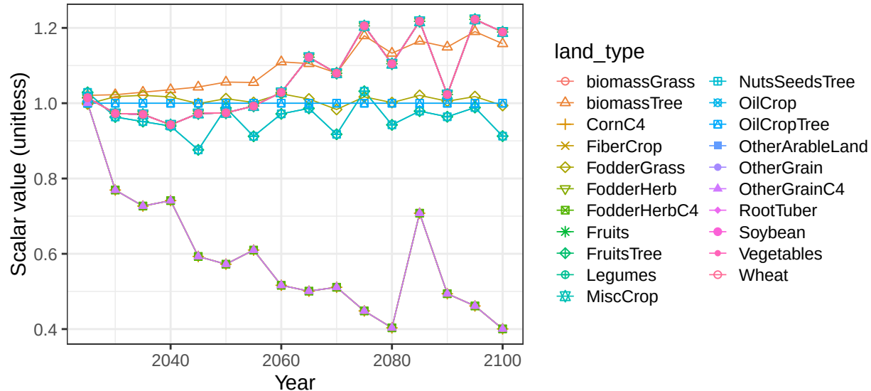
Region Argentina basin ArgCstS crop soil scalars
