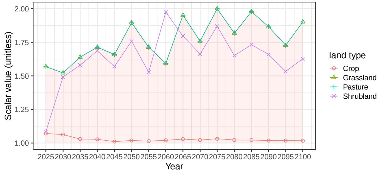
Region Middle East basin ArabianSea average vegetation scalars
