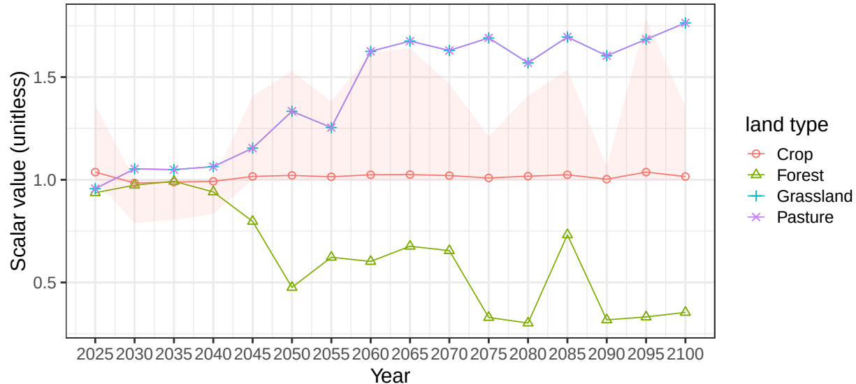
Region EU-15 basin NevaR average vegetation scalars
