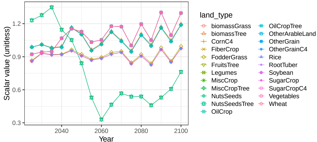
Region Southeast Asia basin BengalBay crop vegetation scalars
