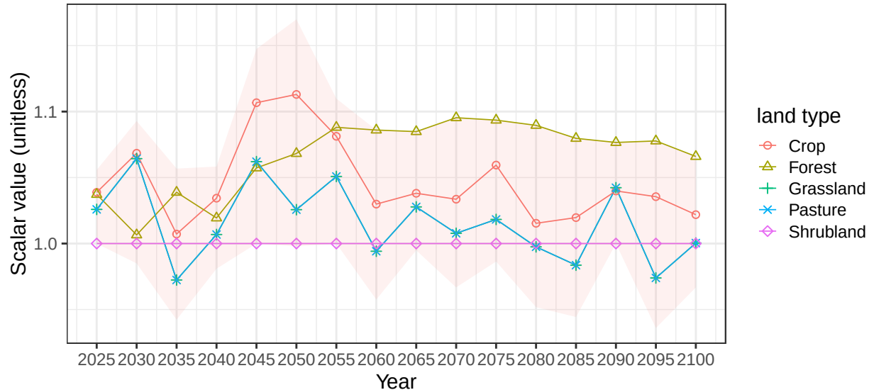
Region Southeast Asia basin XunJiang average soil scalars
