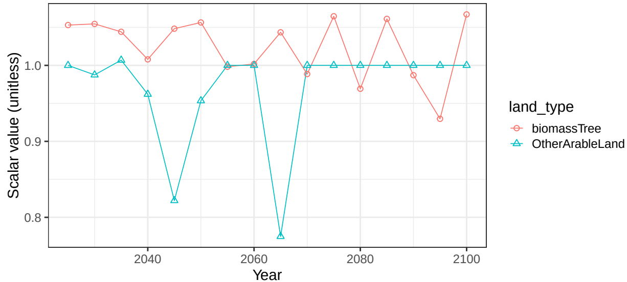
Region USA basin PacArctic crop soil scalars
