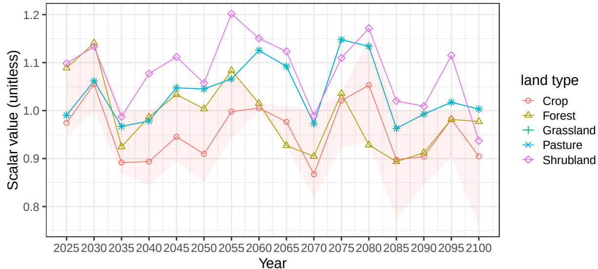
Region Europe_Non_EU basin BlackSeaS average soil scalars
