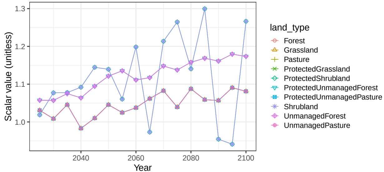
Region South America_Southern basin PeruCst non-crop vegetation scalar
