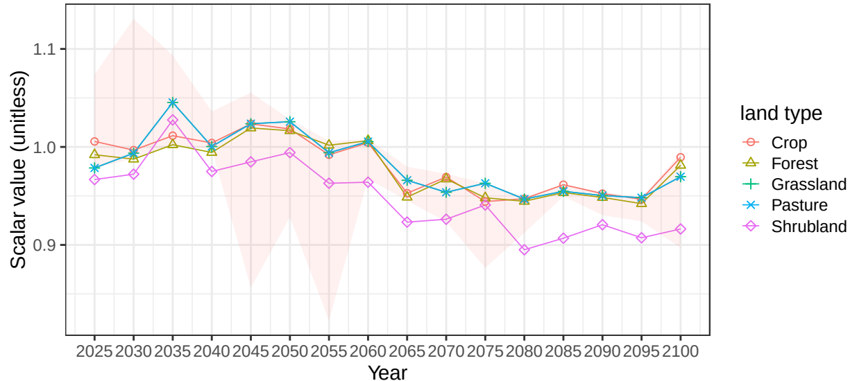
Region Russia basin RusCstSE average soil scalars
