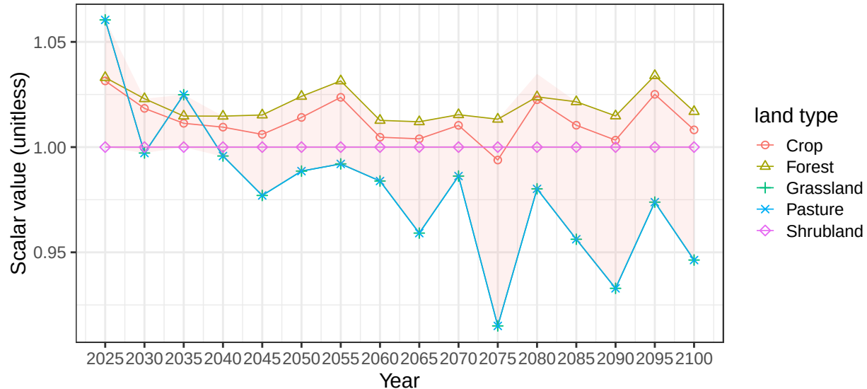
Region Southeast Asia basin MalaysiaP average soil scalars
