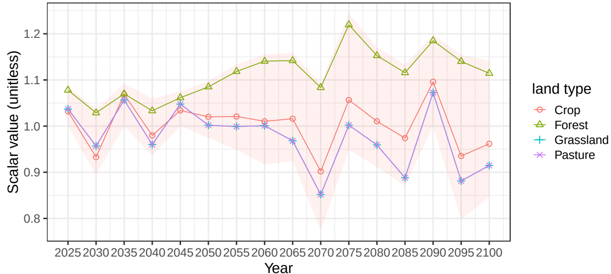
Region EU-15 basin EngWales average vegetation scalars
