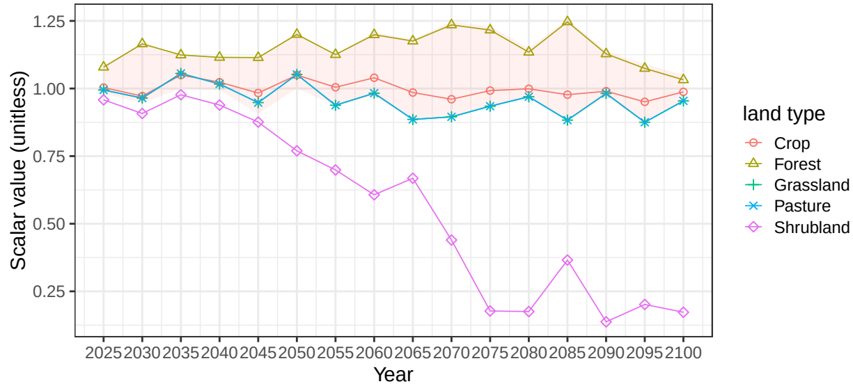
Region Africa_Eastern basin NileR average soil scalars
