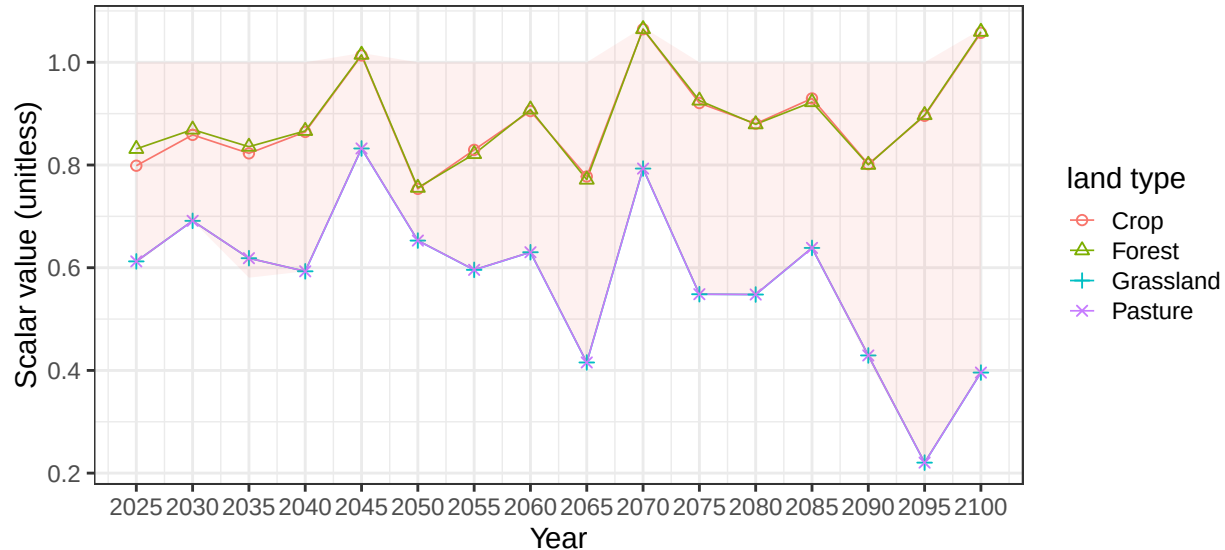
Region Russia basin DaugavaR average vegetation scalars
