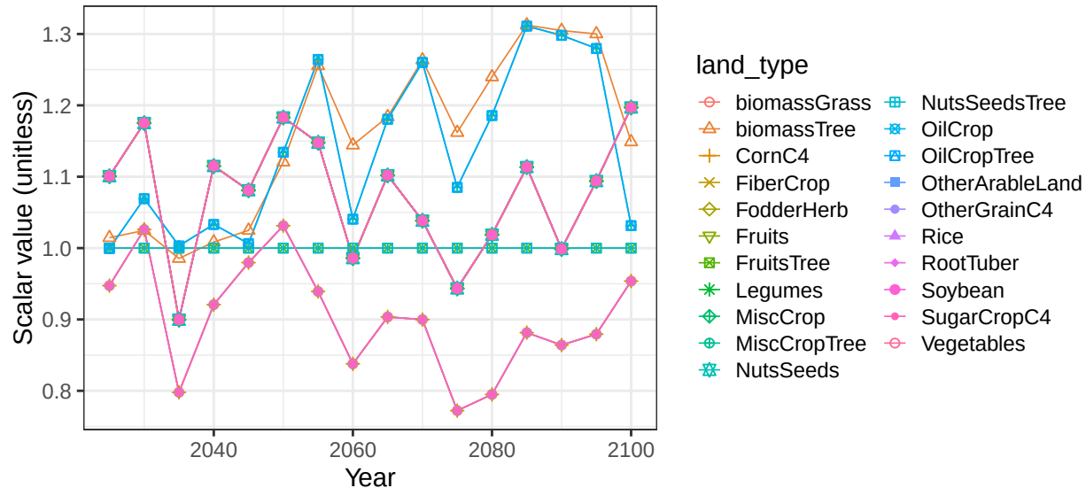
Region Southeast Asia basin SChinaSea crop vegetation scalars
