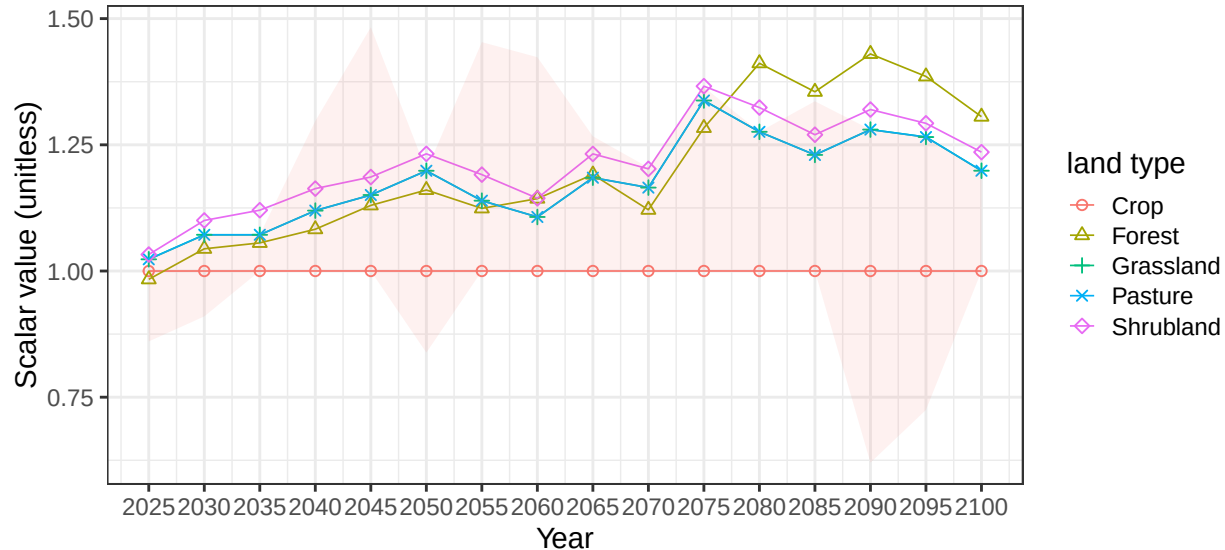
Region Russia basin LenaR average vegetation scalars
