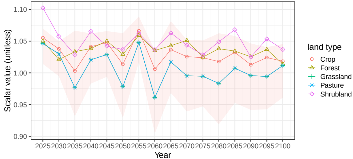
Region China basin XunJiang average soil scalars
