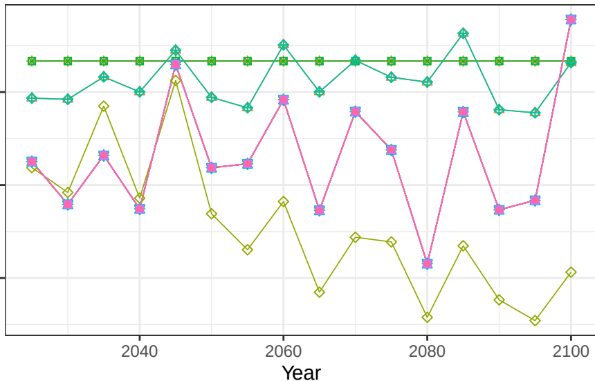
Region EU-12 basin DaugavaR crop vegetation scalars
