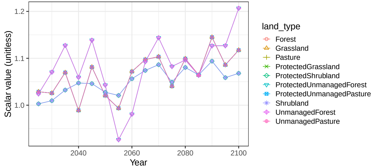
Region South Asia basin GangesR non-crop soil scalars
