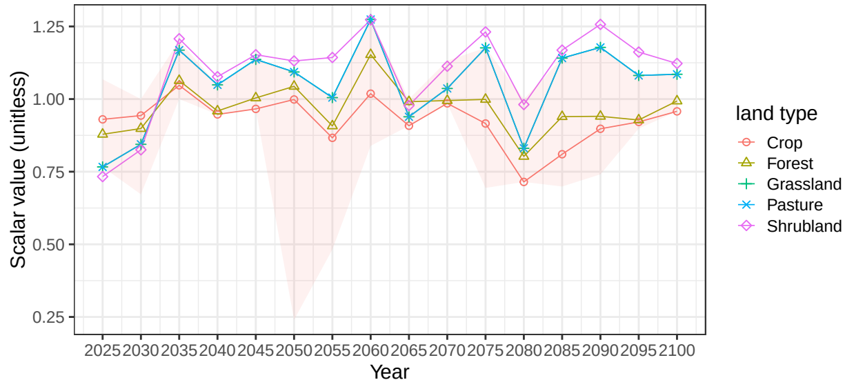
Region Russia basin BarentsSea average vegetation scalars
