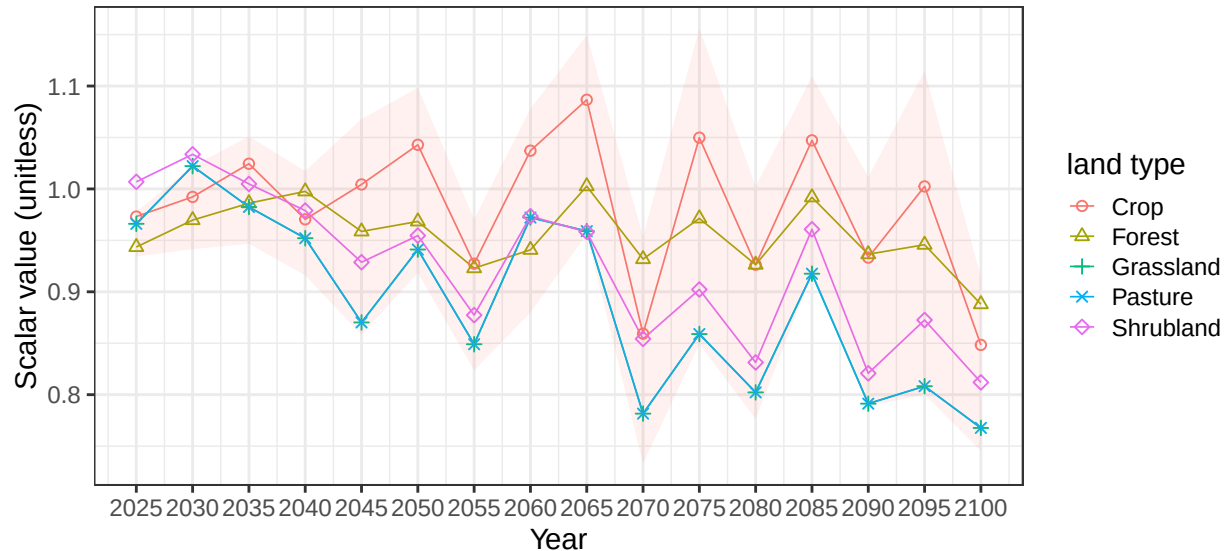
Region Argentina basin RioLaPlata average soil scalars
