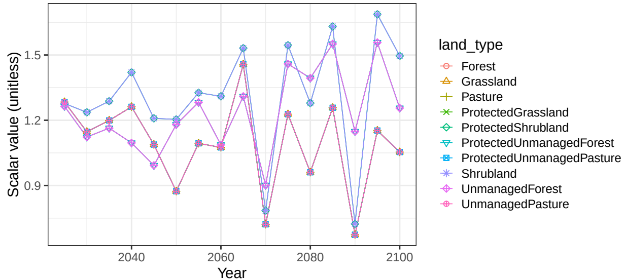
Region Argentina basin ArgColoR non-crop vegetation scalars
