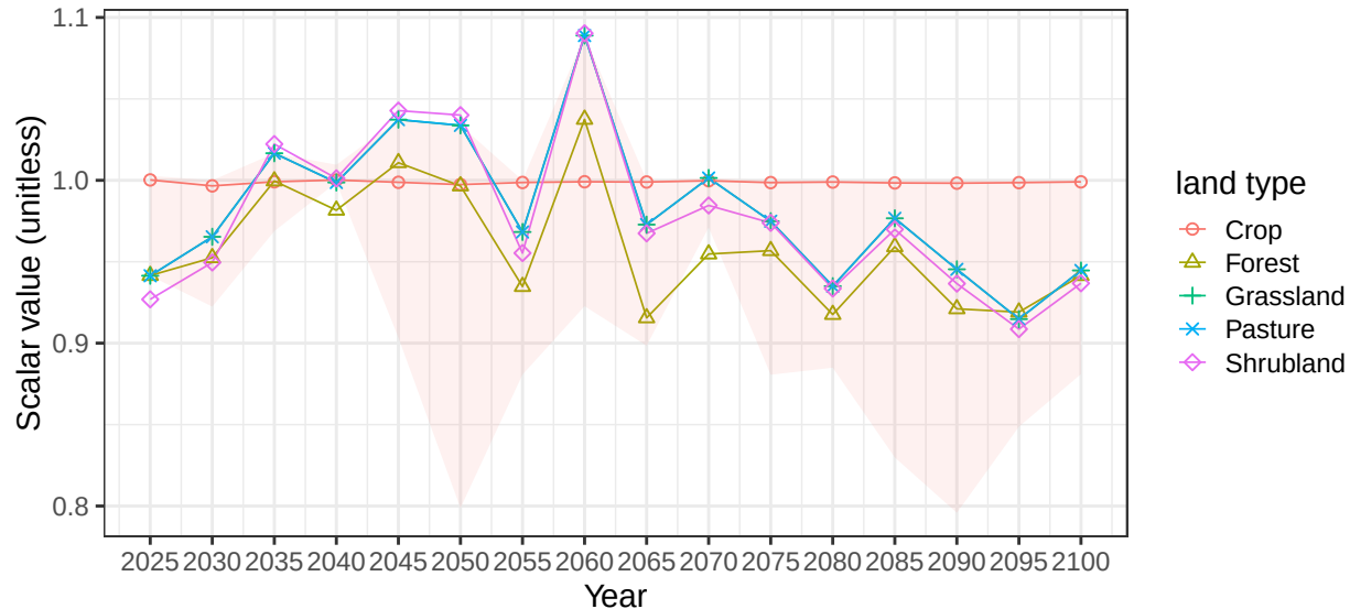
Region Russia basin DvinaRN average soil scalars
