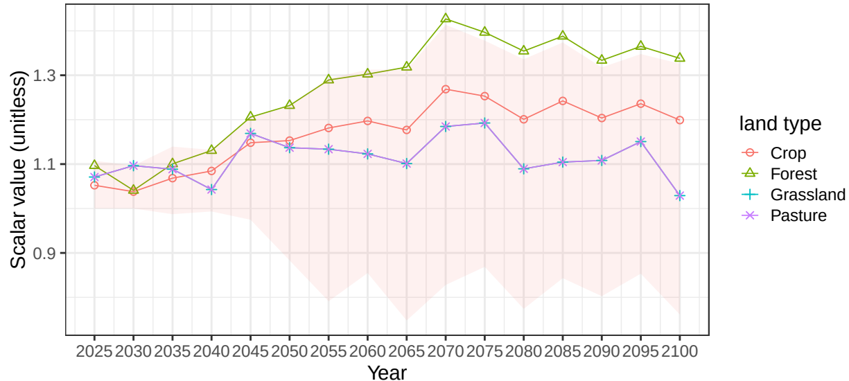
Region South America_Southern basin NegroR average vegetation scalars
