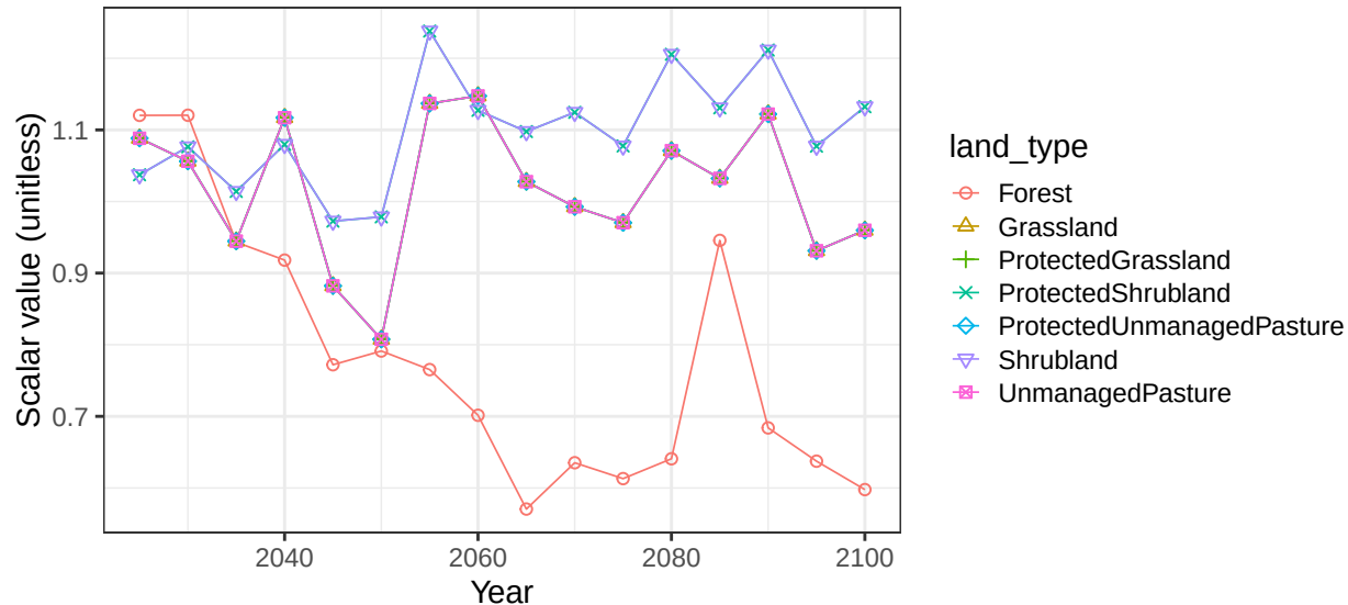
Region EU-15 basin ItalyCstE non-crop vegetation scalars
