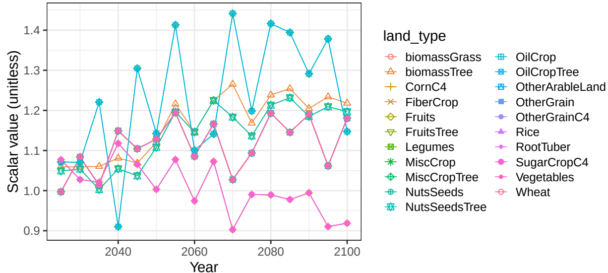
Region Africa_Southern basin AfrCstS crop soil scalars
