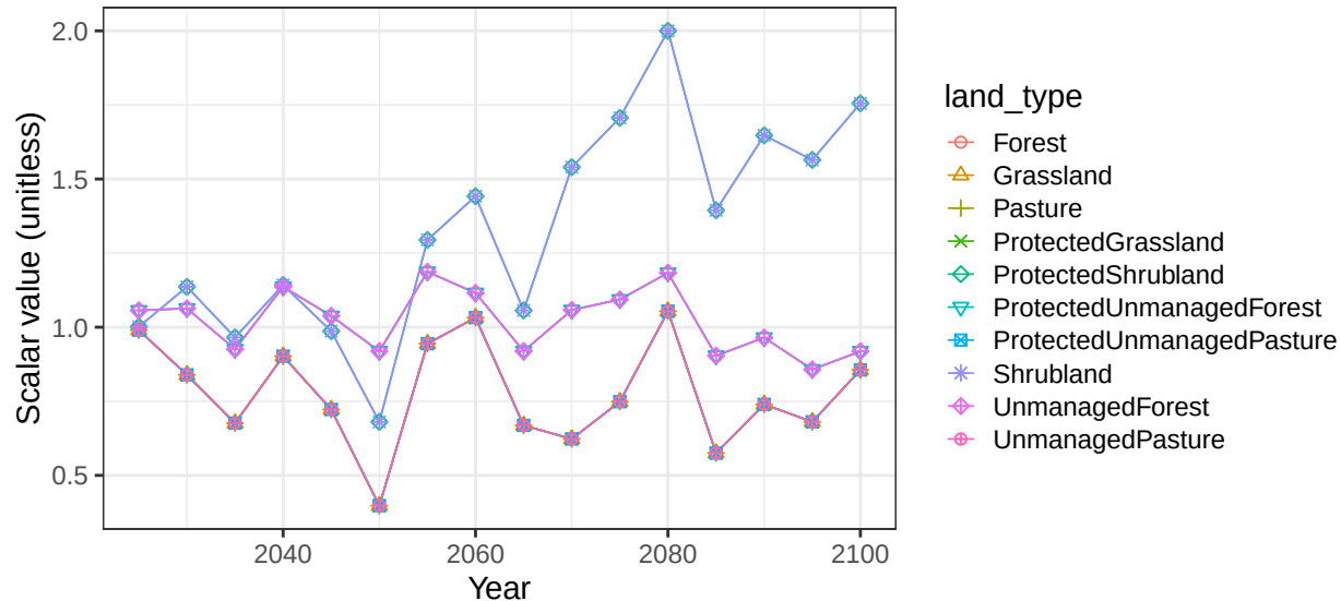
Region EU-12 basin DanubeR non-crop vegetation scalars
