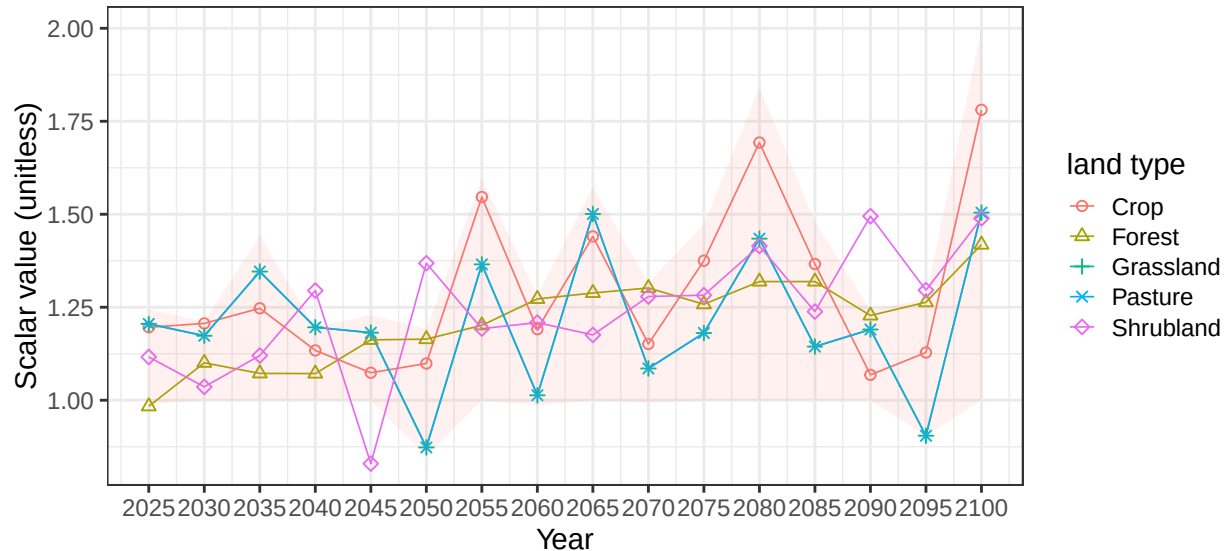
Region Central Asia basin CaspianNE average vegetation scalars
