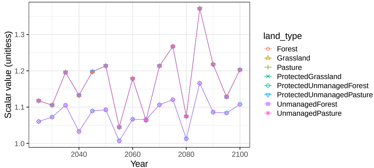
Region USA basin OhioR non-crop vegetation scalars
