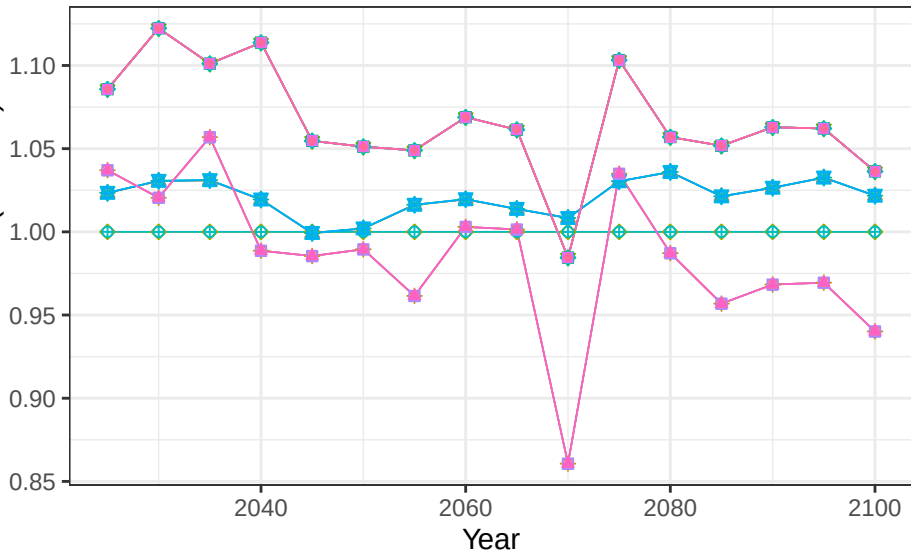
Region Southeast Asia basin IrianJaya crop soil scalars
