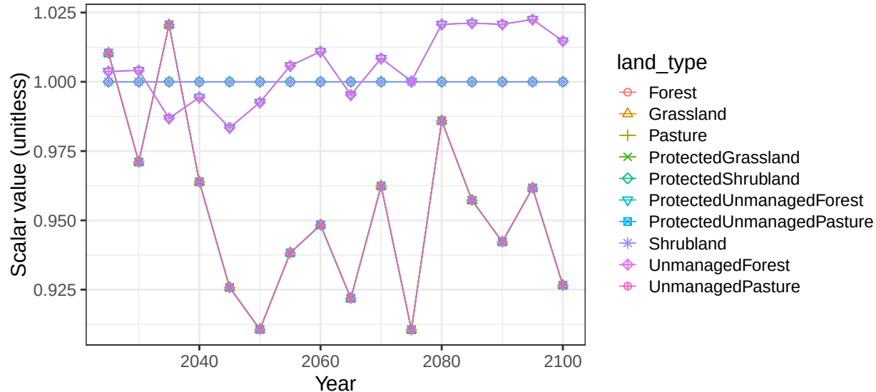
Region Central America and Caribbean basin ColEcuacSt non-crop soil s
