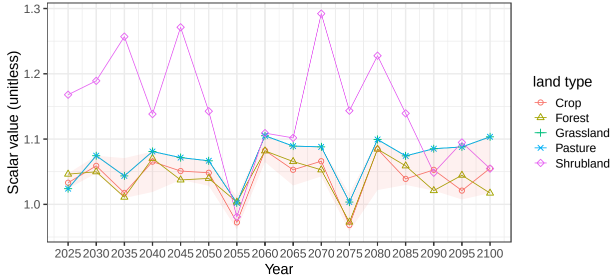
Region Southeast Asia basin Salween average soil scalars
