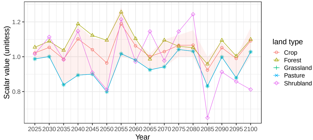
Region Europe_Eastern basin DanubeR average soil scalars
