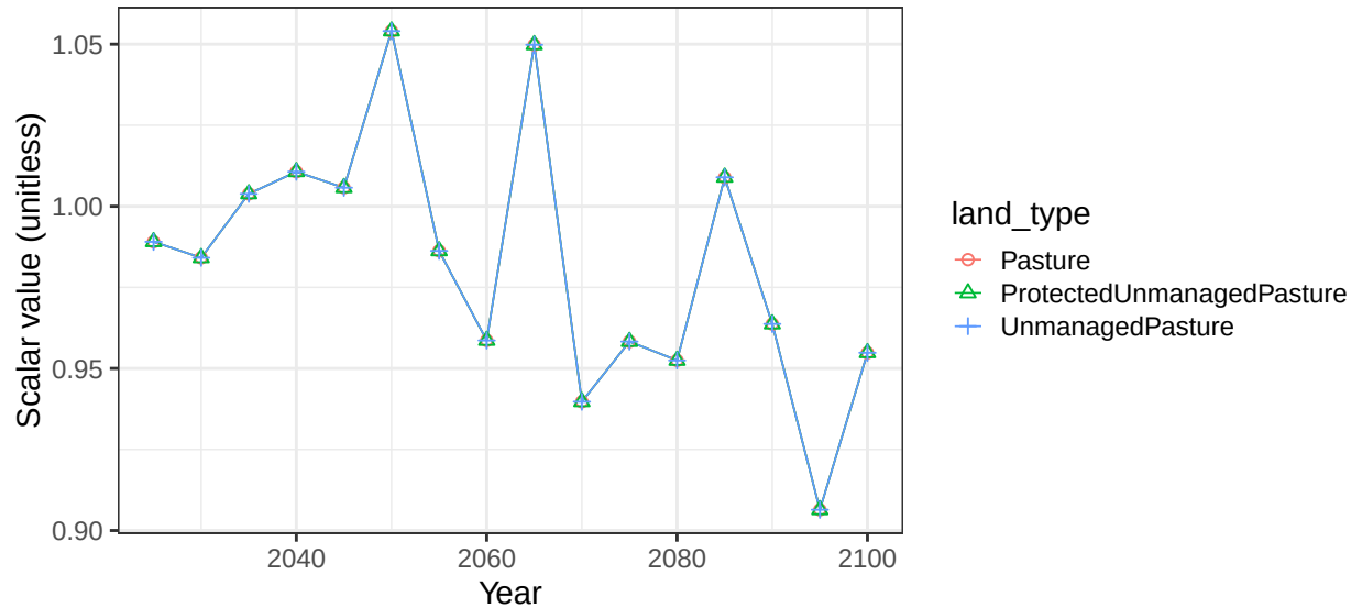
Region China basin SyrDaryaR non-crop soil scalars
