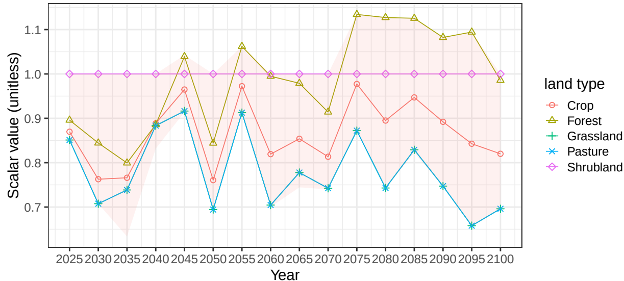
Region Mexico basin YucatanP average vegetation scalars
