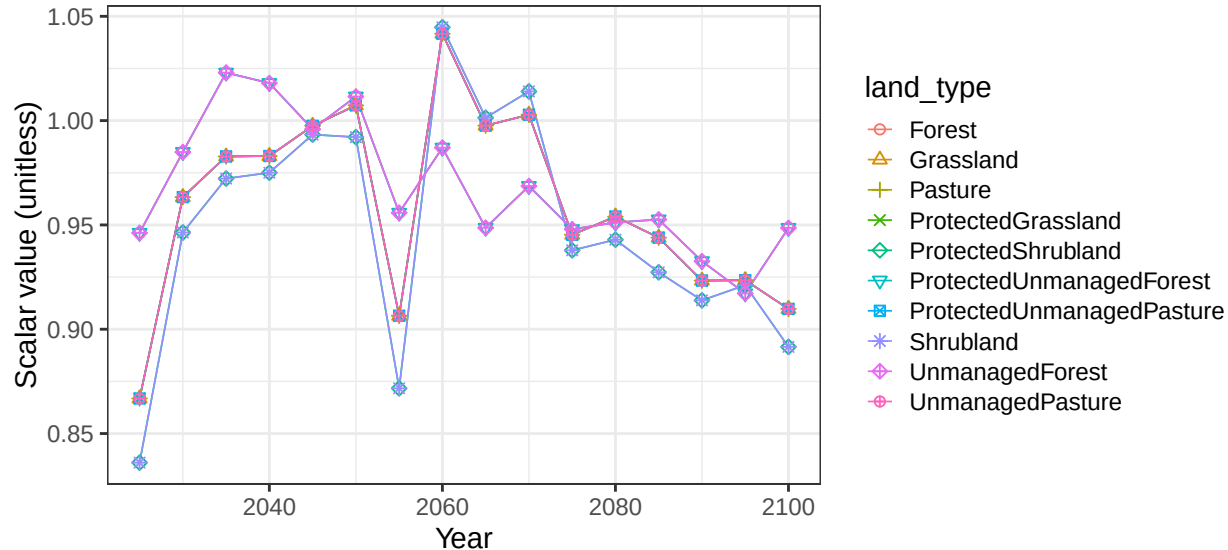
Region Canada basin StLwrncR non-crop soil scalars
