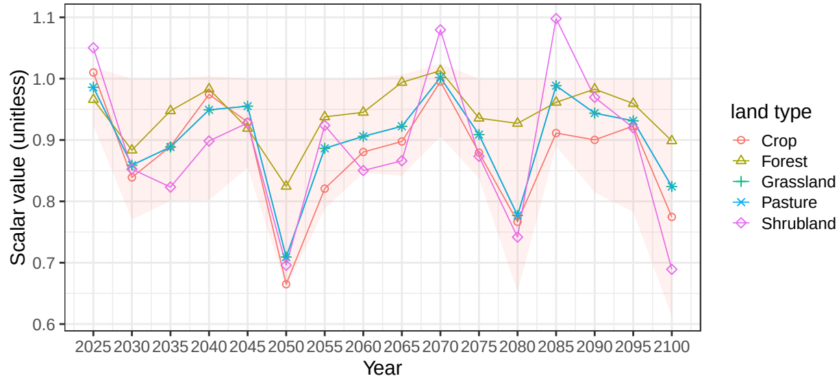
Region Australia_NZ basin MurrayDrlg average soil scalars
