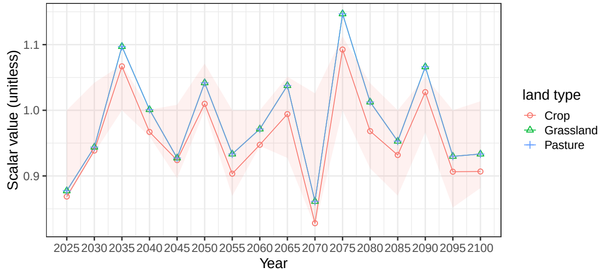
Region South America_Southern basin BrzCstS average soil scalars
