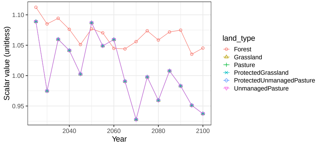
Region Africa_Eastern basin CongoR non-crop soil scalars
