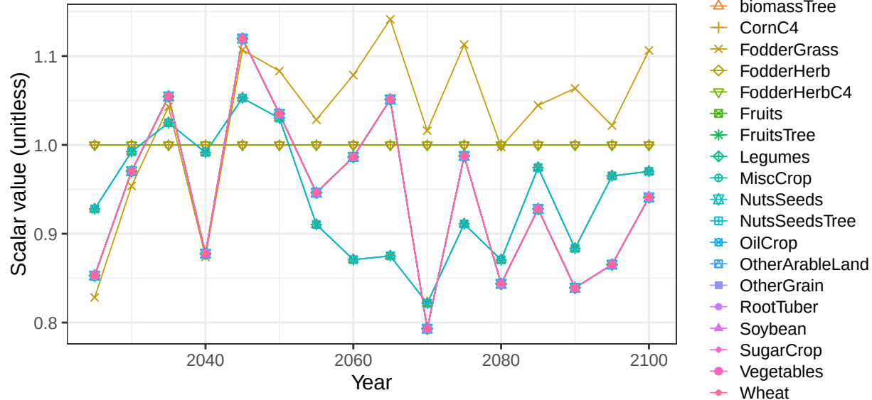
Region EU-15 basin DnkGrnCst crop soil scalars
