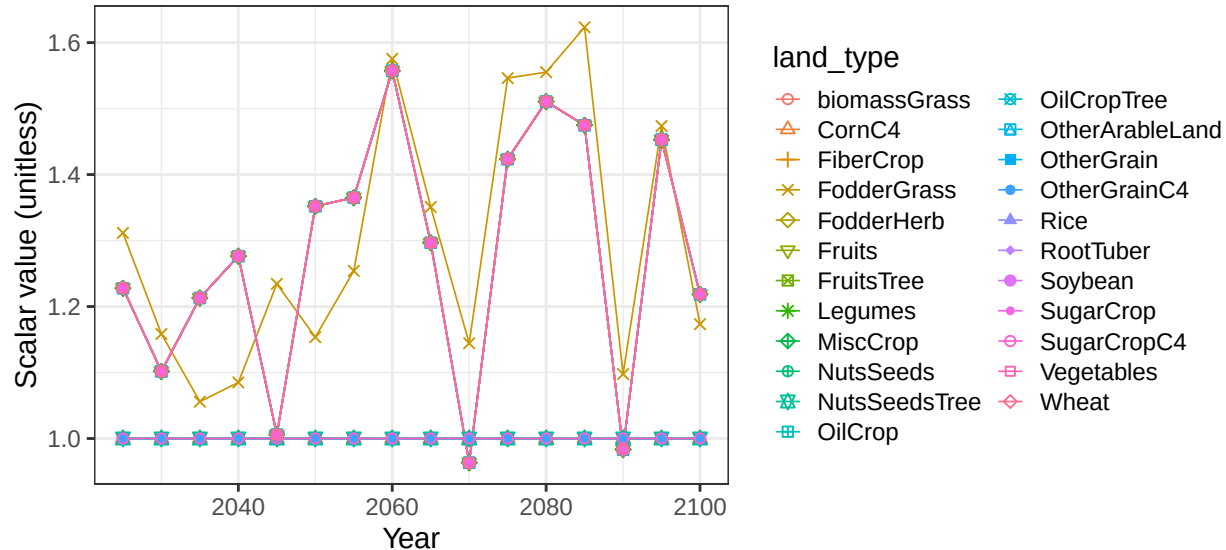
Region Middle East basin FarahrudR crop vegetation scalars
