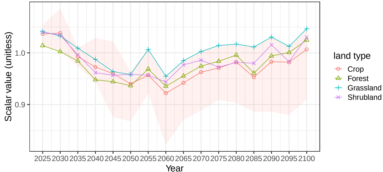
Region Japan basin Japan average vegetation scalars
