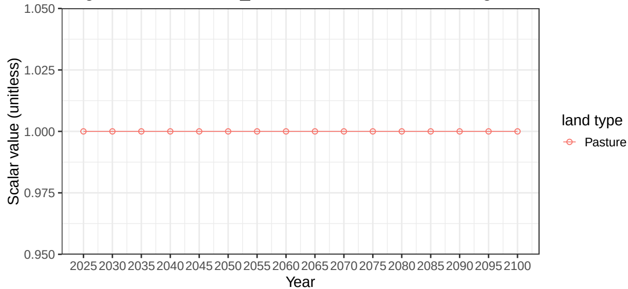
Region South America_Southern basin Salinas average soil scalars
