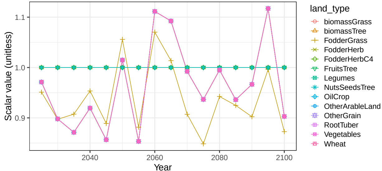
Region Central Asia basin AmurR crop soil scalars
