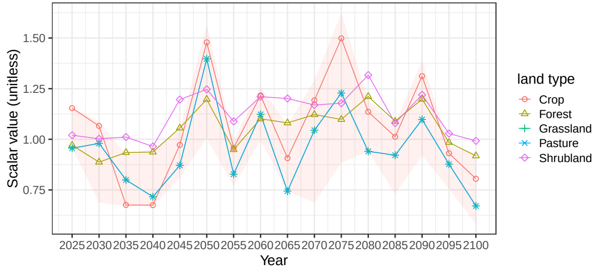
Region Central Asia basin ObR average vegetation scalars
