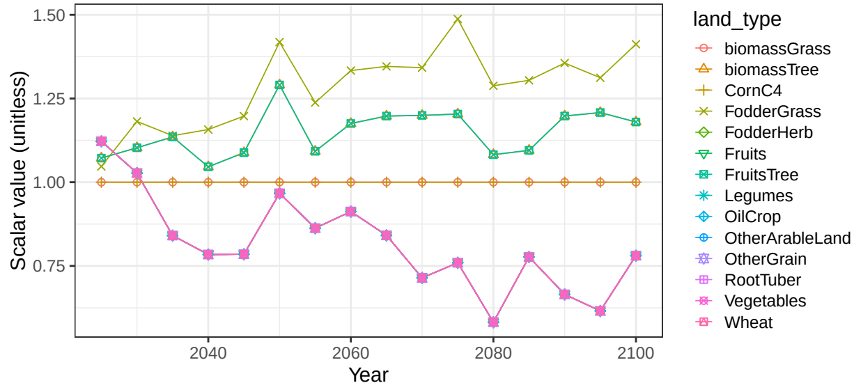
Region European Free Trade Association basin ScndnvN crop vegetation s
