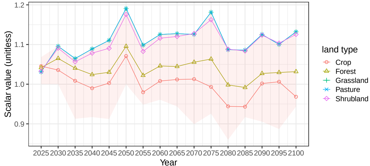
Region European Free Trade Association basin ScndnvN average soil scalar
