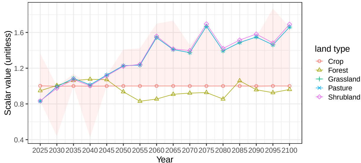
Region Russia basin Finland average vegetation scalars
