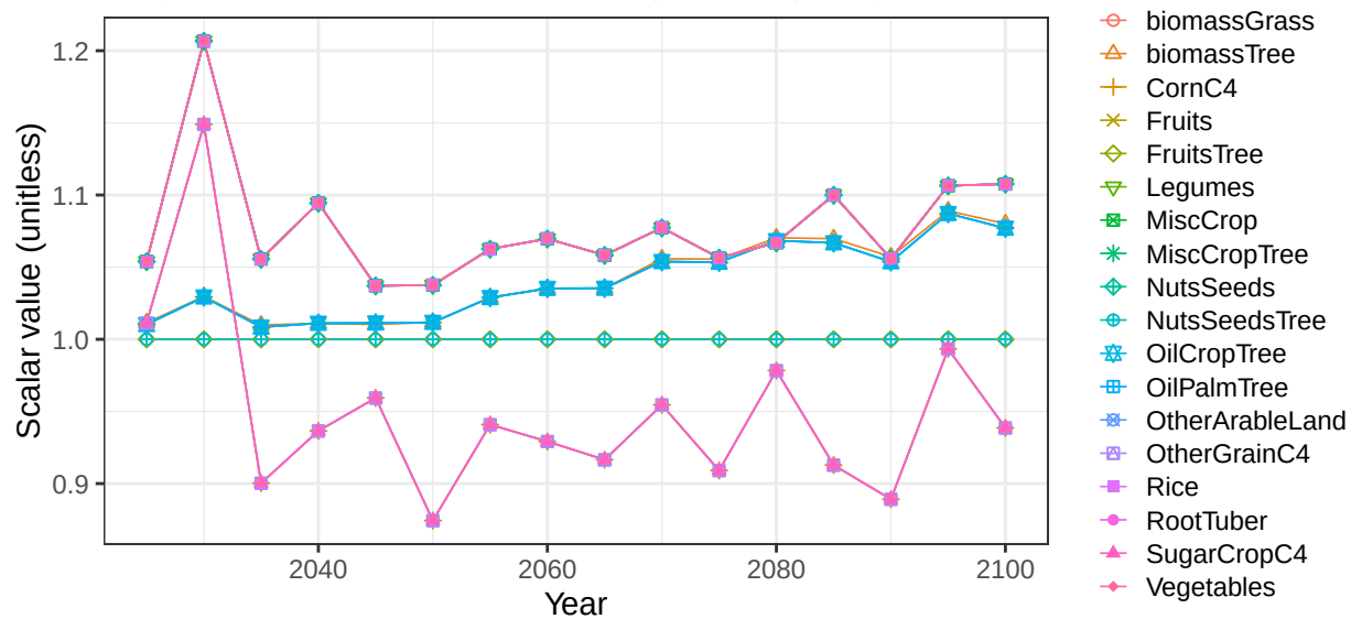
Region Southeast Asia basin SepikR crop vegetation scalars
