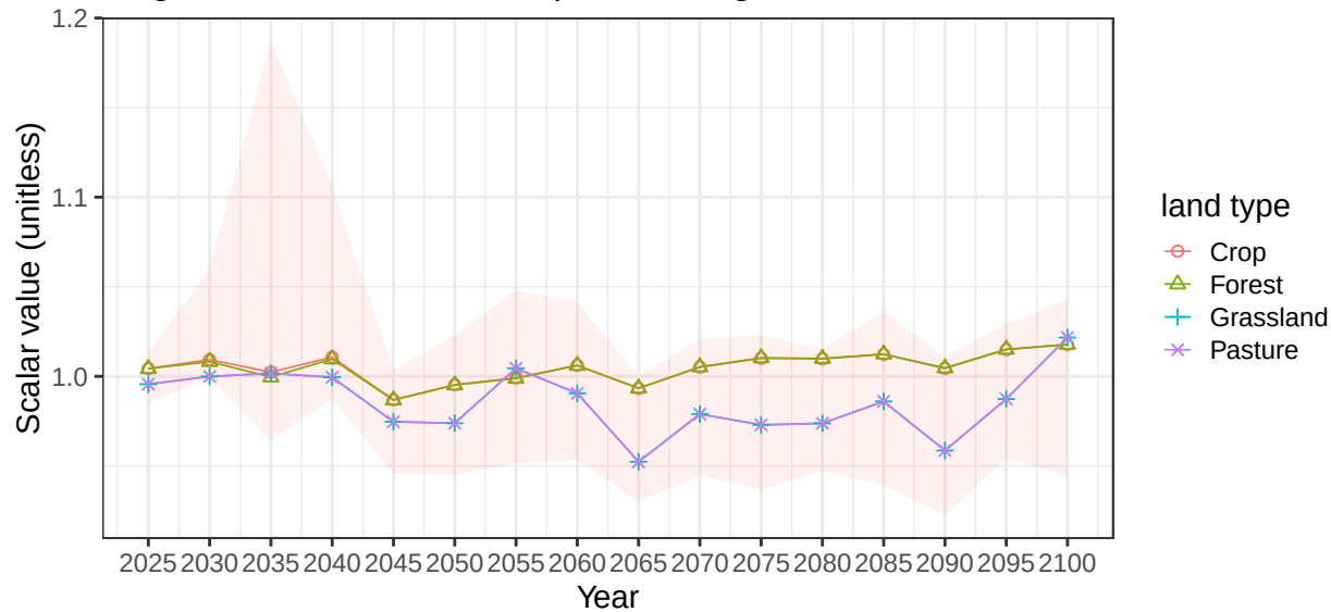
Region Indonesia basin SepikR average soil scalars
