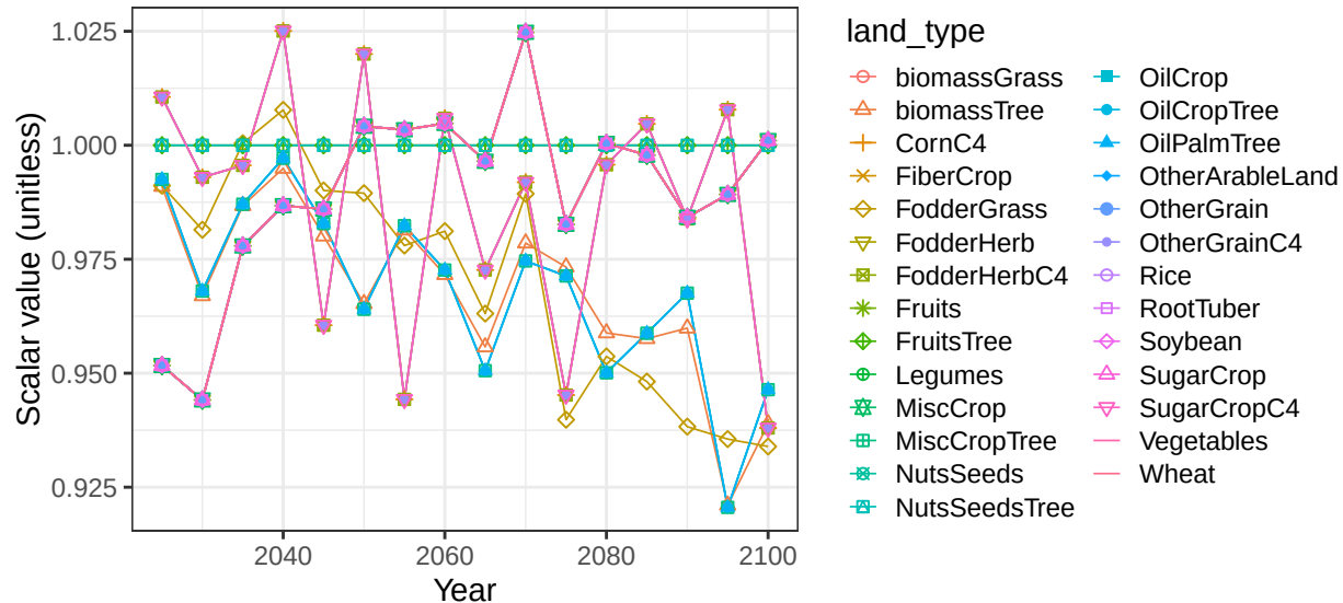
Region South America_ Southern basin LaPuna crop soil scalars
