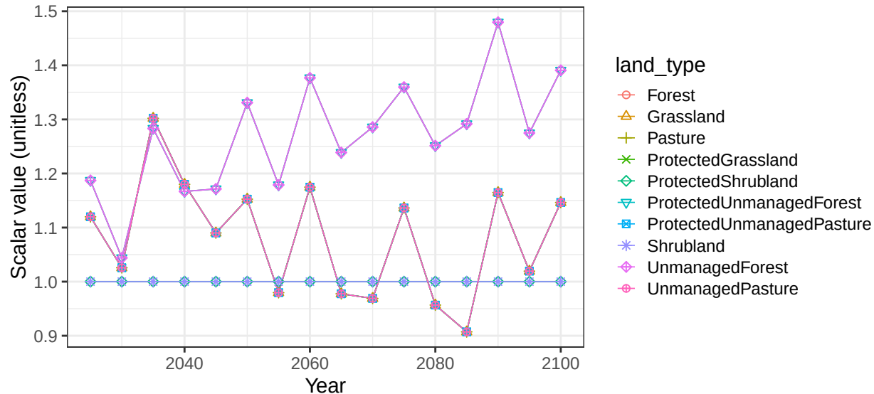
Region Africa_Southern basin RiftValley non-crop vegetation scalars
