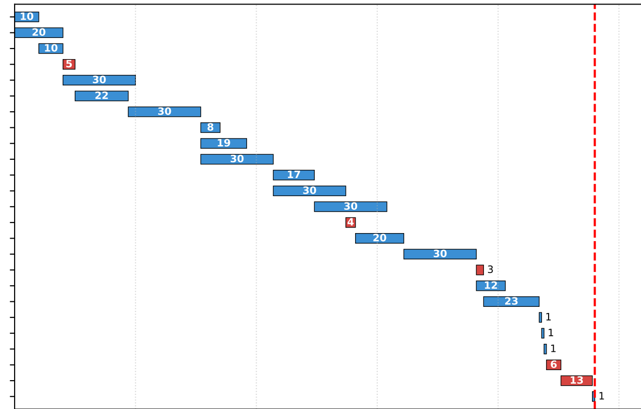
SPOC Optimal Sol 1 of 3 makespan 240, crash cost Z^* = 300
