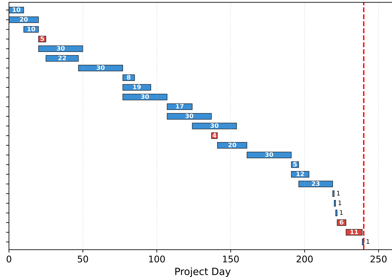
SPOC Optimal Sol 3 of 3 makespan 240, crash cost Z^* = 300
