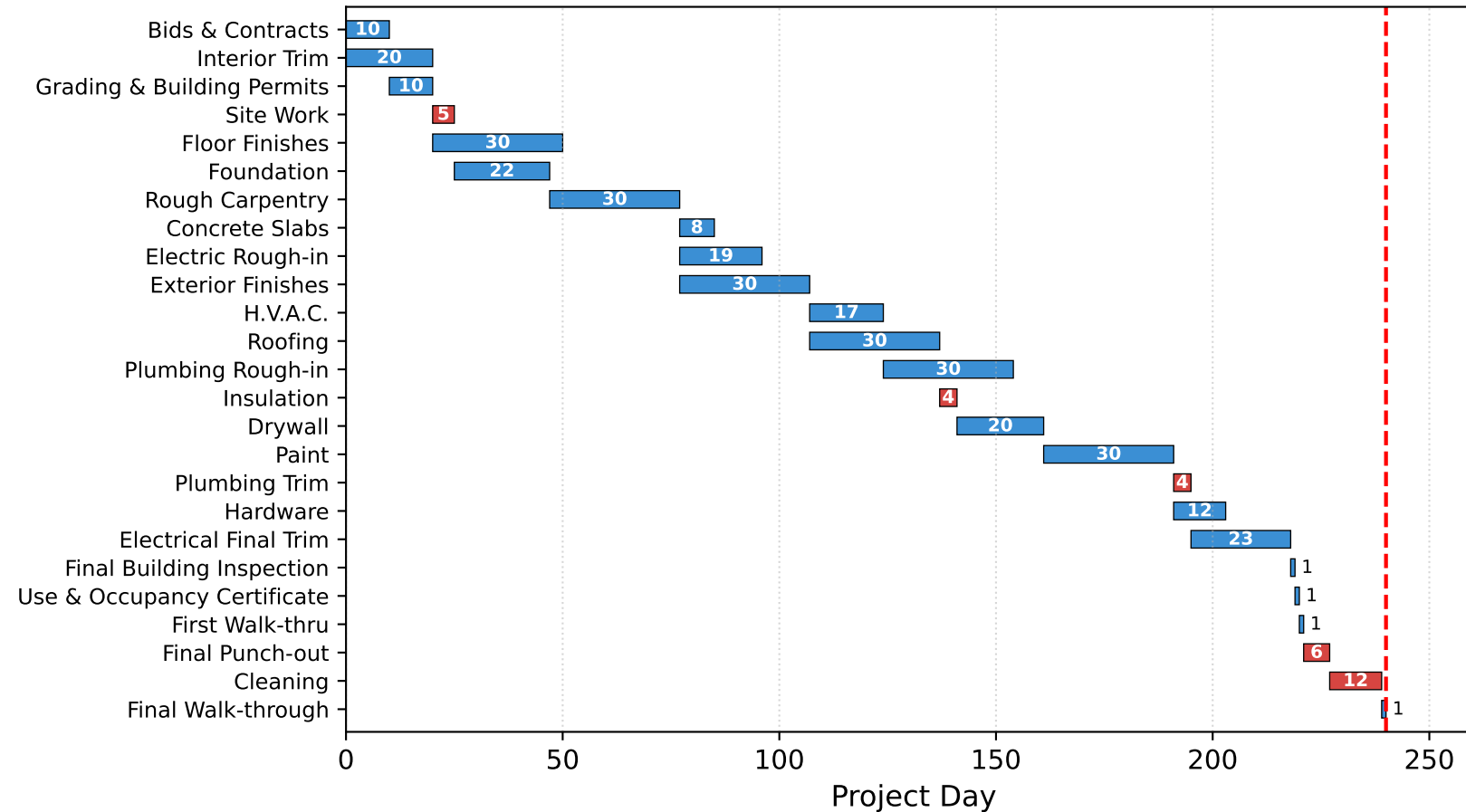
SPOC Optimal Sol 2 of 3 makespan 240, crash cost Z^* = 300
