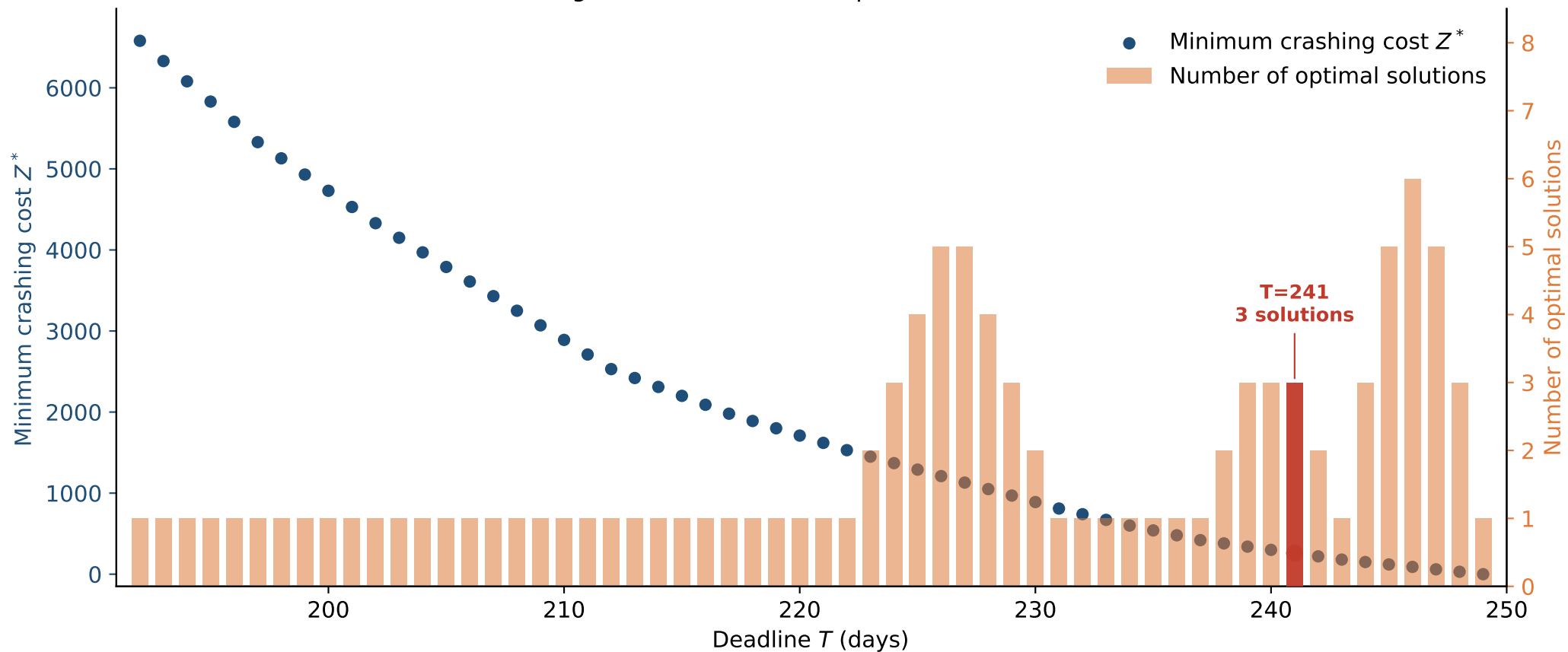
Minimum crashing cost and number of optimal solutions across deadlines
