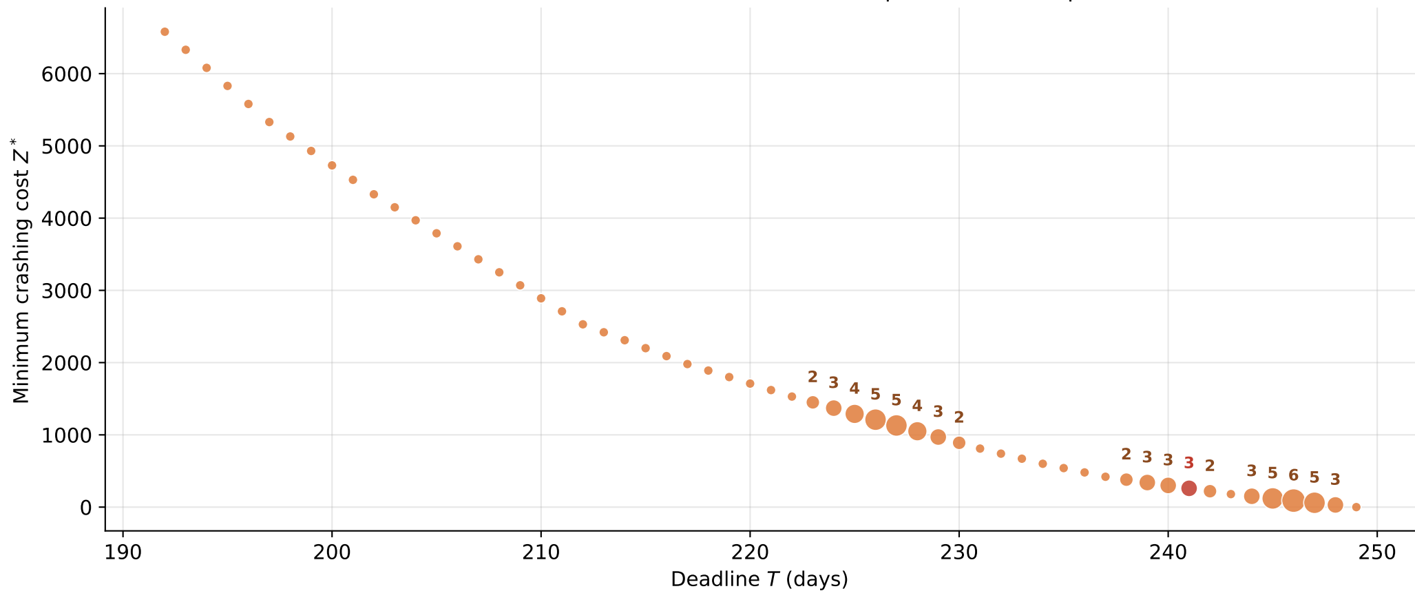
Time-cost frontier; marker size/label = number of optimal solutions per deadline
