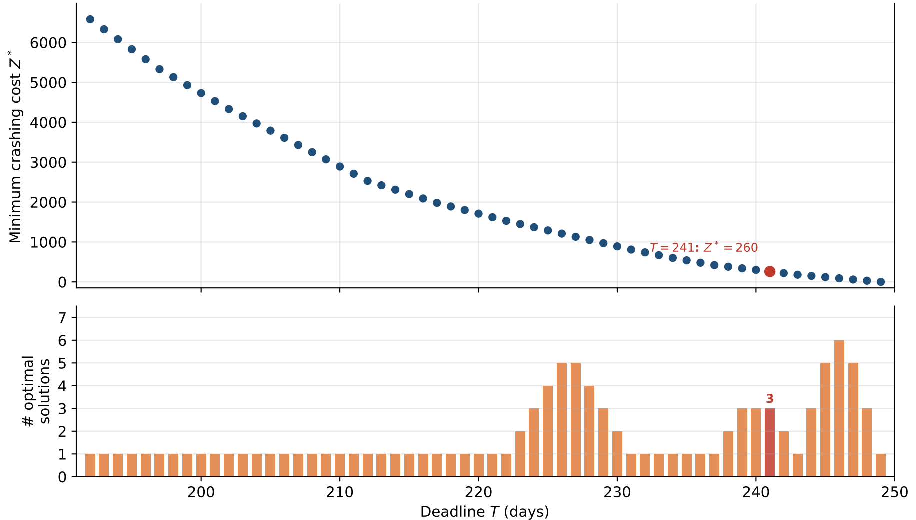
Minimum crashing cost and number of optimal solutions per integer deadline ( T = 192-249 )
