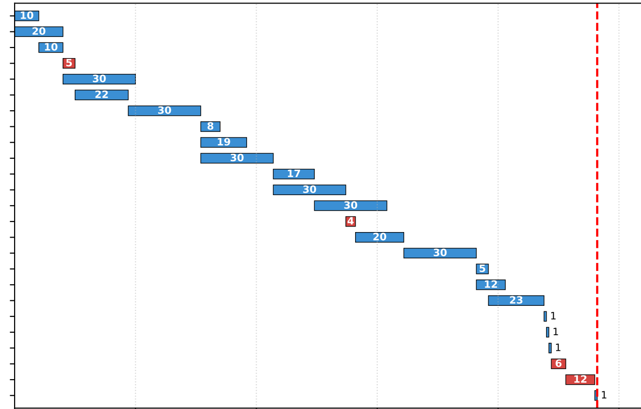
SPOC Optimal Solution 1 of 3 makespan 241, crash cost Z^* = 260
