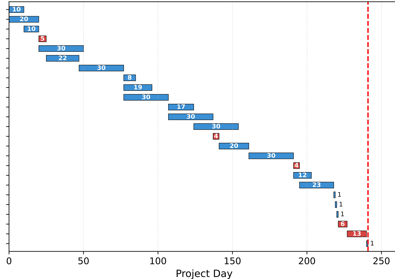
SPOC Optimal Solution 3 of 3 makespan 241, crash cost Z^* = 260
