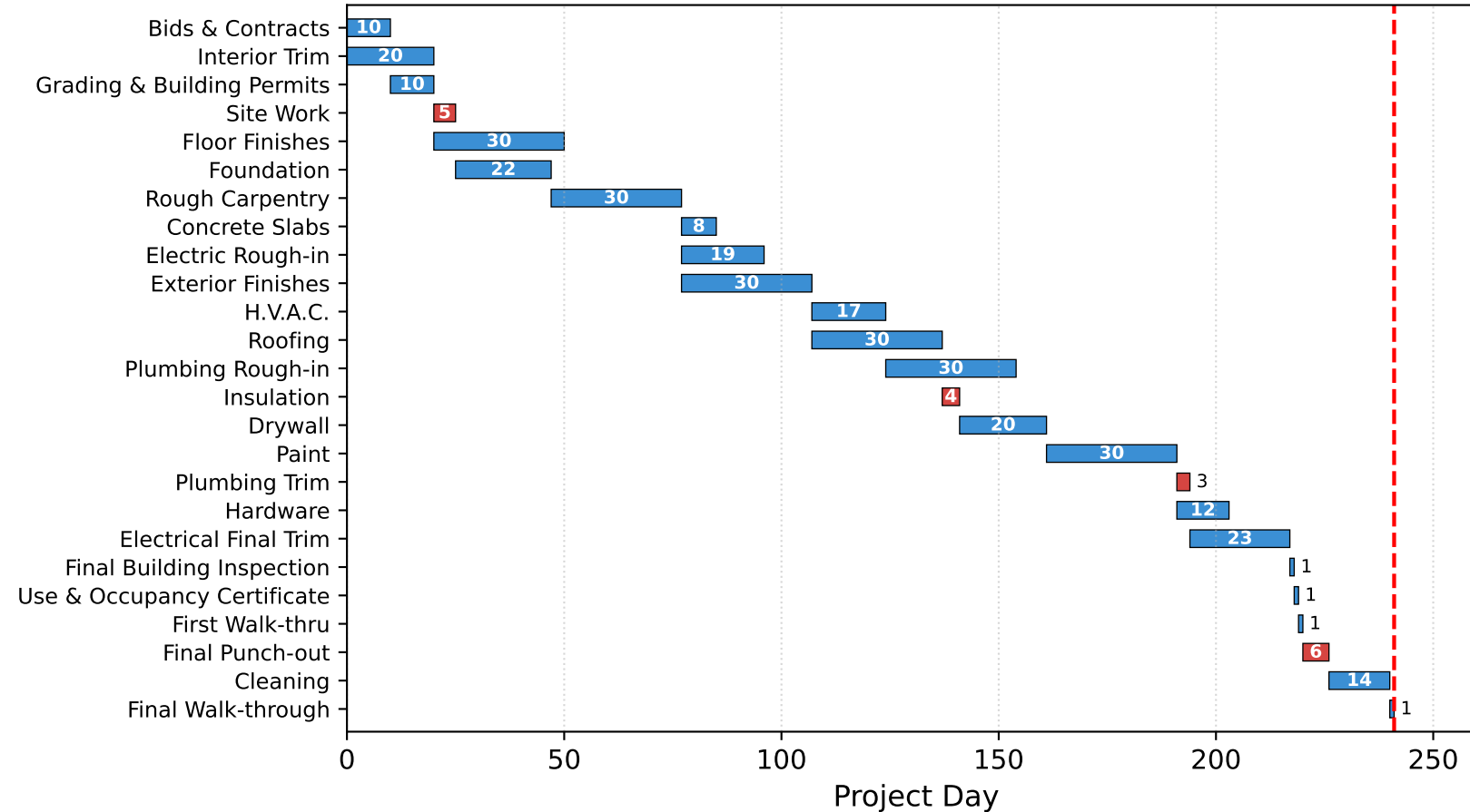
SPOC Optimal Solution 2 of 3 makespan 241, crash cost Z^* = 260
