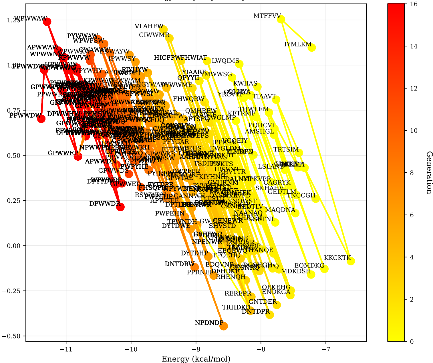
Energy vs Hydrophobicity
