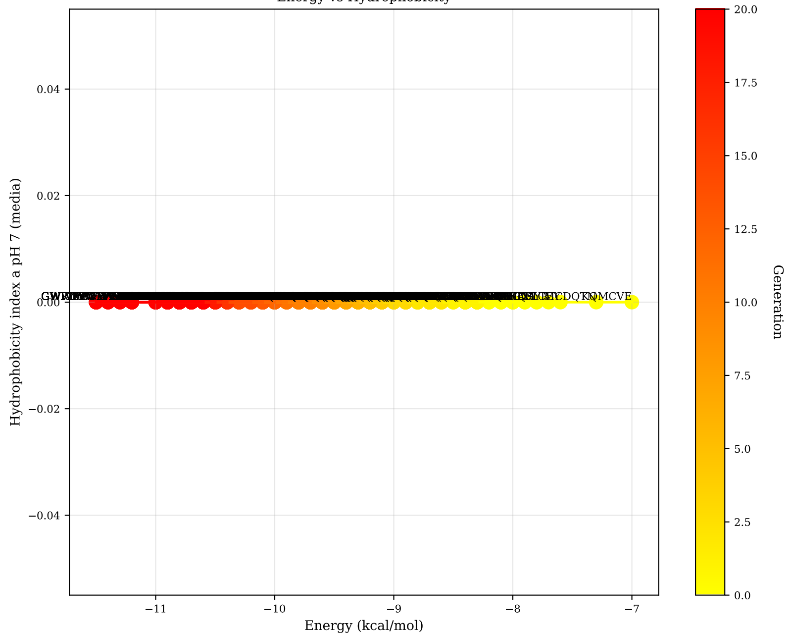
Energy vs Hydrophobicity
