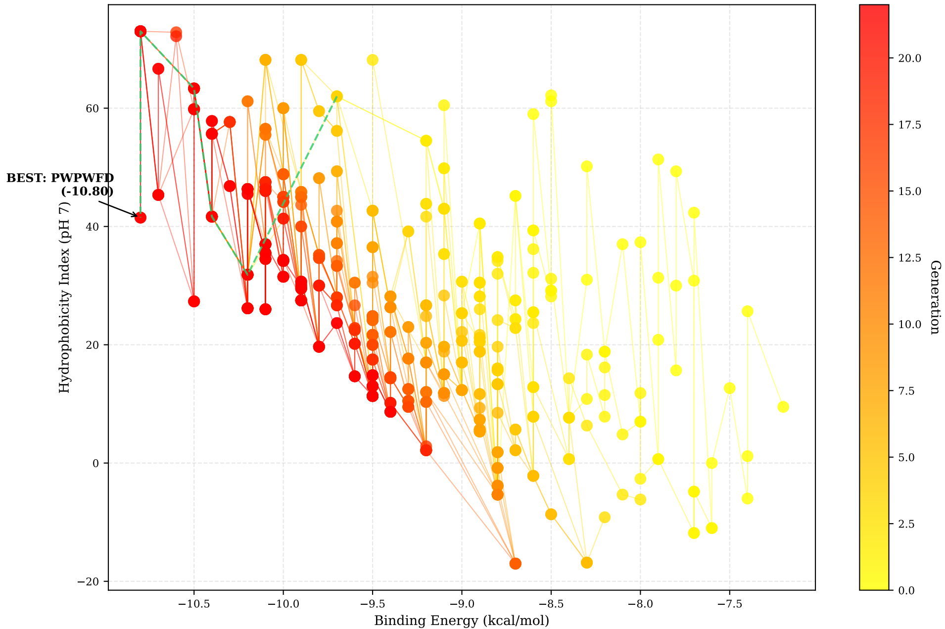
Evolution Landscape (Job 427568)
