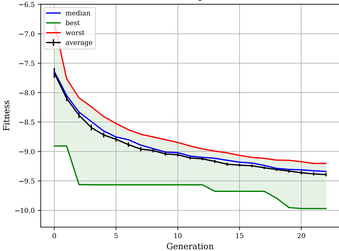
Fitness Trend - Job 427568
