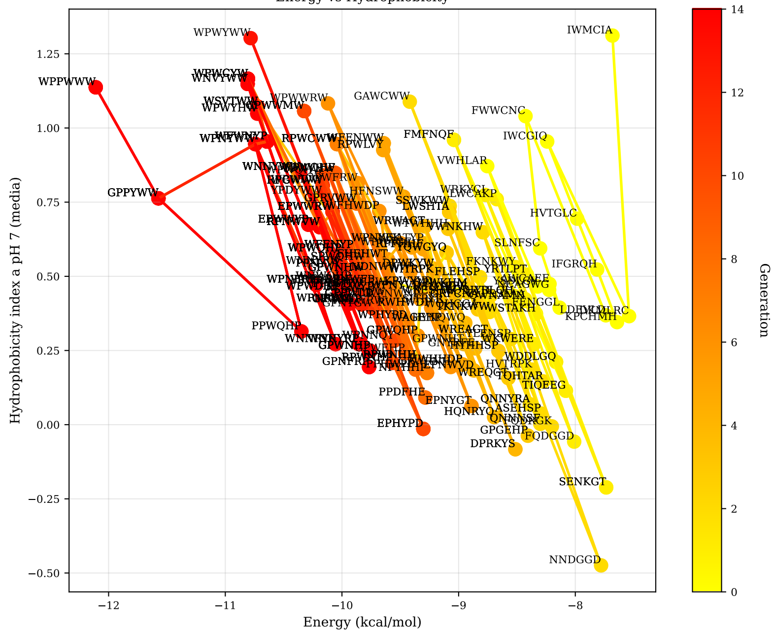
Energy vs Hydrophobicity
