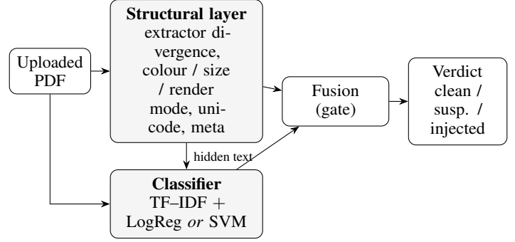
Figure 1: Pipeline. The structural layer localises hidden text and emits typed signals; the classifier scores the document text and the recovered hidden text; fusion gates structural findings behind the classifier and maps the fused risk to a verdict.
