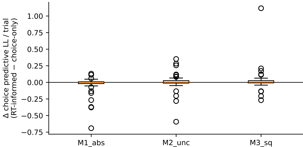
(a) does RT improve held-out choice prediction?
