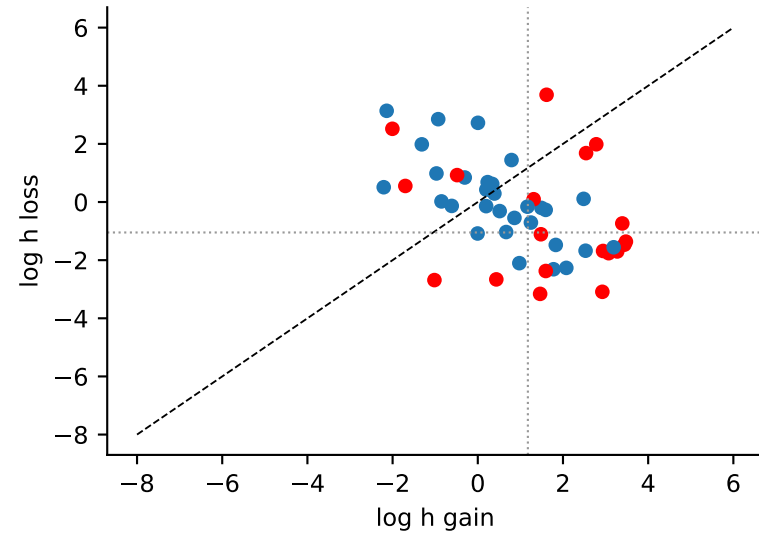
sign effect (red = poorly identified)
