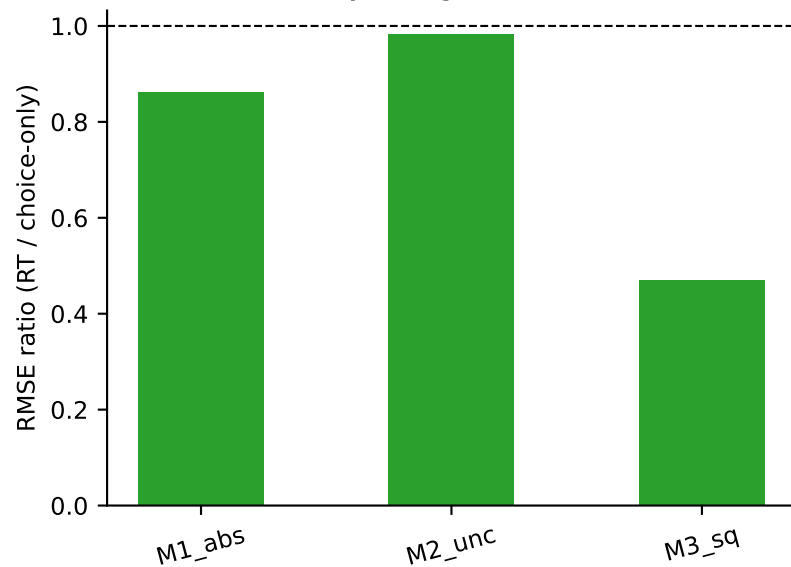
recovery of log h (simulation)
