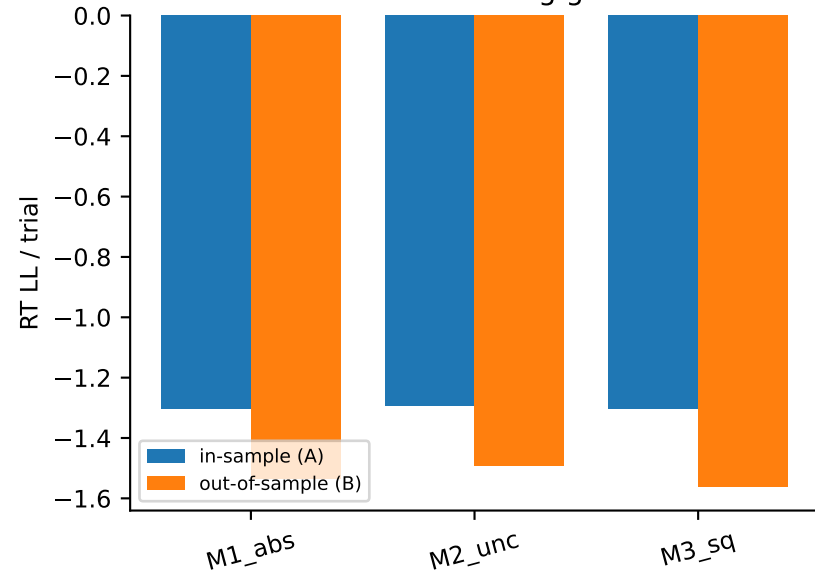
RT fit: does the ranking generalise?
