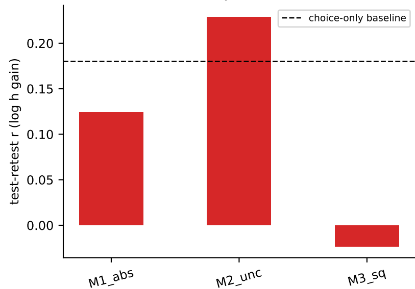
reliability (real data)
