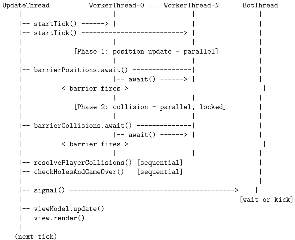
Figure 2: Thread interactions and synchronization points during a single game tick.
