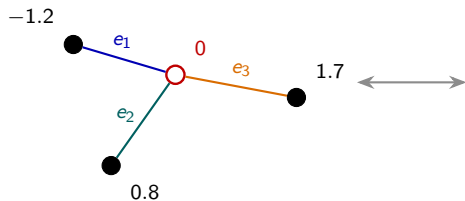
Rooted Labelled Graph G(\xi, p)
