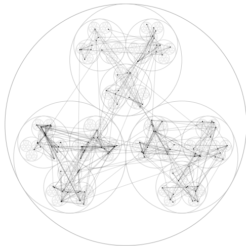
SIRG in \mathbb{Q}_3
