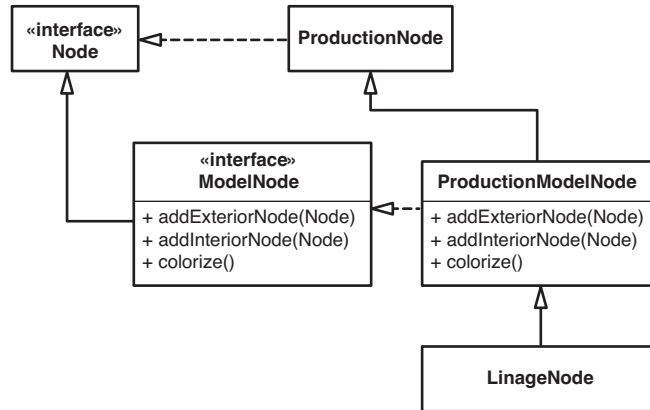
Figure 25.4 Extract Implementer on ModelNode.
