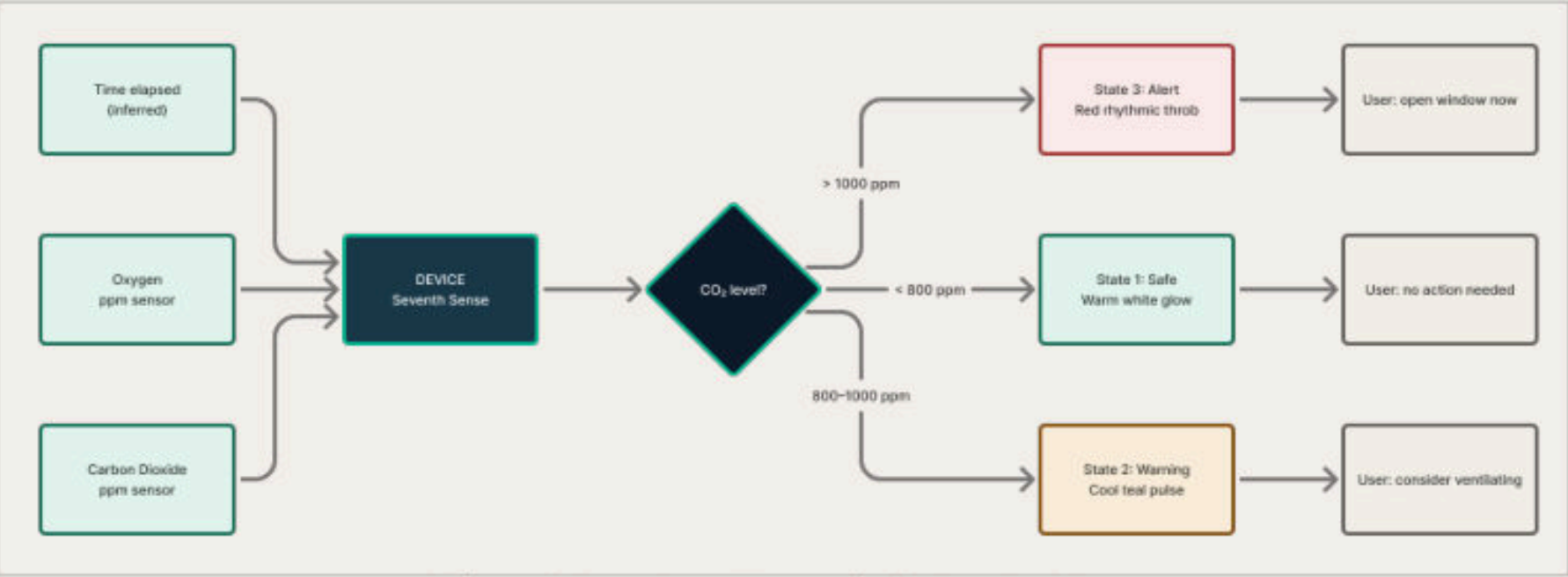
Fig. 05 – Inputs and Outputs Map
