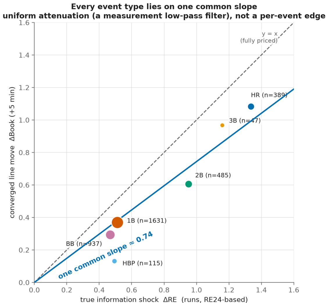
Figure 6. The market transfer function. Every positive-run event type lies on one common slope \approx 0.74 ; marker area is proportional to event count.
