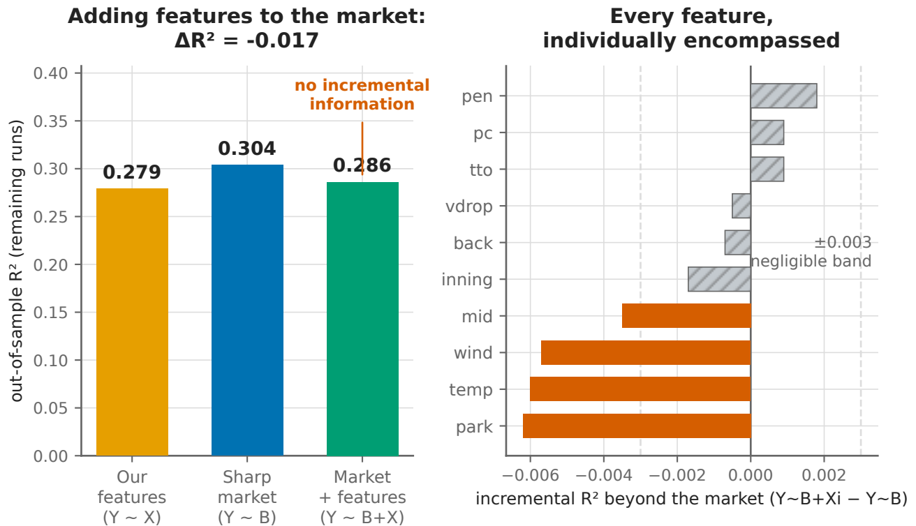
Figure 4. Forecast encompassing. Left: adding the feature set to the market forecast changes out-of-sample R^2 by -0.017 . Right: each feature's individual incremental R^2 beyond the market; bars inside the 0.003 band are drawn in neutral gray.
