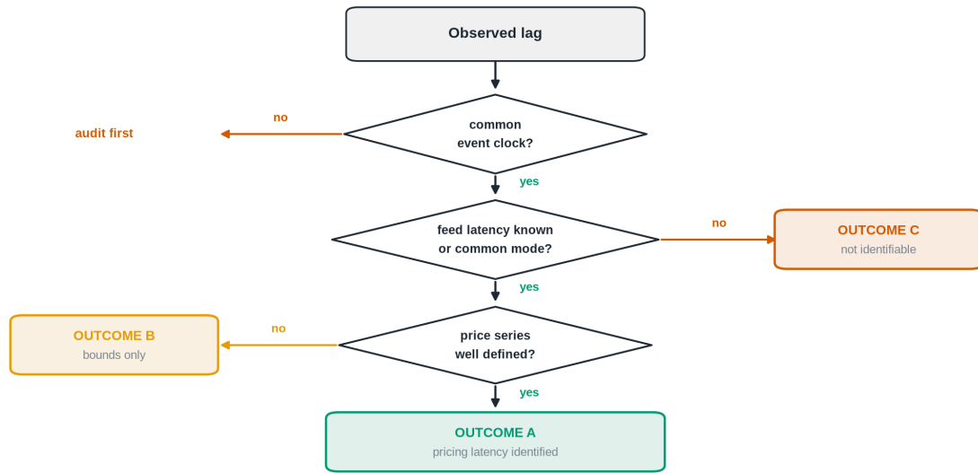
Figure 7. The paper does not presuppose which branch it takes. The same logic, as a decision the reader can walk. All three terminal states are publishable, and the third is the one a study is least likely to report.
