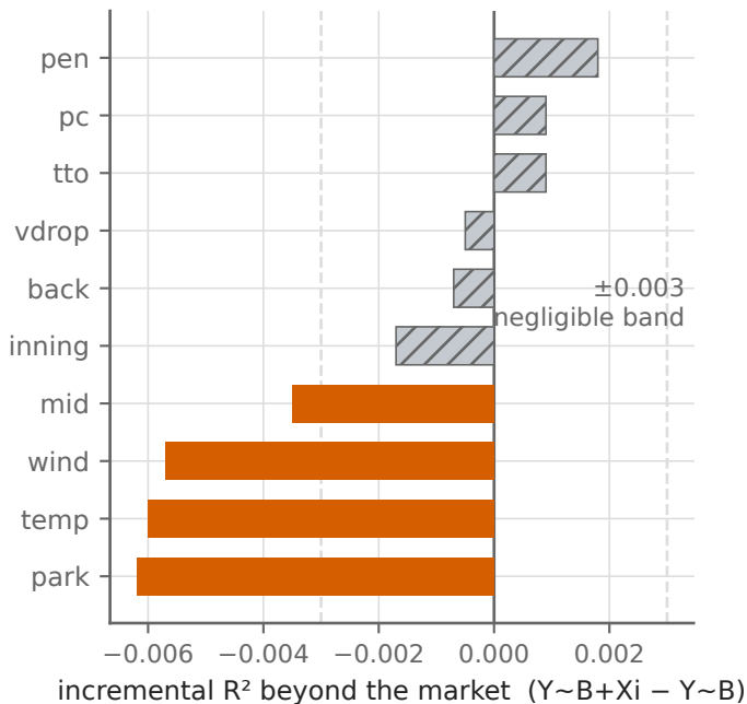
Every feature, individually encompassed
