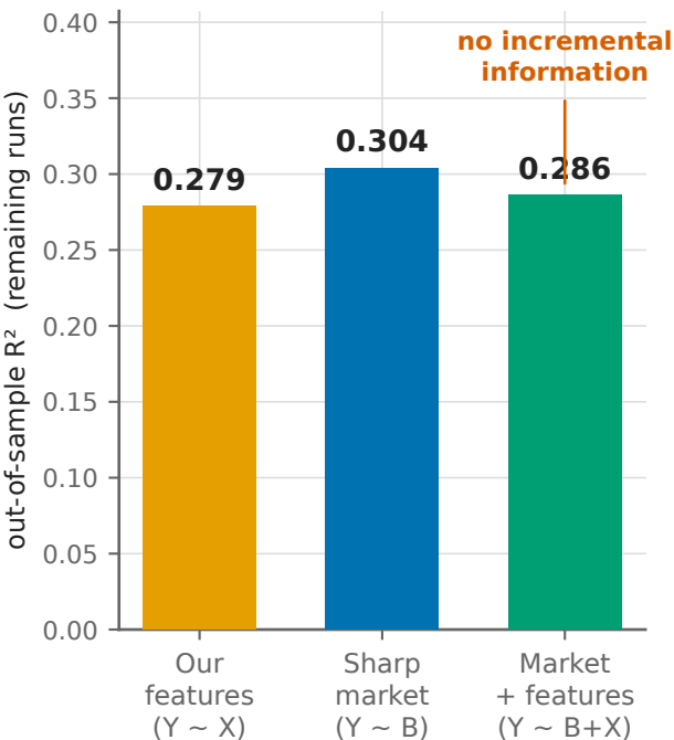
Adding features to the market: \Delta R^2 = -0.017
