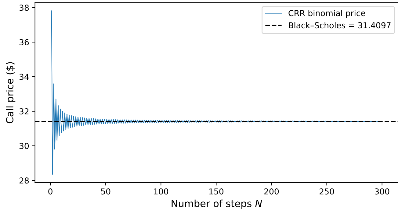
CRR binomial price vs. number of steps
