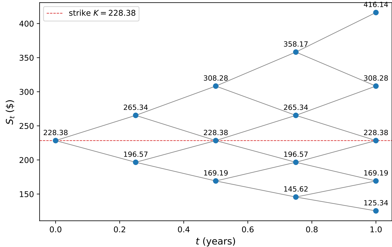
CRR tree for NVDA, N = 4 ( u = 1.1618 , d = 0.8607 , \tilde{p} = 0.4959 )
