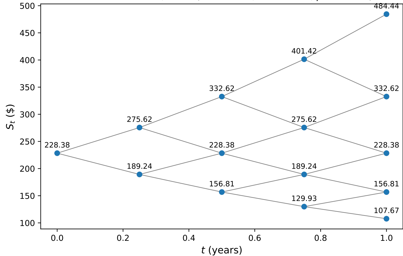
CRR tree for NVDA, N = 4 ( u = 1.2068 , d = 0.8286 , \tilde{p} = 0.4797 )
