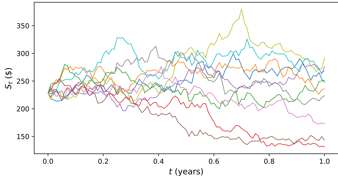
Simulated NVDA price paths under GBM (Euler-Maruyama, N = 100 , 10 paths)
