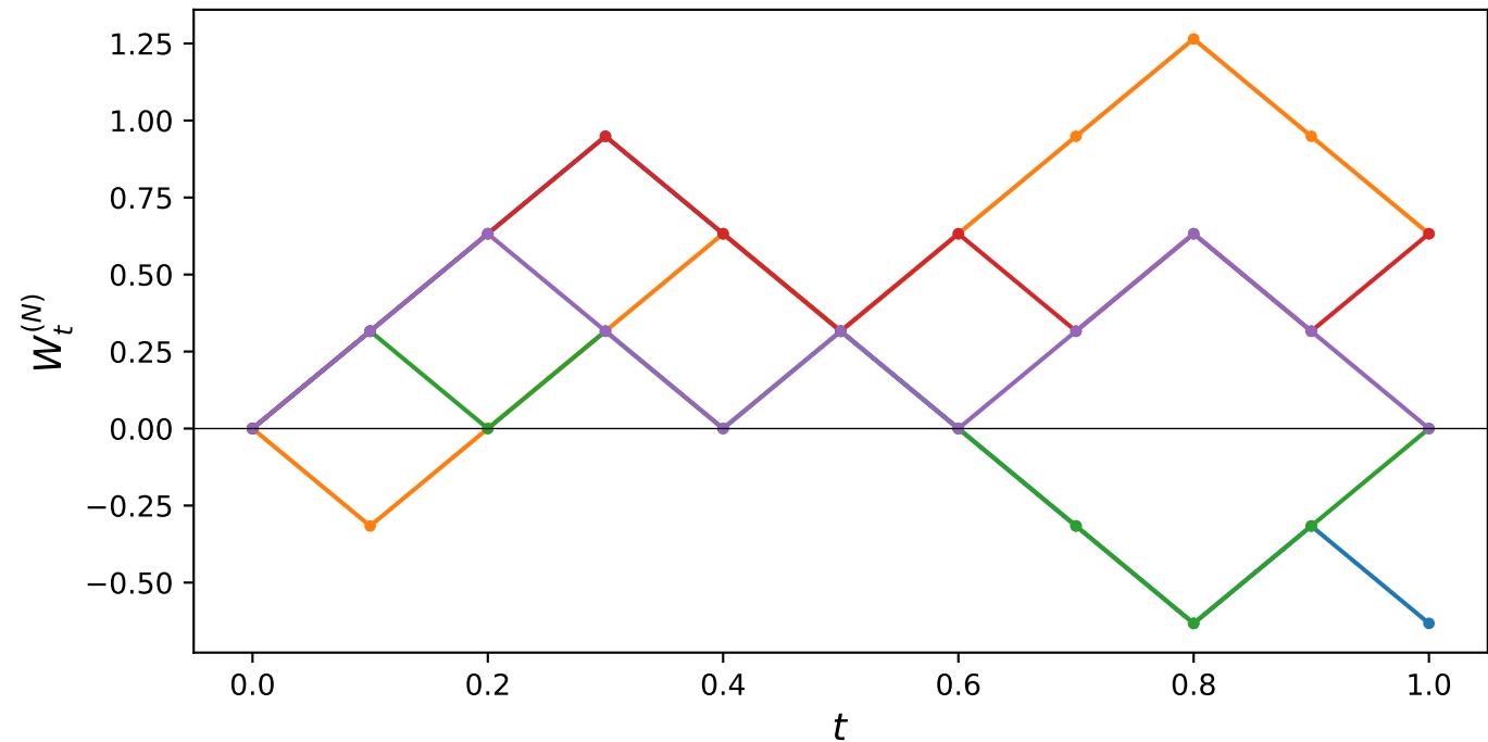
Scaled symmetric random walk, 5 sample paths ( N_2 = 10 )
