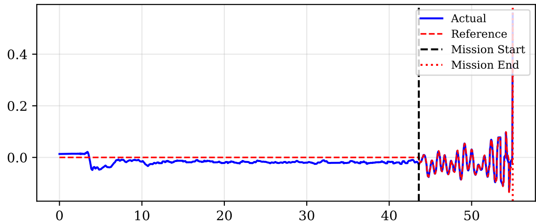
Pitch [rad]
