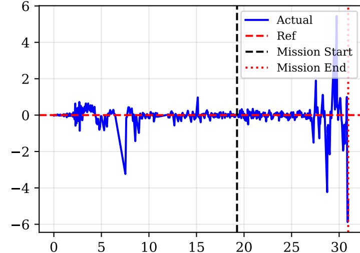
Linear Acc Z [ \text{m/s}^2 ]
