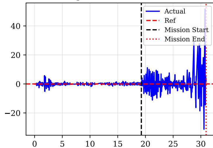
Angular Acc Z [ \text{rad/s}^2 ]
