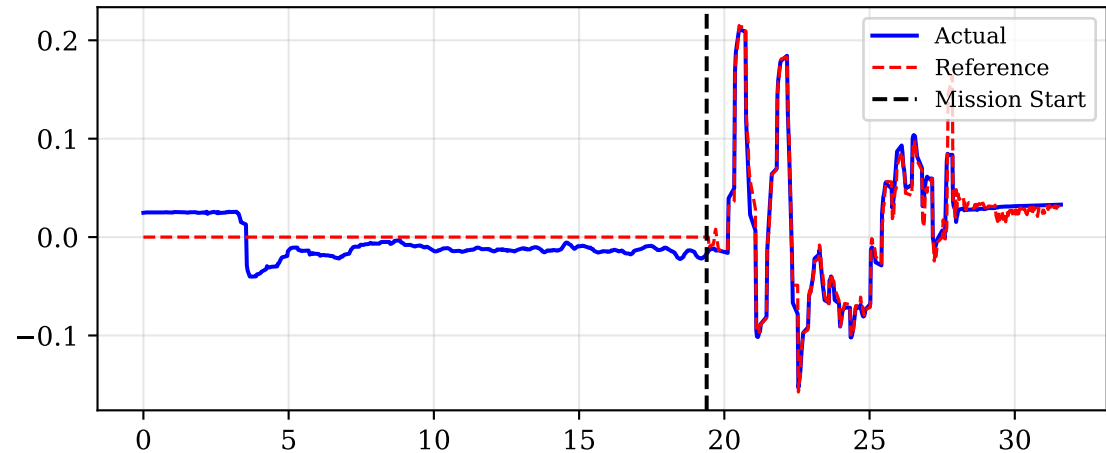
Pitch [rad]
