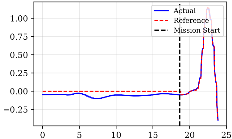
Position Y [m]
